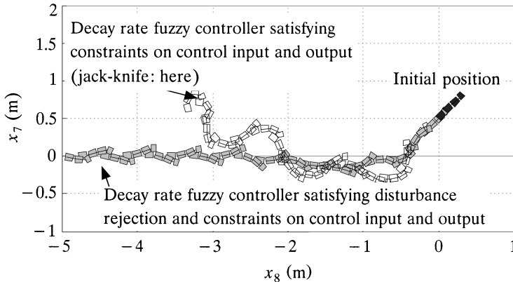
Fig. 8.5 Simulation result 3.
