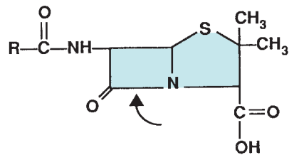
Penicillin nucleus
