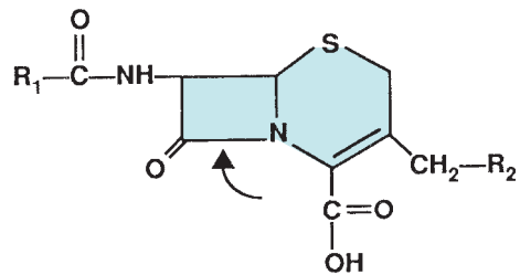
Cephalosporin nucleus
