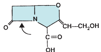
Clavulanic acid
