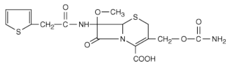
Cefoxitin (a cephamycin)
