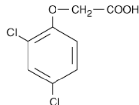
2,4-Dichlorophenoxyacetic acid (2,4-D)
