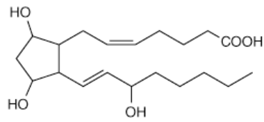
Prostaglandin F 2α (PGF 2α )
