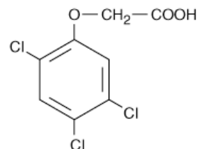
2,4,5-Trichlorophenoxyacetic acid (2,4,5-T)
