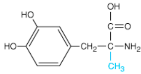
α-Methyldopa (α-methyl group in color)
