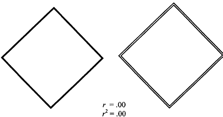
FIGURE 7.4 Uncorrelated variables.
