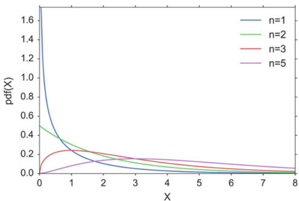
Fig. 6.15 Chi-square distribution
