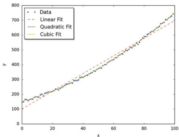
Fig. 11.6 A noisy, slightly quadratic data set, with a linear, a quadratic, and a cubic fit superposed. The quadratic and the cubic lines are almost exactly the same
