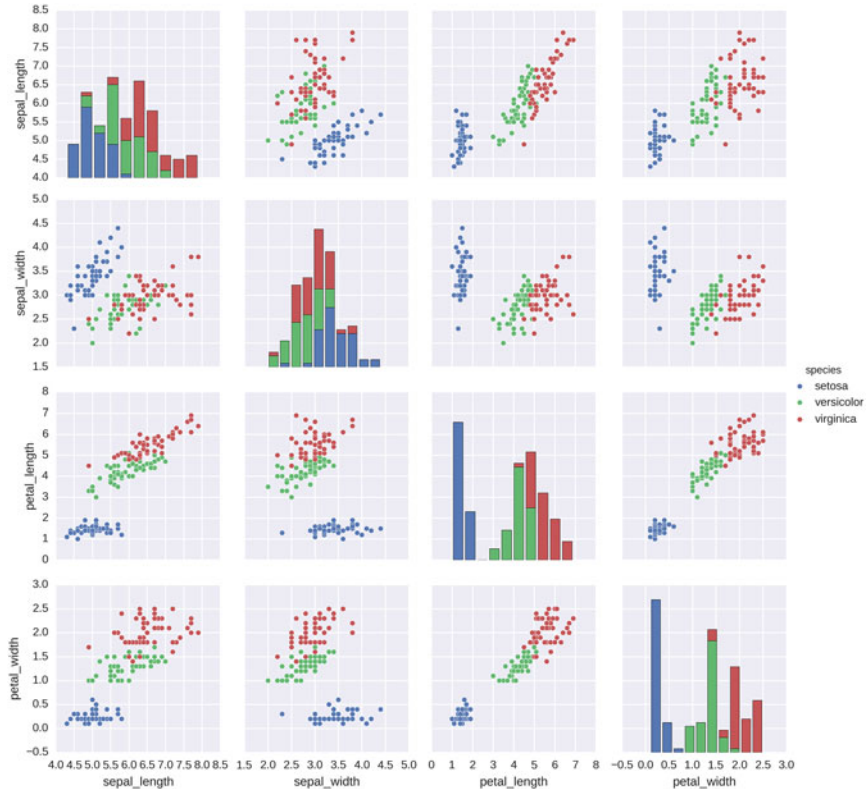
Fig. 12.1 Scatterplot matrix
