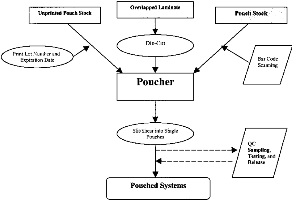
Figure 8 Schematic of transdermal pouching process.
