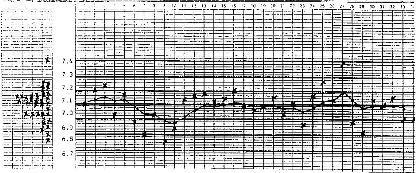
Figure 1 Control/performance chart for the sulfated ash test on a gasoline additive.
