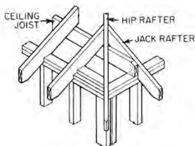
jack rafter
