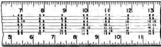
Essex board measure
