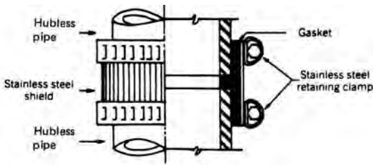
compression coupling
