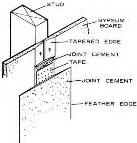
gypsum board: detail showing joint treatment
