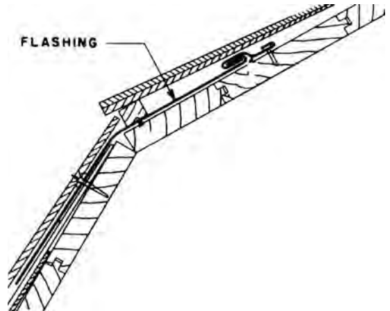
concealed flashing
