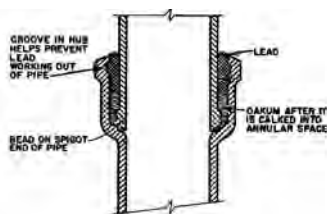
caulked joint
