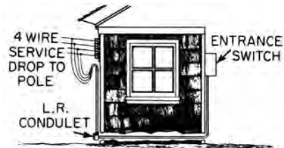
service entrance conductors
