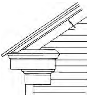
raking molding
