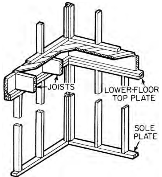
platform frame
