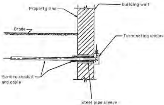
service connection
