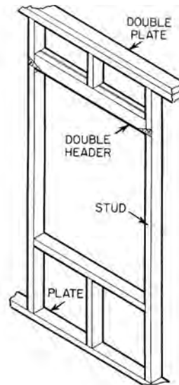
framing, 2 around an exterior wall opening
