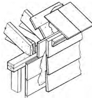
closed cornice
