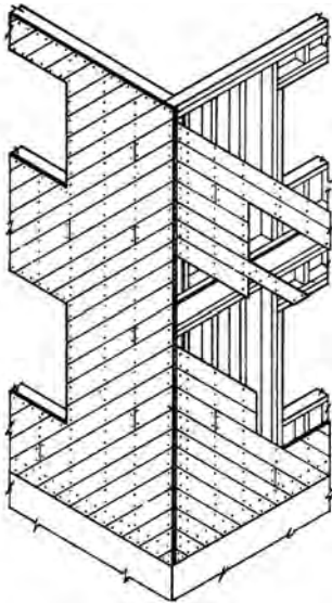
diagonal sheathing
