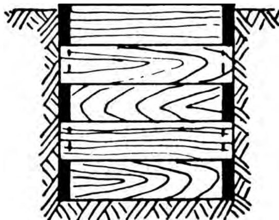
horizontal sheeting
