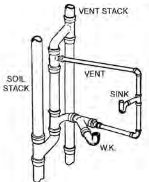
yoke vent, 2
