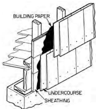
undercourse
