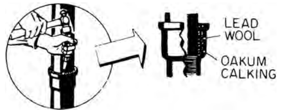
lead wool applied as caulking
