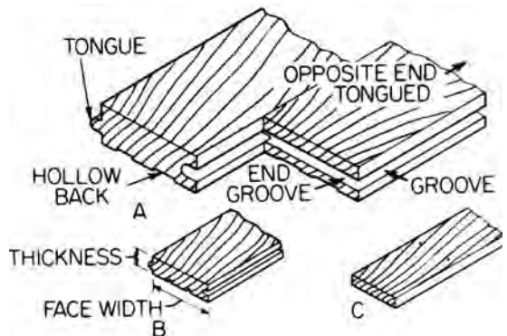
strip flooring: A, side- and end-matched; B, matched; C, square-edged
