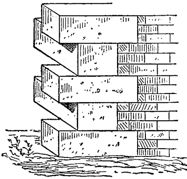
in-and-out bond
