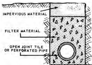
absorption trench
