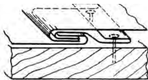
concealed cleat
