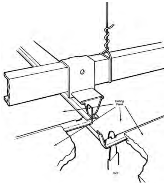
suspended ceiling
