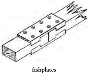
fishplates
