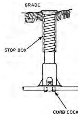
curb cock
