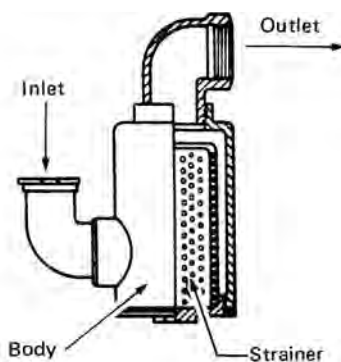
hair interceptor
