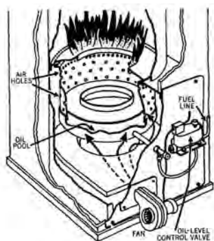
oil burner
