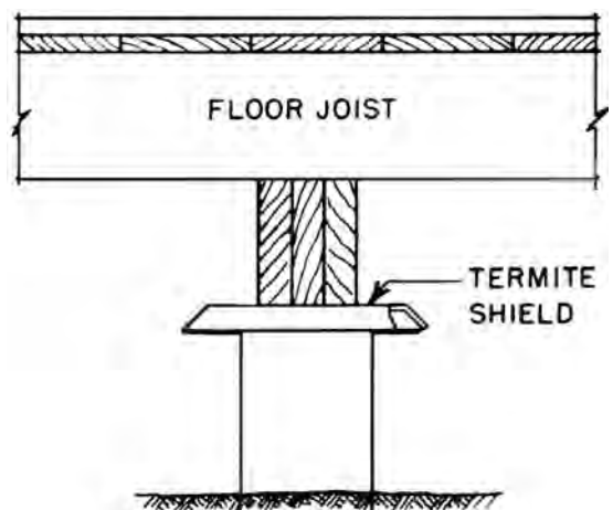
termite shield
