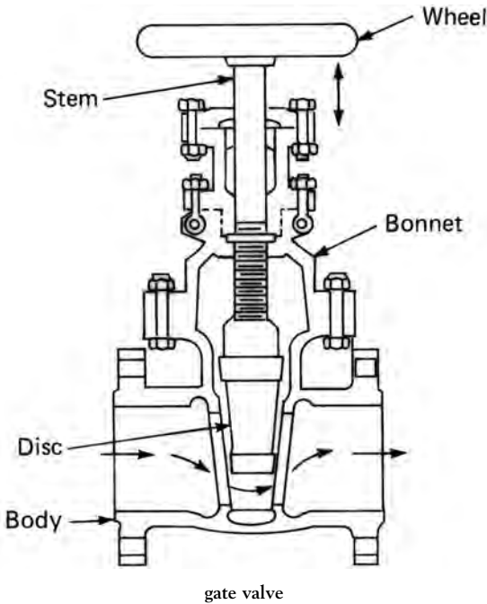
gate valve
