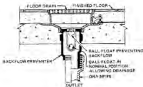
backwater valve: installation
