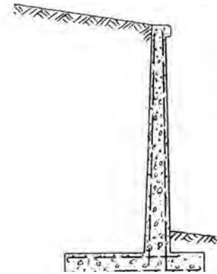
cantilever wall
