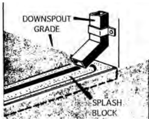
splash block
