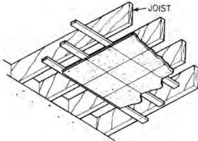
ceiling joists carrying an acoustical ceiling
