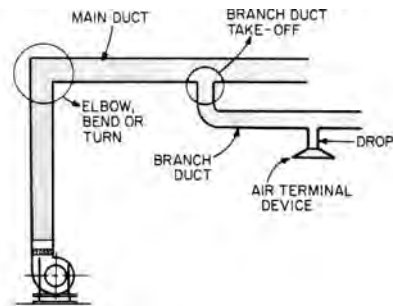
branch duct: installation
