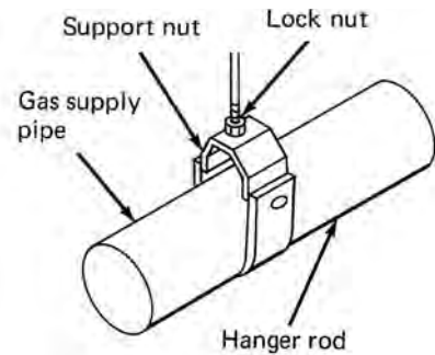
clevis hanger
