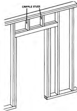
cripples, 1
