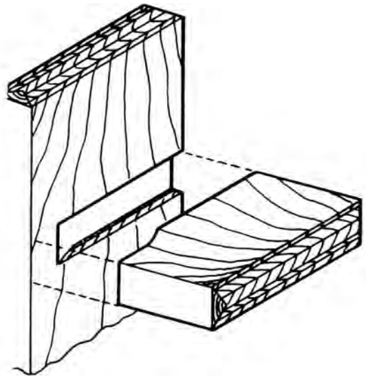
stopped dado
