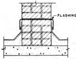
through-wall flashing
