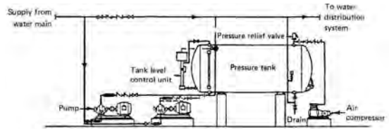
hydropneumatic tank system
