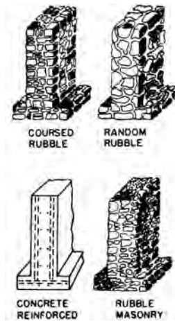
foundation walls
