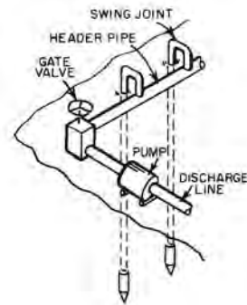
well-point system
