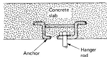
anchor, 9
