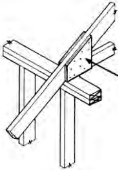
gusset
