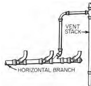
vent stack
