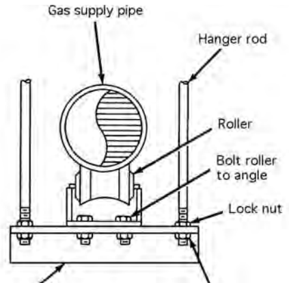
trapeze hanger with roller support
