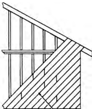
WALL SHEATHING NAILED ON DIAGONALLY
