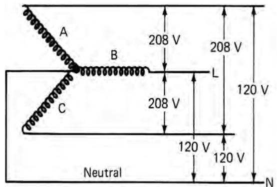
wye connection, 1
