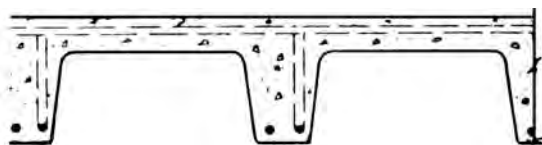
pan construction section view
