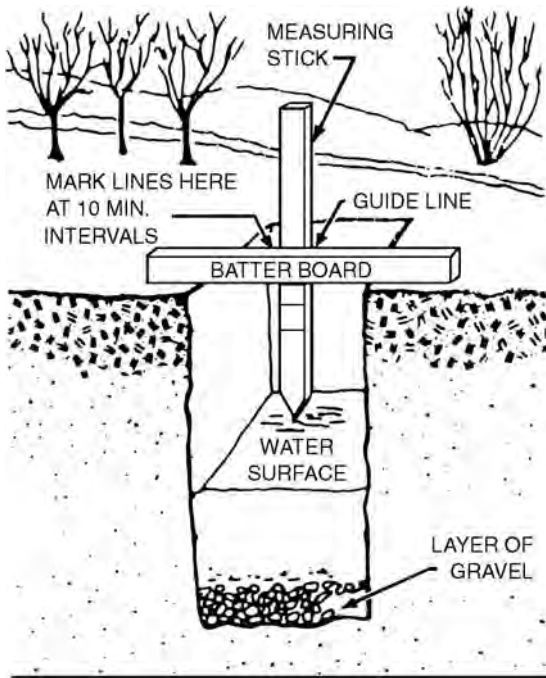
percolation test
