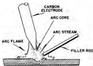
carbon-arc welding
