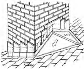
cricket
