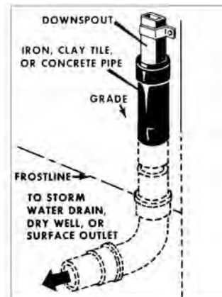
lower portion of a roof drainage system
