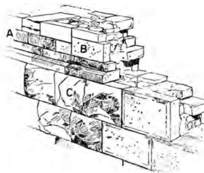
ashlar masonry: A, random-range quarry-faced ashlar; B, random-range dressed-faced ashlar; C, coursed quarry-faced ashlar; D, coursed dressed ashlar with margin draft; E, bonder in ashlar; f, rubble filling back of ashlar
