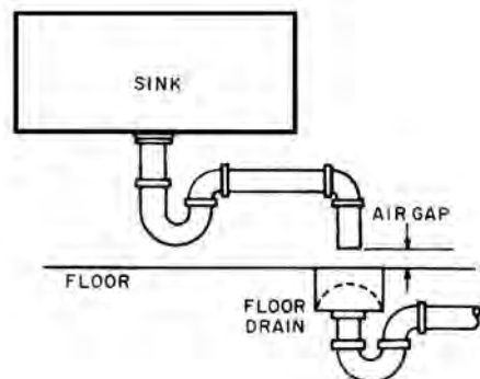
indirect waste pipe
