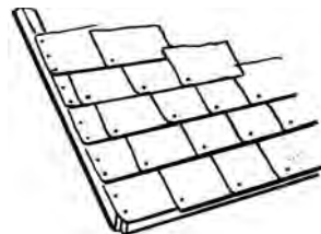
Dutch lap
