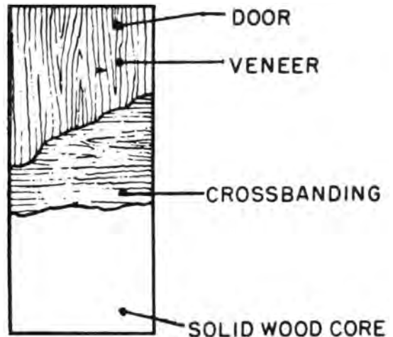
solid-core door
