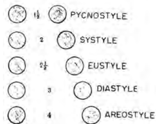
Diagram of intercolumniation
