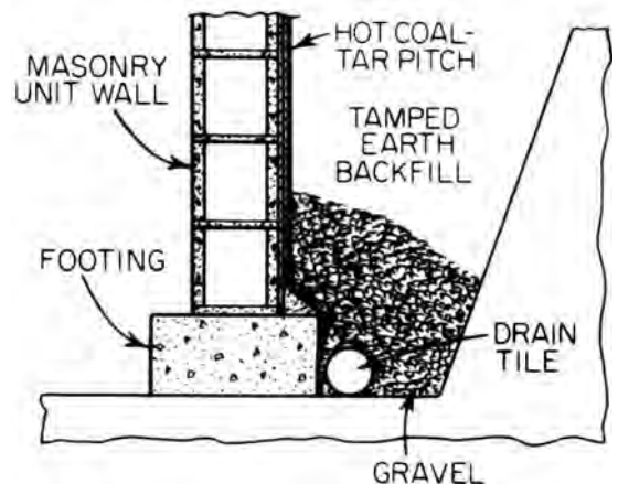
waterproofing applied to masonry wall units
