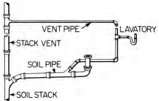
vent pipe, 1
