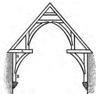
hammer beam: A
