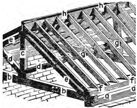
timbers in a roof: a, wall plate; b, tie beam; c, king post; d, strut; e, principal rafter; f, pole plate; g, purlin; h, ridgeboard
