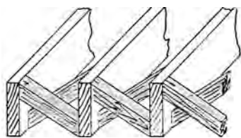
herringbone bridging
