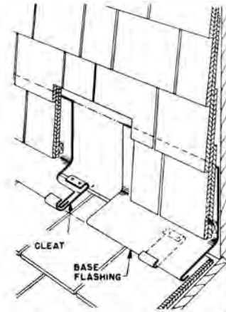
base flashing
