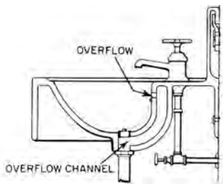
overflow, 1
