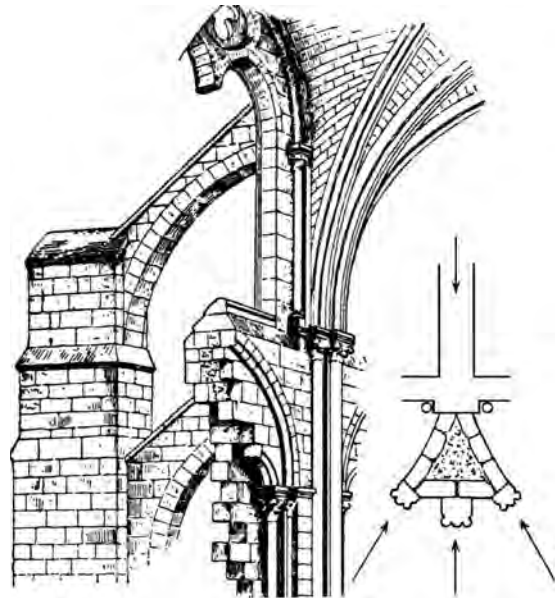
In medieval pointed vaulting, a section taken at the level of the head of the flying buttress; arrows indicate the directions of thrust
