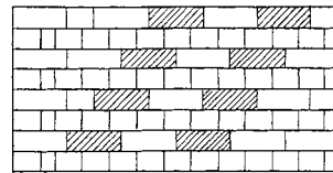
English cross bond
