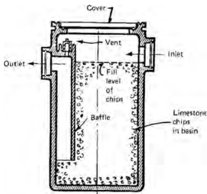
acid neutralizer
