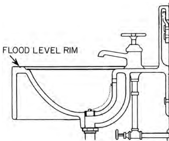
flood-level rim
