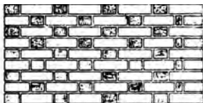
Flemish bond
