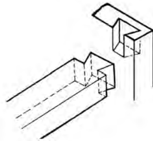
dovetail, 2
