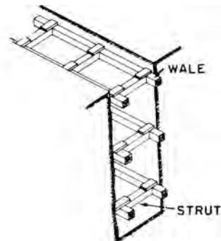
open sheeting
