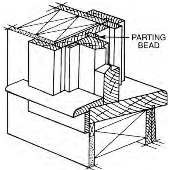
parting bead
