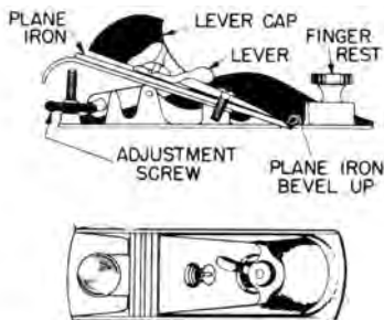
block plane
