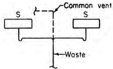
dual vent
