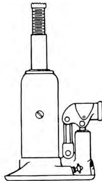
hydraulic jack
