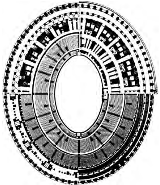
colosseum, 1 showing seating and plan at various levels
