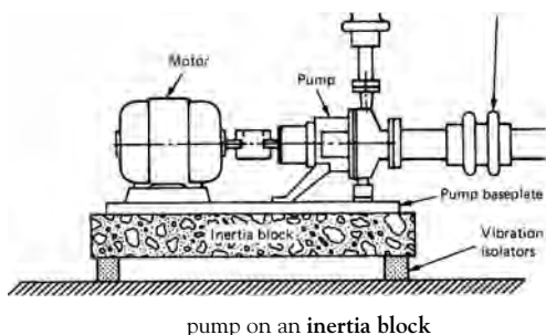
pump on an inertia block
