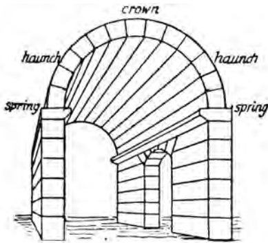
barrel vault
