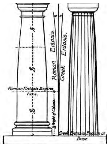
entasis: proportions are much exaggerated
