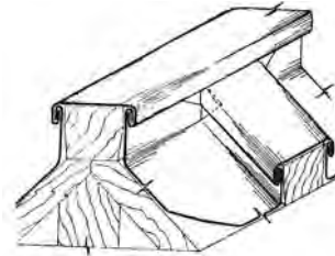
batten seam
