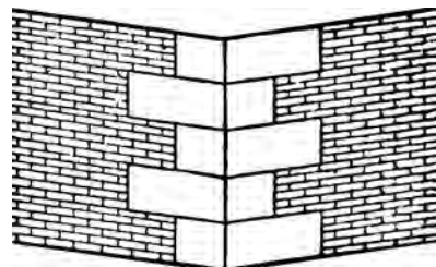
stone quoins set in brickwork
