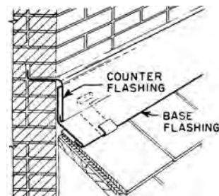
counterflashing
