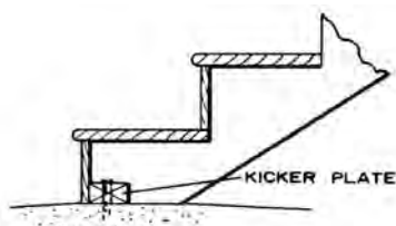
kicker plate
