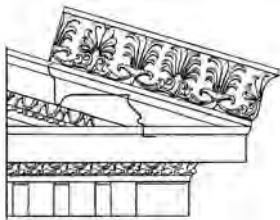
raking cornice
