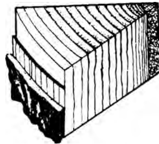
annual rings
