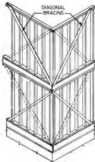
diagonal braces
