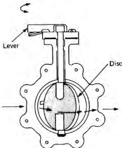
butterfly valve
