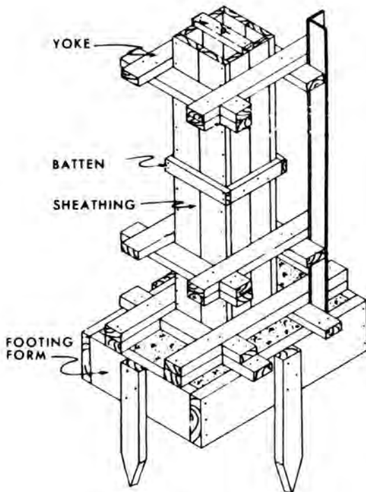
form for a concrete column
