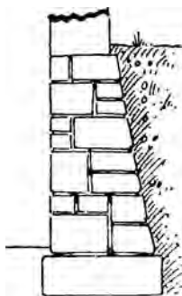
battered wall
