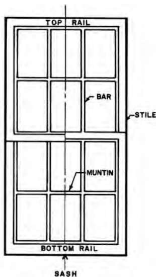
window sashes
