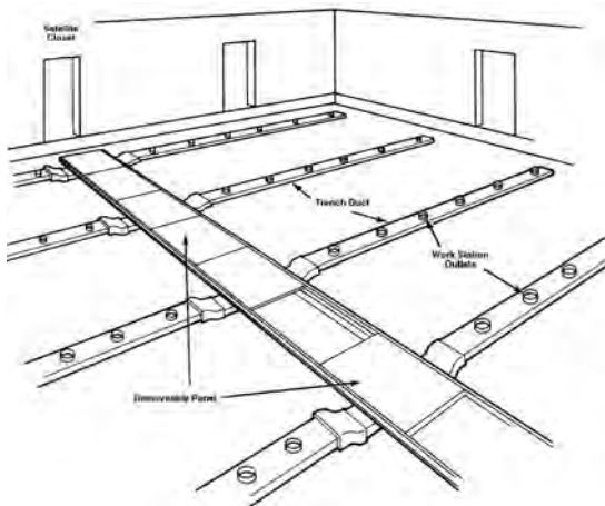
trench duct
