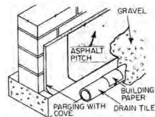
dampproofing, 3
