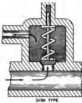
relief valves
