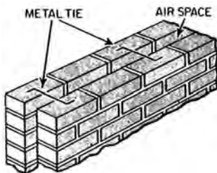
metal ties, 1
