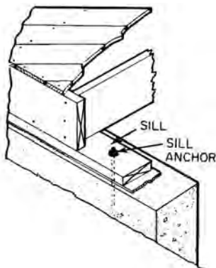
sill, 1
