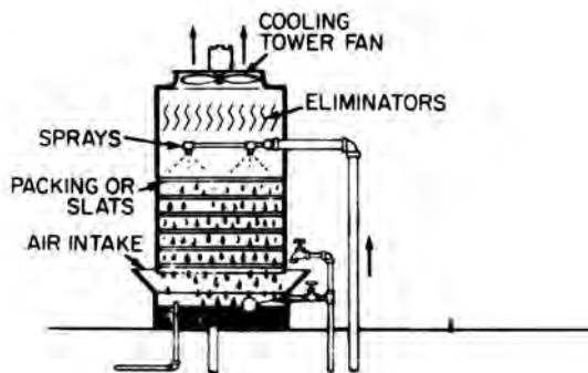
mechanical-draft water-cooling tower
