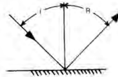
specular angle: angle of incidence, I , equals the angle of reflection, R
