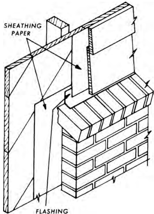
brick veneer
