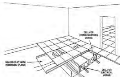
cellular floor
