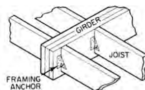
framing anchor
