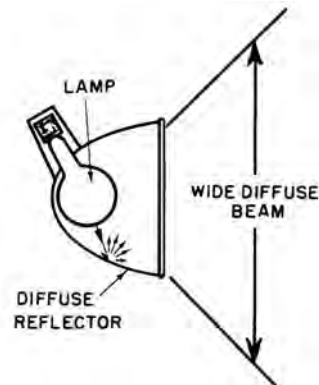
floodlight
