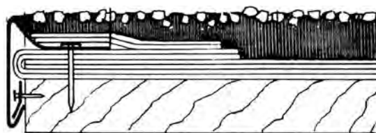
gravel stop
