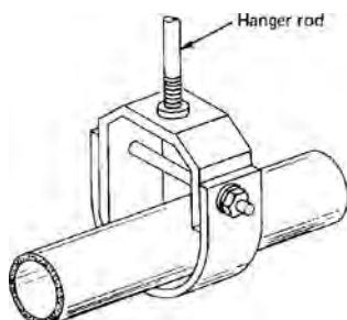
adjustable hanger
