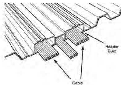
header duct
