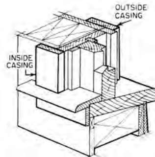
outside casing
