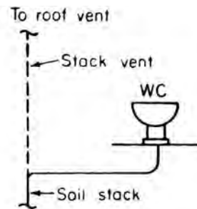
stack vent, 1
