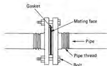
flanged joint
