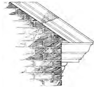
cornice return
