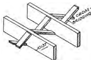
cross bridging
