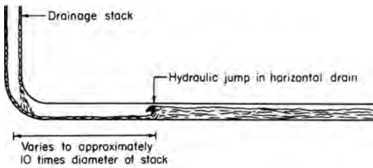
hydraulic jump
