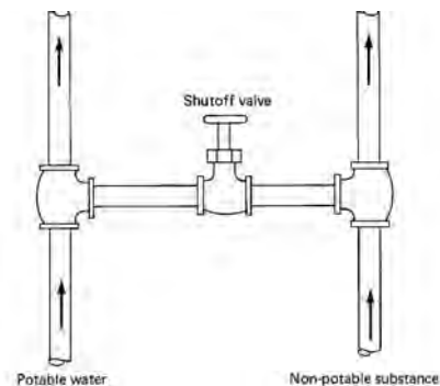
direct cross-connection
