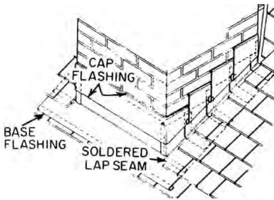
stepped flashing
