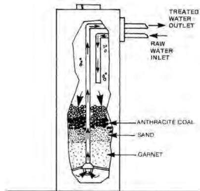
multimedia filter
