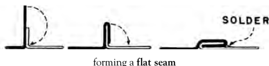
forming a flat seam
