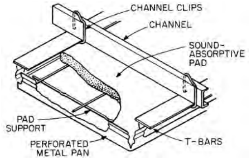
perforated metal pan
