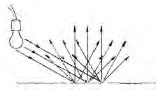
diffuse reflection
