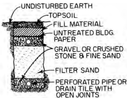
sand filter: plan
