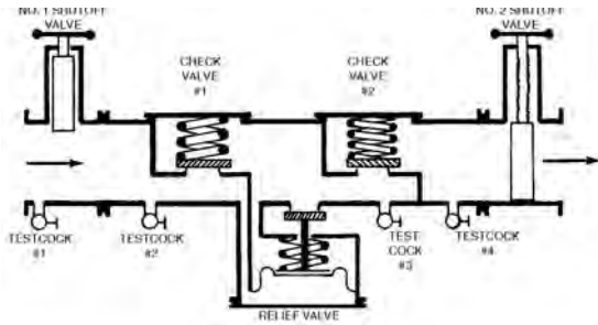
reduced-pressure-principle backflow preventer
