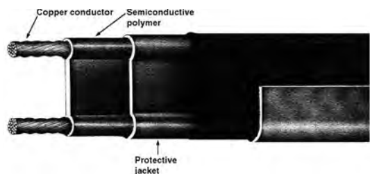
strip heater
