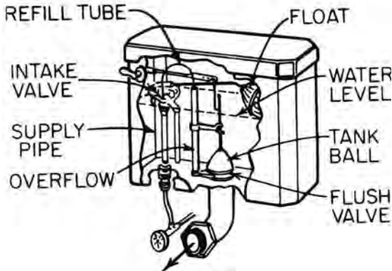
water closet flush tank
