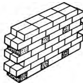
mixed garden wall bond
