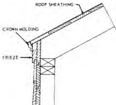
crown molding
