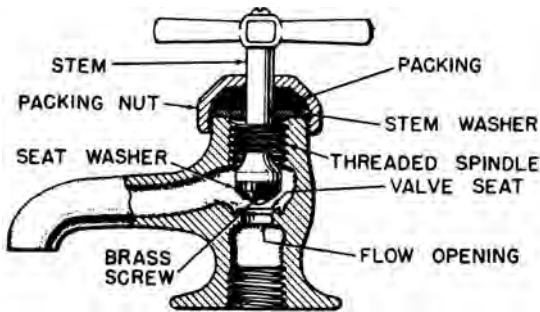
compression faucet
