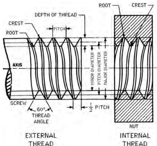
screw: nomenclature
