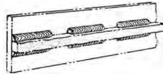
chain intermittent fillet weld
