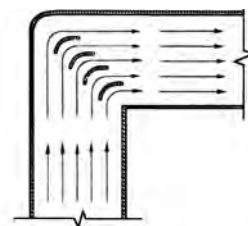
turning vanes
