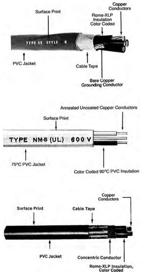
types of nonmetallic sheathed cable
