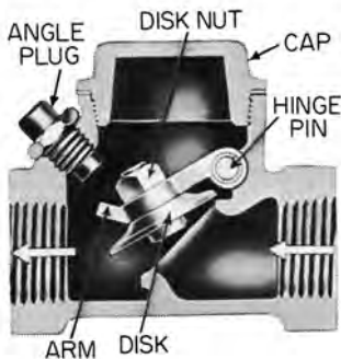
swing check valve
