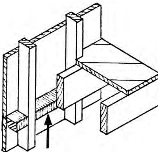
fire stop
