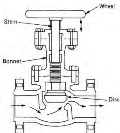
globe valve
