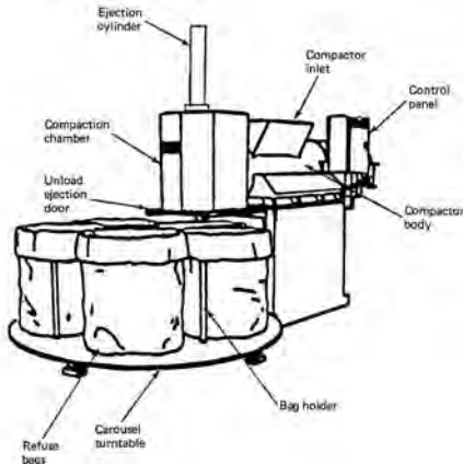
carousel packer
