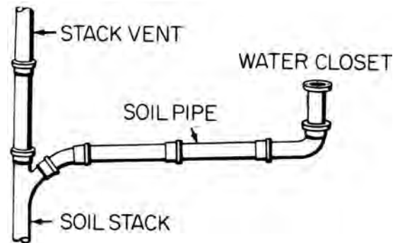
soil stack
