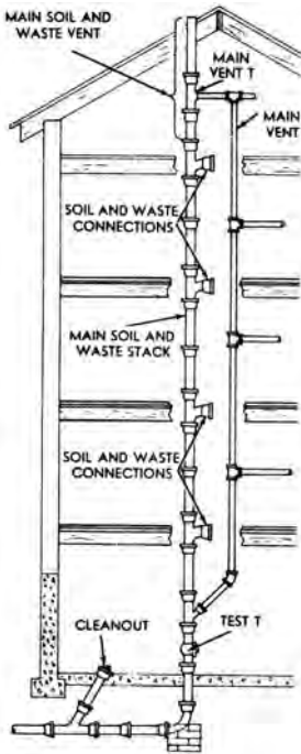
stack, 1: installation
