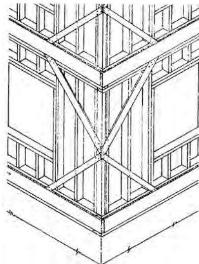
corner brace
