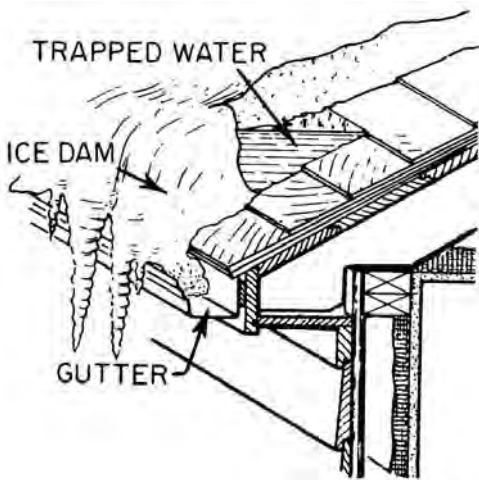
ice dam
