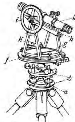
transit: a, tripod stand; b, leveling plates; f, vernier; g, compass; h, h', levels; i, vertical circle; k, telescope
