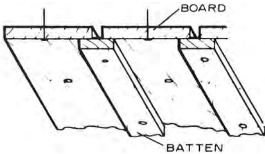
board and batten
