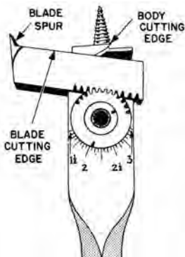
expansion bit
