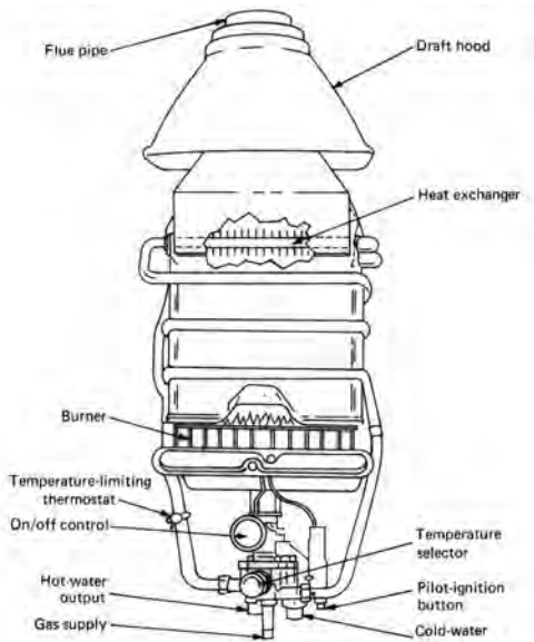
instantaneous-type water heater
