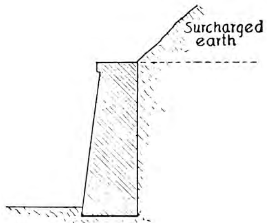
surcharged earth
