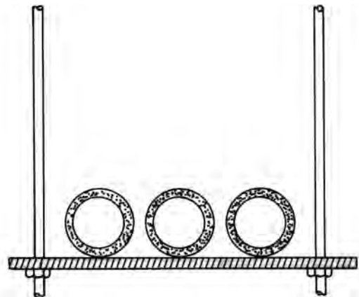
trapeze hanger
