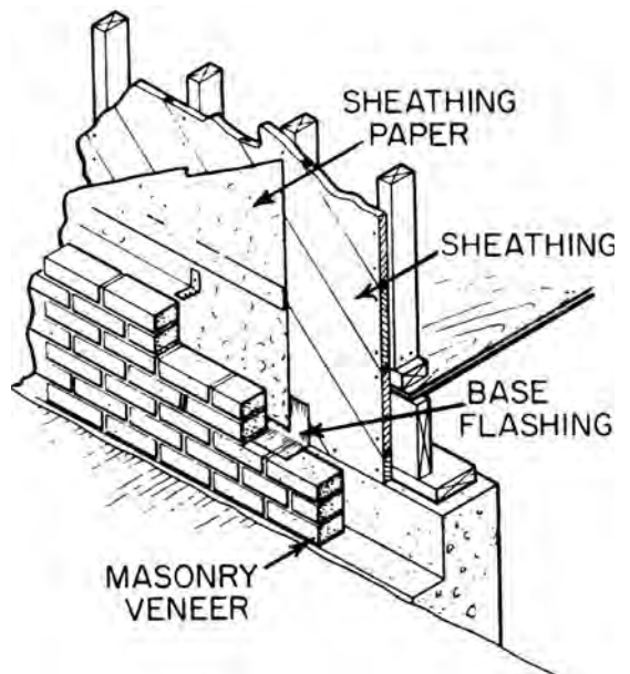
masonry veneer
