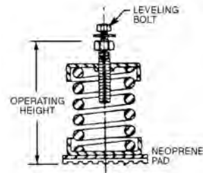
vibration isolator (coil-spring type)
