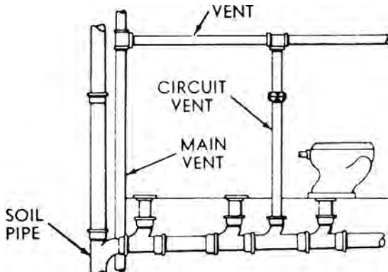
circuit vent
