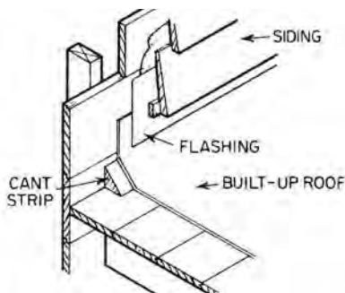
cant strip, 1
