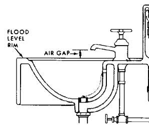
air gap, 2
