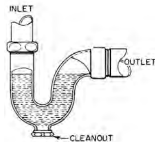
cleanout, 1: above: for cleaning pipe run; below: for a P-trap
