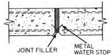
expansion joint, 1
