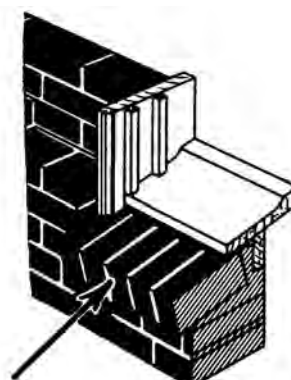
rowlock
