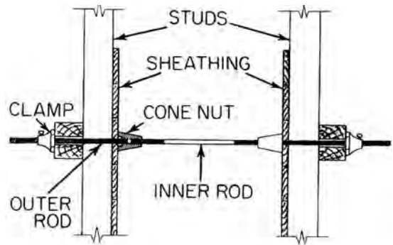
cone-nut tie
