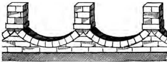
inverted arch
