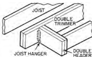
double header
