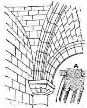
groined rib: A shows an enlarged section
