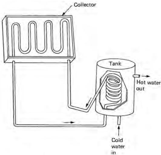
solar water heater
