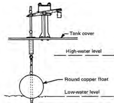
float switch in a water tank
