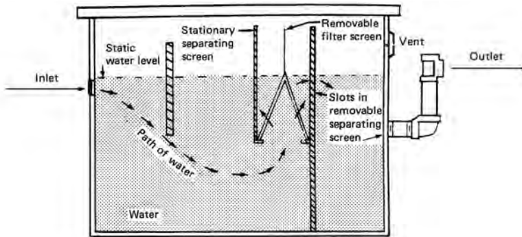
oil interceptor
