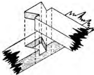
dovetail half-lap joint
