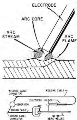
arc welding: above, with bare electrodes; below, circuit
