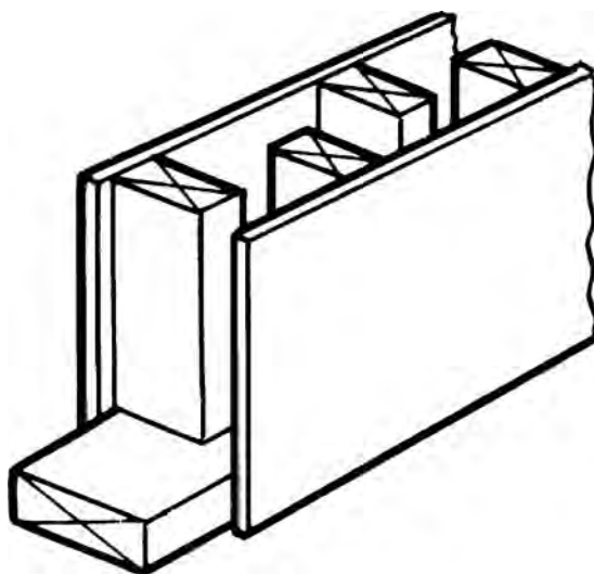
staggered-stud partition
