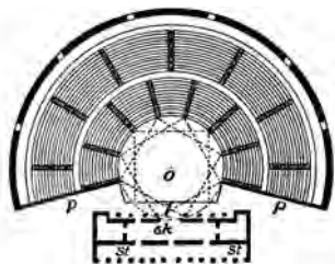
Greek theater: o, orchestra; l, logeion; p, parascenium; sk, skene; st, stoa
