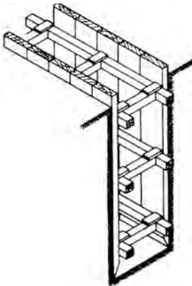
closed sheeting
