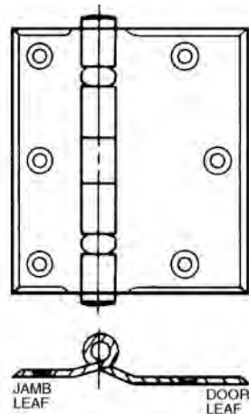
full-surface hinge
