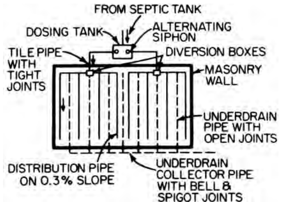
sand filter trench
