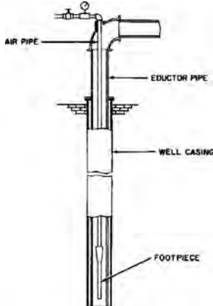
air-lift pump
