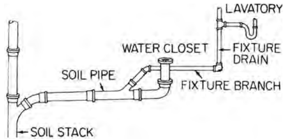
fixture branch
