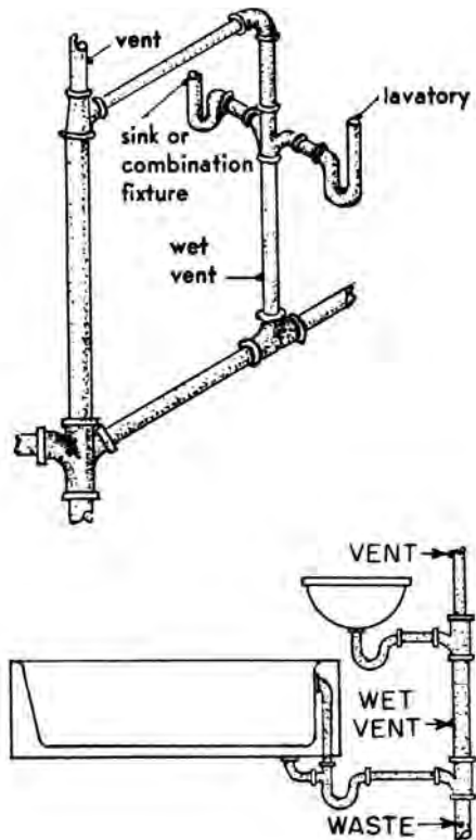
examples of wet vents
