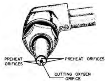
oxygen cutting tip
