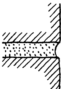
tooled joint
