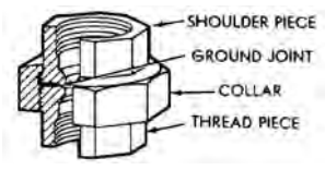
union
