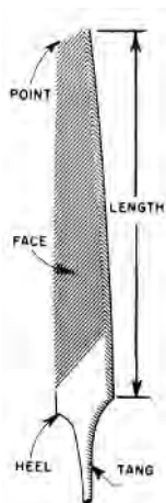
file
