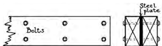
flitch beam
