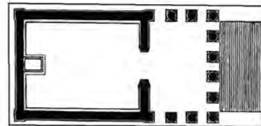
prostyle temple shown in plan
