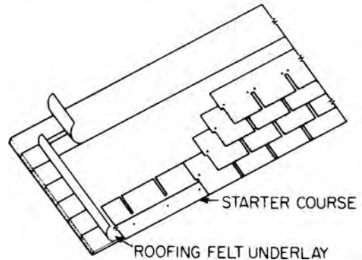
asphalt shingles: above, an asphalt shingle strip; below, installing asphalt shingles
