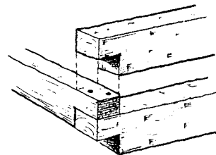
half-cut notch
