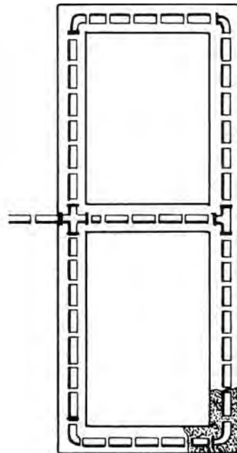
absorption field composed of absorption trenches Extent of coarse aggregate indicated by shaded area
