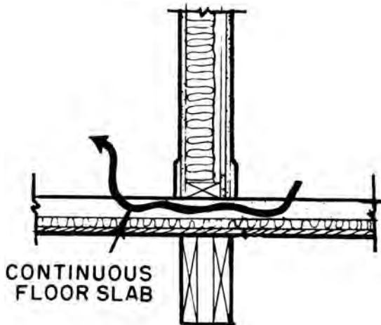
flanking transmission: path, indicated by arrow
