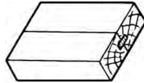
feather joint
