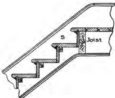
wall string S
