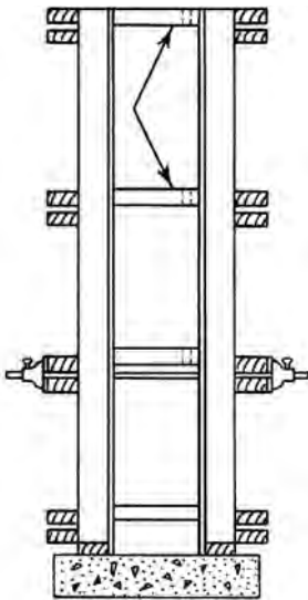
spreaders, 2 in a wall form
