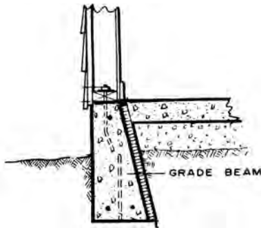
grade beam
