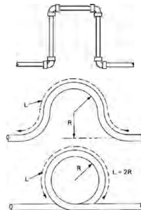
expansion bends
