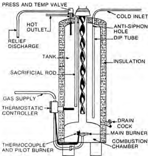
gas-fired water heater
