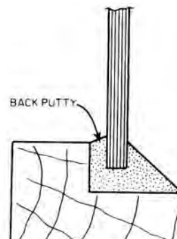
back putty
