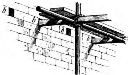
putlogs shown in putlog holes: b
