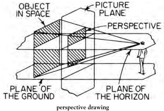
perspective drawing
