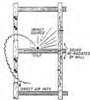
transmission of impact noise
