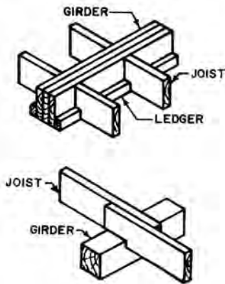
girders supporting floor joists
