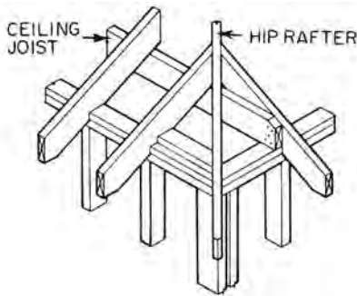
hip rafter
