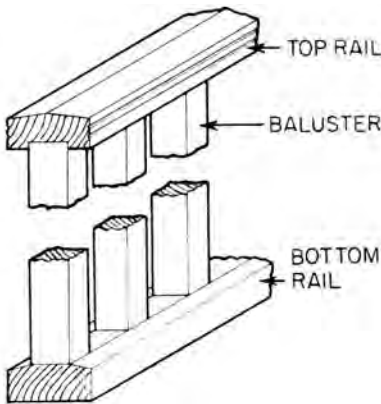
balustrade
