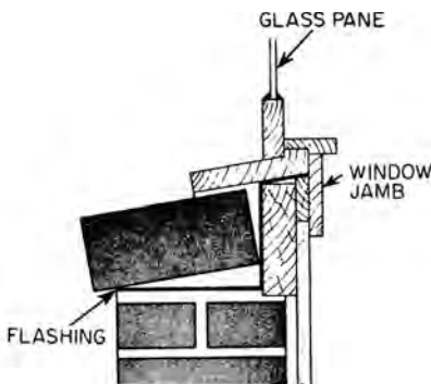
flashing
