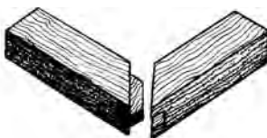
miter joint with spline
