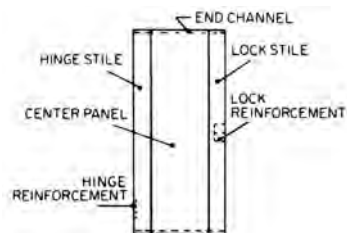
hollow-metal door
