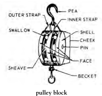
pulley block
