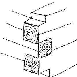
square notches
