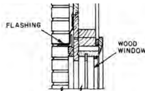
head flashing
