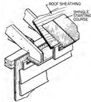
starting course
