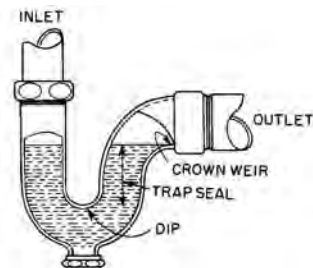
trap seal
