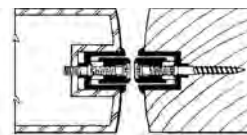
mortised astragal
