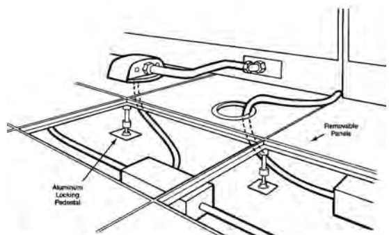
raised floor: cutaway detail of a plate adjacent to the wall
