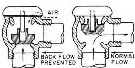
vacuum breaker
