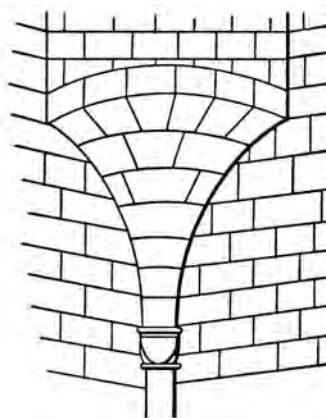
pendentive, 2
