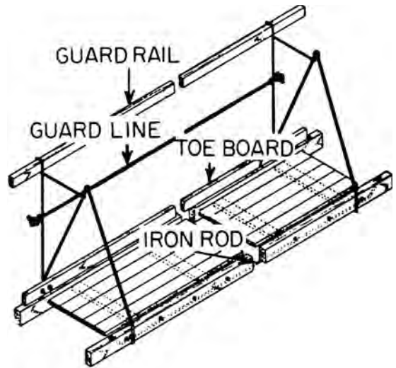
swinging scaffold
