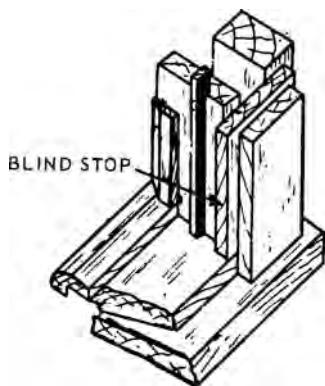
blind stop
