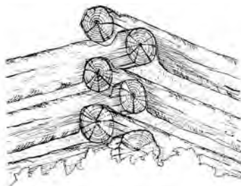
saddle notches
