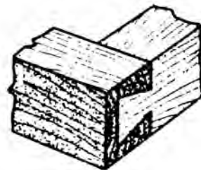
secret dovetail
