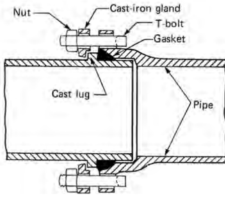
typical mechanical joint
