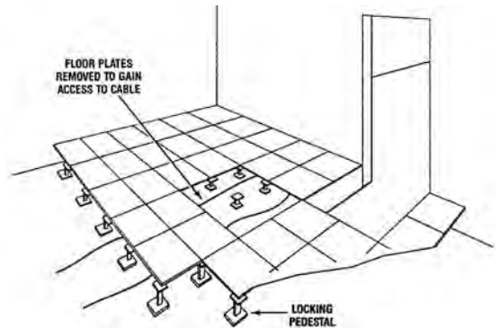
raised floor showing floor plates on pedestals
