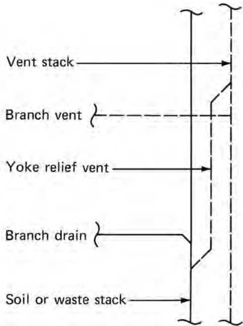
yoke relief vent, 2
