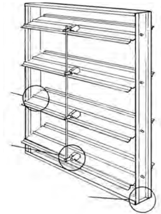
parallel-blade damper
