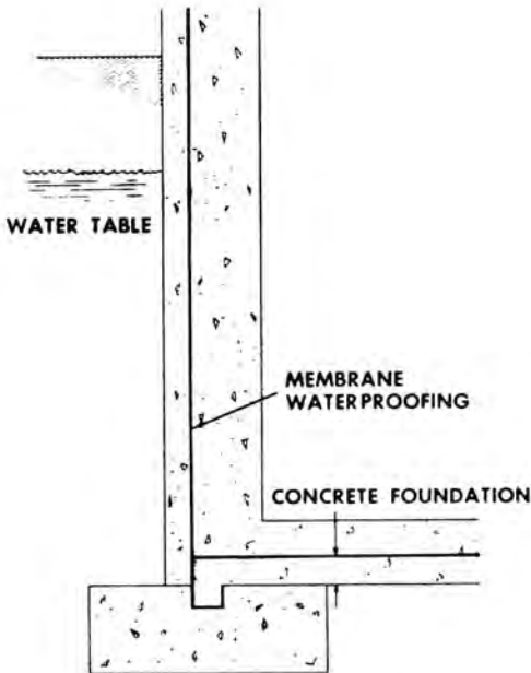
membrane waterproofing
