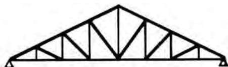
Howe truss
