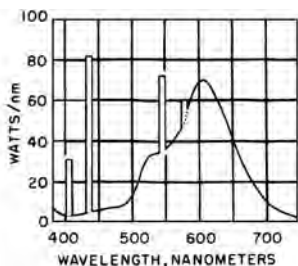
spectral power distribution: deluxe warm white fluorescent lamp
