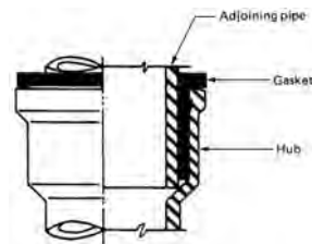
gasketed joint
