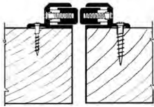
surface-mounted astragal
