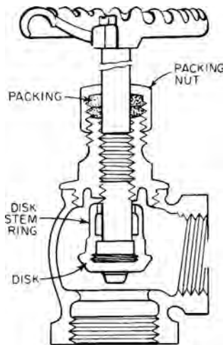
angle valve
