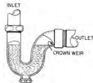
crown weir
