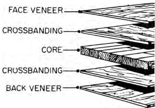
crossbanding, 1
