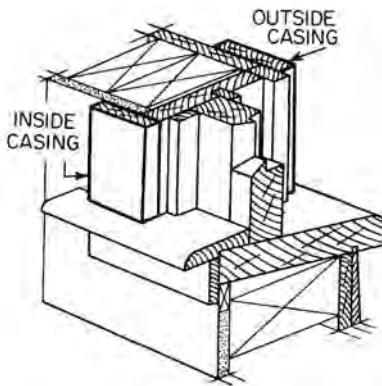
inside casing
