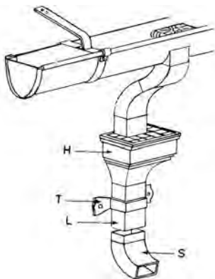
leader: L; leader head, H; leader shoe, S; leader strap, T
