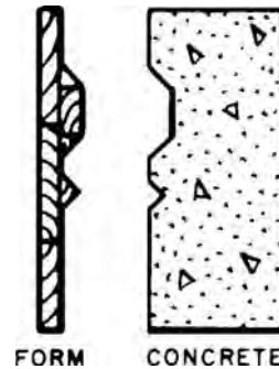
mold for finishing concrete
