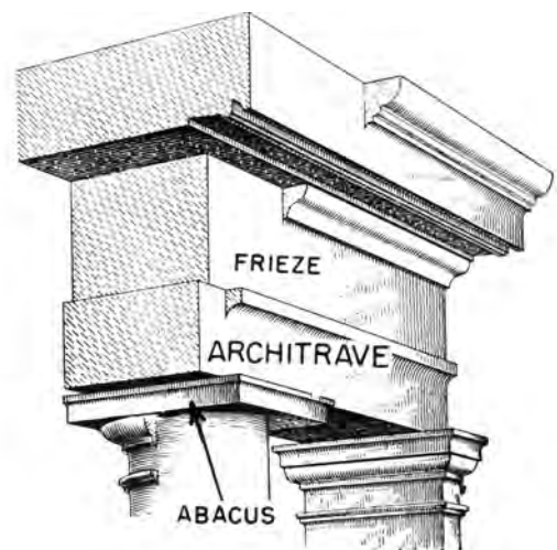
architrave
