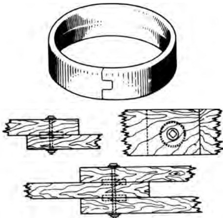
split-ring connector showing a typical joint
