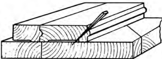
toenailing wood-strip flooring
