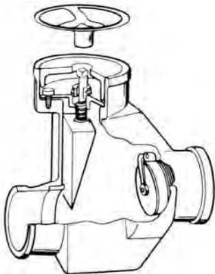
backwater valve
