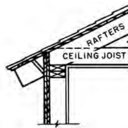
open cornice
