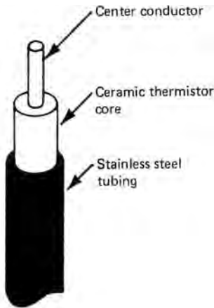
linear-type heat detector
