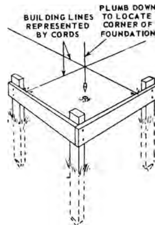
batter boards
