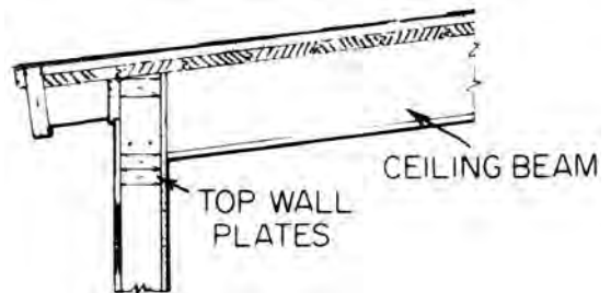
wall plate, 1
