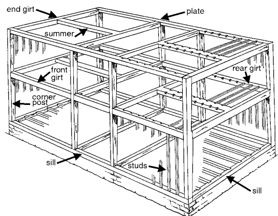
timber-framed house with terminology for many structural members
