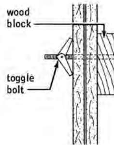
toggle bolts
