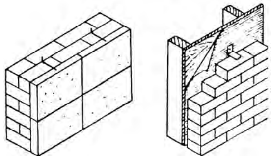
veneered construction (two types)
