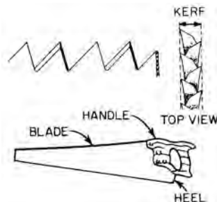
crosscut saw with details showing saw teeth
