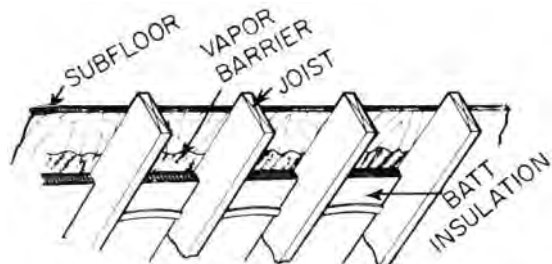
batt insulation installed on underside of subfloor
