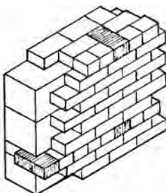
masonry ties, 1
