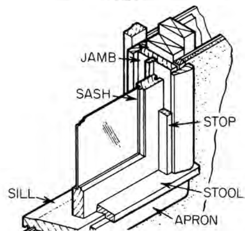
window: details
