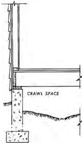
crawl space, 2
