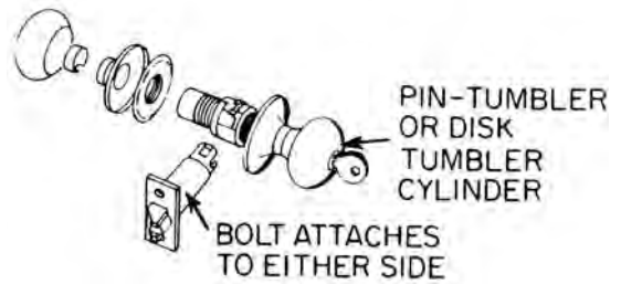
cylindrical lock
