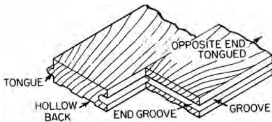
matchboards
