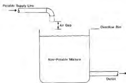
air gap, 1
