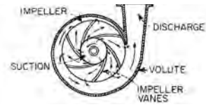
centrifugal pump
