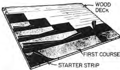
Installing asphalt prepared roofing
