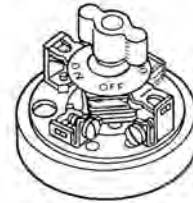
snap switch with cover removed
