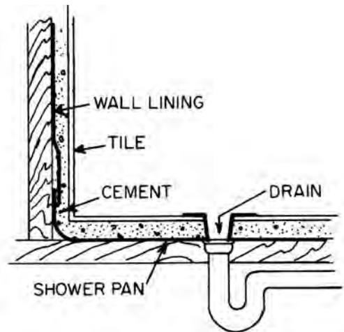
shower pan
