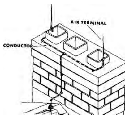
air terminal
