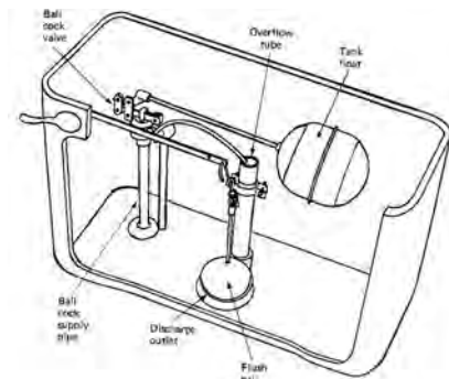
flush tank
