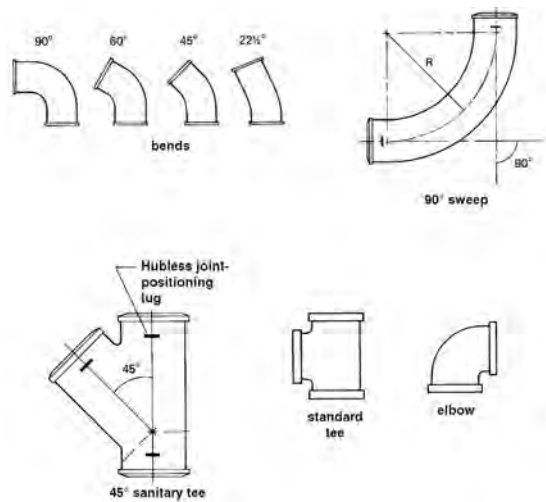
fittings, 1
