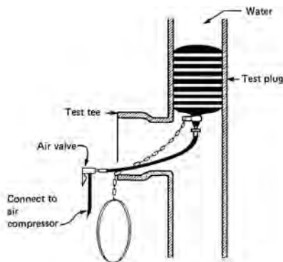
test plug
