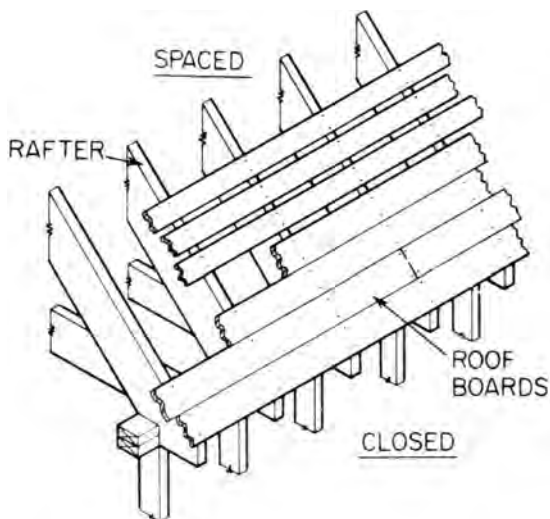
board sheathing
