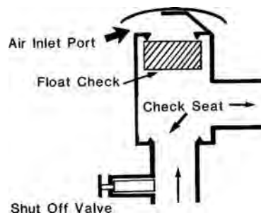
atmospheric-type vacuum breaker
