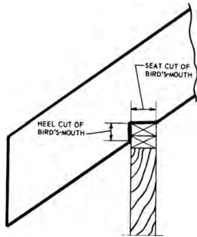
bird's-mouth, 1
