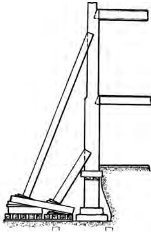
shoring
