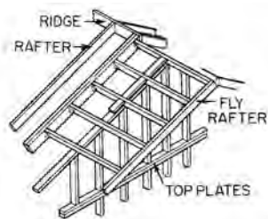
fly rafter
