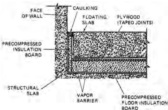
concrete floating floor construction of fiberglass insulation board
