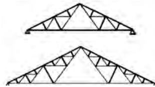
Fink truss, above; long-span Fink truss, below
