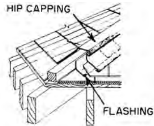
hip capping
