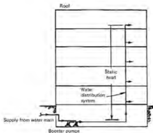
simplified diagram of a water distributor system employing a booster pump
