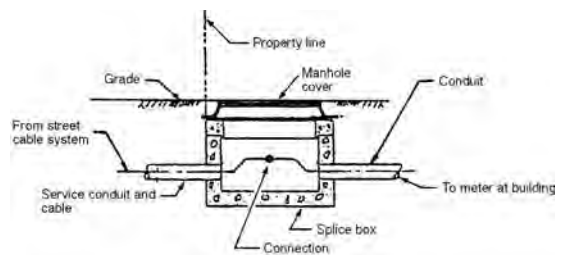
splice box
