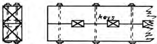
keyed beam
