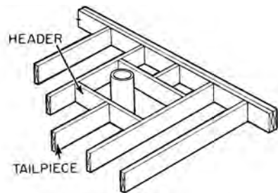
tailpiece, 1
