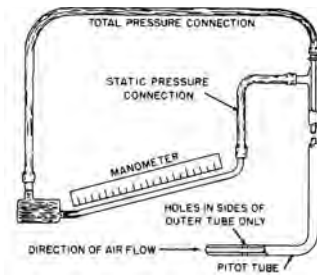
pitot tube
