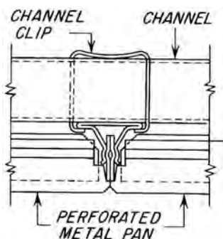
channel clip, 1
