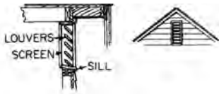
outlet ventilator
