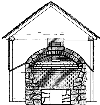
bake oven (longitudinal section)
