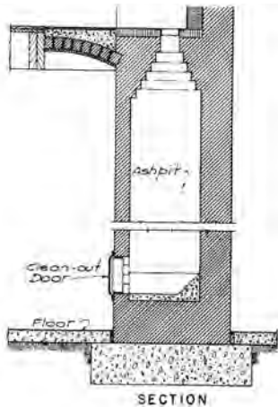
ashpit
