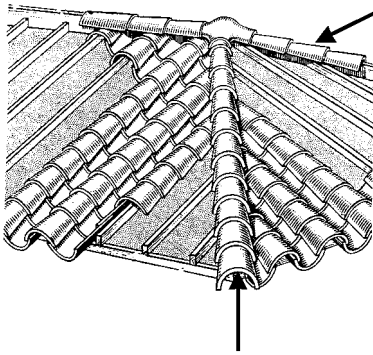
ridge tile
