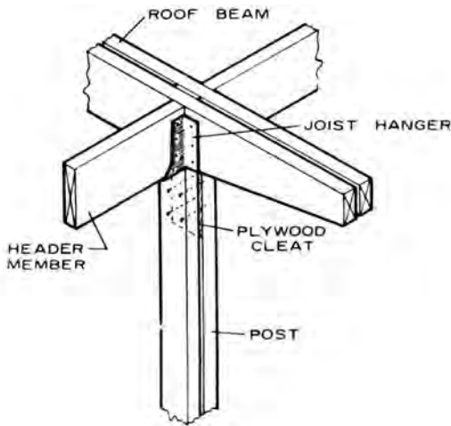
post-and-beam framing
