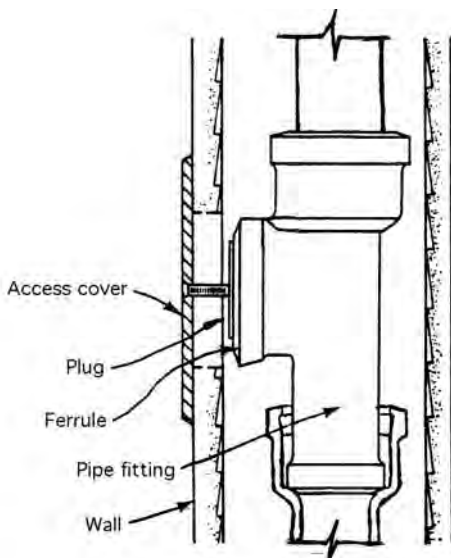
wall cleanout
