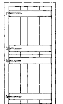
Dutch door: exterior elevation; interior elevation
