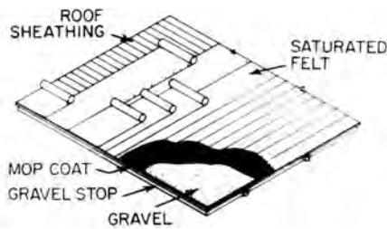
built-up roofing
