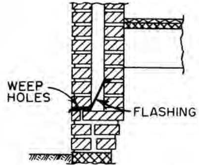
cavity flashing
