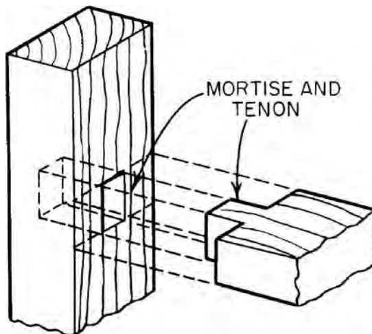
mortise-and-tenon joint
