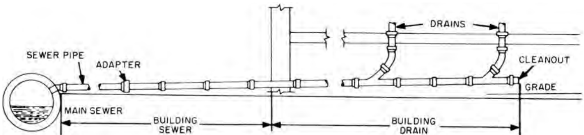
building drain
