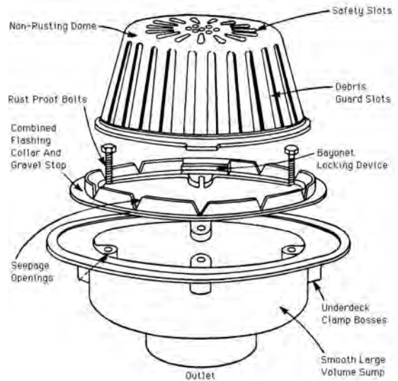
typical roof drain
