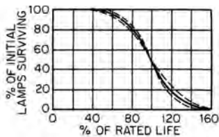
% rated lamp life vs. % of initial lamps which survive A life expectancy curve for incandescent lamps
