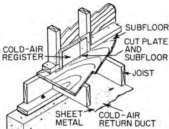
cold-air return
