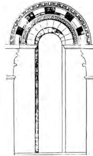
An arch of two orders, 3, each having its carved hood molding
