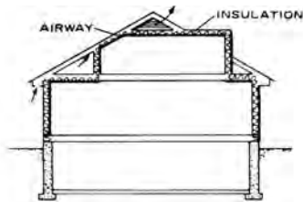
airway
