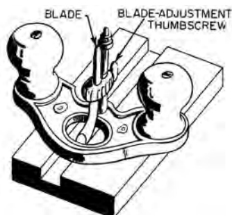
router plane
