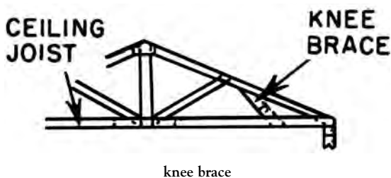
knee brace
