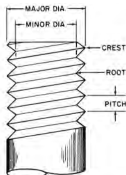
thread: terminology
