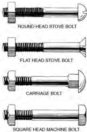
bolts, 1
