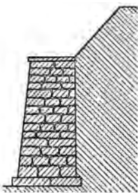
retaining wall
