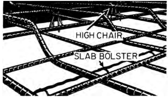
reinforcement, 1
