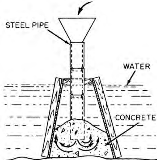
tremie used in placing concrete under water
