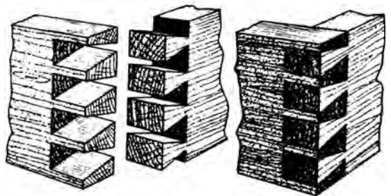
common dovetail
