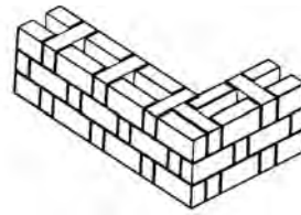
rat-trap bond
