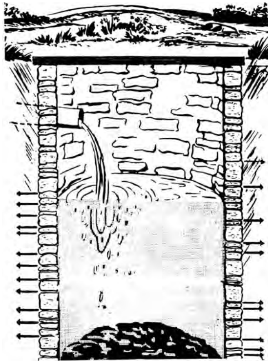
leaching cesspool
