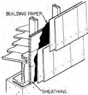
double course
