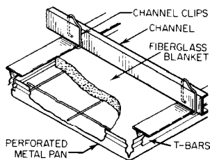
acoustical ceiling system
