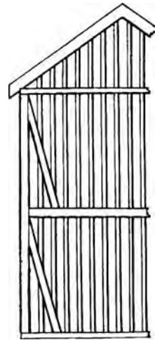
braced frame, 1
