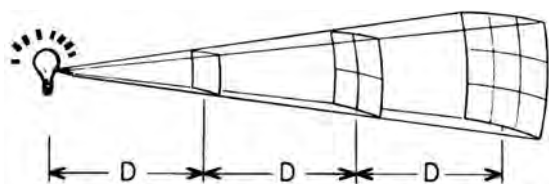
inverse-square law
