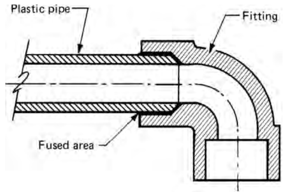
heat-fusion joint
