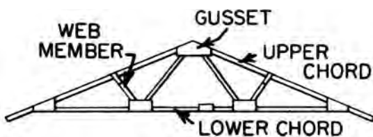
W-truss
