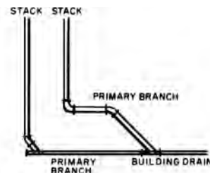
primary branches, 1
