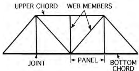
truss
