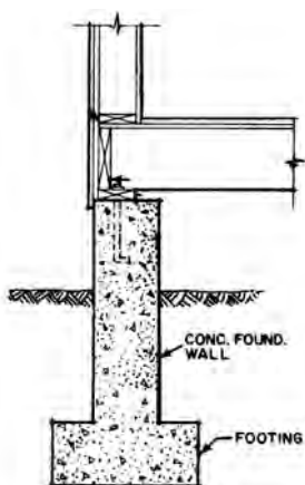
footing
