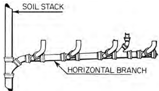
horizontal branch
