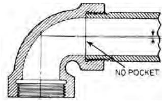
drainage fitting
