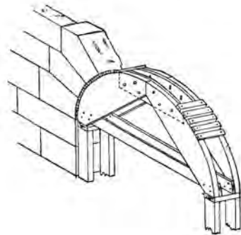
centering: two types
