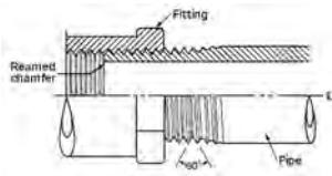
threaded joint
