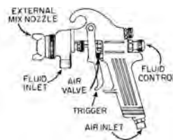
spray gun
