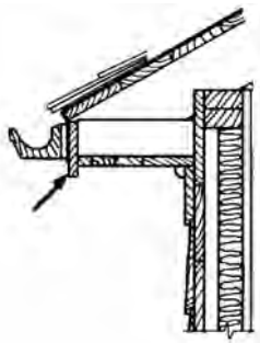
eaves fascia
