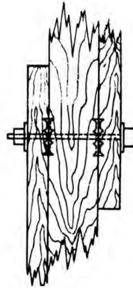
spike grid timber connector; joint employing two timber connectors is shown below
