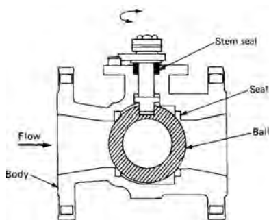
ball valve
