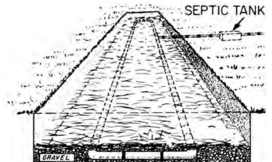
seepage bed
