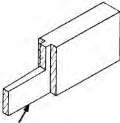
haunched tenon
