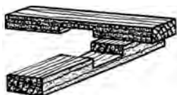
crosslap joint
