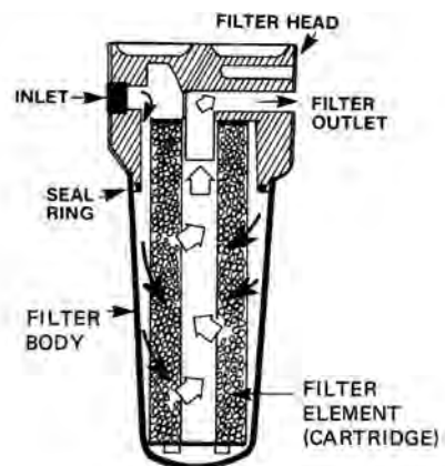
cartridge-type filter
