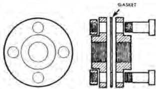
flange union
