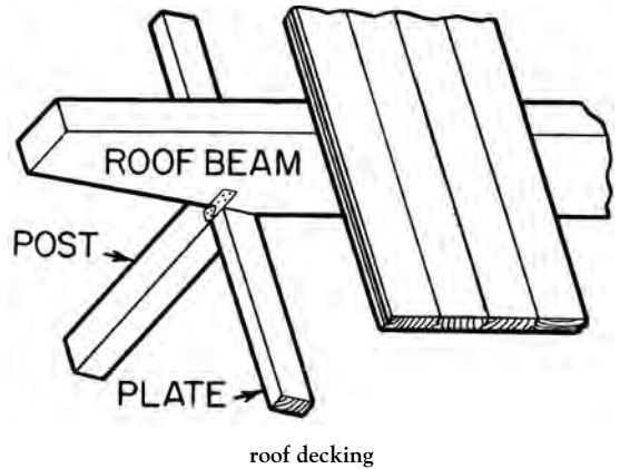
roof decking
