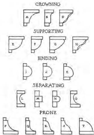
sections of classical moldings: A, cavetto; B, congé; D, cyma recta; E, quarter round; F, ovolo; G, echinus; H, cyma reversa; I, half round; J, torus; K, thumb; L, half hollow; M, fillet; N, bead; O, scotia; P, cavetto; Q, scape; R, cyma recta; S, cyma reversa; T, ovolo
