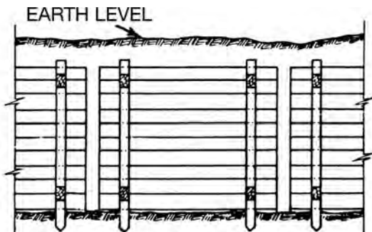
horizontal sheeting
