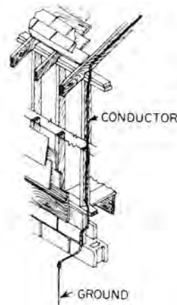
lightning conductor
