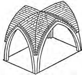
Gothic architecture: vault construction
