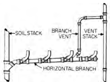
branch vent, 1
