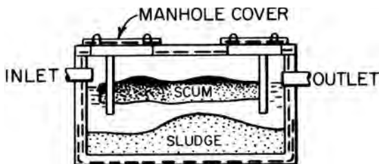
household septic tank, cross section
