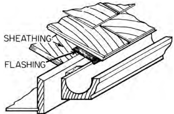
wood gutter
