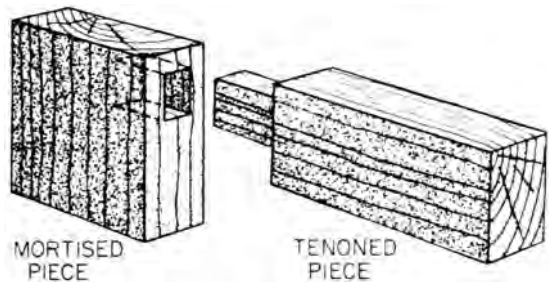
blind-mortise-and-tenon joint
