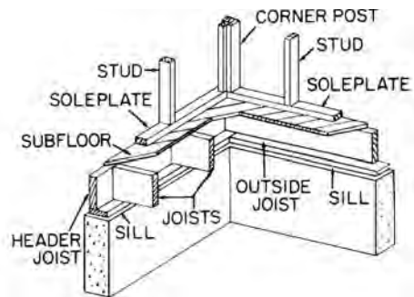
box sill
