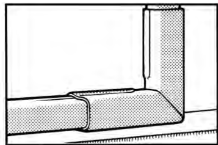
surface metal raceway: 90° bend
