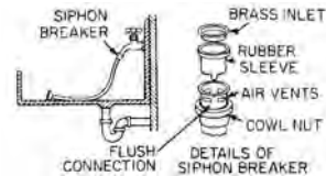
backflow preventer for a hose connection
