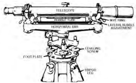
wye level
