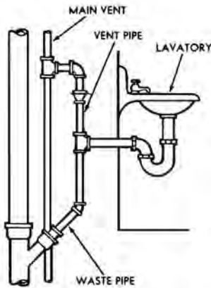
individual vent
