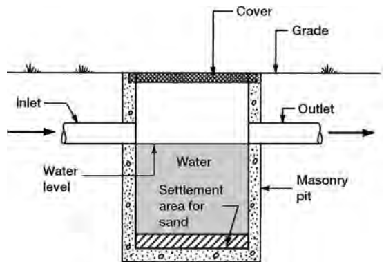
sand interceptor
