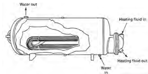
storage-type water heater
