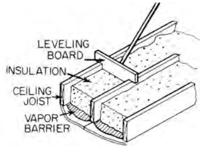
fill insulation being placed between joists
