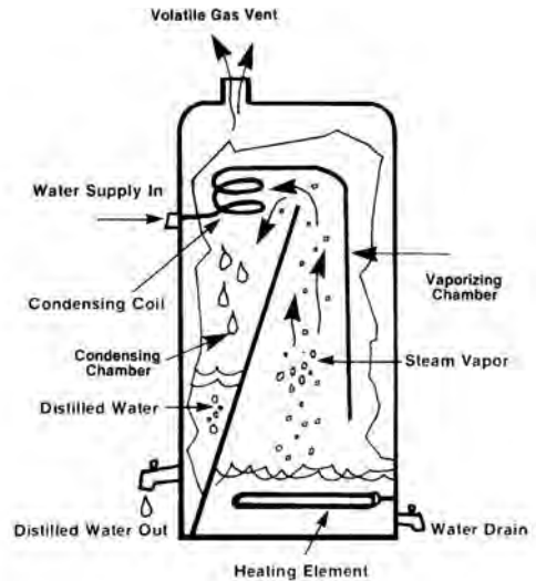
the process of distillation
