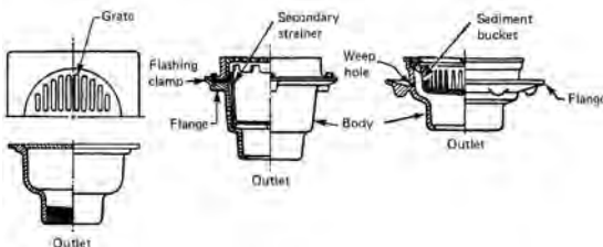
typical floor drains
