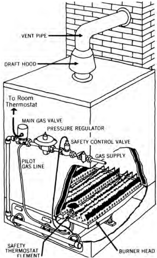
gas furnace
