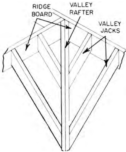
valley jack and valley rafter
