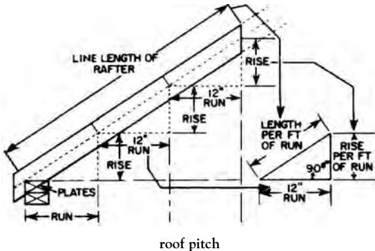
roof pitch
