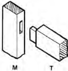
stub mortise (M); stub tenon (T)
