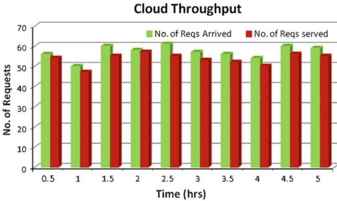
Fig. 3 Cloud throughput
