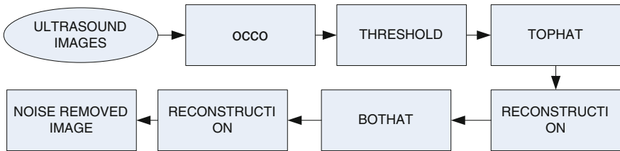
Fig. 3 Preprocessing steps
