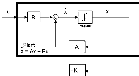
Fig. 3 Quadratic optimal regulator system
