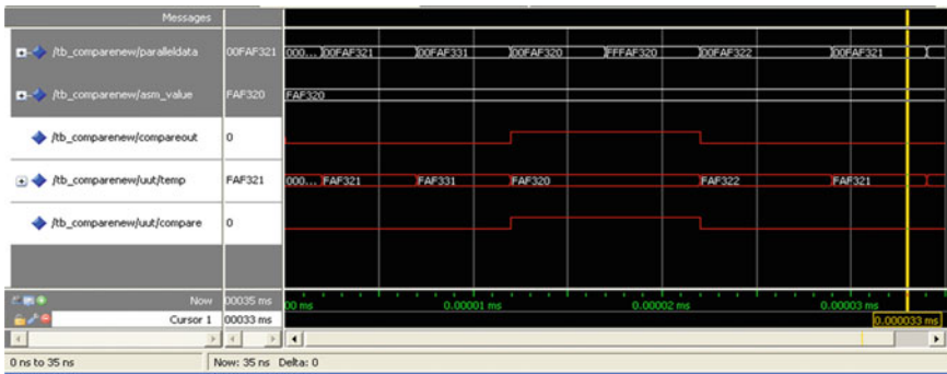
Fig. 13 ASM comparator
