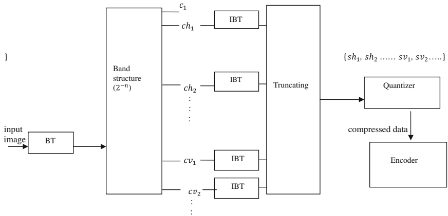
Fig. 3 Block diagram of transform coding system for compressed data
