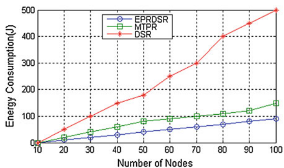
Fig. 5 Routing energy consumption comparison for varying node number
