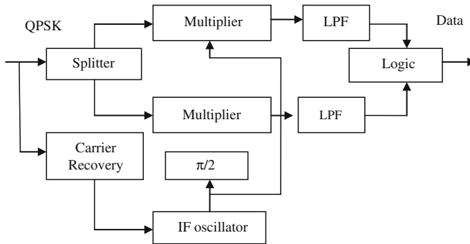
Fig. 2 QPSK demodulator
