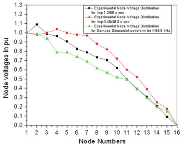
Fig. 9 Experimental node voltage distribution for impulses of 0.46/48.3 and 1.2/50 \mu\text{s} and damped sinusoidal waveform ( f = 65.8 \text{ kHz} )
