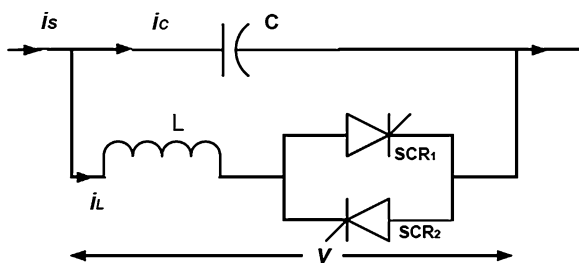
Fig. 1 Configuration of a TCSC
