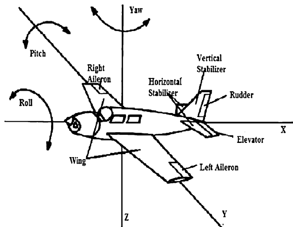
Fig. 1 Yaw, roll, and pitch motions of aircraft [13]
