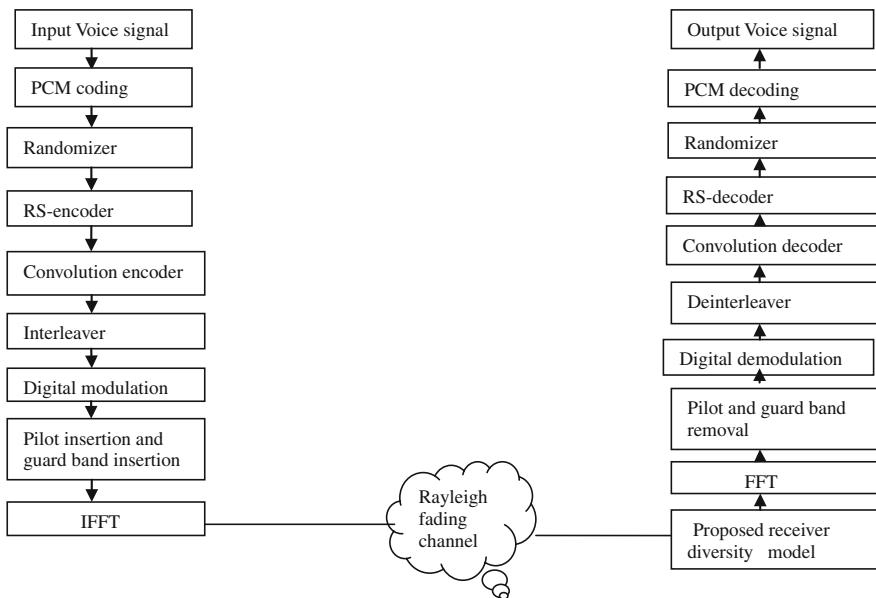
Fig. 1 Proposed end-to-end model
