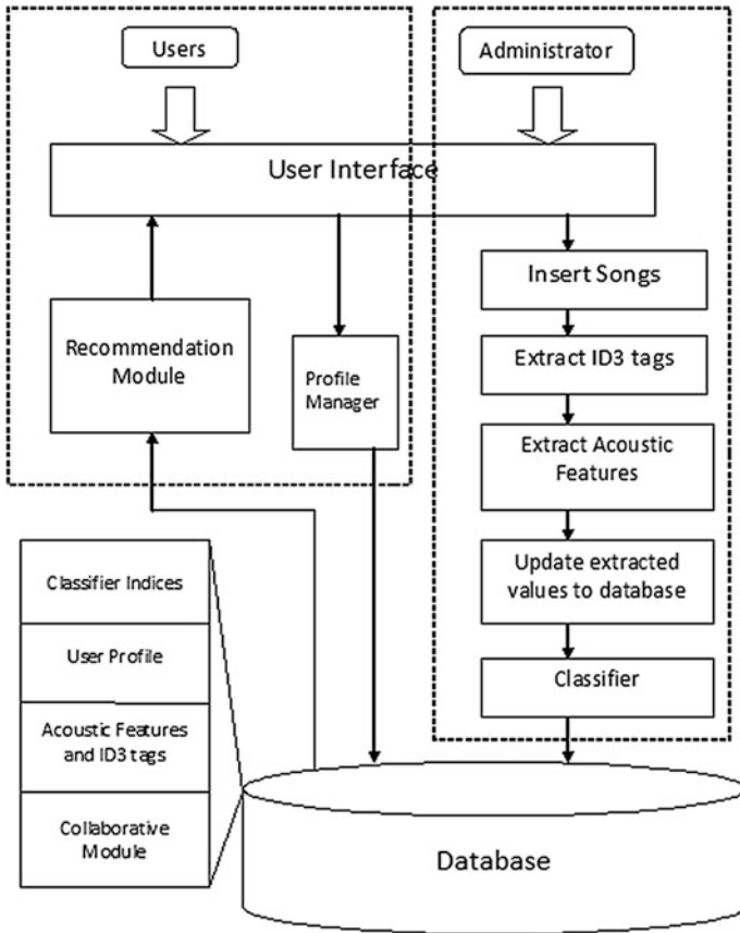
Fig. 1 Hybrid music recommender system design
