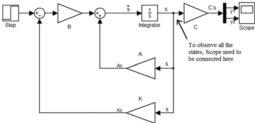
Fig. 4 Simulink model for aircraft state-space model and LQR controller
