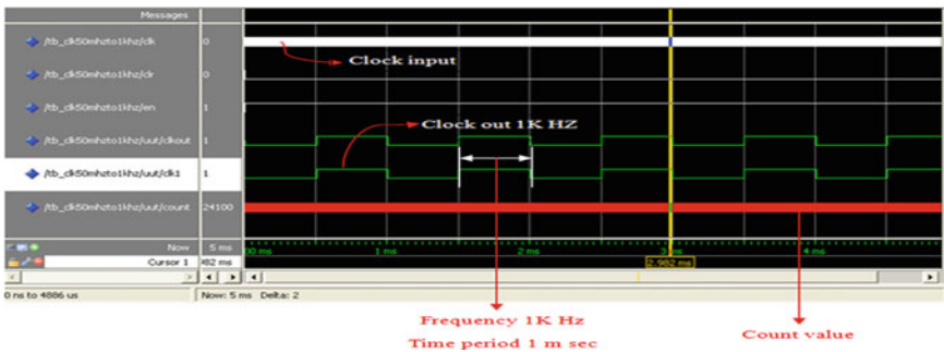
Fig. 8 Clock generator output 1 kHz
