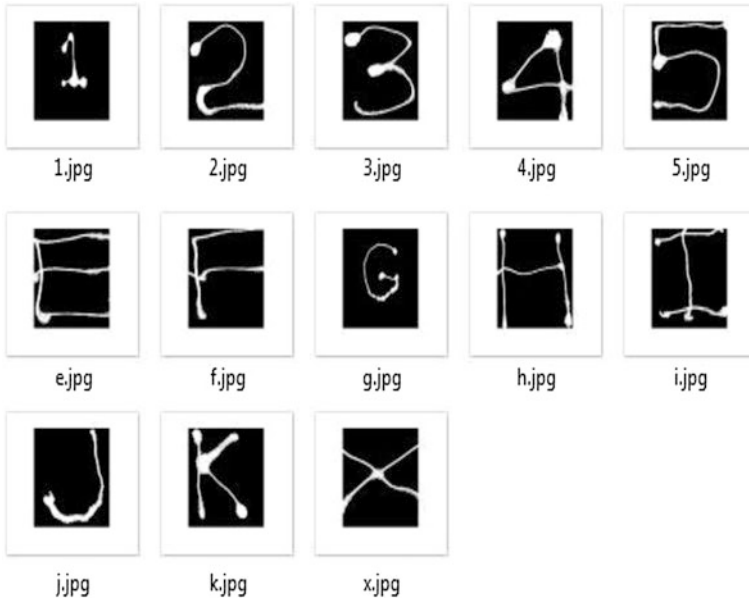
Fig. 9 Noise-reduced images
