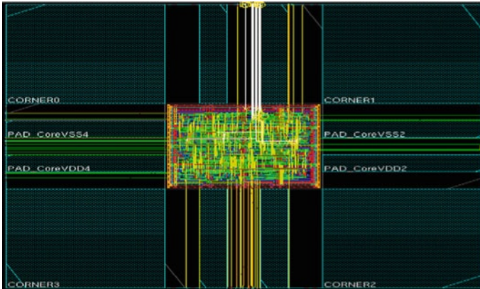
Fig. 8 Routing
