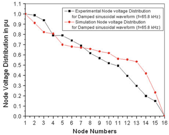
Fig. 11 Comparison of experimental and simulation node voltage distribution for damped sinusoidal waveform of frequency 65.8 kHz
