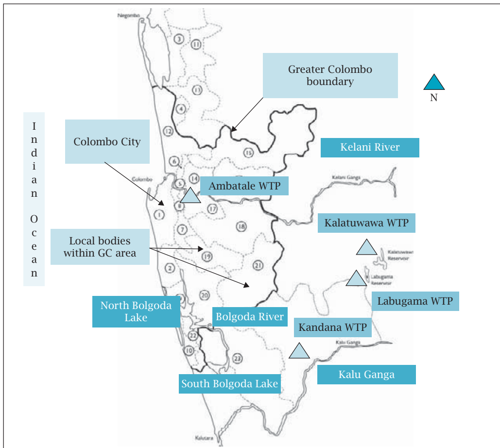
Figure 3 Water Supply System of Greater Colombo Area
