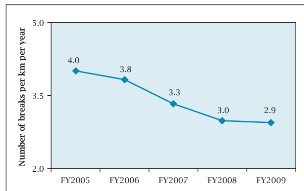
Figure 8 Decline in Pipe Breaks
