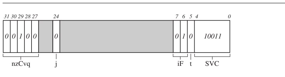
Figure 2.6 Example: cpsr = nzCvqjFiFt_SVC .
