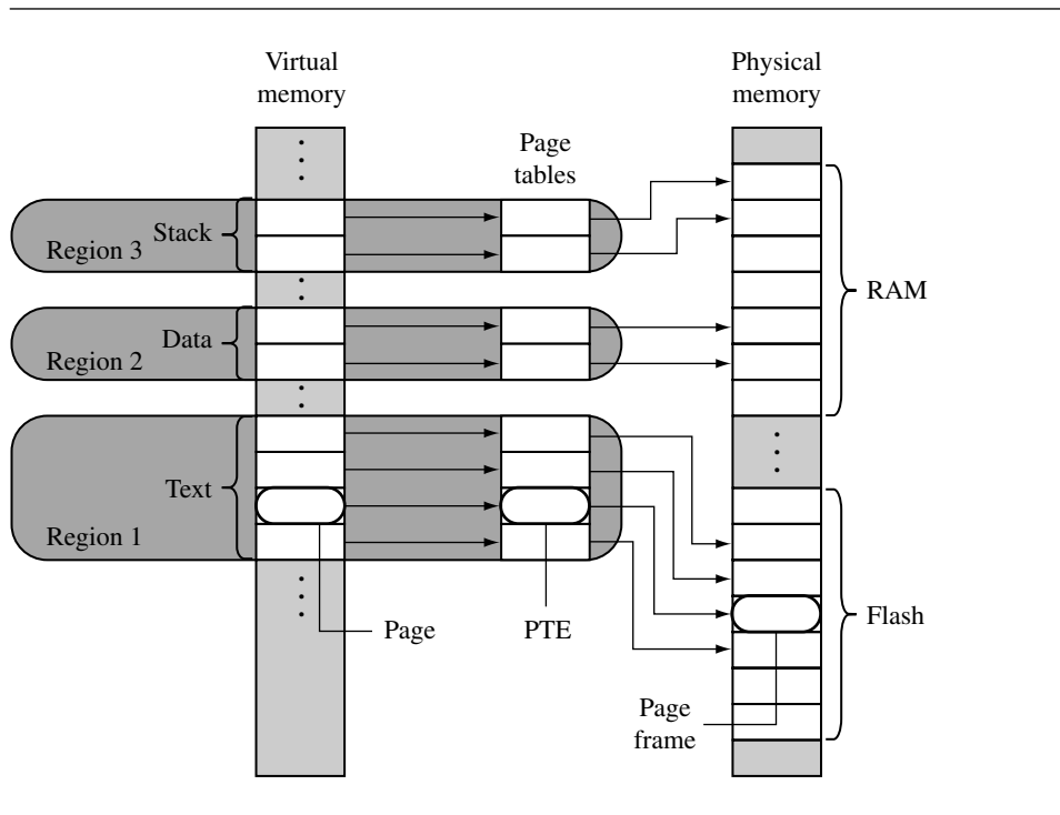
Figure 14.3 An example mapping pages to page frames in an ARM with an MMU.
