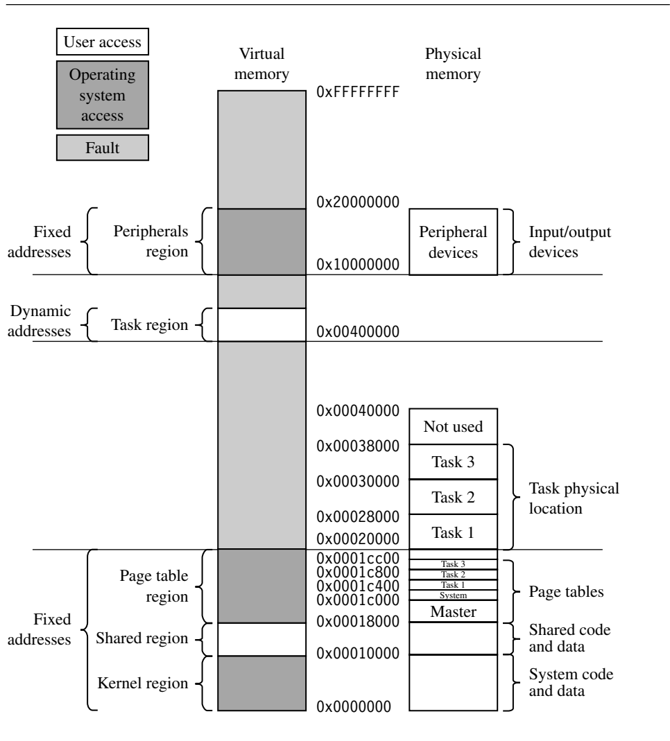
Figure 14.19 Memory map of simple virtual memory example.
