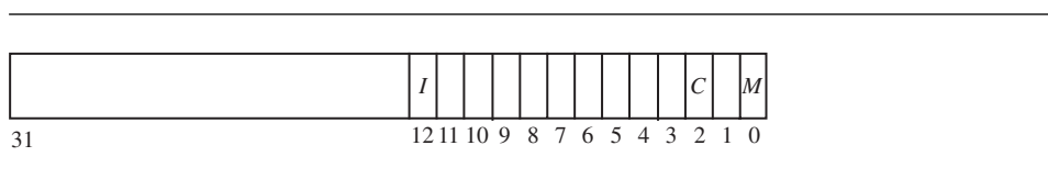
Figure 13.6 Memory protection unit control bits in the CP15:c1:c0 control register.
