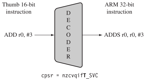
Figure 4.2 Thumb instruction decoding.
