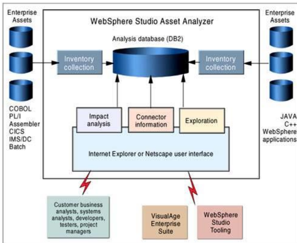
Figure 4-5. WebSphere Studio Asset Analyzer
