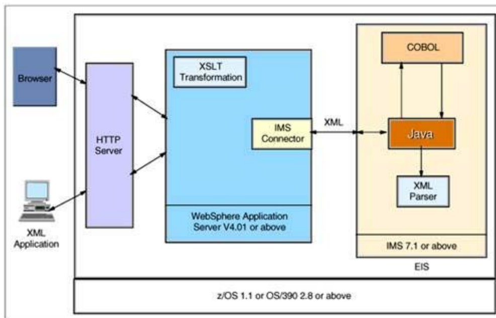
Figure 8-4. IMS Transaction Manager
