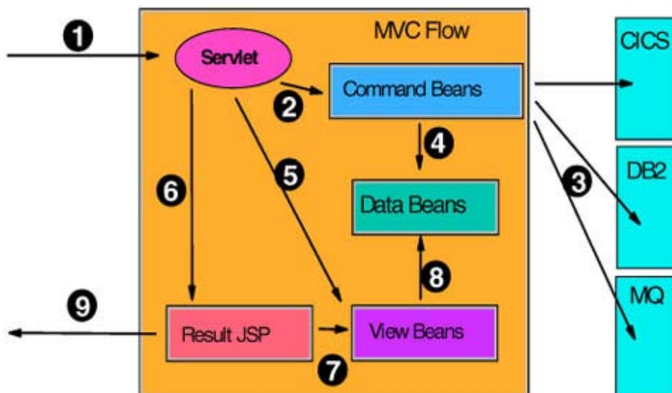
Figure 5-1. A possible scenario utilizing Struts
