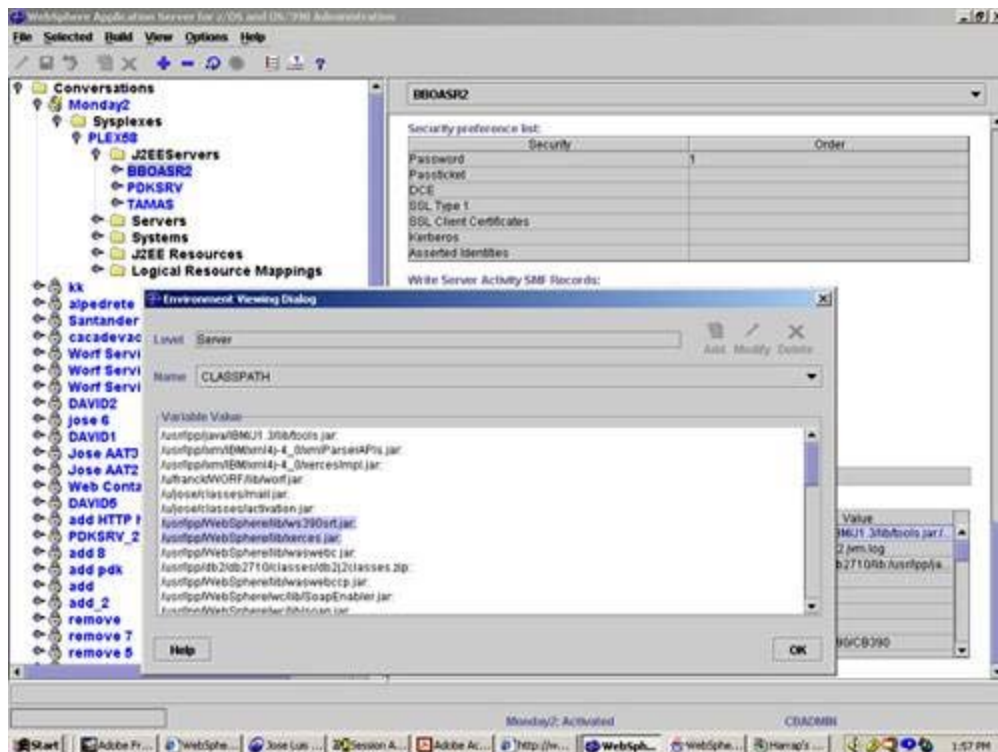
Figure 6-10. Visualize CLASSPATH using SMEUI
