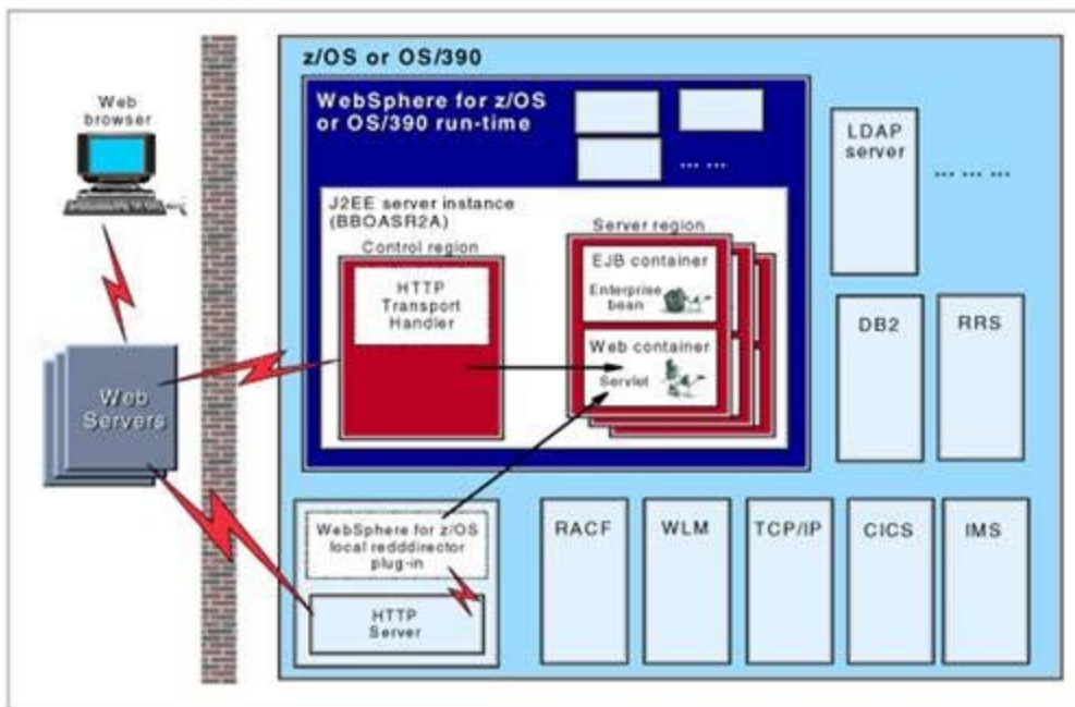
Figure 6-1. WebSphere Application Server in z/OS and OS/390
