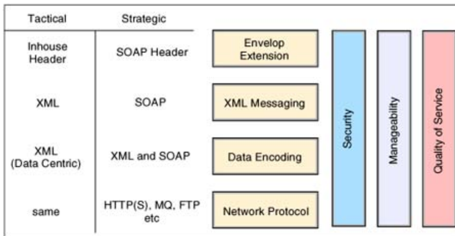
Figure 7-2. Web Services inter-operability
