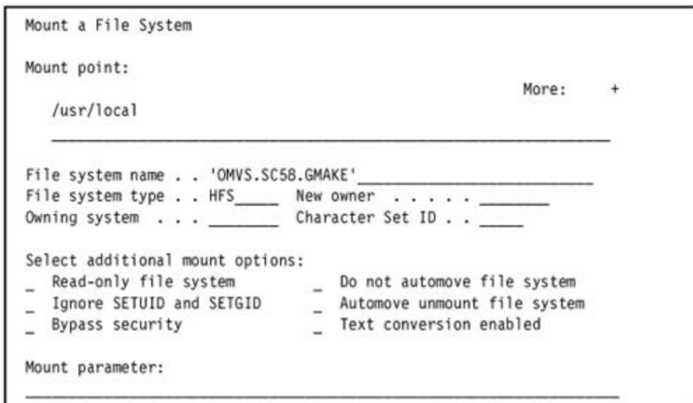
Figure 3-8. Mount a file system
