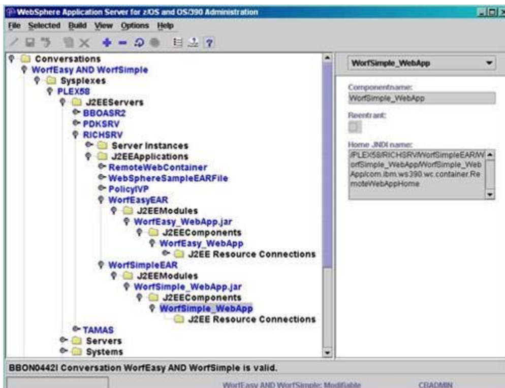
Figure 8-9. Deploying WOLF Web Services samples using a SMEUI conversation
