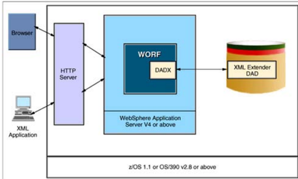
Figure 8-8. Web Services Object Runtime Framework
