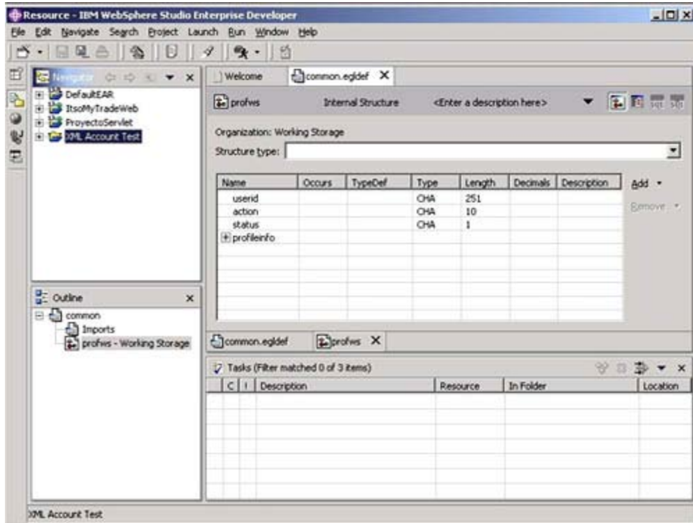
Figure 5-4. New created project
