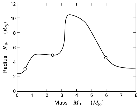
Figure 11.21 Mass-radius relation in a spherical protostar, accreting at the rate 1 \times 10^{-5} M_\odot \text{ yr}^{-1} . The three open circles indicate the onset of full convection, the appearance of the radiative barrier, and the second initiation of central convection, as a result of hydrogen fusion.
