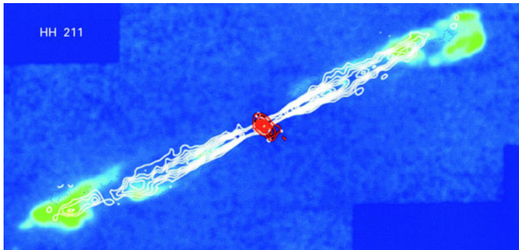
Plate 12 The jet-like HH 211 molecular outflow. The white contours represent J = 2 \rightarrow 1 emission of ^{12}\text{C}^{16}\text{O} , while the central, red contours trace continuum emission at 1.3 mm. Green patches near the ends show emission from the 2.12 \mu\text{m} line of shocked \text{H}_2 . These patches are separated by 2100 AU.
