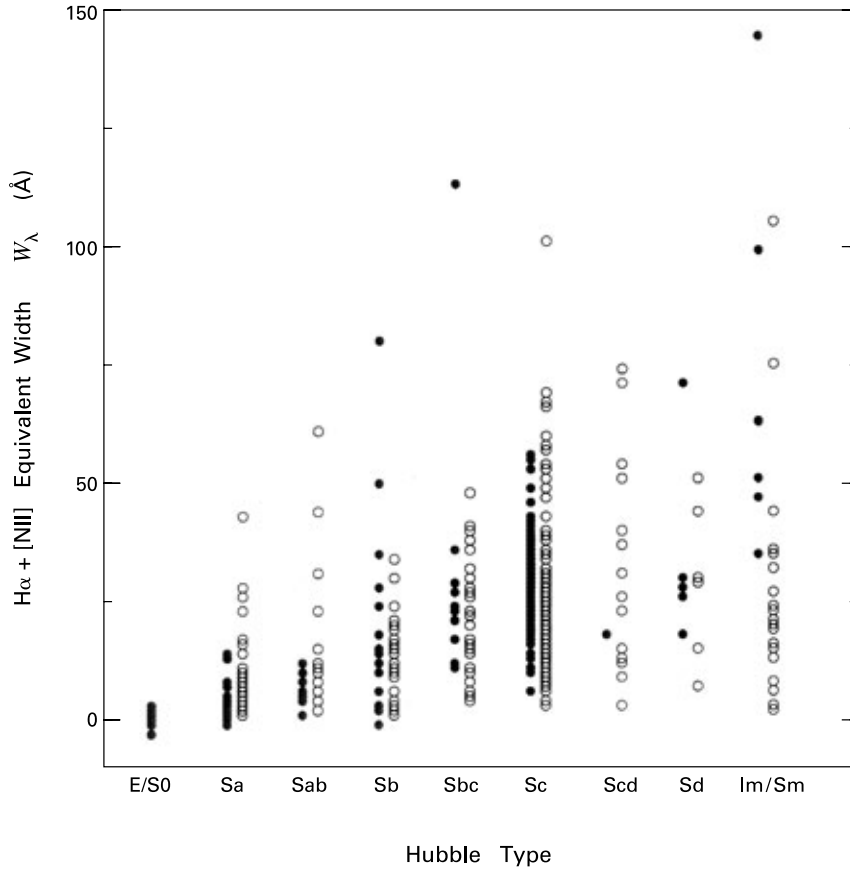
Figure 19.6 Combined equivalent widths of H \alpha and [NII] for field galaxies ( filled circles ) and those in the Virgo Cluster ( open circles ). The galaxies have been binned by Hubble type. Note again the intermediate types, such as Sab.
