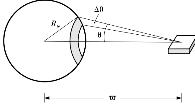
Figure 17.17 Irradiation of a disk patch by a spherical star.
