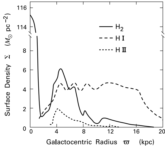
Figure 2.3 Galactic surface densities of \text{H}_2 , HI, and HII gas. The densities are shown as a function of radial distance from the Galactic center. Note the high central peak of the molecular component. The ionized component shown is only that within HII regions.
