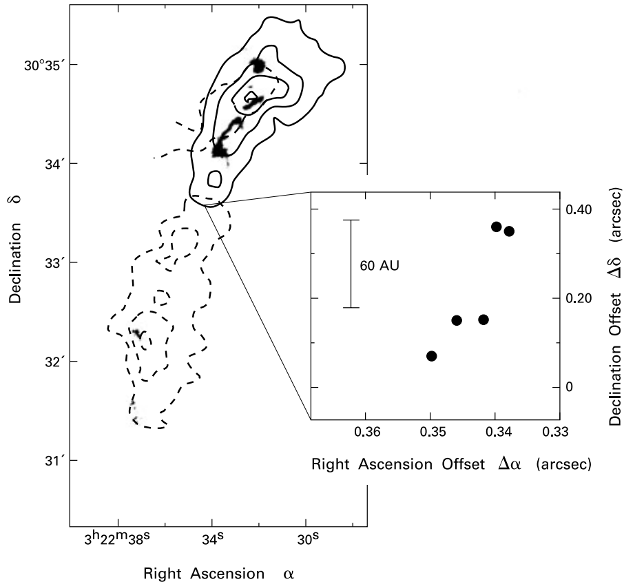
Figure 14.12 Molecular outflow and H 2 O masers in L1448. The solid and dashed contours show, respectively, the blue- and redshifted emission from the J = 2 \rightarrow 1 emission of ^{12}\text{C}^{16}\text{O} , while the dark patches are the 2.12\ \mu\text{m} emission of H 2 . The filled circles within the inset show positions for the 5 brightest H 2 O masers. The angular offsets are measured from \alpha = 3^{\text{h}}22^{\text{m}}34^{\text{s}} , \delta = 30^{\circ}33'35'' .
