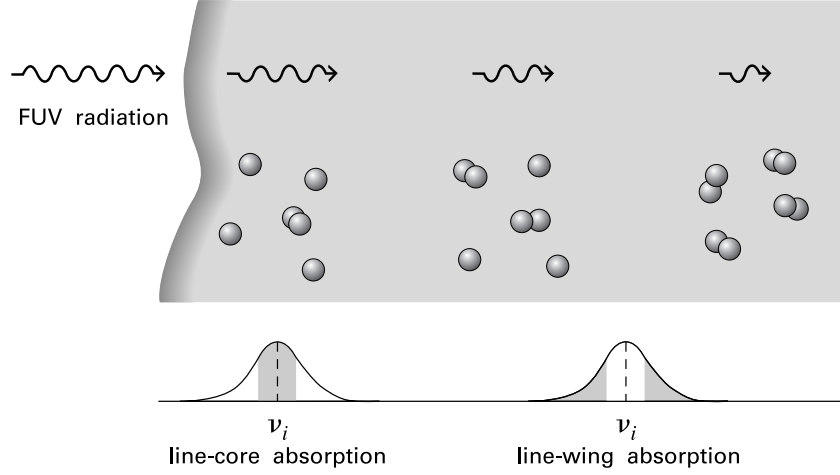
Figure 8.3 Photodissociation of H 2 at the surface of a cloud. The initial absorption of far-ultraviolet photons is at frequencies close to line center for each rovibrational transition. Absorption in the line wings occurs further inside, where the radiation intensity is lower and most atoms are recombined.
