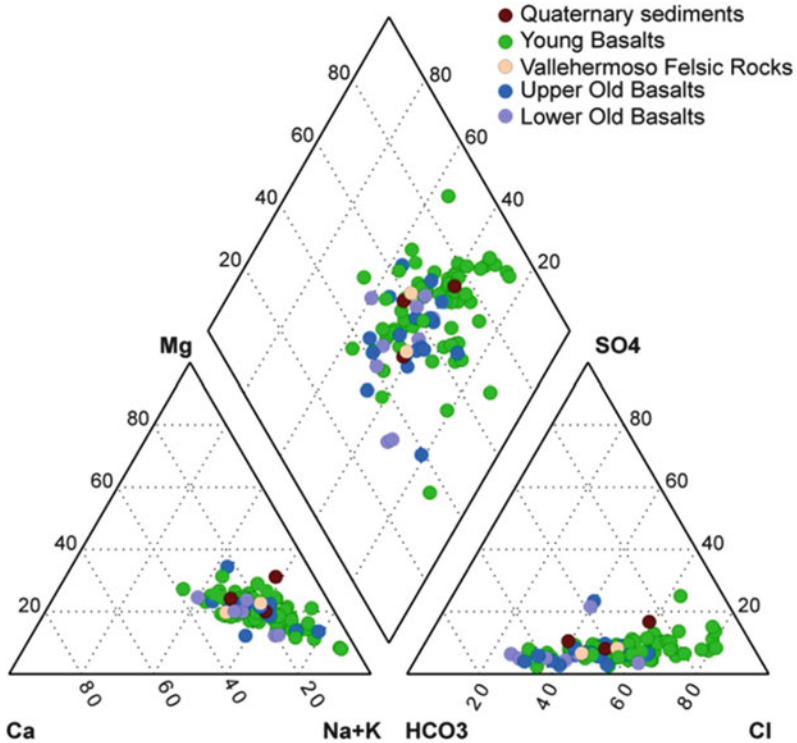
Fig. 28.2 Piper diagram of the spring-waters
