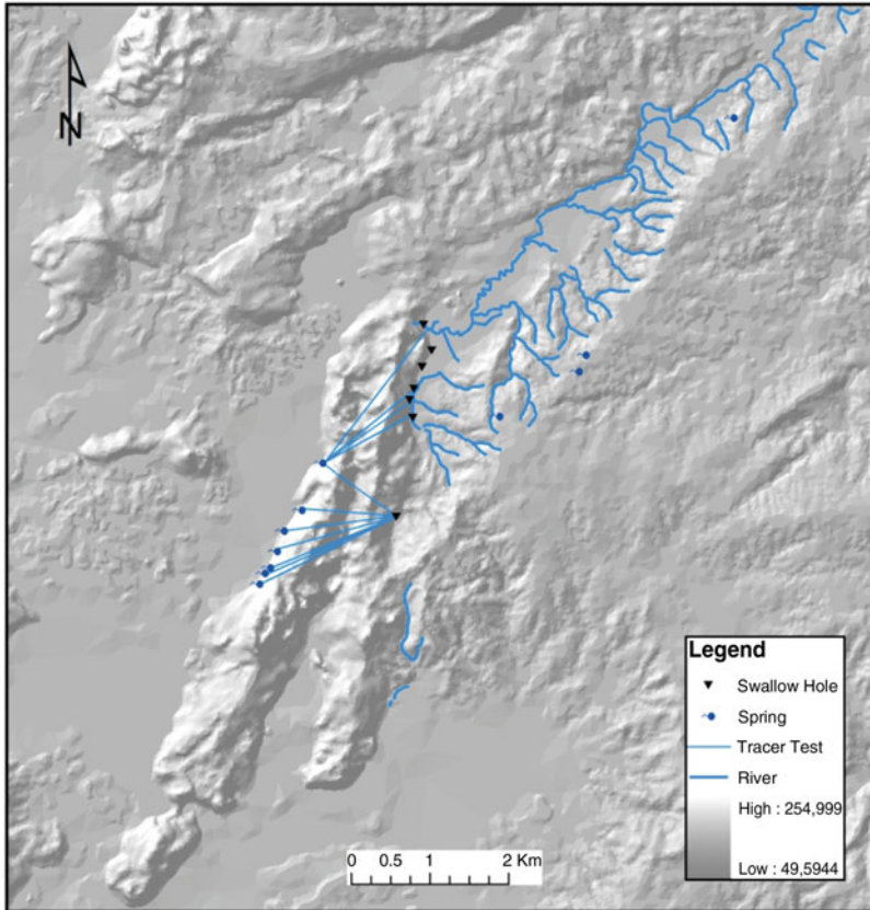
Fig. 16.5 Hydraulic connections defined by tracer tests
