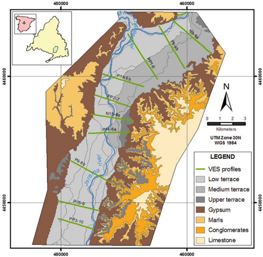
Fig. 19.1 Location map of the study area with geologic units considered for the 3D model. Location of the VES (vertical electrical soundings) profiles is also shown
