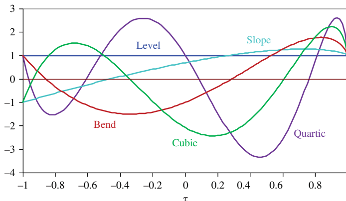
FIGURE 2.3 Forward rate components in \tau space
