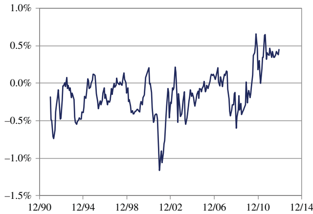
FIGURE 3.4 Historical bend of the Chebyshev basis function
