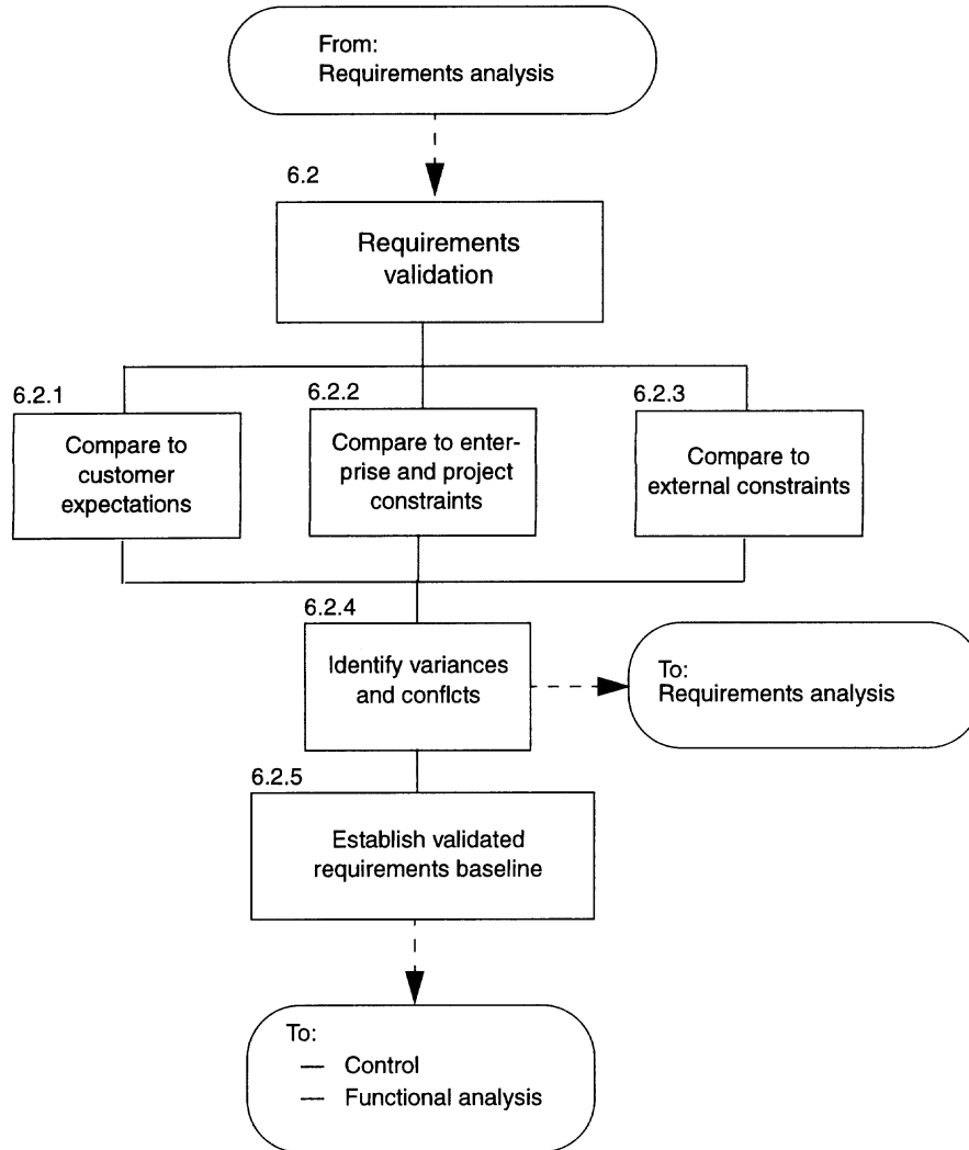
Figure 11—Requirements validation
