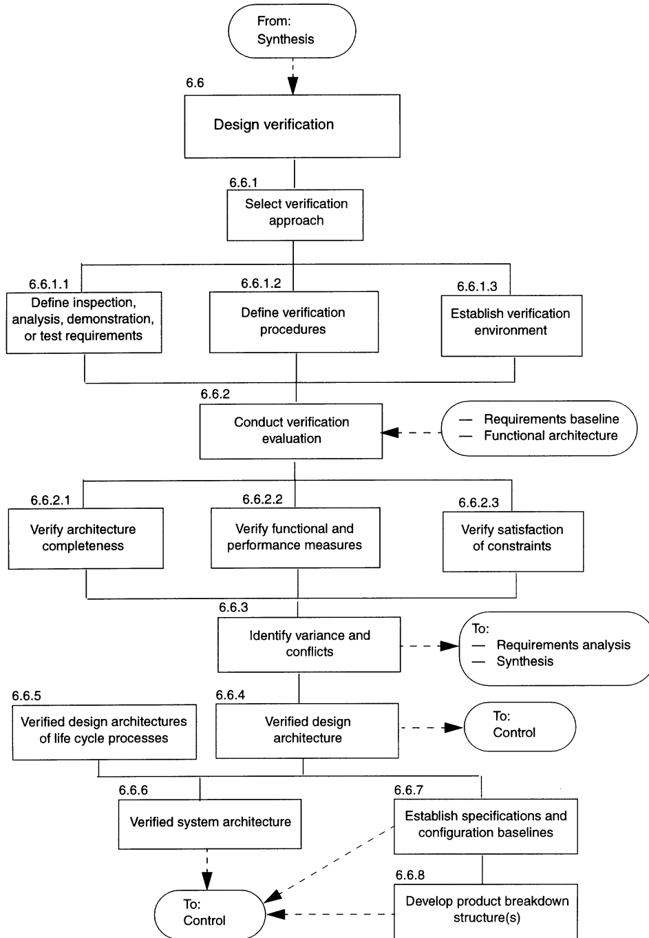
Figure 15—Design verification
