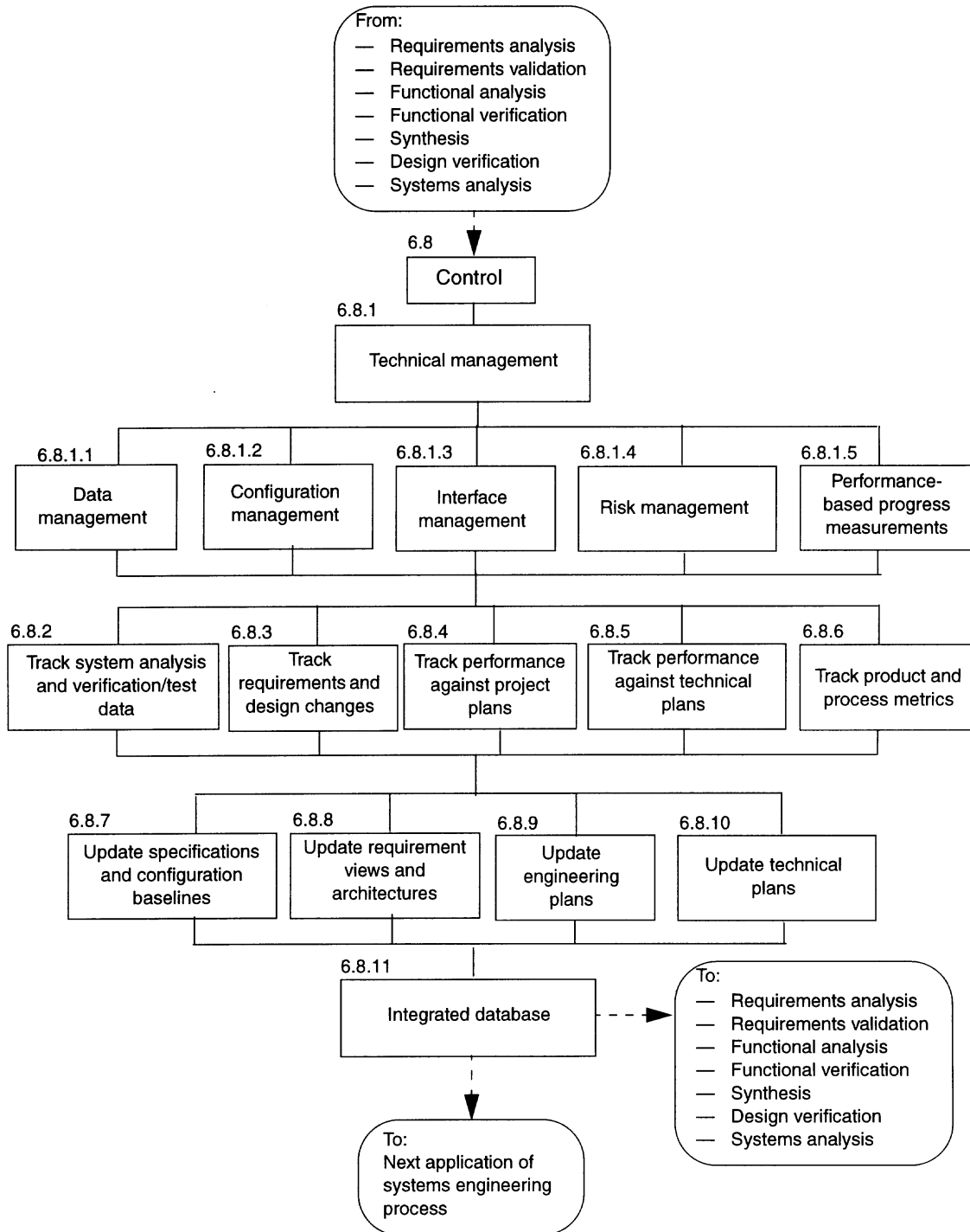
Figure 17—Control process
