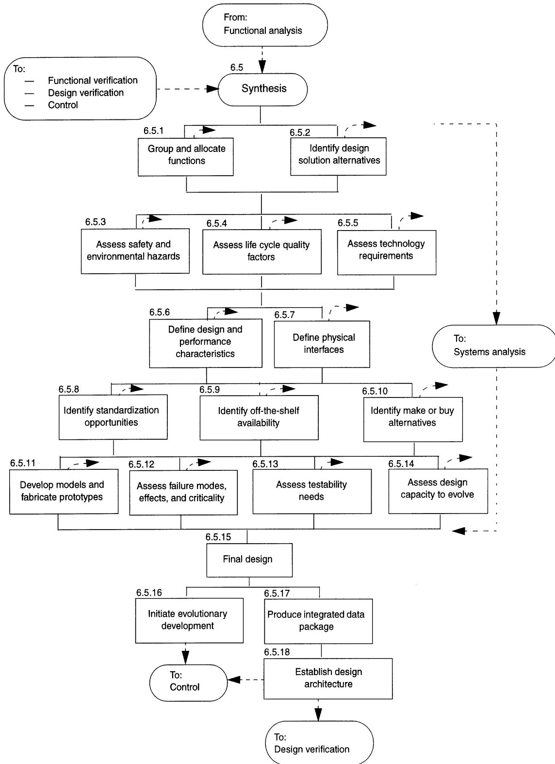
Figure 14—Synthesis process
