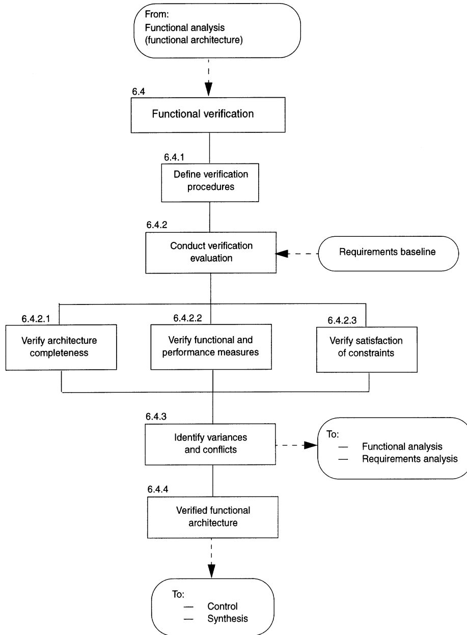
Figure 13—Functional verification
