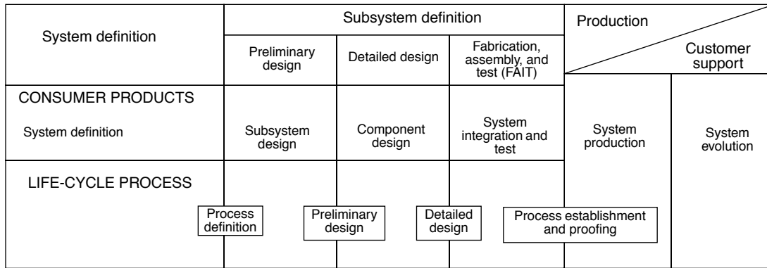
Figure 9—Simultaneous engineering of life cycle processes
