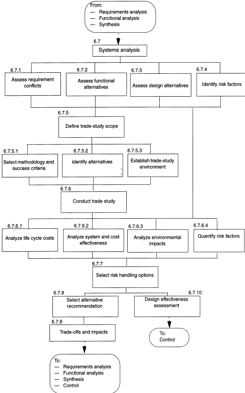
Figure 16—Systems analysis process
