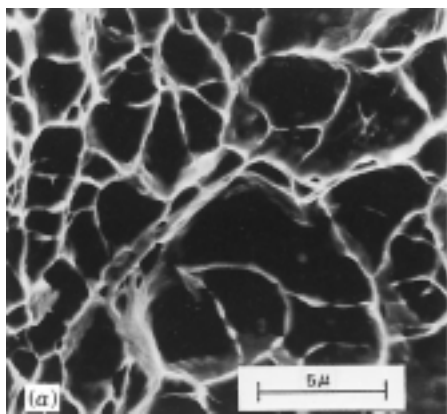
FIGURE 9.4 (a) Scanning electron fractograph showing spherical dimples characteristic of ductile fracture resulting from uniaxial tensile loads. 3300 \times . (b) Scanning electron fractograph showing parabolic-shaped dimples characteristic of ductile fracture resulting from shear loading. 5000 \times . (From R. W. Hertzberg, Deformation and Fracture Mechanics of Engineering Materials , 3rd edition. Copyright © 1989 by John Wiley & Sons, New York. Reprinted by permission of John Wiley & Sons, Inc.)
