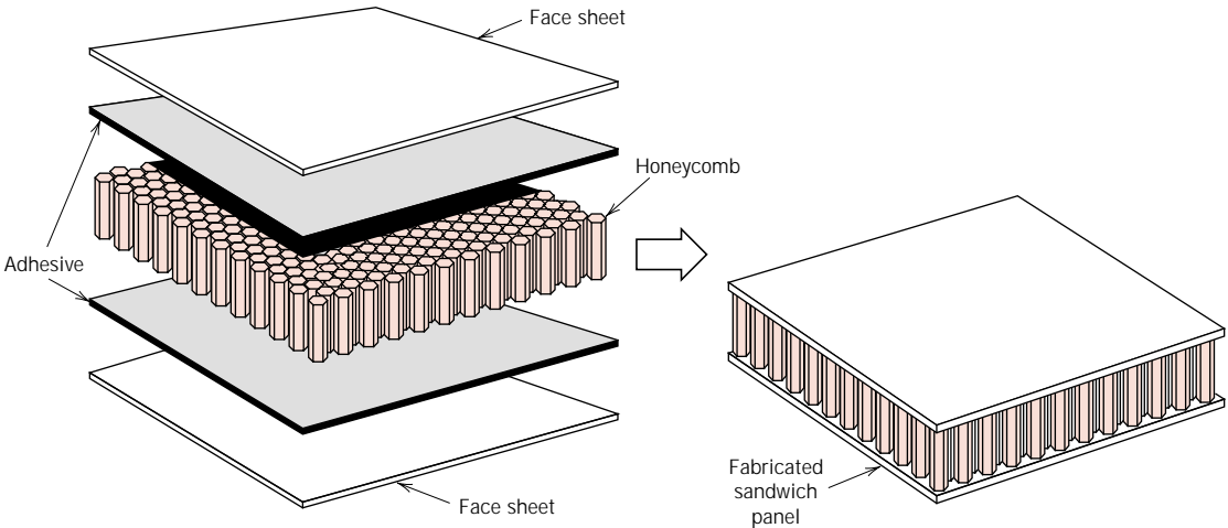
FIGURE 15.17 Schematic diagram showing the construction of a honeycomb core sandwich panel. (Reprinted with permission from Engineered Materials Handbook, Vol. 1, Composites , ASM International, Metals Park, OH, 1987.)
