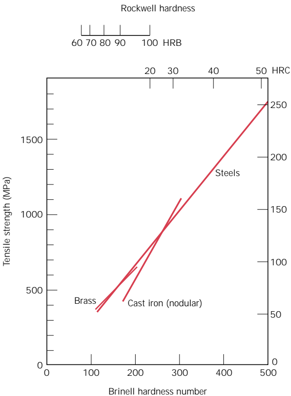
FIGURE 7.31 Relationships between hardness and tensile strength for steel, brass, and cast iron. (Data taken from Metals Handbook: Properties and Selection: Irons and Steels , Vol. 1, 9th edition, B. Bardes, Editor, American Society for Metals, 1978, pp. 36 and 461; and Metals Handbook: Properties and Selection: Nonferrous Alloys and Pure Metals , Vol. 2, 9th edition, H. Baker, Managing Editor, American Society for Metals, 1979, p. 327.)
