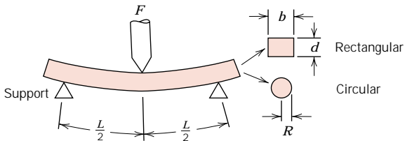
FIGURE 7.18 A three-point loading scheme for measuring the stress-strain behavior and flexural strength of brittle ceramics, including expressions for computing stress for rectangular and circular cross sections.
