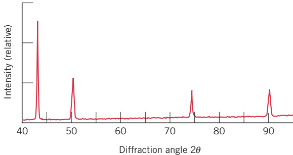
FIGURE 3.41 Diffraction pattern for polycrystalline copper.
