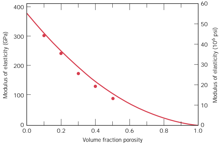
FIGURE 7.20 The influence of porosity on the modulus of elasticity for aluminum oxide at room temperature. The curve drawn is according to Equation 7.21. (From R. L. Coble and W. D. Kingery, "Effect of Porosity on Physical Properties of Sintered Alumina," J. Am. Ceram. Soc. , 39 , 11, Nov. 1956, p. 381. Reprinted by permission of the American Ceramic Society.)
