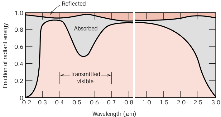
FIGURE 19.8 The variation with wavelength of the fractions of incident light transmitted, absorbed, and reflected through a green glass. (From W. D. Kingery, H. K. Bowen, and D. R. Uhlmann, Introduction to Ceramics , 2nd edition. Copyright © 1976 by John Wiley & Sons, New York. Reprinted by permission of John Wiley & Sons, Inc.)
