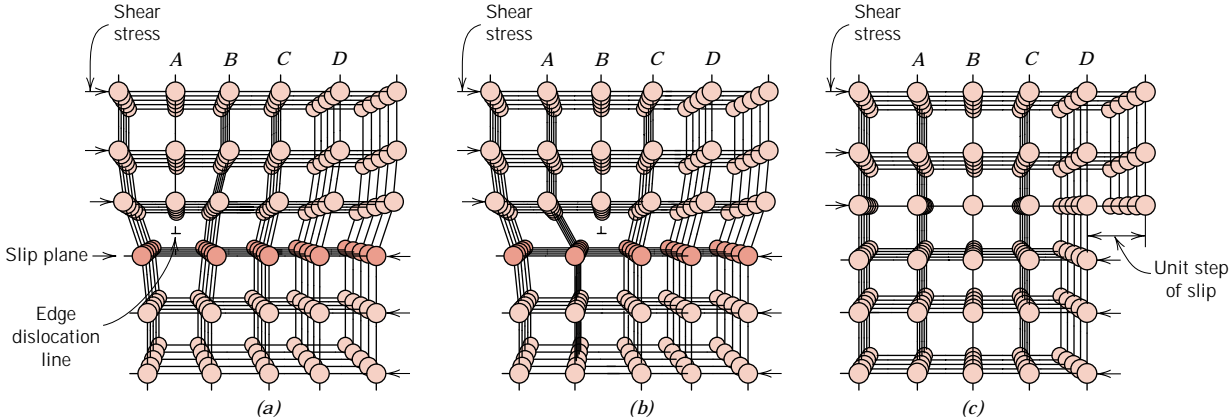
FIGURE 8.1 Atomic rearrangements that accompany the motion of an edge dislocation as it moves in response to an applied shear stress. (a) The extra half-plane of atoms is labeled A. (b) The dislocation moves one atomic distance to the right as A links up to the lower portion of plane B; in the process, the upper portion of B becomes the extra half-plane. (c) A step forms on the surface of the crystal as the extra half-plane exits. (Adapted from A. G. Guy, Essentials of Materials Science , McGraw-Hill Book Company, New York, 1976, p. 153.)
