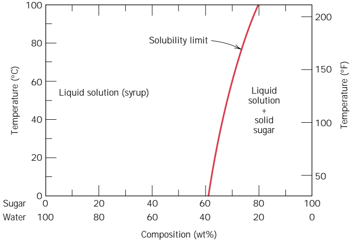
FIGURE 10.1 The solubility of sugar (C 12 H 22 O 11 ) in a sugar-water syrup.
