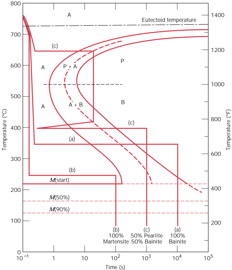
FIGURE 11.16 Isothermal transformation diagram for an iron-carbon alloy of eutectoid composition and the isothermal heat treatments (a), (b), and (c) in Example Problem 11.1.
