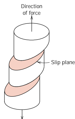
FIGURE 8.8 Macroscopic slip in a single crystal.
