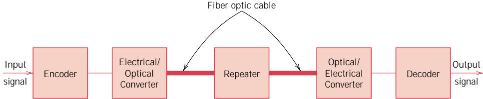
FIGURE 19.16 Schematic diagram showing the components of an optical fiber communications system.
