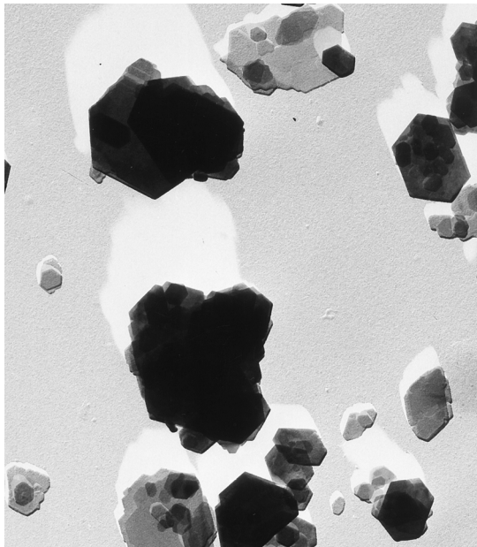
FIGURE 3.15 Electron micrograph of kaolinite crystals. They are in the form of hexagonal plates, some of which are stacked on top of one another. 21,000 \times . (Photograph courtesy of Georgia Kaolin Co., Inc.)
