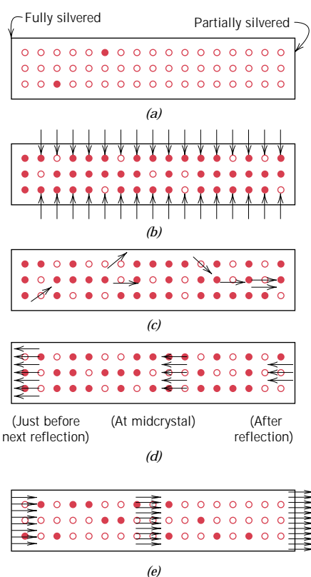
FIGURE 19.13 Schematic representations of the stimulated emission and light amplification for a ruby laser. (a) The chromium ions before excitation. (b) Electrons in some chromium atoms are excited into higher energy states by the xenon light flash. (c) Emission from metastable electron states is initiated or stimulated by photons that are spontaneously emitted. (d) Upon reflection from the silvered ends, the photons continue to stimulate emissions as they traverse the rod length. (e) The coherent and intense beam is finally emitted through the partially silvered end. (From R. M. Rose, L. A. Shepard, and J. Wulff, The Structure and Properties of Materials , Vol. 4, Electronic Properties . Copyright © 1966 by John Wiley & Sons, New York. Reprinted by permission of John Wiley & Sons, Inc.)
