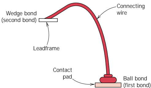
FIGURE 20.23 Schematic diagram showing a connecting wire that is ball bonded to the IC contact pad and wedge bonded to the leadframe. (Adapted from Electronic Materials Handbook, Vol. 1, Packaging , C. A. Dostal, editor, ASM International, 1989, p. 225.)
