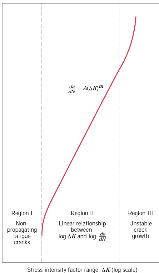
FIGURE 9.34 Schematic representation of logarithm fatigue crack propagation rate da/dN versus logarithm stress intensity factor range \Delta K . The three regions of different crack growth response (I, II, and III) are indicated. (Reprinted with permission from ASM International, Metals Park, OH 44073-9989. W. G. Clark, Jr., "How Fatigue Crack Initiation and Growth Properties Affect Material Selection and Design Criteria," Metals Engineering Quarterly , Vol. 14, No. 3, 1974.)
