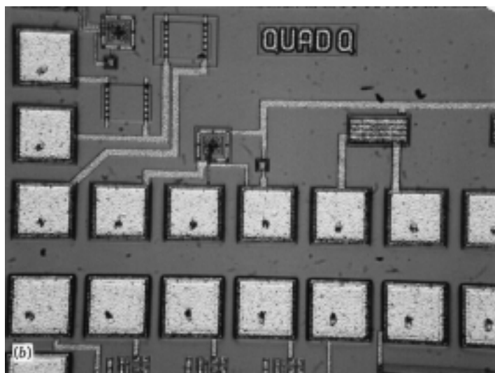
FIGURE 12.25 (a) Scanning electron micrograph showing a small region of a microprocessing chip (a 0.5 MB selected address device). The narrow, white regions are an aluminum top layer that serves as the wiring for this device. The gray regions are diffusion-layer doped silicon that have been coated with an interlayer dielectric. Approximately 2000 \times . (b) An optical photomicrograph showing a portion of a circuit that is used to test microprocessing chips. The narrow, light regions are aluminum connectors, while the white, square areas are test pads (semiconductor devices); test circuits (also composed of semiconductor devices) appear in the upper left-hand corner of the photograph. Approximately 50 \times . (Both photographs courtesy of Nick Gonzales of National Semiconductor Corporation, West Jordan, Utah.)
