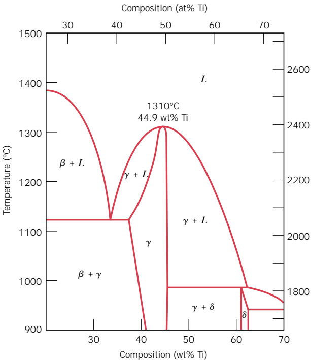
FIGURE 10.20 A portion of the nickel–titanium phase diagram on which is shown a congruent melting point for the \gamma phase solid solution at 1310^{\circ}\text{C} and 44.9 \text{ wt\% Ti} . (Adapted from Phase Diagrams of Binary Nickel Alloys , P. Nash, Editor, 1991. Reprinted by permission of ASM International, Materials Park, OH.)
