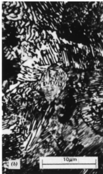
FIGURE 11.6 Photomicrographs of (a) coarse pearlite and (b) fine pearlite. 3000 \times . (From K. M. Ralls, et al., An Introduction to Materials Science and Engineering , p. 361. Copyright © 1976 by John Wiley & Sons, New York. Reprinted by permission of John Wiley & Sons, Inc.)
