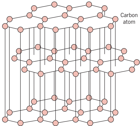
FIGURE 3.17 The structure of graphite.
