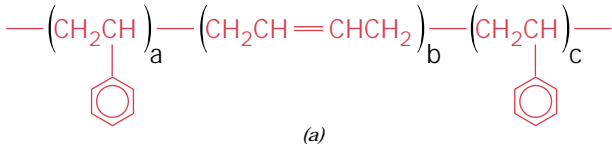
FIGURE 13.10 Representations of the chain chemistries for (a) styrene-butadiene-styrene (S-B-S), and (b) styrene-isoprene-styrene (S-I-S) thermoplastic elastomers.
