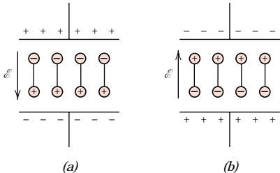
FIGURE 12.31 Dipole orientations for (a) one polarity of an alternating electric field and (b) for the reversed polarity. (From Richard A. Flinn and Paul K. Trojan, Engineering Materials and Their Applications , 4th edition. Copyright © 1990 by John Wiley & Sons, Inc. Adapted by permission of John Wiley & Sons, Inc.)
