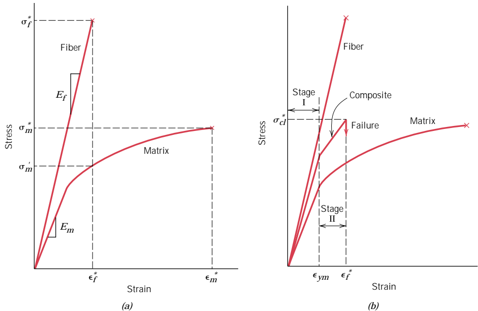
FIGURE 15.9 (a) Schematic stress–strain curves for brittle fiber and ductile matrix materials. Fracture stresses and strains for both materials are noted. (b) Schematic stress–strain curve for an aligned fiber-reinforced composite that is exposed to a uniaxial stress applied in the direction of alignment; curves for the fiber and matrix materials shown in part (a) are also superimposed.
