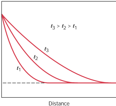
FIGURE 6.5 Concentration profiles for nonsteady-state diffusion taken at three different times, t_1 , t_2 , and t_3 .
