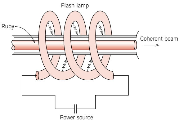
FIGURE 19.11 Schematic diagram of the ruby laser and xenon flash lamp. (From R. M. Rose, L. A. Shepard, and J. Wulff, The Structure and Properties of Materials, Vol. 4, Electronic Properties . Copyright © 1966 by John Wiley & Sons, New York. Reprinted by permission of John Wiley & Sons, Inc.)
