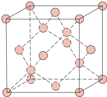
FIGURE 3.16 A unit cell for the diamond cubic crystal structure.
