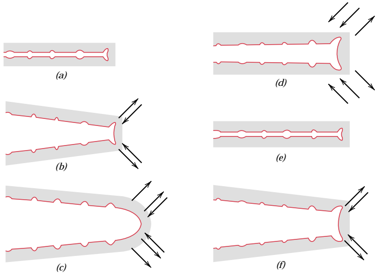
FIGURE 9.29 Fatigue crack propagation mechanism (stage II)
