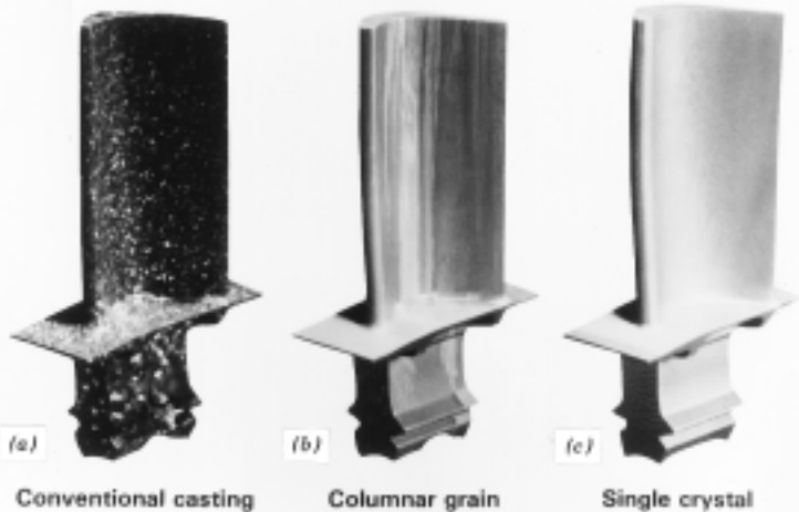
FIGURE 9.45 (a) Polycrystalline turbine blade that was produced by a conventional casting technique. High-temperature creep resistance is improved as a result of an oriented columnar grain structure (b) produced by a sophisticated directional solidification technique. Creep resistance is further enhanced when single-crystal blades (c) are used. (Courtesy of Pratt & Whitney.)
