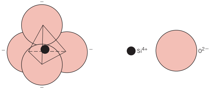
FIGURE 3.10 A silicon–oxygen ( \text{SiO}_4^{4-} ) tetrahedron.
