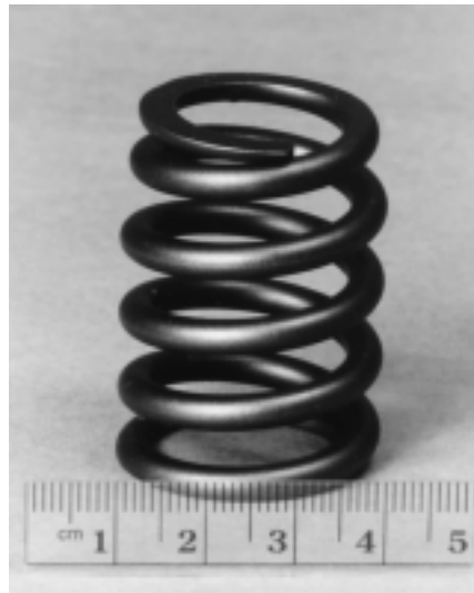
FIGURE 20.7 Photograph of a typical automobile valve spring.
