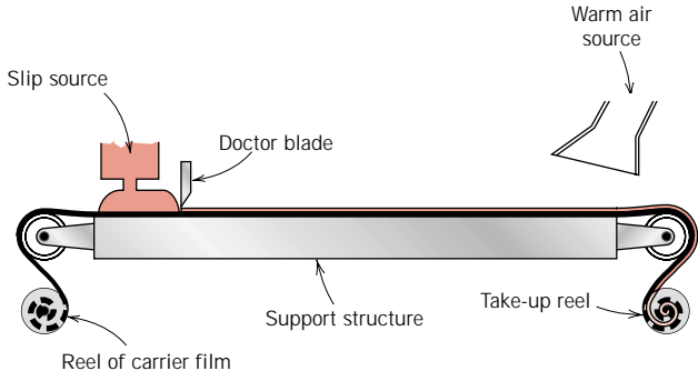
FIGURE 14.26 Schematic diagram showing the tape casting process using a doctor blade. (From D. W. Richerson, Modern Ceramic Engineering , 2nd edition, Marcel Dekker, Inc., NY, 1992. Reprinted from Modern Ceramic Engineering , 2nd edition, p. 472 by courtesy of Marcel Dekker, Inc.)
