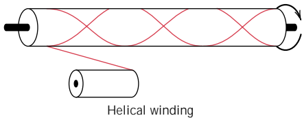
FIGURE 15.14 Schematic representations of helical, circumferential, and polar filament winding techniques. (From N. L. Hancox, Editor, Fibre Composite Hybrid Materials , The Macmillan Company, New York, 1981.)
