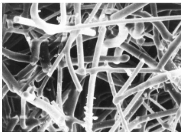
FIGURE 20.18 Scanning electron micrograph of a Space Shuttle Orbiter ceramic tile showing silica fibers that were bonded to one another during a sintering heat treatment. 750 \times . (Photograph provided courtesy of Lockheed Aerospace Ceramics Systems, Sunnyvale, California.)
