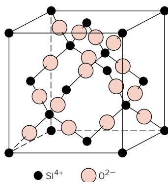
FIGURE 3.11 The arrangement of silicon and oxygen atoms in a unit cell of cristobalite, a polymorph of \text{SiO}_2 .
