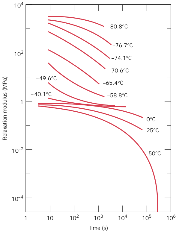
FIGURE 7.35 Logarithm of relaxation modulus versus logarithm of time for polyisobutylene between -80 and 50^{\circ}\text{C} . (Adapted from E. Catsiff and A. V. Tobolsky, "Stress-Relaxation of Polyisobutylene in the Transition Region [1,2]," J. Colloid Sci. , 10 , 377 [1955]. Reprinted by permission of Academic Press, Inc.)
