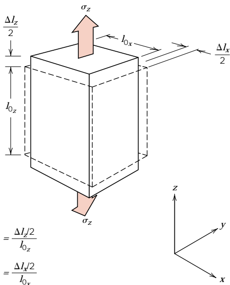
FIGURE 7.9 Axial ( z ) elongation (positive strain) and lateral ( x and y ) contractions (negative strains) in response to an imposed tensile stress. Solid lines represent dimensions after stress application; dashed lines, before.
