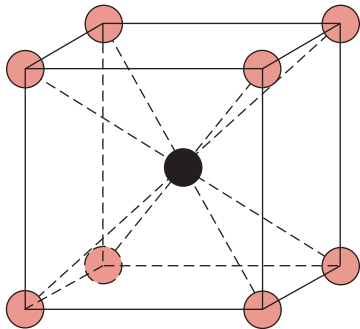
FIGURE 3.6 A unit cell for the cesium chloride (CsCl) crystal structure.
