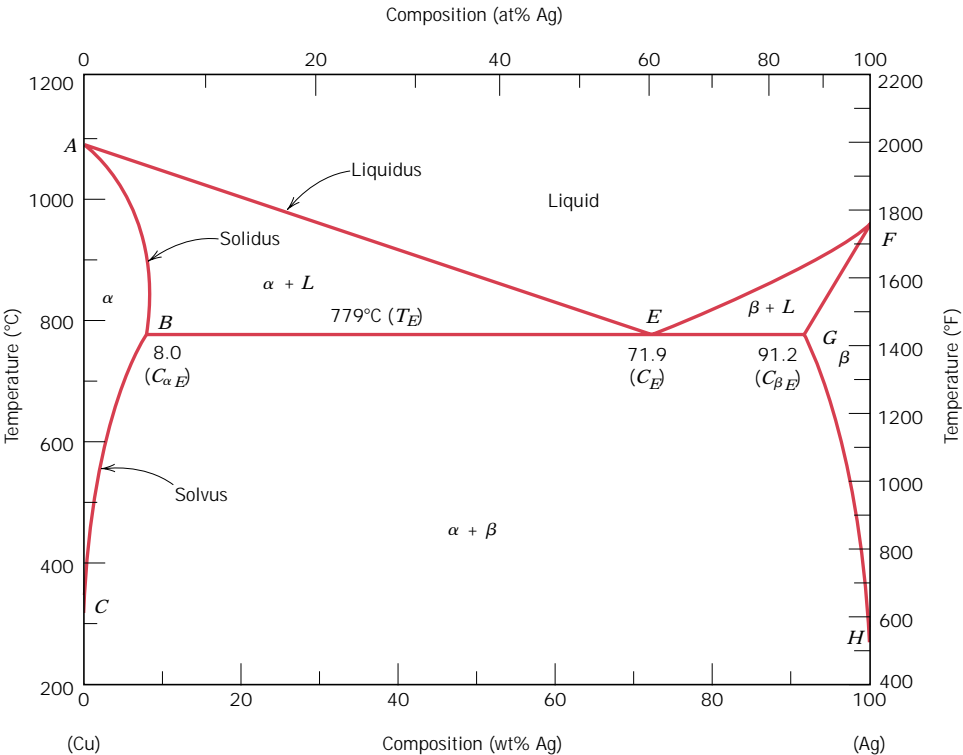
FIGURE 10.6 The copper–silver phase diagram. (Adapted from Binary Alloy Phase Diagrams , 2nd edition, Vol. 1, T. B. Massalski, Editor-in-Chief, 1990.
