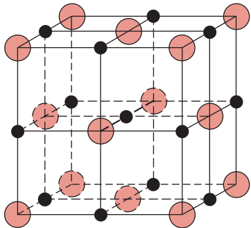
FIGURE 3.5 A unit cell for the rock salt, or sodium chloride (NaCl), crystal structure.
