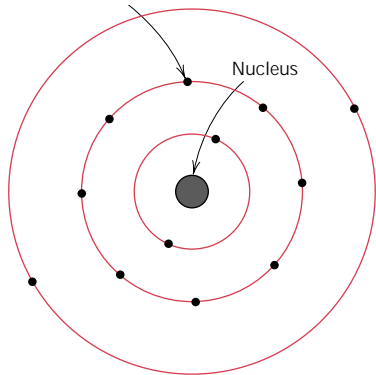
FIGURE 2.1 Schematic representation of the Bohr atom.
