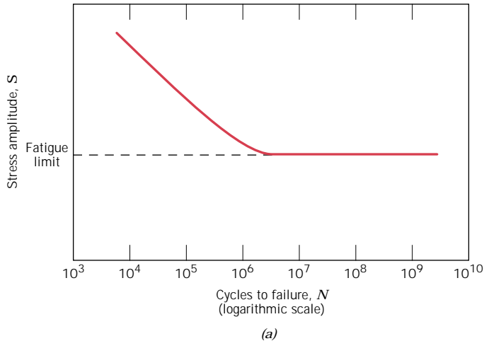
FIGURE 9.25 Stress amplitude ( S ) versus logarithm of the number of cycles to fatigue failure ( N ) for (a) a material that displays a fatigue limit, and (b) a material that does not display a fatigue limit.
