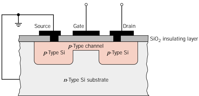
FIGURE 12.24 Schematic cross-sectional view of a MOSFET transistor.
