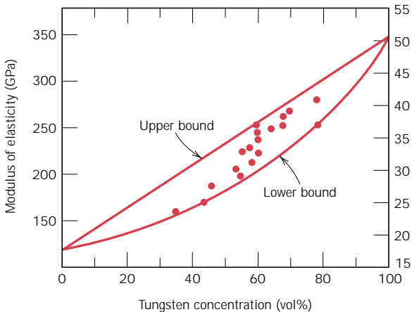
FIGURE 15.3 Modulus of elasticity versus volume percent tungsten for a composite of tungsten particles dispersed within a copper matrix. Upper and lower bounds are according to Equations 15.1 and 15.2; experimental data points are included. (From R. H. Krock, ASTM Proceedings , Vol. 63, 1963. Copyright ASTM. Reprinted with permission.)
