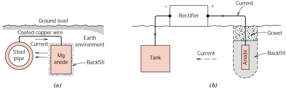
FIGURE 16.22 Cathodic protection of (a) an underground pipeline using a magnesium sacrificial anode, and (b) an underground tank using an impressed current. (From M. G. Fontana, Corrosion Engineering , 3rd edition. Copyright © 1986 by McGraw-Hill Book Company. Reproduced with permission.)
