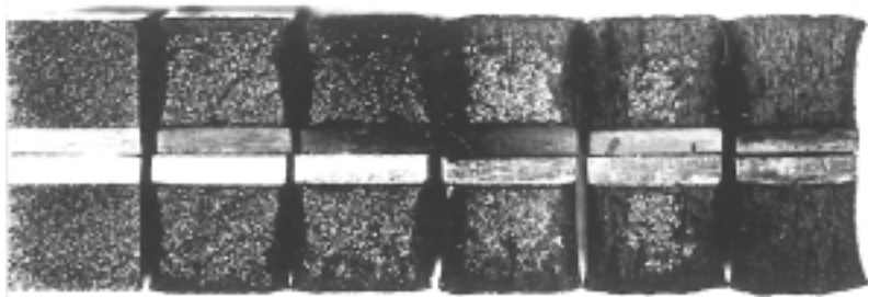
FIGURE 9.21 Photograph of fracture surfaces of A36 steel Charpy V-notch specimens tested at indicated temperatures (in °C). (From R. W. Hertzberg, Deformation and Fracture Mechanics of Engineering Materials , 3rd edition, Fig. 9.6, p. 329. Copyright © 1989 by John Wiley & Sons, Inc., New York. Reprinted by permission of John Wiley & Sons, Inc.)
