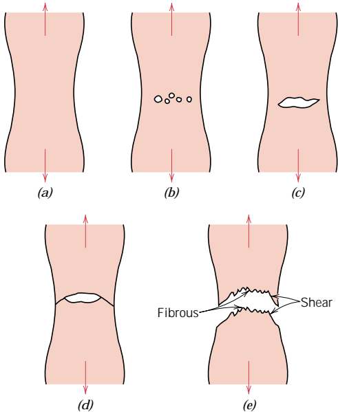
FIGURE 9.2 Stages in the cup-and-cone fracture. (a) Initial necking. (b) Small cavity formation. (c) Coalescence of cavities to form a crack. (d) Crack propagation. (e) Final shear fracture at a 45° angle relative to the tensile direction. (From K. M. Ralls, T. H. Courtney, and J. Wulff, Introduction to Materials Science and Engineering , p. 468. Copyright © 1976 by John Wiley & Sons, New York. Reprinted by permission of John Wiley & Sons, Inc.)
