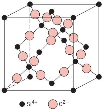
FIGURE 3.11 The arrangement of silicon and oxygen atoms in a unit cell of cristobalite, a polymorph of SiO 2 .
