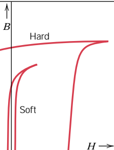
FIGURE 18.16 Schematic magnetization curves for soft and hard magnetic materials. (From K. M. Ralls, T. H. Courtney, and J. Wulff, Introduction to Materials Science and Engineering . Copyright © 1976 by John Wiley & Sons, New York. Reprinted by permission of John Wiley & Sons, Inc.)
