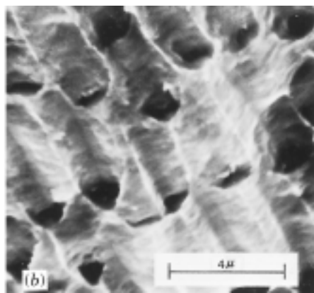
FIGURE 9.4 (a) Scanning electron fractograph showing spherical dimples characteristic of ductile fracture resulting from uniaxial tensile loads. 3300 \times . (b) Scanning electron fractograph showing parabolic-shaped dimples characteristic of ductile fracture resulting from shear loading. 5000 \times . (From R. W. Hertzberg, Deformation and Fracture Mechanics of Engineering Materials , 3rd edition. Copyright © 1989 by John Wiley & Sons, New York. Reprinted by permission of John Wiley & Sons, Inc.)
