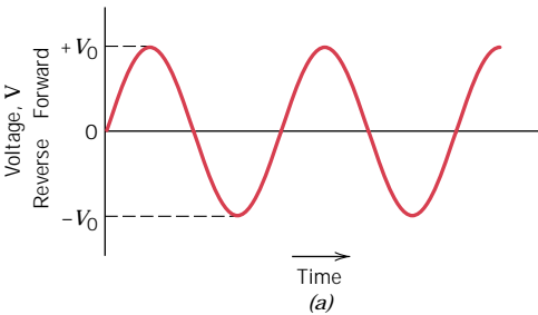
FIGURE 12.21 (a) Voltage versus time for the input to a p - n rectifying junction. (b) Current versus time, showing rectification of voltage in (a) by a p - n rectifying junction having the voltage-current characteristics shown in Figure 12.20.
