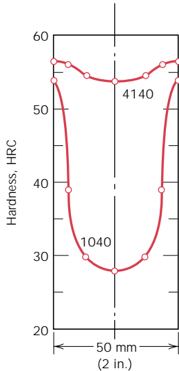
FIGURE 14.12 Radial hardness profiles for (a) 50 mm (2 in.) diameter cylindrical 1040 and 4140 steel specimens quenched in mildly agitated water, and (b) 50 and 100 mm (2 and 4 in.) diameter cylindrical specimens of 4140 steel quenched in mildly agitated water.
