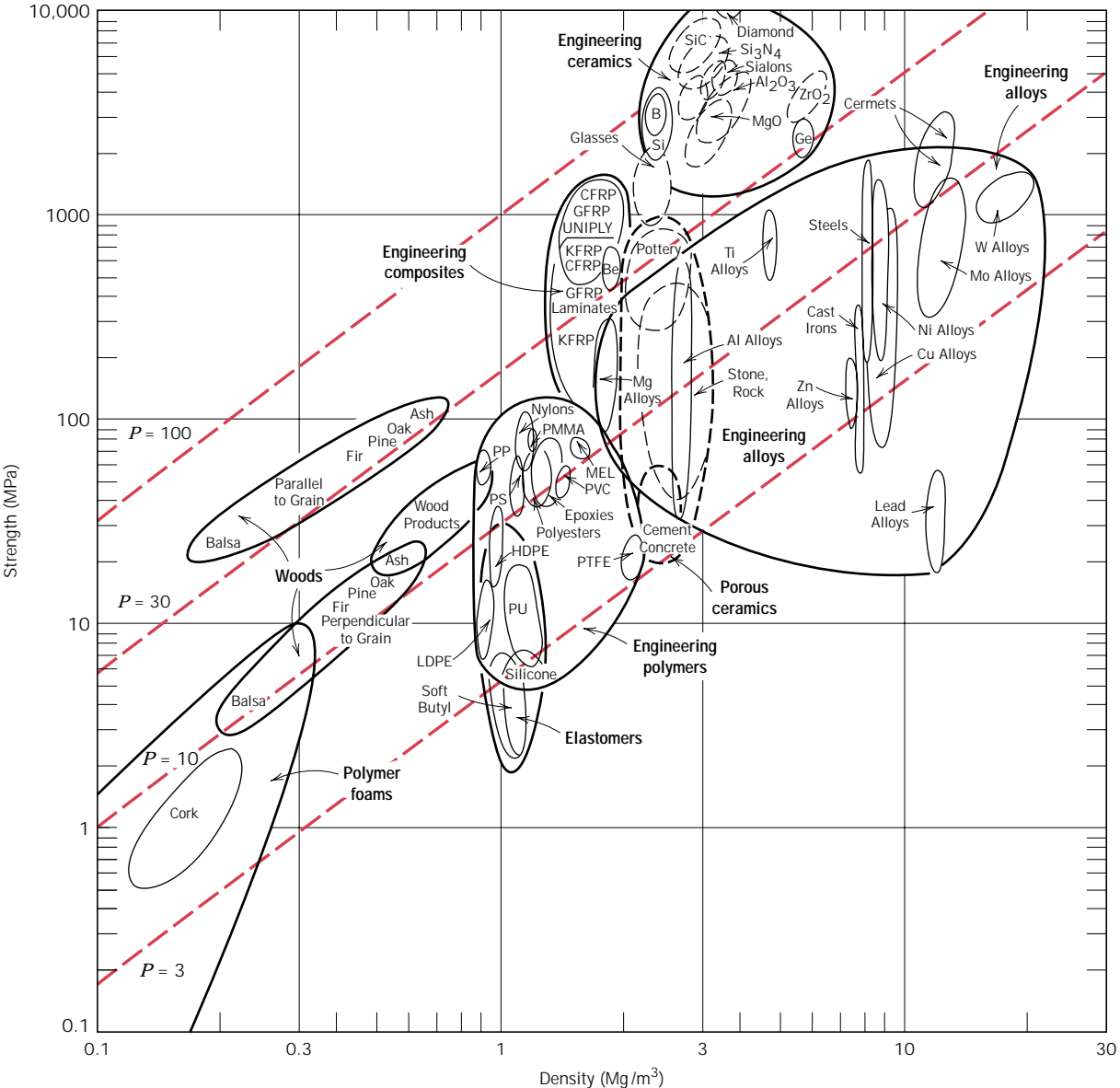
FIGURE 20.2 Strength versus density materials selection chart. Design guidelines for performance indices of 3, 10, 30, and 100 (MPa) 2/3 m 3 /Mg have been constructed, all having a slope of \frac{3}{2} . (Adapted from M. F. Ashby, Materials Selection in Mechanical Design . Copyright © 1992. Reprinted by permission of Butterworth-Heinemann Ltd.)
