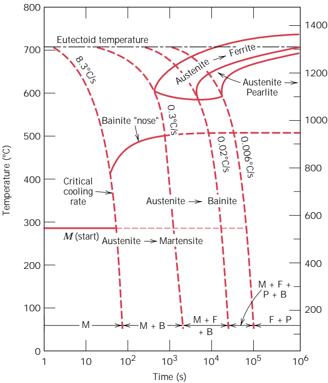
FIGURE 11.20 Continuous cooling transformation diagram for an alloy steel (type 4340) and several superimposed cooling curves demonstrating dependency of the final microstructure of this alloy on the transformations that occur during cooling. (Adapted from H. E. McGannon, Editor, The Making, Shaping and Treating of Steel , 9th edition, United States Steel Corporation, Pittsburgh, 1971, p. 1096.)
