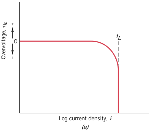
FIGURE 16.9 For reduction reactions, schematic plots of overvoltage versus logarithm of current density for (a) concentration polarization, and (b) combined activation–concentration polarization.
