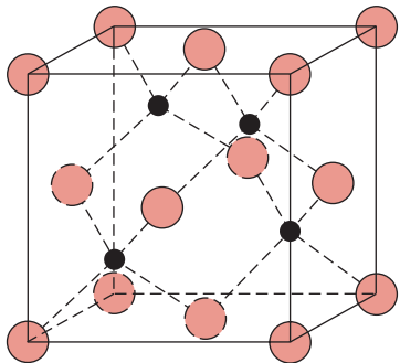
FIGURE 3.7 A unit cell for the zinc blende (ZnS) crystal structure.
