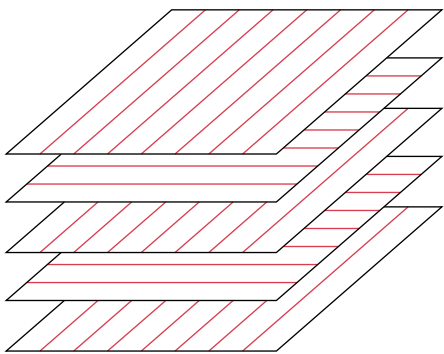
FIGURE 15.16 The stacking of successive oriented, fiber-reinforced layers for a laminar composite.
