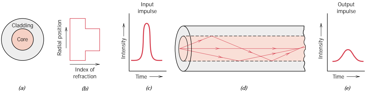
FIGURE 19.19 Step-index optical fiber design. (a) Fiber cross section. (b) Fiber radial index of refraction profile. (c) Input light pulse. (d) Internal reflection of light rays. (e) Output light pulse. (Adapted from S. R. Nagel, IEEE Communications Magazine , Vol. 25, No. 4, p. 34, 1987.)
