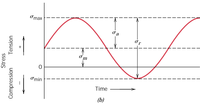
FIGURE 9.23 Variation of stress with time that accounts for fatigue failures. (a) Reversed stress cycle, in which the stress alternates from a maximum tensile stress (+) to a maximum compressive stress (-) of equal magnitude. (b) Repeated stress cycle, in which maximum and minimum stresses are asymmetrical relative to the zero stress level; mean stress \sigma_m , range of stress \sigma_r , and stress amplitude \sigma_a are indicated. (c) Random stress cycle.
