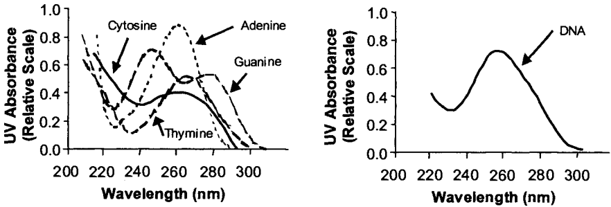
FIGURE 29.2 UV absorbance of nucleotides (left) and nucleic acid (right) at pH 7. (Adapted from Jagger, 1967.)
