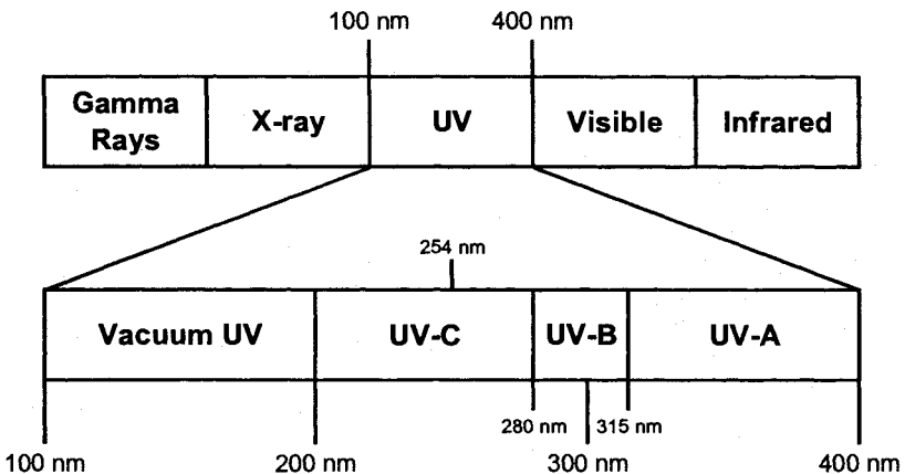
FIGURE 29.1 UV light in the electromagnetic spectrum. (Source: USEPA, 2003a.)
