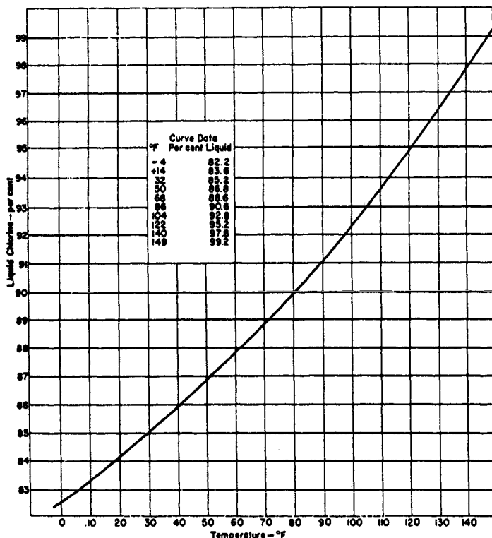
FIGURE A.3 Relationship of volume to temperature in chlorine.
