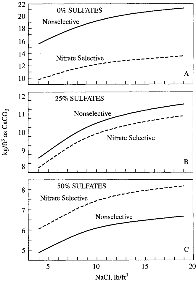
FIGURE 12.5 Removal capacities.
