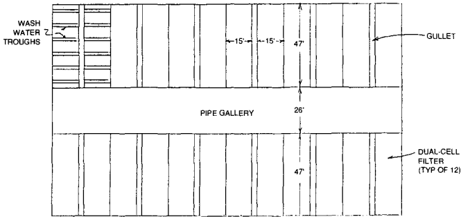
Los Angeles (CA) Aqueduct Water Filtration Plant (300 mgd)
