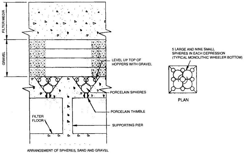
ARRANGEMENT OF SPHERES, SAND AND GRAVEL
