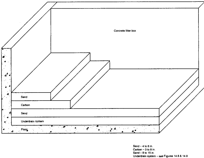
FIGURE 14.11 Media arrangement in a GAC sandwich slow sand filter.
