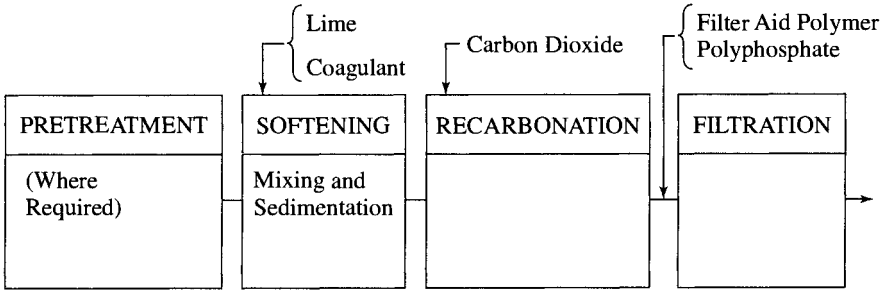
FIGURE 11.1 Single-stage lime process.
