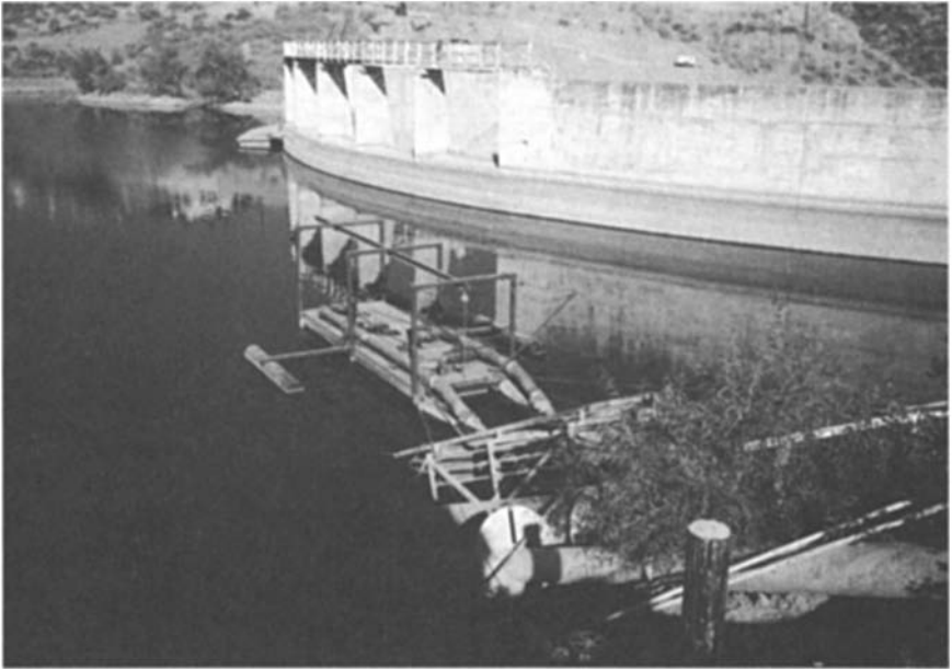
FIGURE 4.10 Floating intakes.
