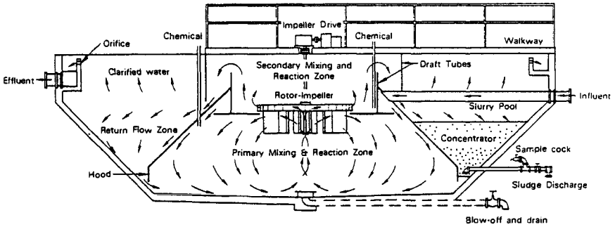
FIGURE 7.18 Accelerator solids contact unit. (Courtesy of Ondeo Degremont.)
