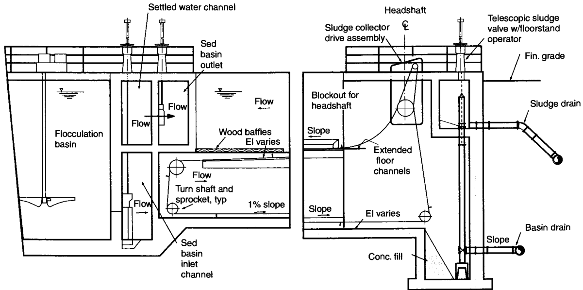
FIGURE 7.2 Two-tray sedimentation basin. (Courtesy of CDM.)
