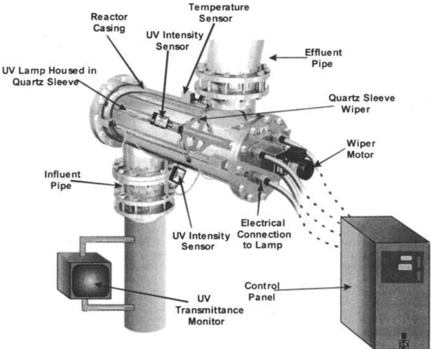
FIGURE 29.4 Schematic of UV disinfection system. (Courtesy of Severn Trent Services.)
