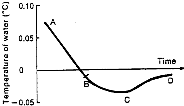
FIGURE 4.15 Frazil ice formation: water temperature sequence.
