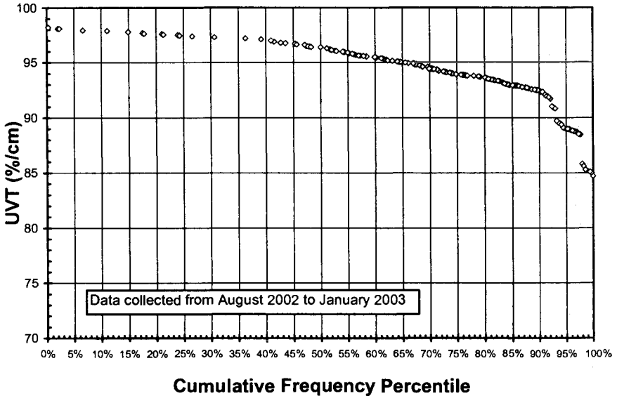
FIGURE 29.10 Example UV transmittance data from sampling program for filtered water from City of Newark, Ohio, WTP. (Photo courtesy of City of Newark, Ohio.)
