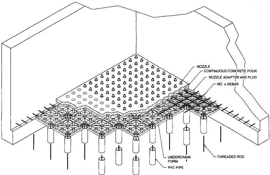
FIGURE 8.17 Underdrain layout. (Courtesy of Ondeo Degremont.)
