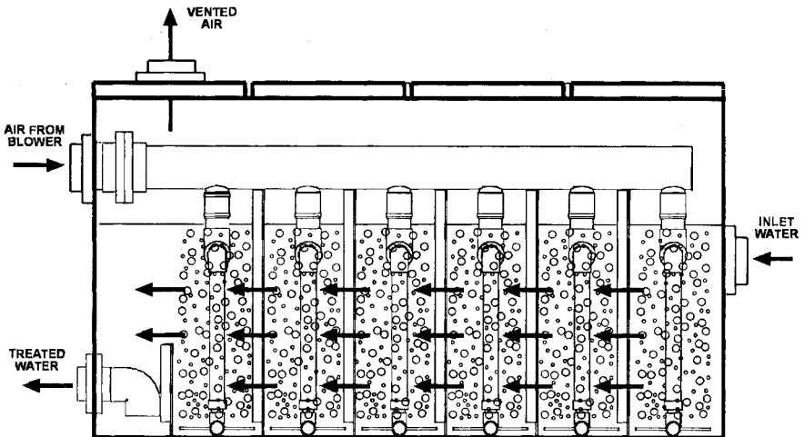
FIGURE 5.3 Schematic of a flow-through low-profile aeration system. (Courtesy of Lowry Aeration Systems.)
