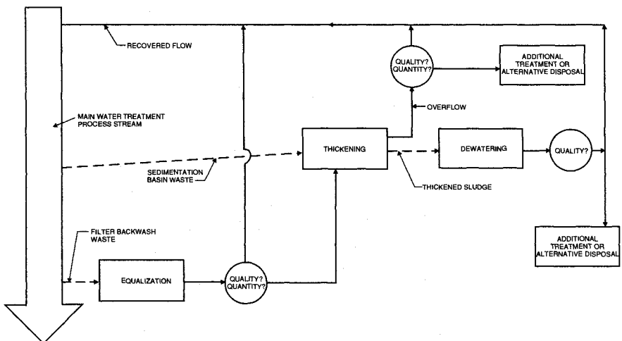
FIGURE 17.30 Concentration and sidestreams.
