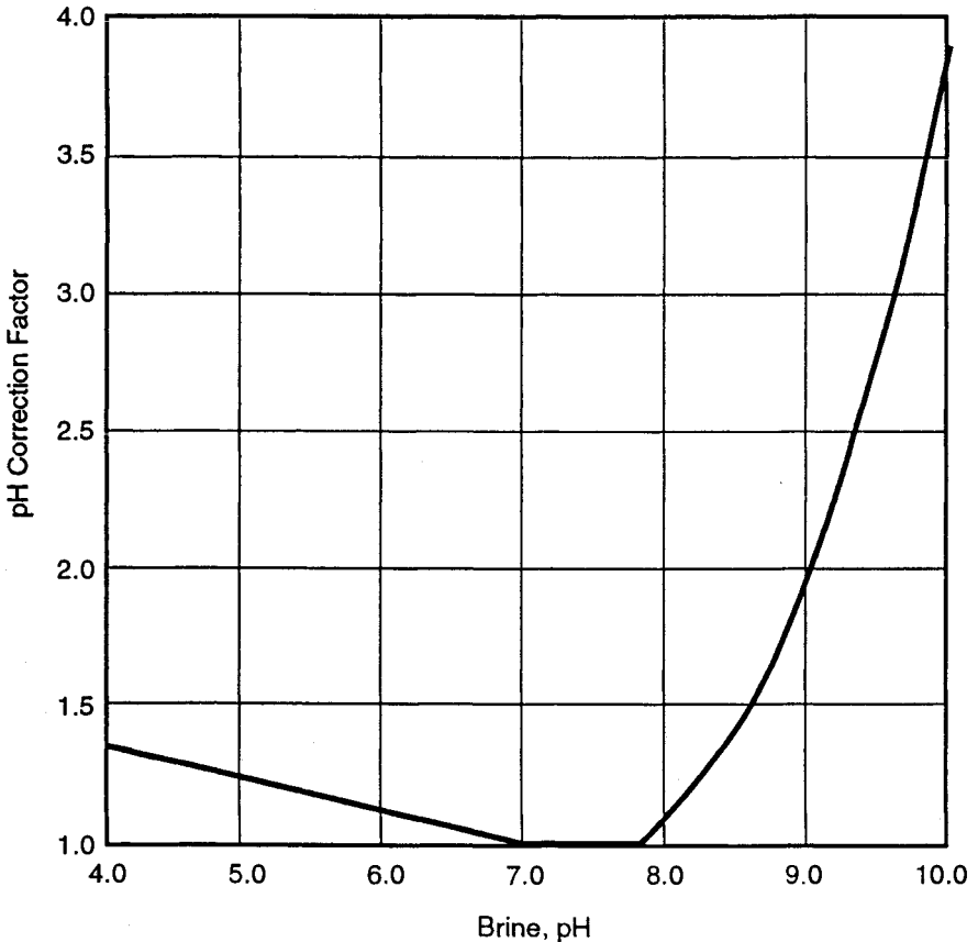
FIGURE 13.18 SiO 2 pH correction factor. (Adapted from DuPont Permasep Products Engineering Manual, 1992.)
