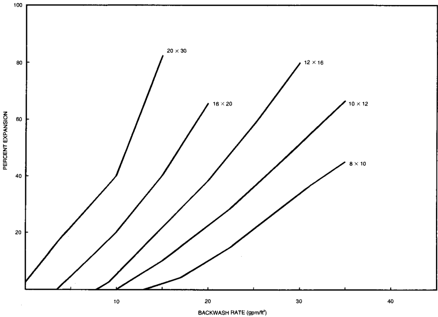
FIGURE 14.5 Backwash characteristics of various mesh sizes at 25° C.
