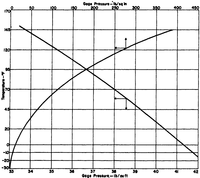
FIGURE A.1 Relationship of pressure-temperature to density-temperature in anhydrous ammonia.
