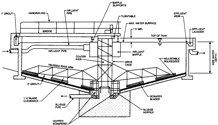
FIGURE 17.7 Gravity thickener section. (Source: U.S. EPA, Process Design Manual: Sludge Treatment and Disposal, 1979.)
