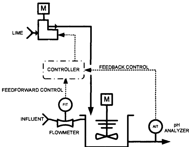
FIGURE 20.5 Compound pH control loop.
