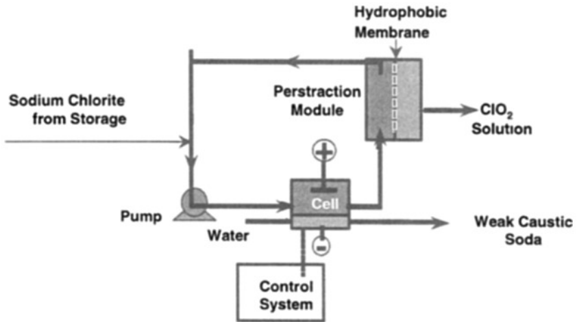
FIGURE 10.17 Electrochemical \text{ClO}_2 .
