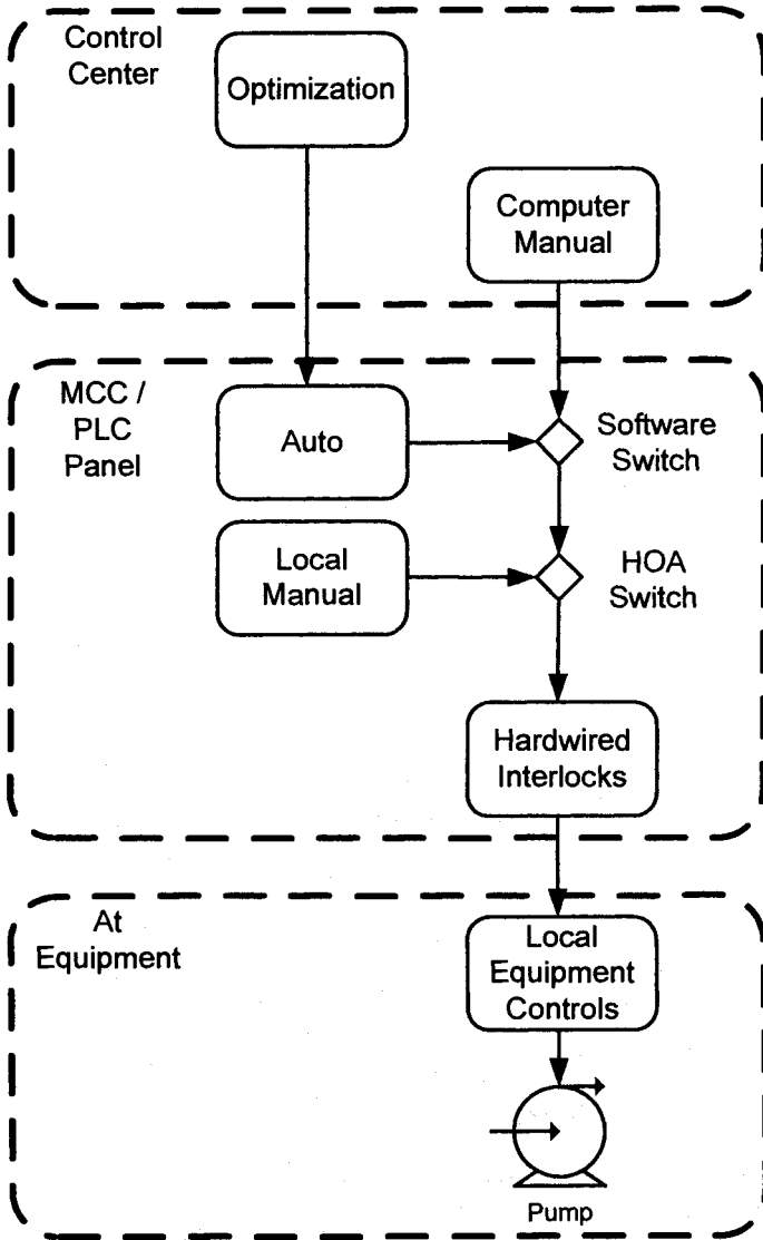
FIGURE 20.1 Example of control hierarchy.
