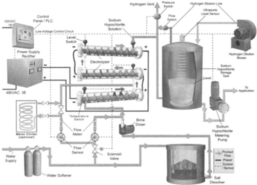
FIGURE 10.11 Schematic of ClorTec™ on-site hypochlorite-generating process. (Courtesy of Severn Trent Services.)
