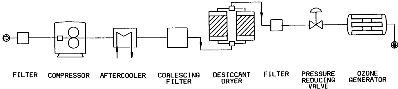
FIGURE 10.24 High-pressure air preparation ozonation system.
