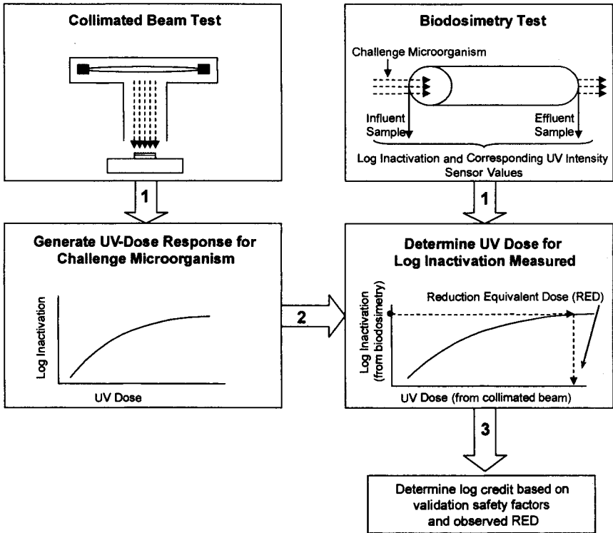
FIGURE 29.14 Biosimetry process. (Adapted from USEPA, 2003a.)
