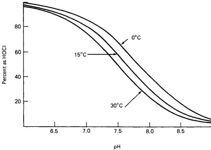
FIGURE 10.6 Influence of pH and temperature on fraction of aqueous chlorine as HOCl.
