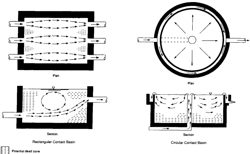
FIGURE 10.2 Examples of poor baffling conditions in basins. (Source: Guidance Manual .)
