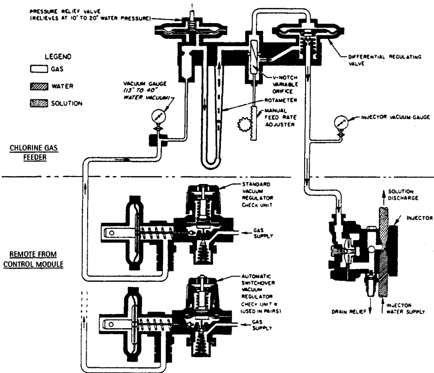
FIGURE 15.7 Flow diagram for conventional chlorinator. (Courtesy of Wallace and Tiernan Division of USFilter.)
