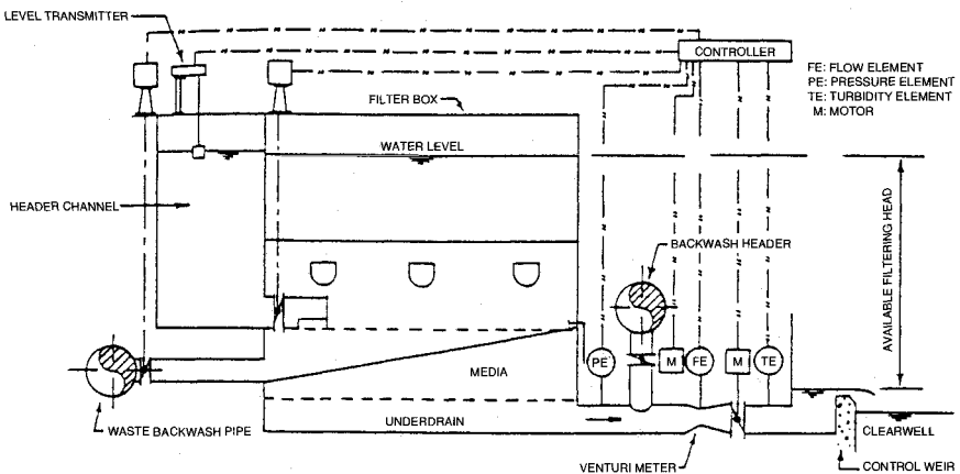
FIGURE 8.2 Constant-rate filter with rate-of-flow controller. (Source: Monk, 1987.)
