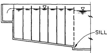
SECTION MAZE FLOCCULATOR
