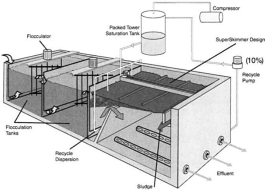
FIGURE 7.21 Typical dissolved air flotation tank. (Courtesy of Parkson Corporation.)
