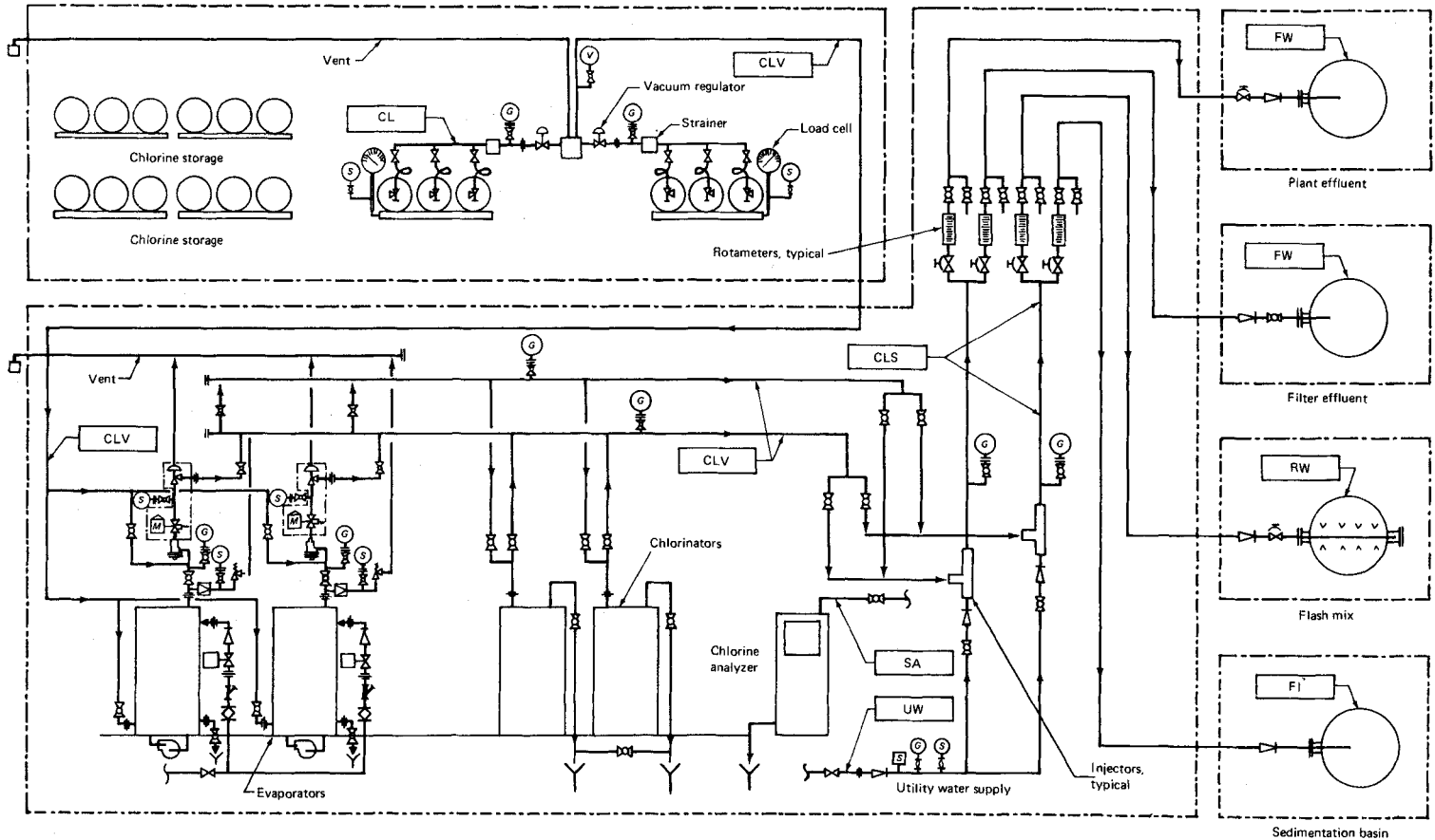
FIGURE 10.8 Chlorine system. CL, chlorine; CLV, chlorine under vacuum; CLS, chlorine solution; SA, sample line; UW, utility water. (Courtesy of MWH Americas Inc.)
