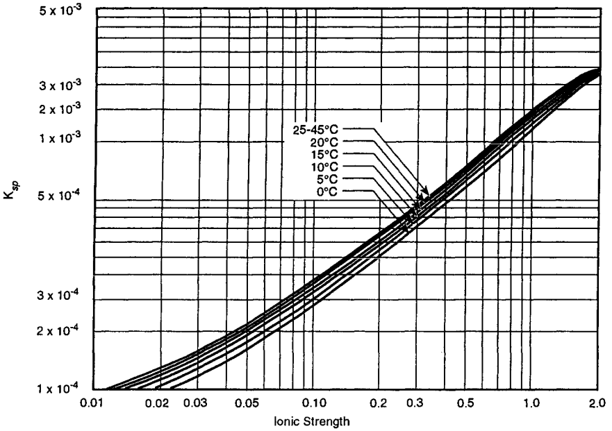
FIGURE 13.15 K_{sp} for \text{CaSO}_4 versus ionic strength. (Adapted from DuPont Permasep Products Engineering Manual, 1992.)
