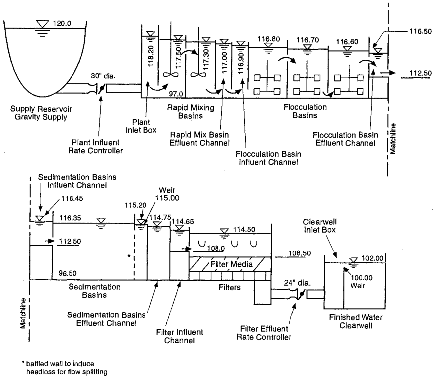
FIGURE 16.1 Typical hydraulic gradeline-maximum day flow (50 MGD) conventional rapid sand filter water treatment plant.
