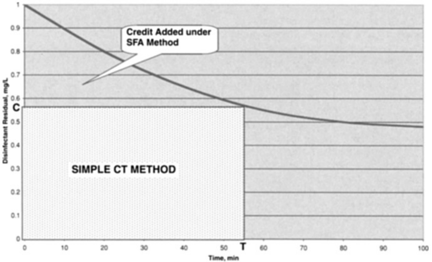
FIGURE 10.1 Disinfection CT .
