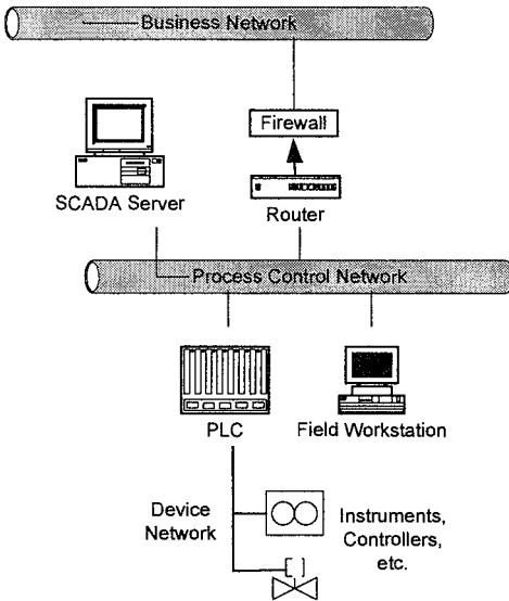
FIGURE 20.10 Treatment plant networks.
