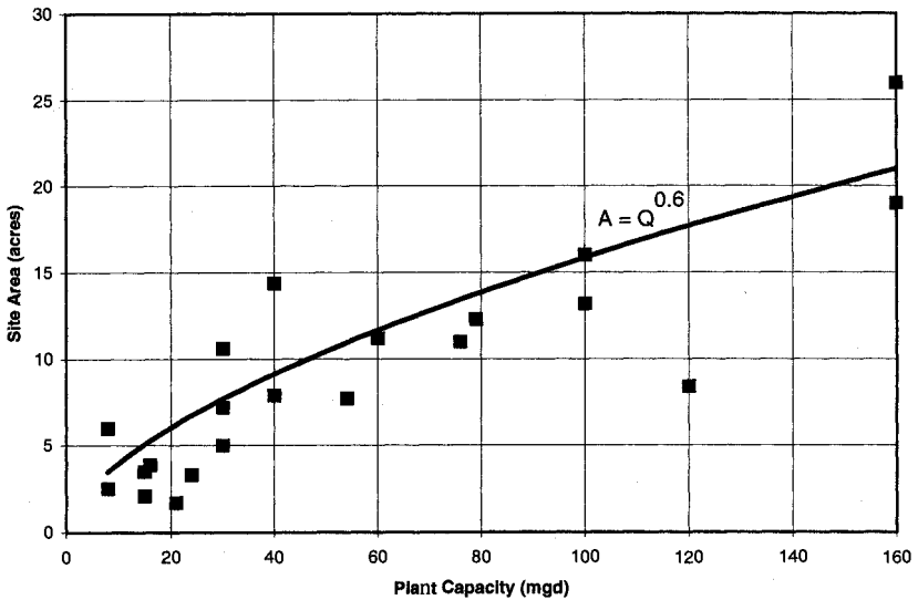
FIGURE 23.1 Minimum site area for conventional treatment plants.
