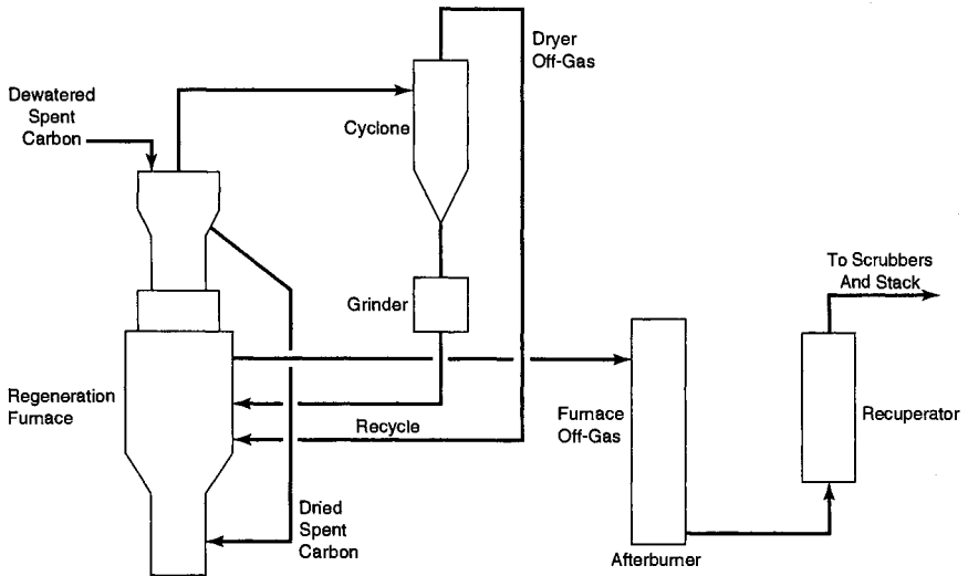
FIGURE 14.14 Activated carbon regeneration system schematic. (Adapted from Westerhoff and Miller, 1986.)
