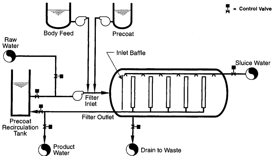
FIGURE 9.16 Pressure system schematic.
