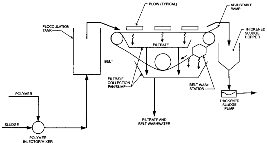
FIGURE 17.9 Gravity belt thickener schematic. (Source: WEF Manual of Practice No. 8, ASCE Manual and Report No. 76, Design of Municipal Wastewater Treatment Plants. Joint Task Force of the Water Environment Federation, Alexandria, Va., and American Society of Civil Engineers, Reston, Va., 1998. Reprinted with permission.)
