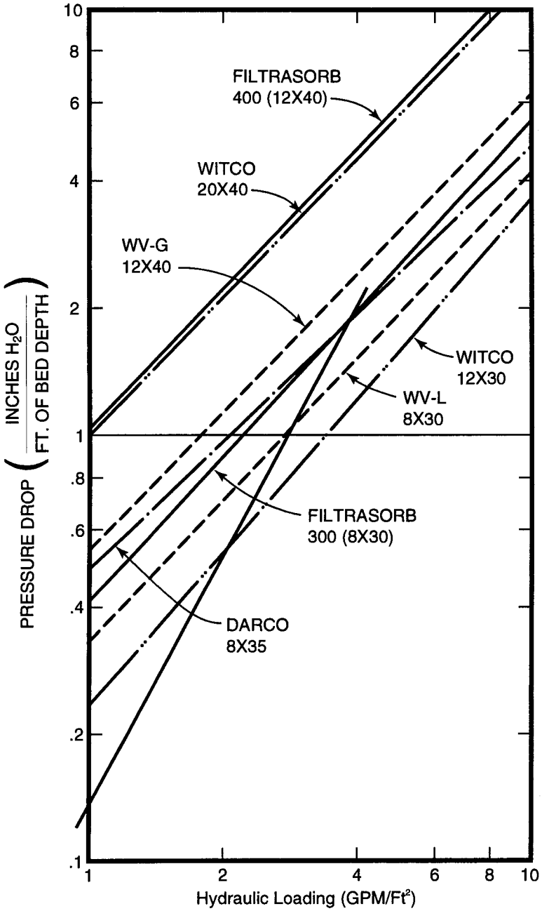
FIGURE 14.4 Carbon bed pressure drop versus hydraulic loading.
