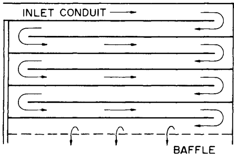
PLAN OF MAZE FLOCCULATOR
