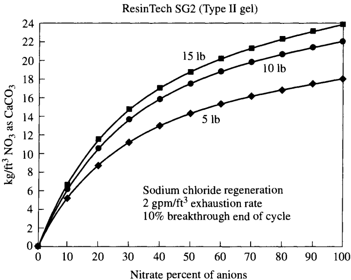
FIGURE 12.2 Nitrate removal capacity.
