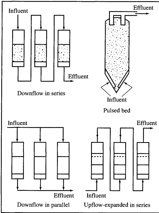
FIGURE 14.12 Commonly used GAC contactor configurations.
