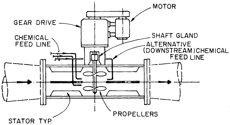
FIGURE 6.5 Typical in-line blender (mixer).
