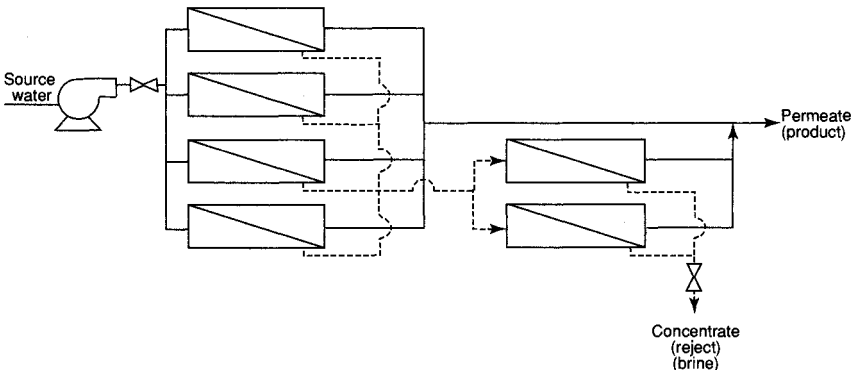
FIGURE 13.20 Concentrate staging (two-stage design shown).
