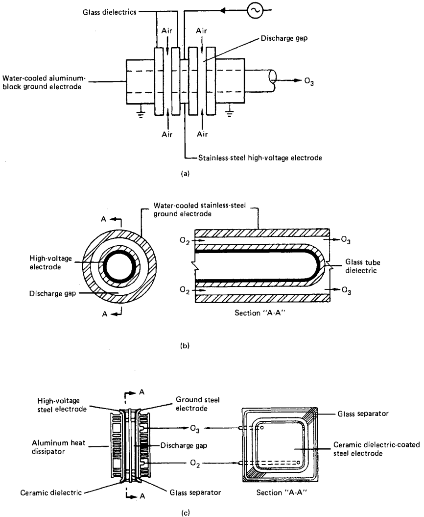
FIGURE 10.21 Alternative ozonator configurations. (a) Otto plate-type generator unit; (b) tube-type generator unit; (c) Lowther plate generator unit. [Source: H. Rosen, "Ozone Generation and Its Relationship to the Economical Application of Ozone in Wastewater Treatment," in F. L. Evans III (ed.), Ozone in Water and Wastewater Treatment , Ann Arbor Science Publishers, Ann Arbor, Mich., 1972.]
