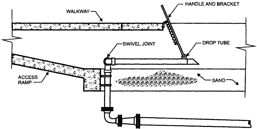
FIGURE 17.15 Lagoon decant structure.
