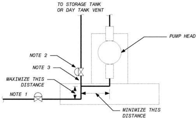
FIGURE 10.10 Metering pump suction piping detail. Notes: (1) Sodium hypochlorite metering pump suction piping shall be routed to slope continuously downward from the day/bulk storage tank. (2) Valve shall remain open except when day/bulk storage tank level is below the pump centerline. (3) Locate tee for vent as close as possible to pump suction connection. The vent piping shall be connected to the run of the tee in the vertical position. Vent piping shall not be connected to the branch of the tee.
