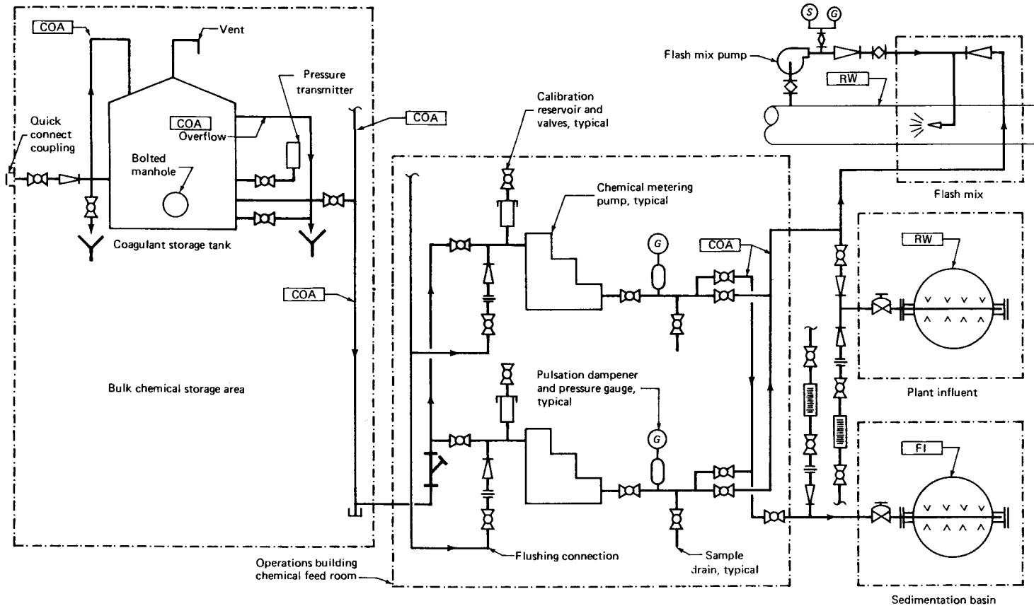
FIGURE 15.3 Coagulant alum/ferric chloride system. (Courtesy of MWH Americas Inc.)
