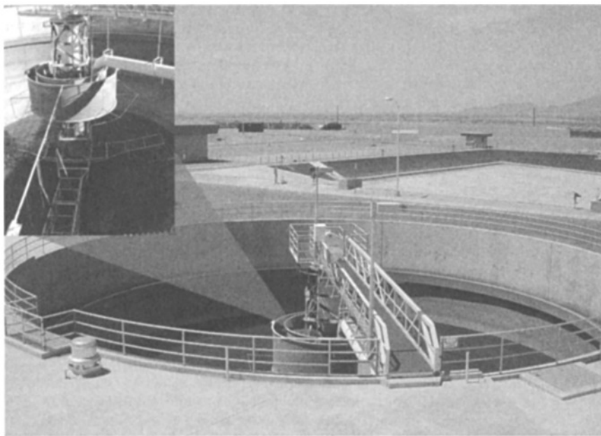
FIGURE 17.8 Gravity thickener. (Courtesy of City of Phoenix Water Services Department.)
