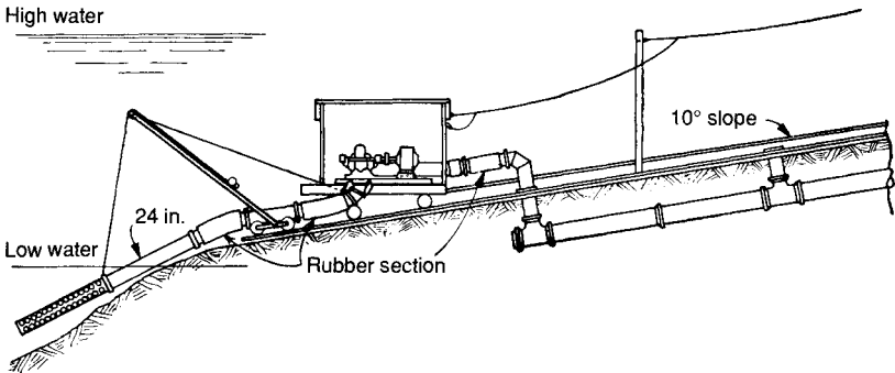
FIGURE 4.11 Intake pump on movable carriage.
