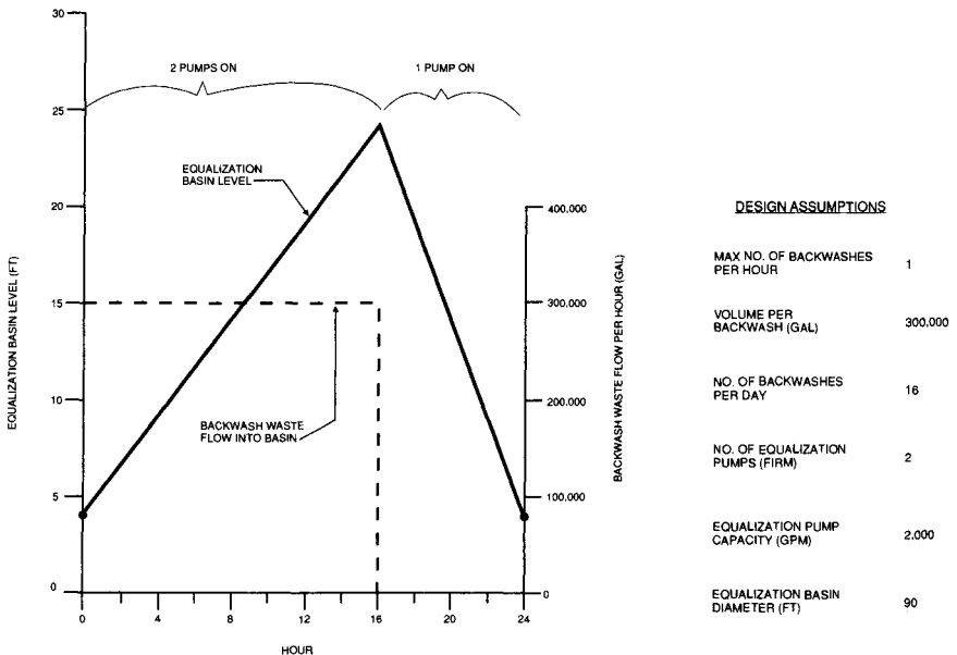
FIGURE 17.5 Equalization storage curve.
