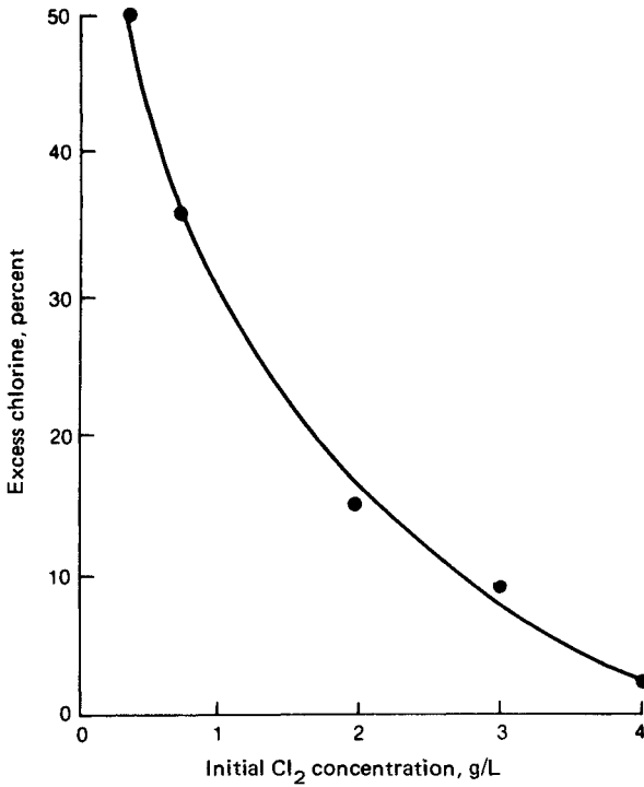
FIGURE 10.14 Excess chlorine necessary for greater than 95% conversion of chlorite to chlorine dioxide. (Source: M. Aieta and J. Berg, "A Review of Chlorine Dioxide to Drinking Water Treatment," Journal AWWA, vol. 78, no. 6, June 1986, p. 62.)
