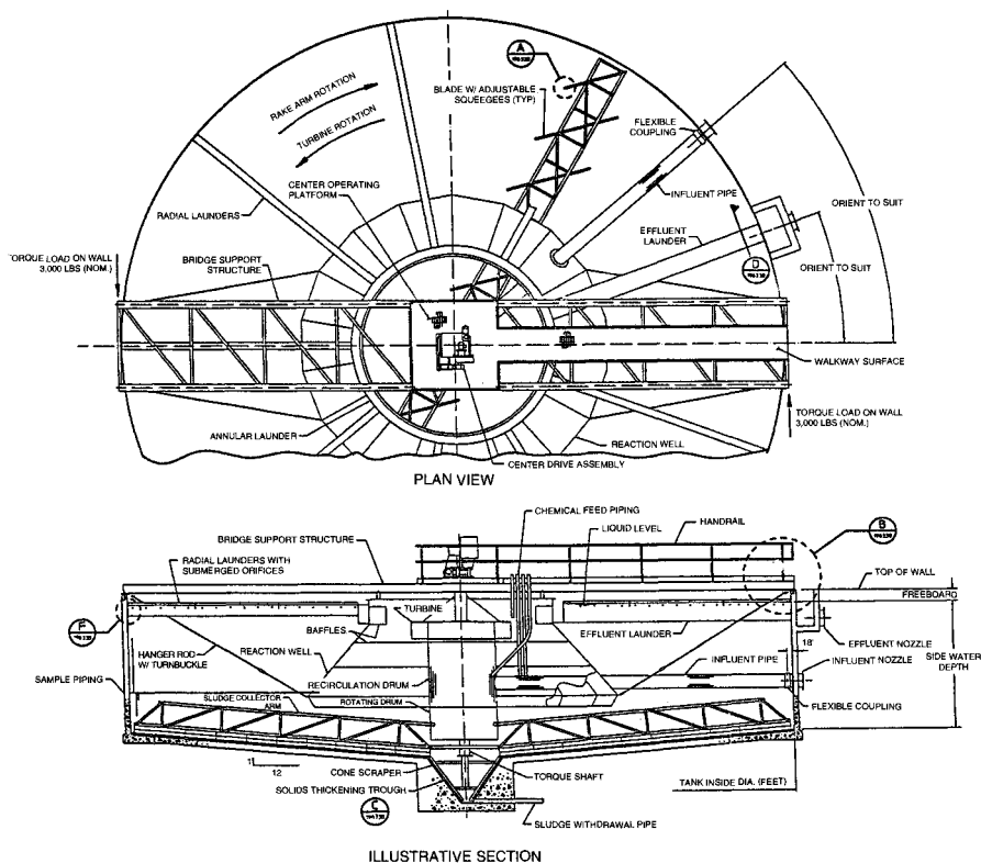
FIGURE 7.17 Typical solids contact slurry recirculation unit. (Courtesy of Eimco Water Technologies.)
