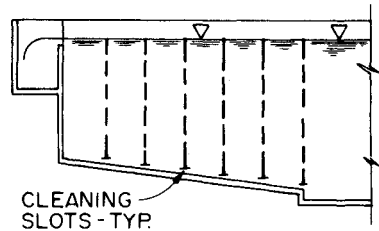
SECTION BAFFLE FLOCCULATOR
