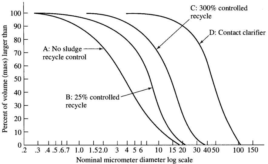
FIGURE 11.4 Particle size distribution comparison.
