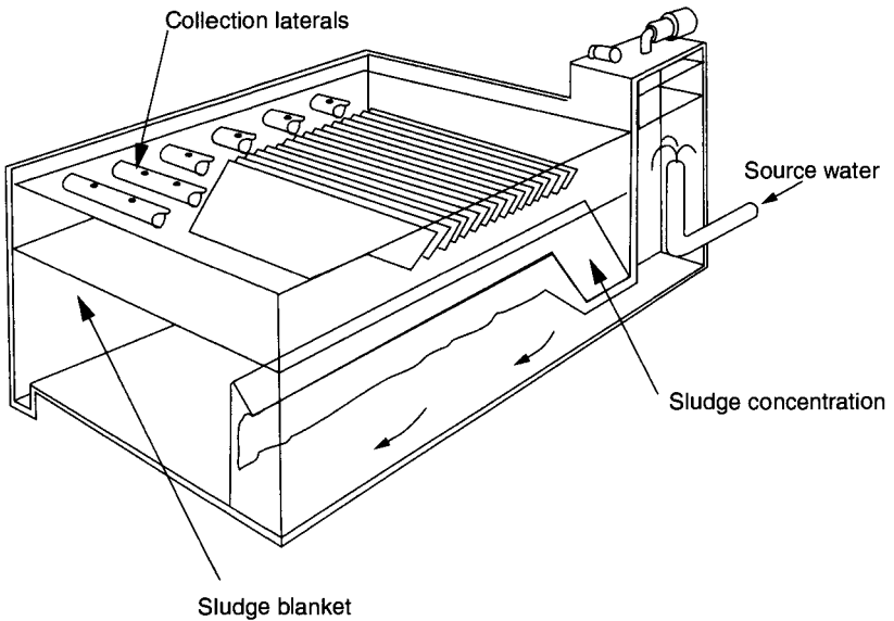
FIGURE 7.20 Cross section of the Superpulsator sludge blanket clarifier. (Courtesy of Ondeo Degremont.)
