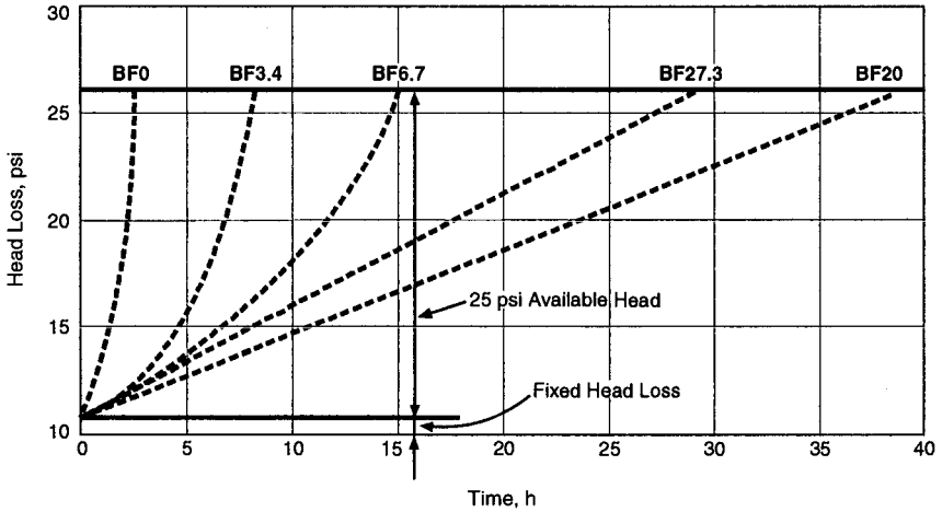
FIGURE 9.8 Effect of varying body feed addition.
