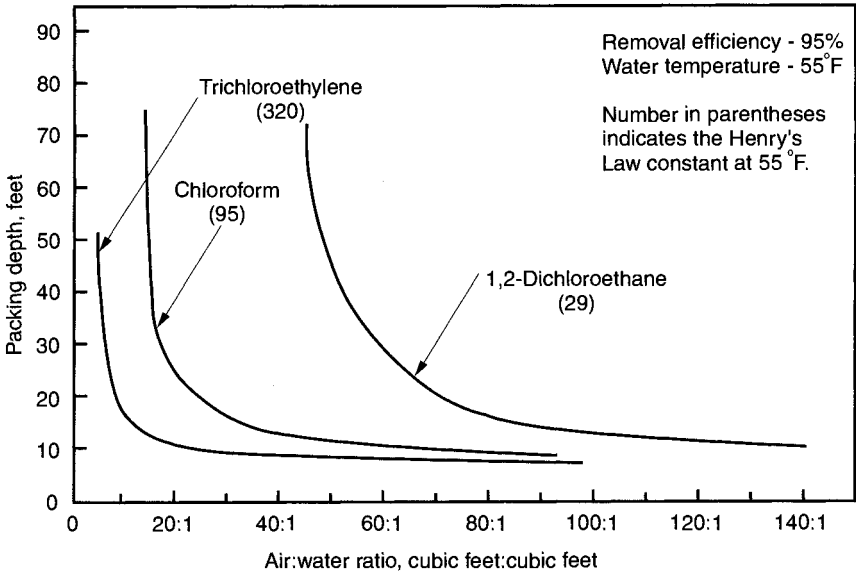
FIGURE 5.5 Effect of type of VOC on packed column design. (Source: AWWARF/KIWA Report, 1983.)
