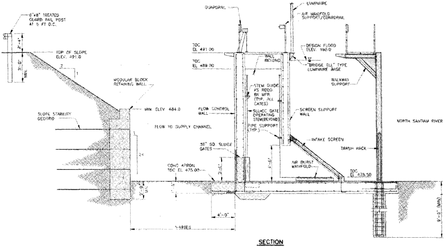
FIGURE 4.18 Concrete intake structure including fish protection system.
