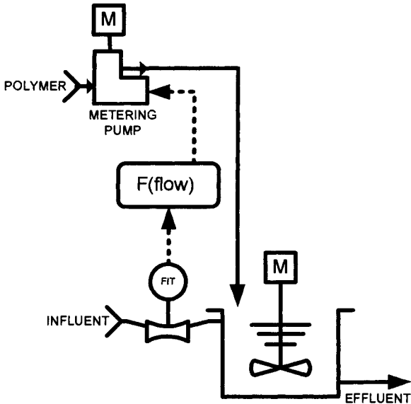
FIGURE 20.2 Feedforward control example: polymer dosing.
