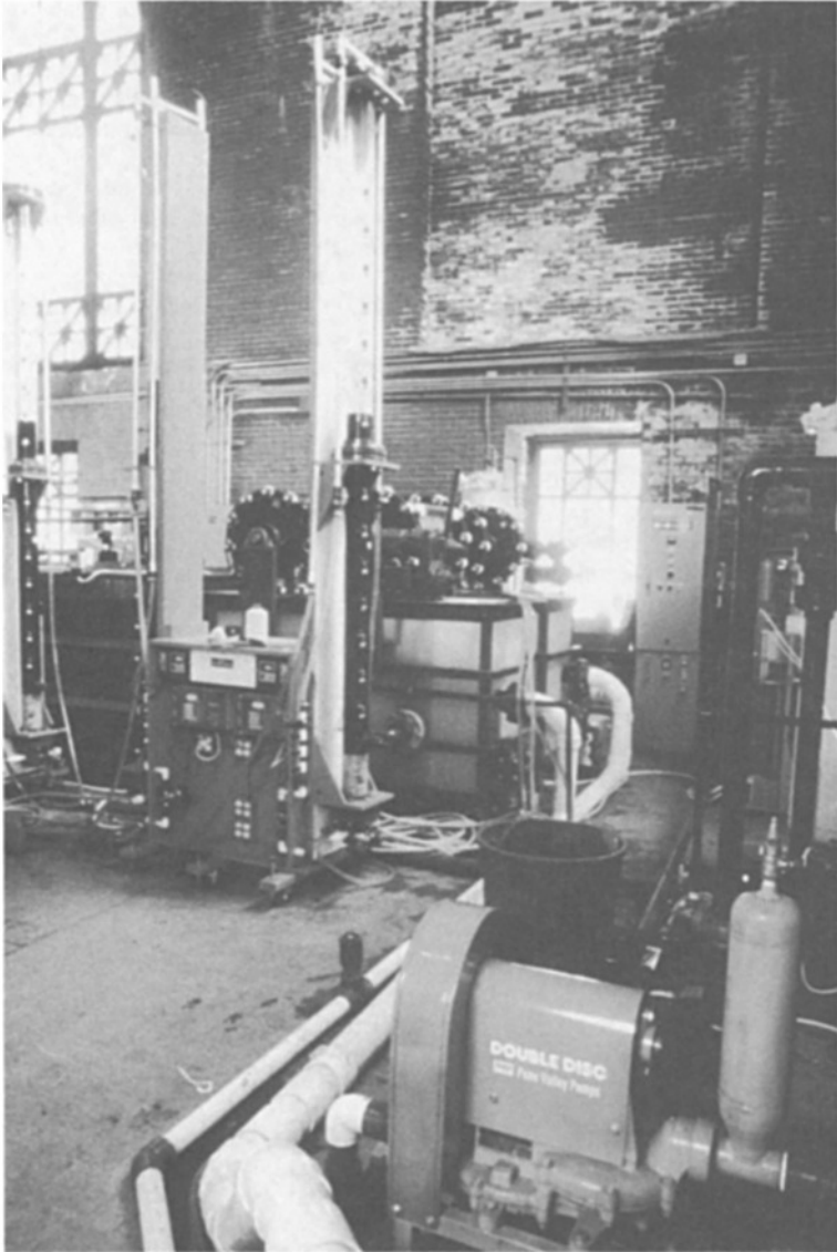
FIGURE 28.5 Mobile field plant modules with filter assembly units mounted on casters, complete with filter, flow controls, turbidimeter, and head loss monitoring. (Courtesy of CDM.)
