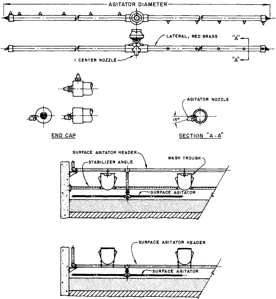
FIGURE 8.7 Typical surface agitator and arrangements. (Source: F. B. Leopold Co., Inc.)
