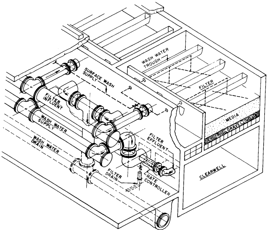
FIGURE 8.18 Typical gravity filter piping. (Courtesy of CDM.)
