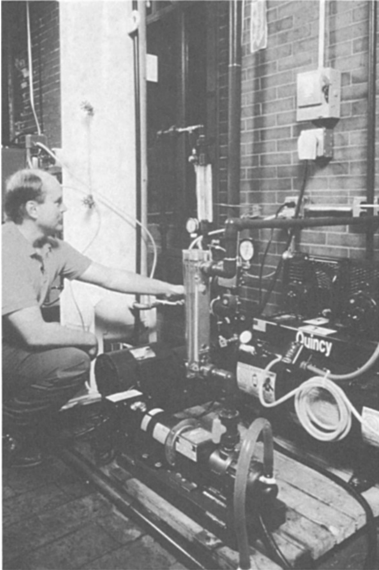
FIGURE 28.3 Author shown adjusting flow to a DAF recycle stream pump adjusted manually based on data from flowmeters and pressure gauges. (Courtesy of CDM.)
