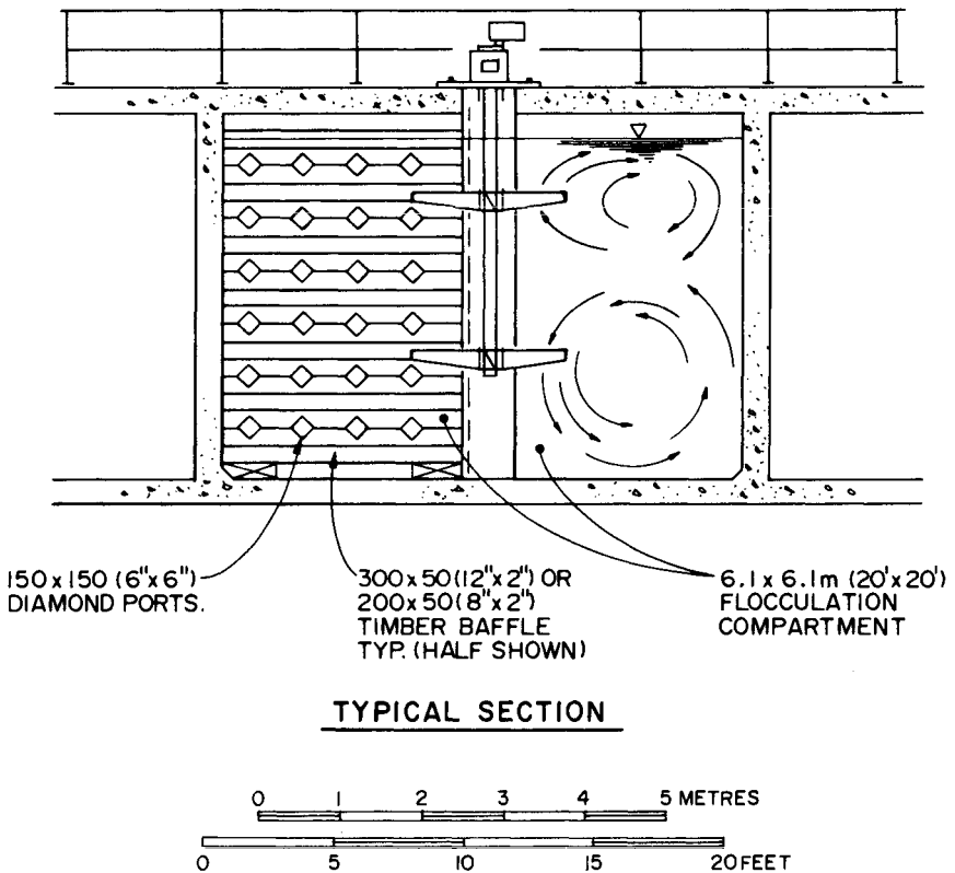
FIGURE 6.9 Vertical paddle flocculator compartment.
