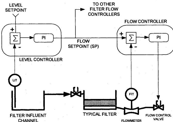
FIGURE 20.6 Example of cascade level/flow control.
