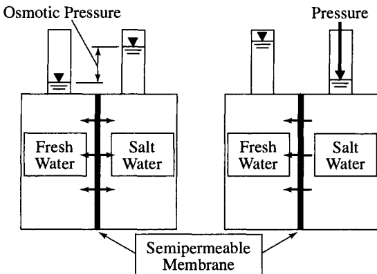
FIGURE 13.8 Simplified concept of osmosis and reverse osmosis.
