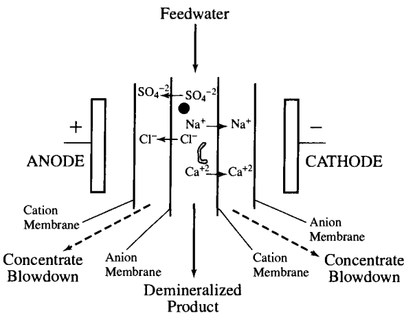
FIGURE 13.3 Voltage-driven electrodialysis process.
