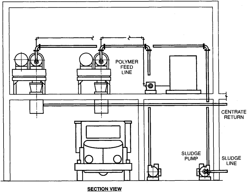
FIGURE 17.23 Typical centrifuge layout. (Source: AWWARF Handbook of Water Treatment Plant Waste Management.)
