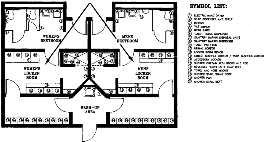
FIGURE 18.2 Locker room, toilet, and shower room plan.
