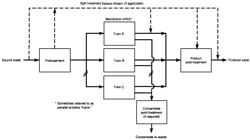
FIGURE 13.9 Typical membrane system flow schematic.
