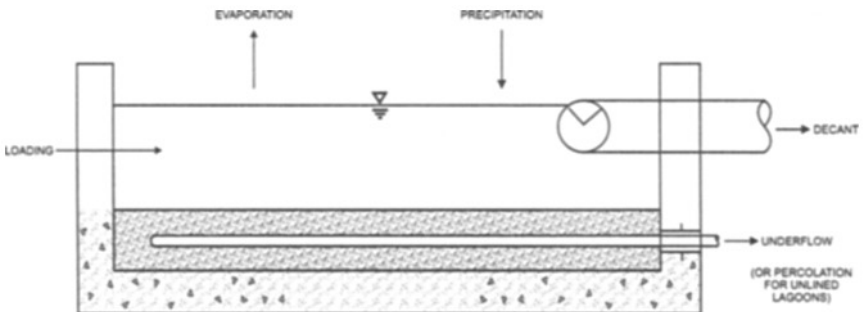
FIGURE 17.10 Natural dewatering sizing parameters.
