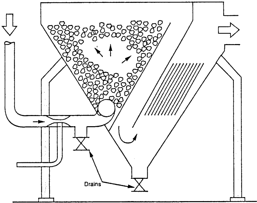
FIGURE 6.13 Upflow gravel bed flocculator. (Source: Schulz et al., 1994.)
