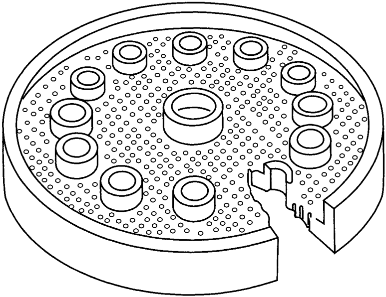
Orifice-type distributor
