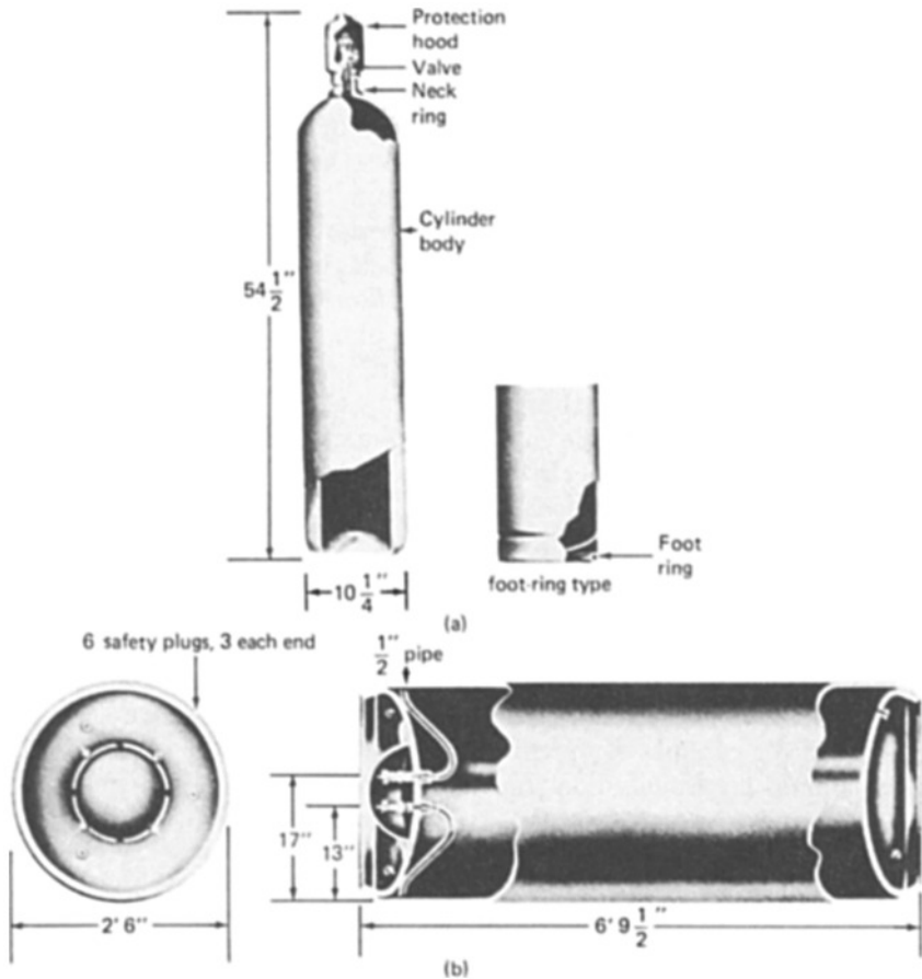
FIGURE 15.1 Dimensions of standard chlorine cylinders. (a) A 150-lb cylinder. (Courtesy of PPG Industries, Inc., Pittsburgh, Pa.) (b) A 1-ton cylinder. (Courtesy of the Chlorine Institute, Inc.)
