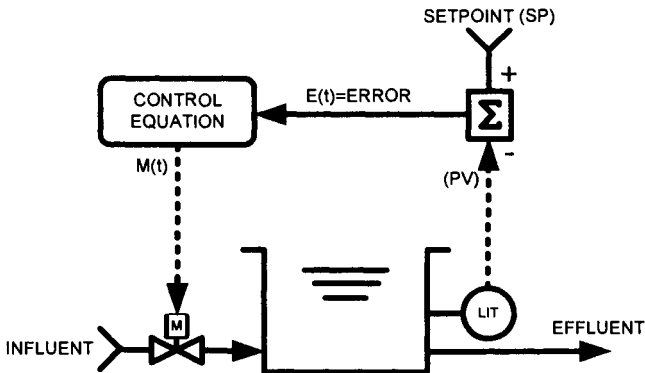
FIGURE 20.3 Feedback control example: tank level control.
