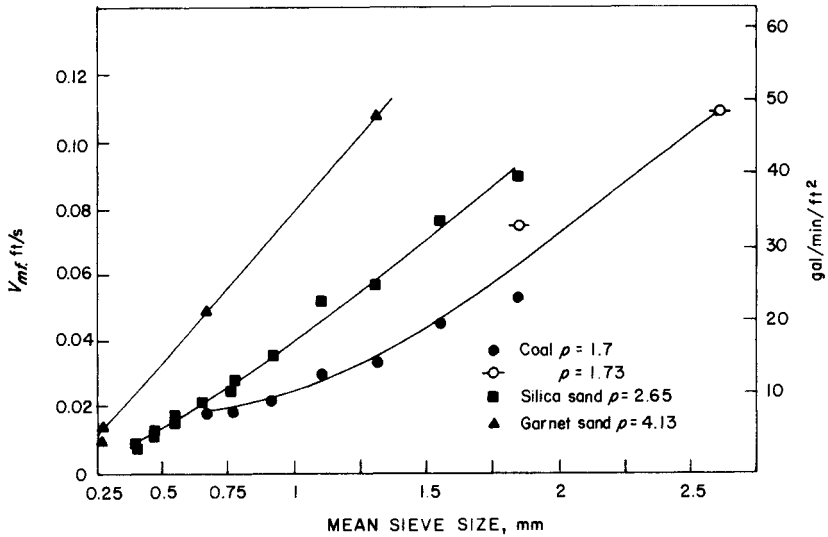
FIGURE 8.8 Minimum fluidization velocity V_{mf} needed to achieve 10% bed expansion at 25° C. (Source: Cleasby and Baumann, 1974.)
