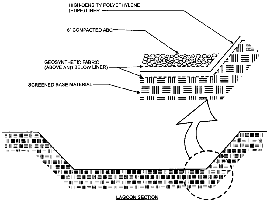
FIGURE 17.14 Lagoon lining profile.
