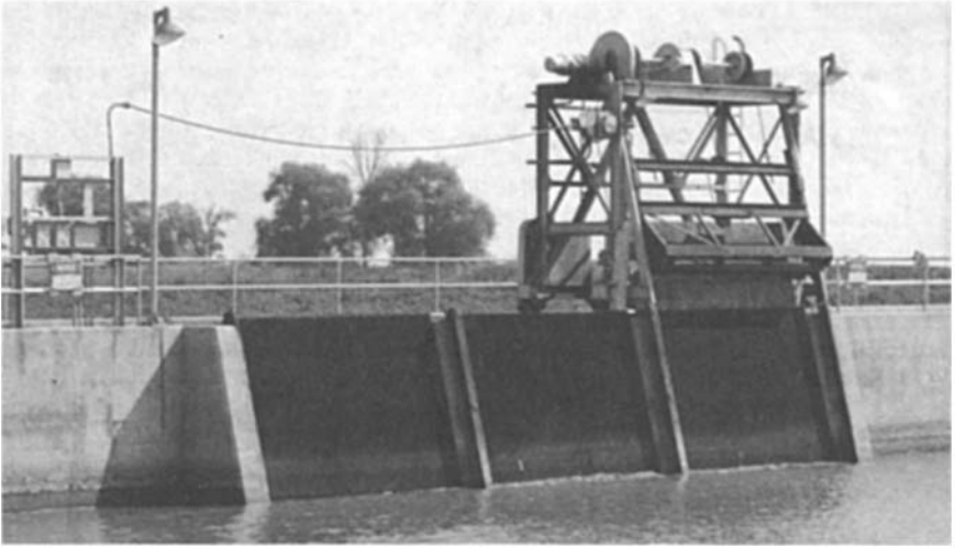
FIGURE 4.19 Course bar screen, mechanically cleaned.
