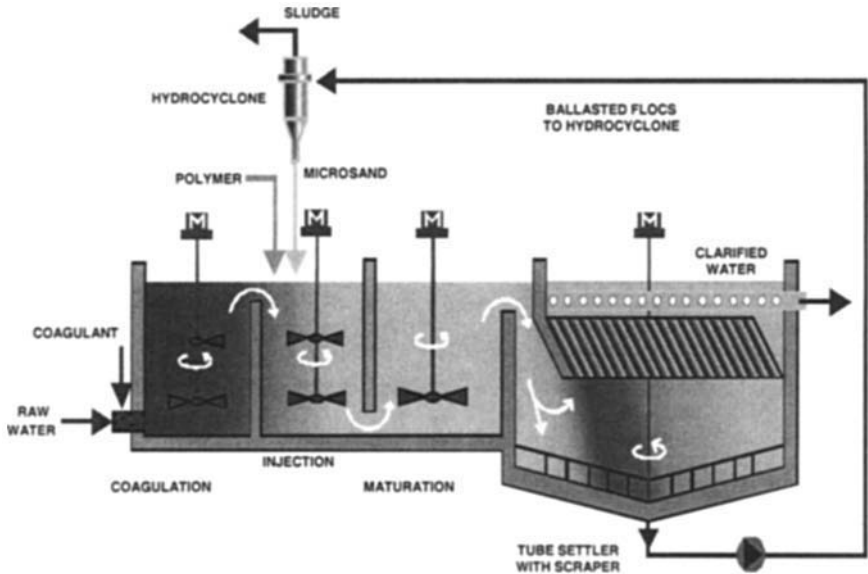
FIGURE 7.14 ACTIFLO process for water treatment. (Courtesy of Kruger Inc.)
