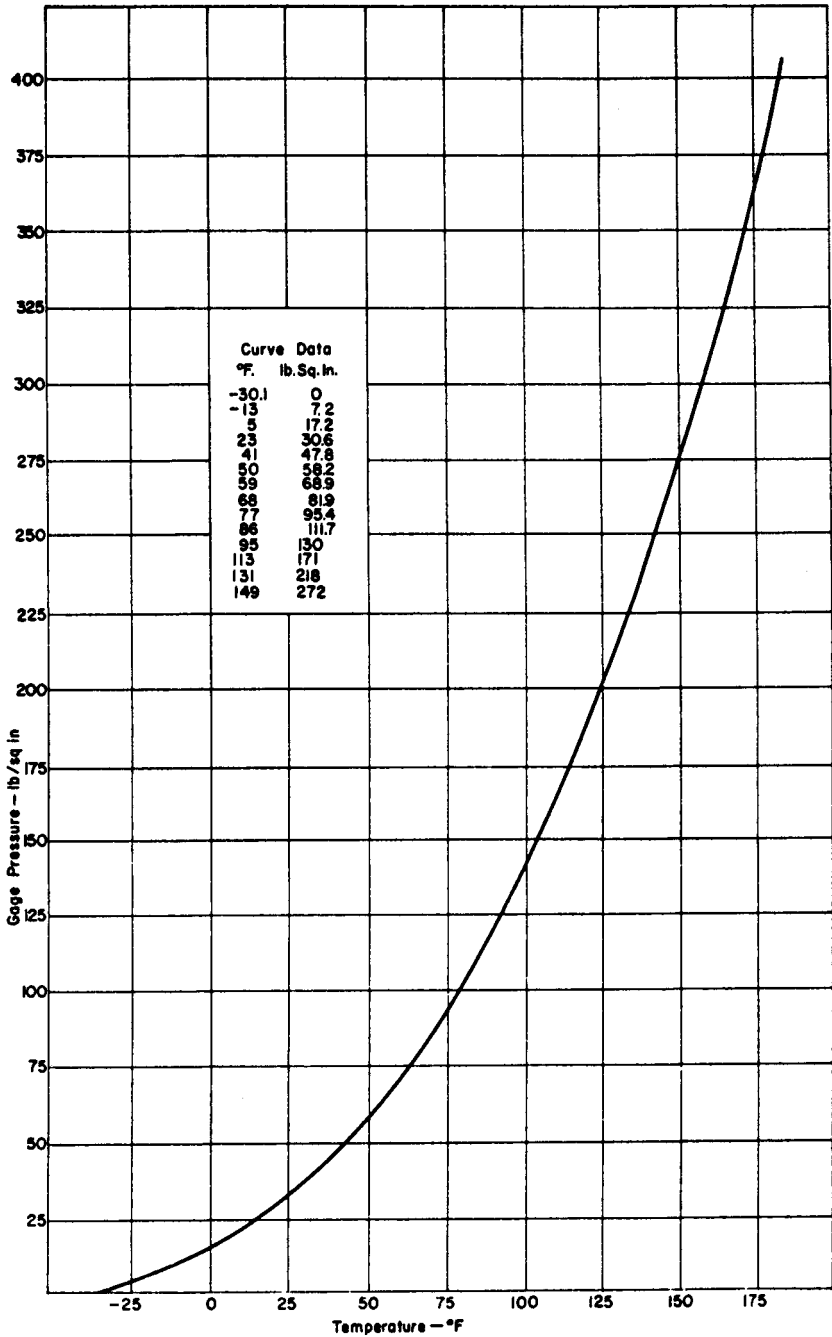
FIGURE A.2 Relationship of temperature to pressure in chlorine.
