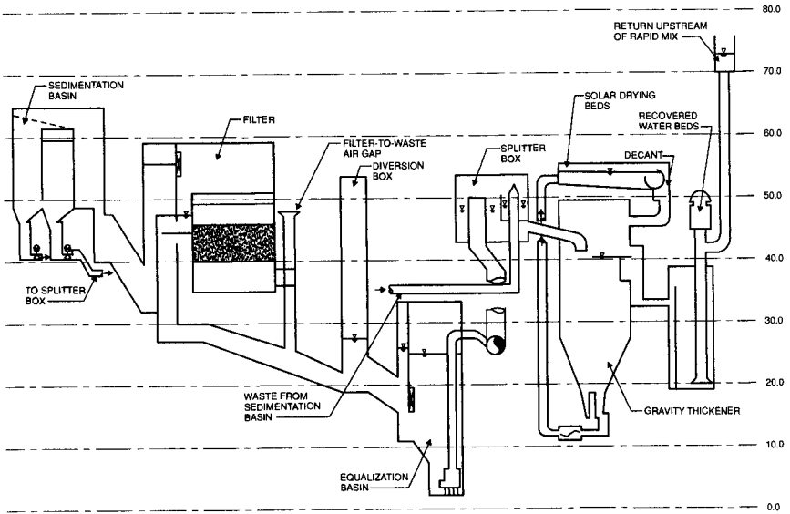
FIGURE 17.32 Waste handling system hydraulic profile. (Courtesy of City of Phoenix Water Services Department.)
