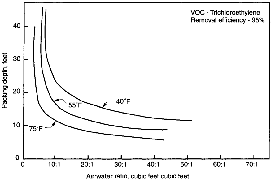
FIGURE 5.7 Effect of water temperature on packed column design. (Source: AWWARF/KIWA Report, 1983.)
