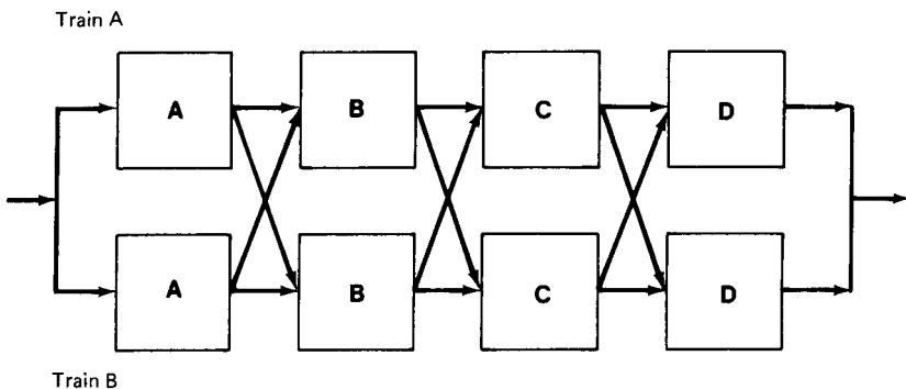
FIGURE 22.4 Interconnected parallel production trains minimize impact of single unit failure.
