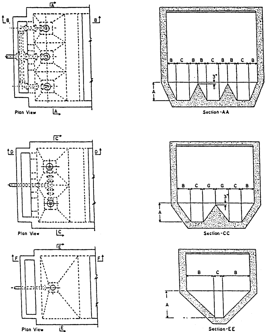
FIGURE 7.7 Typical sludge hopper arrangements for rectangular basins.
