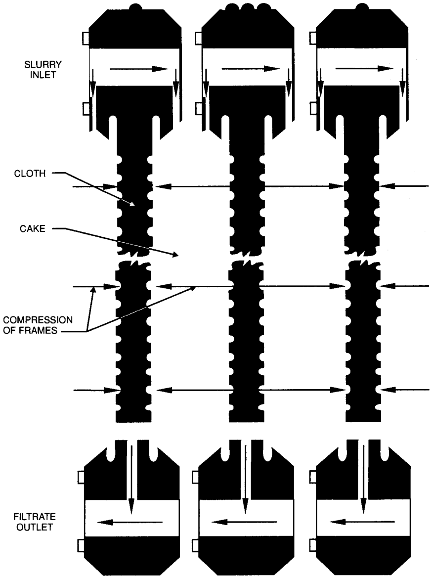
FIGURE 17.18 Dewatering mechanism of plate and frame filter press. (Courtesy of Eimco Water Technologies.)
