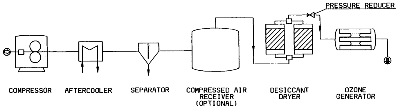
FIGURE 10.23 Medium-pressure air preparation ozonation system.
