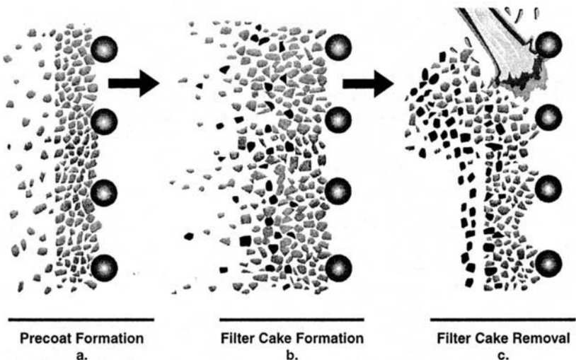
FIGURE 9.7 Precoat filtration cycles.
