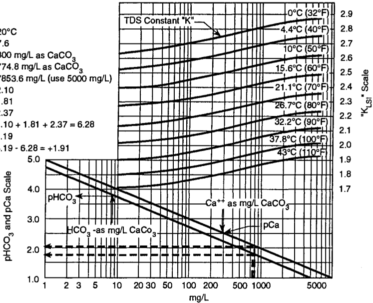
FIGURE 13.13 Langelier saturation index. (Adapted from DuPont Permasep Products Engineering Manual, 1992.)
