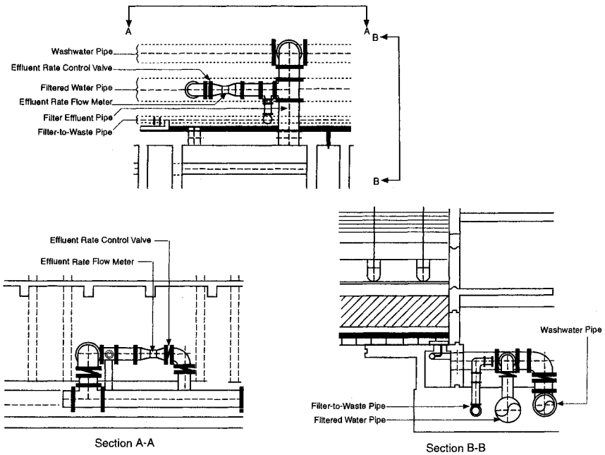
FIGURE 16.2 Typical filter effluent piping.
