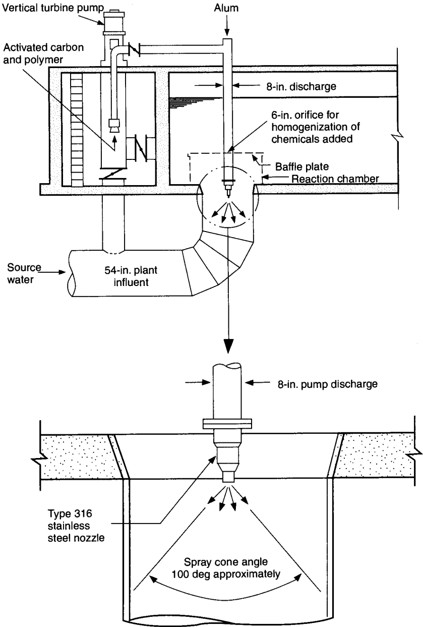
FIGURE 6.3 Flash mixing facility. (After Kawamura, 1976.)
