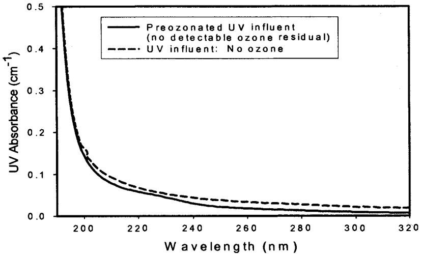
FIGURE 29.6 Example effect of preozonation on UV absorbance if ozone is quenched prior to UV disinfection. (Source: Malley, 2002.)
