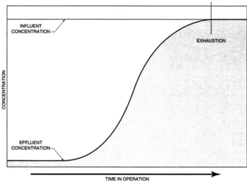
FIGURE 14.3 Typical breakthrough pattern for GAC filter.
