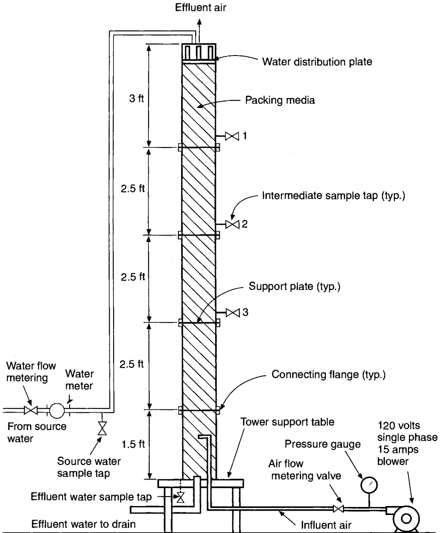
FIGURE 5.12 Schematic of a pilot air stripping column. (Source: USEPA technologies for upgrading existing or designing new drinking water treatment facilities, 1990.)
