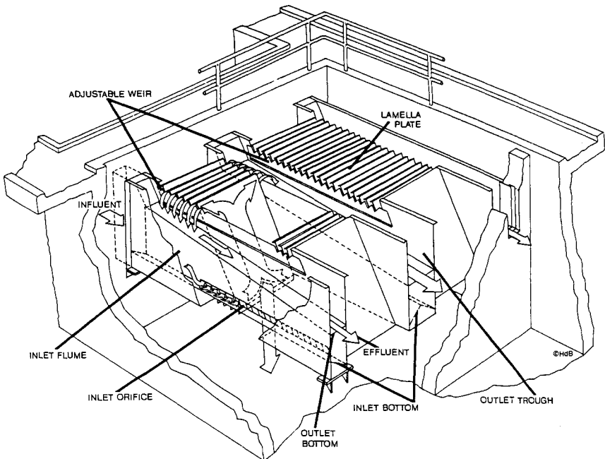
FIGURE 7.15 Plate settlers. (Courtesy of Parkson Corporation.)
