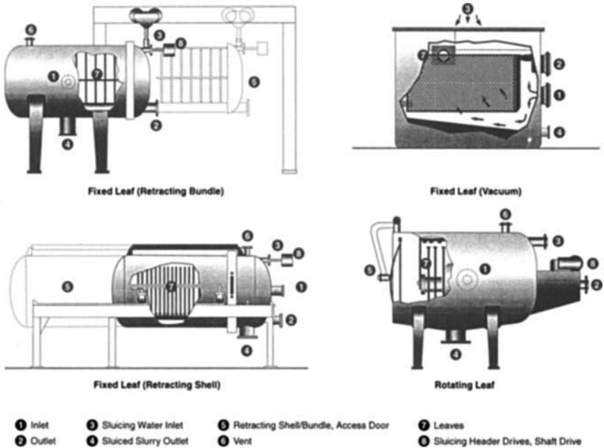
FIGURE 9.11 Common vertical leaf filters.
