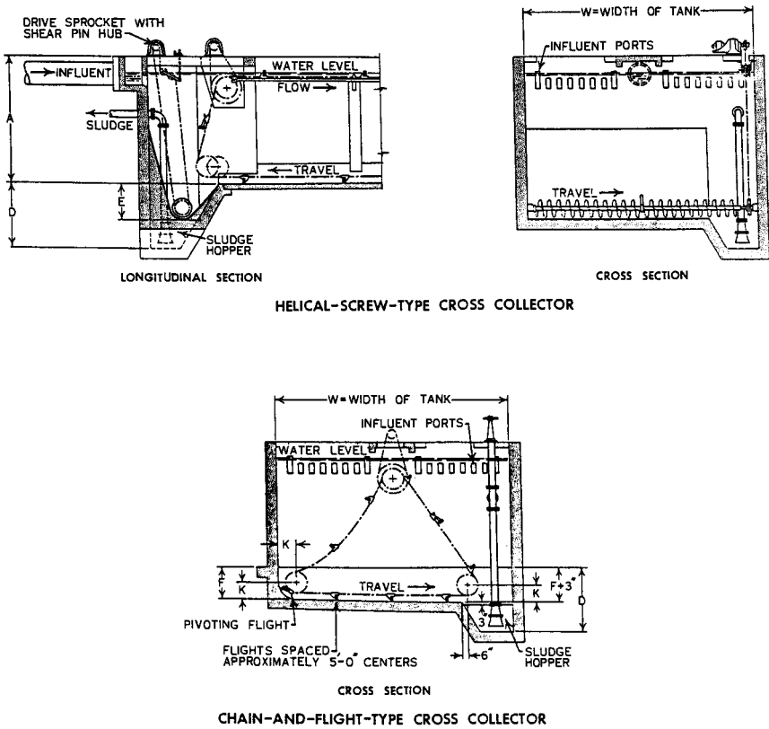
FIGURE 7.6 Typical cross-collector arrangements. (Courtesy of USFilter, Envirex Products.)
