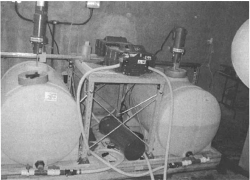
FIGURE 29.12 Equipment skid for on-site validation testing. (Photo courtesy of Clayton County, Ga., Water Authority.)
