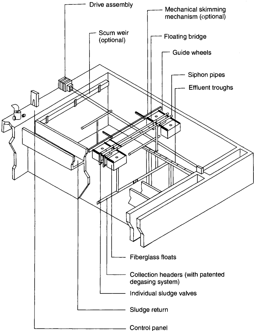
FIGURE 7.10 Floating bridge-type collector. (Courtesy of Leopold.)
