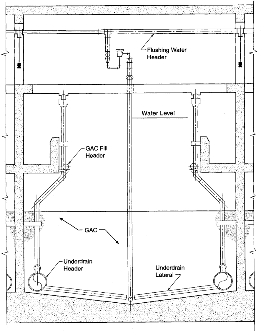
FIGURE 14.13 Cross section through a typical, open-top concrete, rectangular, gravity flow GAC contactor. (Adapted from Westerhoff and Miller, 1986.)
