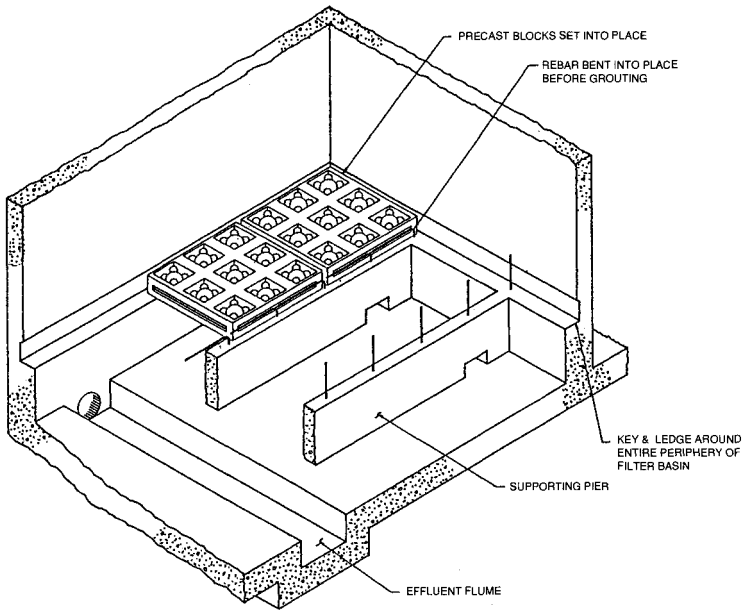
PRECAST WHEELER BOTTOM
