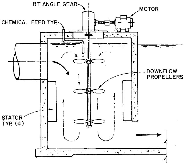
FIGURE 6.1 Propeller-type mechanical flash mixer.
