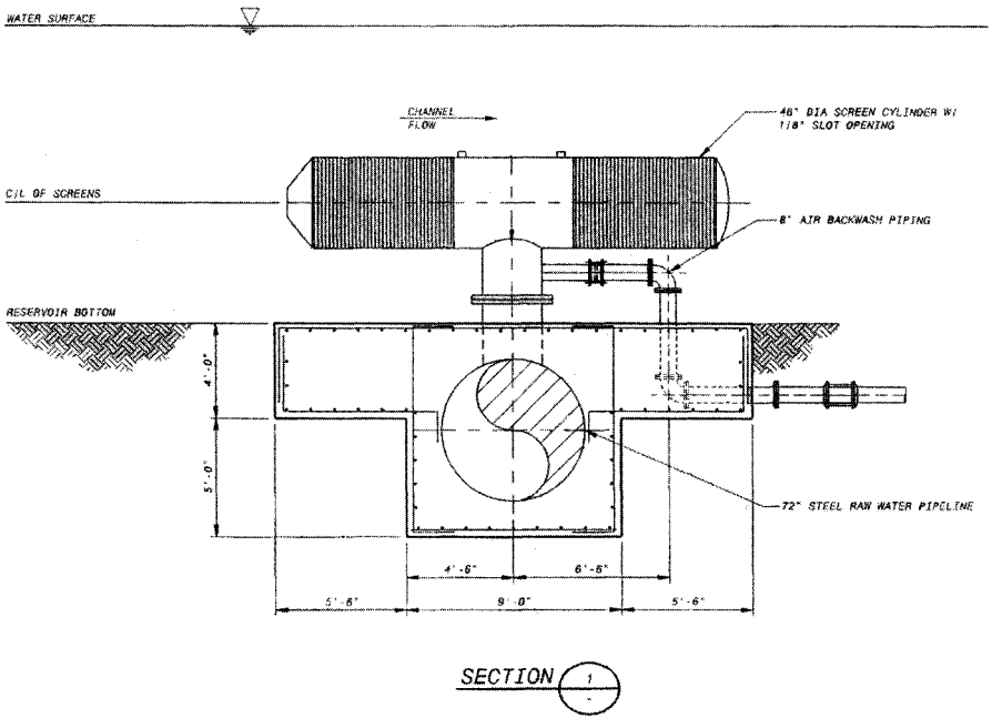
FIGURE 4.9 Submerged intake screens.
