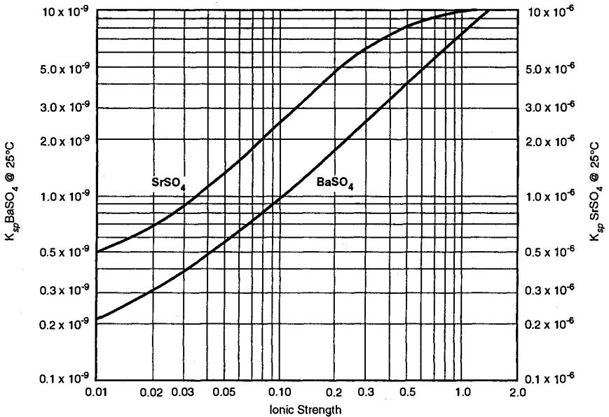
FIGURE 13.16 K_{sp} for \text{BaSO}_4 and \text{SrSO}_4 versus ionic strength. (Adapted from DuPont Permasep Products Engineering Manual, 1992.)
