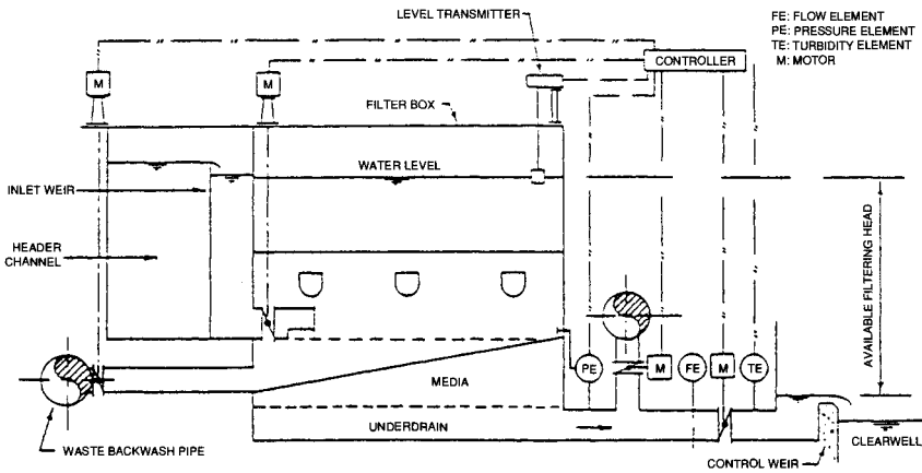
FIGURE 8.3 Constant-rate filter with influent splitting and constant water level. (Source: Monk, 1987.)
