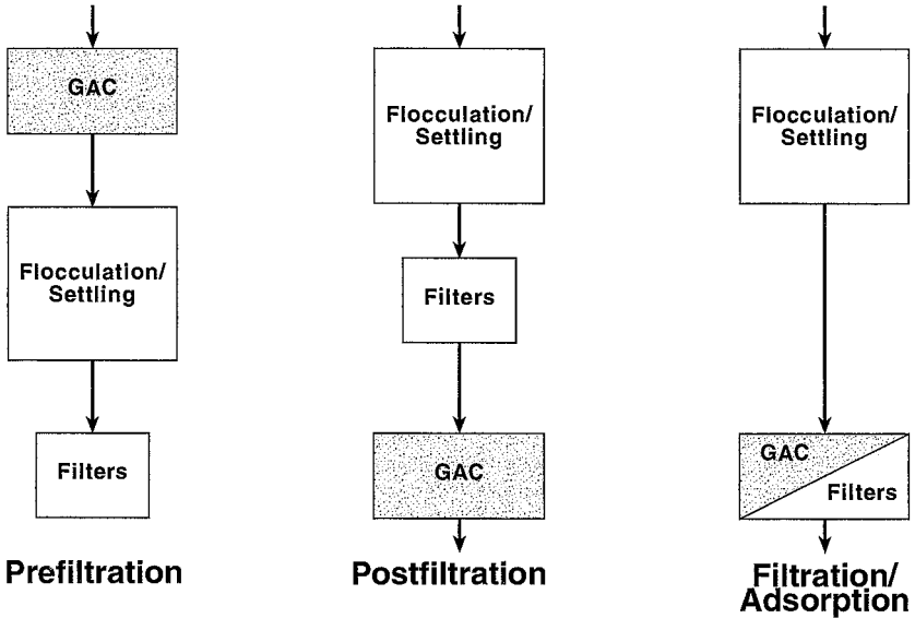
FIGURE 14.2 Basic options for locating GAC treatment.
