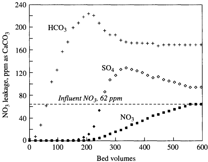
FIGURE 12.4 NO 3 breakthrough pattern for a nitrate-selective resin.
