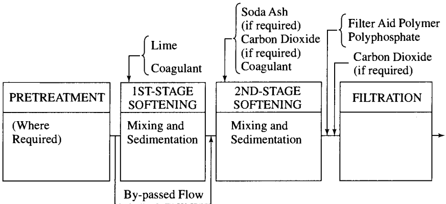
FIGURE 11.3 Split-treatment excess lime process.
