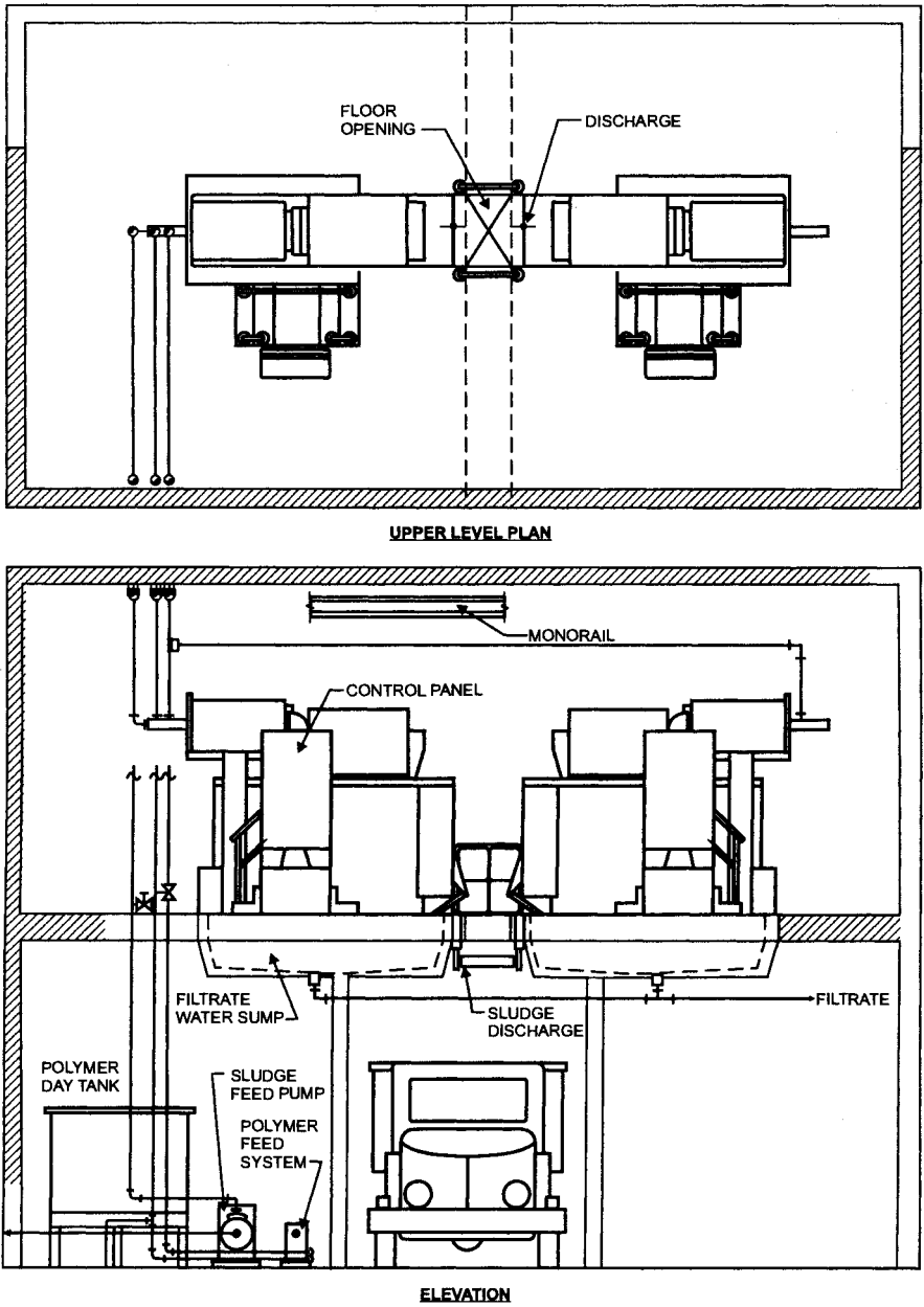
FIGURE 17.21 Typical belt filter press installation. (Source: AWWARF Handbook of Water Treatment Plant Waste Management.)
