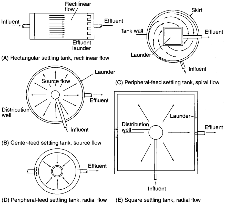
FIGURE 7.1 Typical conventional sedimentation tanks.
