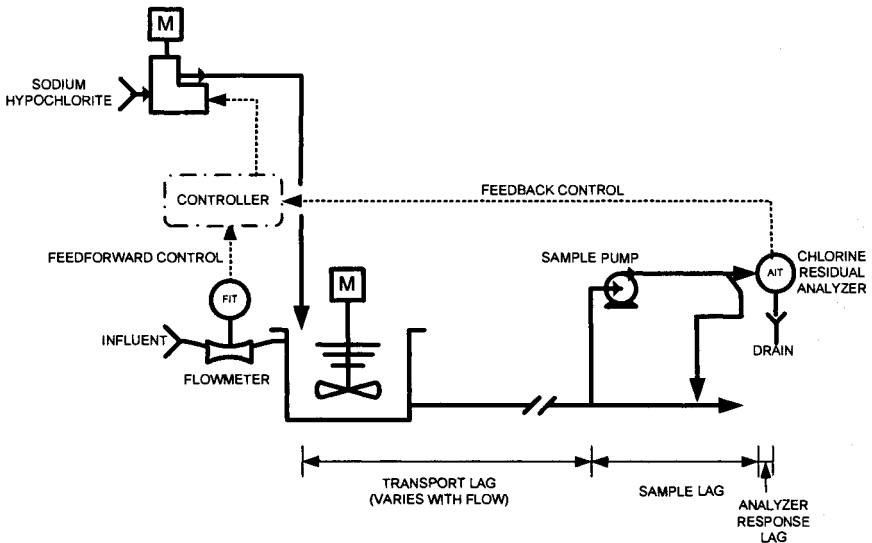
FIGURE 20.8 Compound chlorination control loop with time lags.
