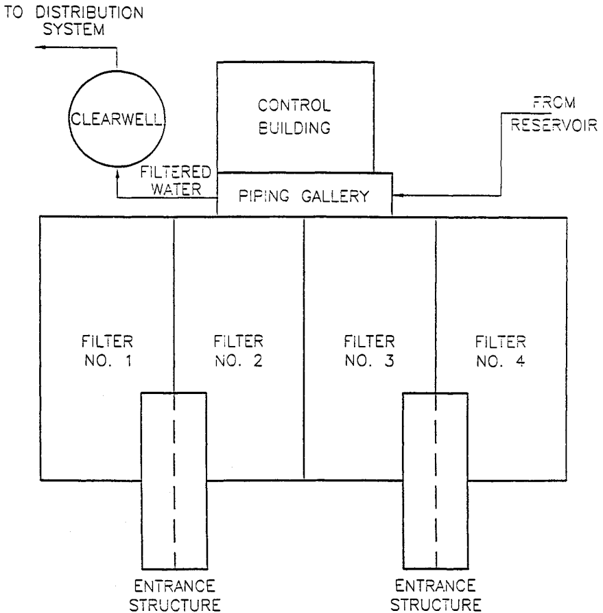
FIGURE 9.4 Typical slow sand plant layout with exterior entrance structures.
