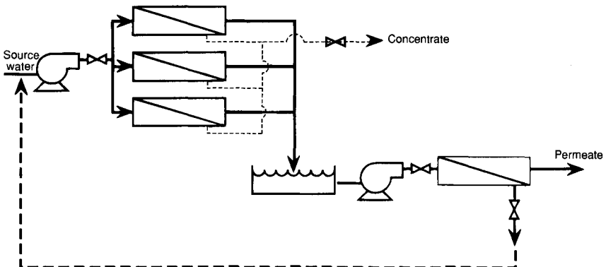
FIGURE 13.21 Permeate staging (multiple-pass design).
