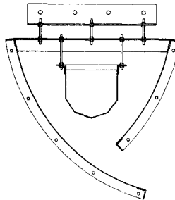
c. Engineered Stainless Steel Design (ESSD TM ) wash trough with Type II MULTIWASH R separator baffles. (Source: General Filter Company.)
