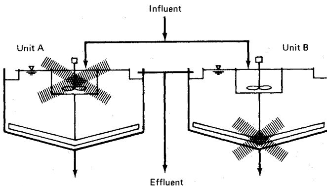
FIGURE 22.2 A-B syndrome—malfunction of two interrelated unit processes.
