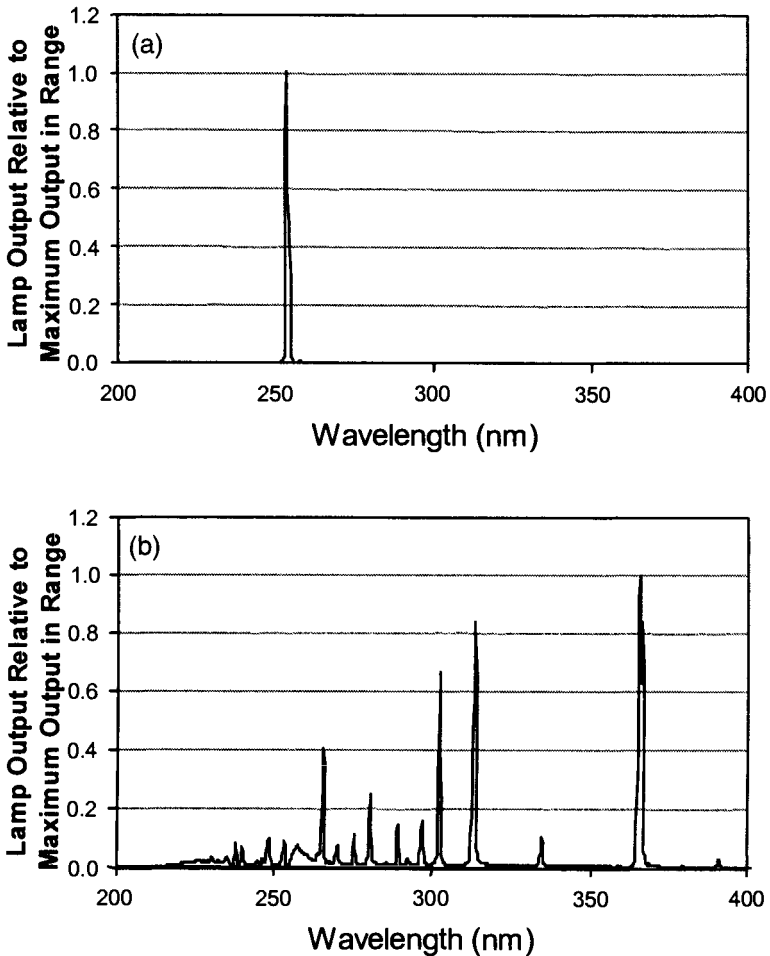
FIGURE 29.5 UV output of (a) low-pressure and (b) medium-pressure lamp types. (Source: Sharpless and Linden, 2001.)
