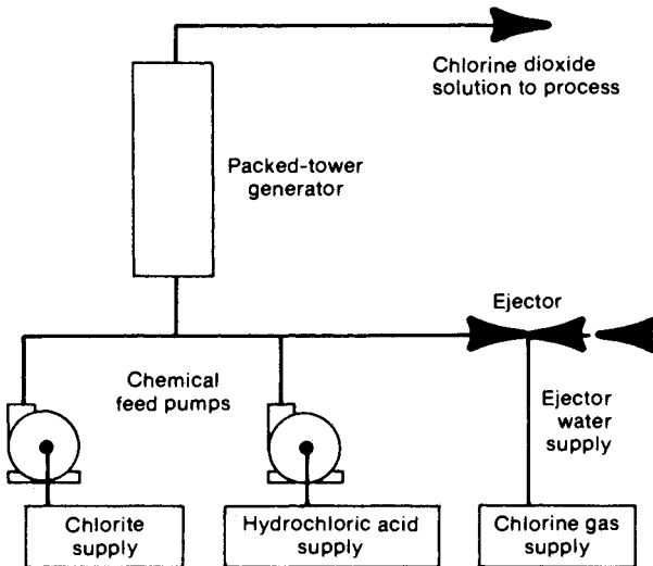
FIGURE 10.15 Aqueous chlorine-sodium chlorite system schematic with optional acid food. (Source: M. Aieta and J. Berg, "A Review of Chlorine Dioxide in Drinking Water Treatment," Journal AWWA, vol. 78, no. 6, June 1986, p. 62.)
