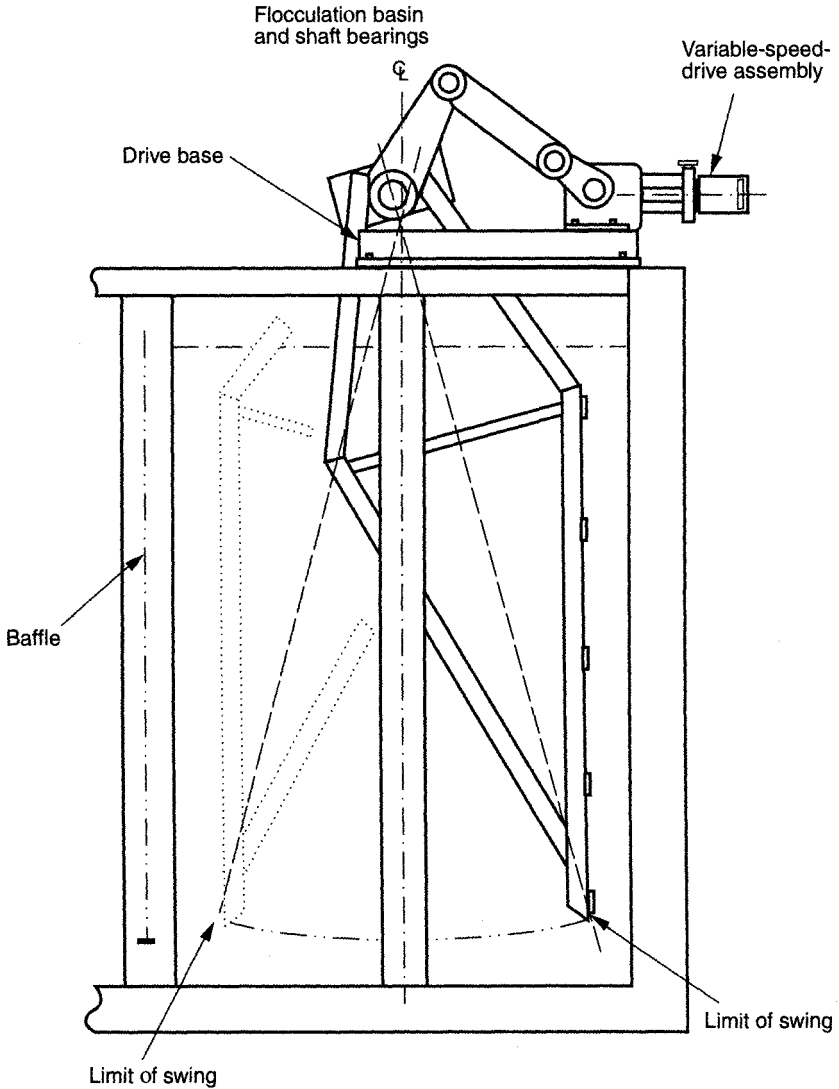
FIGURE 6.10 Oscillating flocculator. (Courtesy of Dorr-Oliver Eimco.)
