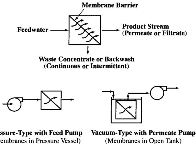
FIGURE 13.1 Pressure-driven processes using feed or permeate pumps.
