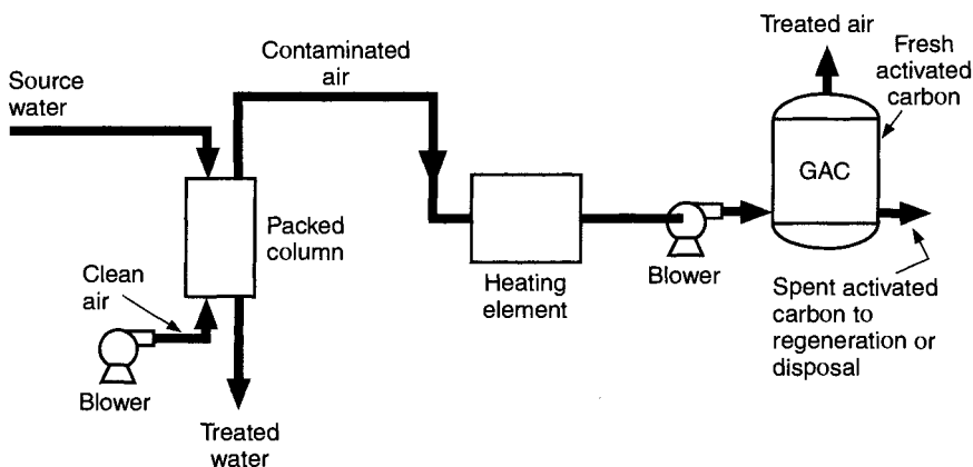
FIGURE 5.11 Schematic of vapor-phase GAC system. (Source: AWWA QGD Committee Report, 1991.)
