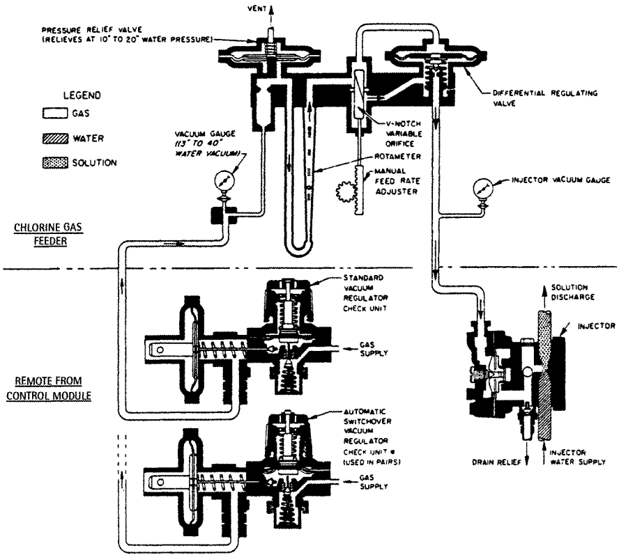
FIGURE 10.9 Flow diagram for conventional chlorinator. (Courtesy of Wallace and Tiernan Division of USFilter.)
