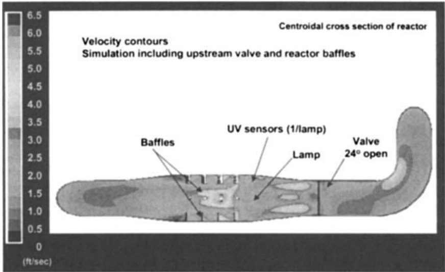
FIGURE 29.11 Example velocity contour output from computational fluid dynamics model. (Courtesy of Alex Mofidi, Metropolitan Water District of Southern California.)
