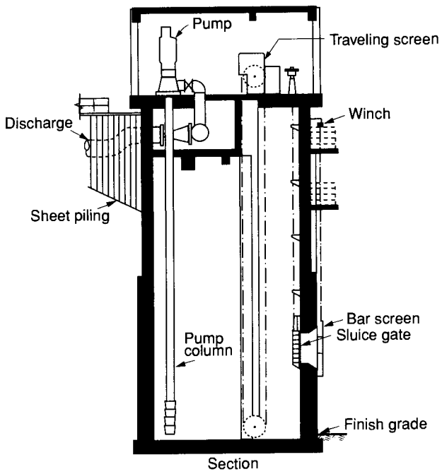
FIGURE 4.12 Multiple inlet gates.
