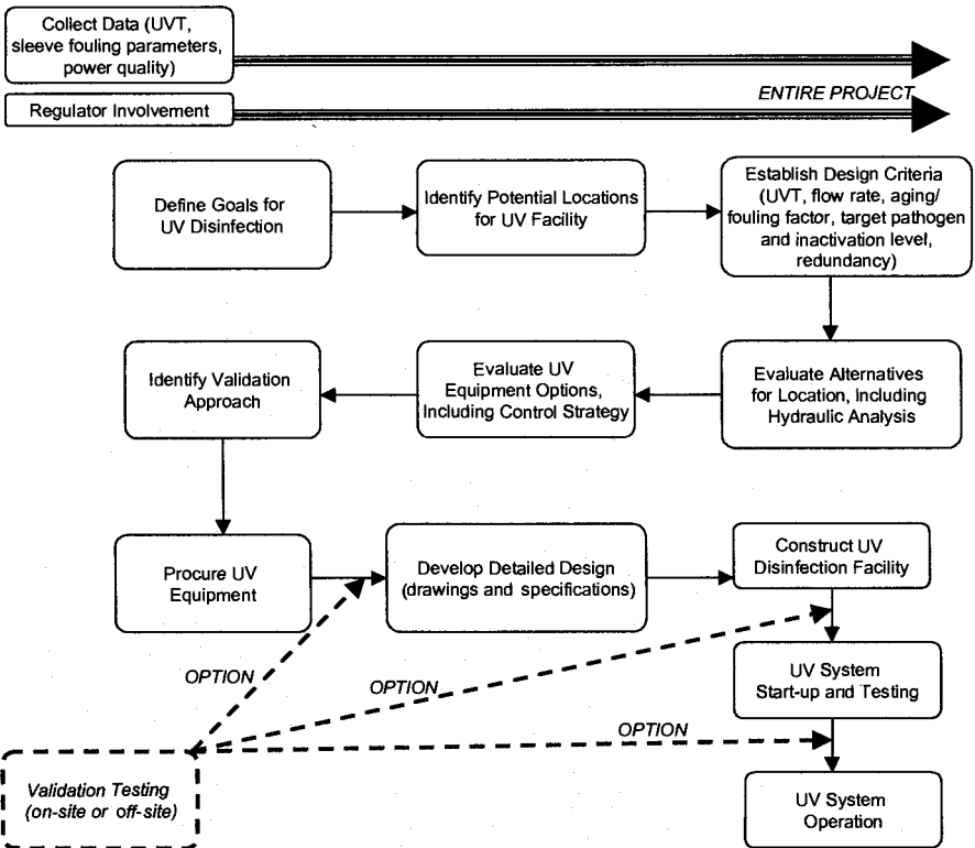
FIGURE 29.7 Flowchart for an approach for UV disinfection project implementation.
