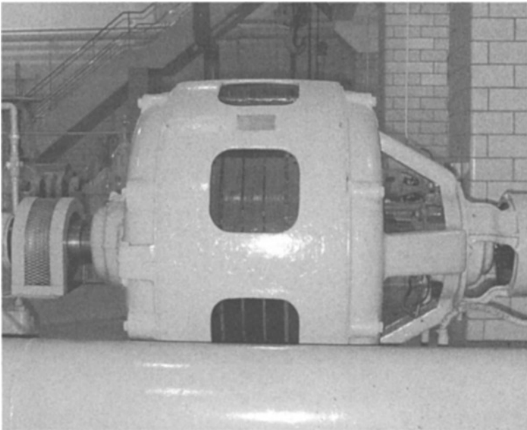
FIGURE 25.2 Electric pump drive functional after more than 70 years.
