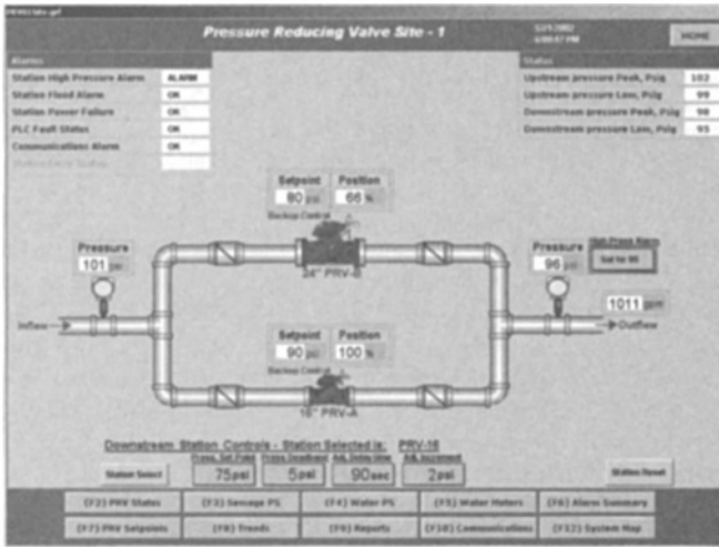
FIGURE 20.11 Example of process graphic.
