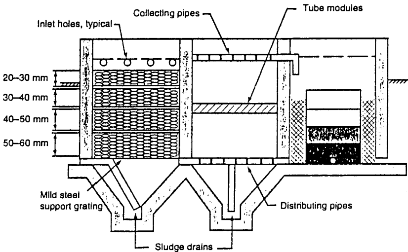
FIGURE 6.14 Downflow gravel bed flocculator. (Source: Schulz et al., 1994.)
