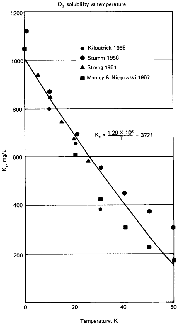
FIGURE 10.18 Effect of temperature on solubility of ozone.
