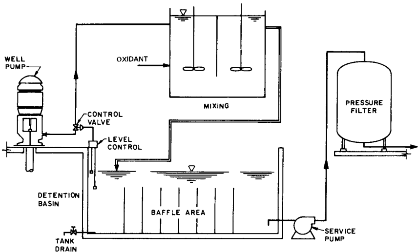
FIGURE 10.5 Chlorination, detention, and filtration (iron and manganese removal).
