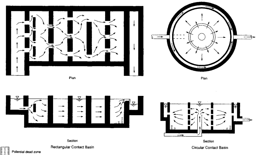
FIGURE 10.4 Examples of superior baffling conditions in basins. (Source: Guidance Manual .)
