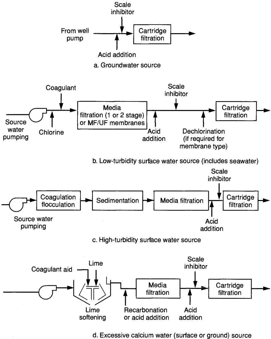
FIGURE 13.12 Typical RO or NF pretreatment processes.
