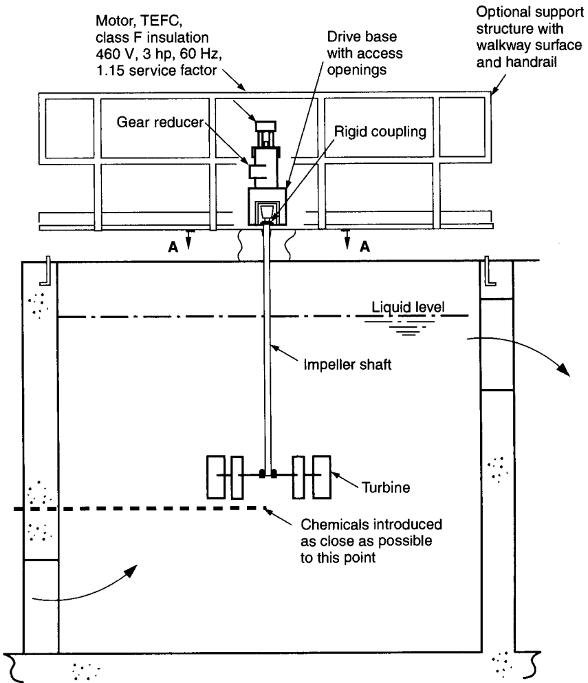
FIGURE 6.2 Turbine-type mechanical flash mixer. (Courtesy of Dorr-Oliver Eimco.)
