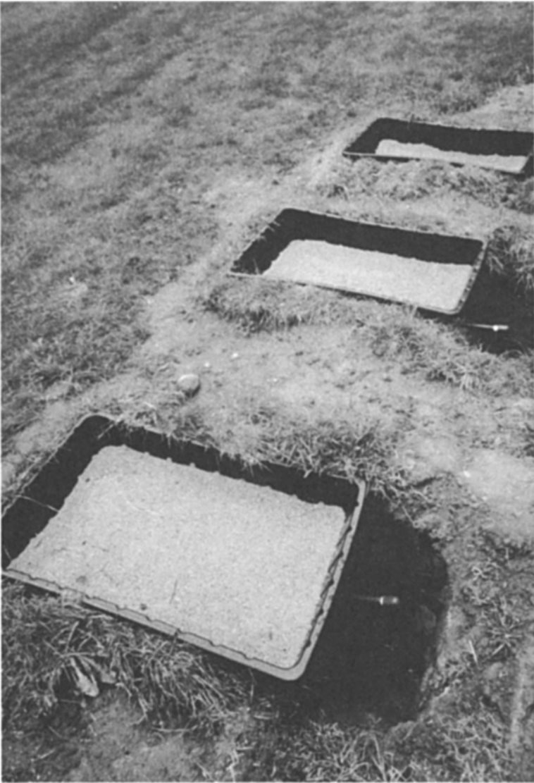
FIGURE 28.8 Water treatment residuals freeze-thaw beds with sand/gravel underdrain and leachate collection system included. Covers made of plywood are not shown. (Courtesy of CDM.)
