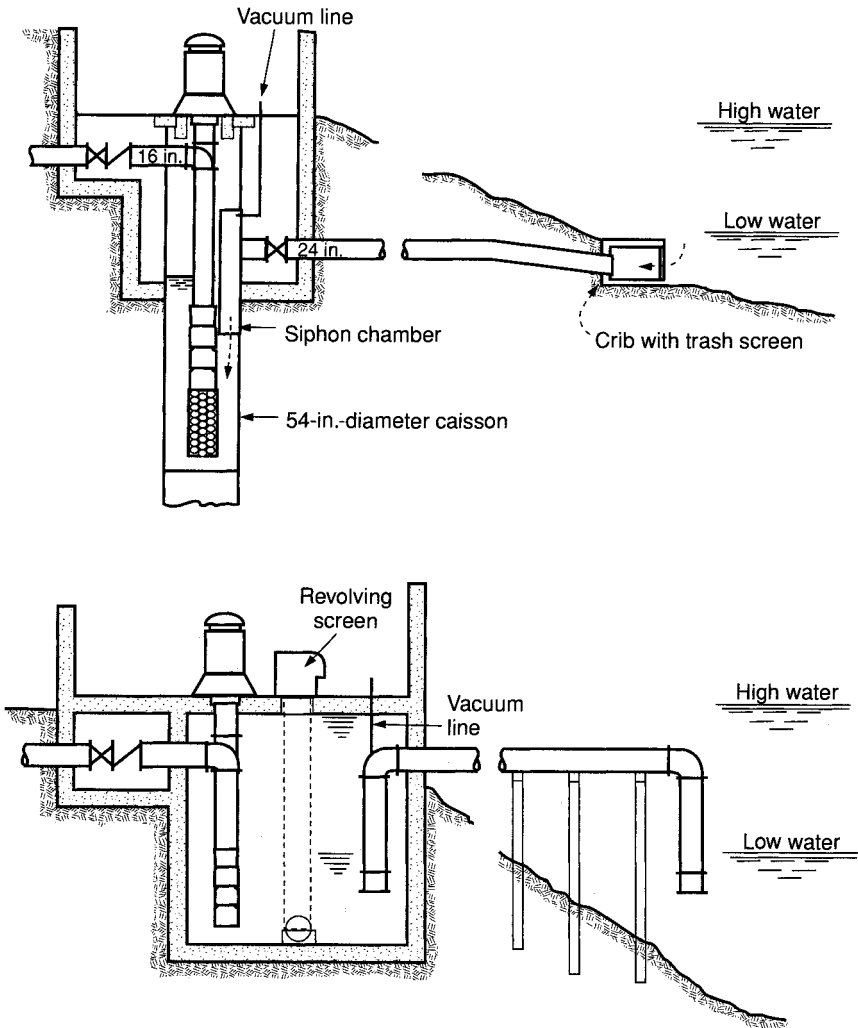
FIGURE 4.4 Siphon well intakes.
