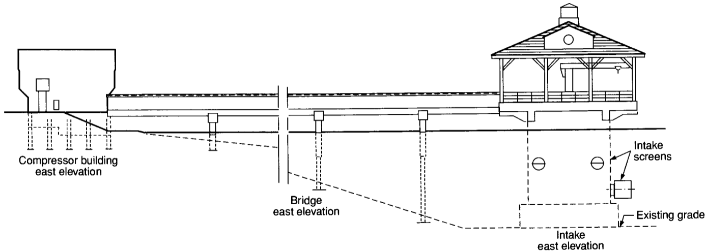
FIGURE 4.8 Lake Norman in-lake tower.
