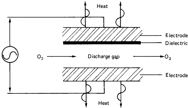
FIGURE 10.20 Basic ozonator configuration. [Source: H. Rosen, "Ozone Generation and Its Relationship to the Economical Application of Ozone in Wastewater Treatment," in F. L. Evans III (ed.), Ozone in Water and Wastewater Treatment , Ann Arbor Science Publishers, Ann Arbor, Mich., 1972.]
