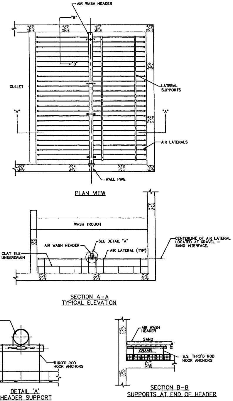
FIGURE 8.13 Vitrified clay tile underdrain with auxiliary air scouring system. (Source: Roberts Water Technologies, Inc.)
