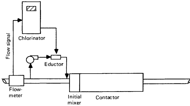
Feedforward control
