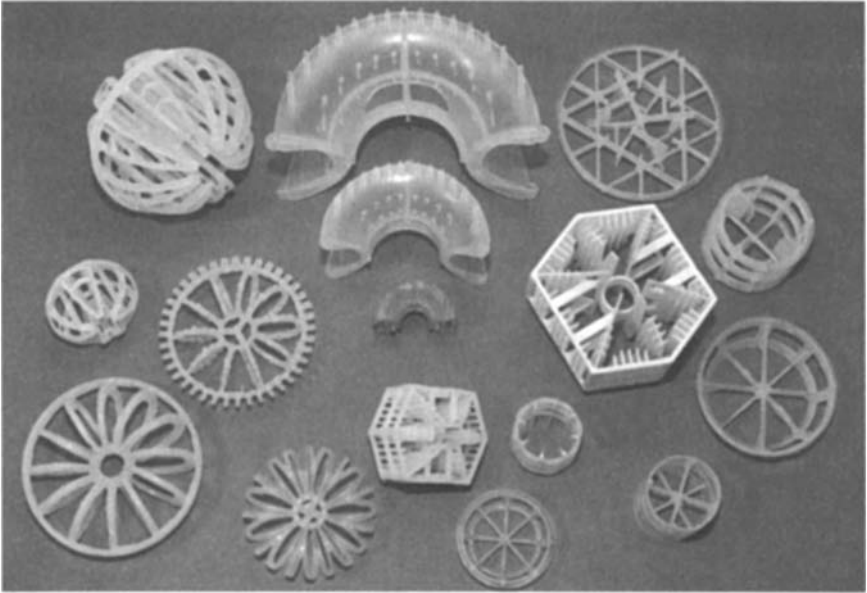
FIGURE 5.10 Some common shapes of plastic packing. (Source: U.S. Environmental Protection Agency.)
