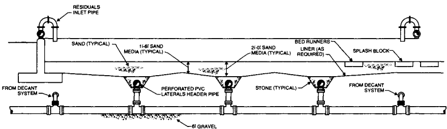
FIGURE 17.11 Sand drying bed underdrain system.
