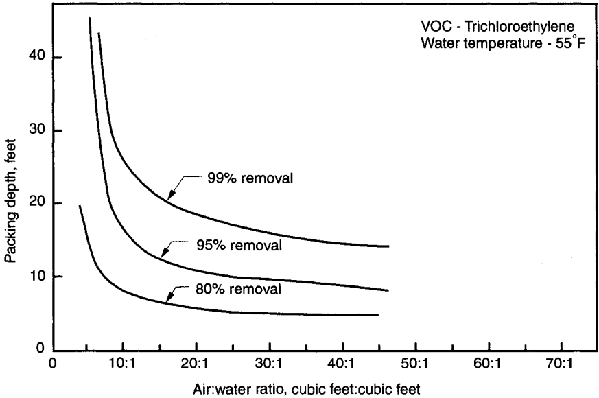
FIGURE 5.6 Effect of removal efficiency on packed column design. (Source: AWWARF/KIWA Report, 1983.)
