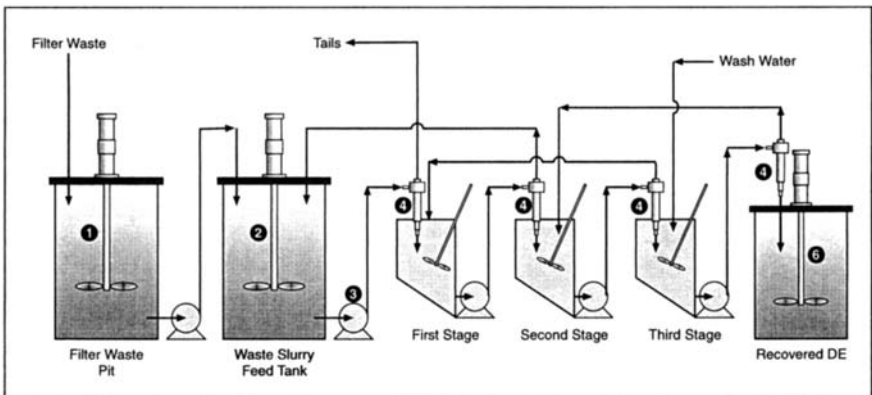
FIGURE 9.18 Schematic of a diatomaceous earth recovery system.
