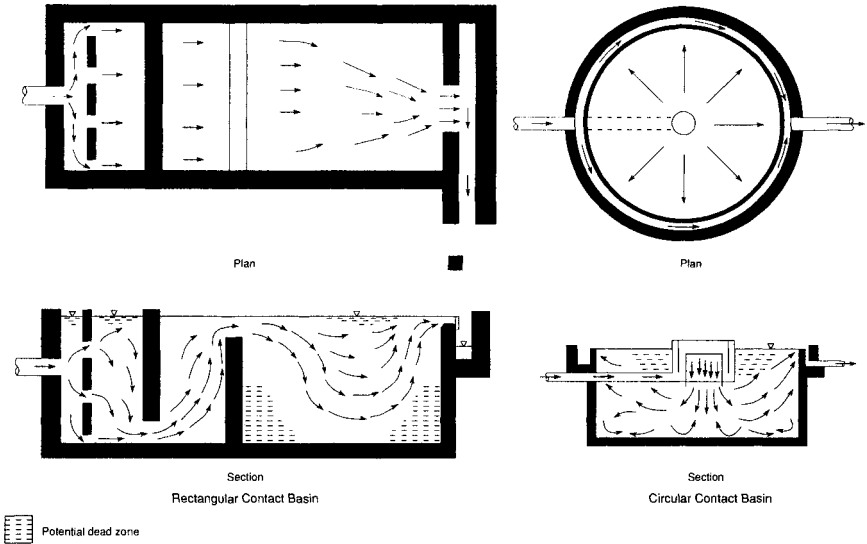
FIGURE 10.3 Examples of average baffling conditions in basins. (Source: Guidance Manual .)
