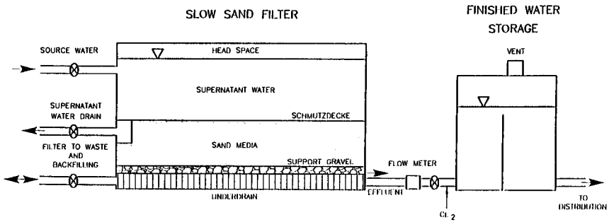
FIGURE 9.1 Typical covered slow sand filter installation.
