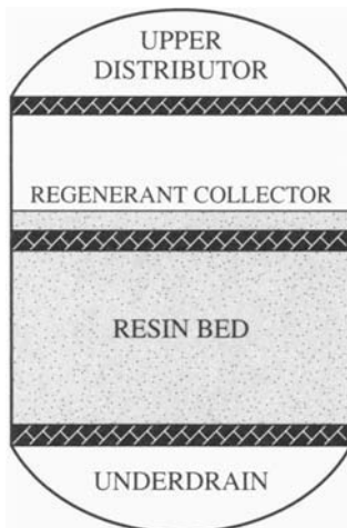
FIGURE 12.9 CCR exchanger.
