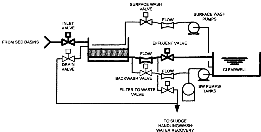
FIGURE 20.7 Example of filter backwash layout.
