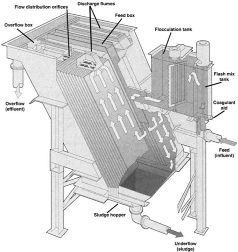
FIGURE 7.16 Plate settlers. (Courtesy of Parkson Corporation.)
