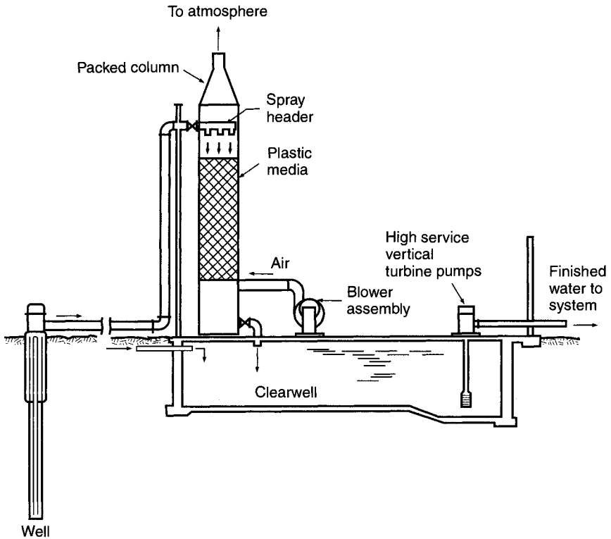
FIGURE 5.8 Packed tower aeration system. (Source: Cook College Office of Continuing Professional Education/SOTC.)
