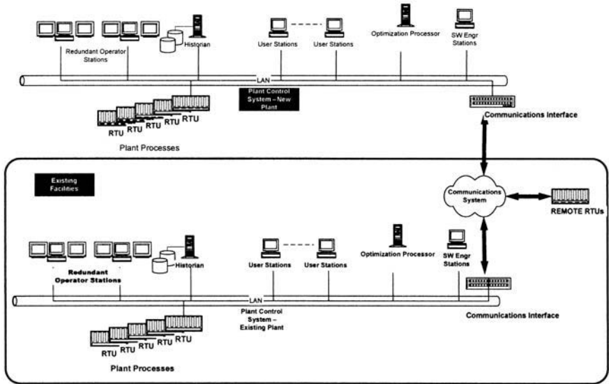
FIGURE 20.9 Example of water system control system architecture.
