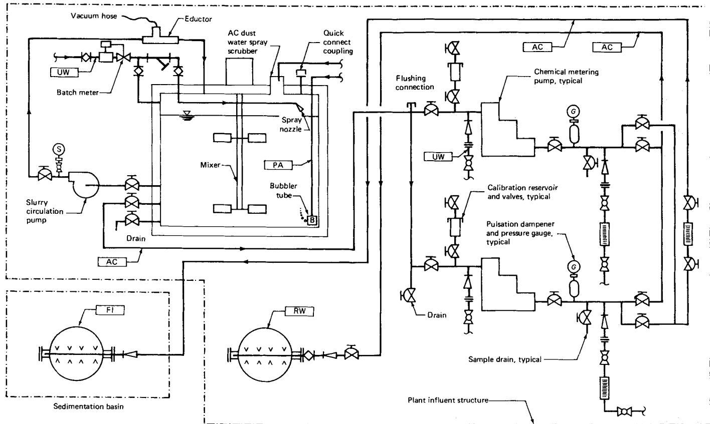
FIGURE 15.10 Activated carbon system. (Courtesy of MWH Americas Inc.)
