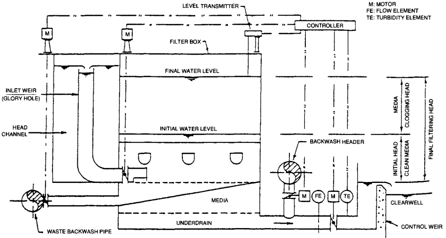
FIGURE 8.4 Constant-rate filter with influent splitting and varying water level. (Source: Monk, 1987.)
