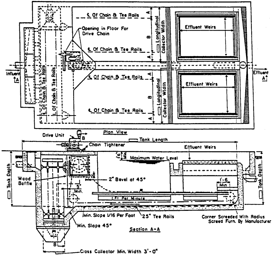
FIGURE 7.5 Typical rectangular basin with chain-and-flight collectors with chain-and-flight cross collectors.
