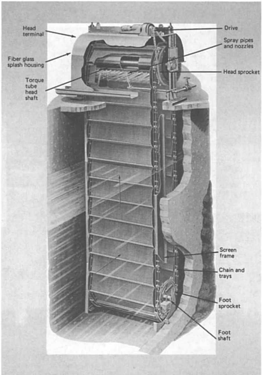
FIGURE 4.20 Traveling water screen.
