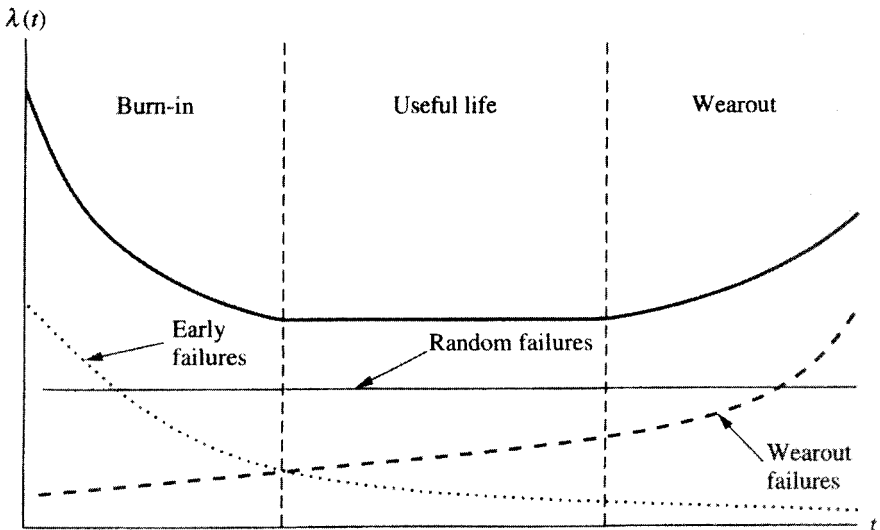
FIGURE 22.1 The bathtub curve. (Source: Charles E. Ebeling, An Introduction to Reliability and Maintainability Engineering , McGraw-Hill, 1997; reprinted with permission of The McGraw-Hill Companies.)
