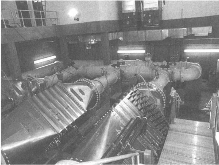
FIGURE 29.9 UV facility to disinfect combined filter effluent in Clayton County, Georgia. (Photo courtesy of Clayton County, Ga., Water Authority, Freeman Road Water Production Plant.)
