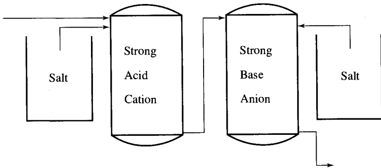
FIGURE 12.1 Strong base dealkalizer.
