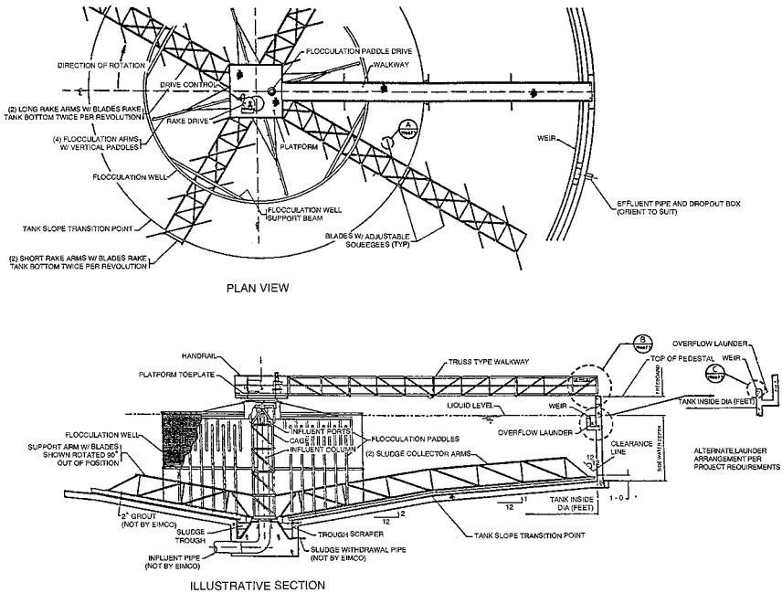
FIGURE 7.12 Typical flocculator clarifier. (Courtesy of Eimco Water Technologies.)
