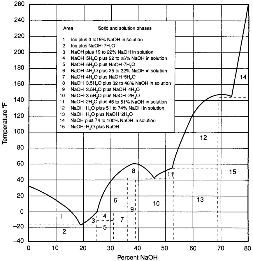
FIGURE 15.4 Freezing points of caustic soda solutions.
