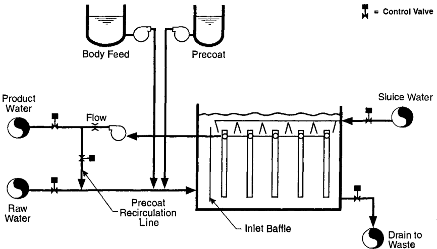
FIGURE 9.17 Vacuum filter system schematic.
