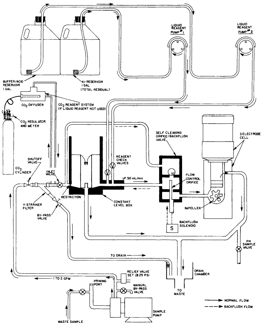
FIGURE 10.13 Flow diagram of amperometric chlorine residual analyzer. (Courtesy of Wallace and Tieren Division of USFilter.)
