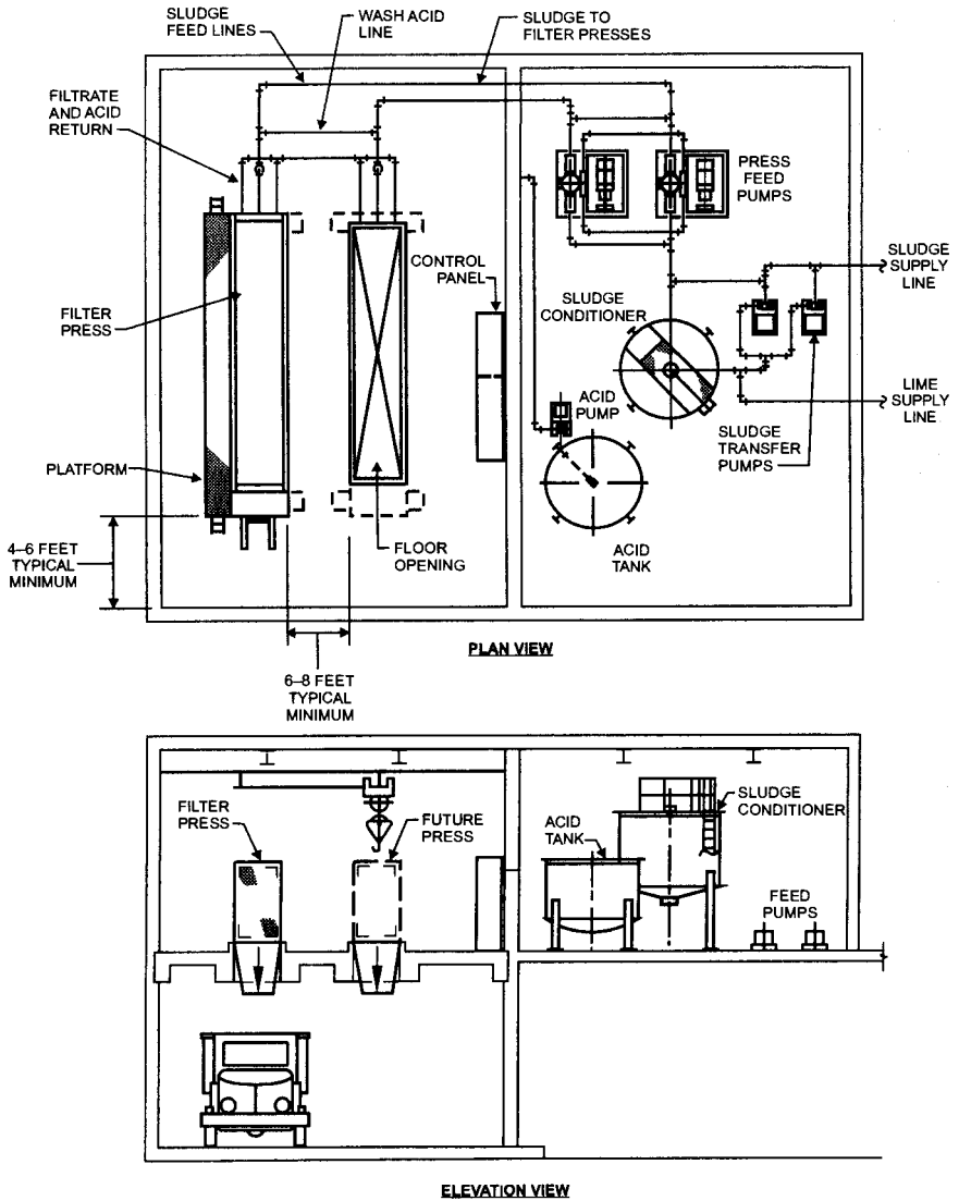
FIGURE 17.20 Typical filter press layout. (Source: AWWARF Handbook of Water Treatment Plant Waste Management.)
