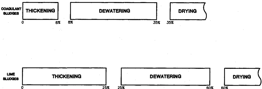
FIGURE 17.3 Percent dry solids for treatment of coagulant and lime sludges.
