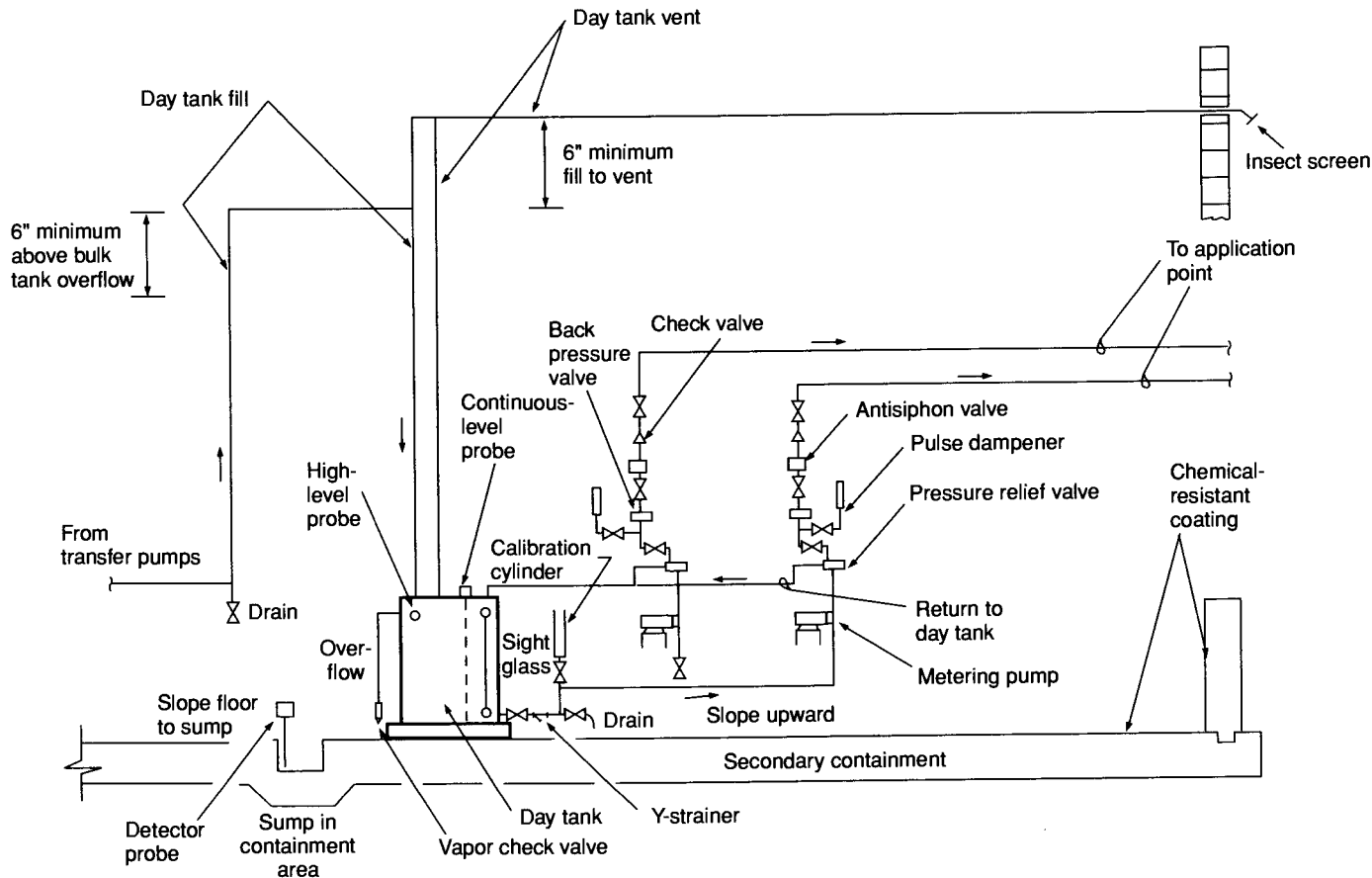
FIGURE 15.9 Typical arrangement for valves and apparatus.
