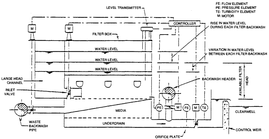
FIGURE 8.5 Declining-rate filter. (Source: Monk, 1987.)
