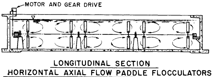
FIGURE 6.7 Sections through horizontal shaft paddle flocculator.
