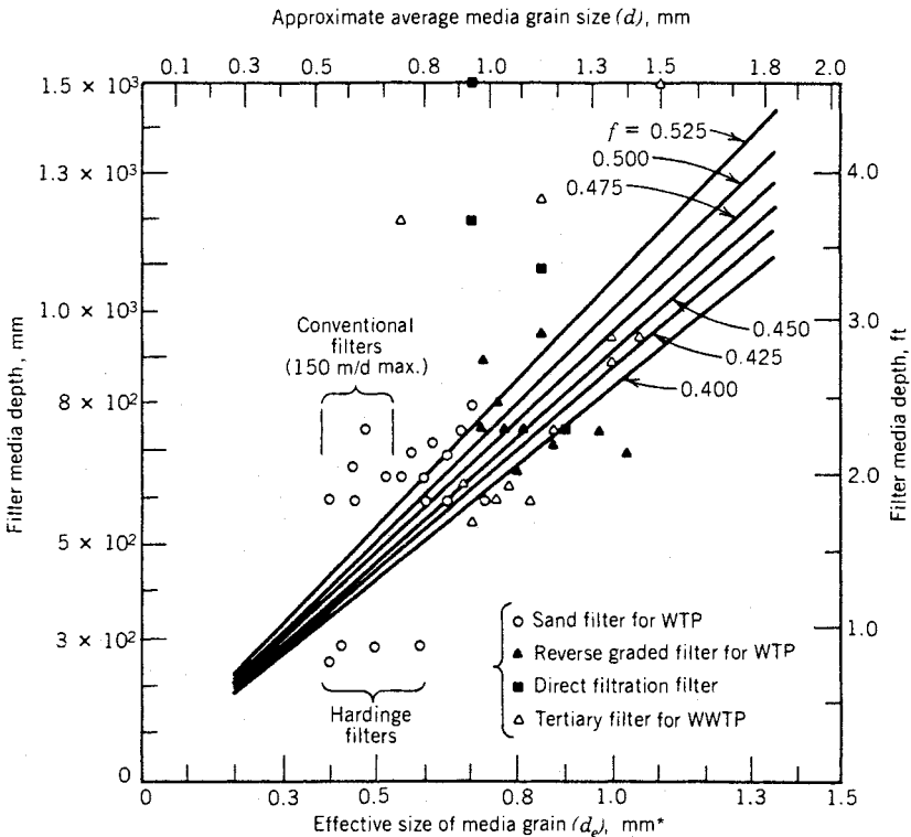
FIGURE 8.1 Relationship between depth and size of media. (Courtesy of MWH Americas Inc.)
