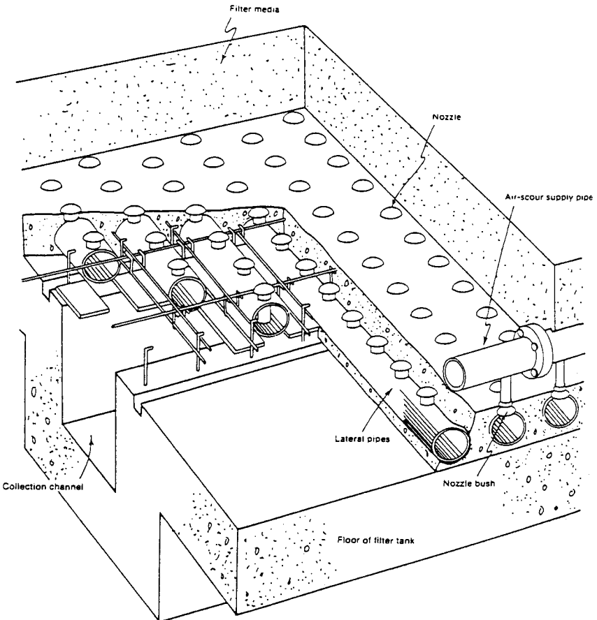
FIGURE 8.11 Pipe lateral underdrain with nozzles. (Courtesy of Paterson Candy Ltd.)
