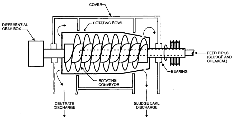
FIGURE 17.22 Centrifuge schematic. (Source: AWWARF Handbook of Water Treatment Plant Waste Management.)
