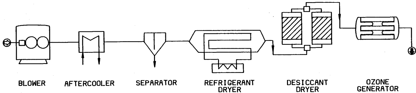
FIGURE 10.22 Low-pressure air preparation ozonation system.
