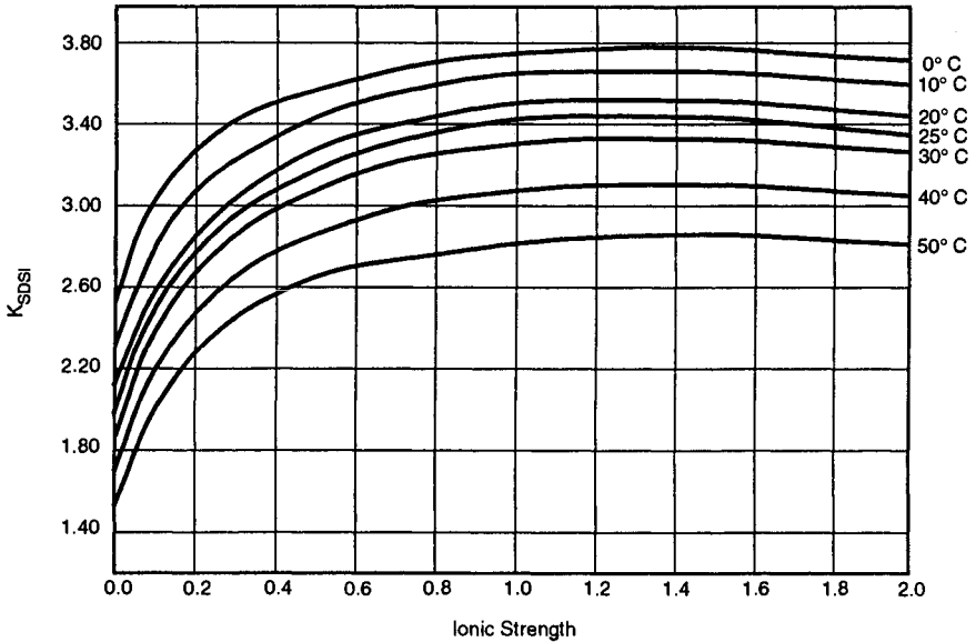
FIGURE 13.14 Stiff and Davis K versus ionic strength and temperature. (Adapted from DuPont Permasep Products Engineering Manual, 1992.)
