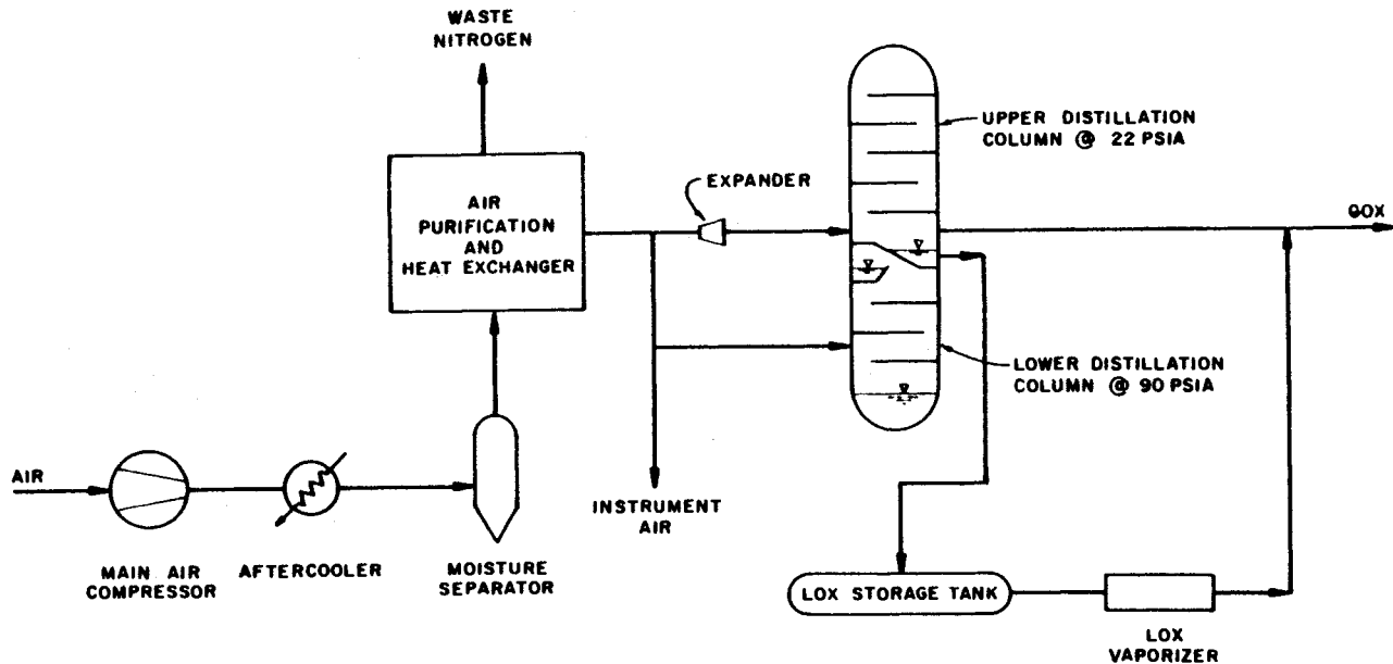
FIGURE 10.25 Typical schematic of cryogenic system.
