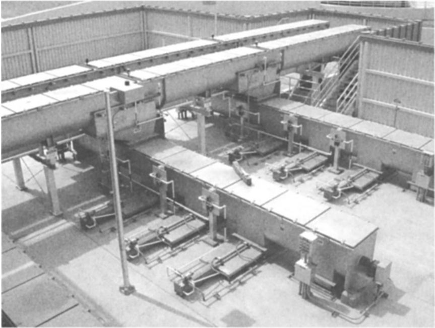
FIGURE 17.27 Conveyor system. (Courtesy of City of Phoenix Water Services Department.)
