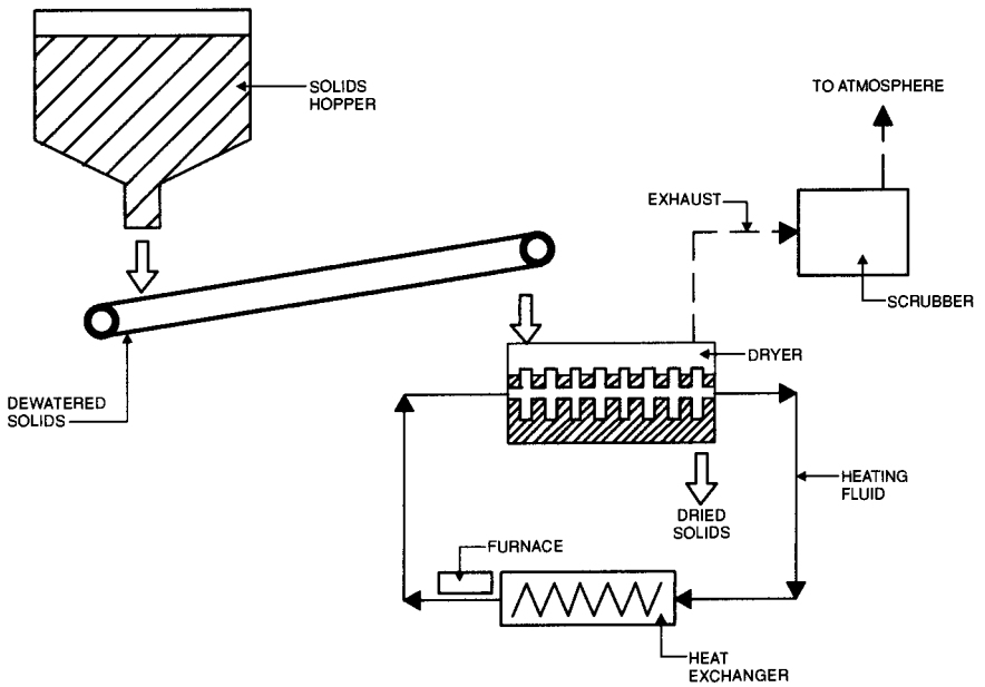
FIGURE 17.25 Heat drying process.
