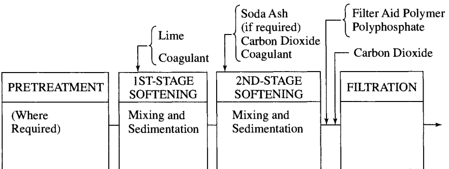
FIGURE 11.2 Excess lime softening process.
