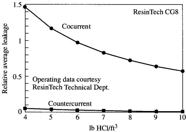
FIGURE 12.6 Regeneration method versus leakage.
