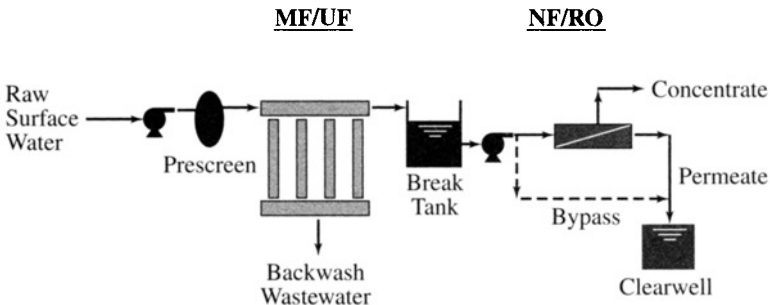
FIGURE 13.10 Example dual-membrane system for treating a saline surface water.
