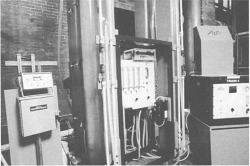
FIGURE 28.7 Ozone disinfection module includes oxygen generator, ozone generator, contact columns, pumps, flowmeters, residual and feedgas monitors, and power supply panel. (Courtesy of CDM.)
