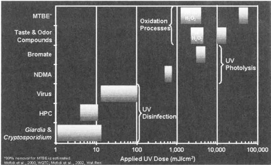
FIGURE 29.3 Summary of UV dose ranges to achieve between 90% and 99% removal. (Courtesy of Alex Mofidi, Metropolitan Water District of Southern California.)
