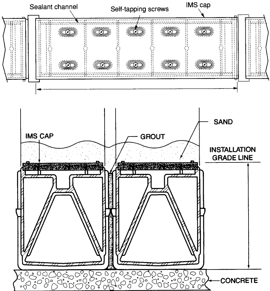
FIGURE 8.15 Integral media support (IMS) cap designed for use without support gravel. (Source: F. B. Leopold Co., Inc.)
