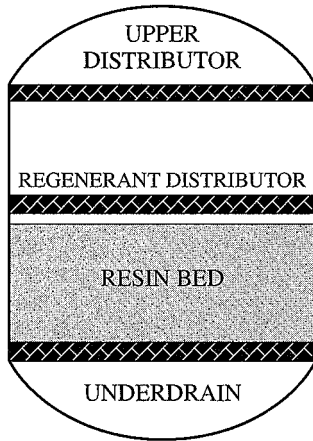
FIGURE 12.7 Coflow exchanger.
