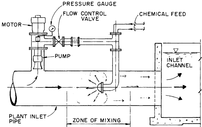
FIGURE 6.4 Section through pump mixer.
