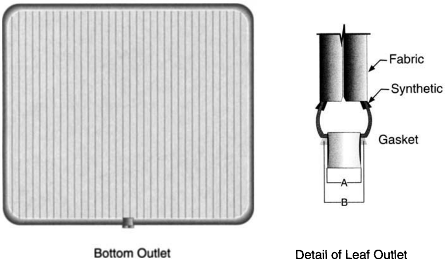
FIGURE 9.13 Vacuum filter leaf.
