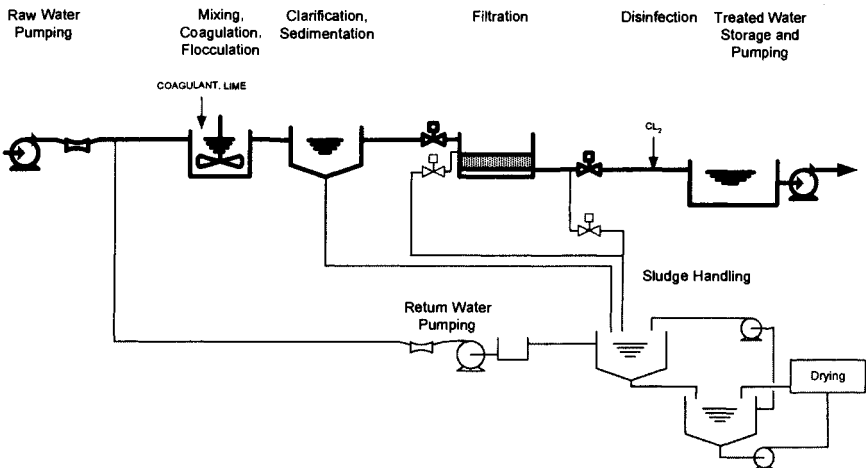
FIGURE 20.4 Example of water treatment plant—primary processes. (Source: Instrumentation and Computer Integration of Water Utility Operations, AWWARF, 1993, revised by the author.)
