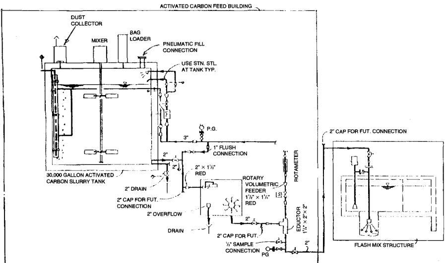
FIGURE 14.1 Activated carbon feeding system.
