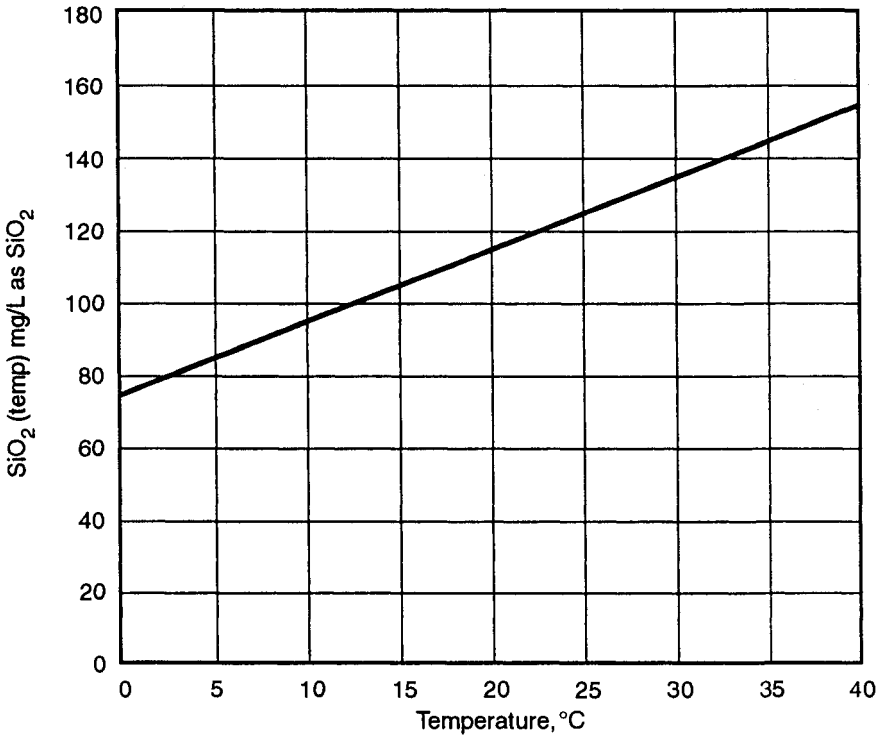
FIGURE 13.17 Effect of temperature on SiO 2 solubility. (Adapted from DuPont Permasep Products Engineering Manual, 1992.)
