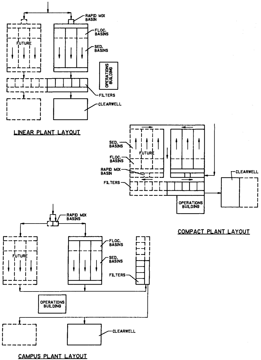
FIGURE 23.2 Basic plant layout types.
