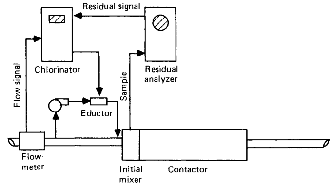
Compound-loop control
