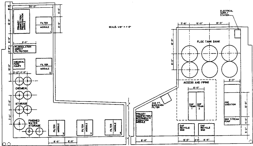
FIGURE 28.9 Pilot plant floor plan.
