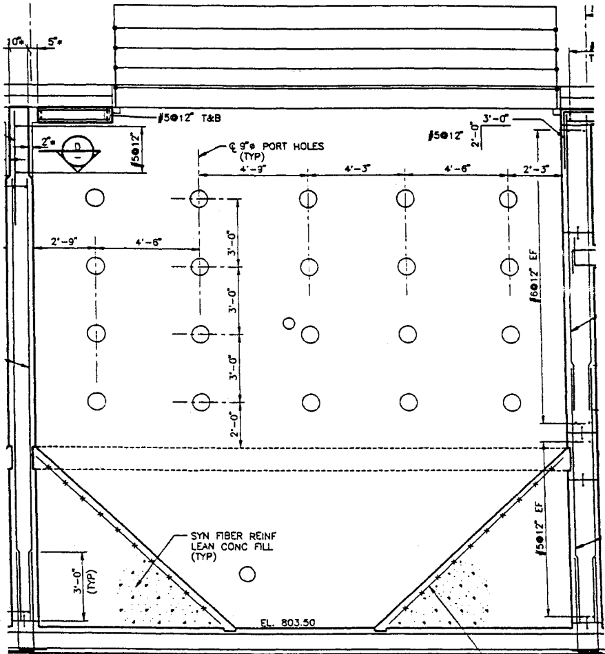
FIGURE 7.3 Typical inlet baffle showing orifices.
