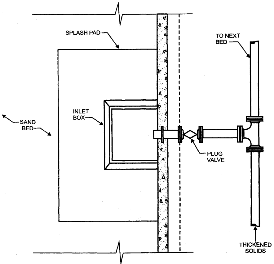
FIGURE 17.12 Drying bed inlet structure.
