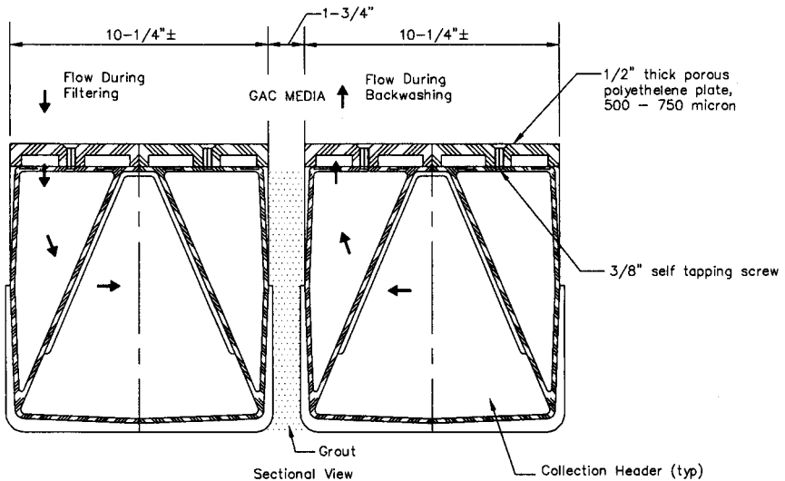
FIGURE 14.9 Block underdrain with porous membrane.
