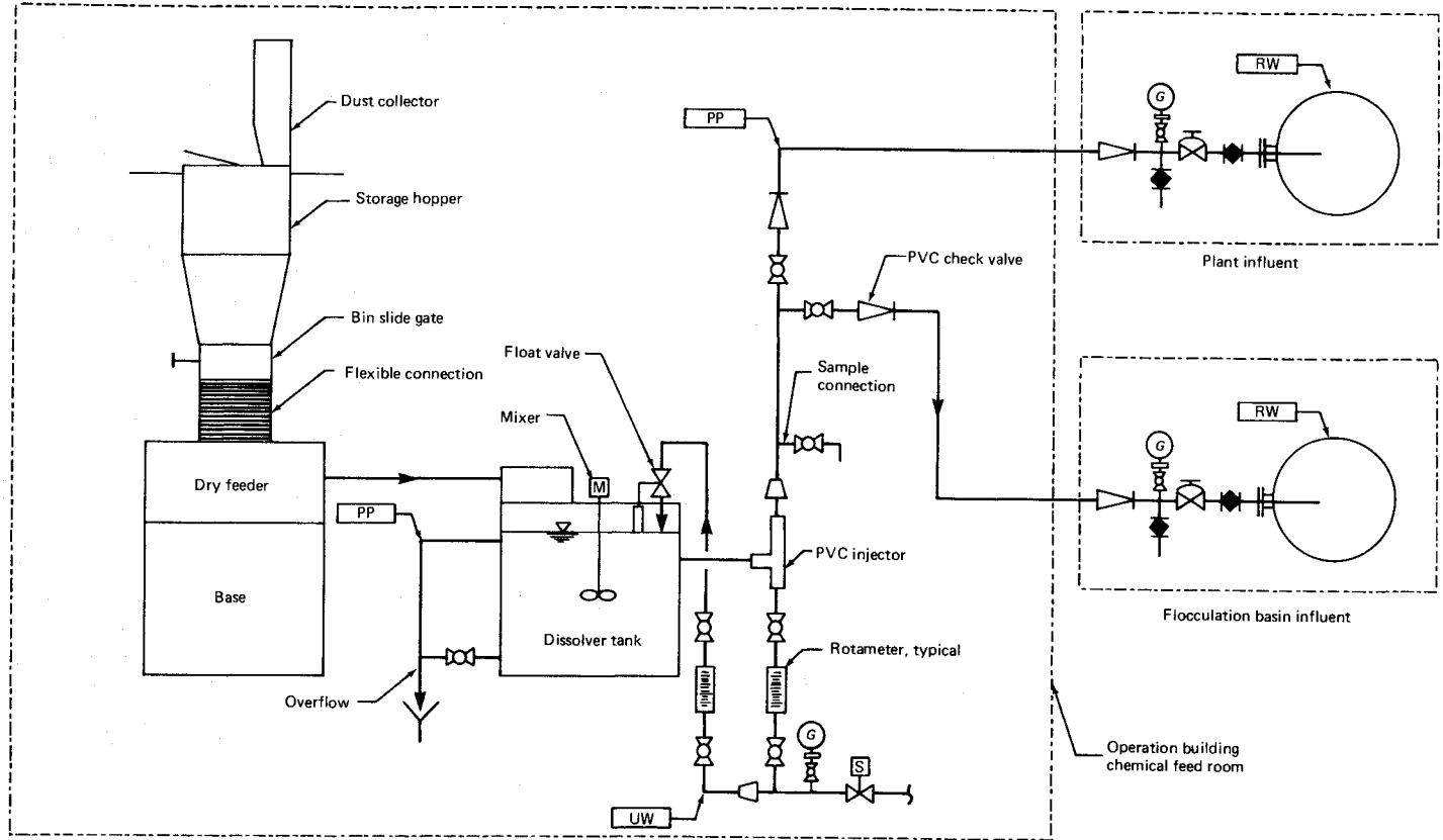
FIGURE 15.8 Potassium permanganate system. (Courtesy of MWH Americas Inc.)
