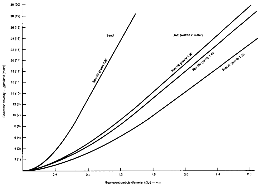
FIGURE 14.6 Determination of appropriate medium size and backwash rate for a water temperature of 68° F (20° C) (backwash velocity = 1.3 \times V_{mf} for D 90 ).
