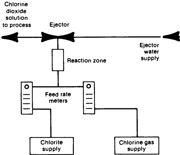
FIGURE 10.16 Gas chlorine-sodium chlorite system schematic. (Source: M. Aieta and J. Berg, "A Review of Chlorine Dioxide in Drinking Water Treatment," Journal AWWA, vol. 78, no. 6, June 1986, p. 62.)
