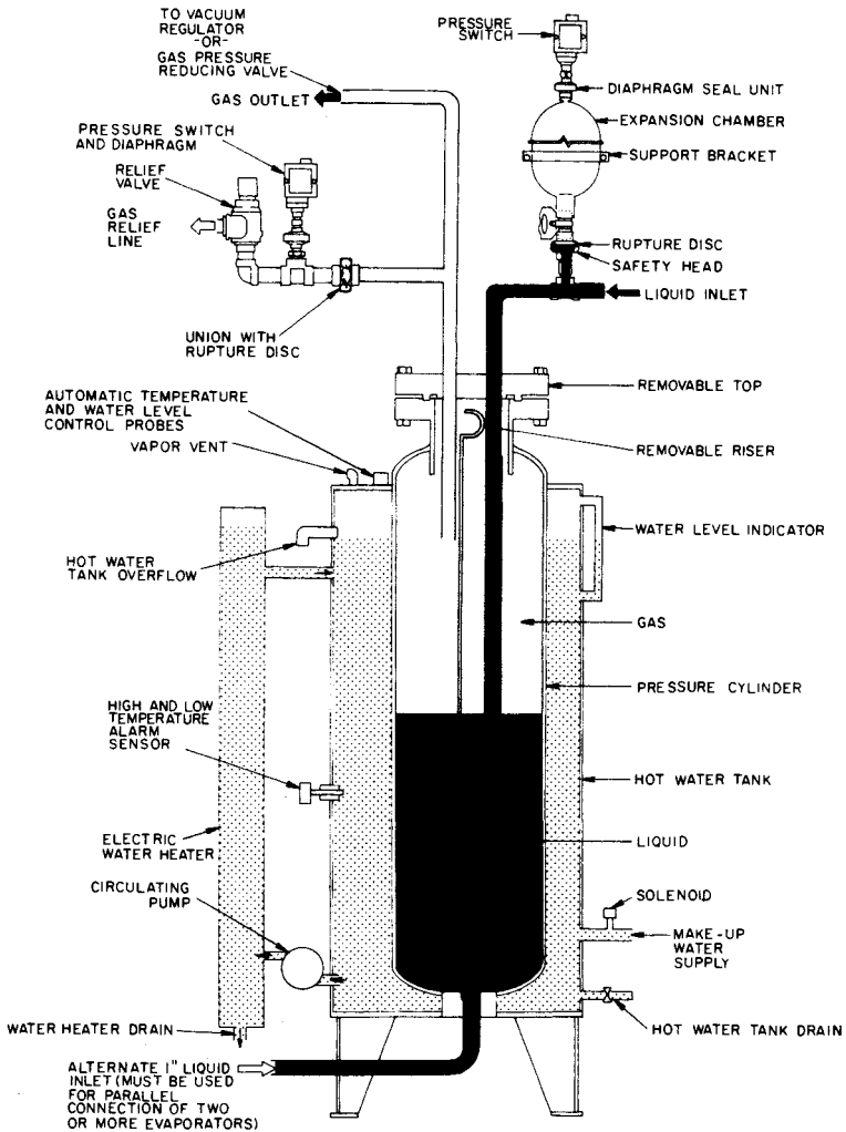
FIGURE 15.2 Cross section of typical evaporator. (Courtesy of Wallace and Tiernan Division of USFilter.)
