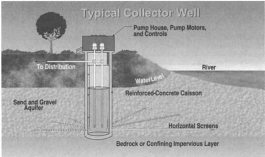
FIGURE 4.6 Horizontal groundwater collection system. (Source: Hydro Group.)
