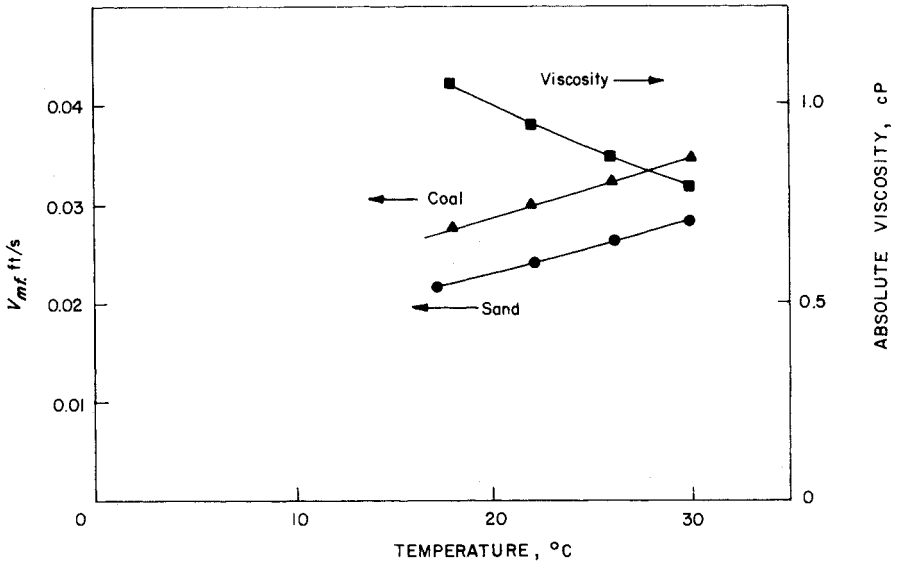
FIGURE 8.9 Effect of water temperature on V_{mf} of sand and coal, and on absolute viscosity of water. (Source: Cleasby and Baumann, 1974.)
