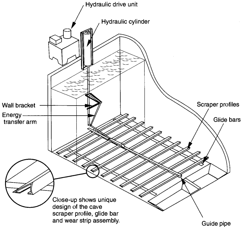
FIGURE 7.8 Indexing grid sludge removal system. (Courtesy of Parkson Corporation.)
