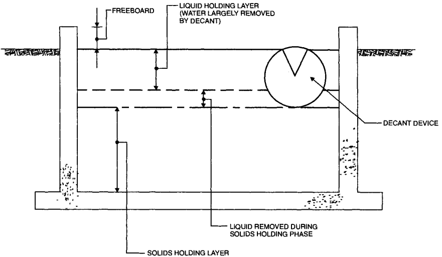
FIGURE 17.16 Drying bed operating layers.
