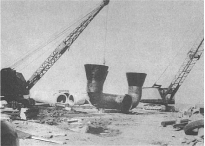
FIGURE 4.14 Hydraulically balanced inlet cones.
