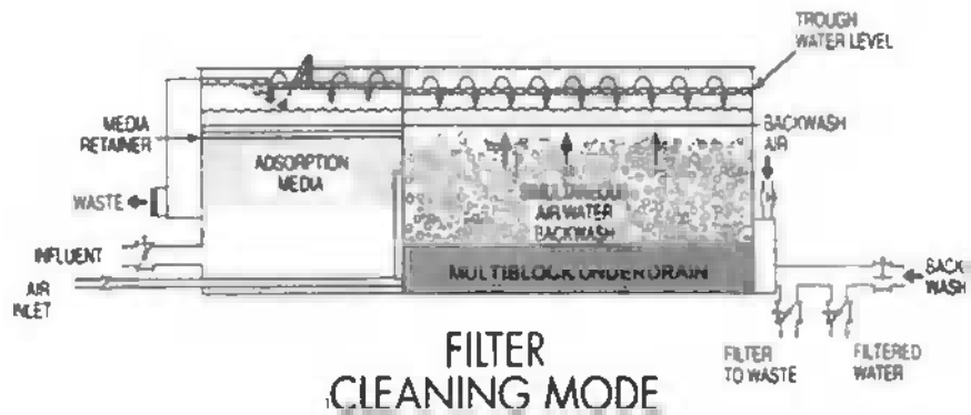
FIGURE 7.22 Adsorption Clarifier. (Courtesy of USFilter, Microfloc Products.)
