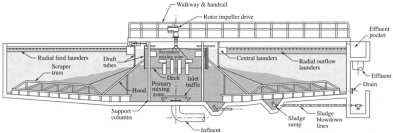
FIGURE 11.5 Solids contact clarifier.
