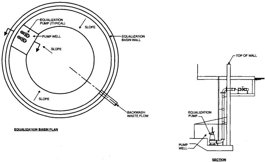
FIGURE 17.6 Typical equalization basin layout.
