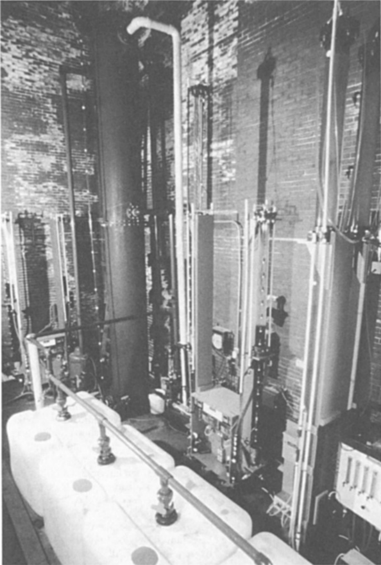
FIGURE 28.6 Manifolder backwash collection, settling and storage tanks in foreground. Large-scale filter (2-ft diameter) in background generates backwash solids. (Courtesy of CDM.)
