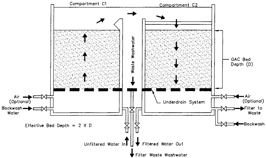
FIGURE 14.10 Conversion of split-cell filters to GAC contactors.
