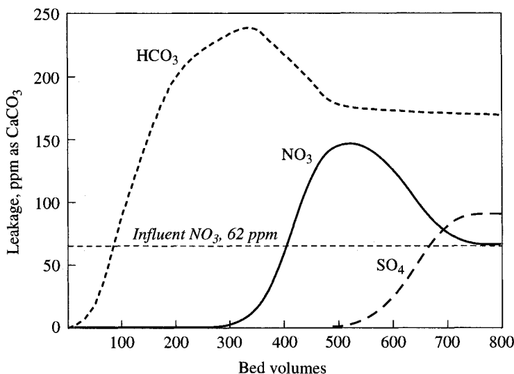
FIGURE 12.3 NO 3 breakthrough pattern for a type II, nonselective resin.
