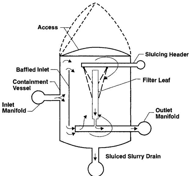
FIGURE 9.9 Principal elements of a flat-leaf filter.
