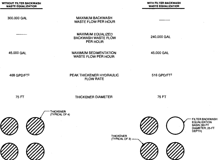
FIGURE 17.4 Impact of equalization on unit process sizing.
