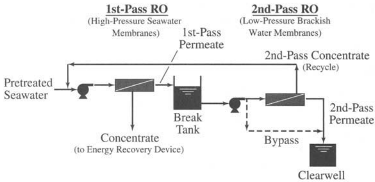
FIGURE 13.11 Example two-pass RO seawater desalination system.
