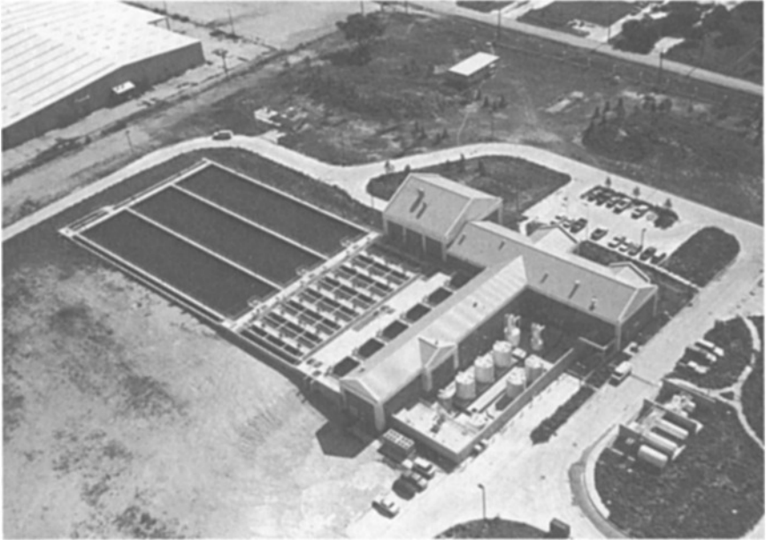
FIGURE 23.3 Aerial view of compact water treatment plant, Eagle Mountain WTP, Fort Worth, Texas.
