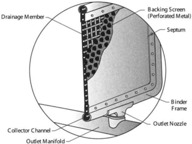
FIGURE 9.12 Typical construction of flat-leaf filter element.
