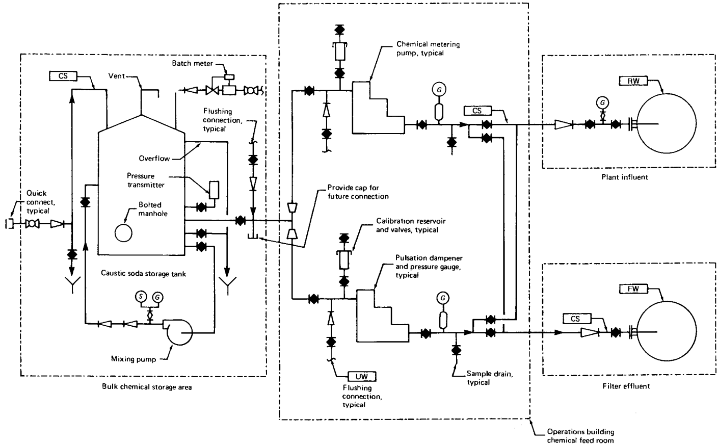
FIGURE 15.5 Caustic soda system. (Courtesy of MWH Americas Inc.)
