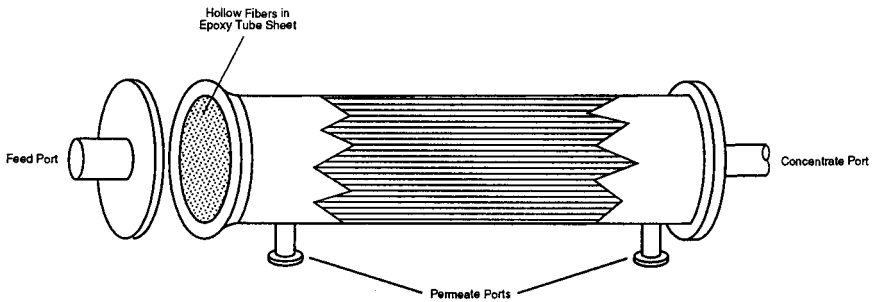
FIGURE 13.6 Representation of hollow-fiber UF module.
