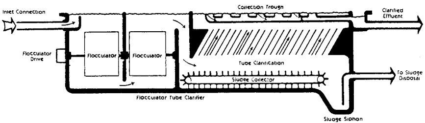
FIGURE 7.13 Typical tube settler. (Courtesy of USFilter, Microfloc Products.)
