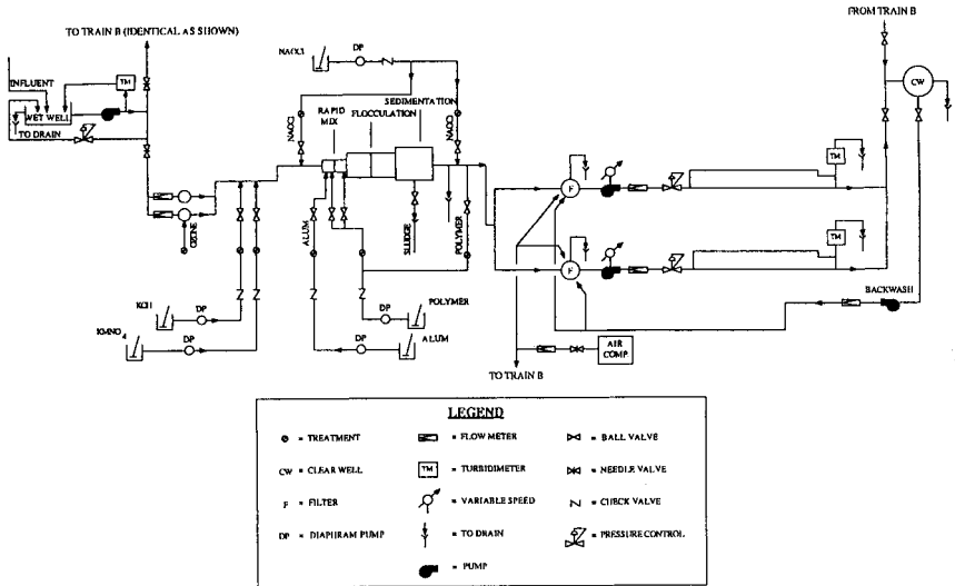
FIGURE 28.10 Pilot plant schematic of train A.
