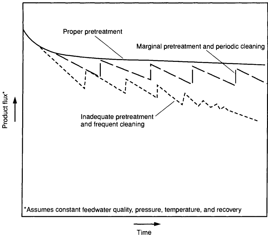
FIGURE 13.19 Membrane flux decline curves under different pretreatment conditions. (Adapted from DuPont Permasp Products Engineering Manual, 1992.)
