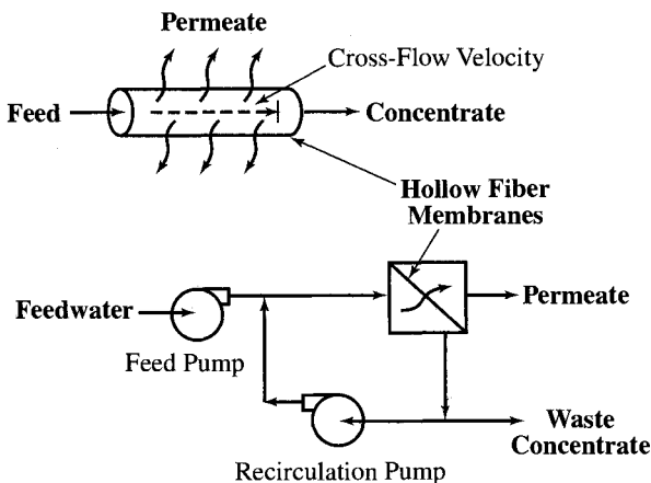
FIGURE 13.23 Use of recirculation pumping to provide needed cross-flow velocities.
