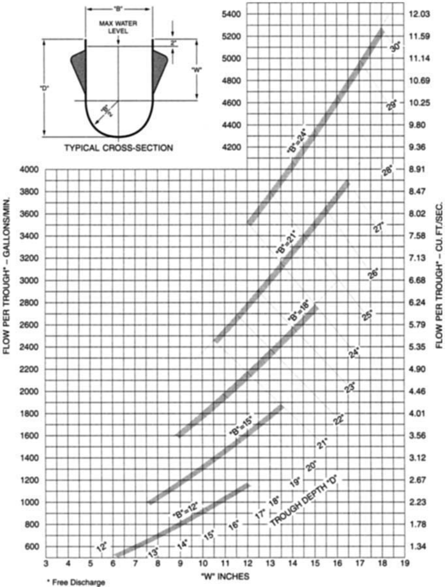
FIGURE 8.20 Washwater trough-sizing diagram. (Source: F. B. Leopold Co., Inc.)
