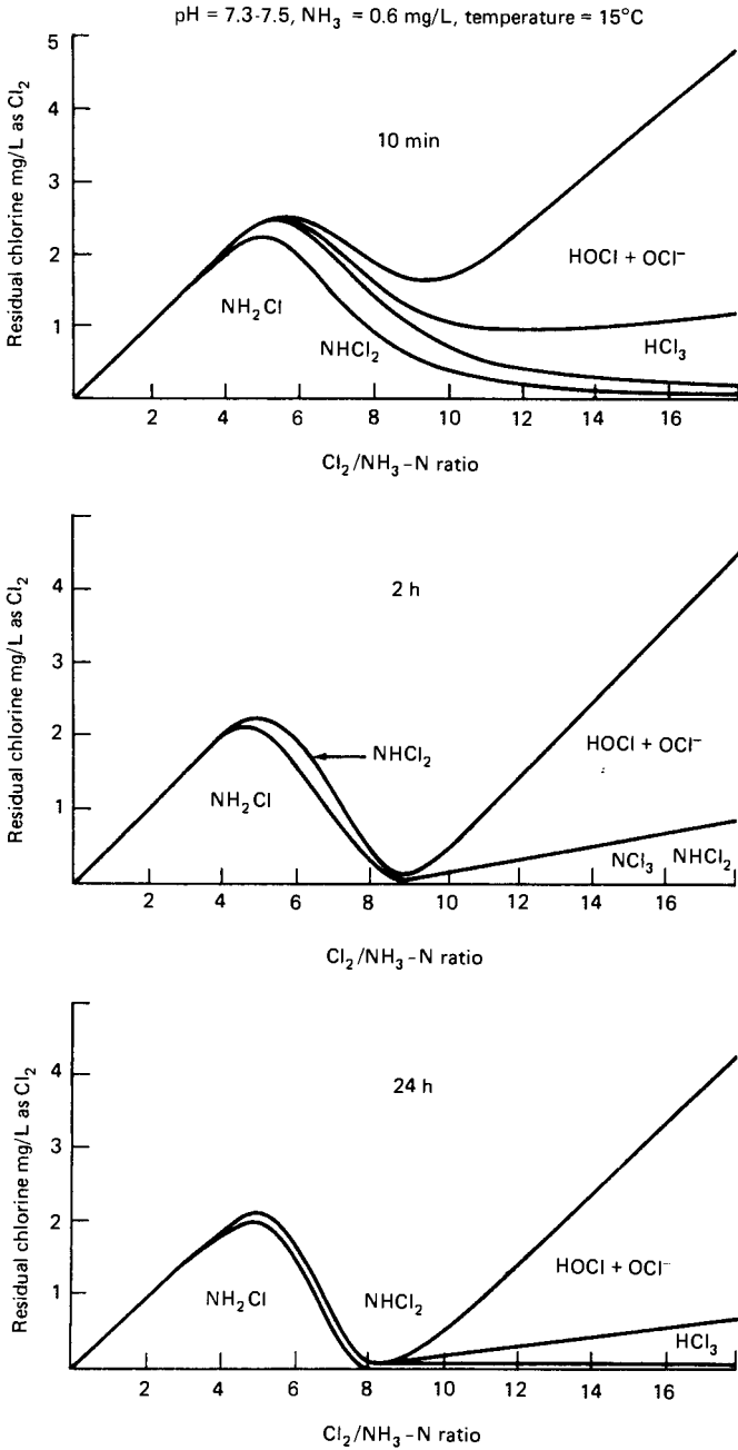
FIGURE 10.7 Free residual chlorine curves. (Source: A. Palin, "A Study of the Chloro Derivatives of Ammonia," Water Engineering , vol. 54, December 1950, p. 151.)
