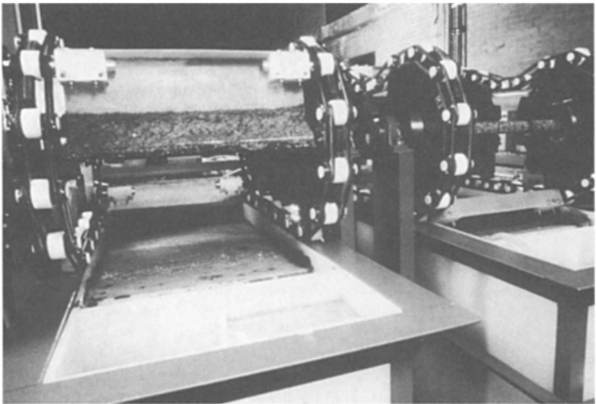
FIGURE 28.2 Parallel DAF tanks with mechanical scrapers (tanks 50 gpm with overflow rate of 6 gpm/ft 2 ). (Courtesy of CDM.)
