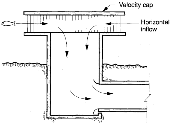
FIGURE 4.16 Velocity cap. (Courtesy of USFilter, Envirex Products.)
