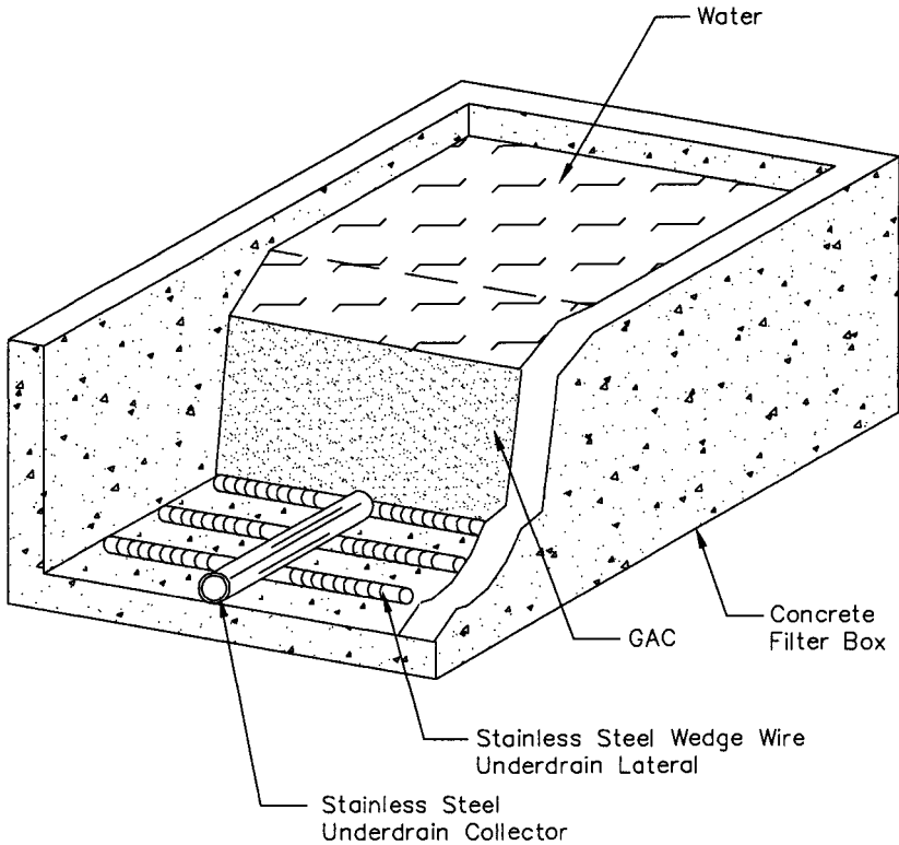
FIGURE 14.8 Wedge wire underdrain for GAC filters.
