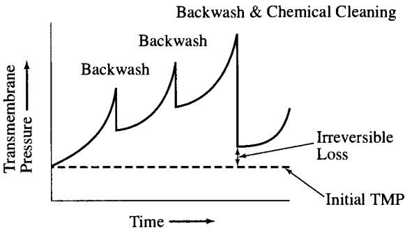
FIGURE 13.24 MF/UF TMP control with periodic backwashing and cleaning.
