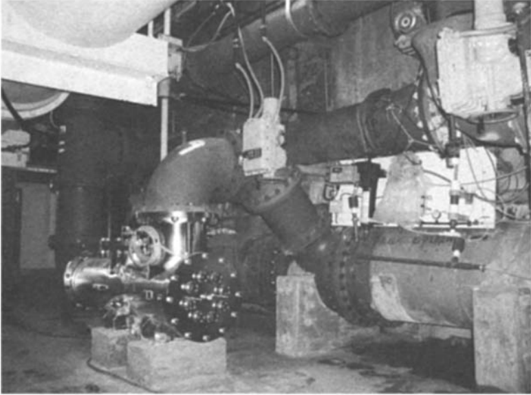
FIGURE 29.8 UV installation in existing filter gallery in Poughkeepsie, New York. (Photo courtesy of Jay Maggi and the Poughkeepsie Water Treatment Facility.)
