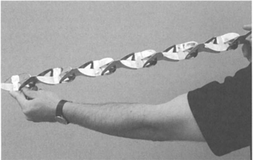
FIGURE 6.6 Typical static mixer. (Courtesy of Komax Systems, Inc., Wilmington, Calif.)
