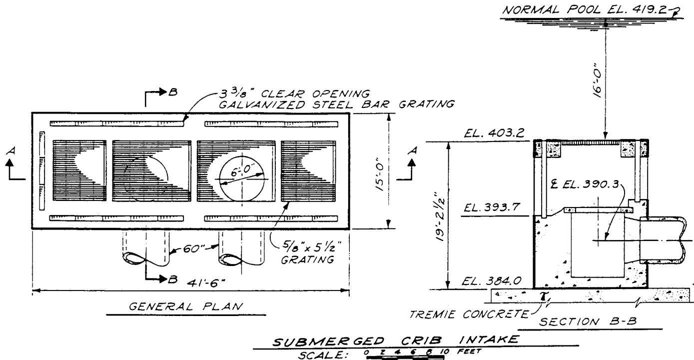
FIGURE 4.5 Louisville Water Company Ohio River intake (crib type).
