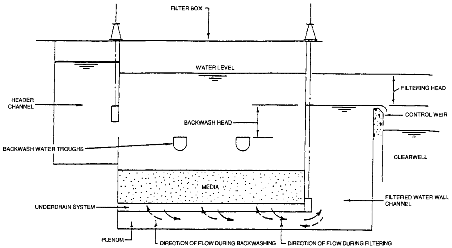
FIGURE 8.6 Self-backwashing filter. (Source: Monk, 1987.)
