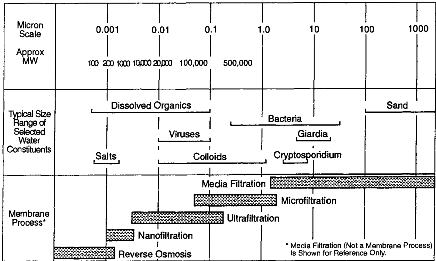
FIGURE 13.2 Pressure-driven membrane process application guide.
