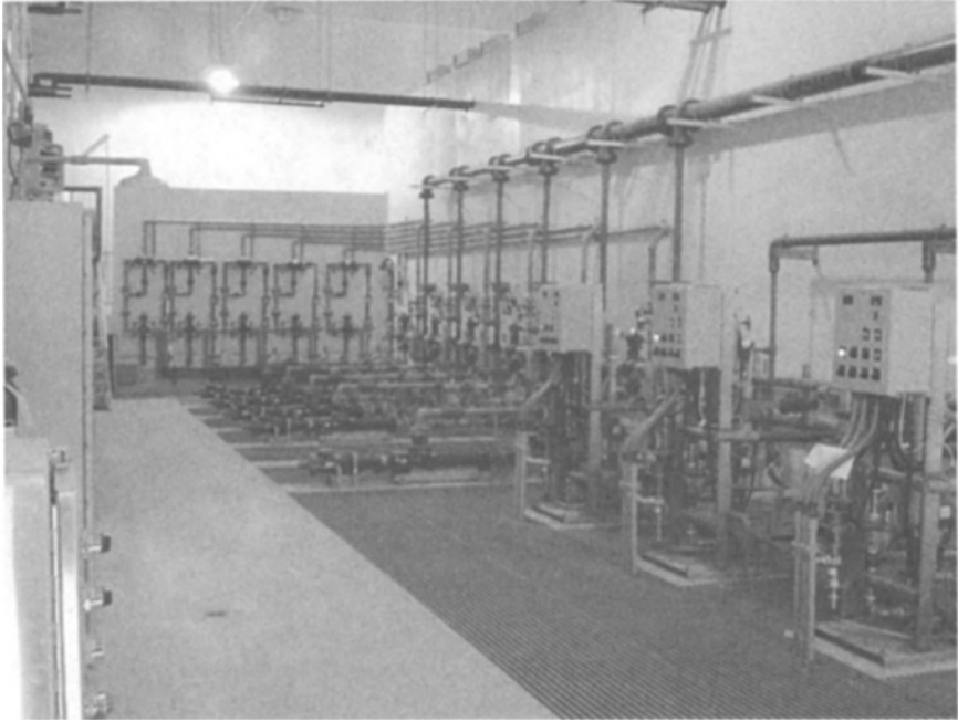
FIGURE 17.28 Polymer feed equipment. (Courtesy of City of Phoenix Water Services Department.)
