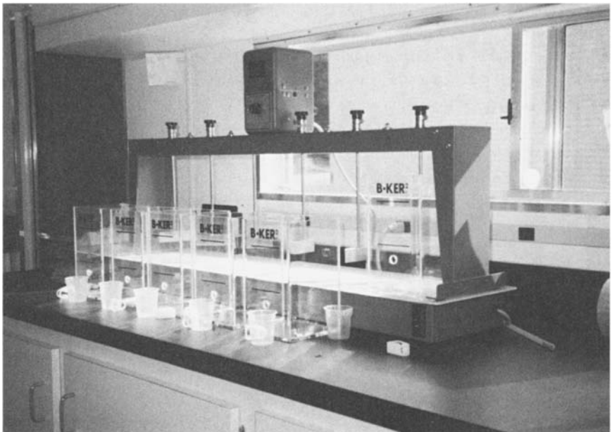
FIGURE 28.1 Typical jar test apparatus for bench-scale testing. (Courtesy of CDM.)
