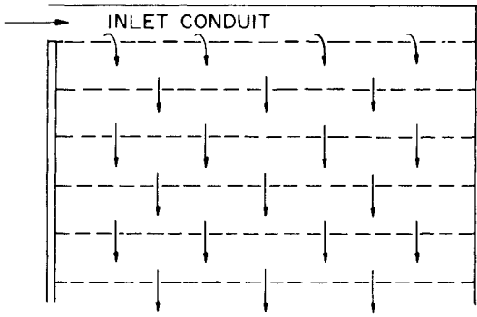
PLAN OF BAFFLE FLOCCULATOR
