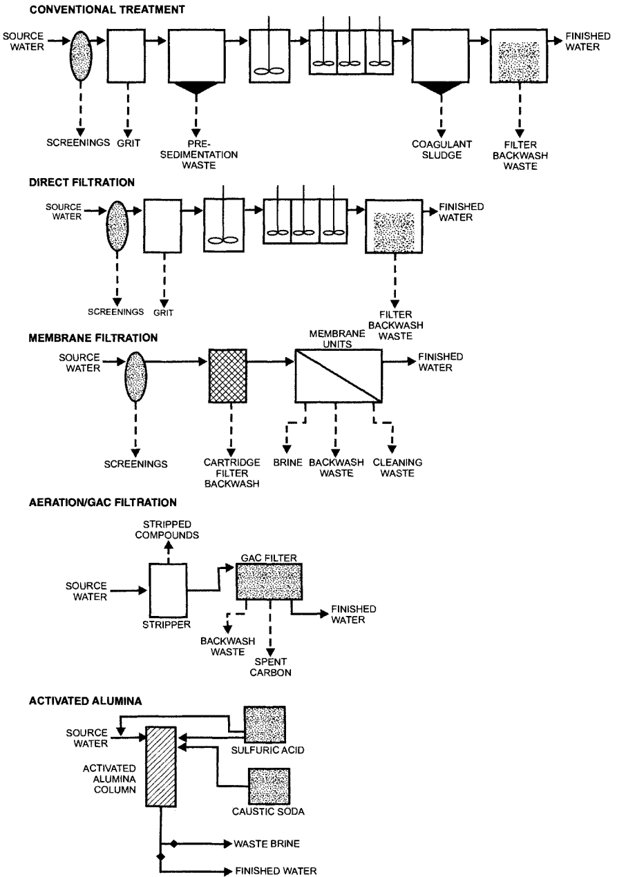
FIGURE 17.2 Water treatment plant wastes.
