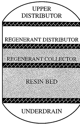
FIGURE 12.8 Split-flow exchanger.
