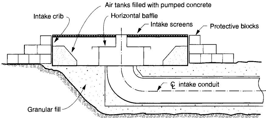
FIGURE 4.13 Lake intake crib.
