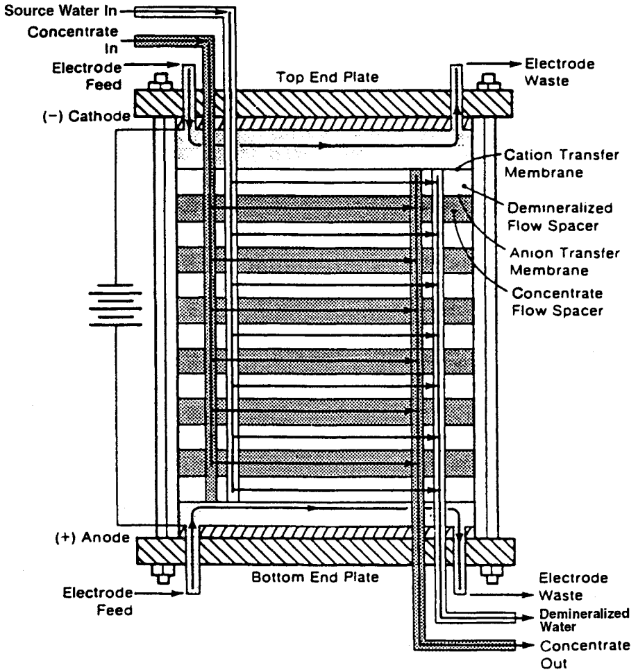
FIGURE 13.7 Typical ED membrane stack. (Adapted from Electrodialysis and Electrodialysis Reversal , AWWA M38, 1995.)
