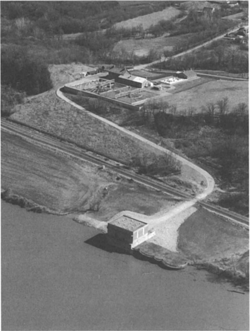
FIGURE 4.2 Missouri River intake (shore structures).
