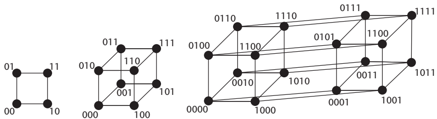
Fig 57 Spaces of all bit-strings of lengths 2, 3, and 4.
