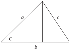
Fig 6 Splitting a triangle into two with right angles.
