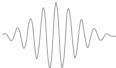
Fig 54 Wave packet.
