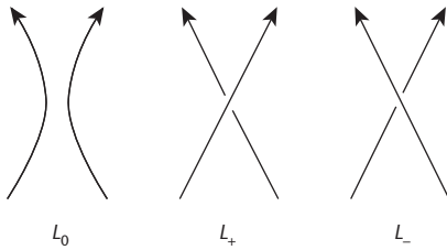
Fig 30 Jones moves.
