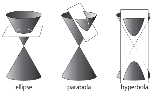
Fig 13 Conic sections.
