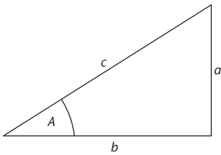
Fig 5 Trigonometry is based on a right-angle triangle.
