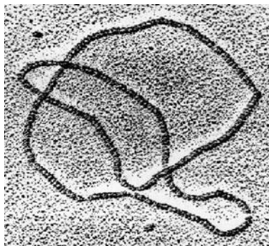
Fig 31 Loop of DNA forming a trefoil knot.
