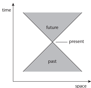
Fig 50 Minkowski space-time, with space shown as one-dimensional.
