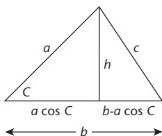
Fig 60 Splitting a triangle into two with right angles.
