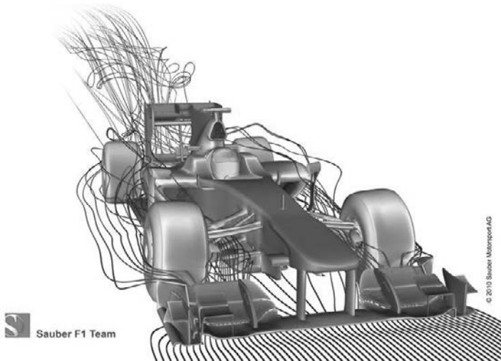
Fig 43 Computed air flow past a Formula 1 car.
