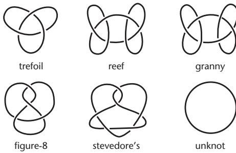
Fig 27 Five knots and the unknot.
