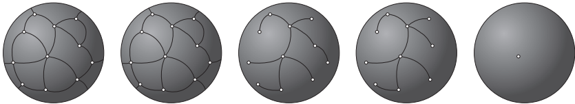
Fig 21 Key stages in simplifying a solid. Left to right: (1) Start. (2) Merging adjacent faces. (3) Tree that remains when all faces have been merged. (4) Removing an edge and a vertex from the tree. (5) End.
