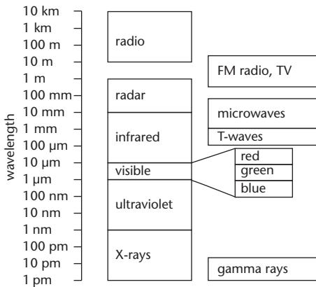
Fig 45 The electromagnetic spectrum.
