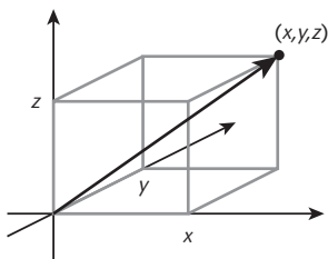
Fig 44 A three-dimensional vector.
