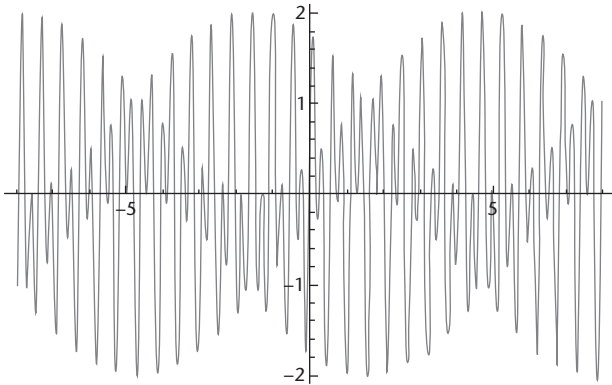
Fig 38 Beats.
