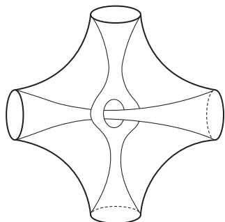
Fig 24 Hole-through-a-hole-in-a-hole.
