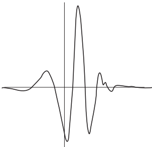
Fig 42 Daubechies wavelet.
