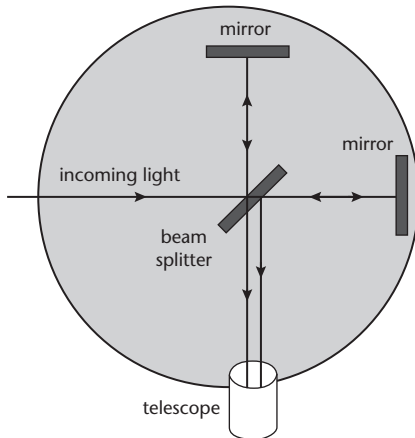
Fig 48 The Michelson–Morley experiment.
