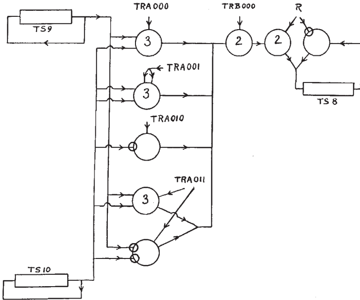
Fig. 29 Logical operations and TS 8.
