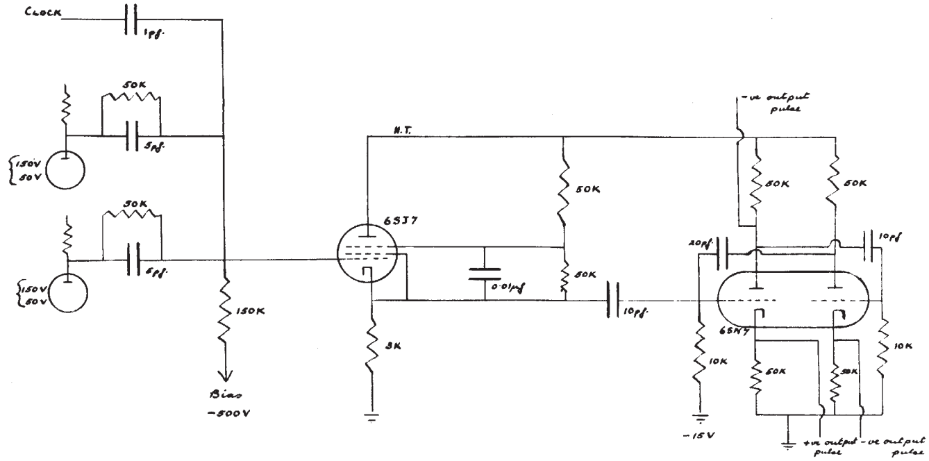
Fig. 47 'Limiting amplifier' circuit.
