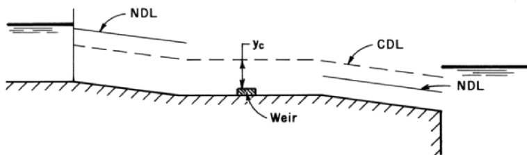
Fig. 5-20. Channels for Prob. 5-13
