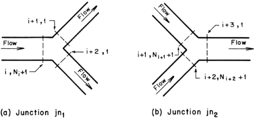
Fig. 6-12. Channel junctions
