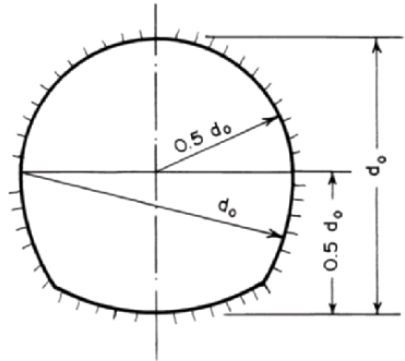
Fig. 4-8. Channel cross section for Prob. 4-10
