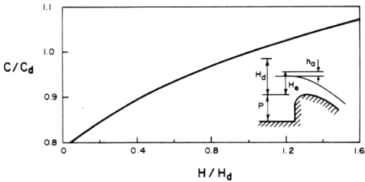
(b) Discharge coefficient at other heads
