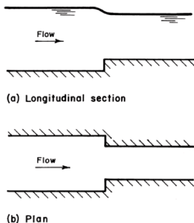
Fig. 7-4. Channel contractions
