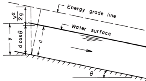
Fig. 2-6. Definition sketch for steep channel
