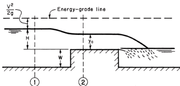
Fig. 7-8. Broad-crested weir
