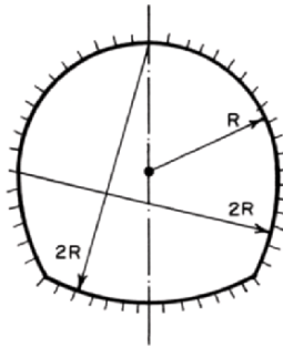
Fig. 3-12. Horseshoe section
