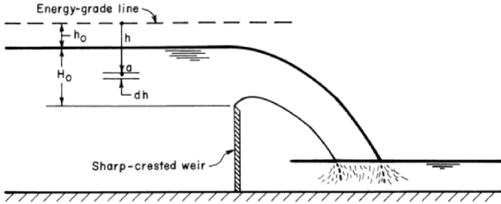
Fig. 7-7. Sharp-crested weir
