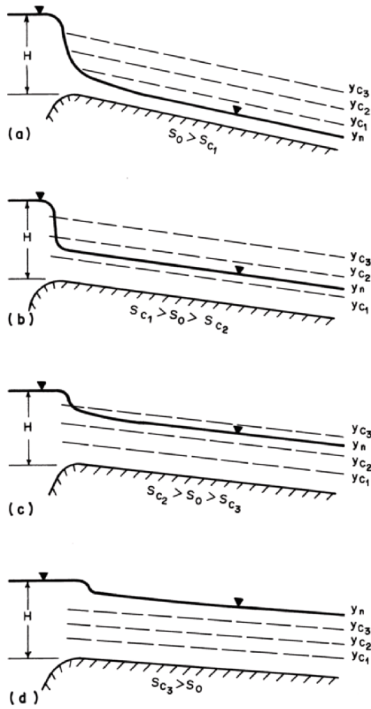
Fig. 5-16. Water surface profiles
