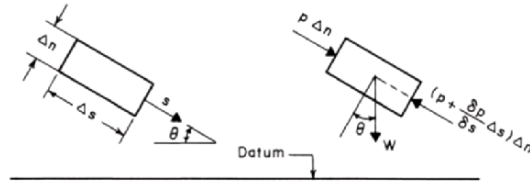
Fig. 2-3. Forces acting on fluid element
