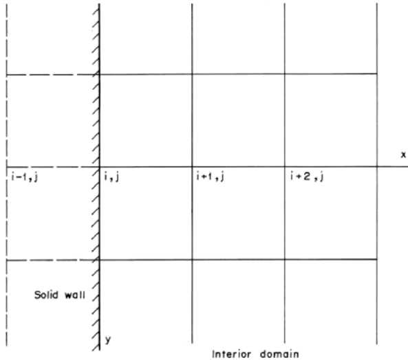
Fig. 15-4. Reflection boundary
