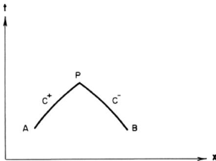
Fig. 13-1. Positive and negative characteristics
