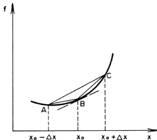
Fig. 14-1. Finite-difference approximations
