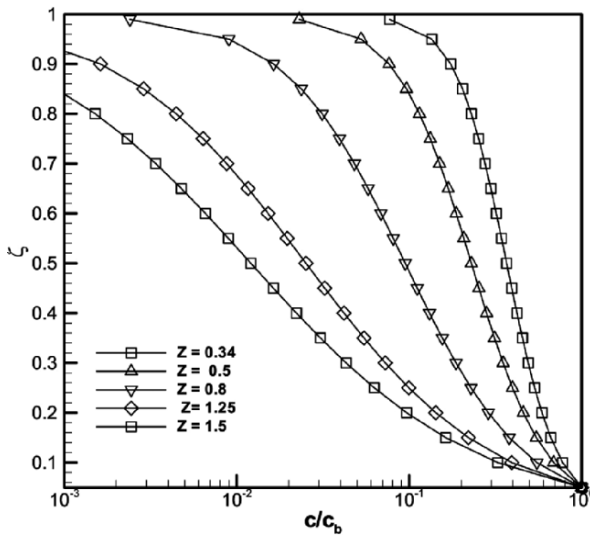
Fig. 16-7. Vertical distribution of suspended sediment concentration.
