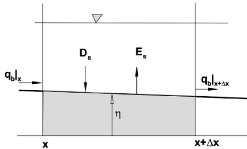
Fig. 16-5. Mass conservation at the river bed.
