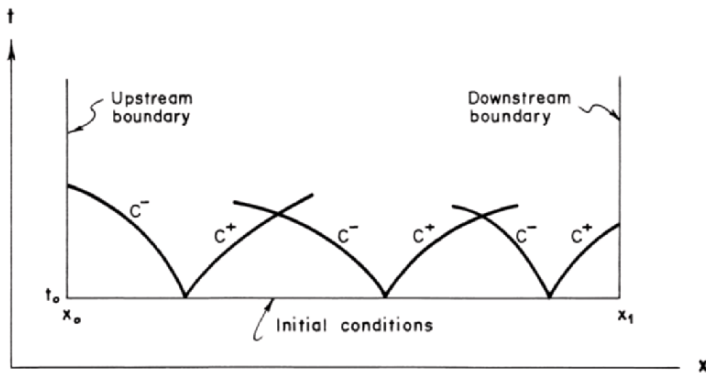
Fig. 13-5. Computaional domain for a one-dimensional system
