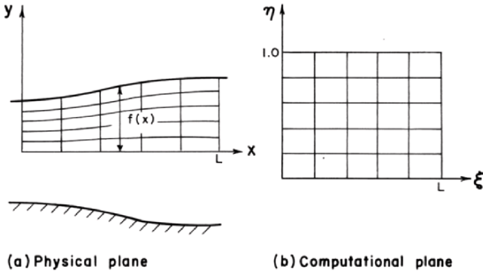
Fig. 8-3. Coordinate transformation
