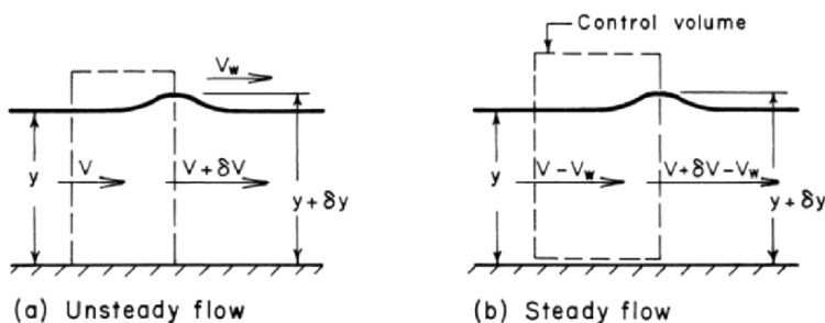
Fig. 3-2. Definition sketch for wave propagation
