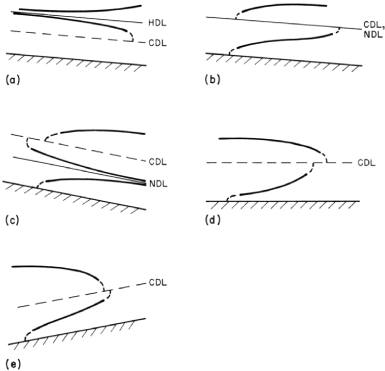
Fig. 5-19. Water-surface profiles
