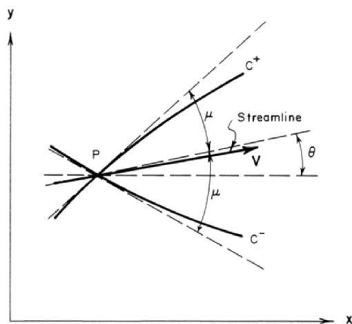
Fig. 8-2. Characteristic directions
