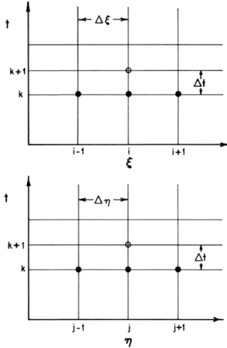
Fig. 8-8. Computational grid
