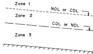
Fig. 5-2. Zones for classification of surface profiles
