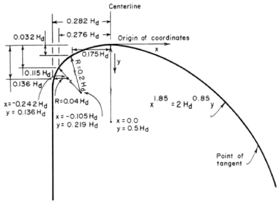
Fig. 7-19. Crest shape
