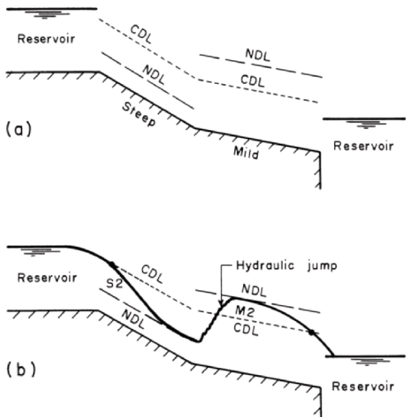
Fig. 5-5. Water surface profiles for Example 5-1
