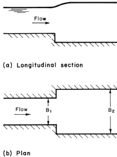
Fig. 7-2. Channel expansion
