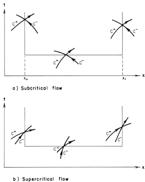
Fig. 13-6. Characteristics at the limits of computational domain (After Cunge, et al. [1980])
