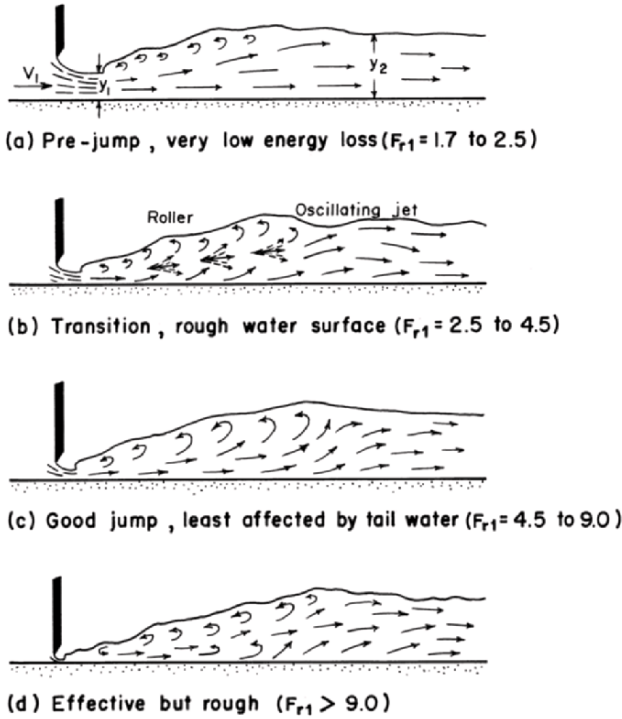
Fig. 7-11. Jump types (After Peterka [1958])
