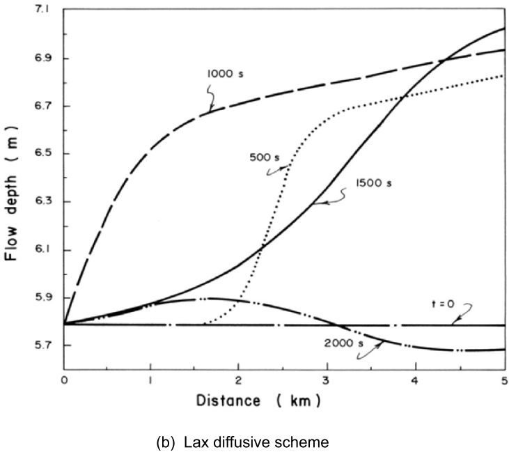
Fig. 14-6. Computed flow depths at different times
