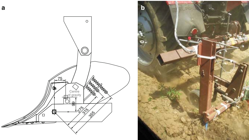
Fig. 3.5 Adapted plough (a) and cultivator (b) performing alternating rotary movement
