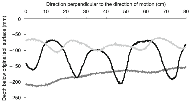
Fig. 4.2 Profile cross-sections of the tilled layer after tillage with a mouldboard plough ( dark grey curve ), a chisel plough ( black curve ) and a disc harrow ( light grey curve ) on a sandy loam. From Keller (2004)
