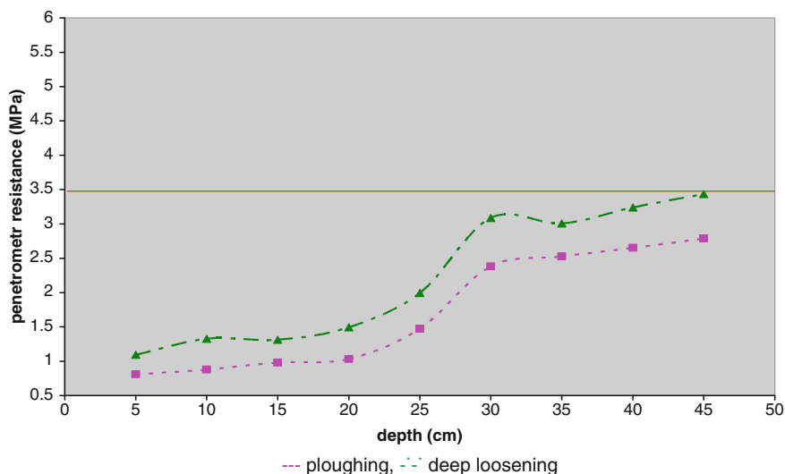
Fig. 2.3 Brown soil locality, spring measurement (Pokorný, 2007)
