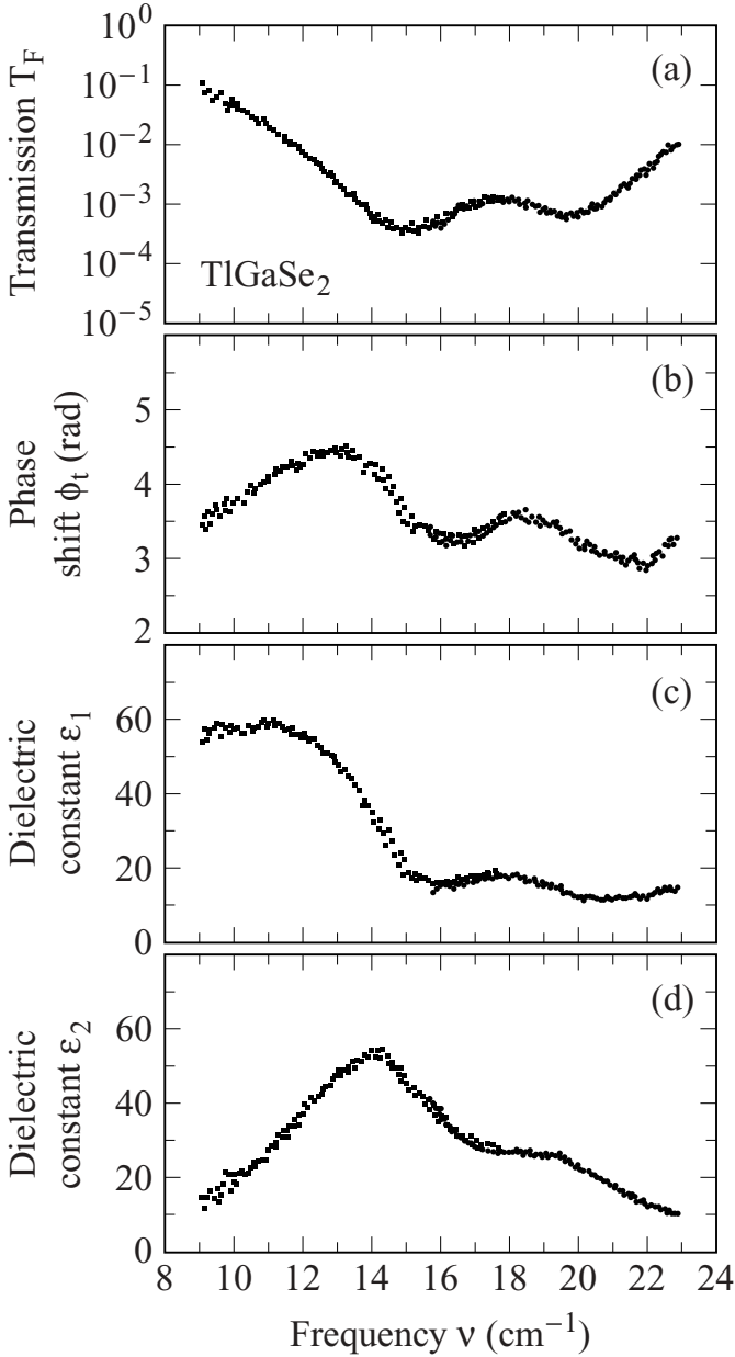
Fig. 10.1. Frequency dependence of the optical properties of TlGaSe 2 measured at T = 300 K by using a submillimeter wave Mach–Zehnder interferometer. (a) The transmission T_F(\omega) and (b) the phase \phi_t(\omega) spectra of a 0.079 mm thick plate are recorded. (c) The real part \epsilon'(\omega) and (d) the imaginary part \epsilon''(\omega) of the dielectric constant are calculated at each frequency according to Eqs (B.9), (B.10b), and (B.12) on the basis of the T_F(\nu) and \phi_t(\nu) spectra given in (a) and (b).
