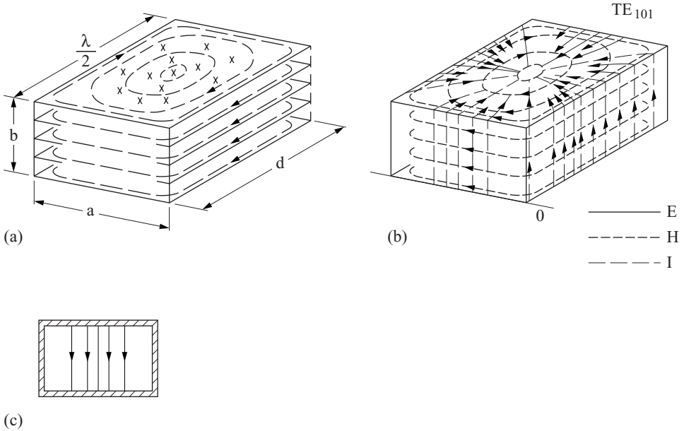
Fig. 9.8. Rectangular TE 101 cavity. (a) The electric field lines E span the space between the top and bottom wall while the magnetic field H circles around. (b) The current I runs up on the side walls and to the center of the top plate; (c) the electric field has its highest density in the center of the cavity.
