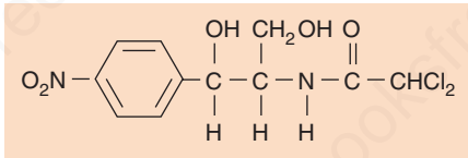
FIGURE 10-7 Chloramphenicol.
