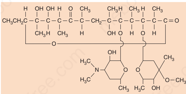
FIGURE 10-8 Erythromycin.
