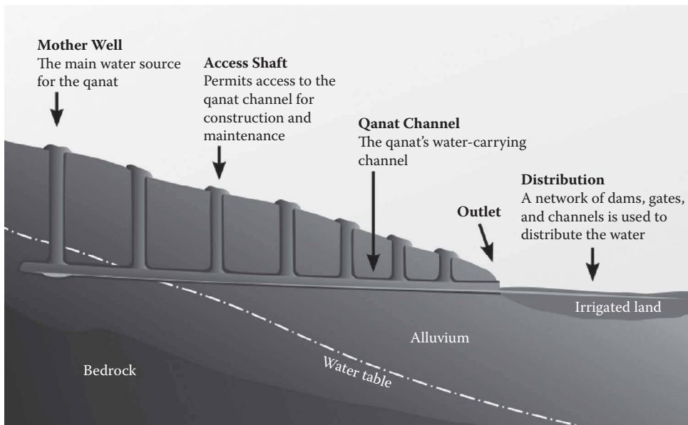
FIGURE 22.2 Karez system.
