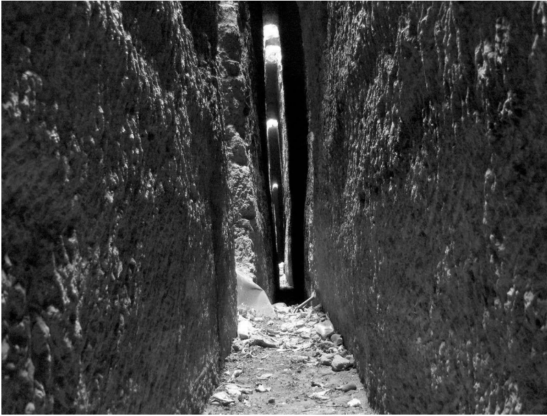
FIGURE 28.5 An interior view of the galería filtrante at the archaeological site of Xochiltlenango. It has a maximum height of 17 m and width of 80 cm. (Courtesy of Norma Peñafleres, 2004.)
