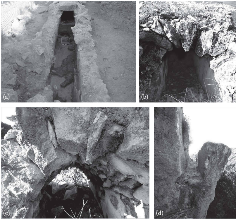
FIGURE 4.13 The aqueduct’s channel. (a) At Prineri Katifori. (b) At the Roman quarry. (c) Detail of the channel’s vaulted top. (d) At Kourtzi thermal springs. (By permission of Y. Kourtzellis.)
