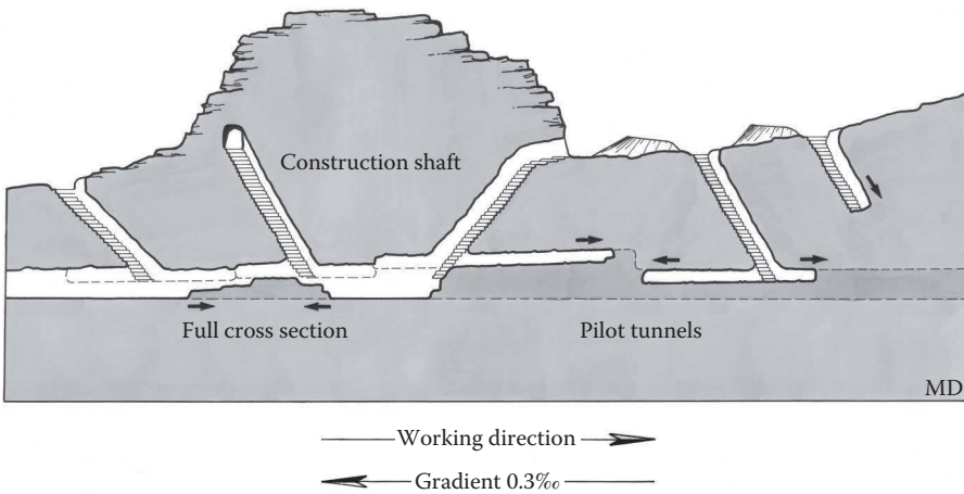
FIGURE 11.17 Tunneling stages.
