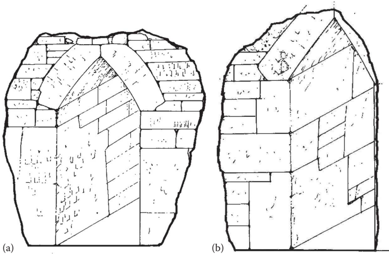
FIGURE 5.13 The support masonry lining made of large stone blocks (a) Ch. 198 and (b) Ch. 263. (From Zambas, C. et al. Study for the restoration of the Aqueduct of Eupalinos. Samos Island. Unpublished Study in Greek. Egnatia Odos SA, Thessaloniki, Greece, 2010. Surveying by C. Zambas. Drawing by G. Thomas. With Permission.)
