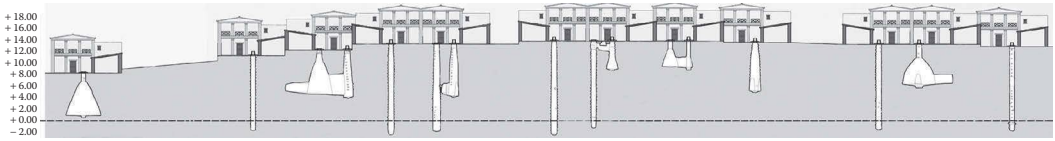
FIGURE 4.5 Hypothetical representation of typical house blocks and underground water structures in section. (Courtesy of A. Bendermacher-Gerosis and G. Peppas.)
