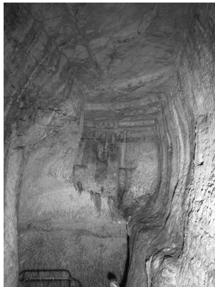
FIGURE 5.8 The face of the north bore at the meeting point. At the bottom of the picture is the south bore eastside. The face of the south bore is at the bottom-left corner.
