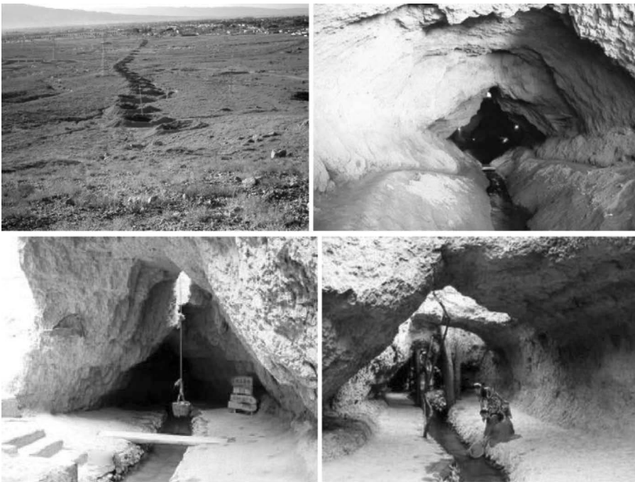
FIGURE 25.9 Ancient karez at Pishin District, Quatta, Balochistan. (From Tanver, A., Traditional Karez Water Management in Pakistan , SCOPE, Pakistan, 2007, p. 16. With Permission.)
