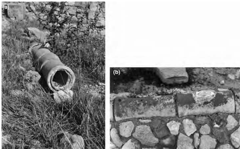
Figure 12.8 Terracotta pipeline for domestic water supply with a small aperture, used as an inspection hole, covered by a flat stone, sealed with gypsum plaster, from Kourion, second century AD.
