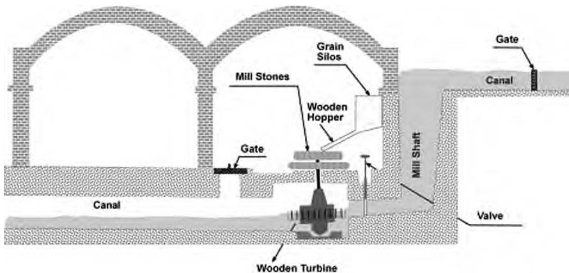
Figure 5.30 Cross section of a water mill
