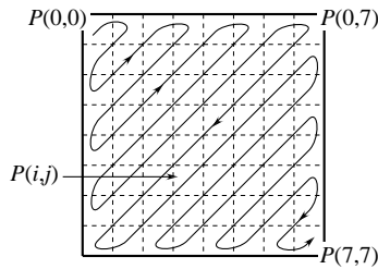
Figure 6.32 – Reading of the DCT coefficients
