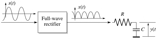
Figure 12.1 – Full-wave rectifier
