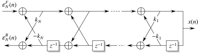
Figure 11.9 – The lattice synthesis filter
