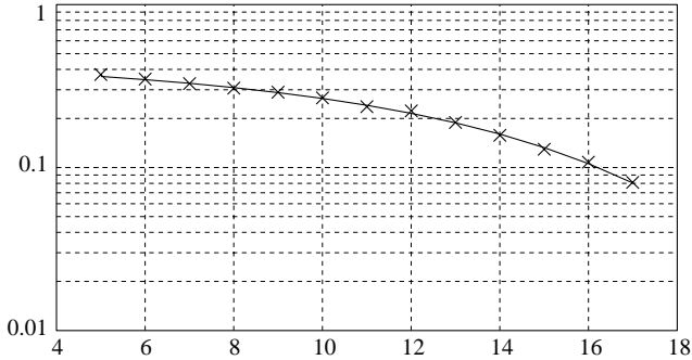
Figure H12.22 – Symbol-by-symbol detection of a Zero Forcing equalizer’s output for a binary transmission. The equivalent channel has the coefficients g_0 = 1 , g_1 = -1.4 , g_2 = 0.8 . The x ’s indicate the probabilities obtained through 5,000 simulations for different values of the signal-to-noise ratio in dB
