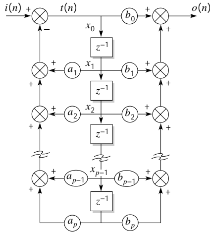
Figure 5.1 – Processing architecture
