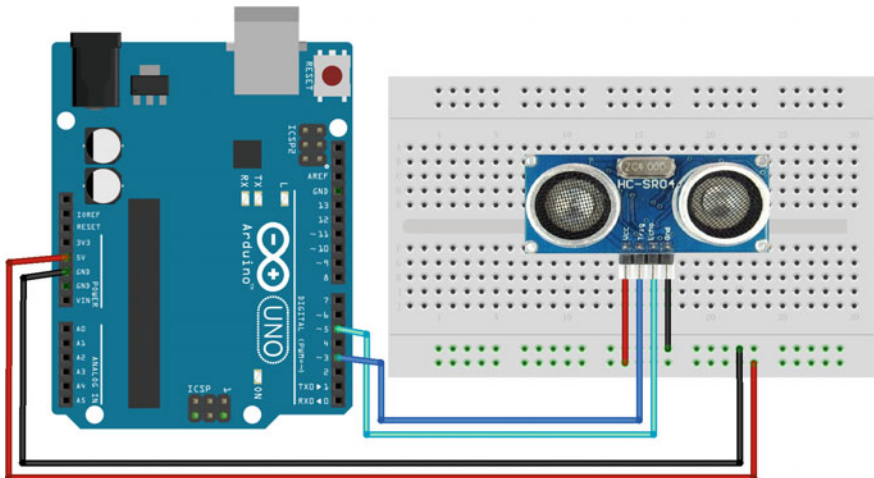
Fig. 3.21 A diagram of the layout of the HC-SR04 and UNO R3
