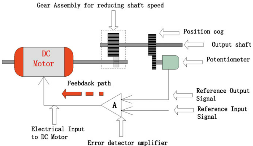
Fig. 4.14 Schematic of DC servo motor
