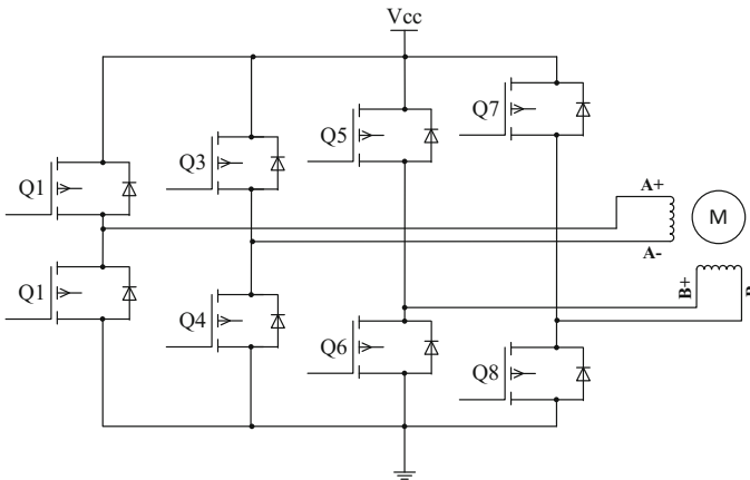
Fig. 4.9 Driven circuits for bipolar stepper motor
