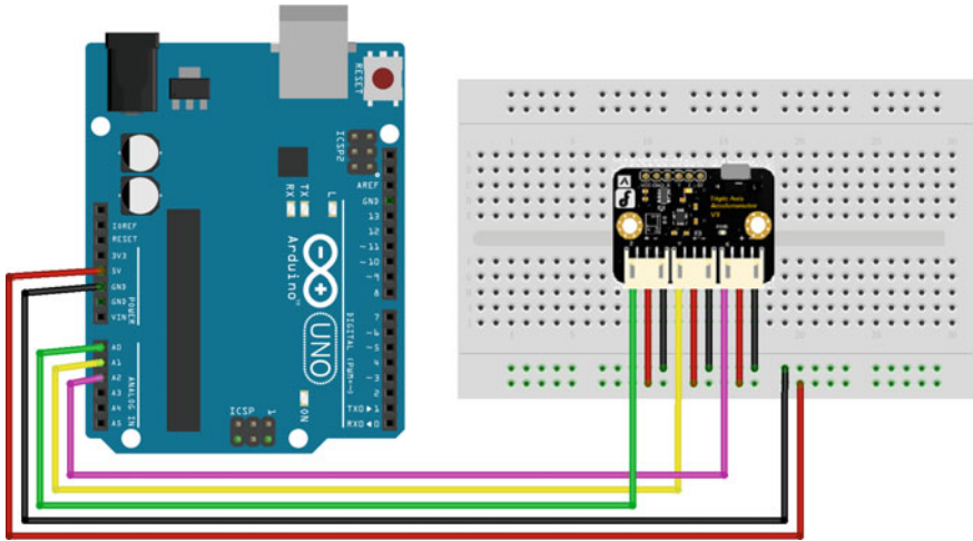
Fig. 3.40 A diagram of the layout of the DFR0143 and UNO R3
