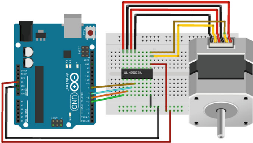
Fig. 4.12 UNO board and driven circuit diagram
