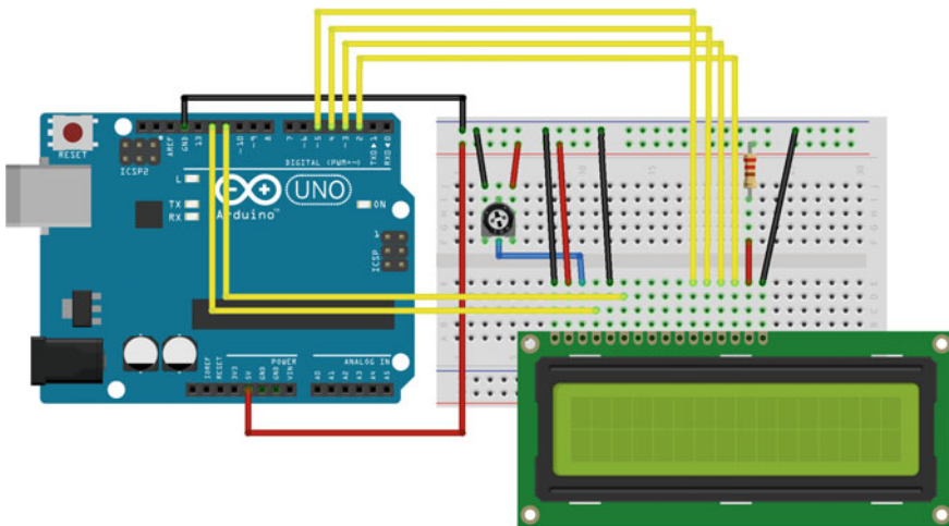
Fig. 6.3 Connecting diagram between UNO and LCD1602
