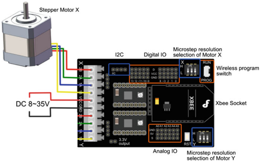
Fig. 4.13 Stepper motor and Romeo board connection diagram
