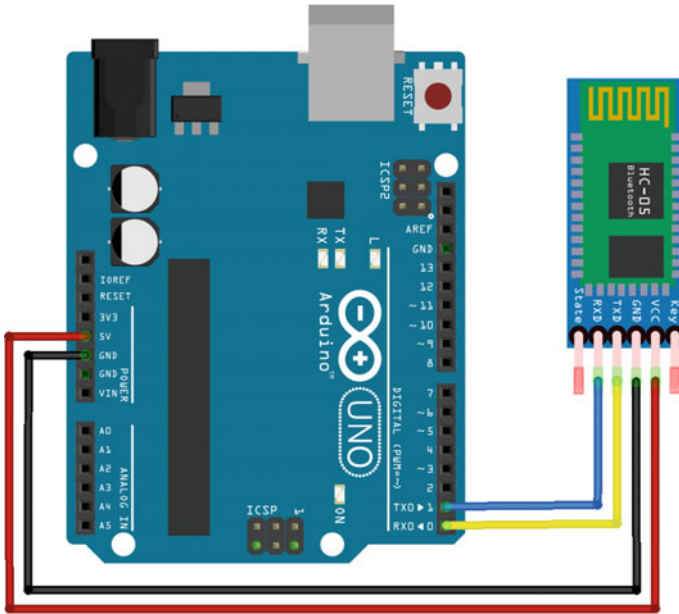
Fig. 6.7 Bluetooth connecting diagram
