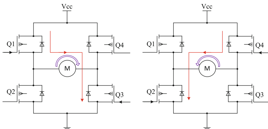
Fig. 4.1 H-bridge and the direction of motor
