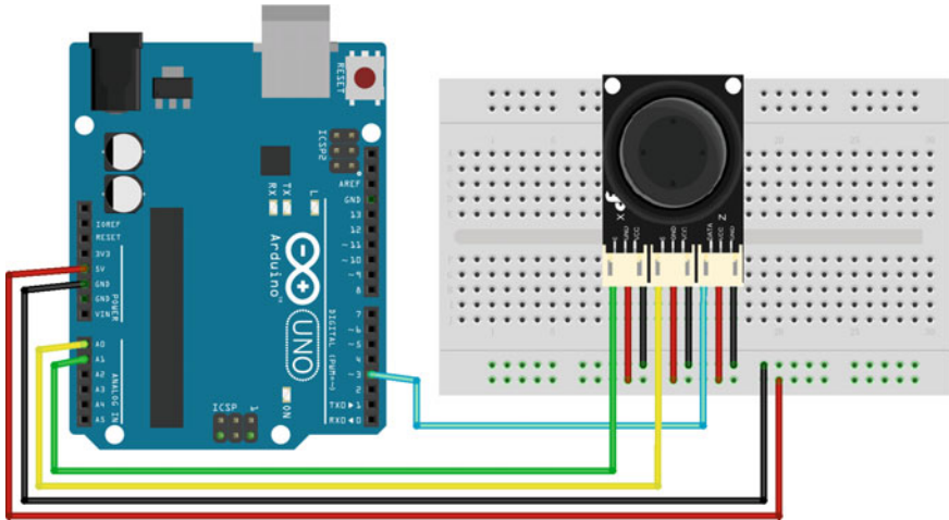
Fig. 3.26 A diagram of the layout of the DFR0061 and UNO R3
