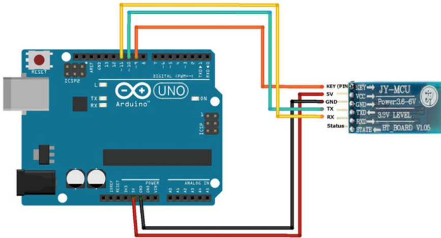
Fig. 5.12 A diagram of the layout of the HC-05 and UNO R3
