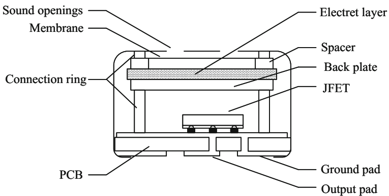
Fig. 3.42 The diagram of an electret condenser microphone
