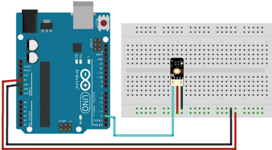
Fig. 3.17 A diagram of the layout of the SEN0017 and UNO R3
