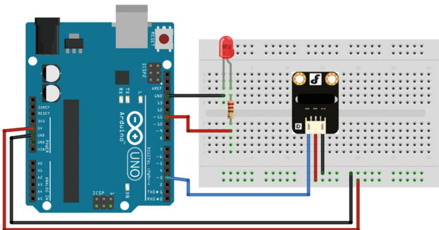
Fig. 3.48 A diagram of the layout of the DFR0027 and UNO R3
