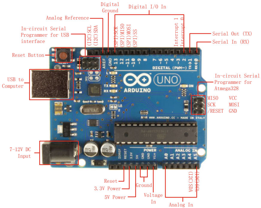
Fig. 1.1 Arduino UNO interface board
