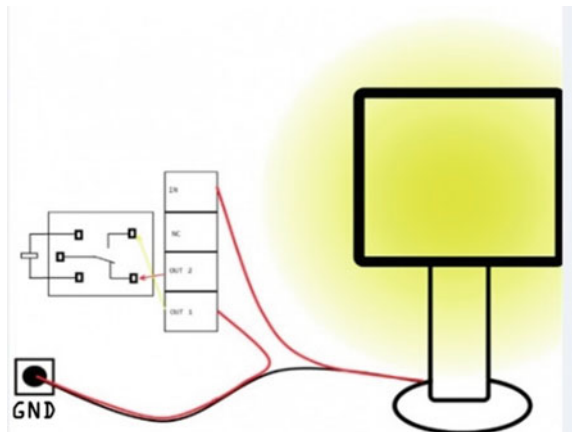
Fig. 8.5 Diagram of plugging in electric bolt or lamp
