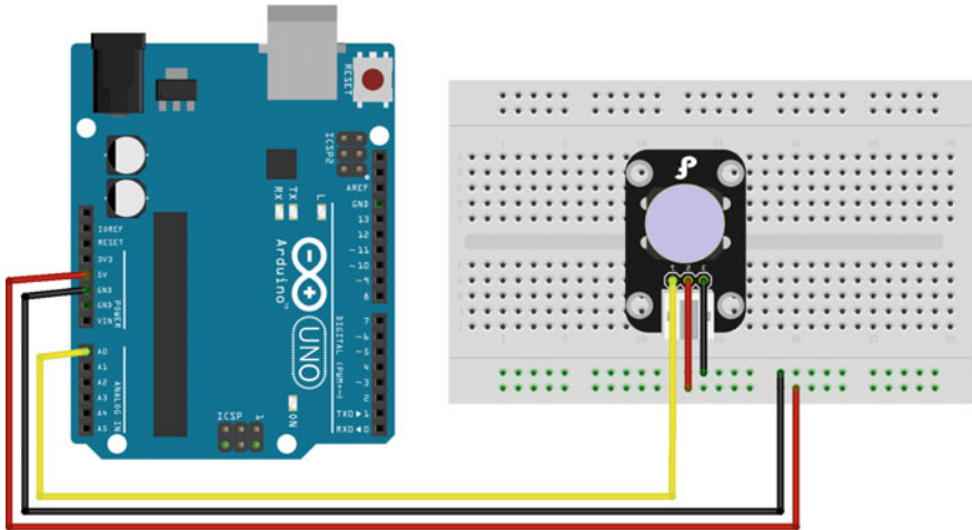
Fig. 3.29 A diagram of the layout of the DFR0049 and UNO R3
