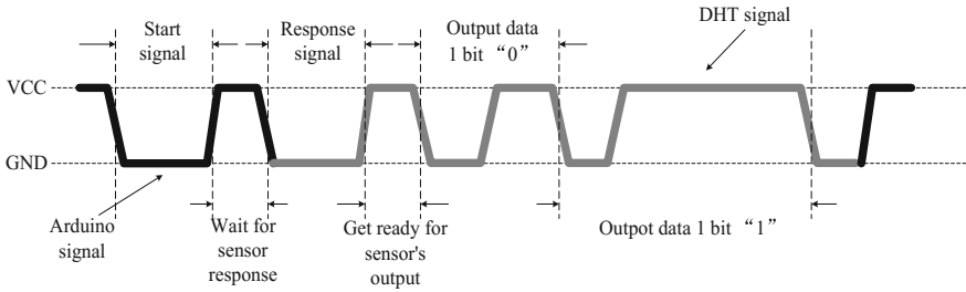
Fig. 3.12 Overall communication process
