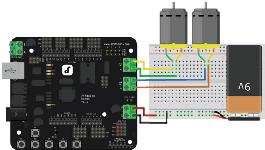
Fig. 4.3 Romeo motor connection diagram
