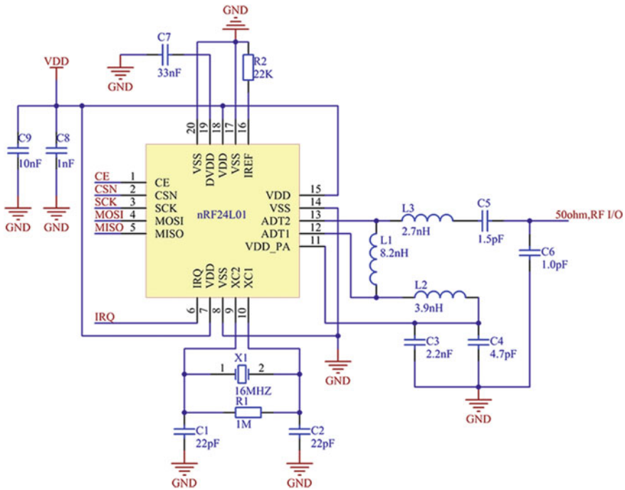
Fig. 5.7 Schematic of NRF24L01 wireless RF transceiver module
