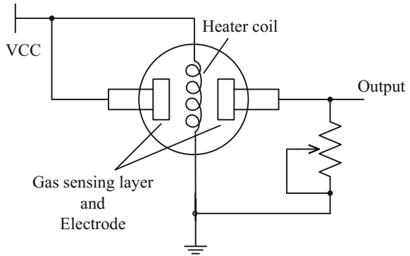
Fig. 3.28 The schematic of a gas sensor
