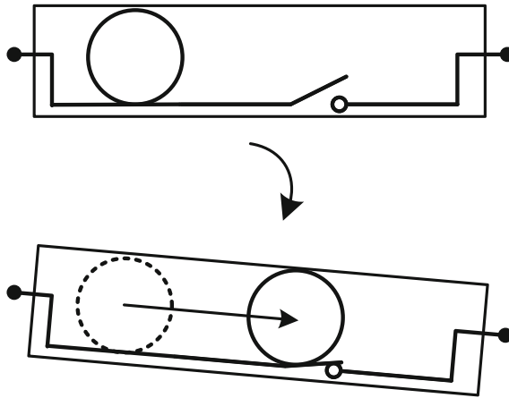
Fig. 3.37 The working principle of a tilt sensor
