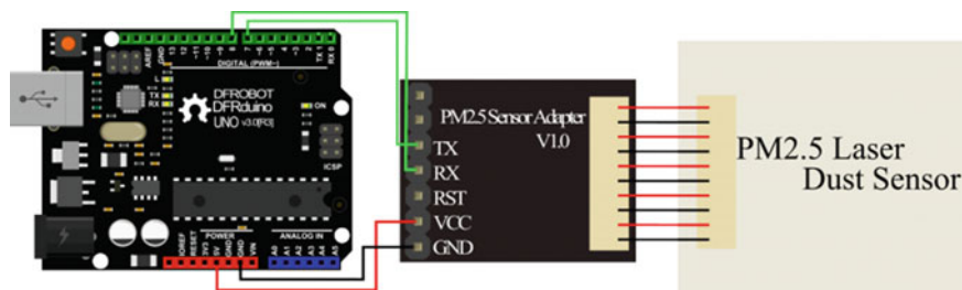
Fig. 6.2 Connecting diagram between UNO and SEN0177
