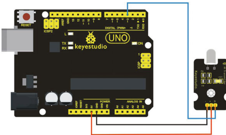
Fig. 5.2 A diagram of the layout of the IR transmitter and UNO R3
