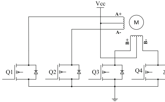
Fig. 4.8 Driven circuits for unipolar stepper motor
