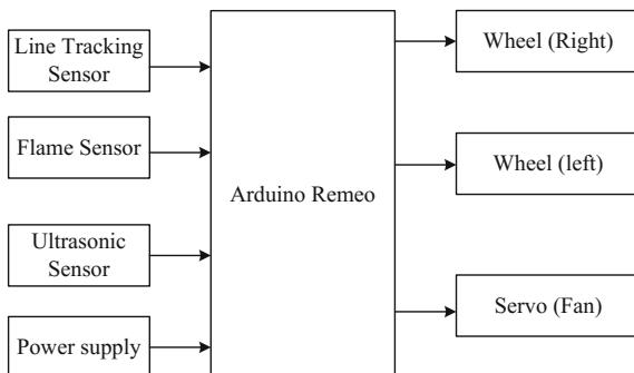
Fig. 7.3 Structure diagram of fire-fighting robot
