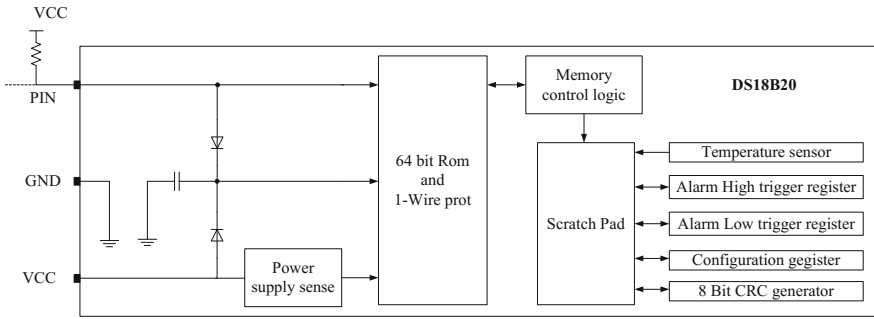
Fig. 3.4 Block diagram of DS18B20
