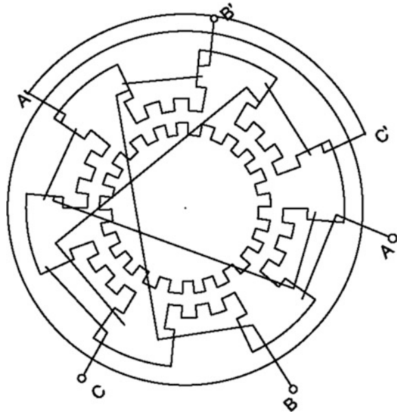
Fig. 4.5 Structure of stepper motor
