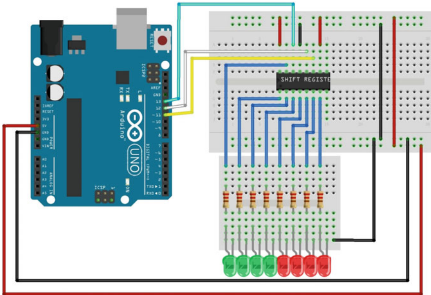
Fig. 2.3 Circuit layout for the shift register
