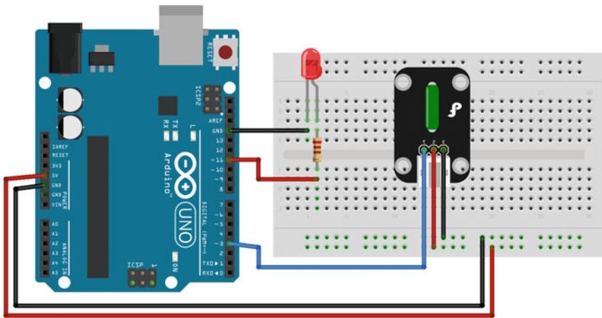
Fig. 3.38 A diagram of the layout of the DFR0028 and UNO R3
