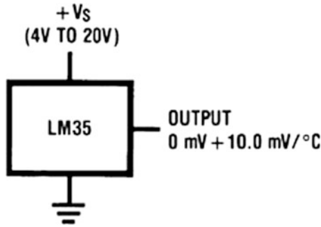
Fig. 3.8 Basic centigrade temperature sensor
