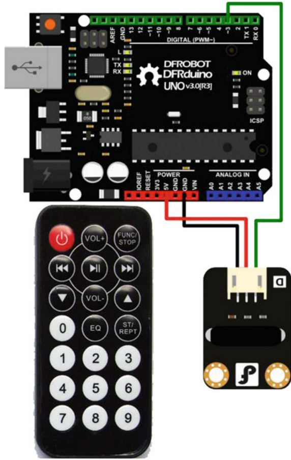
Fig. 5.4 A diagram of the layout of DFR0107 and UNO R3
