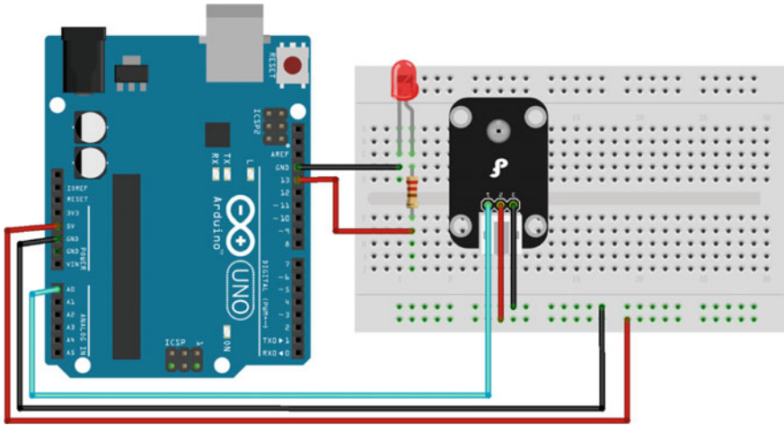
Fig. 3.2 A diagram of the layout of the DFR0026 and UNO R3
