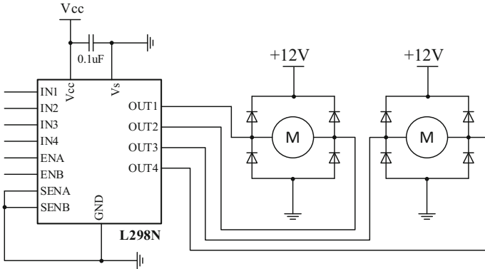
Fig. 4.2 Schematic of L298N driven circuit
