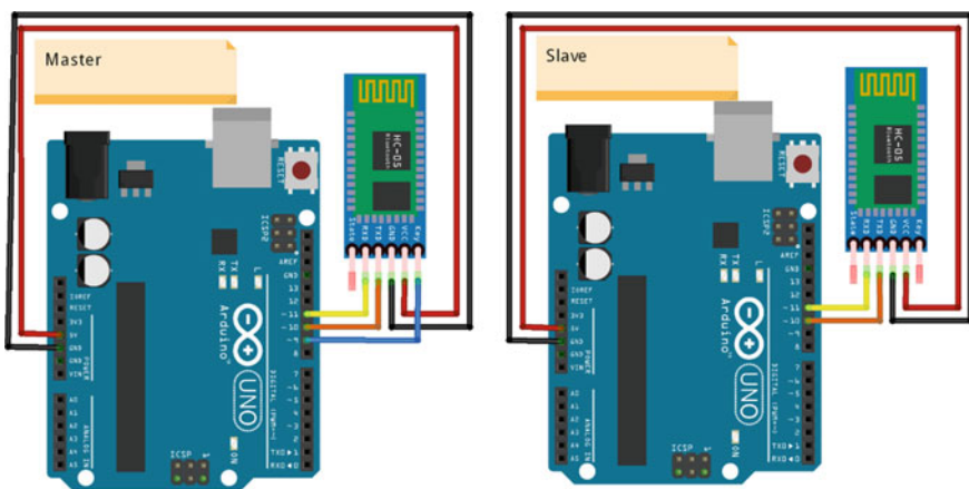
Fig. 5.14 The diagram of layout of two HC-05 modules
