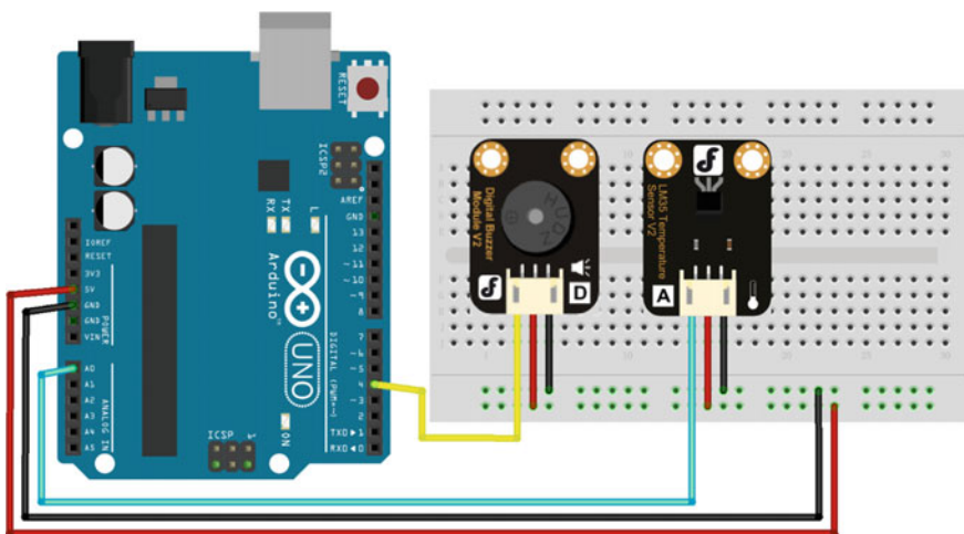
Fig. 3.9 A diagram of the layout of the DFR0023, DFR0032, and UNO R3
