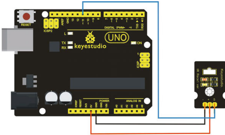
Fig. 5.3 A diagram of the layout of the IR receiver and UNO R3
