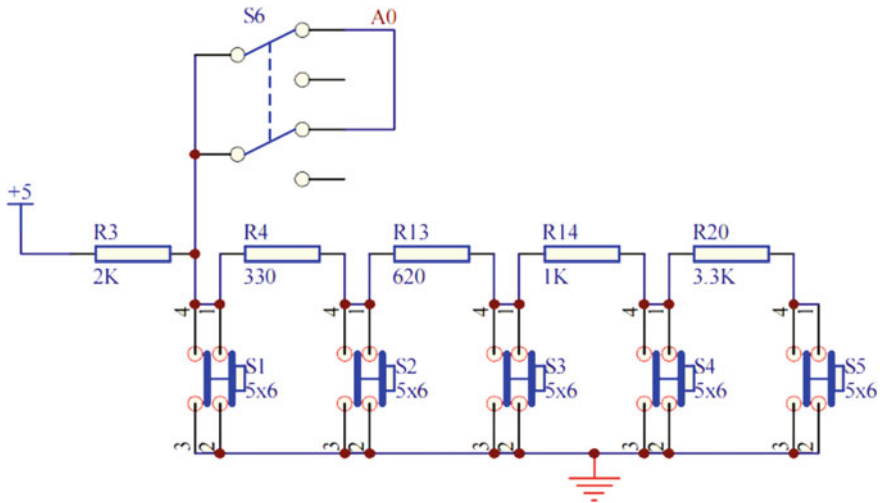
Fig. 4.4 Schematic of button-on-board of Romeo board
