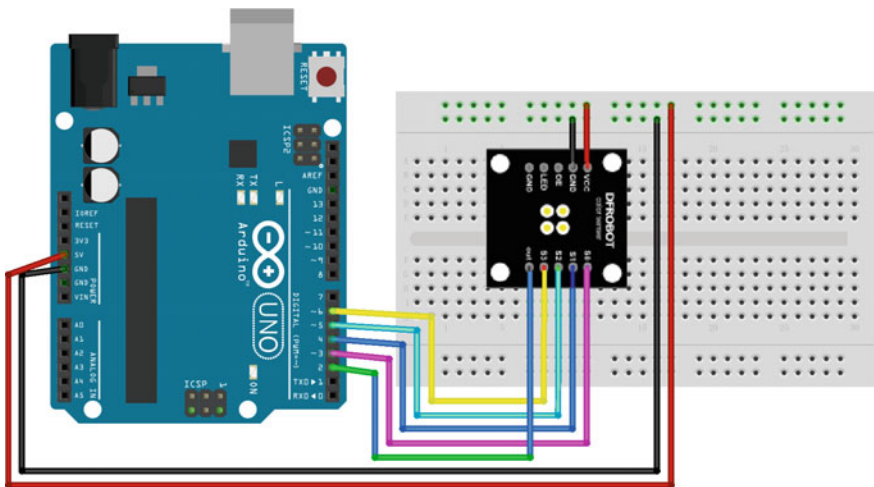
Fig. 3.35 A diagram of the layout of the SEN0101 and UNO R3
