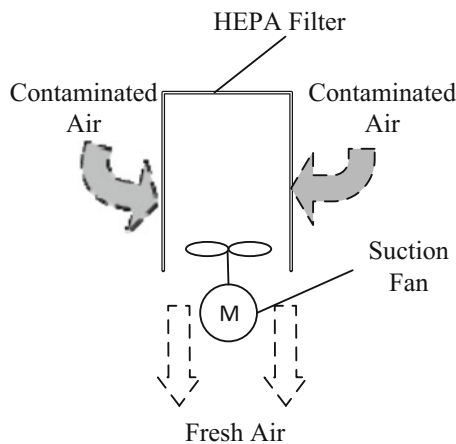
Fig. 6.5 The filtering principle of air indoor
