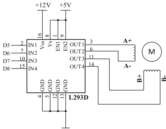
Fig. 4.10 Driving one stepper motor using L293D
