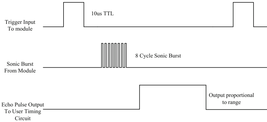
Fig. 3.20 Timing diagram
