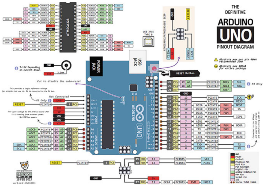
Fig. 1.2 Arduino Uno R3 pinout diagram
