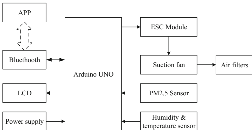
Fig. 6.1 Structure diagram of the indoor air quality monitor
