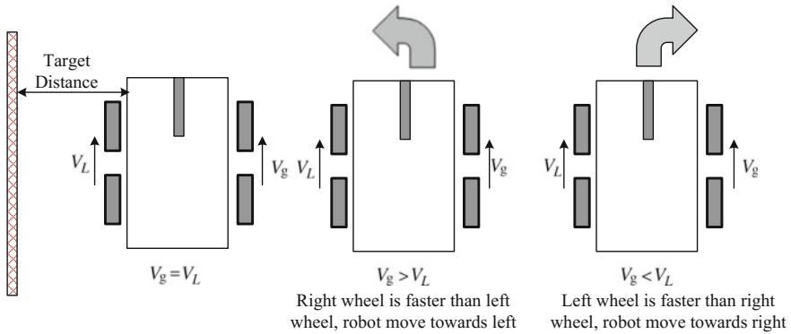
Fig. 7.5 The schematic of wall-following
