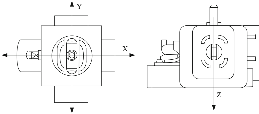
Fig. 3.25 The diagrams of X, Y, and Z axes of Joystick
