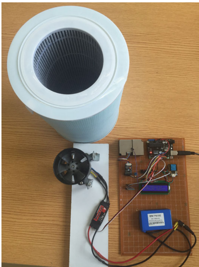
Fig. 6.9 The photo of air quality monitor
