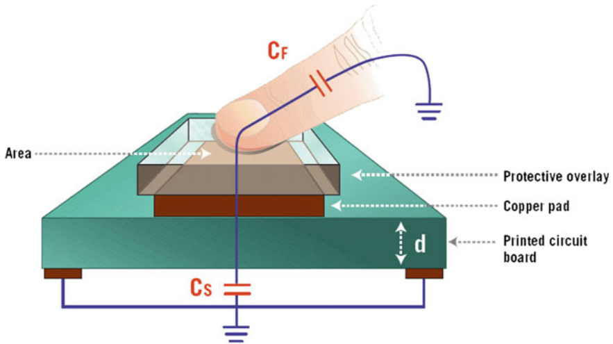
Fig. 3.52 The principle of capacitive touch sensor
