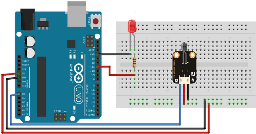
Fig. 3.50 A diagram of the layout of the DFR0076 and UNO R3
