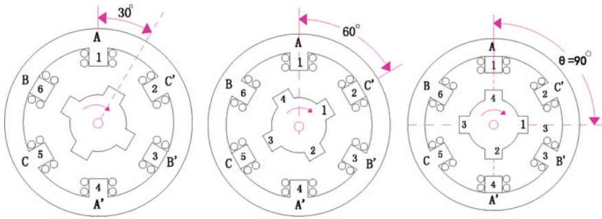
Fig. 4.6 Sequence of supplying current to stator coil
