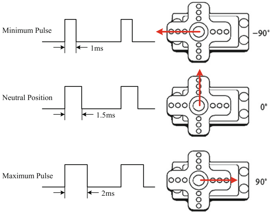
Fig. 4.15 Pulse widths and their corresponding position of the servo motor
