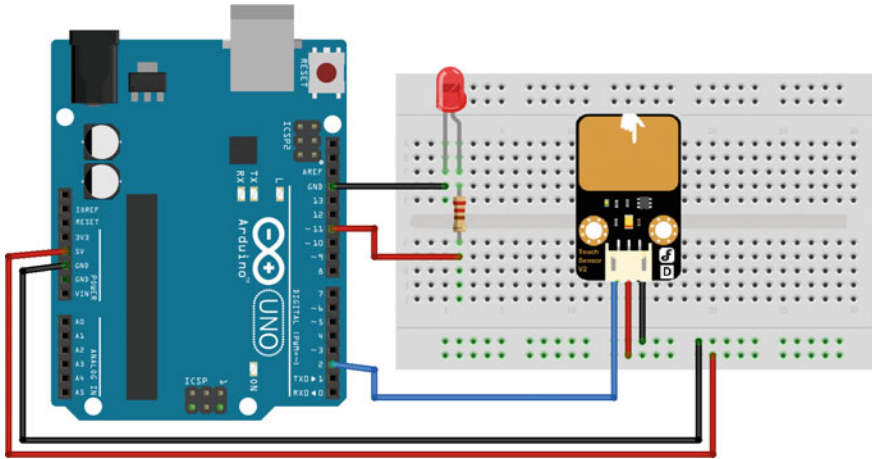
Fig. 3.53 A diagram of the layout of the DFR0030 and UNO R3
