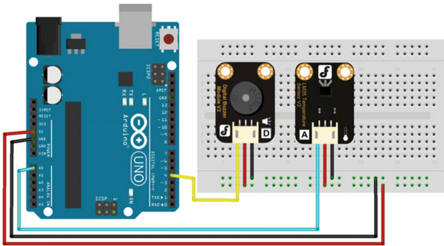
Fig. 3.6 A diagram of the layout of the DFR0024, DFR0032 and UNO R3
