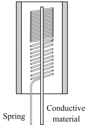
Fig. 3.47 The diagram of a vibration switch
