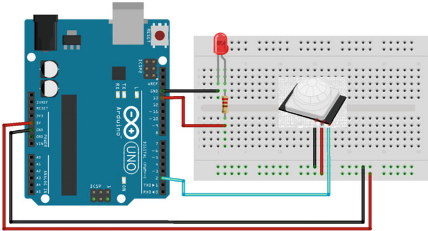
Fig. 3.23 A diagram of the layout of the SEN0018 and UNO R3
