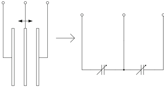
Fig. 3.39 The simplified model of a g-cell structure
