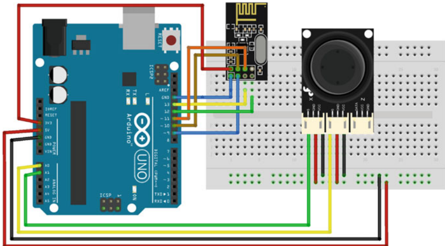
Fig. 5.8 A transmitter diagram of the layout of the nRF24L01 and UNO R3
