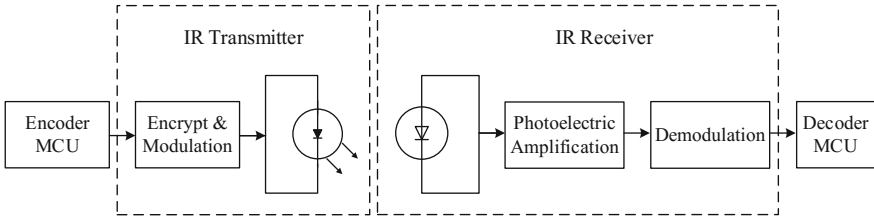
Fig. 5.1 IR transmitter/receiver principle
