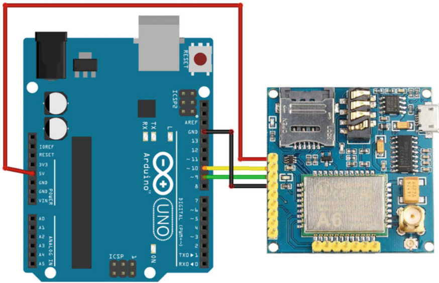
Fig. 5.19 The diagram of layout of A6 GSM/GPRS module
