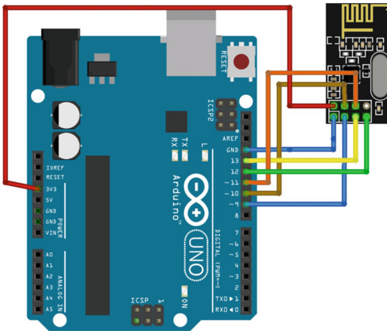
Fig. 5.9 A Receiver diagram of the layout of the nRF24L01 and UNO R3
