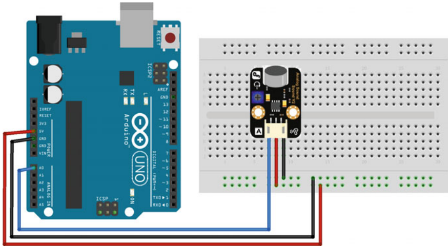
Fig. 3.43 A diagram of the layout of the DFR0034 and UNO R3
