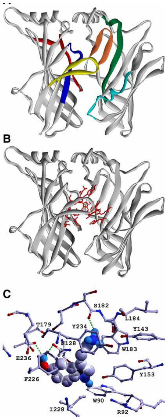
Fig. 4. (continued) Residues (black) are superimposed upon two adjacent subunits from the extracellular domain. Data from ref. 62. (C) The proposed orientation of 5-HT in the 5-HT 3 receptor ligand-binding site. Modified from ref. 62.
