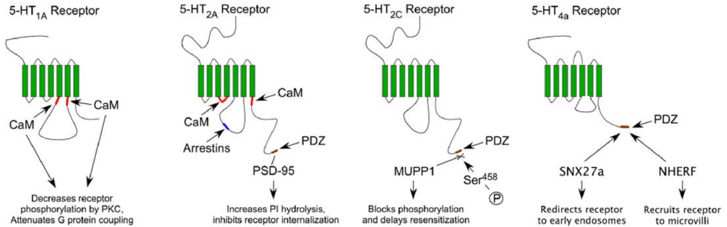
Fig. 2. Novel receptor-interacting partners of selected 5-HT receptors, their interaction domains on the receptors, and consequences of the interactions. Abbreviations: CaM, Ca 2+ /calmodulin; PDZ, a protein interaction domain termed postsynaptic density 95/discs large/ZO-1; PSD-95, a key protein component of the excitatory postsynaptic density; MUPP1, multi-PDZ-domain protein; SNX27a, a member of the new sorting nexin family of proteins; NHERF, NHE regulatory factor. MUPP1 prevents phosphorylation of serine-458 of the 5-HT 2C receptor.
