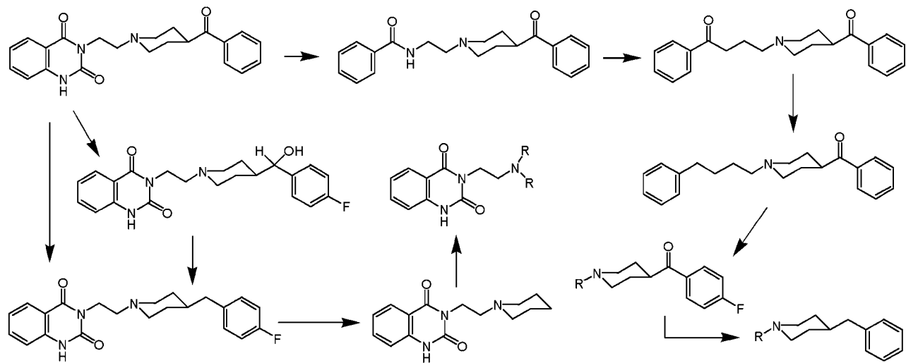
Fig. 2. Examples of some partial structures of ketanserin ( 15 ) examined to determine the minimal structural requirements for binding.
