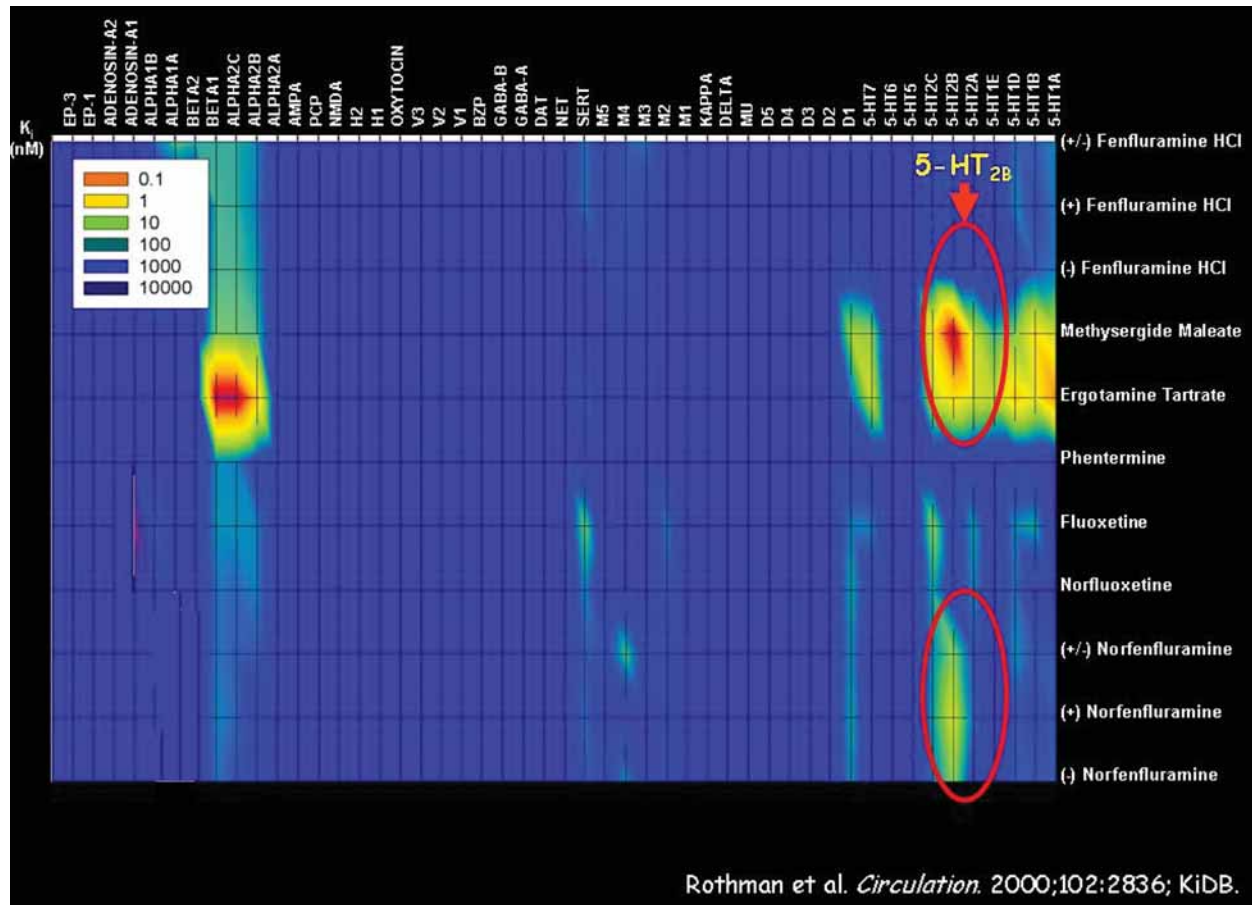
Chapter 13, Fig. 1, p. 426: Three-dimensional representation of VHD-associated and non-VHD-associated drug affinity for a battery of GPCRs, ligand-gated ion channels, and biogenic amine transporters.
