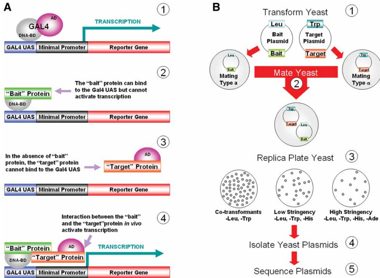
Chapter 8, Fig. 1, p. 260: An overview of yeast two-hybrid screens for FRAPs.
