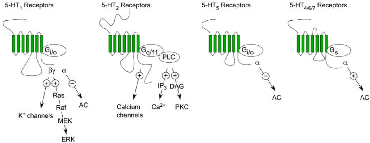
Fig. 1. Major signaling linkages of the subfamilies of G protein-coupled 5-HT receptors are shown. Stimulation is indicated by an arrow overlaid with a “+” sign. Inhibition is indicated by an arrow overlaid with a “-” sign. Abbreviations: AC, adenylyl cyclase; MEK, mitogen and extracellular signal regulated kinase; ERK, extracellular signal regulated kinase; PKC, protein kinase C; DAG, diacylglycerol; IP 3 , inositol trisphosphate.
