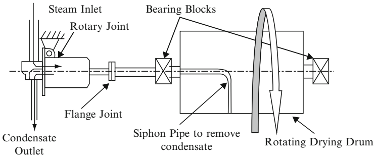
Fig. 1 Schematic of rotary joint arrangement used in paper industry
