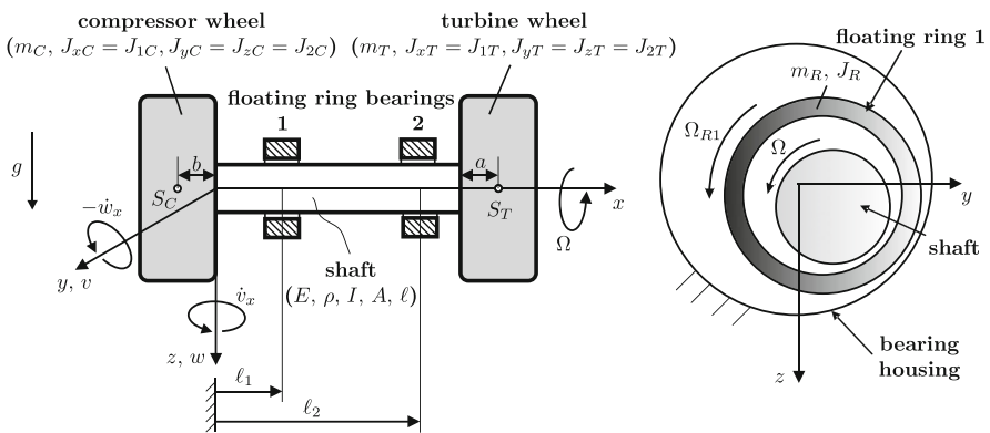
Fig. 2 Mechanical model of a turbocharger rotor supported by floating ring bearings
