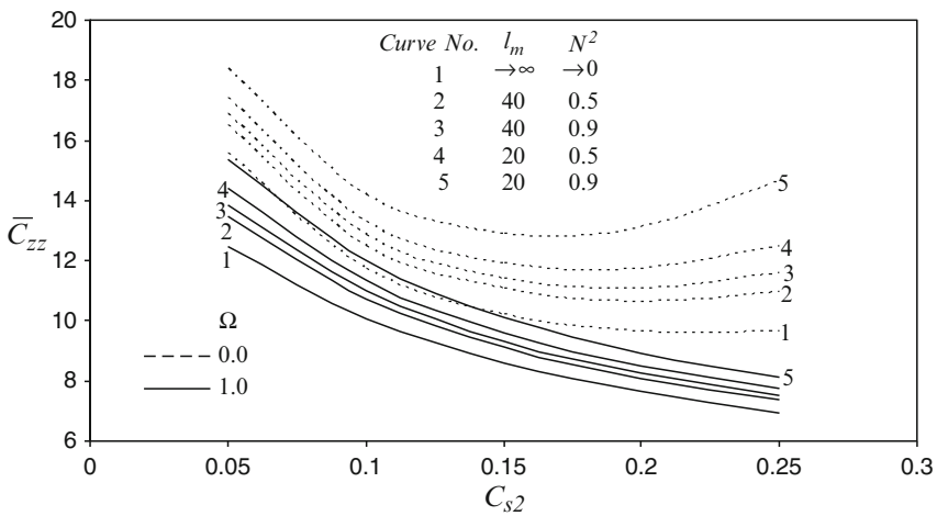
Fig. 9 Variation of \overline{C}_{zz} with restrictor design parameter
