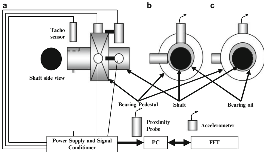
Fig. 2 Mounting of different types of vibration transducers, (a) front view of bearings and shaft, (b) side view – accelerometers not shown for clarity and (c) side view – proximity probes (not shown for clarity)
