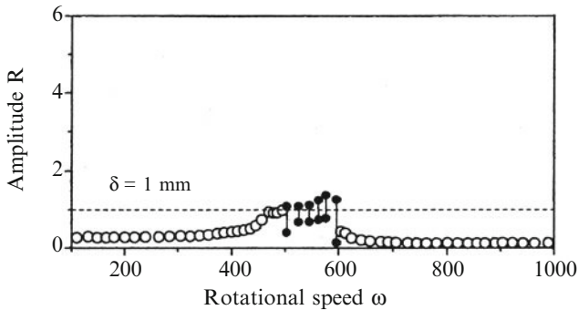
Fig. 5 System with a suppression device (experiment)
