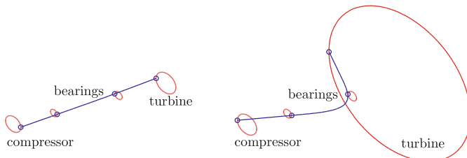
Gyroscopic conical forward mode ( n_1 = 80000 rpm) Gyroscopic bending forward mode ( n_2 = 193000 rpm)
