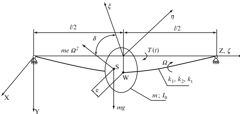
Fig. 1 Physical model of the anisotropic rotor
