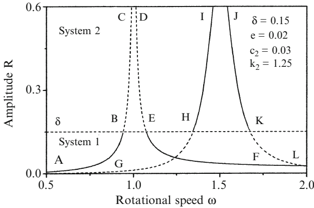
Fig. 2 Principle of suppression
