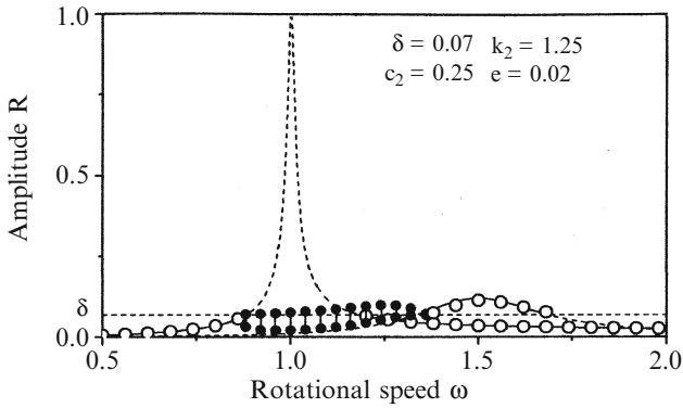
Fig. 3 Numerical simulation
