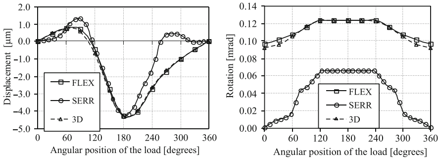
Fig. 8 Deflections of a test beam with 50% crack loaded with bending and torsion: comparison among different models: FLEX is more accurate than SERR, compared to 3D model
