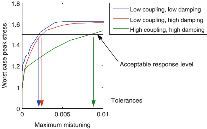
Fig. 8 Assignment of tolerances in different six-bladed disc designs given a upper limit of permissible peak stress
