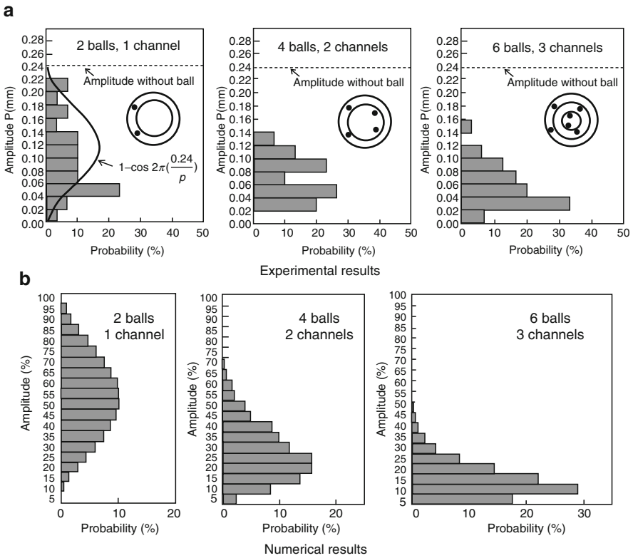
Fig. 20 Comparison of probability among one, two and three channels. (a) Experimental results. (b) Numerical results
