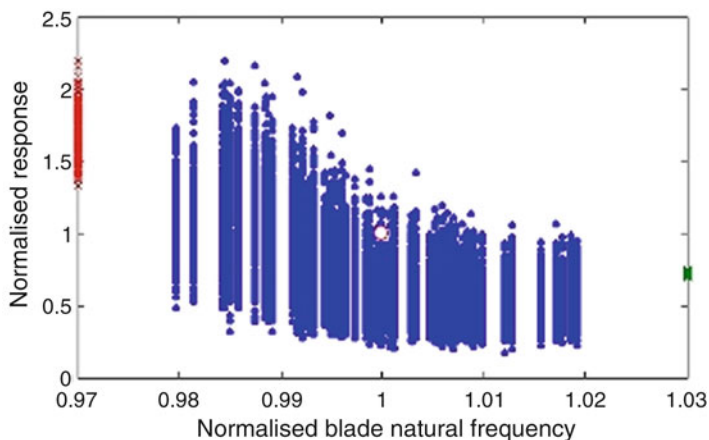
Fig. 5 Scatter plot for one set of blades re-arranged in 100 different configurations to follow
