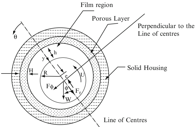
Fig. 2 Bearing geometry
