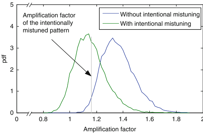
Fig. 9 Amplification factor pdfs for random and controlled mistuning
