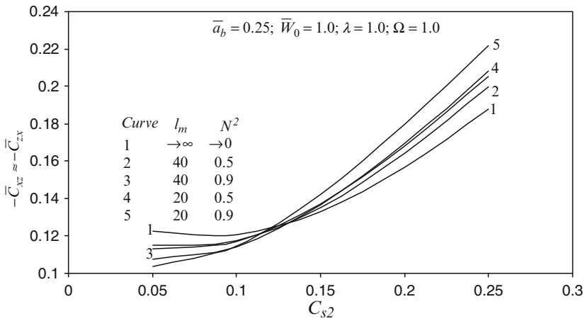
Fig. 8 Variation of \overline{C}_{xz} and \overline{C}_{zx} with restrictor design parameter
