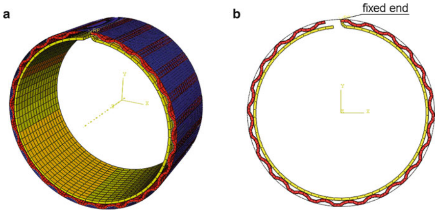
Fig. 5 FEM model of foil bearing structural base ((a) – isometric view, (b) – cross section)
