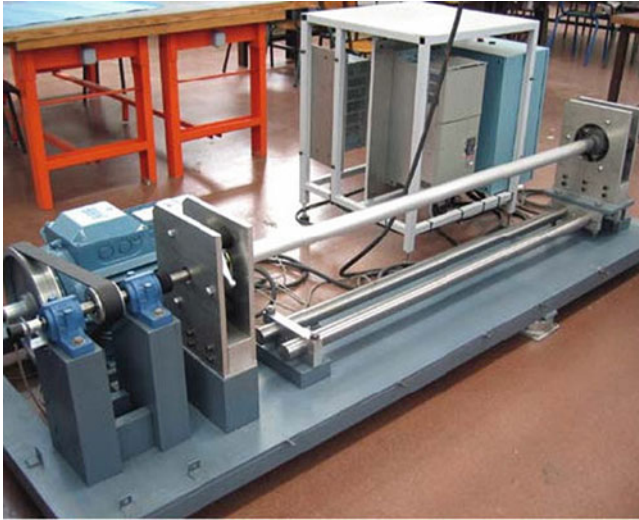
Fig. 5 Testing machine for high-speed tubes
