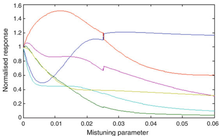
Fig. 4 Dependence of the amplification factor on mistune scatter
