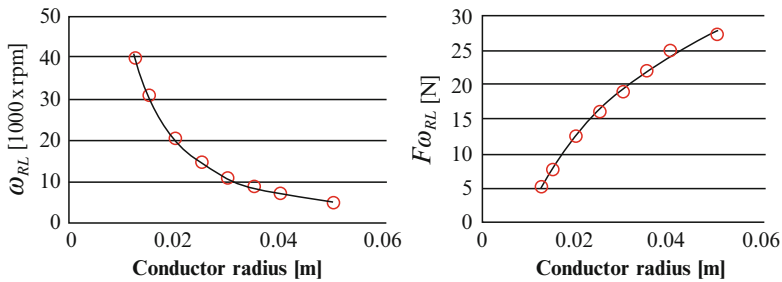
Fig. 5 Sensitivity analysis for various conductor radii
