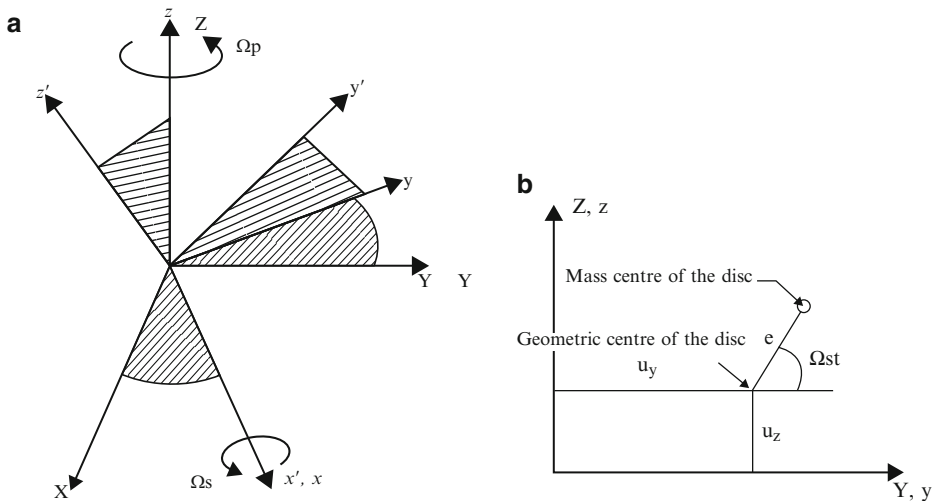
Fig. 2 (a) Coordinate systems fixed to inertial and rotating references (b) location of the centre of mass
