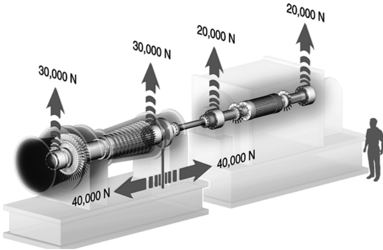
Fig. 5 Gas-turbine/Generator for power generation: four radial bearings and one thrust bearing, 6,010 rpm, 9,000 kW, bearing diameter 400 mm (courtesy S2M)
