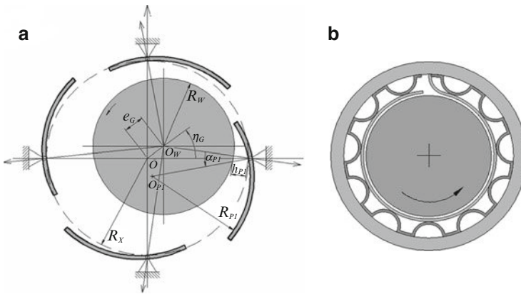
Fig. 1 Variable-geometry bearings selected for the investigation (a) – tilting pad bearing, (b) – bump foil bearing)
