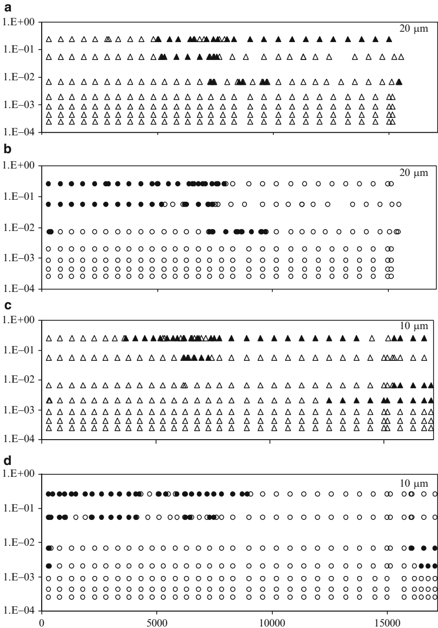
Fig. 6 Maps for instability and chaos at e = 10 \mu\text{m} , (a, b) \gamma_0 = 20 , (c, d) \gamma_0 = 10 \mu\text{m} , (e, f) \gamma_0 = 5 \mu\text{m} (▲ unstable, Δ stable, ● chaotic, ○ non-chaotic)
