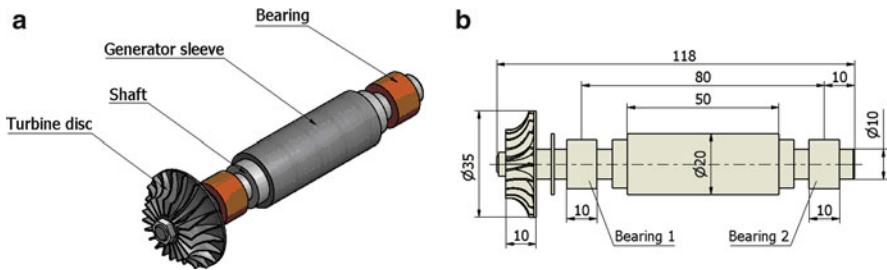
Fig. 6 Two-support shaft with two disc ((a) – isometric view, (b) – dimensions)
