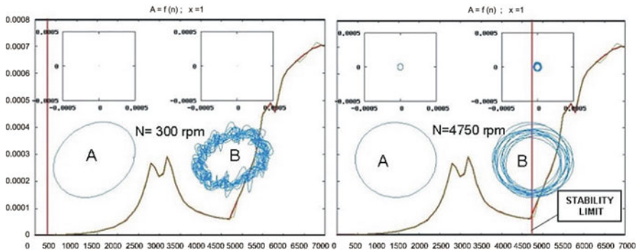
Fig. 8 Displacement trajectories of the rotor centre – within a stable operation range – calculated for the constant excitation force (basic) P (part A) and for the randomly changing – within limits \pm/\Delta P = 20\% (part B) shown at the background of the rotor amplitude-frequency response [8]
