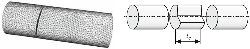
Fig. 7 3D model for breathing and deflection evaluation (left) and equivalent beam model (FLEX approach) for static and dynamic behavior evaluation (right)
