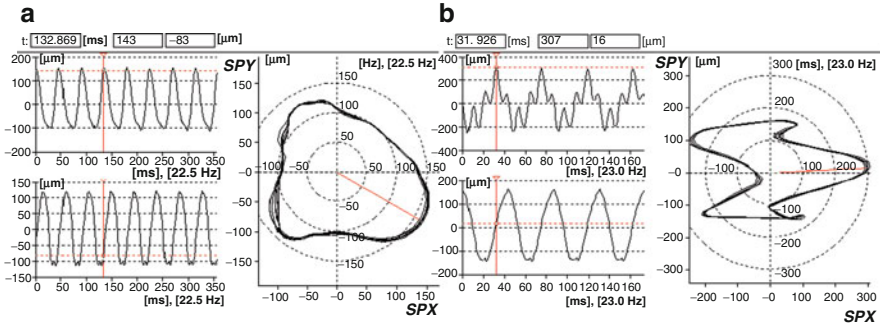
Fig. 6 The vibration displacement plots and kinetic orbits acquired at resonance rotational speed: (a) 7th bearing's S_{\max 7rez} = 165 \mu\text{m} , S_{p-p \max 7Xrez} = 240 \mu\text{m} , S_{p-p \max 7Yrez} = 250 \mu\text{m} ; (b) 8th bearing's S_{\max 8rez} = 307 \mu\text{m} , S_{p-p \max 8Xrez} = 300 \mu\text{m} , S_{p-p \max 8Yrez} = 550 \mu\text{m}
