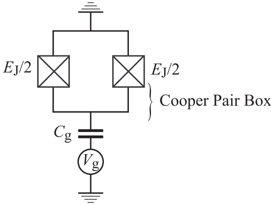
FIGURE 15.8 Charge qubit with a tunable Josephson energy.
