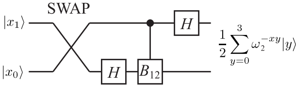
FIGURE 6.2 Implementation of the n = 2 QFT, U_{\text{QFT}2} .
