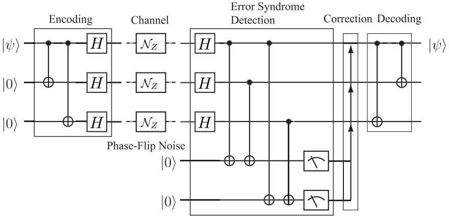
FIGURE 10.4 Three-qubit phase-flip error QECC.
