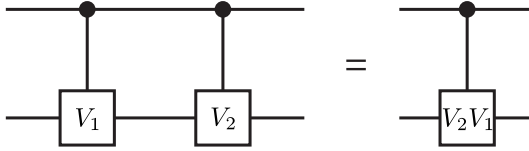
FIGURE 4.10 Equality U_{CV_2}U_{CV_1} = U_{C(V_2V_1)} .
