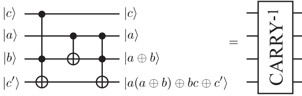
FIGURE 8.8 Inverse of the CARRY gate.
