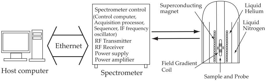
FIGURE 12.4 Schematic diagram of an NMR spectrometer. The test tube and the coils in Fig. 12.3 are in the right-most unit.
