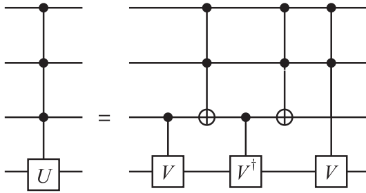
FIGURE 4.13 Decomposition of the C^3U gate.
