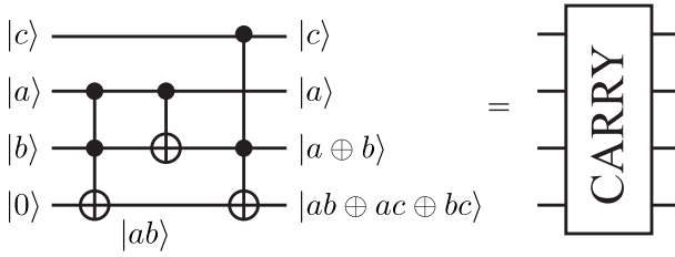
FIGURE 8.6 Quantum circuit which implements the CARRY gate.
