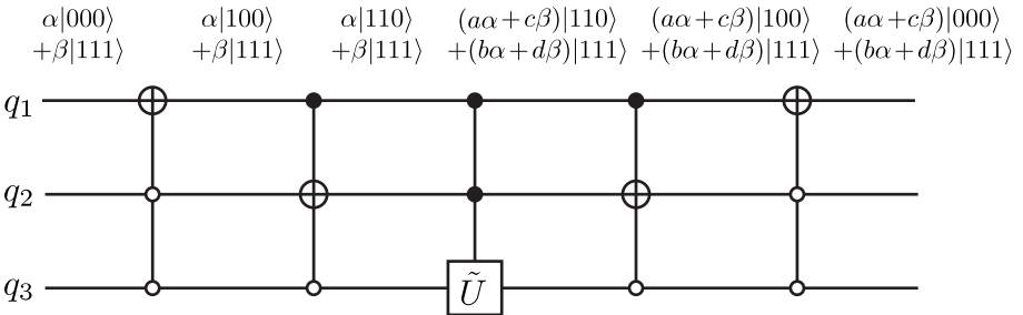
FIGURE 4.7 U -gate acting on \alpha|000\rangle + \beta|111\rangle yields the desired output (\alpha a + \beta c)|000\rangle + (\alpha b + \beta d)|111\rangle .
