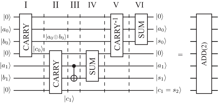
FIGURE 8.7 Quantum circuit to implement the ADD(2) gate, which adds two 2-bit numbers.
