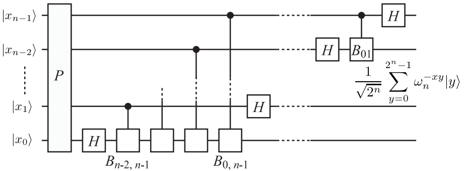
FIGURE 6.4 Implementation of the n -qubit QFT.
