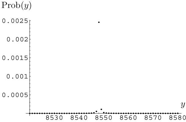
FIGURE 8.3 Probability distribution \text{Prob}(y) for 8,520 \leq y \leq 8,580 .
