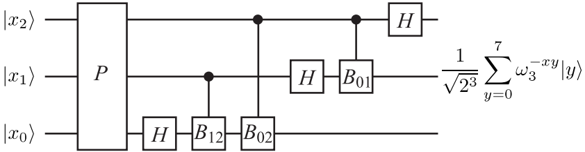
FIGURE 6.3 Implementation of the n = 3 QFT.
