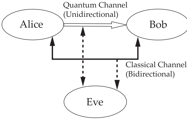
FIGURE 3.2 Quantum key distribution protocol BB84.
