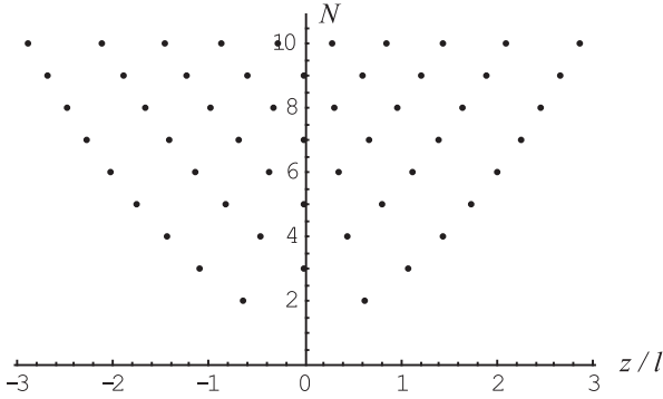
FIGURE 13.8 Equilibrium positions of ions for 2 \leq N \leq 10 .
