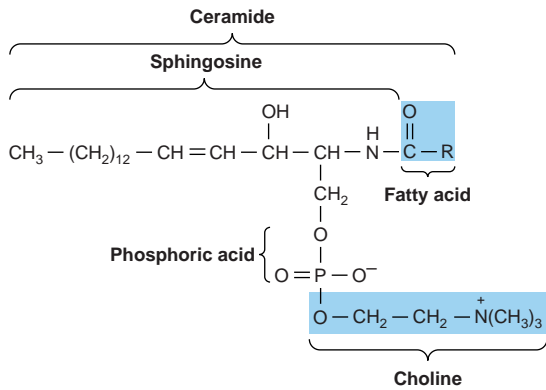
FIGURE 15-11 A sphingomyelin.
