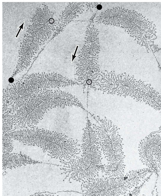
FIGURE 36–4 Electron photomicrograph of multiple copies of amphibian ribosomal RNA genes in the process of being transcribed. The magnification is about 6000 \times . Note that the length of the transcripts increases as the RNA polymerase molecules progress along the individual ribosomal RNA genes from transcription start sites (filled circles) to transcription termination sites (open circles). RNA polymerase I (not visualized here) is at the base of the nascent rRNA transcripts. Thus, the proximal end of the transcribed gene has short transcripts attached to it, while much longer transcripts are attached to the distal end of the gene. The arrows indicate the direction (5' to 3') of transcription. (Reproduced with permission, from Miller OL Jr, Beatty BR: Portrait of a gene. J Cell Physiol 1969;74[Suppl 1]:225. Copyright © 1969. Reprinted with permission from Wiley-Liss, Inc., a subsidiary of John Wiley & Sons, Inc.)
