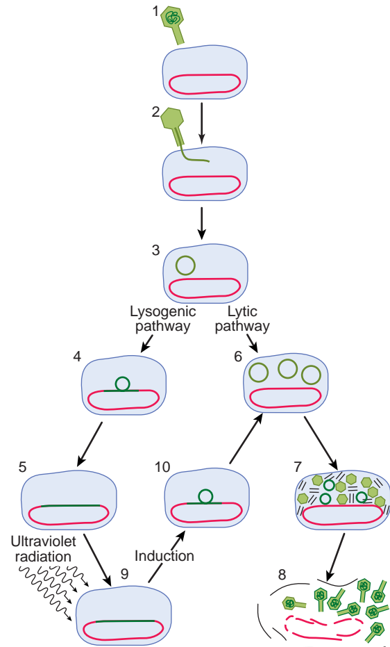
FIGURE 38–4 Infection of the bacterium E. coli by phage lambda begins when a virus particle attaches itself to specific receptors on the bacterial cell (1) and injects its DNA (dark green line) into the cell (2, 3). Infection can take either of two courses depending on which of two sets of viral genes is turned on. In the lysogenic pathway, the viral DNA becomes integrated into the bacterial chromosome (red) (4, 5), where it replicates passively as the bacterial DNA and cell divides. This dormant genomically integrated virus is called a prophage, and the cell that harbors it is called a lysogen. In the alternative lytic mode of infection, the viral DNA replicates itself (6) and directs the synthesis of viral proteins (7). About 100 new virus particles are formed. The proliferating viruses induce lysis of the cell (8). A prophage can be “induced” by a DNA damaging agent such as ultraviolet radiation (9). The inducing agent throws a switch, so that a different set of genes is turned on. Viral DNA loops out of the chromosome (10) and replicates; the virus proceeds along the lytic pathway. (Reproduced, with permission, from Ptashne M, Johnson AD, Pabo CO: A genetic switch in a bacterial virus. Sci Am [Nov] 1982;247:128.)
