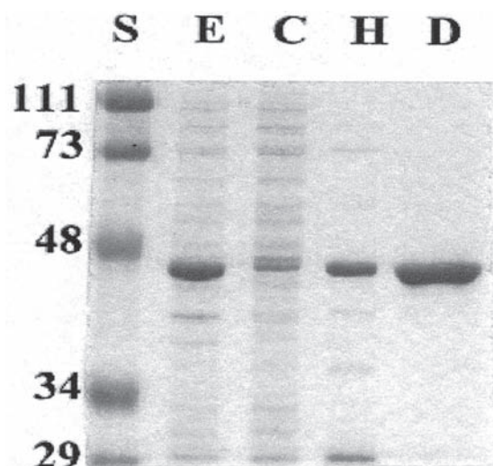
FIGURE 4-5 Use of SDS-PAGE to observe successive purification of a recombinant protein. The gel was stained with Coomassie blue. Shown are protein standards (lane S ) of the indicated M_r , in kDa, crude cell extract ( E ), cytosol ( C ), high-speed supernatant liquid ( H ), and the DEAE-Sepharose fraction ( D ). The recombinant protein has a mass of about 45 kDa.
