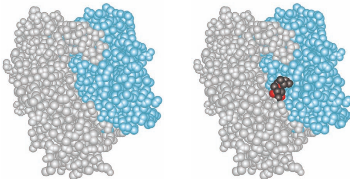
FIGURE 10-2 Shown are space-filling representations of the homodimeric HMG-CoA reductase from Pseudomonas mevalonii with ( right ) and without ( left ) the statin drug lovastatin bound. Each atom is represented by a sphere the size of its van der Waals' radius. The two polypeptide chains are colored gray and blue. The carbon atoms of lovastatin are colored black and the oxygen atoms red. Compare this model with the backbone representations of proteins shown in Chapters 5 & 6. (Adapted from Protein Data Bank ID no. 1t02.)
