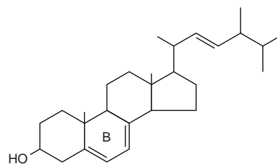
FIGURE 15-18 Ergosterol.
