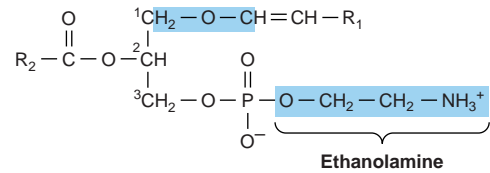
FIGURE 15-10 Plasmalogen.
