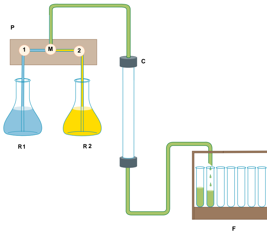
FIGURE 4–2 Components of a typical liquid chromatography apparatus. R1 and R2 : Reservoirs of mobile phase liquid. P : Programmable pumping system containing two pumps, 1 and 2, and a mixing chamber, M . The system can be set to pump liquid from only one reservoir, to switch reservoirs at some predetermined point to generate a step gradient, or to mix liquids from the two reservoirs in proportions that vary over time to create a continuous gradient. C : Glass, metal, or plastic column containing stationary phase. F : Fraction collector for collecting portions, called fractions , of the eluant liquid in separate test tubes.
