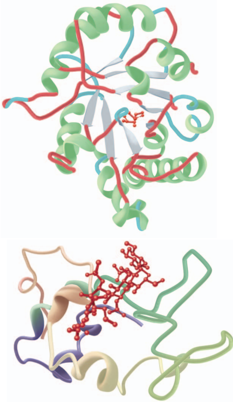
FIGURE 5-6 Examples of tertiary structure of proteins. Top: The enzyme triose phosphate isomerase complexed with the substrate analog 2-phosphoglycerate (red). Note the elegant and symmetrical arrangement of alternating \beta sheets (light blue) and \alpha helices (green), with the \beta sheets forming a \beta -barrel core surrounded by the helices. (Adapted from Protein Data Bank ID no. 1o5x.) Bottom: Lysozyme complexed with the substrate analog penta-N-acetyl chitopentaose (red). The color of the polypeptide chain is graded along the visible spectrum from purple (N-terminal) to tan (C-terminal). Notice how the concave shape of the domain forms a binding pocket for the pentasaccharide, the lack of \beta sheet, and the high proportion of loops and bends. (Adapted from Protein Data Bank ID no. 1sfb.)
