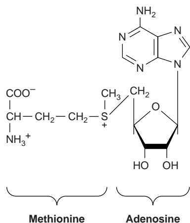
FIGURE 32-12 S-Adenosylmethionine.
