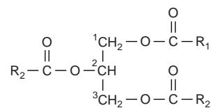
FIGURE 15–6 Triacylglycerol.
