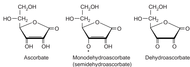
FIGURE 44-19 Vitamin C.
