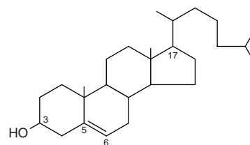
FIGURE 15-17 Cholesterol, 3-hydroxy-5,6-cholestene.
