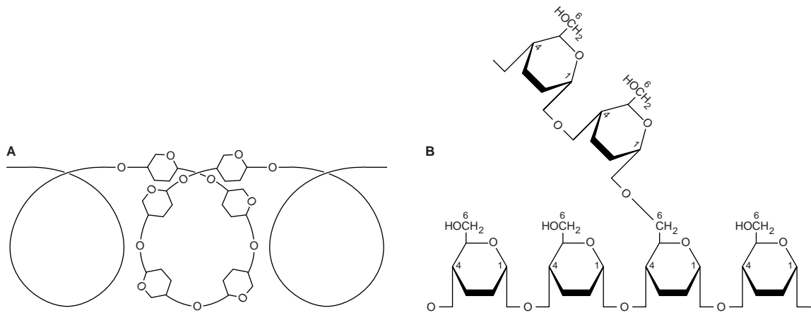
FIGURE 14-12 Structure of starch. (A) Amylose, showing helical coil structure. (B) Amylopectin, showing 1 \rightarrow 6 branch point.
