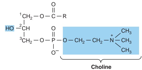
FIGURE 15-9 Lysophosphatidylcholine (lysolecithin).
