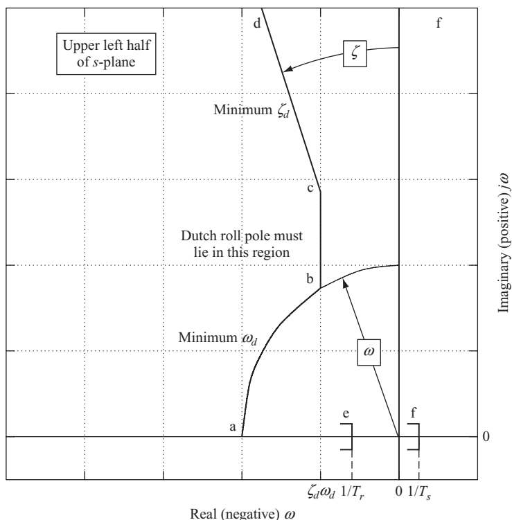
Figure 10.10 Lateral-directional flying qualities requirements on the s-plane.
