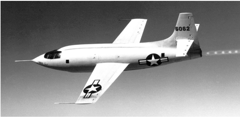
11. The Bell Aircraft X-1 in flight in 1947. The shock-wave pattern in the exhaust plume is visible. The X-1 series aircraft were air-launched from modified Boeing B-29 Superfortress bombers. Air force pilot Chuck Yeager broke the sound barrier for the first time while flying an X-1. (NASA photo)
