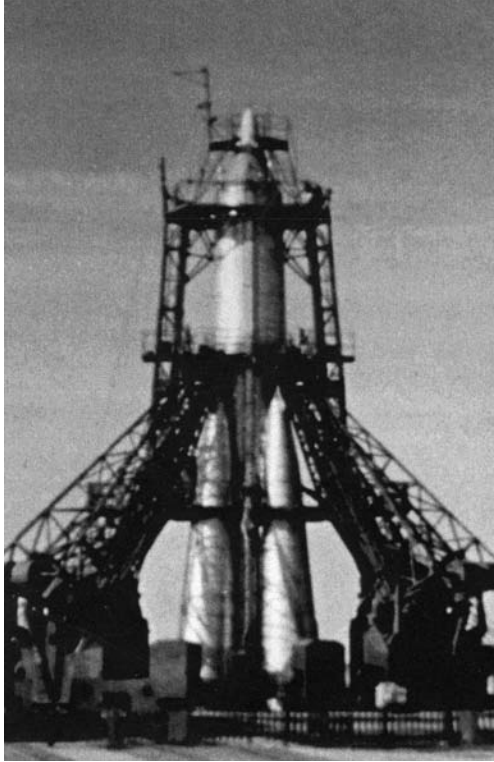
20. Sputnik 2 is shown at the launch pad at Tyura Tam on November 3, 1957. Warm air was piped into the capsule to keep the dog Laika, the first living being to reach orbit, comfortable amid the freezing temperatures. (NASA photo)
