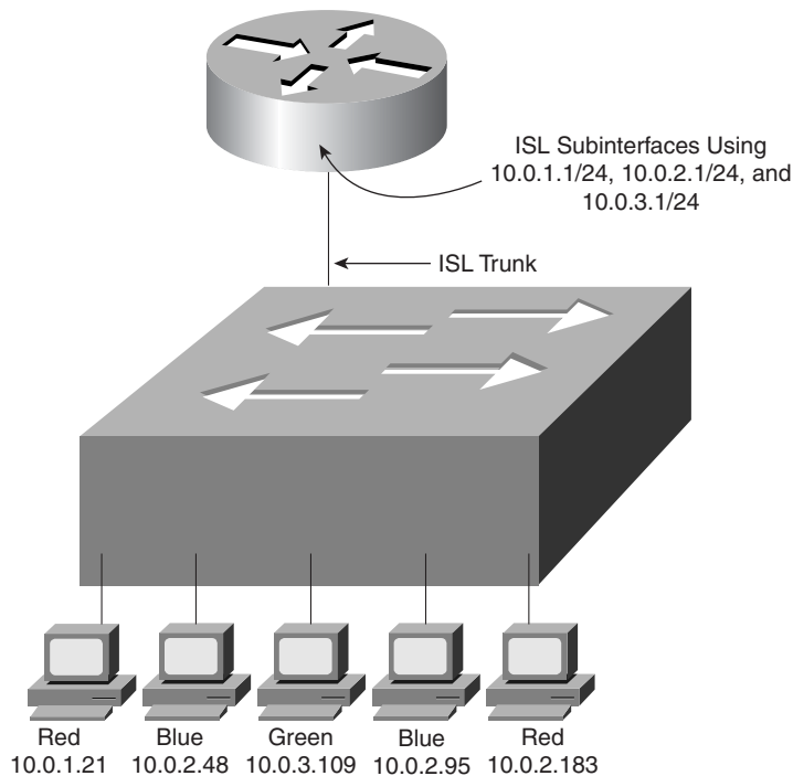
Figure 15-5 Virtual LANs (VLANs)
