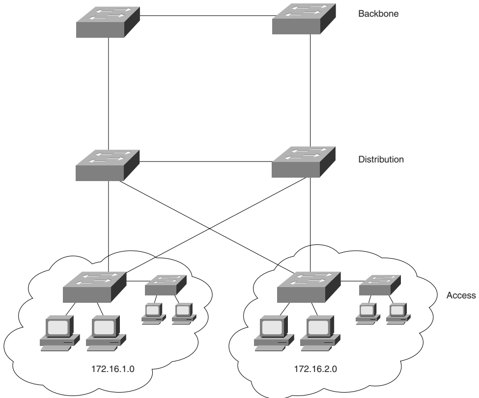
Figure 5-14 Layer 3 Design in a Switched Network
