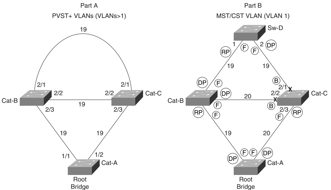
Figure 7-29 IDF MST Switch Load Balancing
