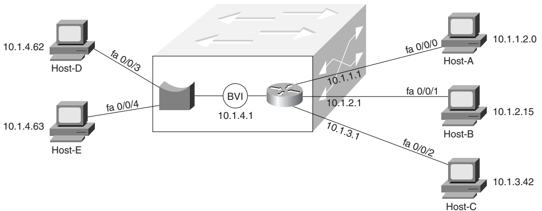
Figure 11-29 A Logical Representation of a BVI
