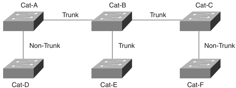
Figure 12-2 A Catalyst VTP Domain Example
