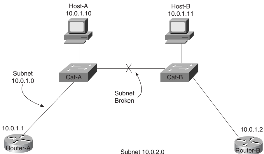
Figure 15-17 Discontiguous Subnets
