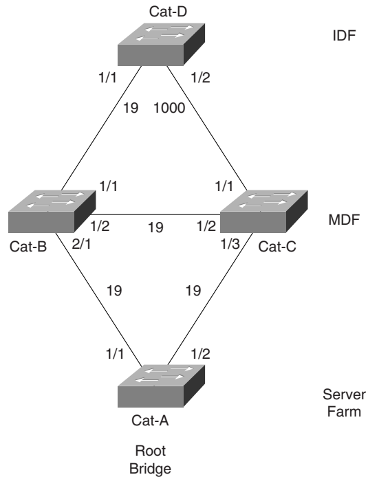
Figure 7-22 A Typical Campus Network Using UplinkFast
