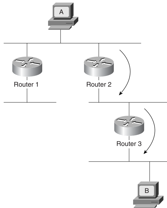
Figure 5-4 Traditional Frame Flow in a Routed Network
