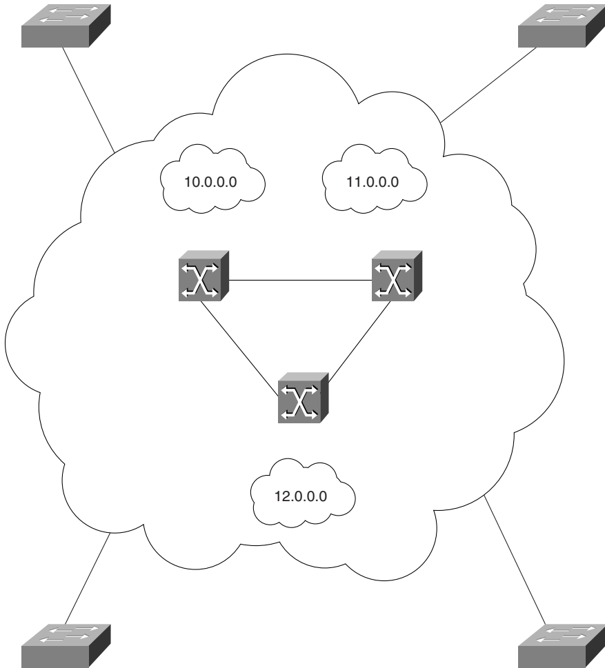
Figure 10-8 LISs in a Nonbroadcast Multi-Access (NBMA) Environment
