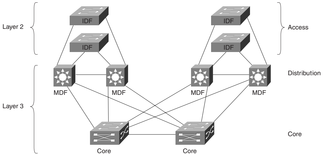
Figure 14-14 A Layer 3 Core
