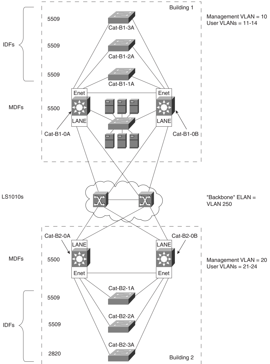
Figure 17-3 MLS Design
