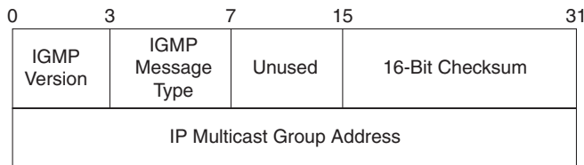
Figure 13-2 IGMP Version 1 Frame Format
