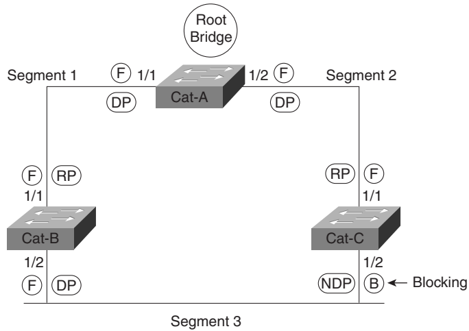
Figure 6-12 Sample Network with Port States Identified
