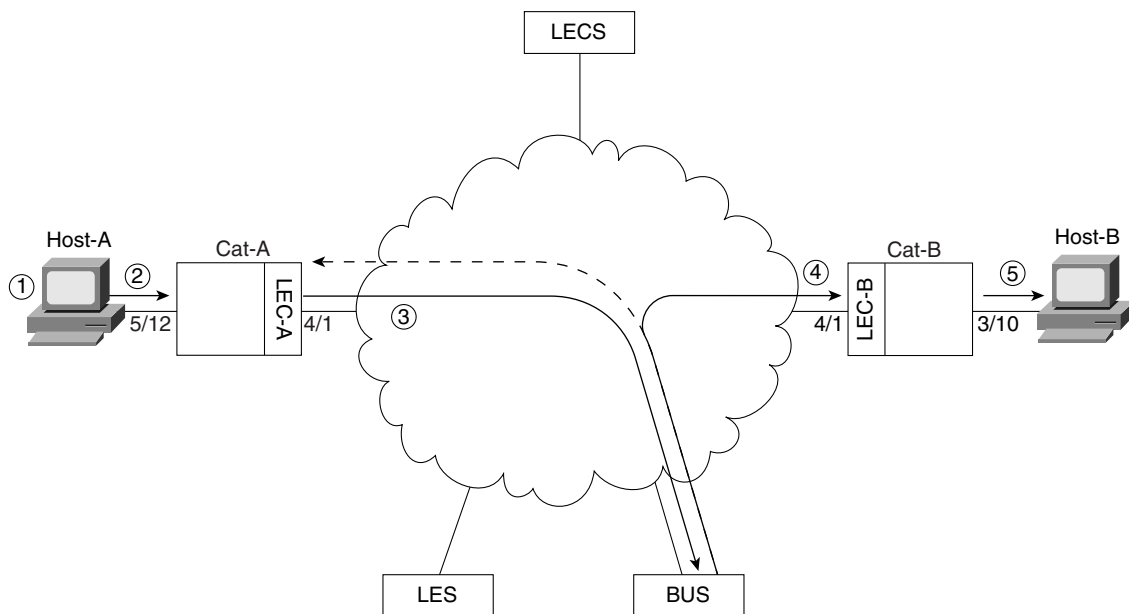
Figure 9-18 The first five steps of the Data Direct VC Creation Process
