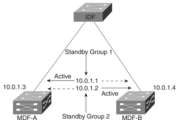
Figure 15-10 MHSRP Load Balancing
