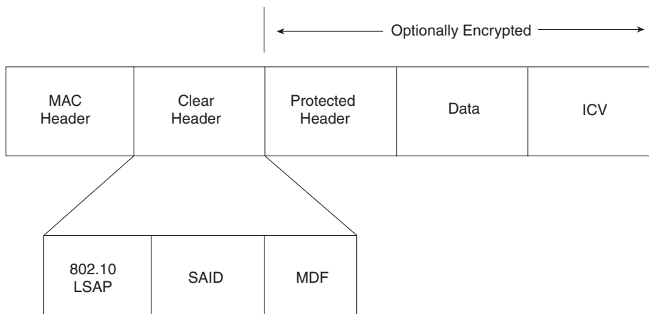
Figure 8-11 802.10 Encapsulation
