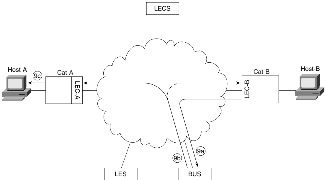
Figure 9-22 Steps 9a–9c in the Data Direct VC Creation Process
