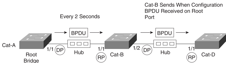
Figure 7-4 Normal Sending of Configuration BPDUs
