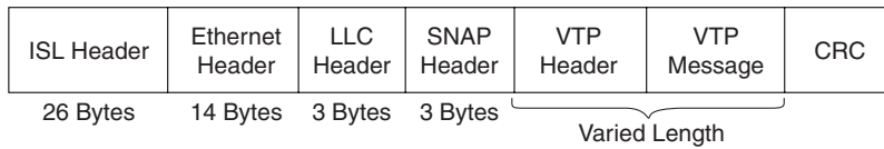
Figure 12-5 VTP Encapsulation over ISL Trunks
