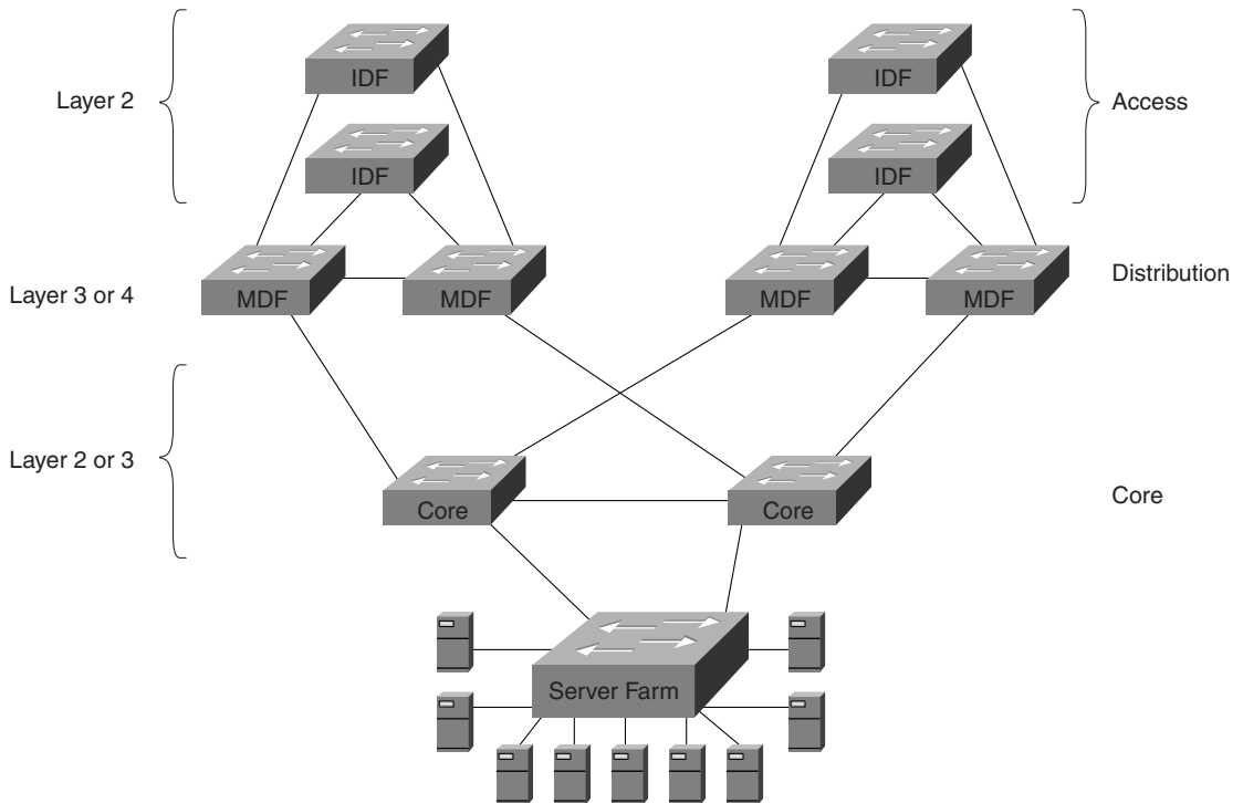
Figure 14-6 Multilayer Model
