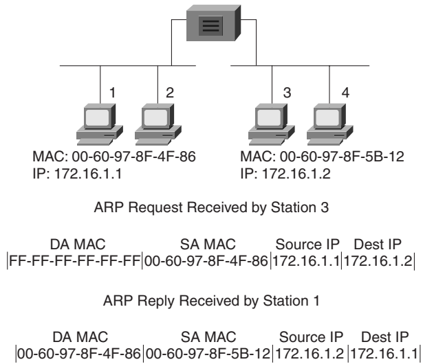
Figure 2-6 ARP Operation in a Repeater Network
