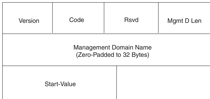
Figure 12-11 VTP Advertisement Request Format
