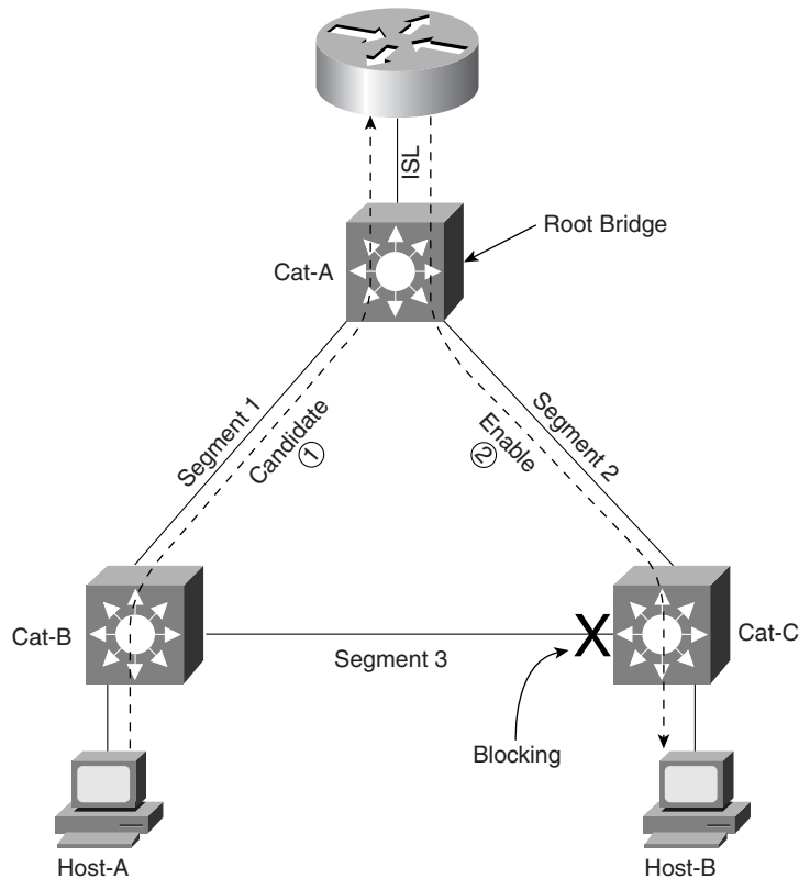
Figure 11-17 A More Complex Network Using MLS
