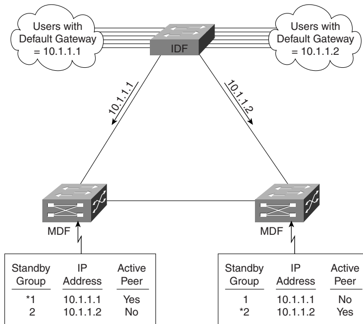
Figure 14-10 MHSRP Load Balancing
