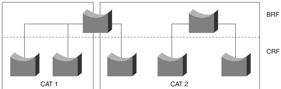
Figure 3-9 TrBRF Extending Across Catalysts
