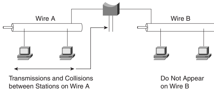
Figure 2-7 Interconnecting Segments with a Bridge
