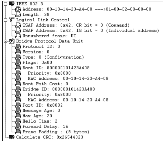
Figure 6-15 Configuration BPDU Decode
