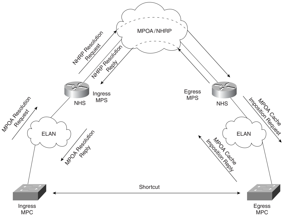
Figure 10-2 MPOA Model
