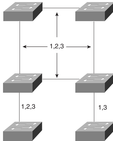
Figure 8-3 The Figure 8-2 Network with Trunk Links
