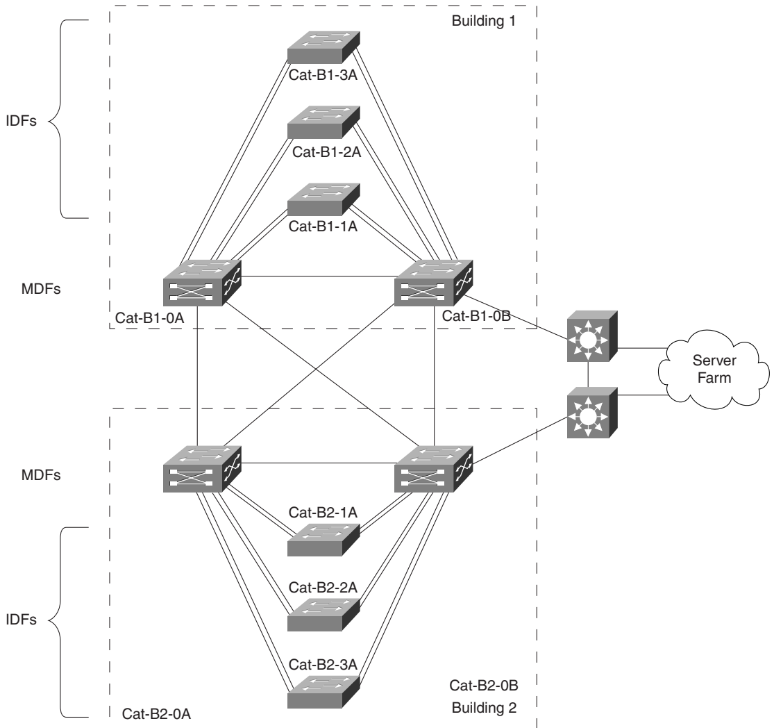
Figure 17-6 Design 2 Network Diagram
