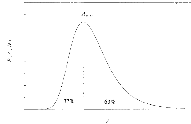
Fig. 3.1. Extreme value distribution (the so-called Gumbel distribution) P(\Lambda, N) when P_{\tau}(\delta x) decreases faster than any power-law. The most probable value, \Lambda_{\text{max}} , has a probability equal to 0.63 to be exceeded.
