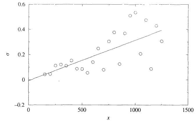
Fig. 2.3. RMS of the increments \delta x , conditioned to a certain value of the price x , as a function of x , for the S&P 500 for the 1985–98 time period.
