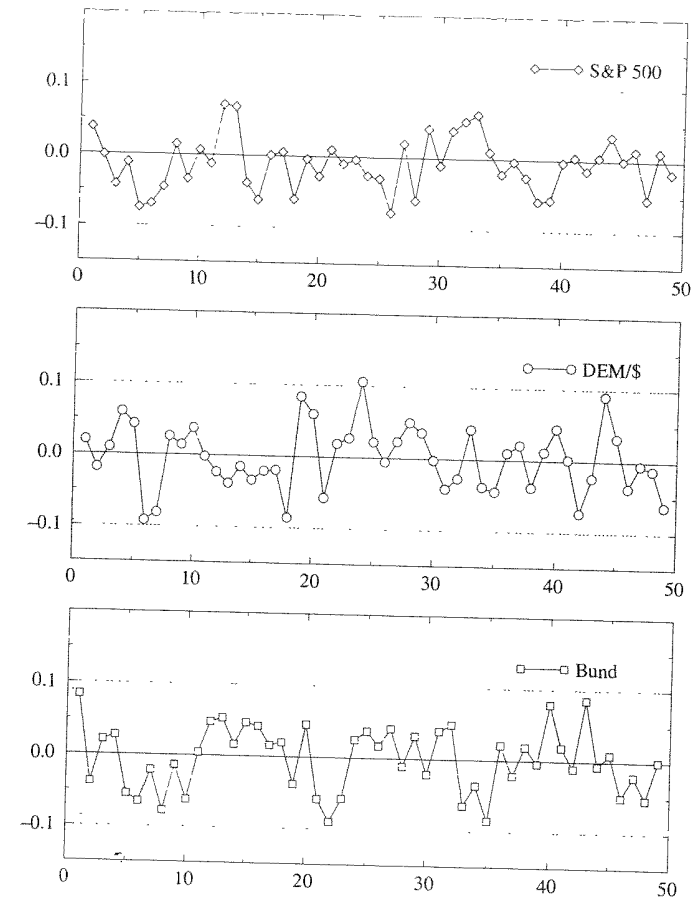
Fig. 2.6. Normalized correlation function C_{k\ell}^{\tau} for the three chosen assets, as a function of the time difference |k - l|\tau , now on a daily basis, \tau = 1 day. The two horizontal lines at \pm 0.1 correspond to a 3\sigma error bar. No significant correlations can be measured.
