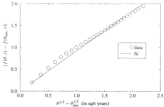
Fig. 2.21. The average FRC in the period 1994–96, as a function of the maturity \theta . We have shown for comparison a one parameter fit with a square-root law, a(\sqrt{\theta} - \sqrt{\theta_{\min}}) . The same \sqrt{\theta} behaviour actually extends up to \theta_{\max} = 10 years, which is available in the second half of the time period.
