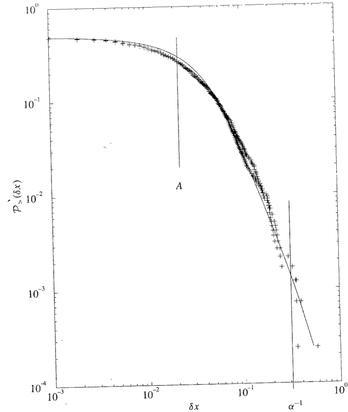
Fig. 2.17. Cumulative distribution \mathcal{P}_{1>}(\delta x) (for \delta x > 0 ) and \mathcal{P}_{1<}(\delta x) (for \delta x < 0 ), for the US 3-month rate (US T-Bills from 1987 to 1996), with \tau = 1 day. The thick line corresponds to the best fit using a symmetric TLD L_{\mu}^{(t)} , of index \mu = \frac{3}{2} . We have also shown the corresponding values of A and \alpha^{-1} , which gives a kurtosis equal to 22.6.
