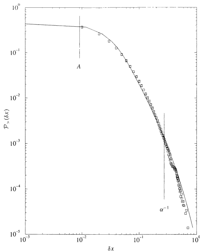
Fig. 2.10. Elementary cumulative distribution for the Bund, for \tau = 15 min, and best fit using a symmetric TLD L_\mu^{(t)} , of index \mu = \frac{3}{2} .
