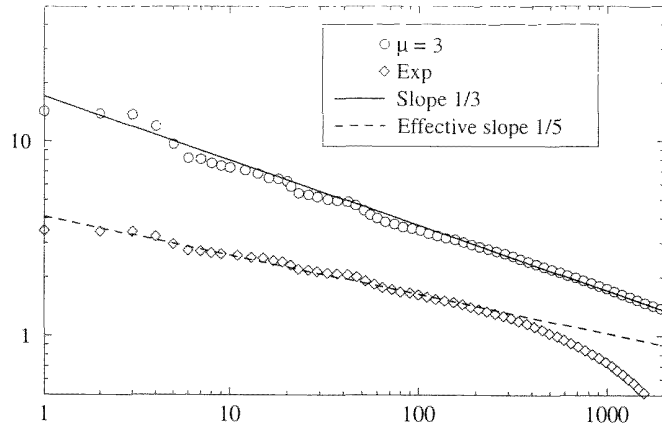
Fig. 1.6. Amplitude versus rank plots. One plots the value of the n th variable A[n] as a function of its rank n . If P(x) behaves asymptotically as a power-law, one obtains a straight line in log-log coordinates, with a slope equal to -1/\mu . For an exponential distribution, one observes an effective slope which is smaller and smaller as N/n tends to infinity. The points correspond to synthetic time series of length 5000, drawn according to a power-law with \mu = 3 , or according to an exponential. Note that if the axes x and y are interchanged, then according to Eq. (1.45), one obtains an estimate of the cumulative distribution, \mathcal{P}_> .
