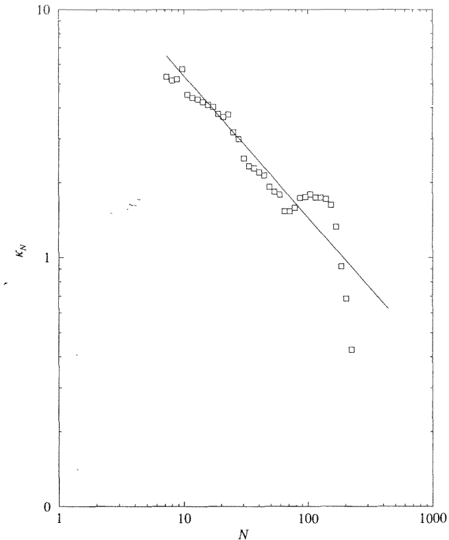
Fig. 2.14. Kurtosis \kappa_N at scale N as a function of N , for the Bund. In this case, the elementary time scale \bar{\tau} is 30 min. If the iid assumption were true, one should find \kappa_N = \kappa_1/N . The straight line has a slope of -0.43 , which means that the decay of the kurtosis \kappa_N is much smaller, as \simeq 20/N^{0.43} .
