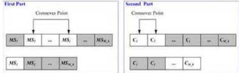
Fig. 4. The variable two-part crossover two-part mutation operation in the HELA.
