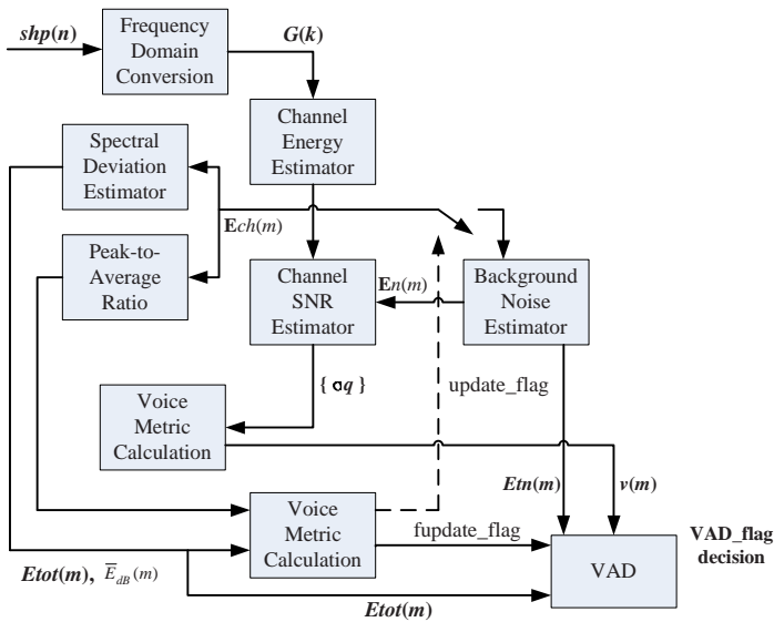
Fig. 2. Block diagram of the VAD algorithm: Option 2 [1]
