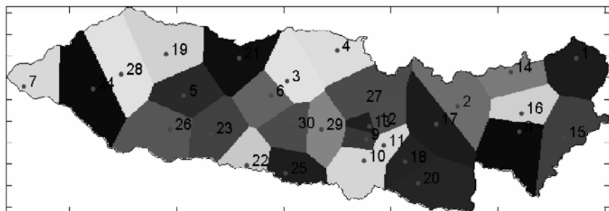
Fig. 2. Thiessen polygons for River Iguazu basin
