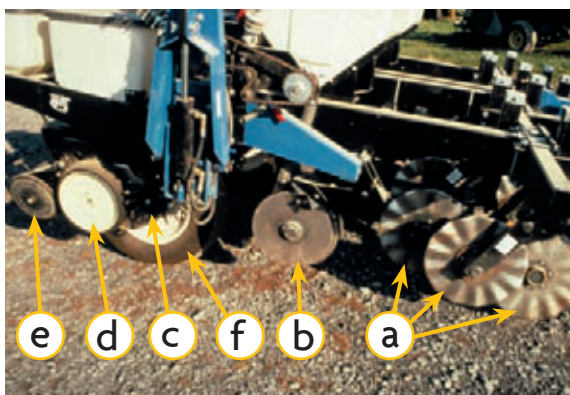
Figure 16.9. Zone-till planter: (a) coulters (cut up residues and break up soil in seed zone); (b) fertilizer disk openers (place granular starter fertilizer in a band next to the seed); (c) spider (trash) wheels (move residue away from the row); (d) seed placement unit; (e) press wheels (create firm seedbed); and (f) wheel used for transporting the planter.
