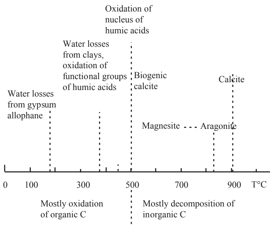
Fig. 10.3. Oxidation of organic C and decomposition of inorganic C as a function of temperature
