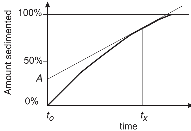
Fig. 2.3. Curve of sedimentation of a complex sample (poly-dispersed system); t_x is time representing the value of the sum of particles X. The intersection of the tangent at point X of the curve with the y-coordinate gives in A the quantity of particles larger than X
