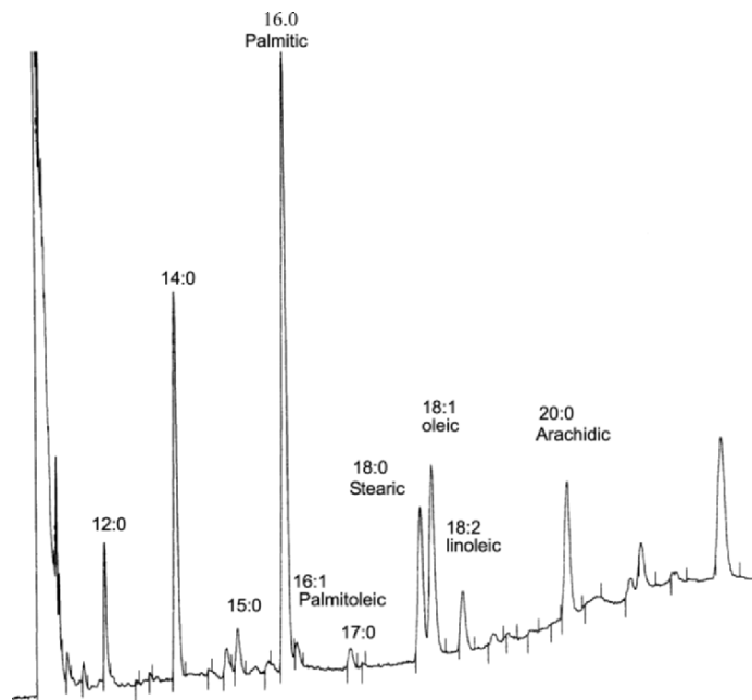
Fig. 13.5. Fractionation of methyl esters of short fatty acids of a tropical ferruginous soil from Burkina-Faso by gas chromatography (conditions described in the text; M Pansu, unpublished data)
