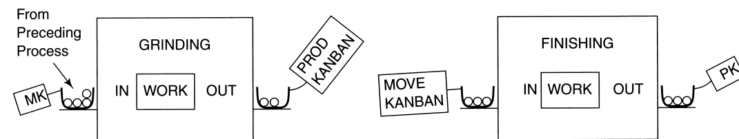
FIGURE 12 Dual-Card Kanban System
