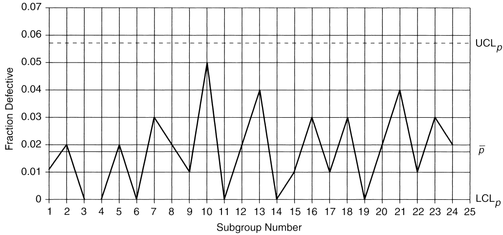
FIGURE 14 p -Chart
