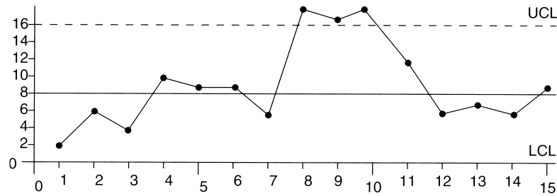
FIGURE 6 Control Chart
