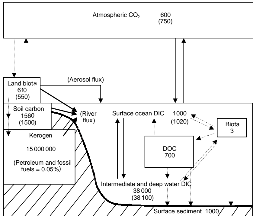
Figure 1 Major global reservoirs involved in active production, exchange and cycling of organic carbon. Reservoir sizes are shown in Gt carbon (1 GtC = 10^{15} g C). Numbers in parentheses are based on 1980s values; numbers without parentheses are estimates of the pre-anthropogenic values. Fluxes primarily mediated by biological reactions are shown with dashed arrows; physical transport processes are shown with solid arrows. (Modified after Siegenthaler and Sarmiento (1993) and Hedges and Oades (1997).)
