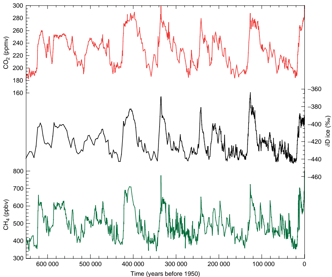
Figure 8 Variations in deuterium ( \delta\text{D} ; black), a proxy for local temperature, and atmospheric concentrations of the greenhouse gases carbon dioxide ( \text{CO}_2 ; red), and methane ( \text{CH}_4 ; green), from measurements of air trapped within Antarctic ice cores. Data from Spahni R, Chappellaz J, Stocker TF, et al. (2005) Atmospheric methane and nitrous oxide of the late Pleistocene from Antarctica ice cores. Science 310: 1317–1321 and Siegenthaler U, Stocker TF, Monnin E, et al. (2005) Stable carbon cycle-climate relationship during the late Pleistocene. Science 310: 1313–1317.
