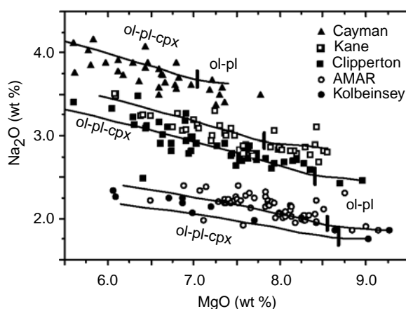
Figure 5 MgO vs. Na 2 O in MORB from five different Ridge segments (Mid Cayman Rise in the Caribbean; near Kane Fracture Zone on the Mid-Atlantic Ridge, 23°N; AMAR on the Mid-Atlantic Ridge around 37°N; East Pacific Rise near the Clipperton Fracture Zone around 10°N; Kolbeinsey Ridge north of Iceland). Lines are calculated Liquid Lines of Descent (LLDs) from high MgO parents. Bar shows where clinopyroxene joins plagioclase and olivine as a fractionating phase. Na 8 is determined by the values of Na 2 O when the LLD is at MgO of 8 wt%. (Adapted with permission from Langmuir et al. , 1992.)
