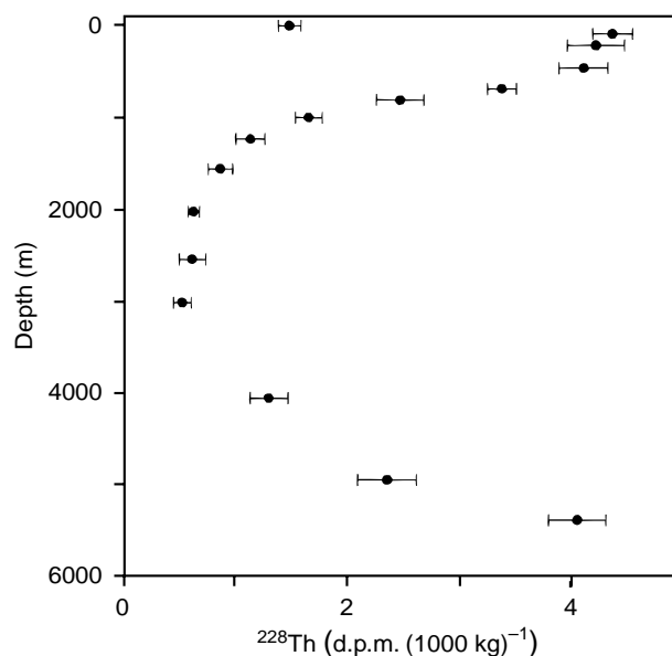
Figure 4 ^{228}\text{Th} distribution in the Pacific. The higher activity levels of ^{228}\text{Th} in near-surface and near-bottom waters reflect that of its parent ^{228}\text{Ra} . Data from Nozaki et al. (1981).
