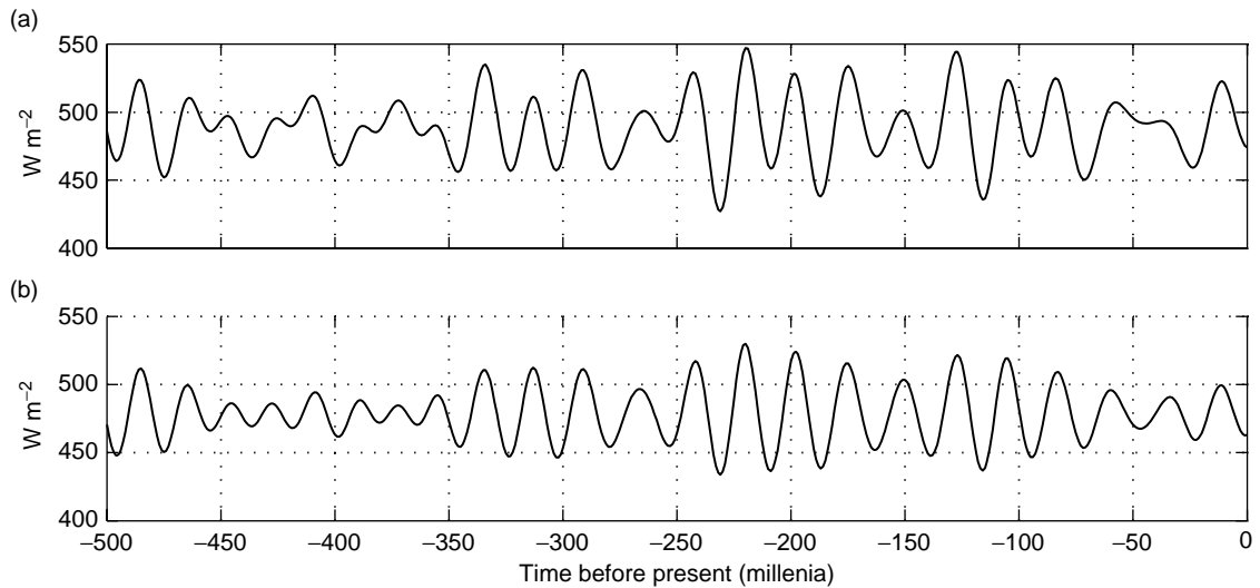
Figure 7 Summer solstice insolation at (a) 65^\circ \text{N} and (b) 25^\circ \text{N} for the past 500 000 years.
