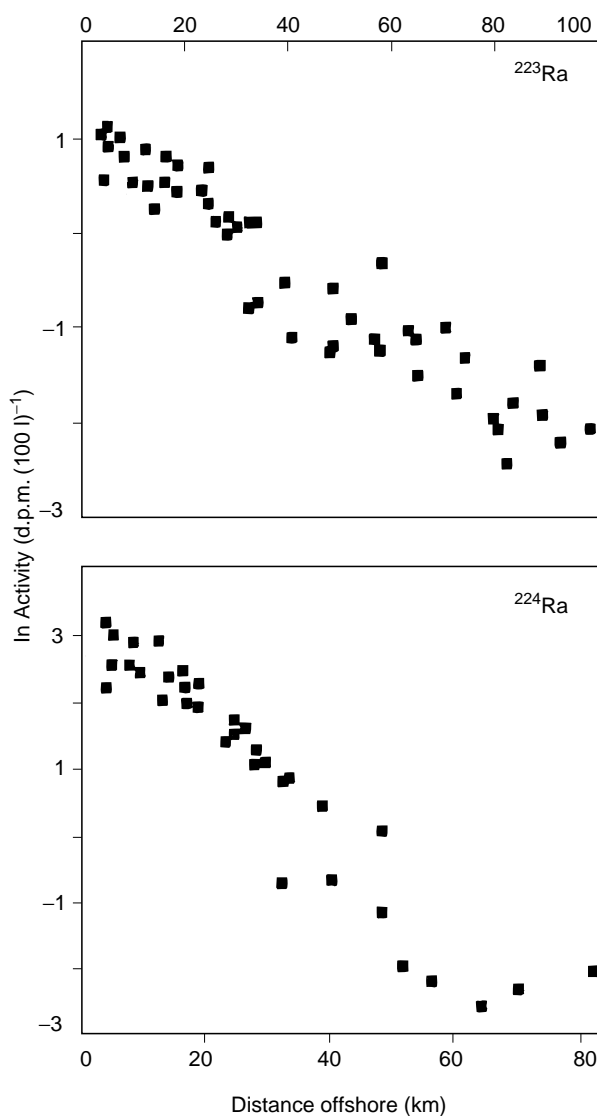
Figure 12 Distributions of ^{223}\text{Ra} and ^{224}\text{Ra} activities as a function of distance off-shore from Winyah Bay off Carolina Coast, USA. These profiles have been modeled to yield horizontal eddy diffusion coefficients. (Modified from Moore, 1999.)
