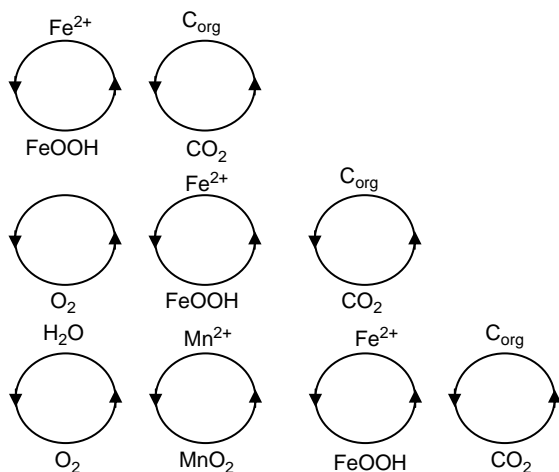
Figure 7 The oxidation of organic matter by FeOOH. In each panel, the oxidation of organic carbon ( C_{org} ) to CO_2 is coupled to the reduction of FeOOH to Fe^{2+} . In the top panel, the source of the FeOOH is the particle flux to the sediments. The lower two panels show that internal cycling within the sediments can also supply Fe(III) for organic matter oxidation. In the middle panel, Fe(II) that was produced by organic matter oxidation is oxidized by O_2 to Fe(III), to be reused to oxidize organic matter. In the lower panel, Fe(II) is oxidized to Fe(III) by MnO_2 . The MnO_2 for this reaction, in turn, may be supplied either by the particle flux to the sediments or by oxidation of Mn(II) to Mn(IV) by O_2 . The figure illustrates that the coupling of organic matter oxidation to Fe(III) reduction can be quantitatively important even if the supply of reactive Fe(III) through the fall or particles to the seafloor is small. When this occurs, the ultimate sink for the electrons for organic matter oxidation by the Fe(III)/Fe(II) pathway is O_2 .
