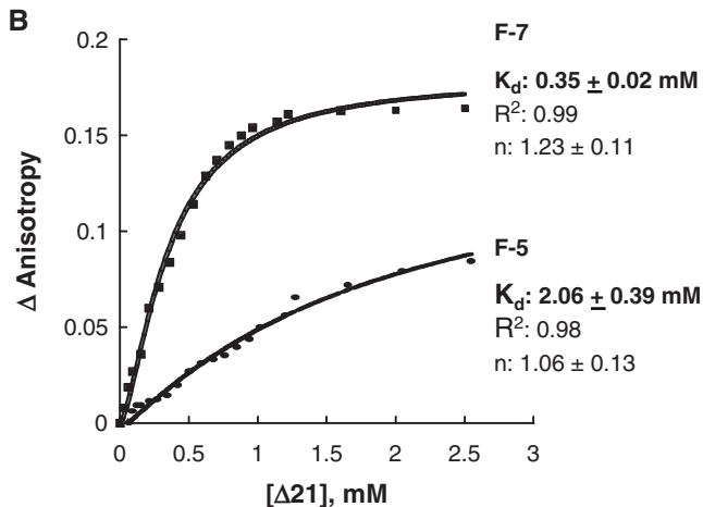
Fig. 2 Analysis of the RNA length required for stable interaction with the HCV RdRp using a fluorescence assay. (A) Sequences of RNAs used and the affinities with the HCV RdRp \Delta 21. FI denotes a fluorescein and ND denotes not determine. (B) The binding isotherms for the RNAs of 7- and 5-nt
