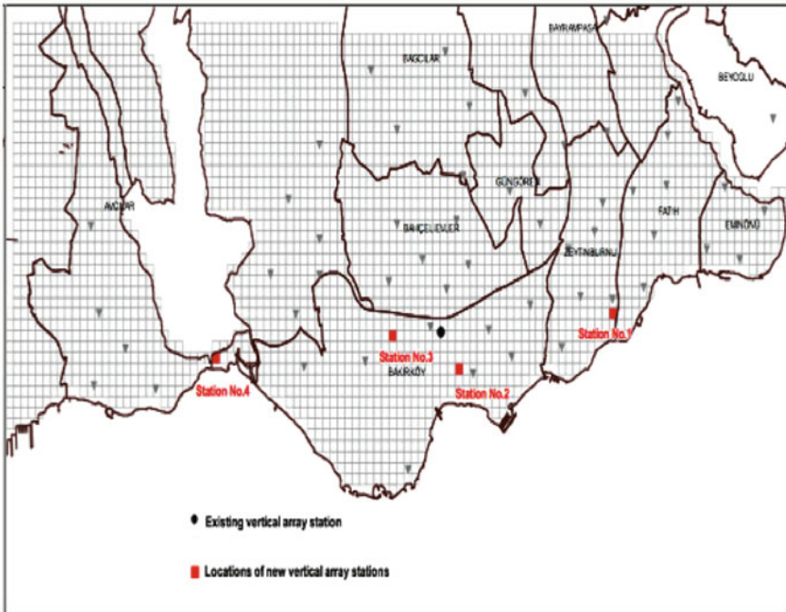
Fig. 18.5 Locations of current and planned downhole stations
