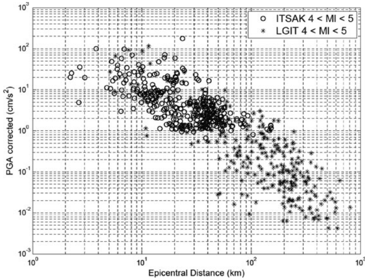
Fig. 9.4 PGA values corresponding to a range of magnitudes between 4 and 5, recorded by LGIT and ITSAK plotted versus epicentral distance
