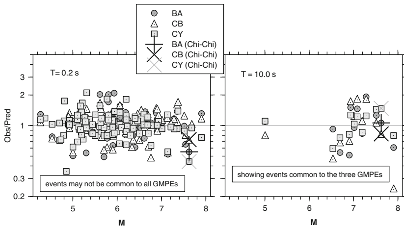
Fig. 1.11 Event residuals (see text). Each symbol represents one event
