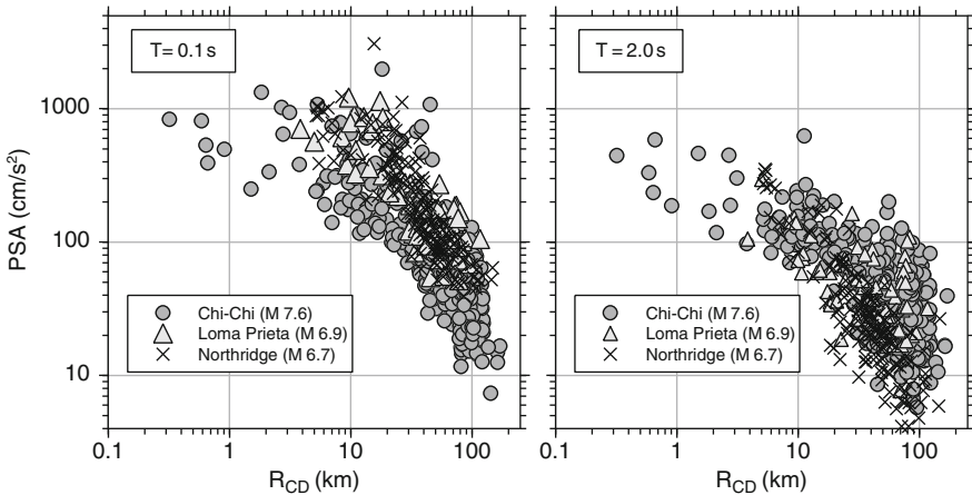
Fig. 1.2 Ground motions for three earthquakes for two oscillator periods. Note that the motions from the M 7.6 Chi–Chi earthquake are smaller and larger than for the smaller earthquakes at short and long period, respectively
