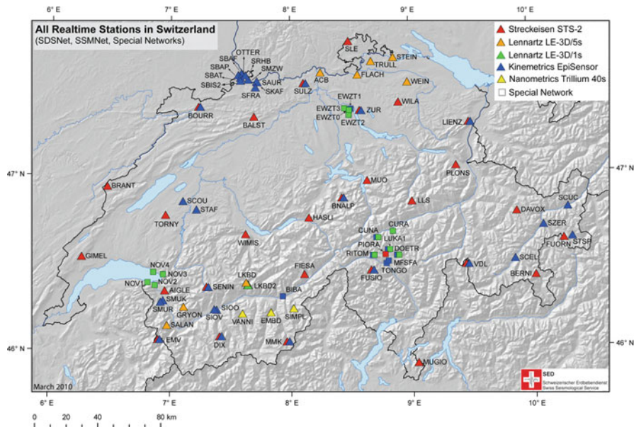
Fig. 15.4 All continuously monitored stations from the CHNet SED. The Swiss digital seismic network (SDSNet) mainly consists of Streckeisen STS-2 seismometers, complimented by short period velocity sensors (~35 stations). High dynamic range accelerometer stations from the SSMNet Swiss strong motion network comprise about 40 stations, some co-located with broadband sensors
