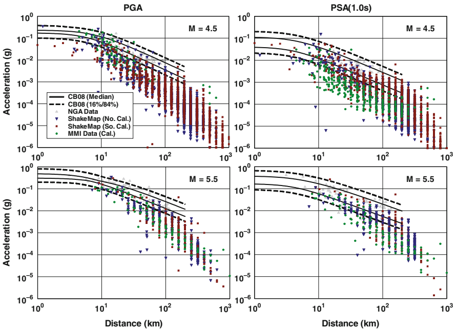
Fig. 7.4 Comparison of the Campbell and Bozorgnia [27] E-GMPE with small-to-moderate magnitude NGA and ShakeMap ground motion recordings and MMI data that have been converted to ground motion parameters. Data courtesy of G. Atkinson (personal communication, [4])
