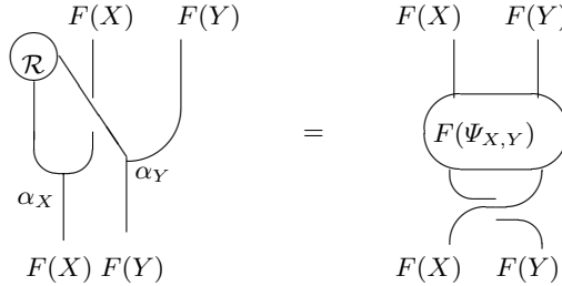
Fig. 5.13. Defining structure of opening by reconstruction theorem with transfers in diagrammatic form.
