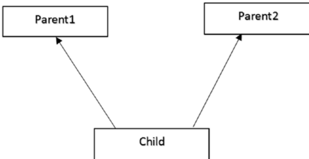
Figure 3-4. Multiple inheritance
