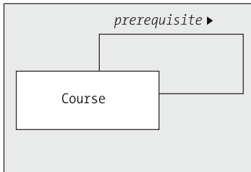
Figure 10-17. A reflexive association involving the Course class
