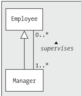
Figure 10-35. Indicating both inheritance and an association between the Employee and Manager classes
