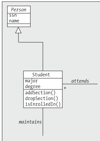
Figure 14-3. The Student class
