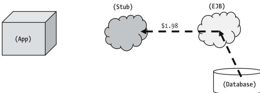
Figure 17-13. The EJB retrieves the necessary data from the data access layer, returning it to the stub . . .
