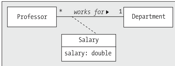
Figure 10-54. Placing an association class on a one-to-many association
