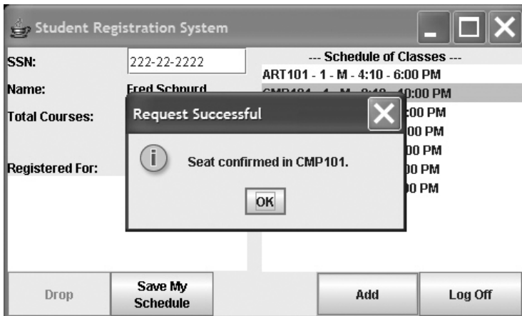
Figure 11-6. Fred's view of things, part 2
