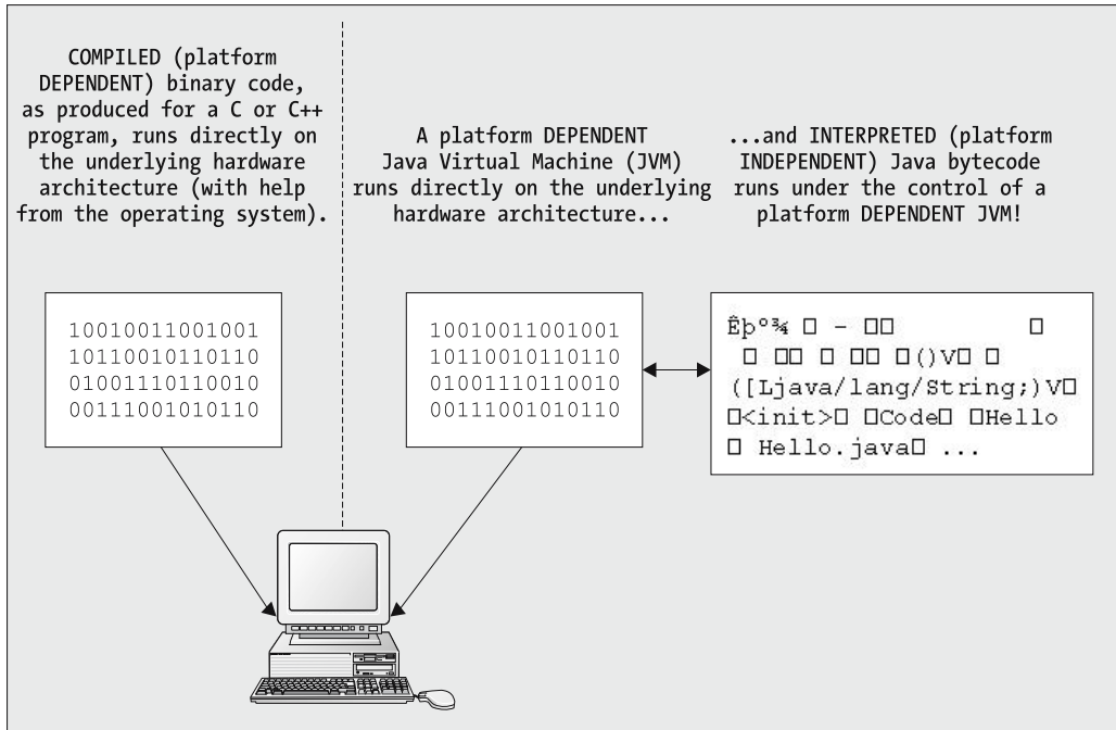
Figure 2-3. A platform-dependent JVM is used to execute platform-independent bytecode.
