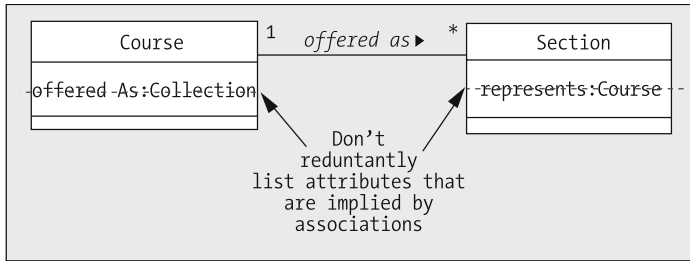
Figure 10-42. Redundantly reflecting references as attributes is inappropriate; the presence of an association implies these.
