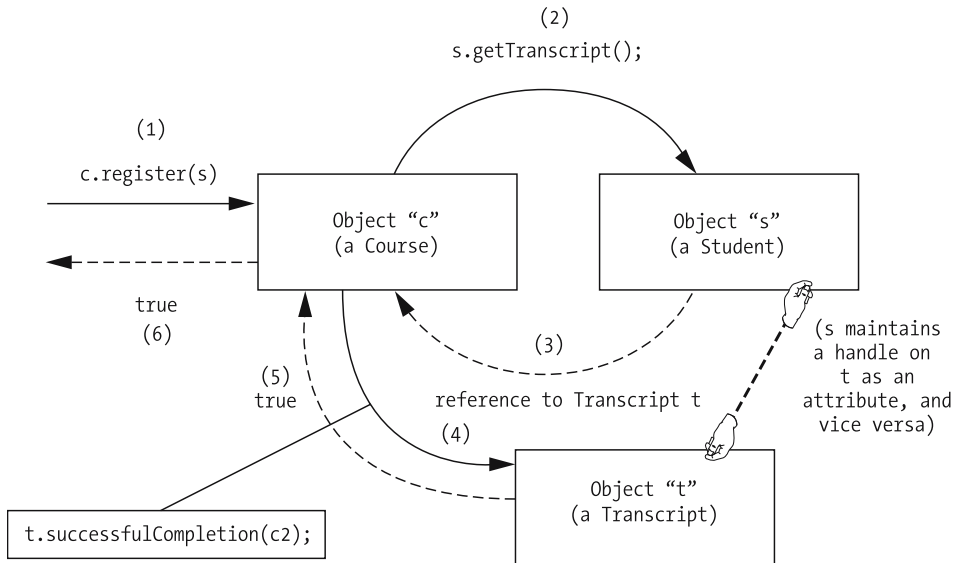
Figure 4-4. A more complex message-passing example involving three objects
