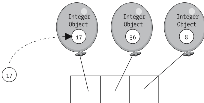
Figure 6-15. We must “box” primitive values in objects in order to insert them into a collection.
