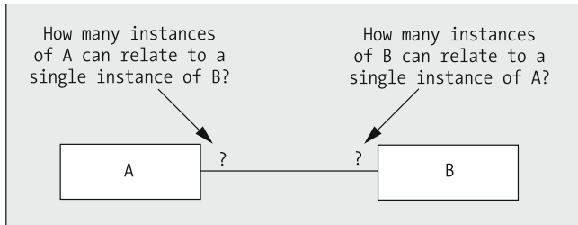
Figure 10-27. Indicating multiplicity between classes
