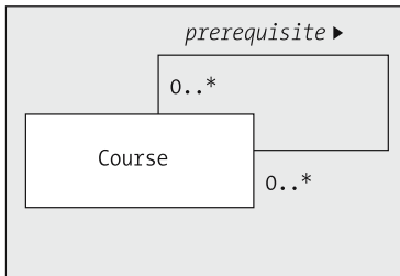
Figure 10-32. An example of optional many-to-many multiplicity on a reflexive association
