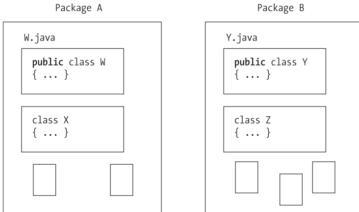
Figure 13-28. Two packages, A and B, each contain one public and one package accessible class.
