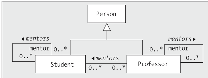
Figure 10-50. Specific mentor associations made explicit.
