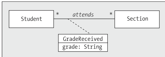
Figure 10-60. Initial portrayal of the attends association
