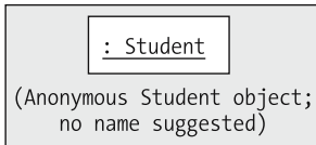
Figure 10-38. Representing an anonymous object
