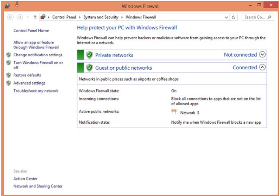
Figure 3-3. Windows Firewall
