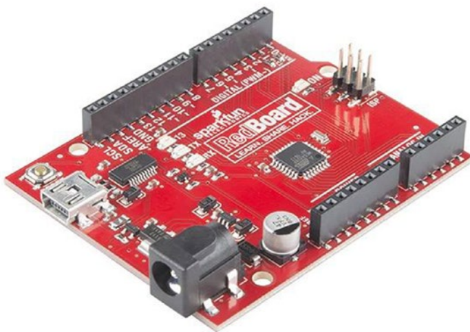
Figure 1-9. SparkFun RedBoard
