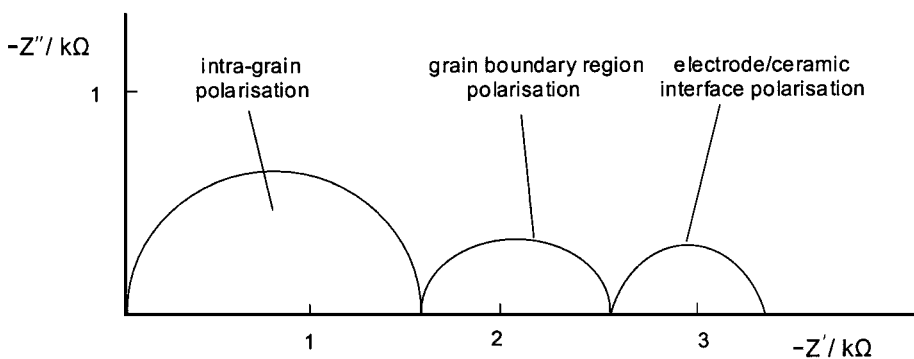
Fig. 2.56 Form of impedance plot for an yttria-stabilized zirconia (see Section 4.5.3.1(b)) at 490^{\circ}\text{C} ( p_{\text{O}_2} = 10^{-2} atm.) based on data by E.J.L Schouler et al. (1983) Solid State Ionics 9 and 10 , 989.
