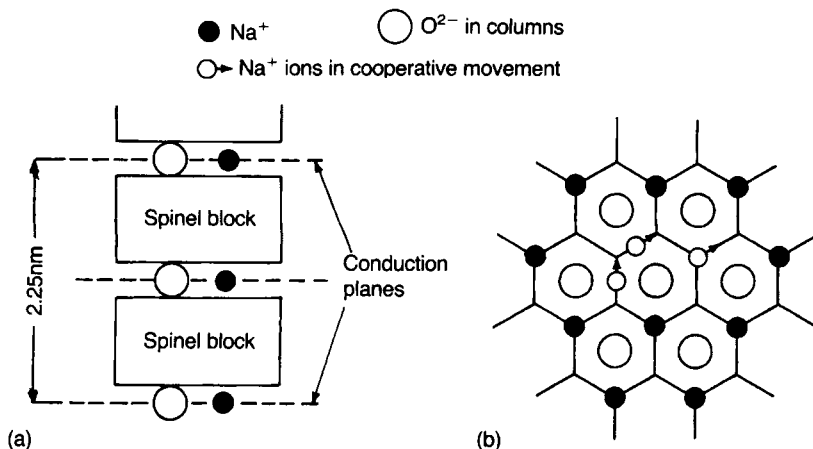
Fig. 4.30 Structure of \beta'' -alumina: (a) alternating spinel blocks and conduction planes; (b) migration pathway of Na + ions indicating paths of concerted motion.
