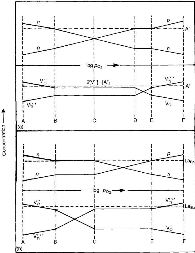
Fig. 2.13 Schematic representation of the dependence of n , p , [V_{Ti}^{\prime\prime\prime}] and [V_{O}^{\bullet\bullet}] on p_{O_2} for (a) acceptor-doped and (b) donor-doped BaTiO_3 .
