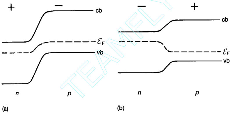
Fig. 2.24 n-p junction: (a) reverse biased; (b) forward biased.
