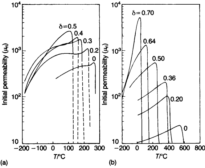
Fig. 9.18 The variation with temperature of the initial relative permeability \mu_{ri} for different \delta values in (a) Mn_{1-\delta}Zn_{\delta}Fe_2O_4 and (b) Ni_{1-\delta}Zn_{\delta}Fe_2O_4 (after [10]).
