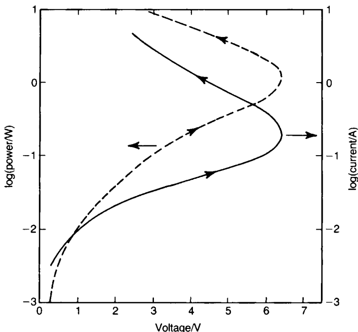
Fig. 4.16 Power and current versus voltage for an NTC thermistor with R_{\infty} = 4.54 \times 10^{-3} \Omega , B = 3000 \text{ K} , T_0 = 300 \text{ K} and T - T_0 = 30 \text{ P K} .
