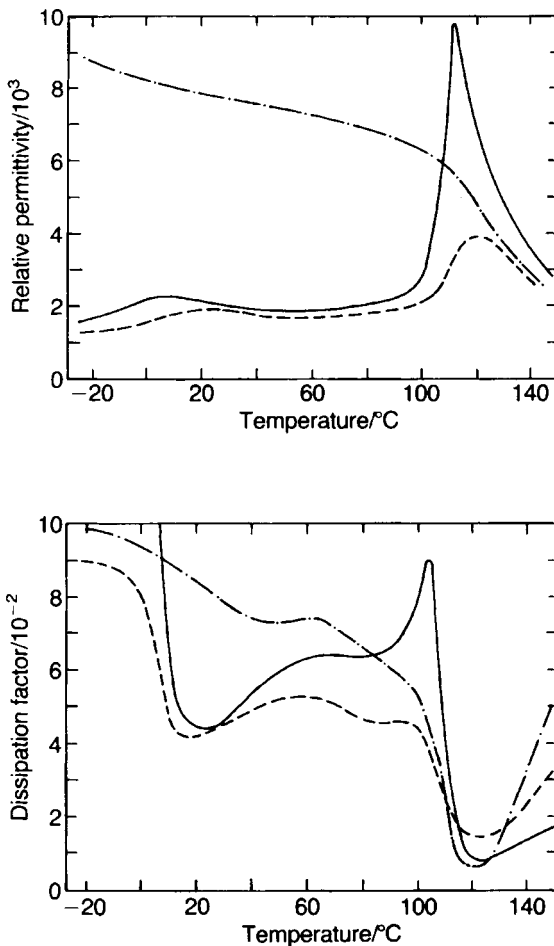
Fig. 5.43 Dielectric properties of technical grade \text{BaTiO}_3 ceramic under various field conditions: —, 15 \text{ kV m}^{-1} peak and 1 \text{ kHz} ; ---, 15 \text{ kV m}^{-1} peak and 1 \text{ kHz} + 1.43 \text{ MV m}^{-1} d.c.; -·-, 1.6 \text{ MV m}^{-1} peak and 50 \text{ Hz} .
