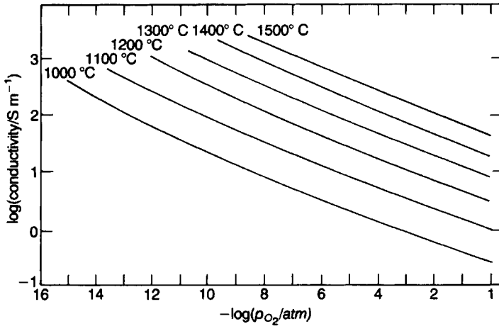
Fig. 5.30 The conductivity measured in the c direction of a rutile single crystal as a function of oxygen pressure and temperature (after R.N. Blumenthal et al. : see [7] p. 145).
