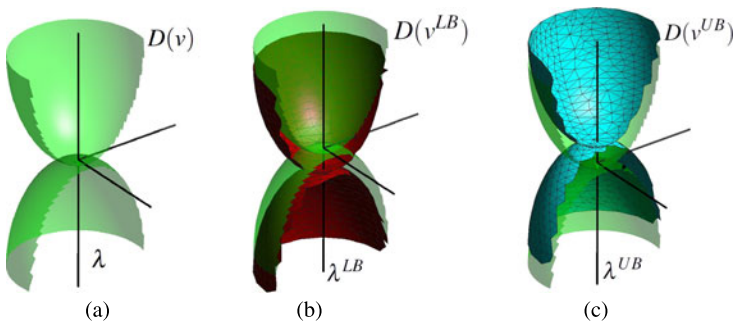
Fig. 1 Illustration of saddle point problem for the (a) analytical solution of limit analysis problem, (b) lower bound discrete limit analysis problem, and (c) upper bound discrete limit analysis problem
