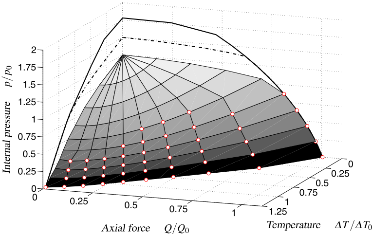
Fig. 9 Three-dimensional shakedown domain with hardening \sigma_H = 1.25\sigma_\gamma
