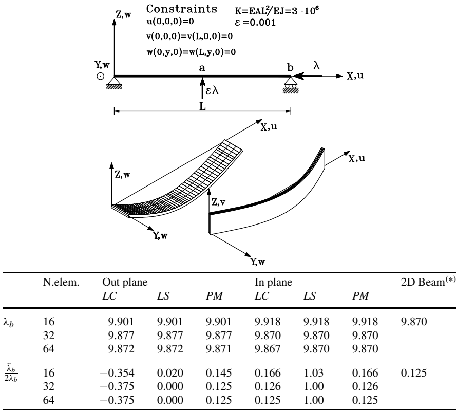
Fig. 3 Euler beam: problem description and buckling and post-buckling parameters
