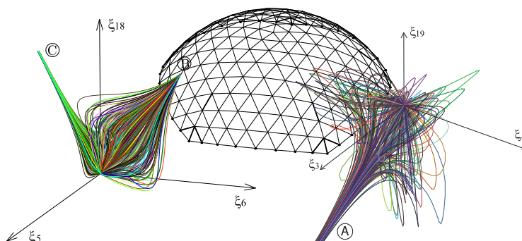
Fig. 10 Geodetic dome: modal interaction between 20 critical modes
