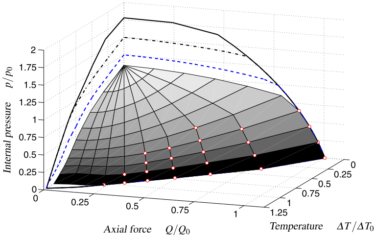
Fig. 8 Three-dimensional shakedown domain with hardening \sigma_H = 1.1\sigma_\gamma
