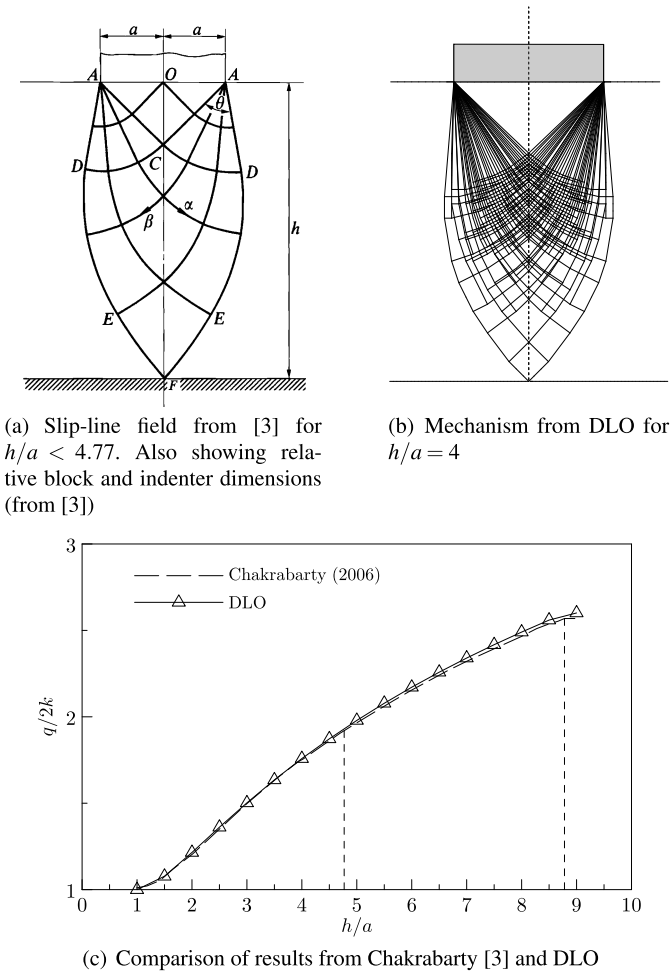
Fig. 13 Punch indentation of a block of finite depth example
