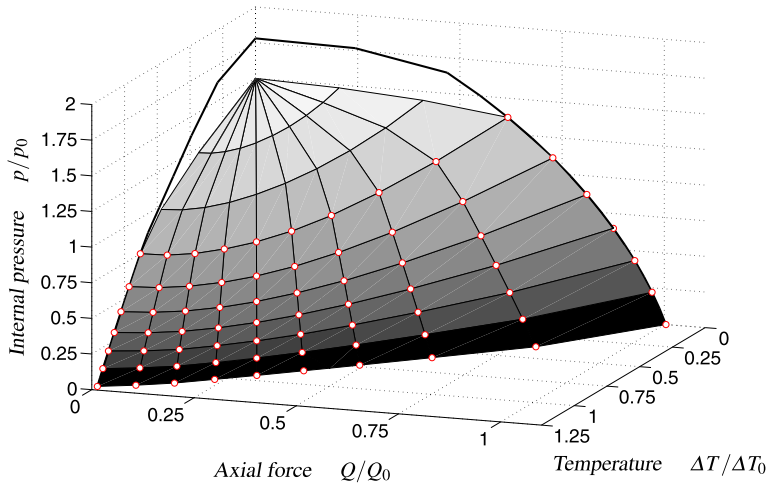
Fig. 10 Three-dimensional shakedown domain with hardening \sigma_H = 1.5\sigma_\gamma
