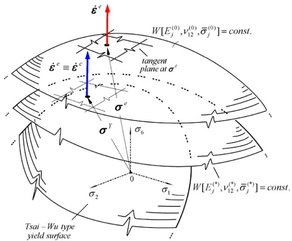
Fig. 1 Matching procedure at a GP in the FE mesh:
