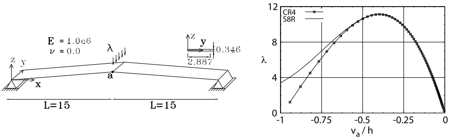
Fig. 5 Shallow arch
