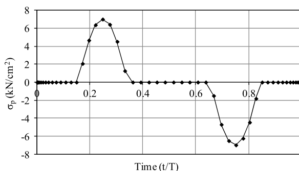
Fig. 6 Predicted \sigma_p^{cs}(t) distribution at steady state inside a cycle for element 1 (load case b—alternating plasticity)
