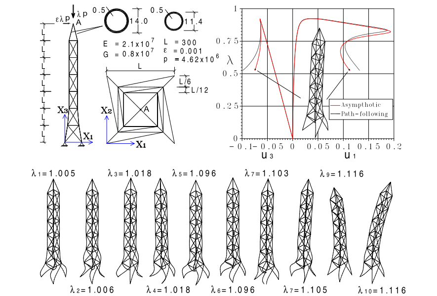
Fig. 7 3D tower: buckling modes and equilibrium paths
