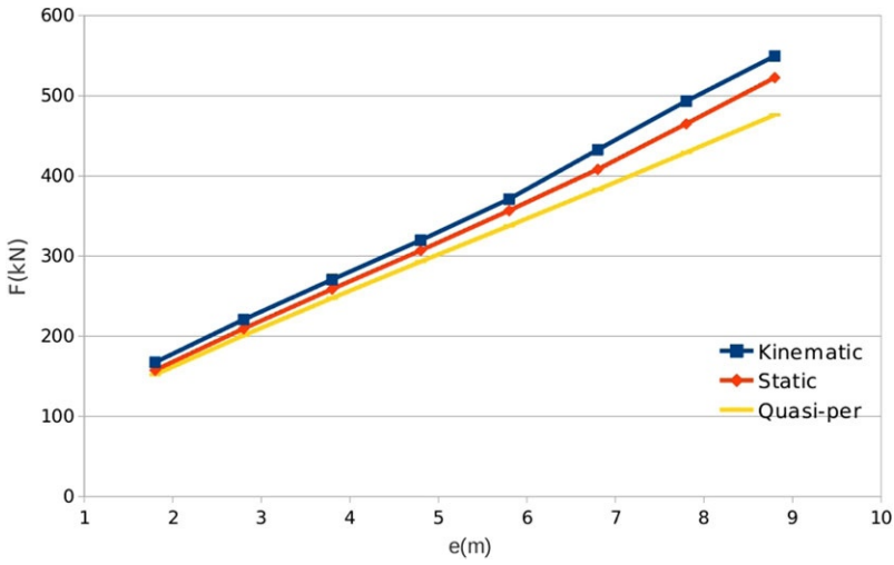
Fig. 8 Limit load for different values of spacing
