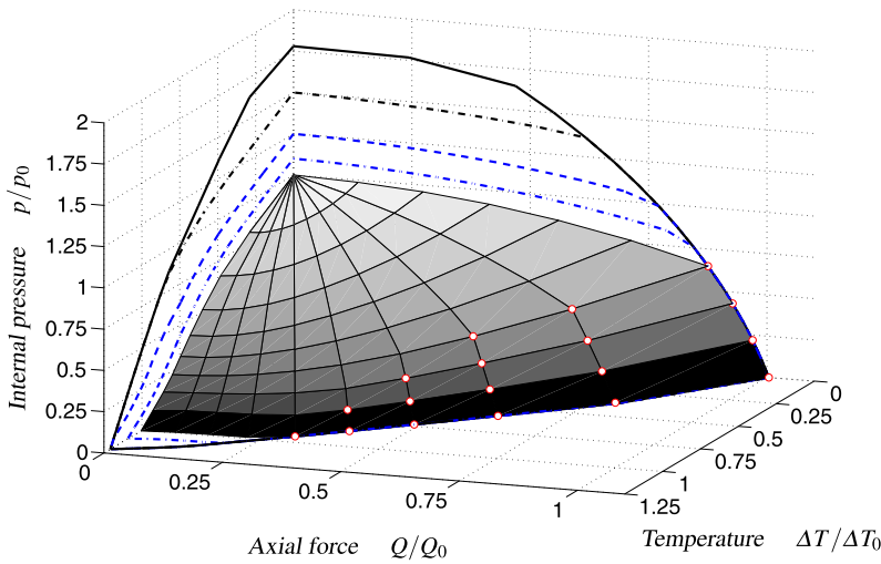
Fig. 7 Three-dimensional shakedown domain without hardening
