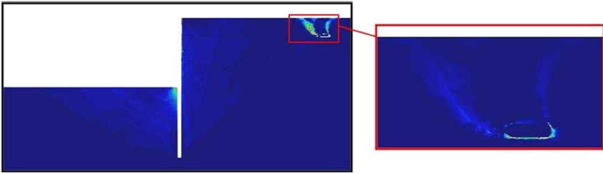
Fig. 10 Contour plot of the dissipation power on an anchored wall. Left : domain without the wall. Right : zoom on the domain surrounding the anchor. Interface soil-anchor and soil-wall conditions are rough with no tension
