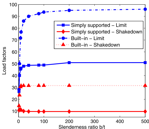
Fig. 5 Plastic collapse and shakedown loads of a rectangular plate
