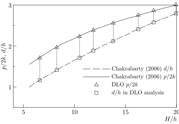
Fig. 16 Combined end and side extrusion example: comparison of results from [3] and DLO
