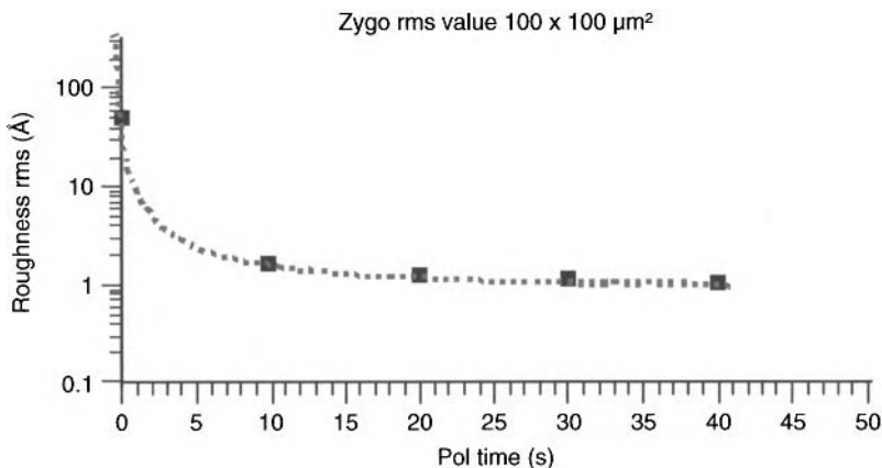
Figure 14.6. Micro-roughness RMS value versus polishing time on polySi, as measured by a Zygo Corp. optical interferometer profiler. Reproduced with permission of SOITEC.
