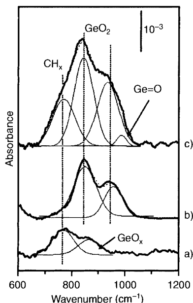
Figure 12.11. Transmission absorption IR spectra of germanium oxides formed a) after 90 min in air, b) after 30 min UV/O 3 exposure and c) after 10 sec in H 2 O 2 (30 wt%). The reference spectrum is H/Ge(100) in all cases (see Section 12.3.4). Gaussian lines are used for the fitting. Unpublished results, used with permission from Chabal.
