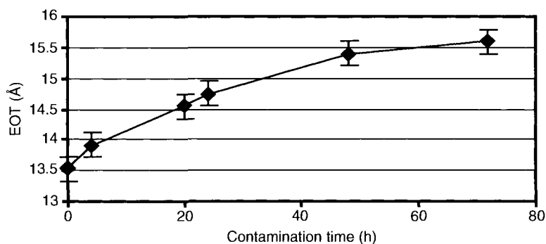
Figure 14.20. Equivalent oxide thickness vs. contamination time upon exposure to an organic material measured by spectroscopic ellipsometry. The film thickness increase is due to the out-gassing of the organic materials and deposition on the silicon surface. Measurement accuracy is better than \pm 0.3 Å. Reproduced with permission of CEA-LETI.
