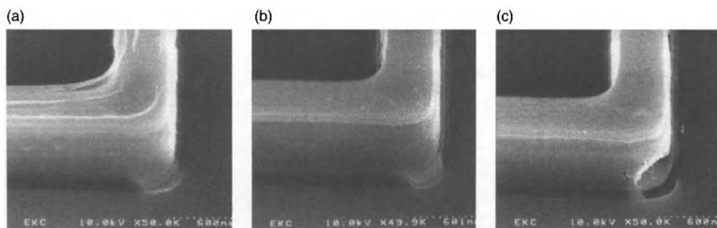
Figure 9.10. Scanning electron microscope images of metal lines over tungsten-filled via a) showing residue remaining after etching and stripping and showing residue removal after cleaning illustrating b) an intact tungsten via, and c) a corroded tungsten via. Courtesy of DuPont/EKC Technology (2010).
