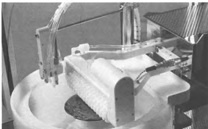
Figure 14.10. Single side brush scrubbing module integrated onto an automatic bonding tool [75]. Reproduced with permission of EV Group (EVG).
