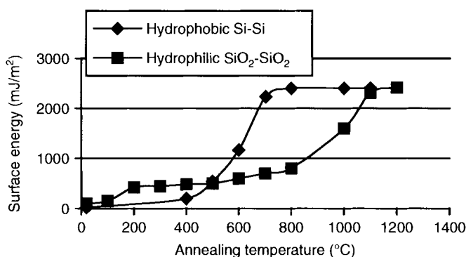
Figure 14.2. Variation of surface energies versus thermal annealing temperature for a) Si-Si hydrophobic bonded structures and b) SiO 2 -SiO 2 hydrophilic bonded structures [19]. Reproduced with permission of Solid State Phenomena, Trans Tech Publications, from Moriceau, H., Rieutord, F., Morales, C., Charvet, A.M., Rayssac, O., Bataillou, B., Fournel, F., Eymery, J., Pascale, A., Gentile, P., Bavard, A., Mézière, J., Maleville, C., and Aspar, B. Solid State Phenomena , Trans Tech Publications.
