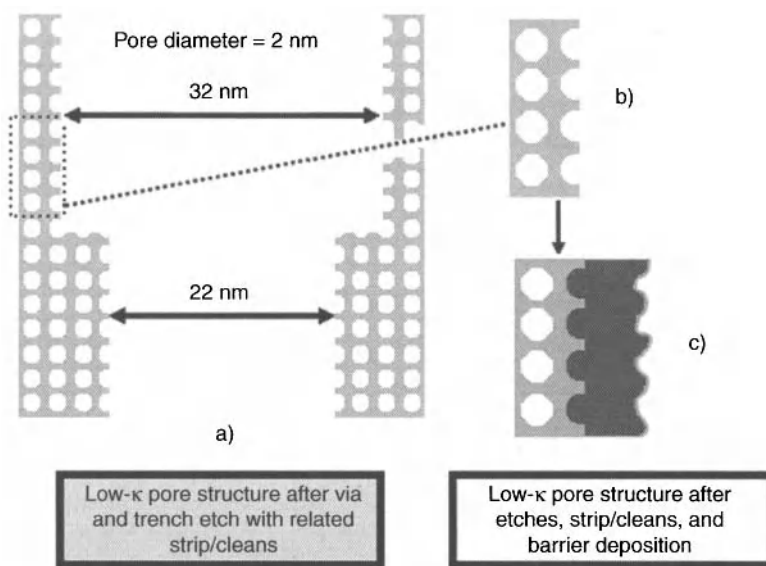
Figure 10.10. A depiction of a porous low- \kappa structure a) after etch/strip/clean exposing pores, b) magnification of exposed surface roughness, and c) transfer of roughness to barrier layer. Note that pore size, via widths, and barrier thickness are to a common scale. Used with the permission of the author.
