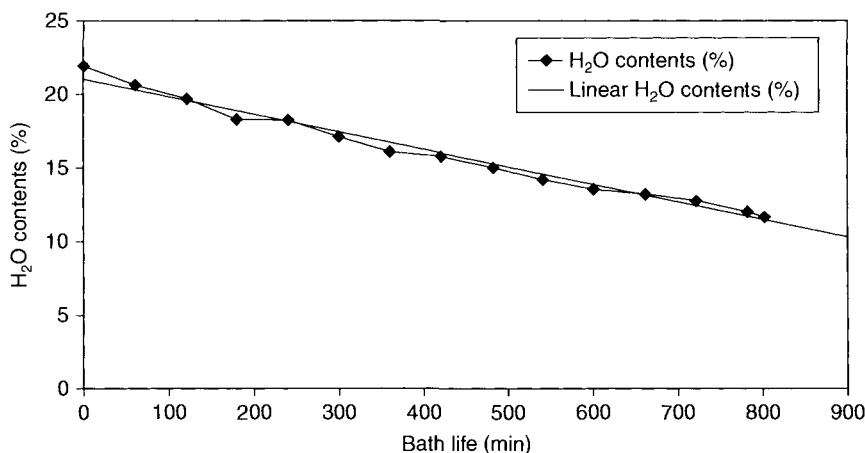
Figure 5.4. The decrease of the water content in hydroxylamine chemistry over the bath life [40]. Reprinted from MICRO . Copyright Tom Cheyney, Los Angeles, CA. Used with permission.
