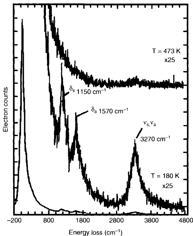
Figure 12.13. High-resolution electron-energy-loss spectra of \text{NH}_3 on \text{Ge}(100) 2 \times 1 . The lower curve shows \text{Ge}(100) exposed to 10L of \text{NH}_3 at T=180\text{K} . The upper curve was taken after annealing the sample at 473K for two minutes and then cooling the sample back down to 180K [68]. Reprinted from Surface Science , Vol. 330(1) and Tindall, C., and Hemminger J. C., "HREELS studies of nitrogen hydrides on Ge (100): Formation of a surface nitride at low temperatures", page 67. Copyright (1995) with permission from Elsevier.
