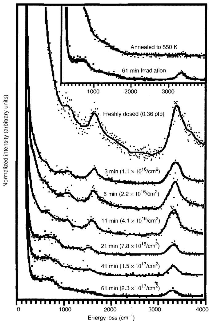
Figure 12.14. High-resolution electron-energy-loss spectroscopy spectra for ammonia adsorbed on Ge(100) 2 \times 1 at 110 K after several exposure times [70]. Reprinted from Applied Surface Science , Vol. 171(3–4), Sanders, M. and Craig, Jr., J.H., "HREELS study of electron irradiation effects on ammonia adsorbed on the Ge(100) surface", page 283. Copyright (2001) with permission from Elsevier.
