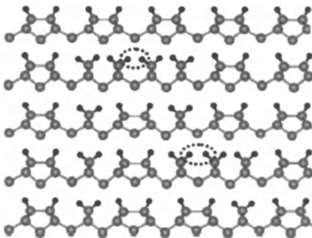
Figure 12.20. Schematic diagram for the Ge 2 \times 1 :H to 3 \times 1 :H transition and antiphase mono-hydride dimer row formation [91]. Reprinted with permission from Maeng, J. Y., Lee, J. Y., Cho, Y. E., Kim, S., and Jo, S. K., Appl. Phys. Lett. , 81(19):3555 (2002). Copyright 2002, American Institute of Physics.
