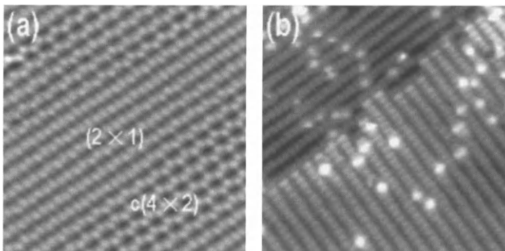
Figure 12.19. Filled-state STM images ( 15 \times 15 \text{ nm}^2 ) of a) the adsorbate-free Ge(100) 2 \times 1 surface and b) the nearly mono-hydride-saturated surface [91]. Reprinted with permission from Maeng, J. Y., Lee, J. Y., Cho, Y. E., Kim, S., and Jo, S. K., Appl. Phys. Lett. , 81(19):3555 (2002). Copyright 2002, American Institute of Physics.
