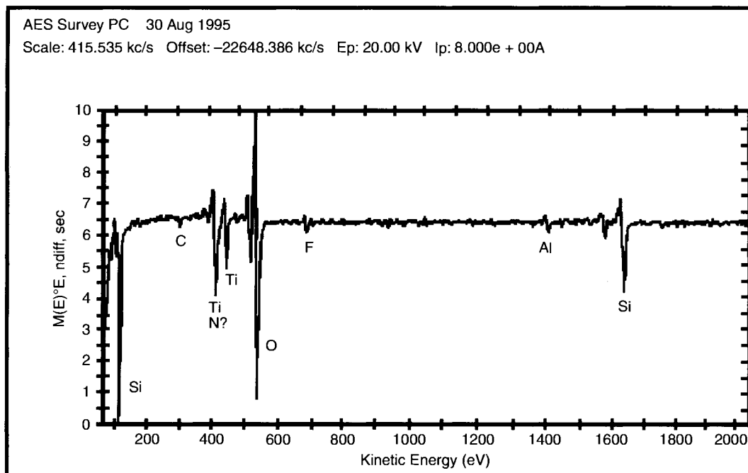
Figure 9.9. Example of Auger electron analysis spectrum of sidewall via residue after O_2 plasma stripping [49]. Reproduced with permission of ECS – The Electrochemical Society from Wang, Y., Graham, S. W., Chan, L., and Loong, S., Journal of the Electrochemical Society .
