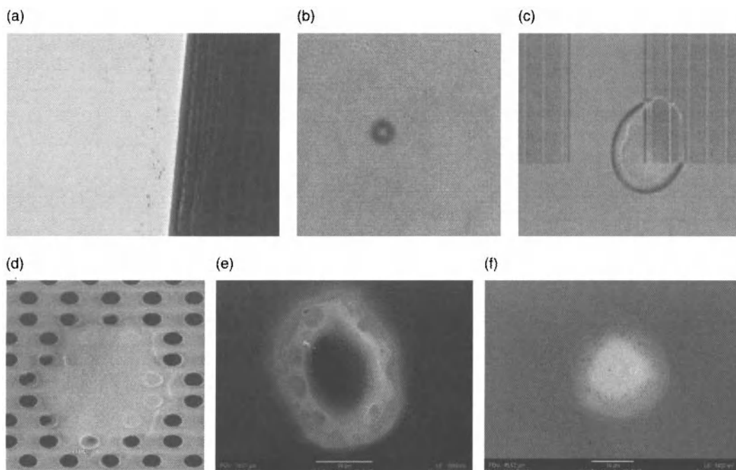
Figure 4.12. Various examples of watermarks; microscope photos of a) spider web-like watermark on the edge of a blanket silicon wafer after SRD, b) round symmetrical watermark on oxide wafer after Marangoni drying probably from a bubble or droplet from a splash and c) round watermark on the edge of a patterned feature; scanning electron microscope (SEM) images of d) 3- \mu\text{m} diameter watermark on contact pattern after single wafer STG drying, probably caused by back-splash, and e) 20–30- \mu\text{m} diameter silica watermark on blanket silicon surface and f) 20- \mu\text{m} diameter watermark on copper. a) and b) Used with permission of the author. c) Courtesy of FSI International. d) Used with permission of DNS. e) and f) Used with permission of Yehiel Gotkis, KLA-Tencor.
