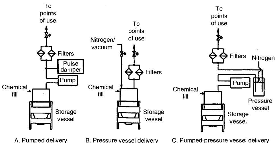
Figure 6.1. Schematics of different types of bulk chemical delivery train designs. Used with permission from CT Associates, Inc.
