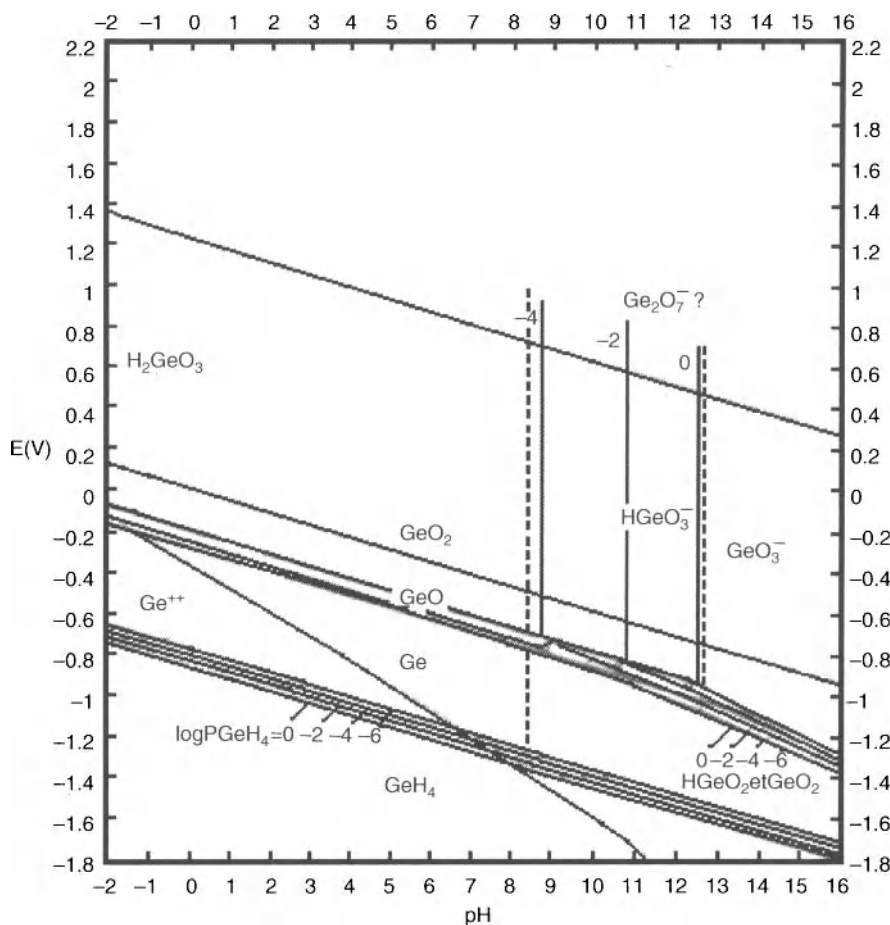
Figure 12.1. Potential-pH equilibrium diagram for the system germanium-water, at 25°C. Reprinted with permission from Pourbaix, M., Atlas of Electrochemical Equilibria in Aqueous Solutions , p. 468, National Association of Corrosion Engineers (NACE) International, Cebelcor, Houston, Texas (1974).
