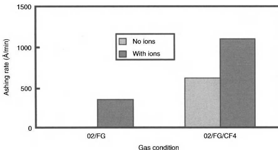
Figure 8.17. Crust removal gas compositions with and without bias power [41]. The temperature is 120 \pm 30^\circ\text{C} . FG = forming gas. Used with permission of Axcelis Technologies.
