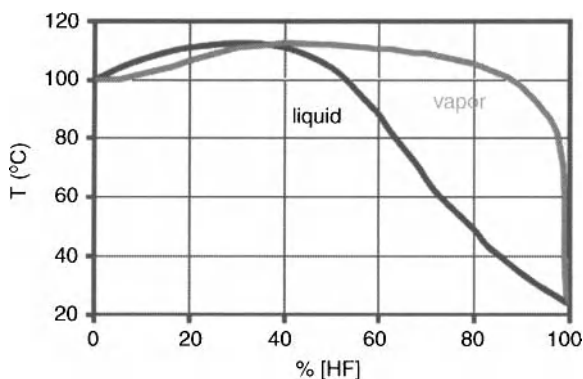
Figure 2.29. Normal boiling point-composition diagram of HF-water in equilibrium. Data points selected from reference [88]. Used with permission of the author.
