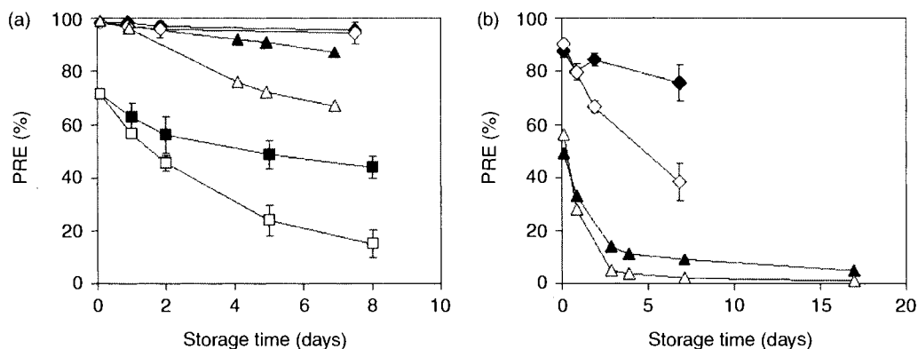
Figure 10.14. Particle removal efficiency vs. storage time for a) 78 nm and b) 34 nm SiO 2 particles. Contaminated wafers stored in dry condition (■ ▲ ◆) and standard (□ ◇ △) clean-room atmosphere [108]. Used with permission from IMEC.
