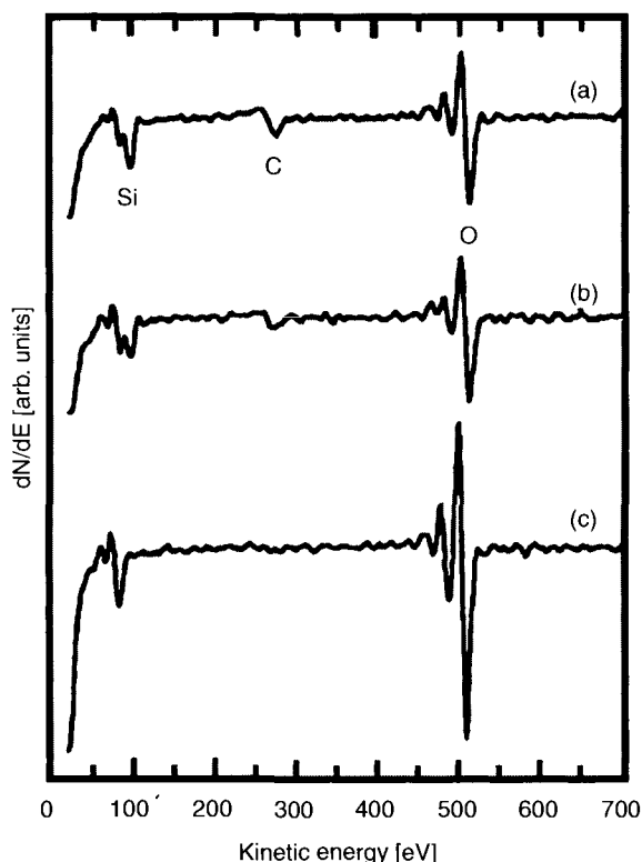
Figure 14.16. Auger survey spectra from a Si wafer a) untreated, b) after RCA cleaning, and c) after H_2 -plasma exposure [100]. The weaker carbon signal after plasma treatment indicates that surface carbon contaminants are more effectively removed with plasma than by RCA cleaning. Reproduced with permission of the Korean Physics Society from Choi, W. B., Ju, C. M., Lee, J. S., and Sung, M. Y., J. Korean Phys. Soc.
