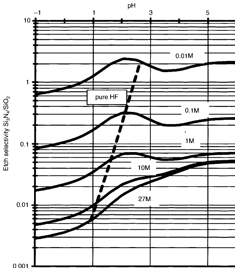
Figure 3.26. The etch selectivity between LPCVD Si 3 N 4 and thermally grown SiO 2 as a function of pH at different total fluoride concentrations (25°C) [49]. Reprinted from MICRO Magazine , Copyright 2005, Tom Cheney, Los Angeles, CA. Used with permission.
