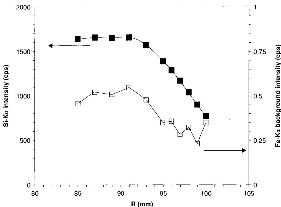
Figure 15.6. Intensity dependence on radius, R , in measurement coordinates for Si-K \alpha and Fe-K \alpha backgrounds for a 200-mm silicon wafer [24]. Used with permission from H. Takahara.
