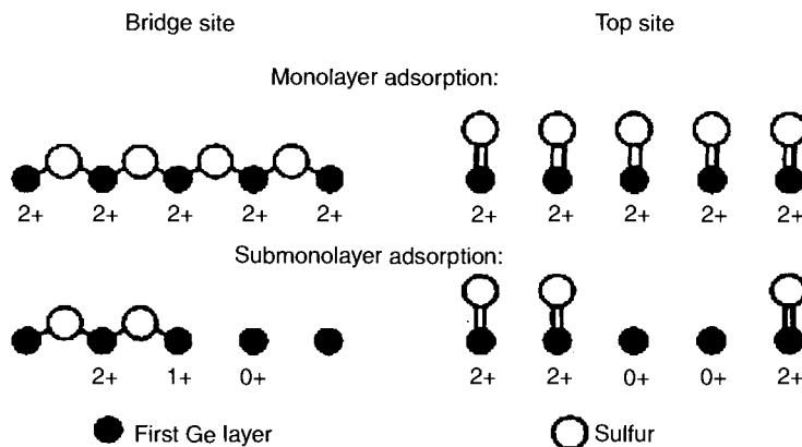
Figure 12.31. Bridge-site and top-site bonding can be distinguished by the appearance of the oxidation state 1^+ in the case of low-coverage adsorption [112]. Reprinted figure with permission from Weser, T., Bogen, A., Konrad, B., Schnell, R. D., Schug, C. A., and Steinmann, W., Phys. Rev. , B35(15):8184 (1987). Copyright 1987 by the American Physical Society.
