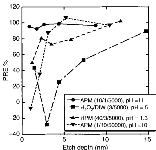
Figure 12.7. Particle removal efficiency of silica particles from Ge using • APM (SC-1) (5000:1:10) ▼ APM (50000:10:1) ■ H 2 O 2 /DIW (3/5000), and ▲ HPM (SC-2) (5000:3:40) [47]. All solutions have an etching rate ~3 nm/min except APM (50000:10:1), which etches at a rate of 1.3 nm/min. APM is ammonium hydroxide hydrogen peroxide mixture and HPM is hydrochloric hydrogen peroxide mixture. Used with permission of IMEC.
