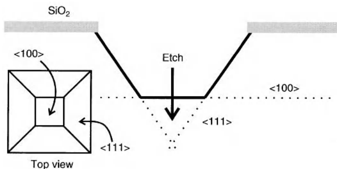
Figure 3.16. Etch profile due to anisotropic etch of \langle 100 \rangle silicon in \text{KOH} (aq). Used with permission of the author.
