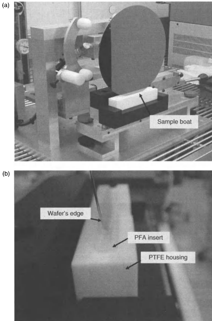
Figure 15.10. (a) Wafer vertically supported for analysis of the bevel and edge, and (b) side view of the wafer edge making contact with the extraction solution in the Teflon® perfluoroalkoxy (PFA) insert of the sample boat [46]. Used with permission from SPIE; Sparks, C., Gondran, C., Lysaght, P., and Donahue, J., "Novel Technique for Contamination Analysis Around the Bevel and Edge Exclusion Areas of 200 and 300 mm Silicon Wafers," Process and Materials Characterization and Diagnostics in IC Manufacturing , Volume 5041 (2003).
