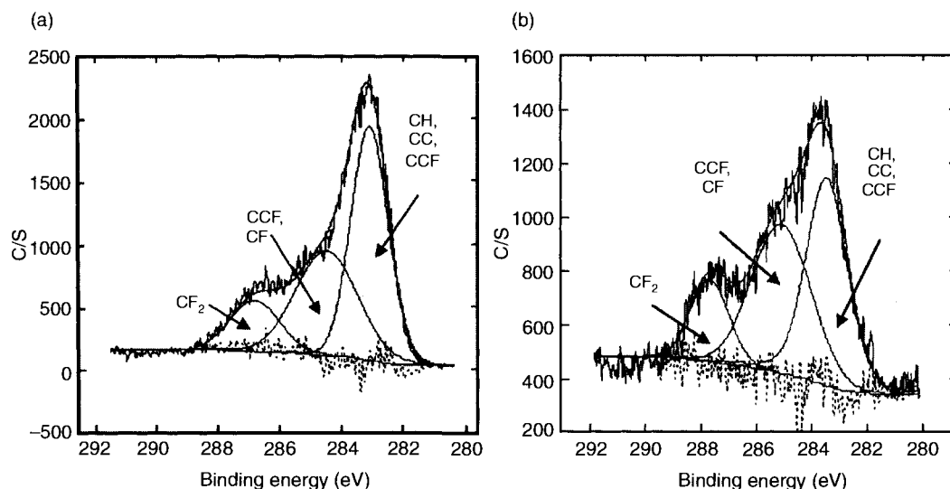
Figure 10.3. X-ray photoelectron spectrum of a) residue on the sidewall and bottom of a dual damascene via structure and b) comparison of a fluorocarbon polymer sample obtained from Air Products [15]. Reproduced with permission of ECS – The Electrochemical Society from Levitin, G., Myneni, S., and Hess, D. W., Journal of the Electrochemical Society .
