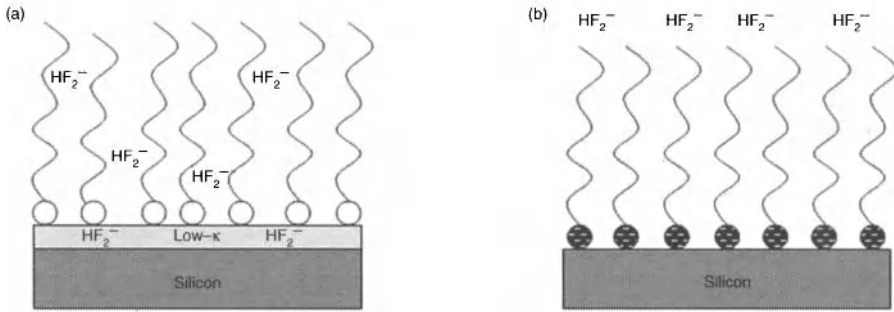
Figure 13.10. The wetting behaviour of the (a) surfactant A allowing the penetration of the active low- \kappa etching species, \text{HF}_2^- , to the film surface to perform dissolution and the passivating behavior of (b) surfactant B on the silicon surface blocking the active etching species from damaging the underlying substrate surface. Used with permission of the authors.
