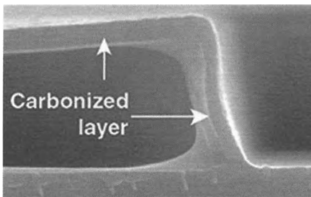
Figure 8.6. Cross section SEM of high dose ion implanted photoresist at 50 keV, 15 mA, As + . For illustration, a delineation etch removed the unchanged resist leaving behind only the heavily carbonized crust [9]. Used with permission from Axcelis Technologies.
