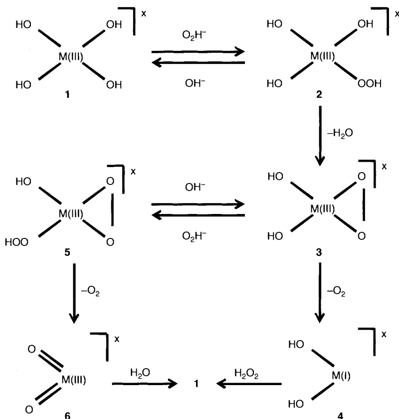
Figure 2.8. Proposed reaction mechanism of metal-ion catalyzed \text{H}_2\text{O}_2 decomposition. In this example, the metal ion has an oxidation state III, and the species has a charge of x = -1 . \text{H}_2\text{O}_2 is represented by its \text{O}_2\text{H}^- anion [28]. Reproduced with permission of ECS – The Electrochemical Society from Knotter, D. M., Gendt, S. D., Baeyens, M., Mertens, P. W., and Heyns, M. M., Journal of the Electrochemical Society .
