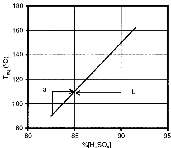
Figure 2.22. Estimation of equilibrium temperature set by water attraction and evaporation of \text{H}_2\text{SO}_4 dissolved in water under clean room condition [68]. Used with permission of the author.
