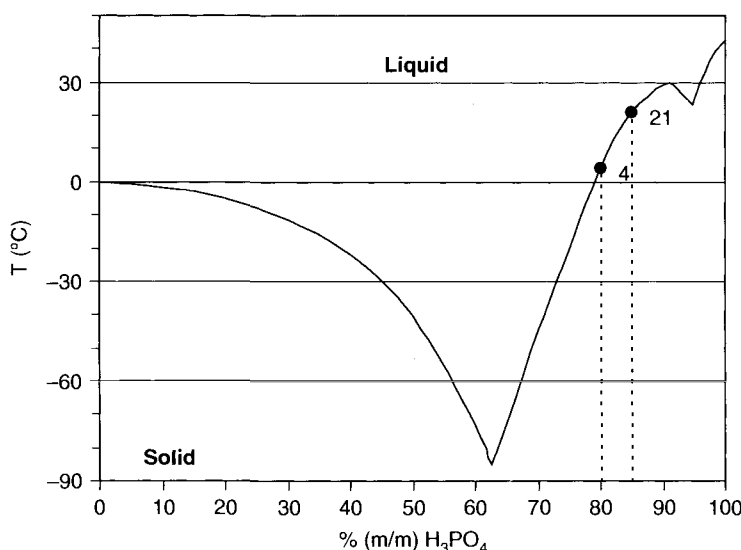
Figure 3.30. Phase diagram of \text{H}_3\text{PO}_4 . Commercially available 85% \text{H}_3\text{PO}_4 can crystallize at room temperature [56]. Reprinted with permission from Brown, E. H. and Whitt, C. D., Industrial and Engineering Chemistry , 44(3):615. Copyright 1952 American Chemical Society.
