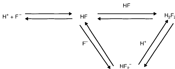
Figure 3.7. Equilibrium reaction between fluoride species. Used with permission of the author.
