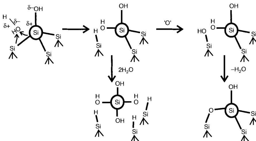
Figure 3.13. Etching of a monolayer of SiOH by water and, alternatively, formation of a silicon dioxide layer. Used with permission of the author.
