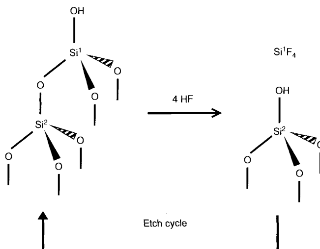
Figure 3.3. Depiction of layer-by-layer etching of SiO 2 by HF [11]. Reprinted with permission from Knotter, D. M., J. Am. Chem. Soc. , 122(18):4345. Copyright 2000 American Chemical Society.
