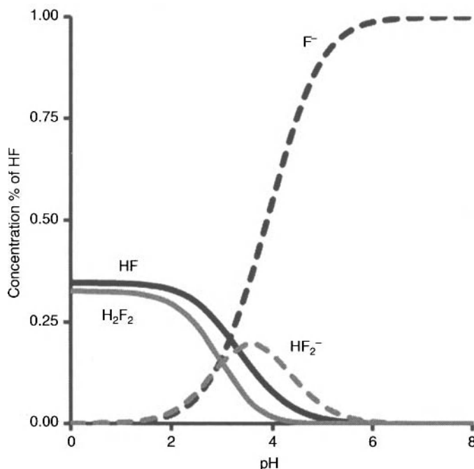
Figure 3.8. Concentration of F-containing species as function of pH in water with C_F = 1 M (~2 wt% HF) based on reference [13]. Reproduced with permission of ECS – The Electrochemical Society from Verhaverbeke, S., Teerlinck, I., Vinckier, C., Stevens, G., Cartuyvels, R. and Heyns, M. M., Journal of the Electrochemical Society .
