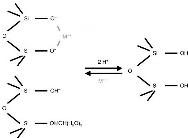
Figure 2.20. Examples of metal-ion desorption. Used with permission of the author.
