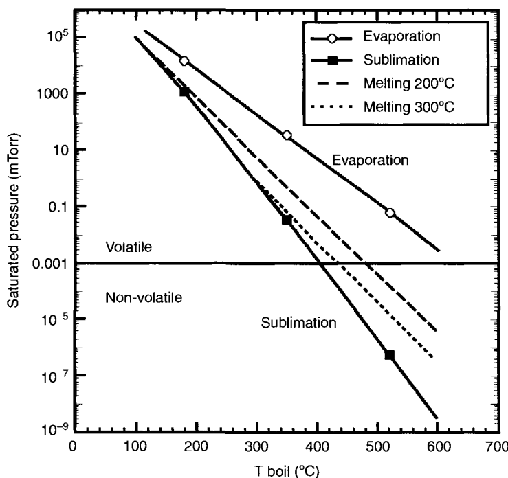
Figure 7.12. Saturated vapor pressure of compounds with melting temperatures of 200 and 300°C as a function of their boiling temperature at atmospheric pressure. Data is compiled from [112]. Used with permission from Shamiryan.
