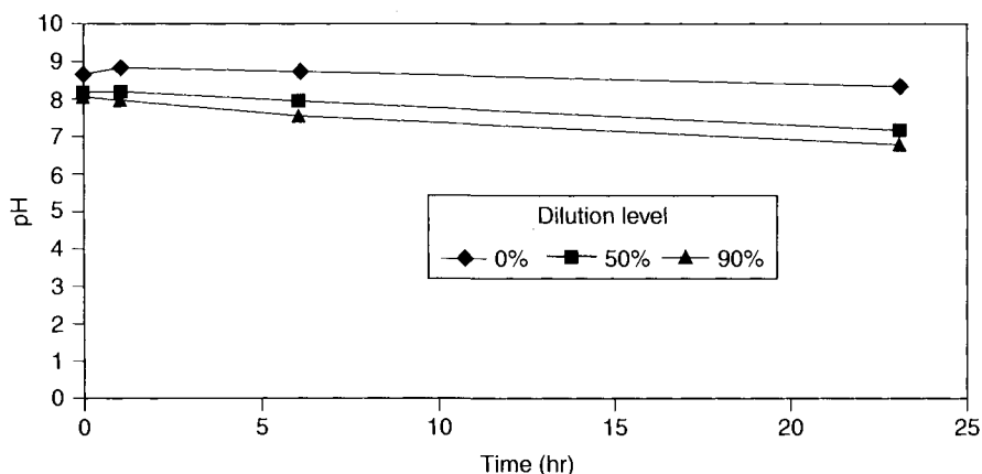
Figure 5.3. pH drift vs. bath life for semiaqueous chemistry with different dilution levels [31]. Reprinted from MICRO . Copyright Tom Cheyney, Los Angeles, CA. Used with permission.
