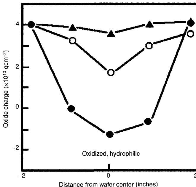
Figure 4.3. The charge across the diameter of hydrophilic oxidized wafers \triangle prior to dump rinse, \circ after dump rinse and spin dry, and \bullet after dump rinse and spin rinse dry [17]. Used with permission of V., Wu, A. T., Chatterjee, A., and Fraser, D. B., IEEE VLSI Symposium Technical Digest . © 1990 IEEE.
