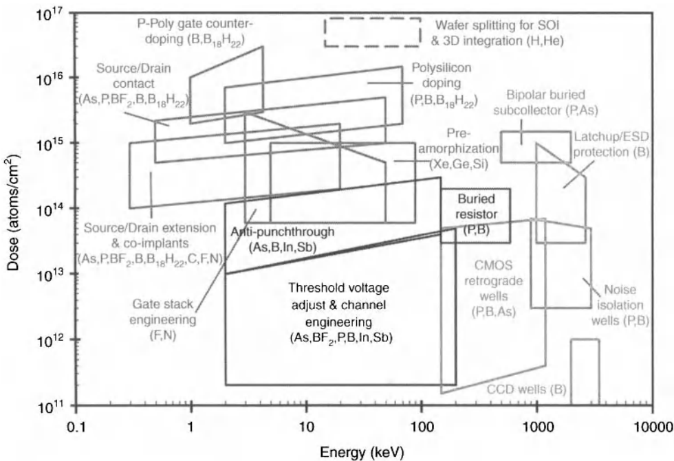
Figure 8.1. The high dose implant regime is defined as greater than 5 \times 10^{14} atoms/cm 2 . Various implant layers are shown that use high doses. Adapted from [1]. Updated 2010 and used with permission from Axcelis Technology.
