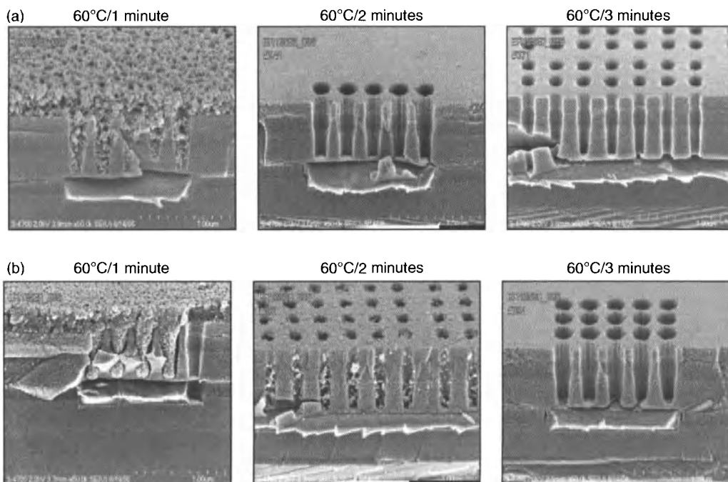
Figure 16.4. Scanning electron microscope image for the removal of photoresist at the BEOL trench level, used for reworking the lithography layer; a) center location and b) edge location [37]. Reproduced with permission of ECS – The Electrochemical Society from Wu, A., Baryschpolec, E., Molnar, L., Henry, S.-A., Detterbeck, S., Brilz, L., Bartsch, C., Sulzer, G., and Ott, A., ECS Transactions .
