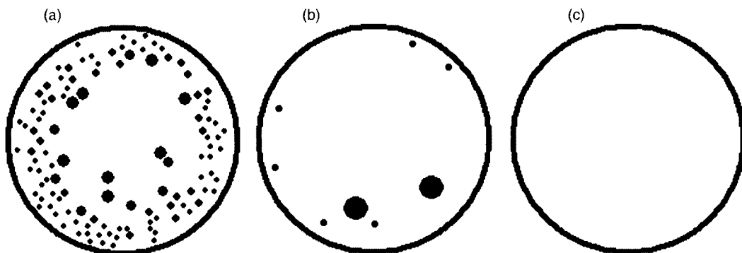
Figure 14.26 Scanning acoustic microscopy images obtained after 400°C post-bonding anneals of 200-mm Si-Si bonded wafers: a) reference (RCA-based cleaning), b) 400°C-pre-bond anneal and c) 500°C pre-bond anneal [65]. Reproduced with permission of ECS – The Electrochemical Society from Ventosa, C., Rieutord, F., Libralesso, L., Fournel, F., Morales, C., and Moriceau, H., The Journal of the Electrochemical Society .
