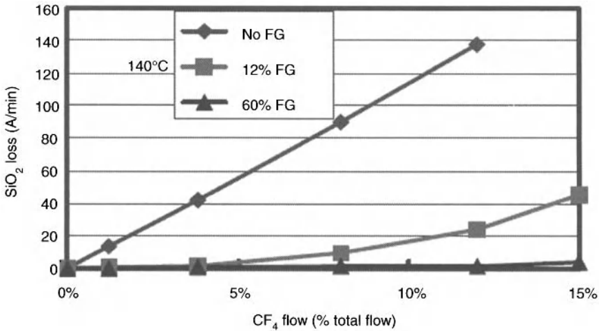
Figure 8.18. Silicon dioxide loss with respect to \text{CF}_4 concentration with varying amounts of forming gas (4% \text{H}_2 and 96% \text{N}_2 ) [67]. Used with permission of Axcelis Technologies.
