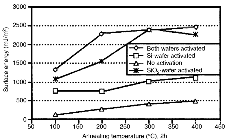
Figure 14.15. Surface energy of SiO_2 / Si bonded pairs as a function of annealing temperature for ( \Delta ) no activation and Ar plasma activation for 30 sec; ( \square ) Si, ( * ) SiO_2 wafer, and ( \diamond ) both wafers [92]. Reproduced with permission of ECS – The Electrochemical Society from Suni, T., Henttinen, K., Suni, I., and Makinen, J., The Journal of the Electrochemical Society .
