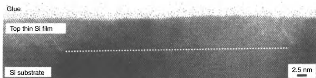
Figure 14.30. Cross sectional TEM image of stacking faults from twist interface dislocations. The bonding interface is highlighted by the white dotted line [147]. Reprinted with permission of American Institute of Physics from Rousseau, K., Rouvière, J. L., Fournel, F. and Moriceau, H., Applied Physics Letters . © 2002, American Institute of Physics.
