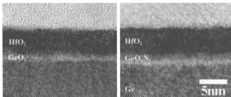
Figure 7.10. Transmission electron microscope images of interfacial oxide layer on germanium of a) \text{GeO}_x or b) \text{GeO}_x\text{N}_y [95]. Used with permission from Kim, H., McIntyre, P. C., Chui, C. O., Saraswat, K. C., Cho, M.-H, Applied Physics Letters , 85(1404):2902 (2004). Copyright 2004, American Institute of Physics.
