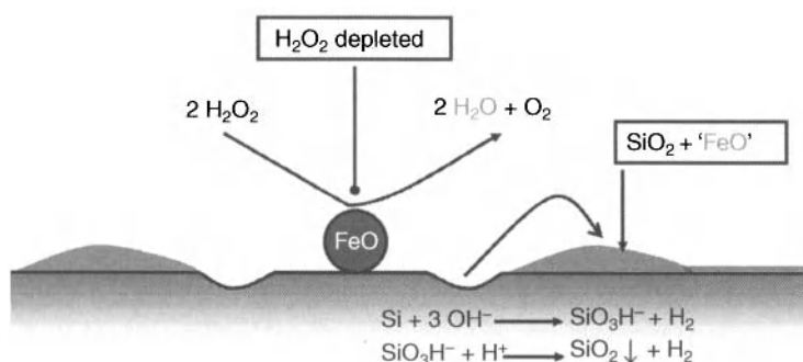
Figure 2.18. Schematic of hydrogen peroxide concentration profile around an Fe precipitate and the resulting etch profile. Within the circle, the \text{H}_2\text{O}_2 concentration is below an 3 mmol/L [34]. Reproduced with permission of ECS – The Electrochemical Society from Knotter, D. M., Gendt, S., Mertens, P. W., and Heyns, M. M., Journal of the Electrochemical Society .
