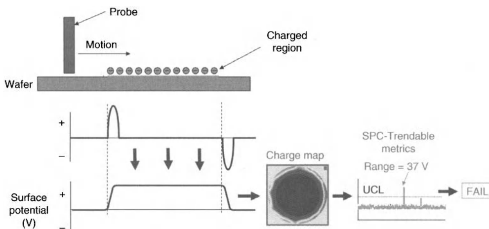
Figure 15.13. Schematic of surface potential difference imaging from Qcept [50]. Used with permission from Qcept Technologies.
