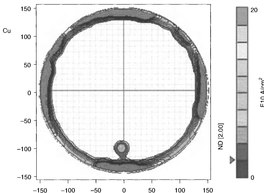
Figure 15.7. Copper contamination detected on the back surface of a 300-mm wafer, near the edge [24]. Reprinted with permission from Kohno, H., Yamagami, M., Formica, J., and Shen, L., Abstracts of Frontiers of Characterization and Metrology for Nanoelectronics . Copyright 2009, American Institute of Physics.
