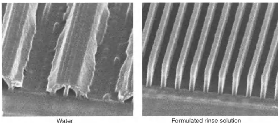
Figure 16.5. Pattern collapse of high aspect ratio features with water and its elimination with a formulated rinse solution [38].
