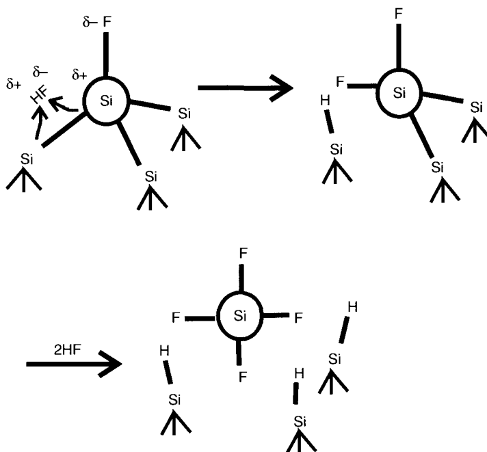
Figure 2.27. Oxidative addition of HF on a Si-Si bond. Due to the polarity of HF and Si-F, the F binds to the silicon already bonded F-atom. After three successive additions SiF 4 liberates, and the Si-surface is H-terminated. Used with permission of the author.
