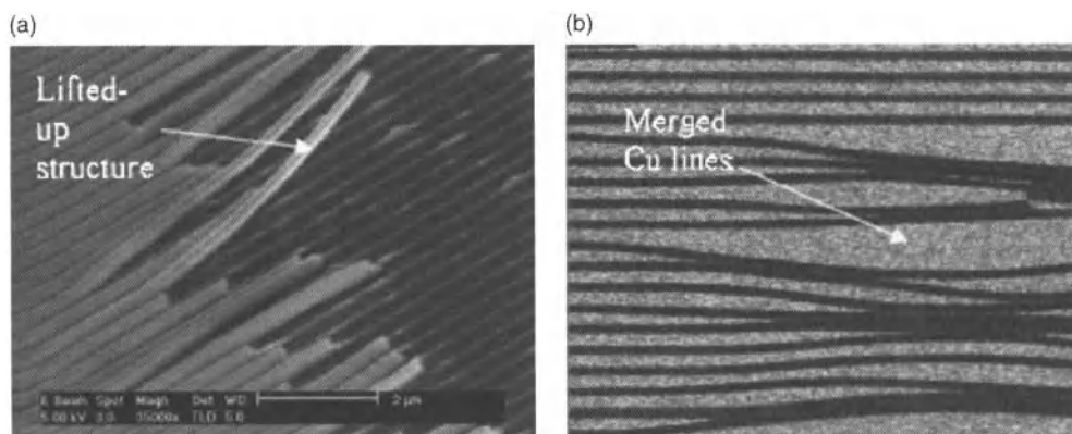
Figure 16.3. Comb structures of copper in a low- \kappa structure; a) after processing in SWT with amine-based cleaning and b) after CMP [34]. Reprinted from Microelectronics Reliability , Vol. 45, Tsang, C. F., Chang, C. K., Krishnamoorthy, A., Ee, K. J., Su, Y. J., Li, H. Y., Li, W. H., and Wong, L. Y., “A study of post-etch wet clean on electrical and reliability performance of Cu/low \kappa interconnections”, page 517. Copyright (2005) with permission from Elsevier.
