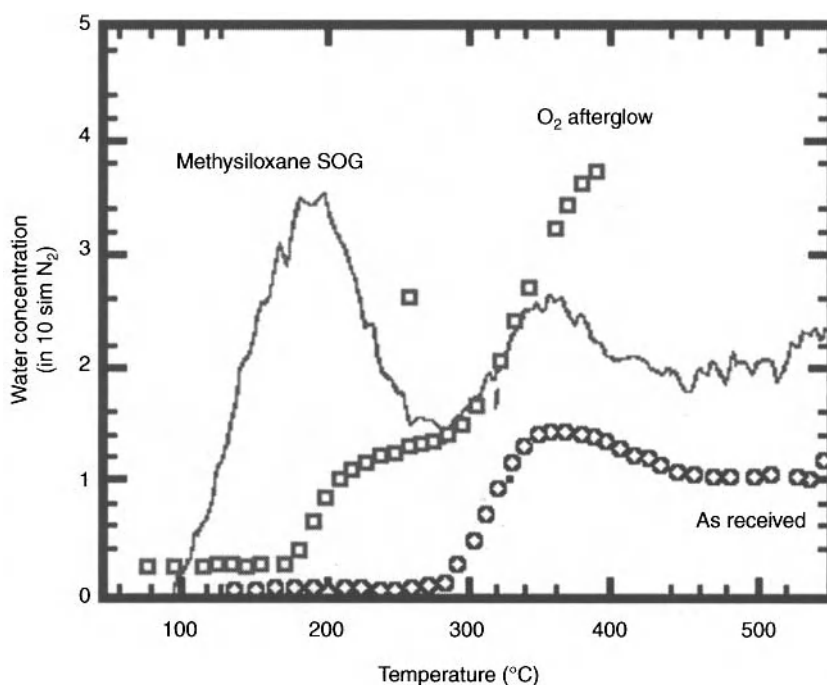
Figure 10.6. Water thermal desorption spectrum of untreated and \text{O}_2 plasma-treated films showing the water concentration [26]. The plasma treated films had significant water absorbed compared to the untreated SOG MSQ films. Reproduced with permission of ECS – The Electrochemical Society from Kondoh, E., Baklanov, M. R., Bender, H., and Maex, K., Electrochemical and Solid State Letters .
