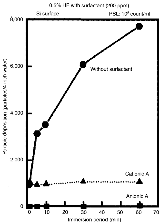
Figure 10.18. Particle deposition vs. surfactant type for PSL spheres on and Si wafers [140]. The amount of particles deposited increased with immersion time when a surfactant was not used. Reproduced with permission of ECS – The Electrochemical Society from Itano, M., Kezuka, T., Ishii, M., Unemoto, T., Kubo, M., and Ohmi, T., Journal of the Electrochemical Society .
