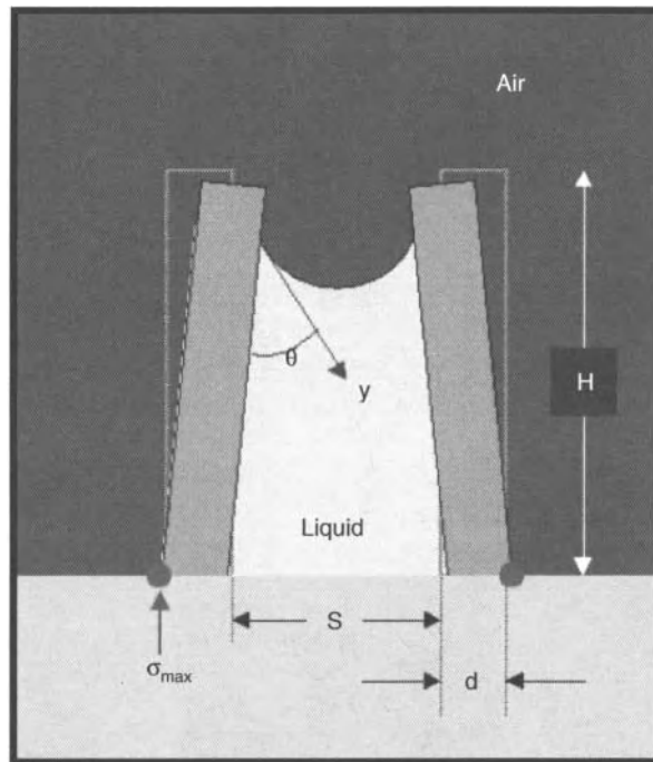
Figure 16.7. Physics of photoresist collapse, stress model [40]. Reproduced with permission from Petricich, G., Suzuki, K., Munemasa, J., Yoshikawa, T., Kawakami, N., Shimizu, S., and Watanabe, M., "Supercritical Resist Dry Technique for Electron-Beam Projection Lithography (EPL)" Proc. SPIE, Emerging Lithographic Technologies VII , 5037:917 (2003).
