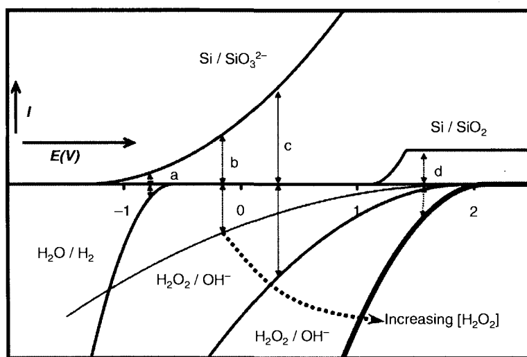
Figure 2.3. Model of the I-E (current-potential) curve for the etching of silicon with ammonia (pH = 10.5) and hydrogen peroxide. The relative position on the y-axis is not on scale. The vertical arrows indicate positions of possible equilibrium potentials. Used with permission of the author.
