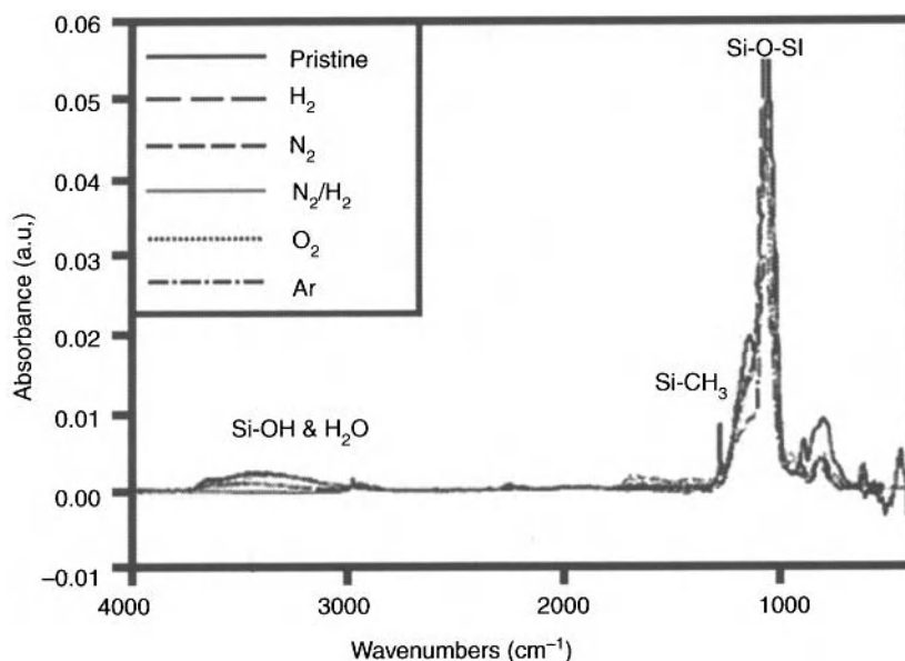
Figure 10.7. Fourier transform infrared spectra of CDO low- \kappa film after the photoresist pattern has been stripped with various chemistries [38]. Argon has the highest affect on the Si-CH 3 bond, while N 2 or O 2 plasmas have the highest affect on the Si-O-Si bonds. Reprinted with permission from Bao, J., Shi, H., Liu, J., Huang, H., and Ho, P. S., Goodner, M. D., Moinpour, M., and Kloster, G. M., Journal of Vacuum Science Technology , B26(1):219. Copyright 2008, American Institute of Physics.
