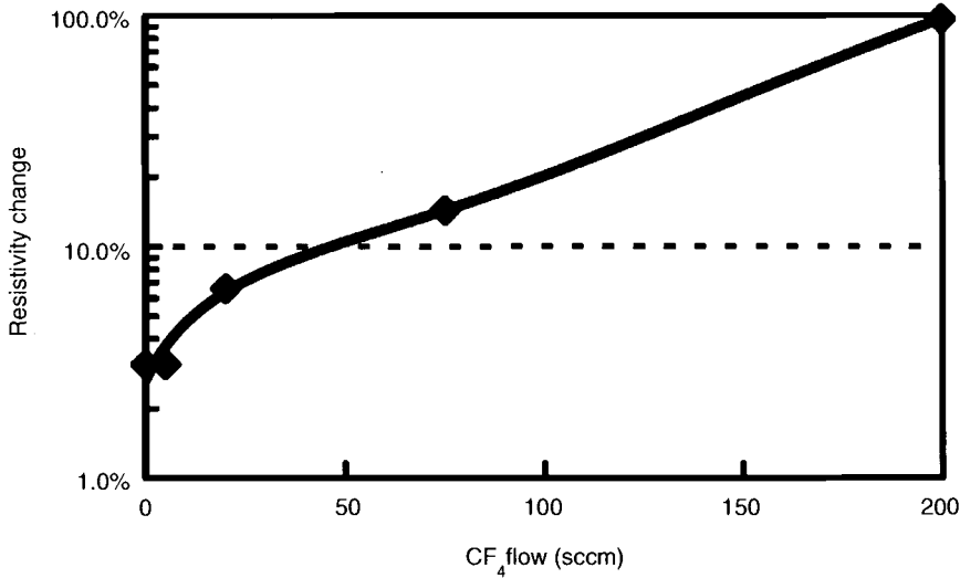
Figure 8.13. The change in sheet resistance caused by \text{CF}_4 -containing plasma stripping process, as compared to a \text{CF}_4 -free stripping process [40]. The plasma process conditions are 7000 sccm total flow with 10% \text{H}_2/\text{N}_2 in \text{O}_2 . The implant conditions are 2.0 keV As at 5 \times 10^{14} atoms/ \text{cm}^2 dose, then annealed 10 sec at 1000^\circ\text{C} . Used with permission of Berry, I. L., Waldfried, C., Han, K., Luo, S., Sonnemans, R., and Ameen, M., 8th International Workshop Junction Technology (IWJT) . © 2008 IEEE.
