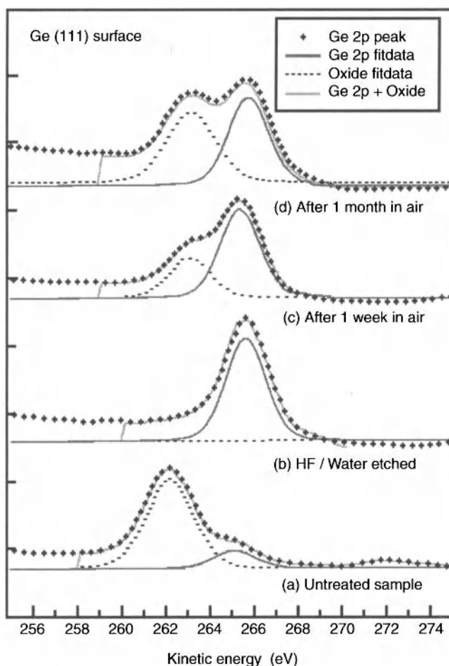
Figure 12.22. Ge 2p_{1/2} core level of Ge(111) a) as received, b) after HF/water etched, c) etched sample after 1 week in air, d) etched sample after 1 month in air [94]. Reprinted from Applied Surface Science , Vol. 123/124, Deegan, T. and Hughes, G., "An X-ray photoelectron spectroscopy study of the HF etching of native oxides on Ge(111) and Ge(100) surfaces" page 66. Copyright (1998) with permission from Elsevier.
