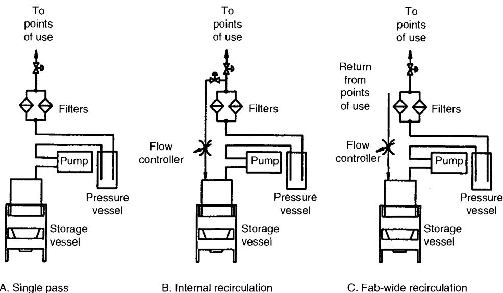
Figure 6.2. Bulk chemical delivery system designs with recirculation for improved particle performance. Used with permission from CT Associates, Inc.
