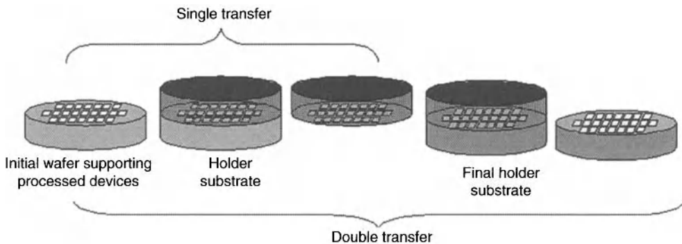
Figure 14.4. Transfer of an integrated circuit thin film pattern onto a substrate [29]. Reproduced with permission of ECS – The Electrochemical Society from Aspar, B., Lagahe-Blanchard, C., and Moriceau, H., Semiconductor Wafer Bonding: Science, Technology, and Applications VIII .
