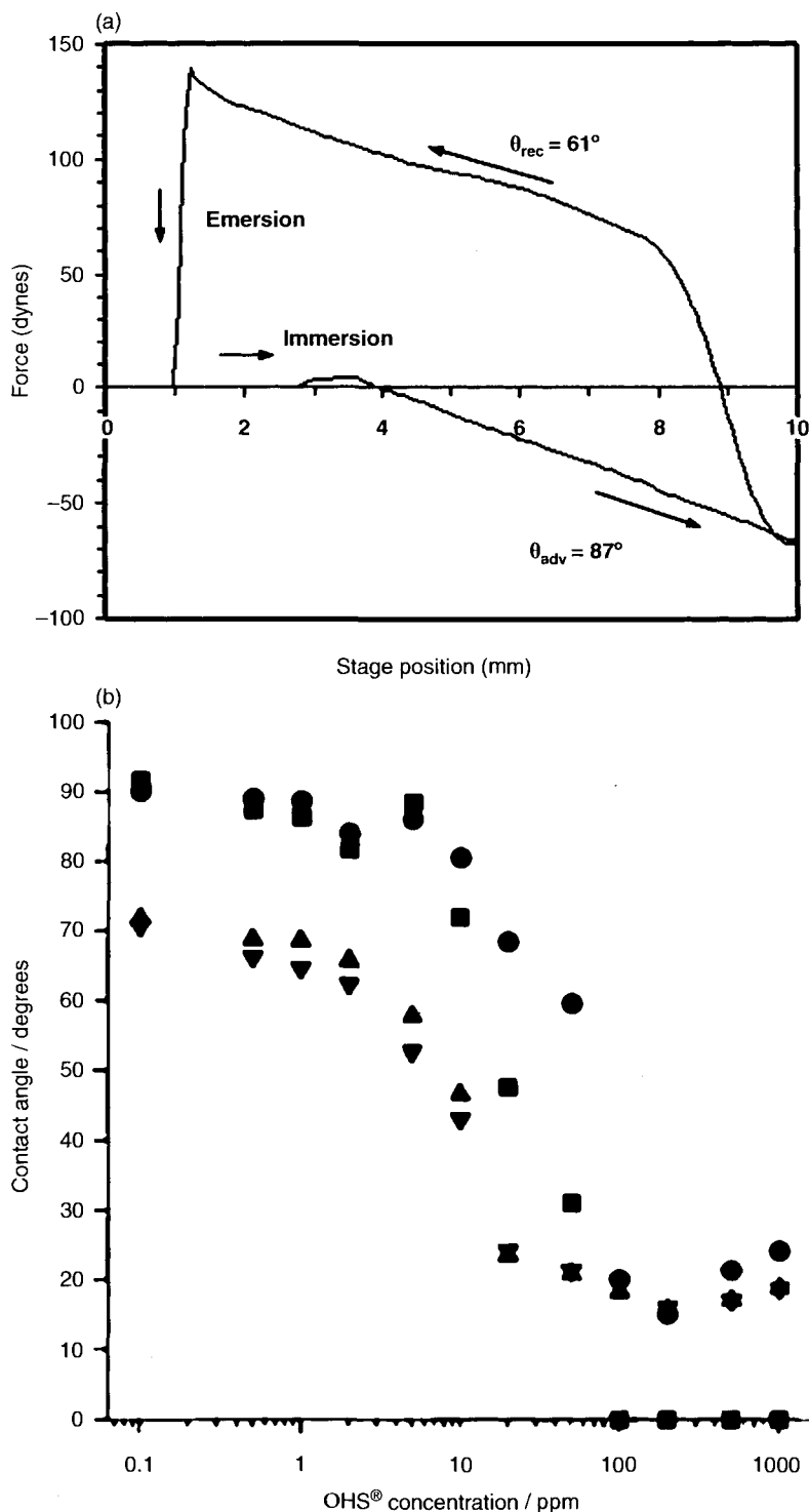
Figure 1.16. Advancing and receding contact angles of a) DIW on hydrogen terminated silicon, and b) 100:1 HF on silicon as a function of OHS ® concentration (●) cycle 1 advancing, (■) cycle 2 advancing, (▲) cycle 1 receding, (▼) cycle 2 receding [64]. a) Used with permission from authors. b) Reproduced with permission of ECS – The Electrochemical Society from Haworth, P., Kovach, M., Sperline, R., and Raghavan, S., Journal of the Electrochemical Society .
