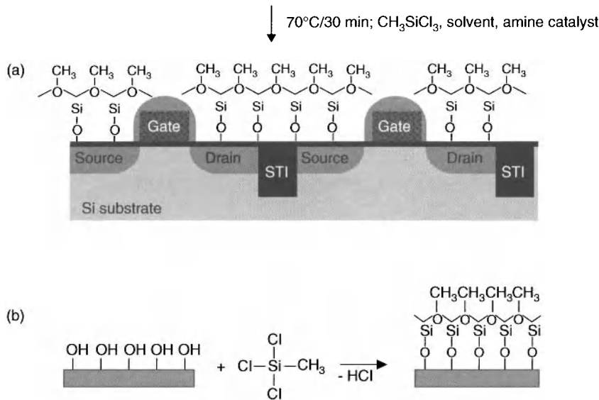
Figure 8.23. Schematic representation of a NMOS/PMOS gate structure with (a) the self-assembled monolayer formation on exposed SiO 2 film and (b) silanization mechanism for the hydroxyl terminated substrate surface [12]. Used with permission of ATMI.
