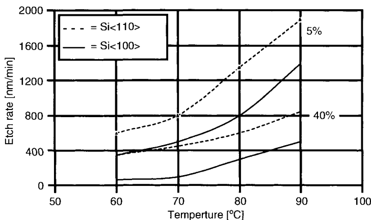
Figure 3.20. Etching rates of silicon in 5 and 40 wt% TMAH [43]. Used with permission of A. A. M. van de Vorst (NXP).
