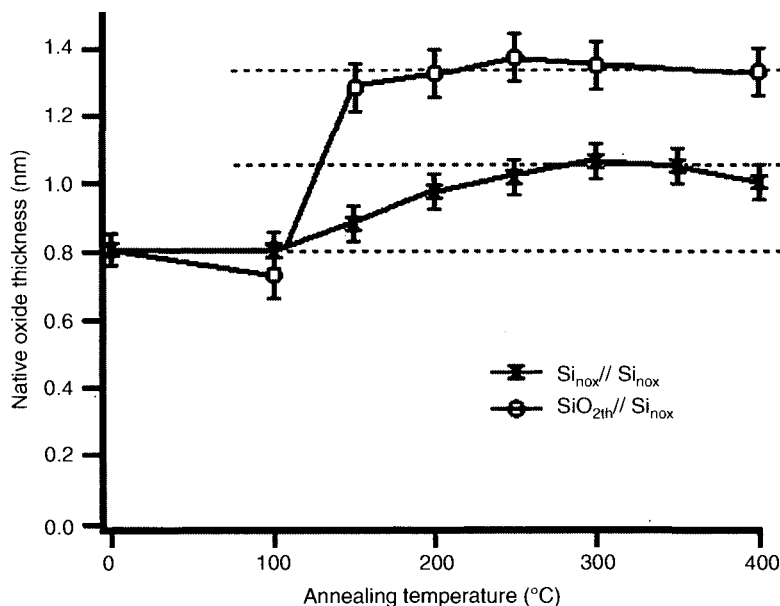
Figure 14.27. Growth of native silicon dioxide film for bonded wafers as a function of the post-bonding anneal temperature for Si//SiO 2 bonding (only a native oxide, empty circles) compared to Si//Si bonding (two native oxides, full triangles) [138]. Reprinted with permission of American Institute of Physics from Ventosa C., Rieutord F., Libralesso L., Morales C., Fournel F. and Moriceau H., Journal of Applied Physics . © 2008, American Institute of Physics.
