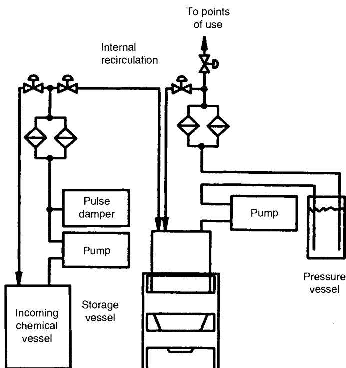
Figure 6.4. Optimized bulk chemical delivery equipment design. Used with permission from CT Associates, Inc.
