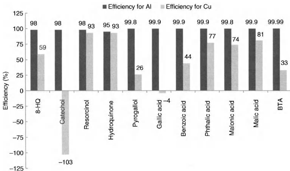
Figure 11.15. Corrosion inhibitor efficiency in a solvent mix of DMAC and water with choline hydroxide to raise the pH to about 11. Equimolar amounts of inhibitor were used for each test. Based on reference [11]. Used with permission of the author.
