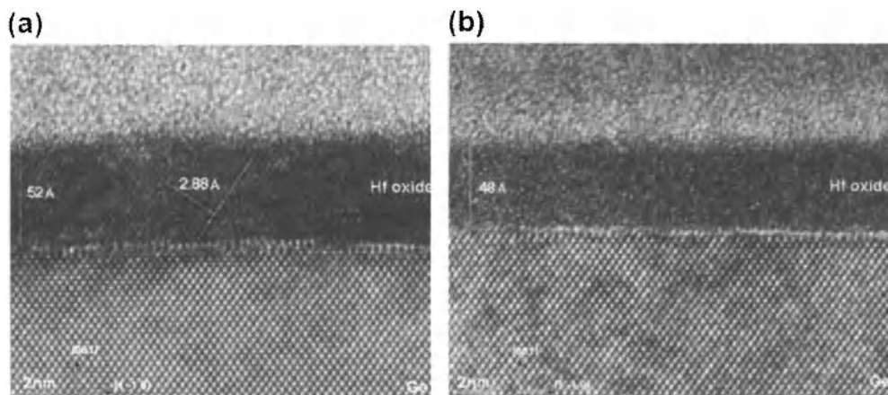
Figure 12.17. Transmission electron microscopy images of 5-nm \text{HfO}_2 deposited onto Ge by ALD after a) dilute HCl pre-clean and b) thermal oxynitridation in \text{NH}_3 at 600^\circ\text{C} [79]. Reprinted with permission from Gusev, E. P., Shang, H., Copel, M., Gribelyuk, M., D'Emic, Kozłowski, C. P., and Zabel, T., Appl. Phys. Lett. , 85(12):2334 (2004). Copyright 2004, American Institute of Physics.
