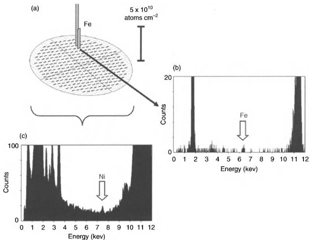
Figure 15.3. Result of the test of sweeping-TXRF for a 300-mm wafer, with uniform Ni and localized Fe contamination; (a) Fe is detected at a spot, (b) Fe-K \alpha peak can be seen at the spot, and (c) the accumulated spectra showed the presence of relatively uniform Ni at ca. 3 \times 10^9 atoms \text{cm}^{-2} [18]. Reprinted from Spectrochimica Acta Part B , Volume 59, Mori, Y., Uemura, K., Kohno, H., Yamagami, M., Yamada, T., Shimizu, K., Onizuka, Y., and Iizuka, Y., "Detection of unknown localized contamination on silicon wafer surface by sweeping total reflection X-ray fluorescence analysis", page 1277. Copyright (2004) with permission from Elsevier.
