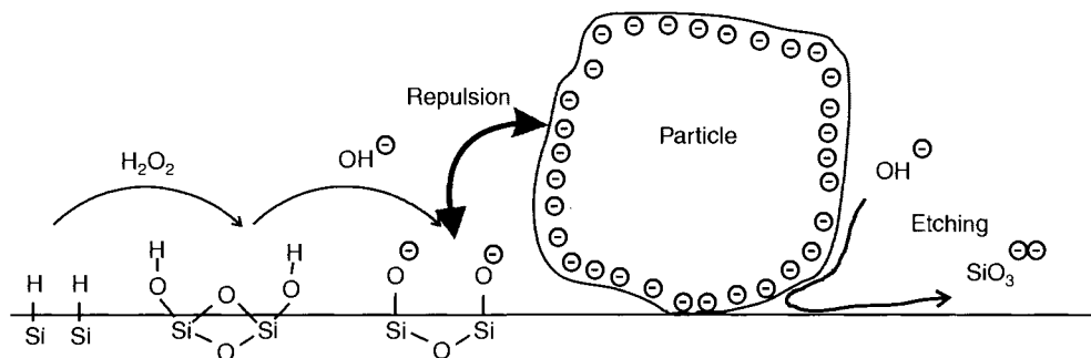
Figure 2.2. Schematic of the SC-1 cleaning mechanism. Silicon is oxidized by the hydrogen peroxide; accomplished by deprotonation of the silanol group, surface charging of particles, and undercutting particles by etching the silicon dioxide. Used with permission of the author.
