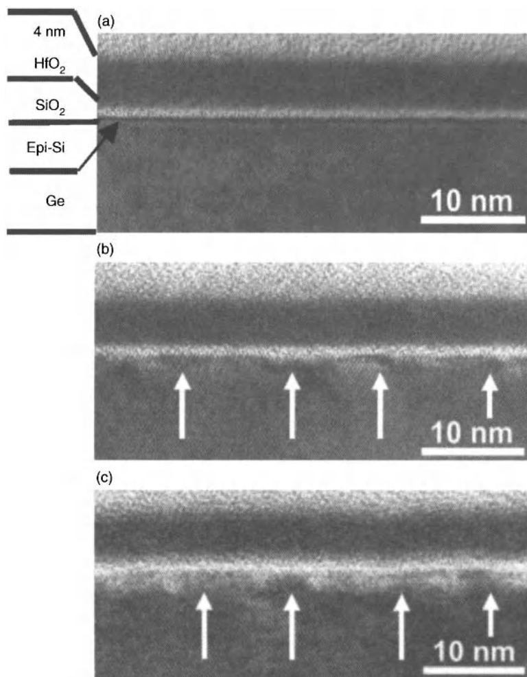
Figure 12.32. Transmission electron microscopy analysis of HfO 2 /Si/Ge gate stacks incorporating a) 4, b) 8, or c) 12 monolayers of Si, in a) the slightly darker interfacial layer is silicon while the brighter interfacial layer is SiO 2 . The arrows emphasize the periodicity of the contrast variations observed on the TEM images [125]. Reprinted from Microelectronic Engineering , Vol. 80, De Jaeger, B., Bonzom, R., Leys, F., Richard, O., Steenbergen, J. V., Winderickx, G., Van Moorhem, E., Raskin, G., Letertre, F., Billon, T., Meuris, M., and Heyns, M., "Optimization of a thin epitaxial Si layer as Ge passivation layer to demonstrate deep sub-micron n- and p-FETs on Ge-On-Insulator substrates", page 26. Copyright (2005) with permission from Elsevier.
