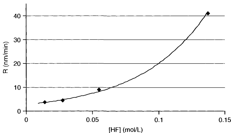
Figure 3.38. Silicon nitride etching rate in water at 125°C as a function of HF concentration [49]. Reprinted from MICRO Magazine , Copyright 2005, Tom Cheney, Los Angeles, CA. Used with permission.
