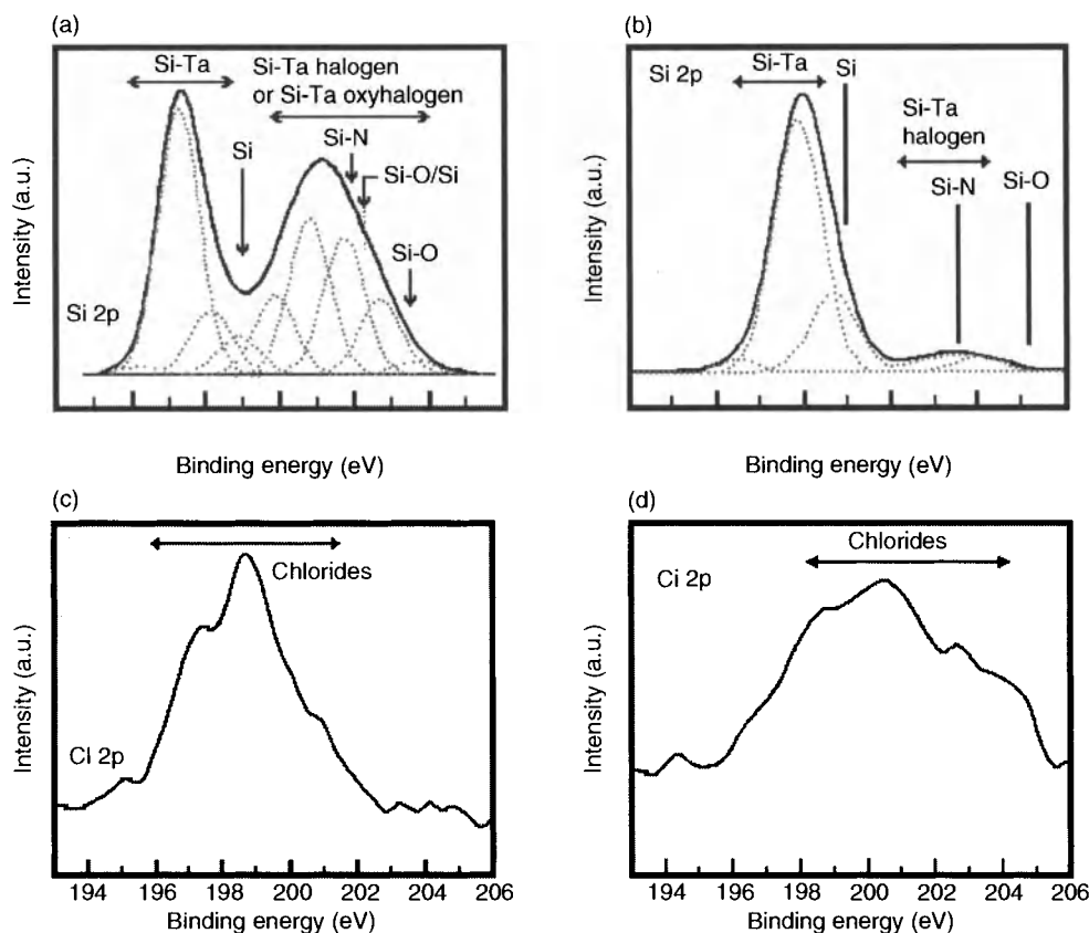
Figure 7.17. Angle resolved XPS spectra of the residue after etching TaN gate stack with \text{Cl}_2 -based plasma; a) is the top view of Si 2p spectrum, b) is the side view of Si 2p spectrum, c) is top view of Cl 2p spectrum, and d) is the side view of Cl 2p spectrum [154]. Reprinted from Studies in Surface Science and Catalysis , Vol. 159, Hwang, W. S., Ngu, H. H., Yoo, W. J., and Bliznetsov, V., "Chemical analysis of etching residues in metal gate stack for CMOS process", page 365. Copyright (2006) with permission from Elsevier.
