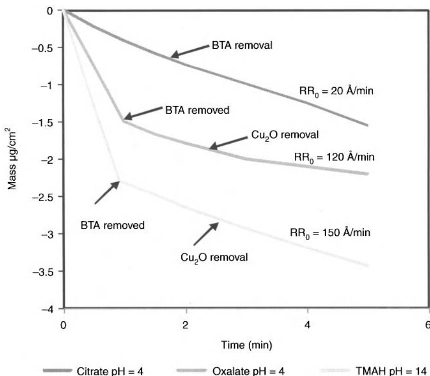
Figure 11.9. Quartz microbalance data for the removal of BTA with various solution. (a) Removal of BTA with citrate solution. The pH of the solution is increased with ammonium hydroxide. The time necessary to remove a 75-Å BTA film is more than 3 minutes. (b) Removal of BTA with oxalic acid solution. The pH of the solution is increased with ammonium hydroxide. The time necessary to remove a 75-Å BTA film is more than 1 minute. (c) Removal of a 150-Å thick BTA film with a dilute TMAH solution at pH = 14. This solution also removes the underlying cuprous oxide film. The graph is based on data from [46]. Used with permission from the author.
