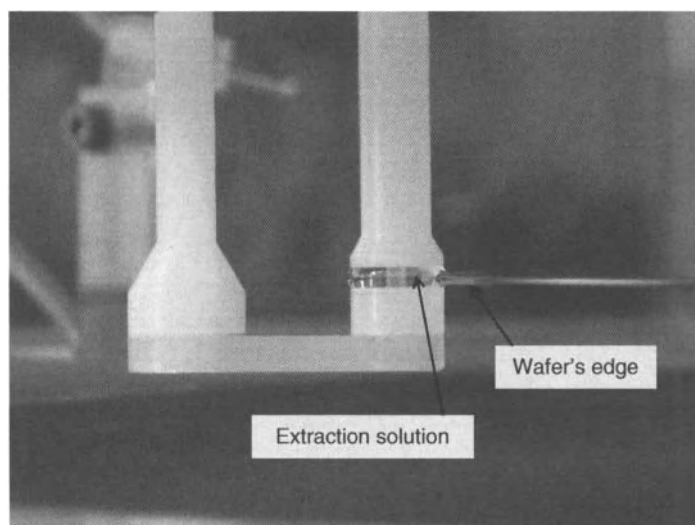
Figure 15.12. Automated bevel and edge analysis chemical extraction design from Technos International [24]. Used with permission from H. Takahara.
