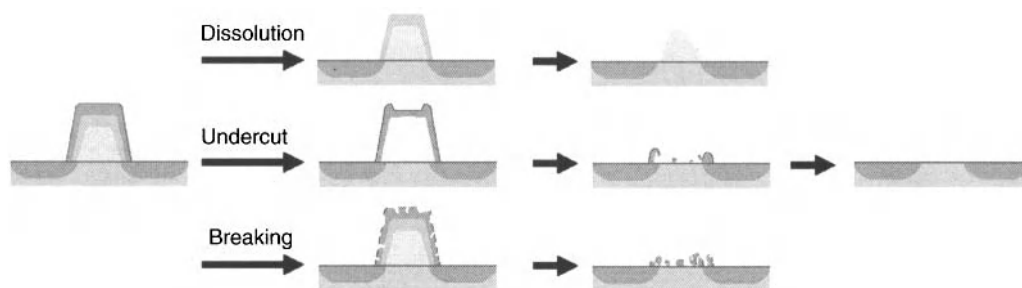
Figure 8.19. Example mechanisms for all-wet high dose implant stripping. Adapted from [71]. Used with permission of the authors.
