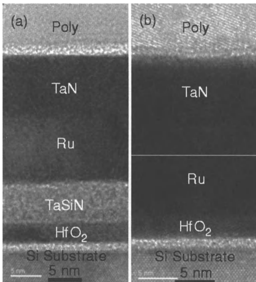
Figure 7.2. Cross section TEM images of dual metal gate a) NMOS and b) PMOS gate stacks structures from the same CMOS device [52]. Reproduced with permission of ECS – The Electrochemical Society from Zhang, Z., Song, S. C., Huffman, C., Hussain, M. M., Barnett, J., Moumen, N., Alshareef, H. N., Majhi, P., Sim, J. H., Bae, S. H., and Lee, B. H., Electrochemical and Solid State Letters .
