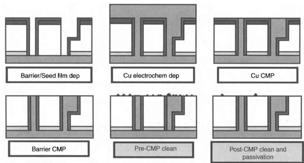
Figure 10.2. Cross section schematic of dual damascene with metal deposition and copper CMP with polishing of the etch-stop layer. Used with permission of the author.
