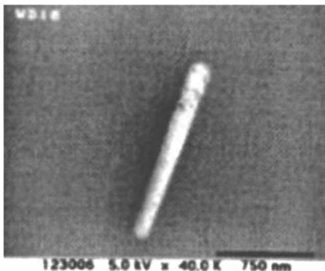
Figure 2.23. Sulfate crystal formed after SPM cleaning. Used with permission from A. L. P. Rontondaro.
