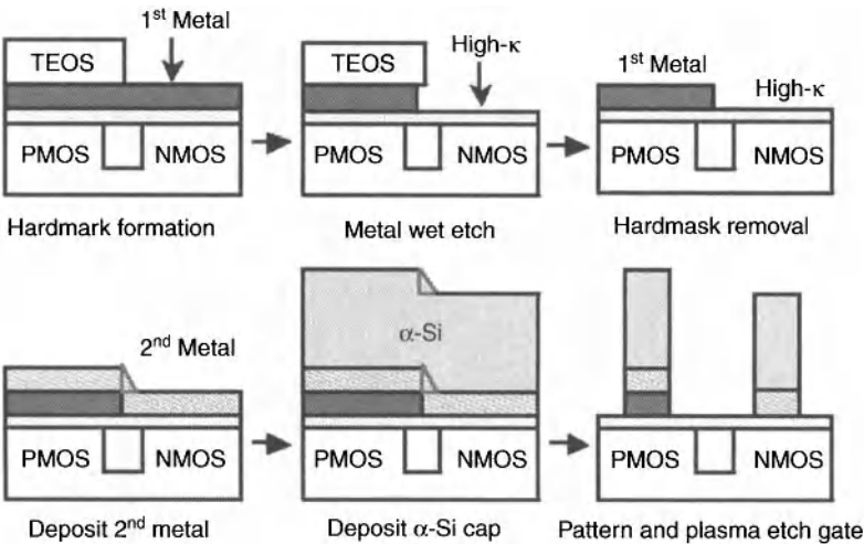
Figure 7.1. Schematic of the dual gate-first process flow using metal wet etch for removing the first metal layer (αSi is amorphous silicon) [52]. Reproduced with permission of ECS – The Electrochemical Society from Zhang, Z., Song, S. C., Huffman, C., Hussain, M. M., Barnett, J., Moumen, N., Alshareef, H. N., Majhi, P., Sim, J. H., Bae, S. H., and Lee, B. H., Electrochemical and Solid State Letters .
