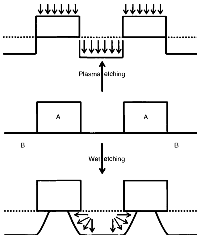
Figure 3.1. Difference between plasma etching (an isotropic) and wet etching (isotropic). A is the photoresist mask and B is the film to be etched. Used with permission of the author.
