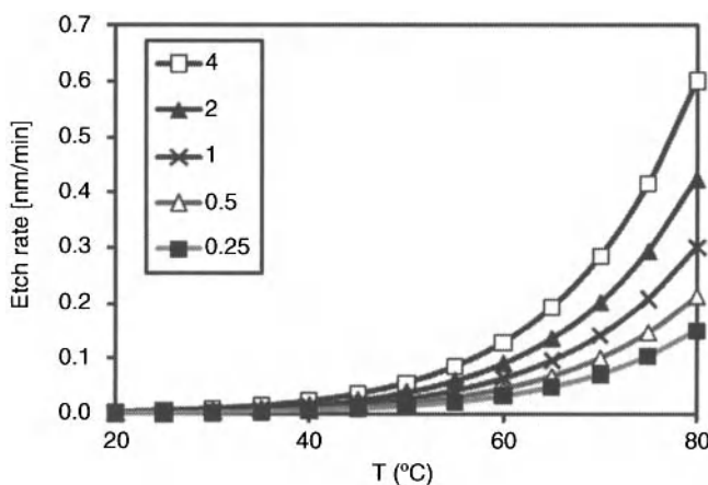
Figure 2.7. The \text{SiO}_2 -etching rate of APM as function of temperature and \text{NH}_4\text{OH}:\text{H}_2\text{O}_2 ratio. Used with permission of the author.
