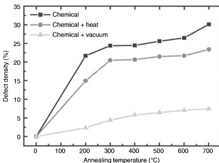
Figure 14.25. Interfacial defectivities as a function of post-bonding annealing temperatures for a (■) wet chemical surface preparation, (●) with an additional 300°C pre-bonding treatment, and (▲) for bonding under vacuum [131]. Reproduced with permission of ECS – The Electrochemical Society from Beneyton R., Fournel F., Morales C., Rieutord F. and Moriceau H., The Electrochemical Society Transactions .
