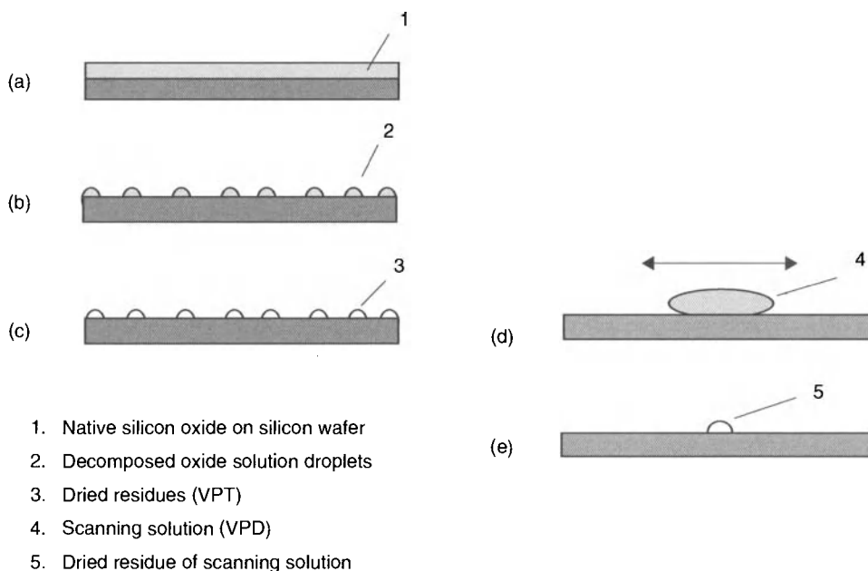
Figure 15.8. Flow schematic diagram of VPT-TXRF method compared with conventional VPD-TXRF method [44]:
