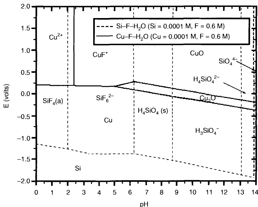
Figure 13.16. Pourbaix diagram of Cu-F-H 2 O system superimposed on that of Si-F-H 2 O system [49]. The shaded area emphasizes the redox potential lower than 0.2 V and in acidic F - conditions (pH < 6), where Cu metal formation is thermodynamically favorable. Used with permission of Srini Raghavan.
