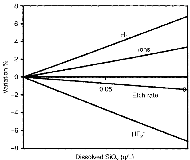
Figure 2.30. Model calculation: variation of some typical parameters in an ideal 2 wt% HF bath as a function of amount of etched SiO 2 . Used with permission of the author.
