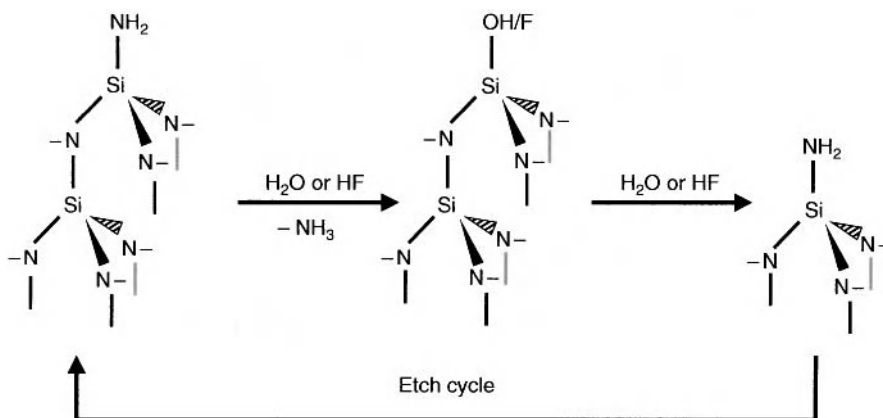
Figure 3.23. The continuous etch process of \text{Si}_3\text{N}_4 1) activating the top Si layer by replacing the \text{NH}_2 -group and 2) the removal of the activated-silicon layer. Used with permission of the author.
