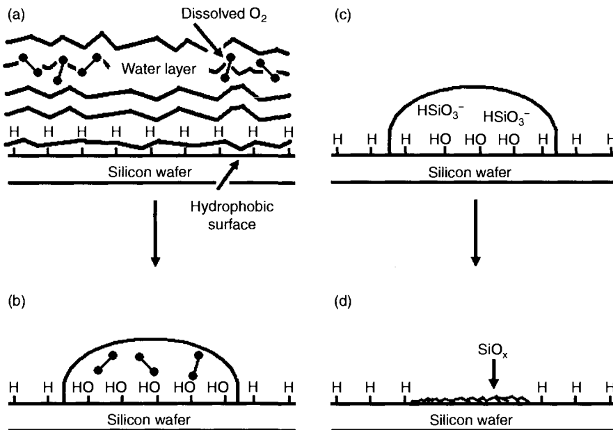
Figure 4.11. Schematic of the formation of watermarks on a hydrophobic surface by leaving spots of residual water; a) dissolution of O_2 in the rinsing water, b) causes oxidation of the silicon surface shown in the water droplet left on the wafer after drying c) that allows the dissolution of silica into the oxidized silicon into the water, and d) complete drying of the droplet and the formation of the watermark. Used with permission of the author.
