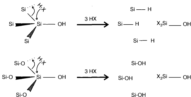
Figure 2.5. Similarity between etching of the \equiv\text{Si-OH} unit out of a Si or \text{SiO}_2 matrix, where \text{X} = \text{OH} or \text{F} . Used with permission of the author.
