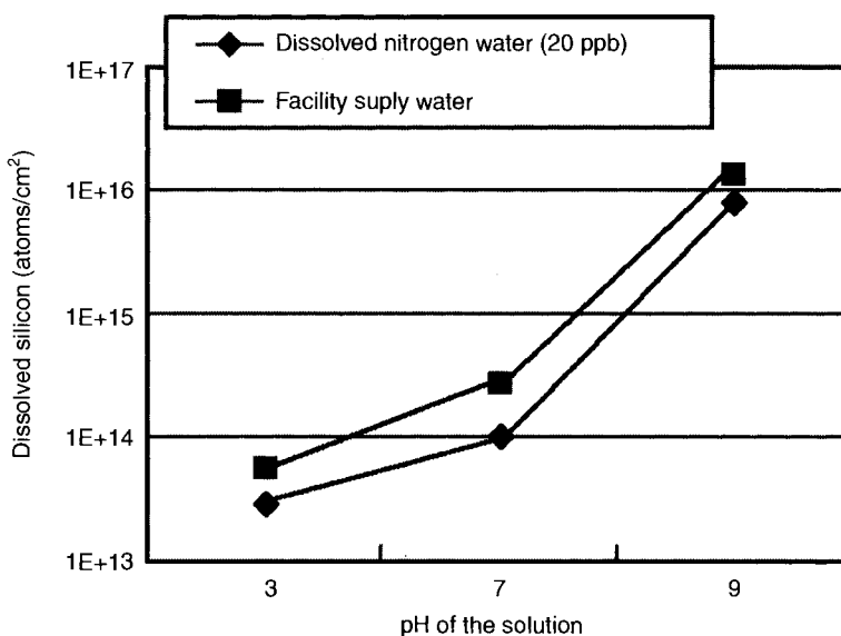
Figure 4.10. The solubility of silicon in water with respect to the pH and the gases dissolved in the water [49]. Used with permission from DNS.
