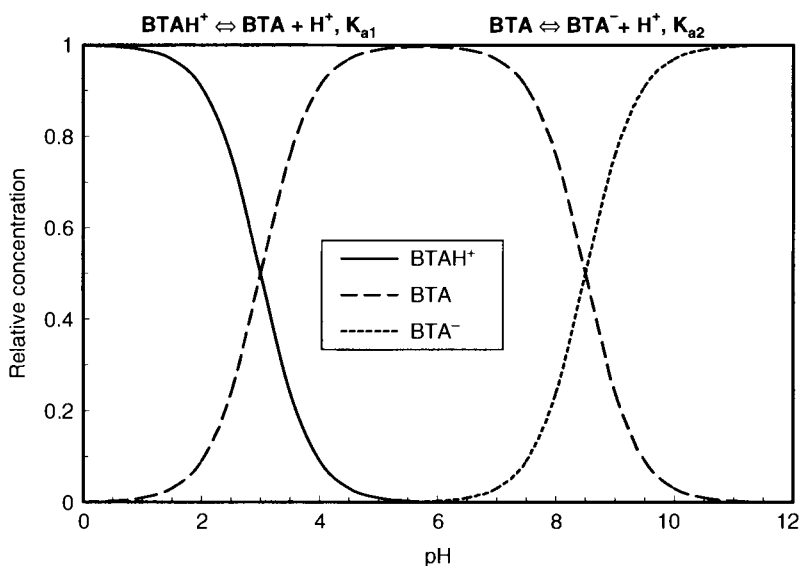
Figure 11.5. Benzotriazole species versus pH. The dominate species at pH values below \text{pK}_{a1} is \text{BTAH}^+ , above \text{pK}_{a2} , \text{BTA}^- is the dominate species, and between \text{pK}_{a1} and \text{pK}_{a2} , \text{BTA} is the dominate species. Used with permission from the author.
