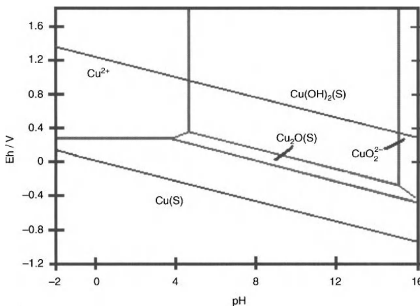
Figure 11.1. Pourbaix diagram for the Cu-H 2 O system [4]. Drawn with HSC Engineering software [5].
