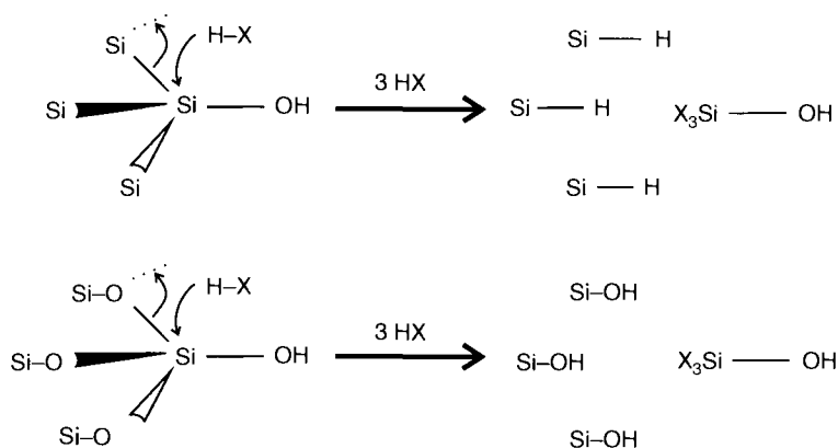
Figure 3.12. Similarity between etching of a Si-OH unit out of a Si or SiO 2 matrix: X - = F - or OH - . Used with permission of the author.
