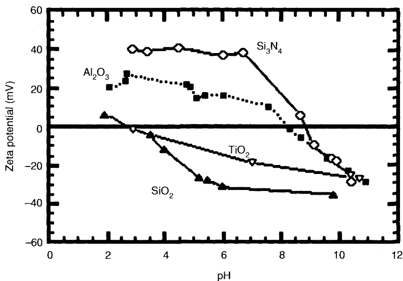
Figure 10.16. Zeta potential as a function of pH for various particles on a silicon wafer [132]. Reproduced with permission of ECS – The Electrochemical Society from Vos, R., Lux, M., Xu, K., Fyen, W., Kenis, K., Conard, T., Mertens, P. W., Heyns, M., Hatcher, Z., and Hoffman, M., The Journal of the Electrochemical Society .
