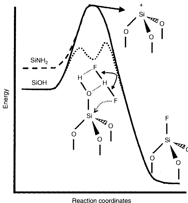
Figure 3.28. Proposed energy diagram of Si-N and Si-O bond breaking. Used with permission of the author.
