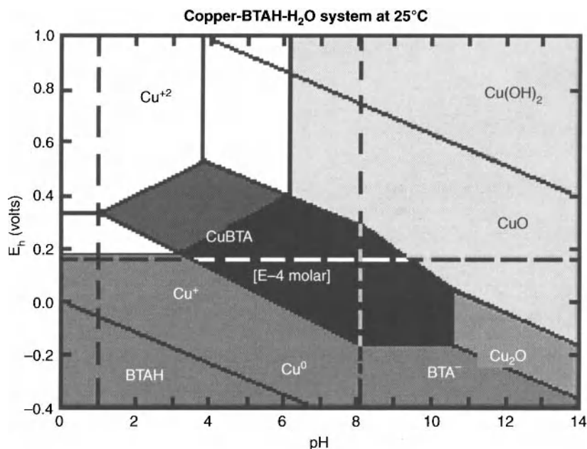
Figure 11.2. Stability diagram for the Cu-BTA-H 2 O system. Adapted from [6]. Reproduced with permission of ECS – The Electrochemical Society from Tromans, D. J. J., Journal of the Electrochemical Society .
