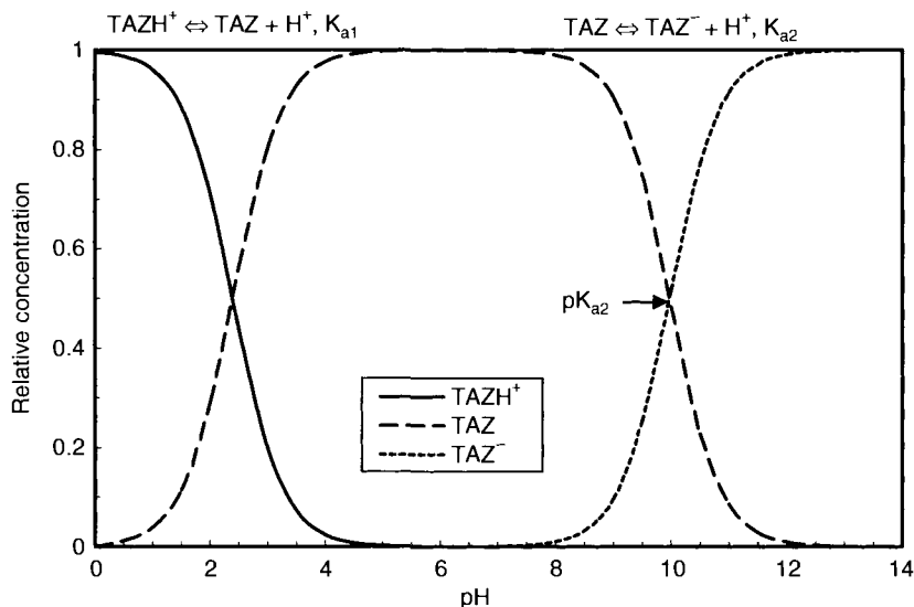
Figure 11.7. 1,2,4-triazole species versus pH. The dominant species below pK_{a1} is TAZH^+ , above pK_{a2} , TAZ^- is the dominant species, and between pK_{a1} and pK_{a2} , TAZ is the dominant species. Used with permission from the author.
