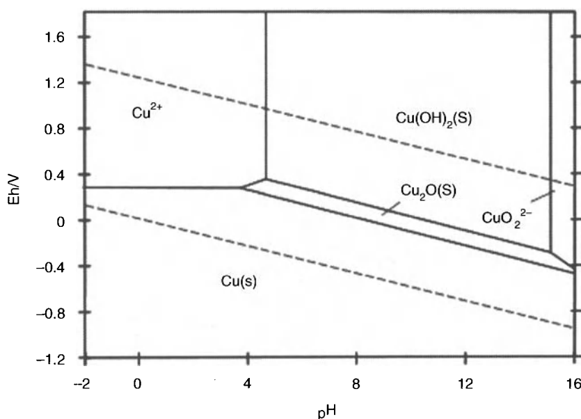
Figure 6.12. Pourbaix diagram for copper in water [22]. Drawn with HSC Engineering software [24].
