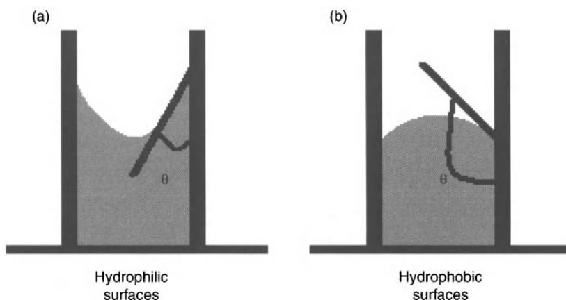
Figure 4.6. Depiction of a liquid droplet on a solid surface; a) hydrophilic surfaces with contact angle <90^\circ and b) hydrophobic surface with contact angle >90^\circ . The contact angle of the droplet is shown in relationship to the surface energies of the materials. Used with permission of the authors.
