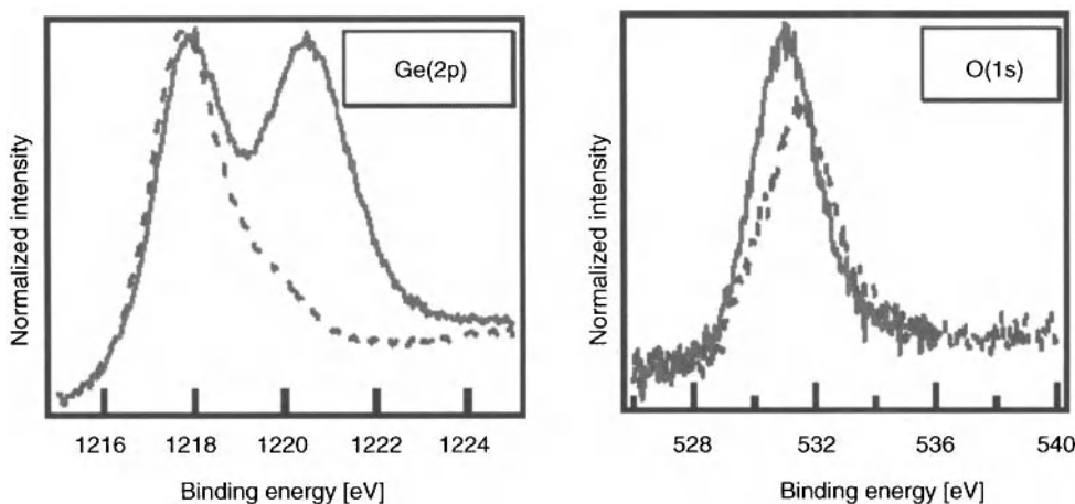
Figure 12.23. Ge2p 3/2 and O1s core level spectra of Ge(111) as received (solid line), and after HF/water etched (dashed line) using XPS [97]. Reprinted from Surface Science , Vol. 543(1-3), Bodlaki, D., Yamamoto, H., Waldeck, D. H., and Borguet, E., "Chemical Surface Passivation of Ge Nanowires", page 63. Copyright (2003) with permission from Elsevier.
