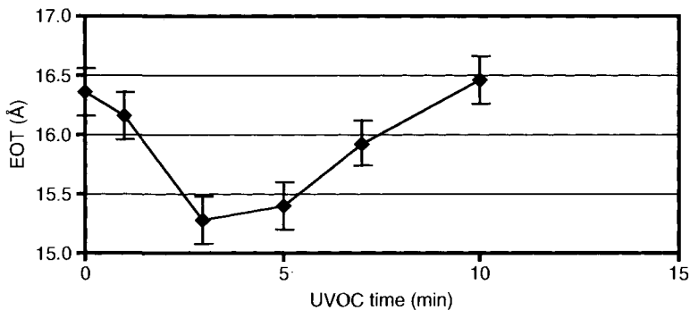
Figure 14.21. Cleaning efficiency is shown by the decrease of EOT upon exposure to UV/O 3 (UVOC) for up to 4 min. Over 4 min room temperature, oxidation occurs indicated by an increase of EOT. Reproduced with permission of CEA-LETI.
