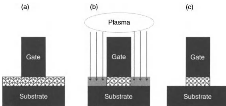
Figure 7.16. Schematic of combined dry and wet removal; a) the initial gate stack illustrating the crystalline high- \kappa film, b) after plasma removal damages the high- \kappa , and c) after the wet process step that completely removes the damaged high- \kappa . Used with permission from Shamiryan.
