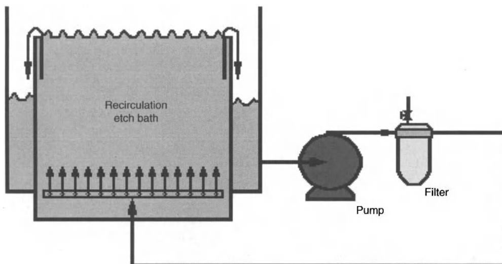
Figure 6.5. Schematic of a recirculating etch bath. Used with permission from CT Associates, Inc.
