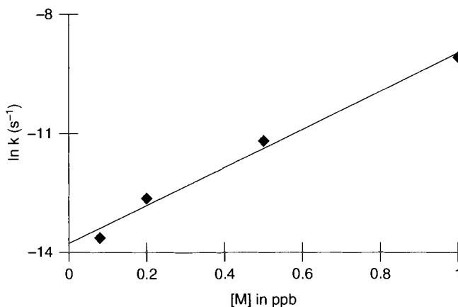
Figure 2.9. The ratio rate constant ( k ) of the catalytic decomposition of peroxide in APM as a function of iron concentration [28]. Reproduced with permission of ECS – The Electrochemical Society from Knotter, D. M., Gendt, S. D., Baeyens, M., Mertens, P. W., and Heyns, M. M., Journal of the Electrochemical Society .
