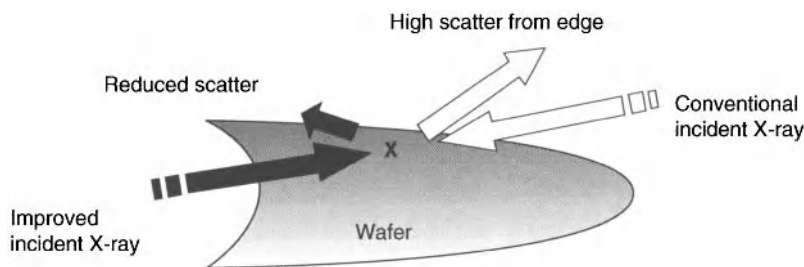
Figure 15.5. Example of edge contamination detection by TXRF [24]. Used with permission from H. Takahara.
