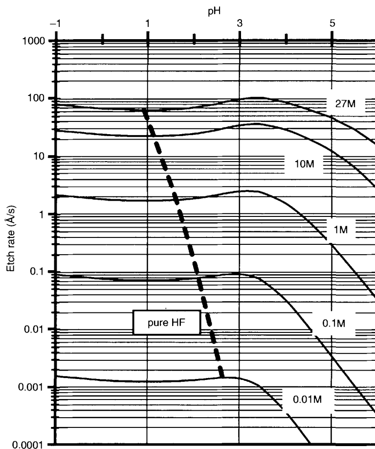
Figure 3.10. Etching rate of thermally grown \text{SiO}_2 in HF solutions with different total fluoride concentrations, data from reference [11]. Used with permission of the author.
