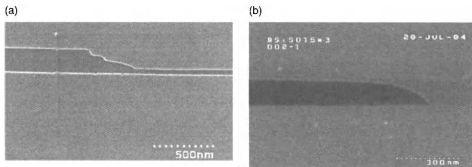
Figure 14.5. Scanning electron microscope images of a) a PSOI structure containing both ~35-nm thin and 200-nm thick Box areas and b) a PSOI structure with a 150-nm thick Box area and direct Si-Si bonded area [33]. Reproduced with permission of IEEE from Moriceau, H., Yalicheff, C., Gorla, C., Charvet, A. M., Morales, C., Zussy, M., Dechamp, J., Kernevez, N., Letertre, F., Ghyselen, B., Proceedings IEEE SOI Conference . © 2004 IEEE.
