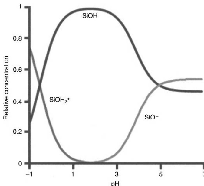
Figure 3.5. Relative concentrations of \text{SiO}^- , \text{SiOH} , and \text{SiOH}_2^+ on a \text{SiO}_2 surface in water. Based on kinetic parameters in reference [11]. Reprinted with permission from Knotter, D. M., J. Am. Chem. Soc. , 122(18):4345. Copyright 2000 American Chemical Society.
