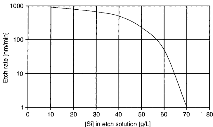
Figure 3.22. Etching rate of Al in 20 wt% TMAH (90°C) as a function of silicon concentration [43]. Used with permission of A. A. M. van de Vorst (NXP).
