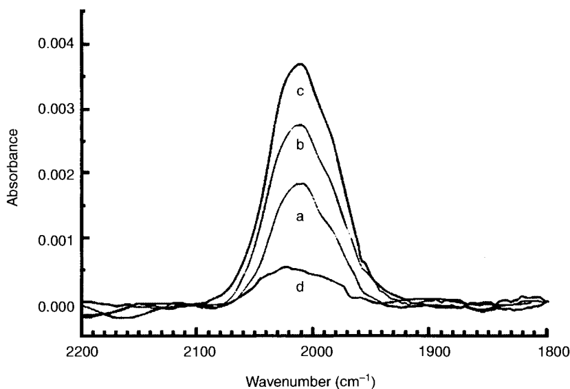
Figure 12.24. Attenuated total reflection (ATR)-FTIR spectra of the v(GeH x ) stretching region for the hydrogen-terminated Ge(100) surface prepared by etching with an aqueous 10 wt% HF solution: after a) 2 min, b) 5 min, c) 10 min, d) 15 min [97]. Reprinted from Surface Science , Vol. 543(1-3), Bodlaki, D., Yamamoto, H., Waldeck, D. H., and Borguet, E., "Chemical Surface Passivation of Ge Nanowires", page 63. Copyright (2003) with permission from Elsevier.
