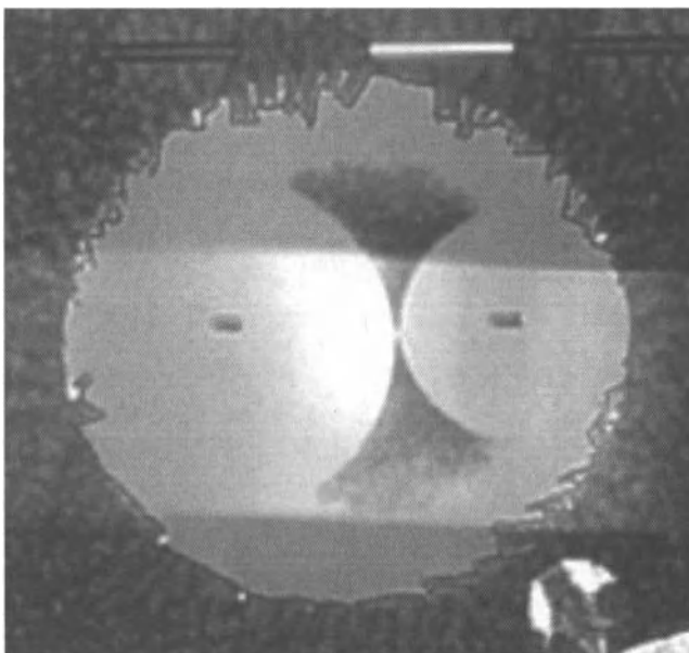
Figure 8.27. Close-up of an impact area of the cryoaerosol particle showing crust removal [101]. Reproduced with permission of ECS – The Electrochemical Society from Totir, G. G., Frank, M. M., Vos, R., Arnauts, S., Bearda, T., Kenis, K., Delande, M., Le, Q. T., Kesters, E., Vereecke, G., Mannaert, G., Lux, M., Hofliijk, I., Conard, T., Banerjee, S., Malhouitre, S., Leunissen, P. and Mertens, P. W., ECS Transactions .
