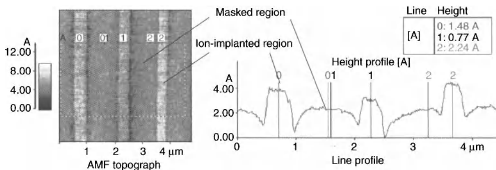
Figure 8.25. Atomic force microscope topographic image and line profile of the surface after photoresist stripping with co-solvent/chelator in \text{SCCO}_2 [96]. Reproduced with permission of ECS – The Electrochemical Society from Saga, K., Kuniyasu, H., Hattori, T., Korzenski, M. B., Visintin, P. M., and Baum, T. H., ECS Transactions .
