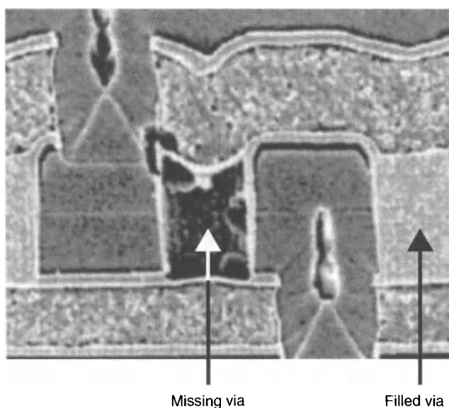
Figure 5.2. A scanning electron microscope image cross section of a hydroxylamine formulation-cleaned via with a missing metal in the via [34]. Reproduced with permission of ECS – The Electrochemical Society from Florence, D., Williams, B., Belisle, C., Hatcher, C., and Prasad, J., Electrochemical Society Transactions .
