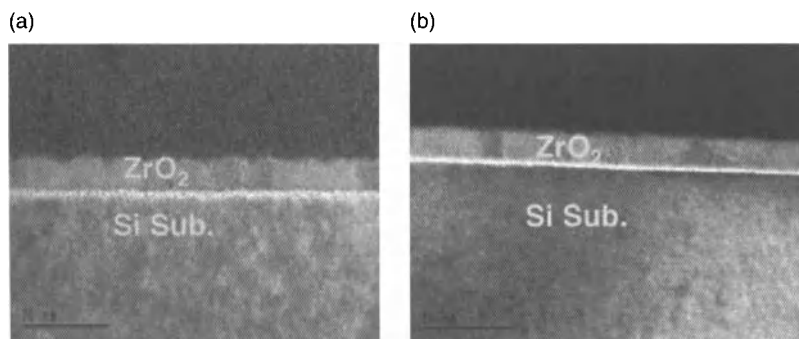
Figure 7.9. Transmission electron microscope images of interfacial oxide layer cleaned with a) SC-1/SC-2 and b) O_3 , followed by a 600°C NH_3 anneal [66]. Used with permission of Future Fab International .
