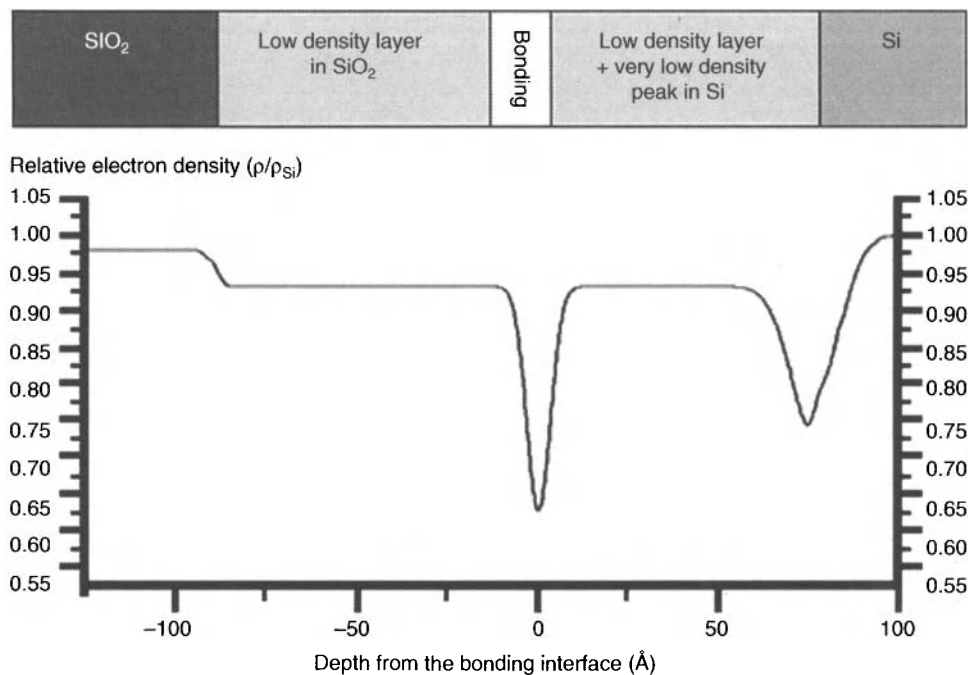
Figure 14.19. Low electron density layers evidenced by x-ray reflectivity measurements [95]. Reproduced with permission of ECS – The Electrochemical Society - from Moriceau, H., Bataillou, B., Morales, C., Cartier, A. M., and Rieutord, F., Semiconductor Wafer Bonding : Science, Technology, and Applications VII .
