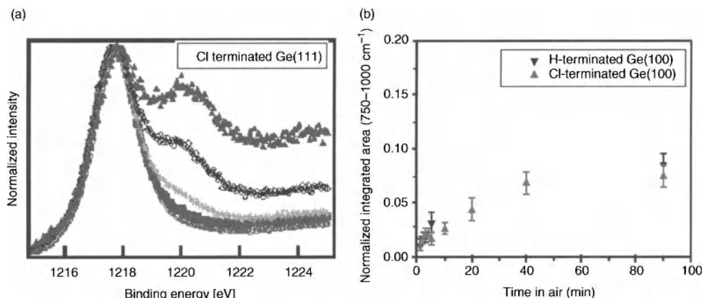
Figure 12.29. a) Ge2p core level spectra of the oxidation of Cl-terminated Ge(111) immediately after preparation (o), after 1 hr (■), after 1 day (+), after 1 week (◇) after 1 month (▲) air exposure [97]. Reprinted from Surface Science , 543(1-3) and Bodlaki, D., Yamamoto, H., Waldeck, D. H., and Borguet, E., "Ambient stability of chemically passivated germanium interfaces", page 63. Copyright (2003) with permission from Elsevier. b) Variation of the integrated area for the increase of GeO x /CH x modes as a function of the passivated Ge(100) surface exposed to air for H- and Cl-terminated Ge(100) surfaces [62] Used with permission from Material Research Society, reprinted from Rivillon-Amy, S., Chabal, Y.J., Amy, F., Kahn, A., Krugg, C., and Kirsch, P., Wet Chemical Cleaning of Germanium Surfaces for Growth of High-k Dielectrics , Vol. 917: (Jammy, R., Shanware, A., Misra, V., Tsunashima, Y., and De Gendt, S., eds.) San Francisco (2006) page E01–05.
