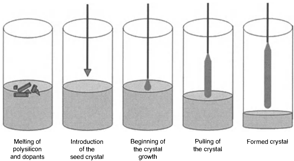
Figure 13.2. A schematic showing the silicon crystal growing process for wafer production. Used with permission of the authors.
