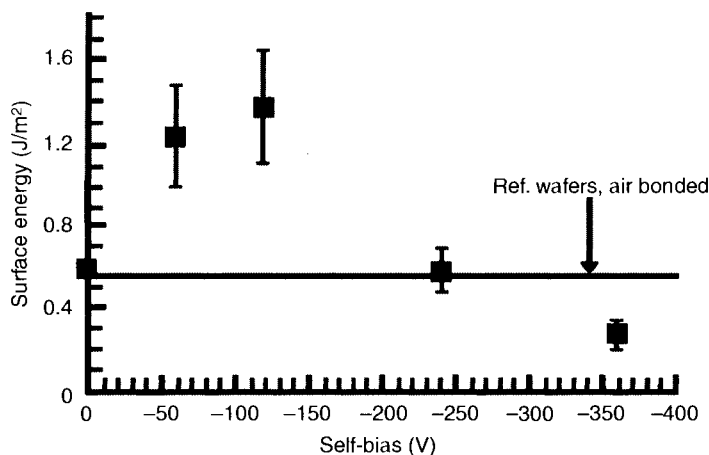
Figure 14.14. Surface energy as a function of self-bias voltage of silicon wafers bonded after RIE oxygen plasma activation for 5 min at 56 mTorr and 30 sccm O_2 and annealing for 2 hr at 200°C [91]. Reprinted from Sensors & Actuators A , 82(1–3) and Pasquariello, D., Lindeberg, M., Hedlund, C., and Hjort, K., "Surface energy as a function of self-bias voltage in oxygen plasma wafer bonding", page 239. Copyright (2000) with permission from Elsevier.
