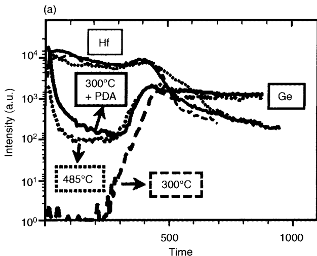
Figure 12.27. Time-of-flight secondary ion mass spectroscopy (TOF-SIMS) depth profiles for \text{HfO}_2 layers deposited onto HF-cleaned Ge(100) at 300°C (without or with post-deposition anneal, PDA, at 550°C), or at 485°C [81]. Reprinted with permission from Elshocht, S. V., Brijs, B., Caymax, M., Conard, T., Chiarella, T., De Gendt, S., De Jaeger, B., Kubicek, S., Meuris, M., Onsia, B., Richard, O., Teerlinck, I., Steenberg, J. V., Zhao, C., and Heyns, M. Appl. Phys. Lett. , 85(17):3824 (2004). Copyright 2004, American Institute of Physics.
