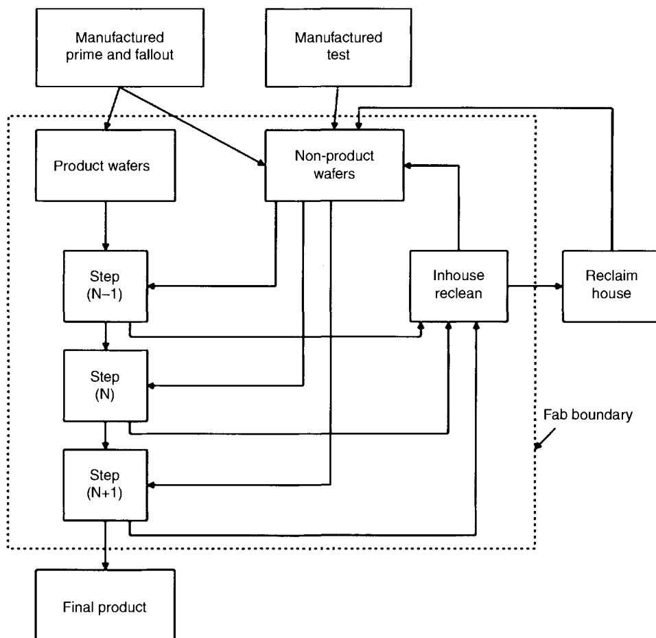
Figure 13.4. Schematic flow of wafers through a typical semiconductor fab. Adapted from [10]. Used with permission of Sage Concepts.
