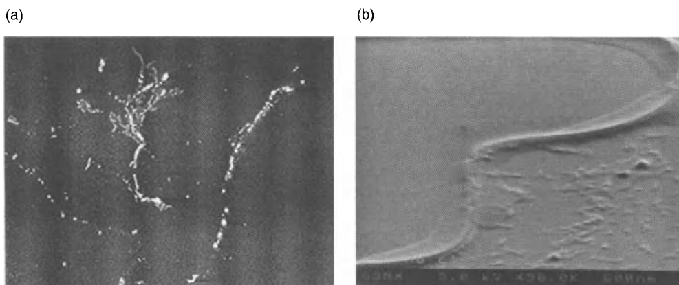
Figure 8.11. Examples of residues after stripping and cleaning. (a) Micrograph of post-O 2 plasma sputtered residue [19]. Reprinted from MICRO . Copyright Tom Cheyney, Los Angeles, CA. Used with permission. (b) SEM of post-O 2 plasma resist strip residue, showing delineation at edge of lithography feature. Used with permission of Novellus Systems.
