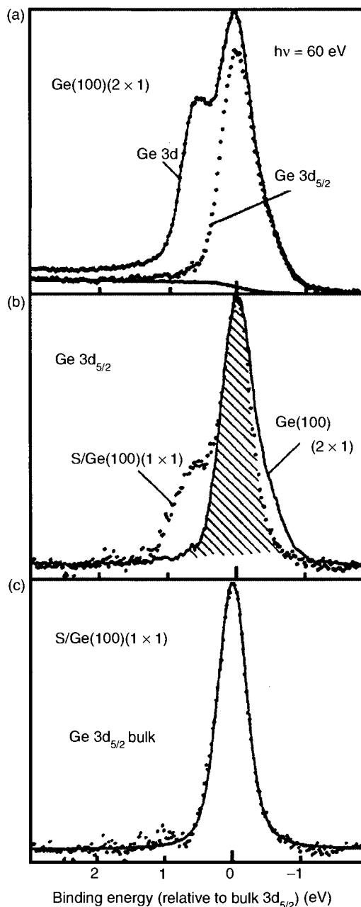
Figure 12.30. Ge3d core level photoemission spectra for clean and sulfur-covered Ge(100) surfaces. a) spin orbit splitting and secondary electron background, b) determination of bulk emission, c) surface-bulk deconvolution for S/Ge(100) 1×1 [112]. Reprinted figure with permission from Weser, T., Bogen, A., Konrad, B., Schnell, R. D., Schug, C. A., and Steinmann, W., Phys. Rev. , B35(15):8184 (1987). Copyright 1987 by the American Physical Society.
