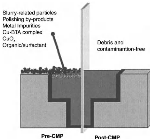
Figure 10.13. Schematic of the wafer surface before and after post-CMP cleaning showing issues related to polishing and the final surface. Courtesy of DuPont/EKC Technology (2010).
