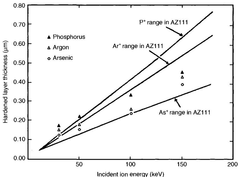
Figure 8.5. Plot of the thickness of the carbonized crust layer as a function of the ion energy for various implants. The photoresist is AZ@111 manufactured by AZ Electronics Materials. The lines are the calculated maximum thickness of the crust layers, the actual averages are designated by the symbols [8]. Reprinted from Nuclear Instruments and Methods in Physics Research , B7/8, Orvek, K., and Huffman, C., "Carbonized Layer Formation in Ion Implanted Photoresist Masks", page 501. Copyright (1985) with permission from Elsevier.
