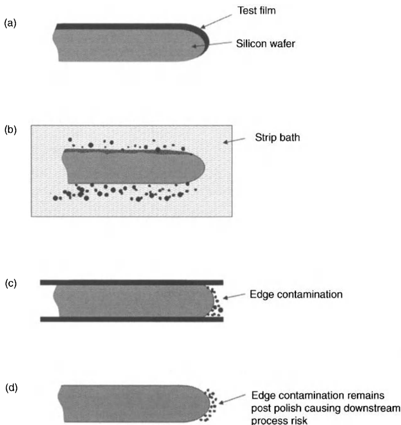
Figure 13.8. Depiction of edge contamination: (a) test wafer prior to the reclaim process, (b) the immersion in a chemical stripping bath to remove the material on the wafer surface, (c) double-side polishing of the wafer to remove surface damage, and (d) the wafer post-reclaim with edge contamination. Used with permission of the authors.
