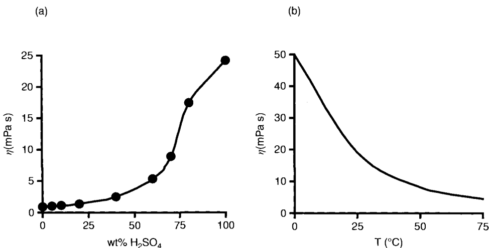
Figure 2.25. Viscosity ( \eta ) of \text{H}_2\text{SO}_4 at a) 25°C and b) of 95 wt% \text{H}_2\text{SO}_4 at various temperatures. Data points selected from reference [72]. Used with permission of the author.
