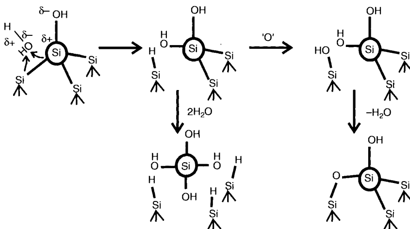
Figure 2.6. Etching of a monolayer of Si-OH by water and, alternatively, formation of a silicon dioxide layer. Used with permission from the author.
