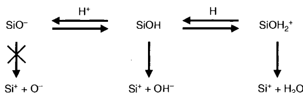
Figure 3.4. Acid/base equilibrium of the amphoteric surface silanol group. Used with permission of the author.
