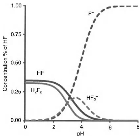
Figure 2.28. Concentration of F-containing species as function of pH in 2 wt% HF (note that pH of pure 2 wt% HF is 1.6). Used with permission of the author.
