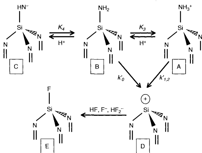
Figure 3.24. The rate limiting reaction step in the etching of Si 3 N 4 showing terminated Si groups reference [47]. Reproduced with permission of ECS – The Electrochemical Society from Knotter, D. M. and Denteneer, T. J. J., Journal of the Electrochemical Society .
