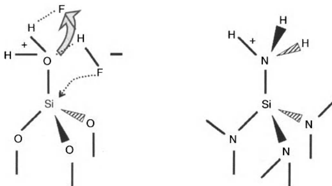
Figure 3.27. In contrast to \text{Si-NH}_3^+ , the \text{Si-OH} or \text{Si-OH}_2^+ group has a free electron pair on the O atom to aid with the addition of \text{HF}_2^- [47]. Reproduced with permission of ECS – The Electrochemical Society from Knotter, D. M. and Denteneer, T. J. J., Journal of the Electrochemical Society .
