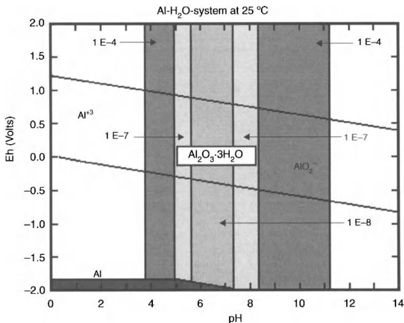
Figure 9.5. Pourbaix diagram of aluminum-water system. The solid lines represent the regime of stable water; the solid lines represent the solubilities of the species. Courtesy of Robert Small, RS Associates.
