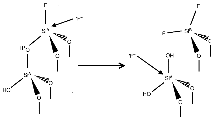
Figure 3.11. Etching of non-stoichiometric \text{SiO}_4 -unit [11]. Reprinted with permission from Knotter, D. M., J. Am. Chem. Soc. , 122(18):4345. Copyright 2000 American Chemical Society.
