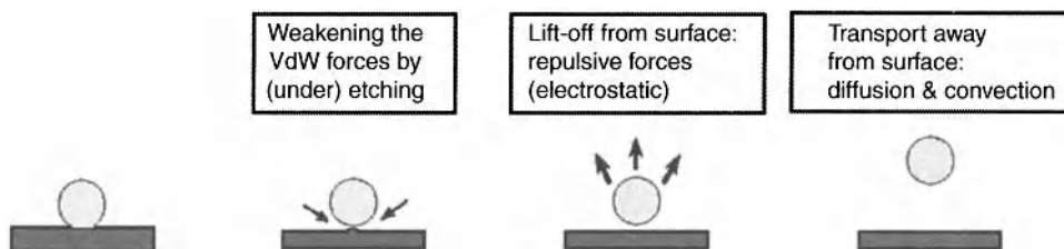
Figure 10.15. Schematic of the particle lift-off mechanism [132]. Adapted with permission of ECS – The Electrochemical Society from Vos, R., Lux, M., Xu, K., Fyen, W., Kenis, K., Conard, T., Mertens, P. W., Heyns, M., Hatcher, Z., and Hoffman, M., The Journal of the Electrochemical Society .
