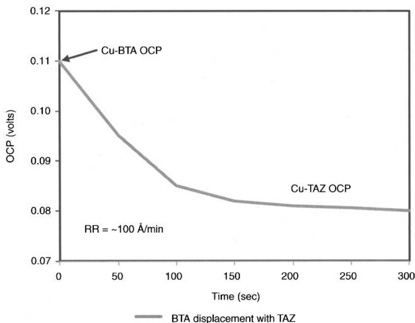
Figure 11.11. Open circuit potential measurements over time showing the displacement of a 200-Å thick BTA film by a 20-Å thick TAZ film. The BTA removal rate was about 100 Å/min. The graph is based on data from [46]. Used with permission from the author.
