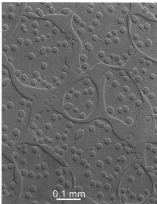
Figure 2.11. Micrograph of a hydrophobic silicon surface exposed to APM (70°C) vapor for 15 sec showing pattern etching. Experiment conducted and photo taken by L. Winters, NXP Semiconductors [36]. Used with permission of Léon Winters (NXP).
