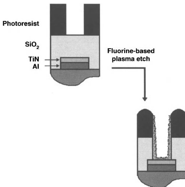
Figure 9.6. Schematic of a) Al via etching and b) residue creation. Used with permission of the author.
