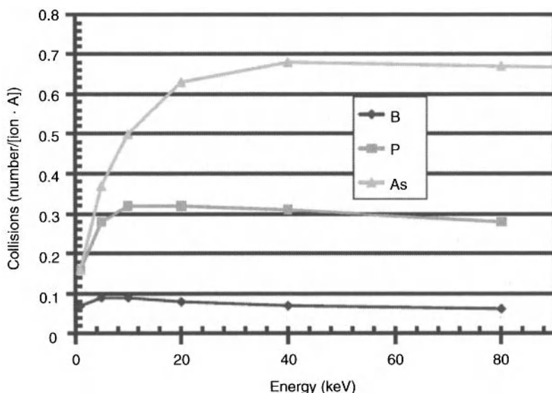
Figure 8.9. The peak level of collision events as a function of ion energy and implanted species [15]. Reproduced with permission of ECS – The Electrochemical Society from Christenson, K., ECS Transactions .
