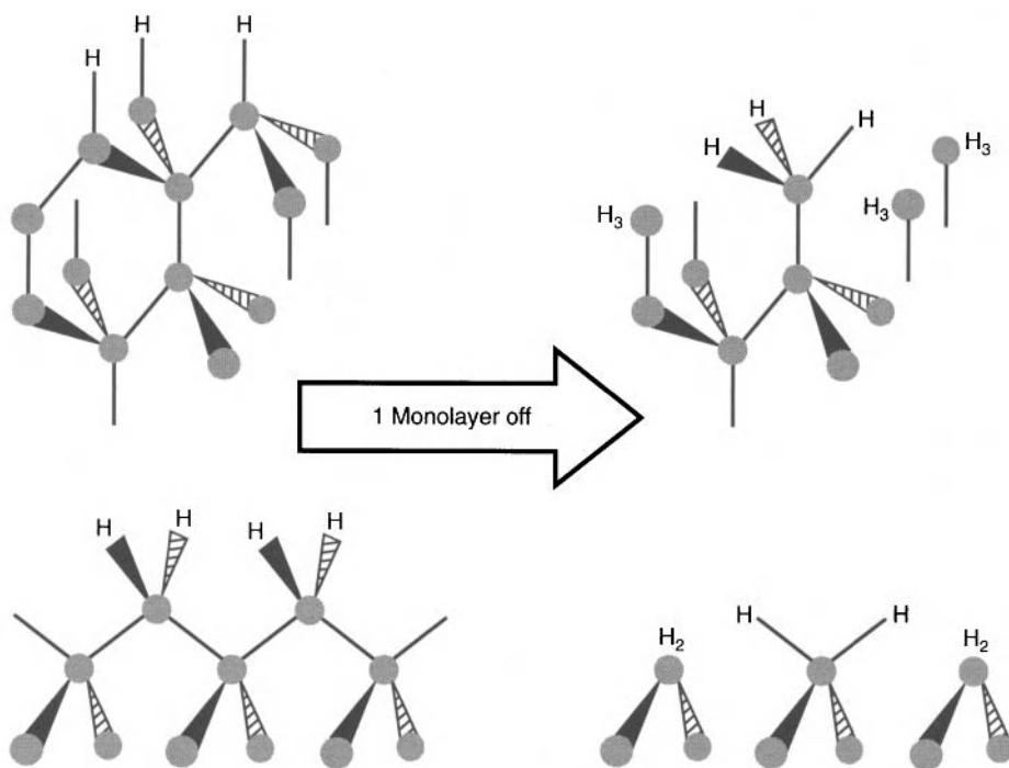
Figure 3.17. Etching of the surface layer of silicon: top is \text{Si } \langle 111 \rangle and bottom is \langle 100 \rangle or \langle 110 \rangle . Used with permission of the author.
