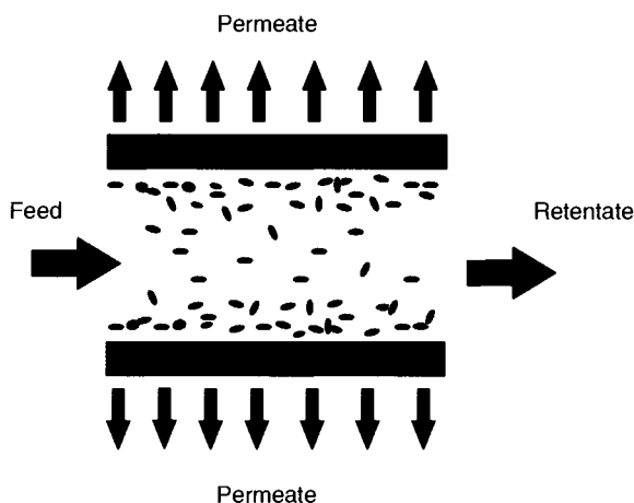
Figure 6.18. Cross flow designed filter. Used with permission from Pall Corporation.
