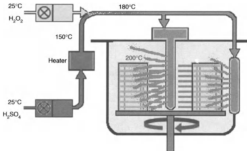
Figure 8.20. Example of a batch spin spray processor for high dose implant stripping showing the chemical being pre-heated [72]. Courtesy of FSI International.
