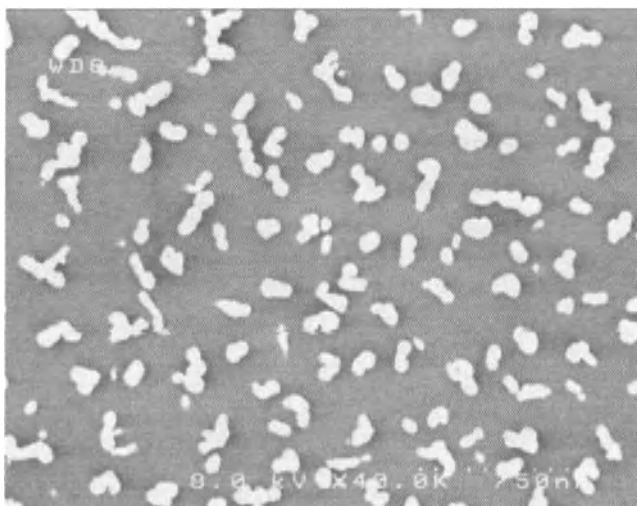
Figure 8.29. Cluster residue shown after the plasma stripping step. The clusters are swept away with the cryoaerosol [100]. Used with permission from NanoClean Technology Inc.
