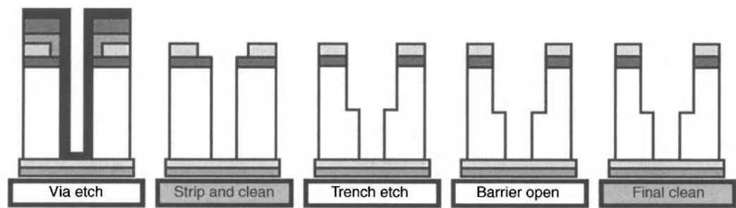
Figure 10.1. Cross section schematics of dual damascene of via etch, trench etch, and barrier etch with the strip process flow for a metal hard mask process. Used with permission of the author.
