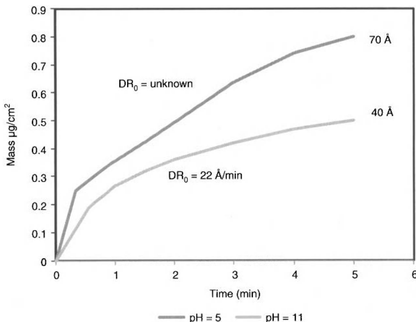
Figure 11.6. Benzotriazole film deposition kinetics on Cu at pH = 5 and 11 determined using a quartz microbalance in an electrochemical cell. The solution consisted of 1000 ppm of BTA in water. \text{DR}_0 is the deposition rate. The graph is based on data from [46]. Used with permission from the author.
