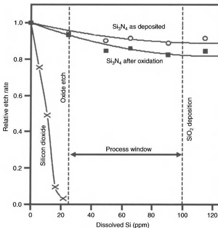
Figure 3.35. Relative etching rate variation in \text{H}_3\text{PO}_4 at 160^\circ\text{C} for LPCVD \text{Si}_3\text{N}_4 and thermally grown \text{SiO}_2 [66]. Used with permission of the author. Used with permission of S. van der Loo, (NXP).
