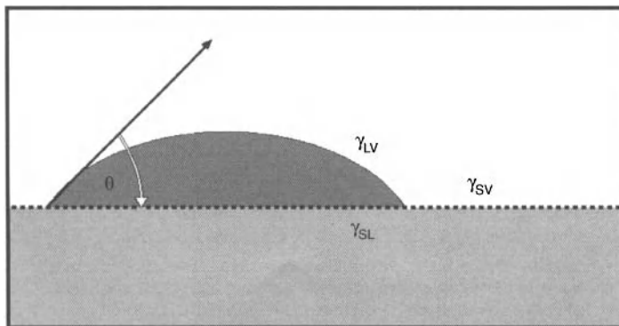
Figure 4.5. Depiction of a liquid droplet on a solid surface. The contact angle of the droplet is shown in relationship to the surface energies of the materials. Used with permission of the authors.
