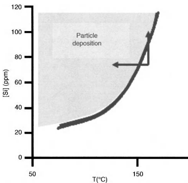
Figure 3.34. Saturation concentration of silica in boiling \text{H}_3\text{PO}_4 [64]. The etching rates of \text{SiO}_2 depend on the amount of dissolved silicates relative to the saturation level of dissolved silica [65]. Compiled and used with permission of the author.
