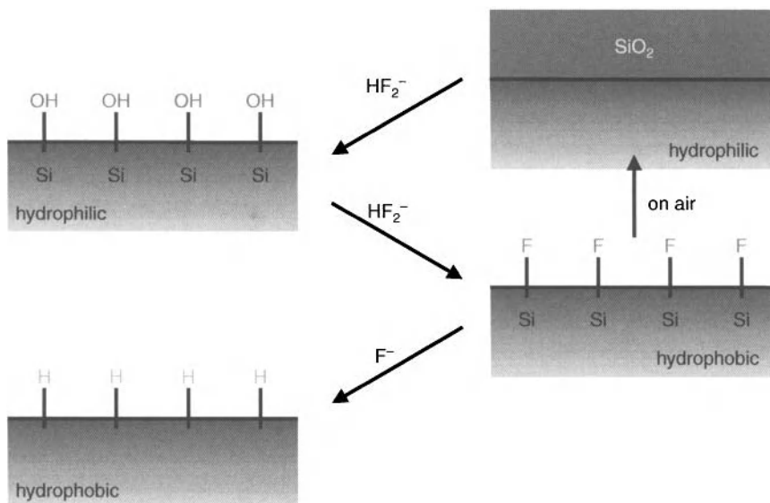
Figure 2.26. The three reaction steps to convert a silicon surface with a silicon dioxide layer to a hydrogen-terminated surface. Used with permission of the author.
