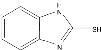
Figure 11.17. Structure of 2-mercaptobenzimidazole (2-MBI). Passivation film formation can occur through both nitrogen atoms and the sulfur atom. Both protons are acidic and can be removed at high pH; 2-MBI is not stable under acidic conditions.
