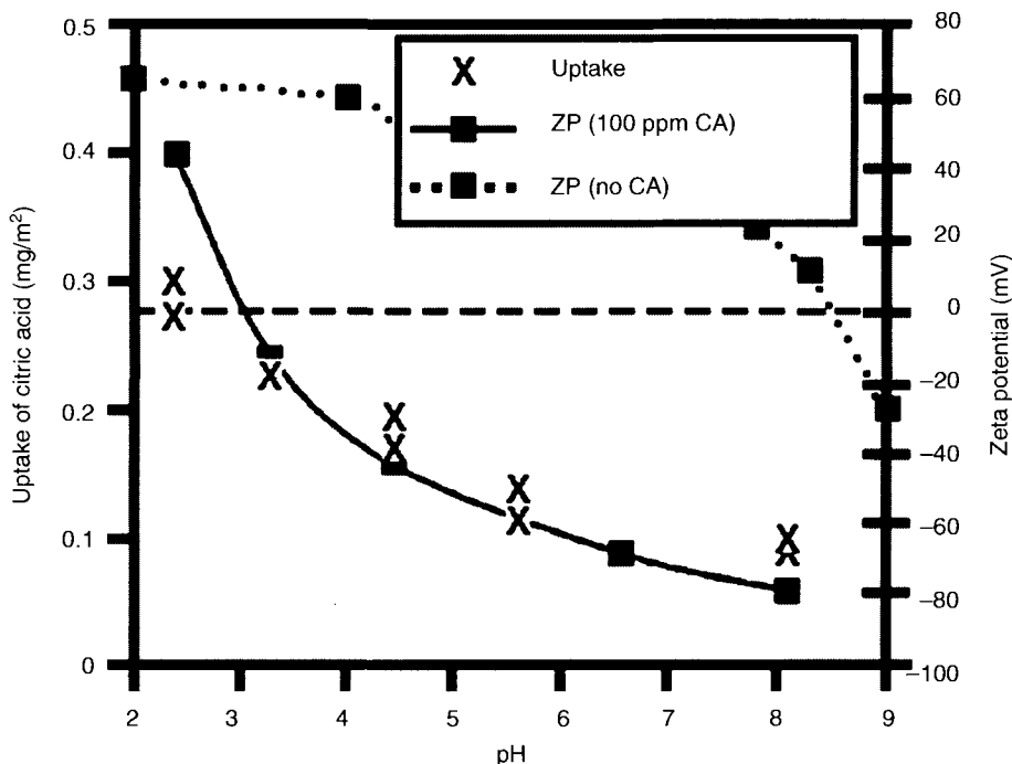
Figure 10.17. Zeta potential as a function of pH and specific adsorption for citric acid [138]. Reproduced with permission of ECS – The Electrochemical Society from Zhang, L., Raghavan, S., Meikle, S., and Hudson, G., Journal of the Electrochemical Society .
