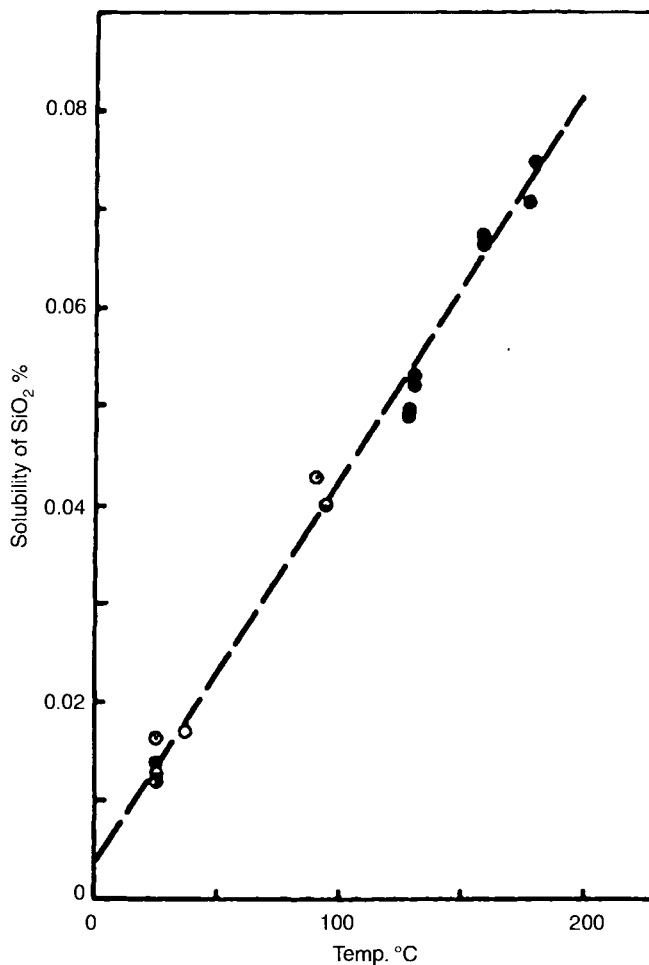
Figure 4.9. The solubility of amorphous silica, wt%, in neutral pH water at atmospheric pressure for various temperatures [39]. Reprinted with permission from Alexander, G. B., Heston, W. M., and Iler, R. K., Journal of Physical Chemistry , 58(6):453. Copyright 1954 American Chemical Society.
