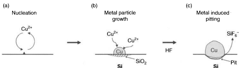
Figure 13.14. The mechanism of MIP in Cu/HF systems [43]. Reproduced with permission of ECS – The Electrochemical Society from Morinaga, H., Suyama, M., and Ohmi, T., Journal of The Electrochemical Society .
