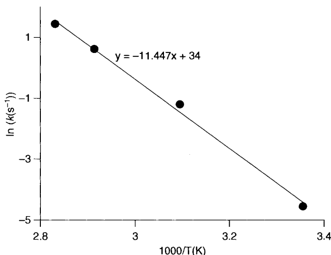
Figure 2.21. Arrhenius plot of \text{H}_2\text{O}_2 decomposition in 5:1:1 HPM. Adapted from [30]. Used with permission of the author.
