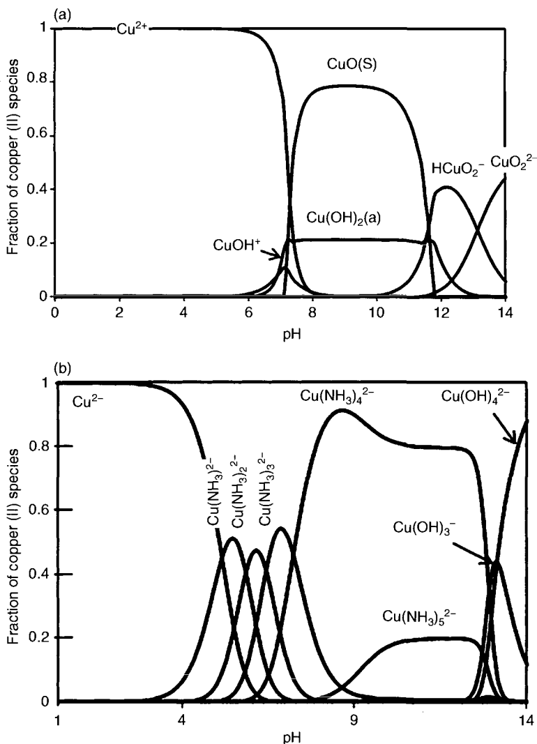
Figure 1.12. Speciation of copper in an aqueous solution a) without and b) with 1 M total ammonia, as a function of pH, for a total copper concentration of 10 ppb. Used with permission from the authors.
