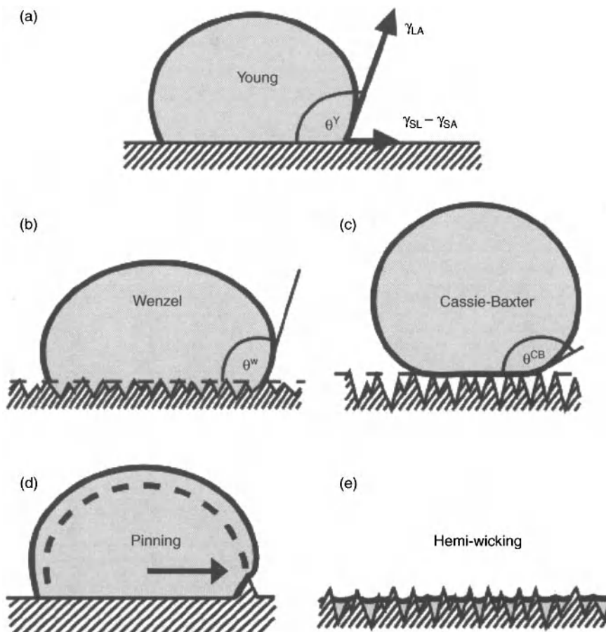
Figure 4.8. Graphic showing the physical differences as related to various theories of wetting [30]. Reprinted with permission from Langmuir , 24(10):5411 (2008). Copyright 2008, American Chemical Society. Note that the Spori et al. [30] employ different notation for the respective surface energies than used in Eqs. 4.2, 4.3 and Figure 4.5 (using A for ambient rather than V for vapor).
