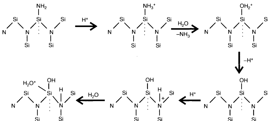
Figure 3.31. Reactions to transform \text{SiN}_4 -units to soluble silicates. Protonation of N makes the neighboring Si more susceptible for a nucleophilic substitution reaction by \text{H}_2\text{O} , with \text{NHR}_2 ( \text{R} = \text{H} or Si) being the 'leaving' group [56]. Reprinted with permission from Brown, E. H. and Whitt, C. D., Industrial and Engineering Chemistry , 44(3):615. Copyright 1952 American Chemical Society.
