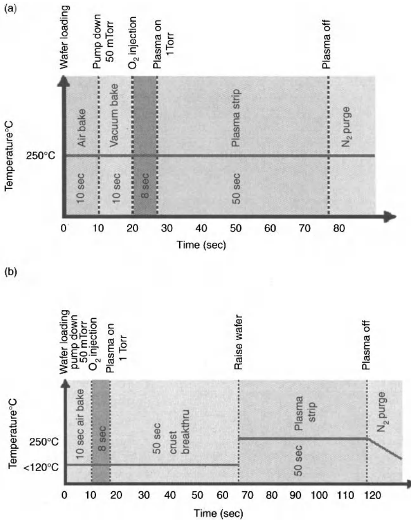
Figure 8.16. Examples of (a) typical temperature ramp and (b) controlled in-situ bake temperature profile for plasma processing used to prevent popping of the photoresist. Adapted by the authors from [41] and [44].
