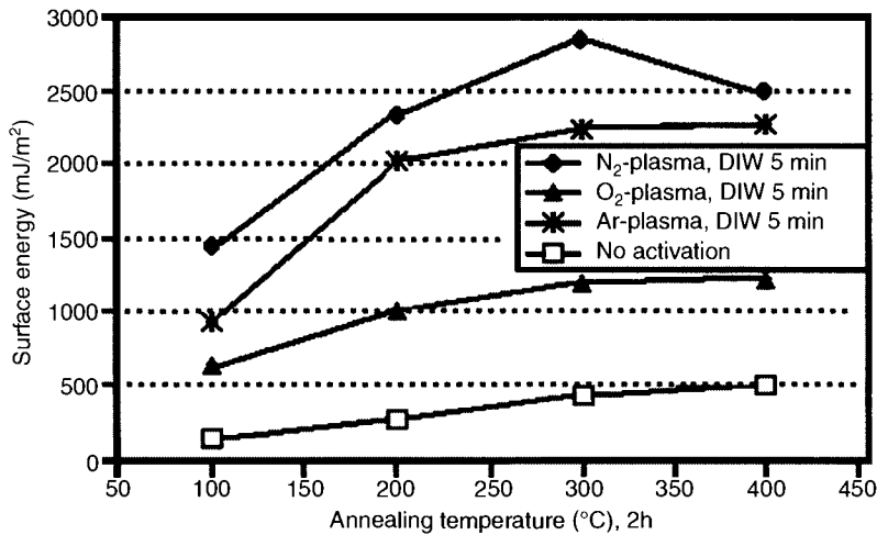
Figure 14.13. Surface energy of SiO 2 / Si bonded pairs as a function of annealing temperature for different plasma gases [92]. Reproduced with permission of ECS – The Electrochemical Society from Suni, T., Henttinen, K., Suni, I., and Makinen, J., The Journal of the Electrochemical Society .
