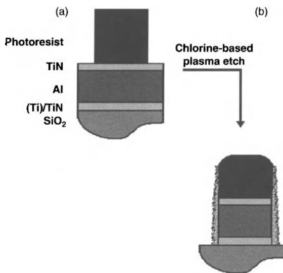
Figure 9.2. Schematic Al metal line a) before etching and b) after etching showing residue creation. Used with permission of the author.
