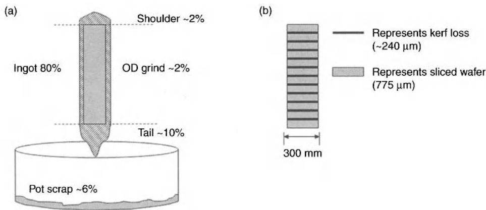
Figure 13.3. Graphical representation showing identity and distribution of scrap silicon waste during the wafer manufacturing process [10]. Used with permission of Sage Concepts.
