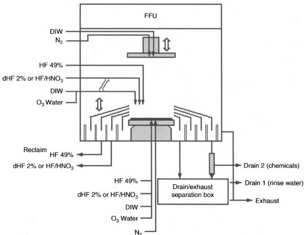
Figure 6.7. Schematic diagram of a single wafer cleaning tool. FFU is the filter fan unit. Used with permission of CT Associates, Inc.
