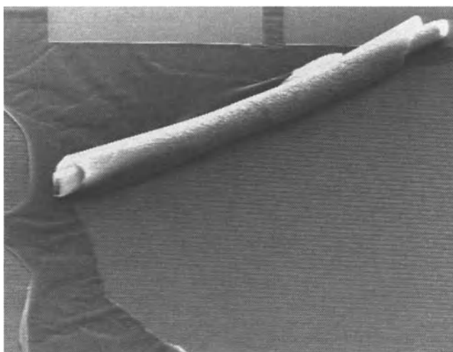
Figure 8.28. Crust is shown after wet stripping step. The crust is fragmented, allowing wet cleaning solution to strip underlying photoresist [101]. Reproduced with permission of ECS – The Electrochemical Society from Totir, G. G., Frank, M. M., Vos, R., Arnauts, S., Bearda, T., Kenis, K., Delande, M., Le, Q. T., Kesters, E., Vereecke, G., Mannaert, G., Lux, M., Hofliijk, I., Conard, T., Banerjee, S., Malhouitre, S., Leunissen, P. and Mertens, P. W., ECS Transactions .
