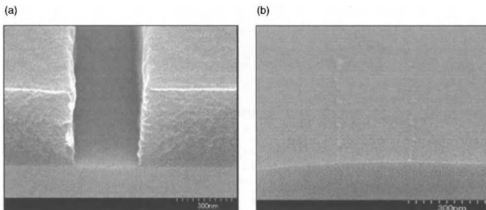
Figure 8.12. Example of a densely patterned region for a high-dose arsenic-implant wafer (a) before cleaning and (b) after cleaning showing remaining residue [12]. Reproduced with permission of ECS – The Electrochemical Society from Visintin, P. M., Korzenski, M. B., and Baum, T. H., Journal of the Electrochemical Society .
