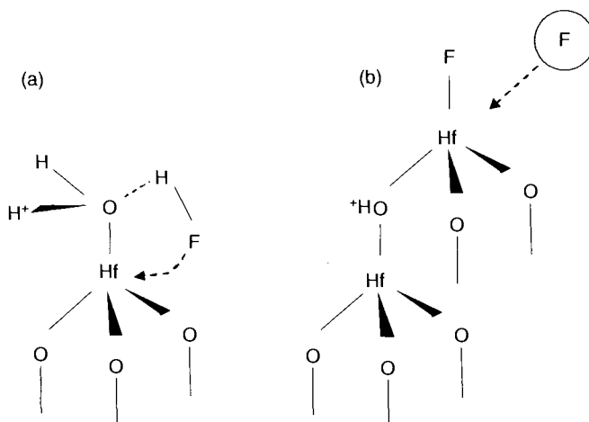
Figure 7.14. Etching mechanism proposed for \text{HfO}_2 etch in HF based solutions. Used with permission from Vasile Paraschiv.
