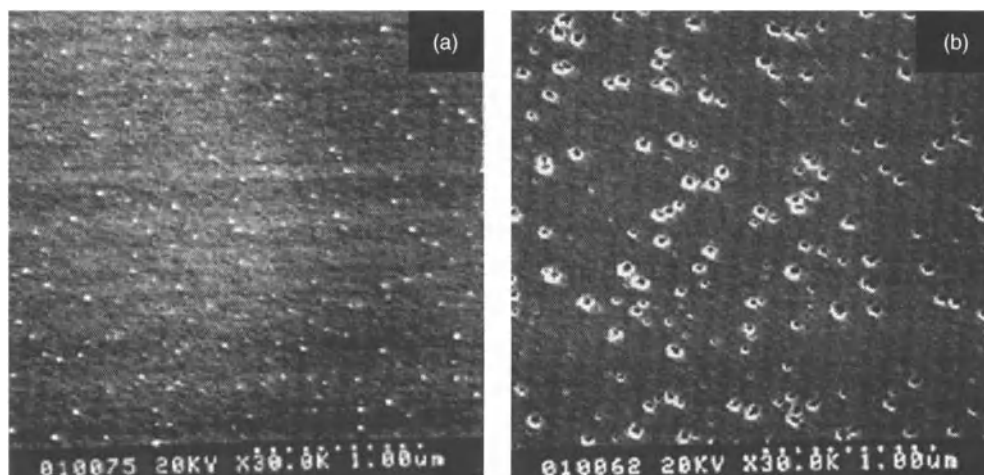
Figure 13.15. Scanning electron micrographs of (a) in situ p-doped Si and (b) on undoped Si surfaces after Cu contamination in a 0.5 wt% HF spiked with 1 ppm Cu using \text{CuCl}_2 for 3 min [48]. Reproduced with permission of ECS – The Electrochemical Society from Choi G.-M. and Ohmi, T., Journal of the Electrochemical Society .
