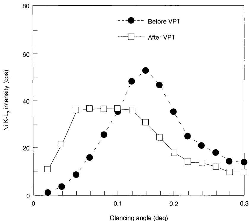
Figure 15.9. Angular dependence of fluorescent X-rays before and after VPT for 2 \times 10^{13} atoms/cm 2 Ni-contaminated standard wafer [44]. Reprinted with permission from the Japanese Journal of Applied Physics , Shimazaki, A., Miyazaki, K., Matsumura, T., and Ito, S., Volume 45(12), Page 9037 (2006).
