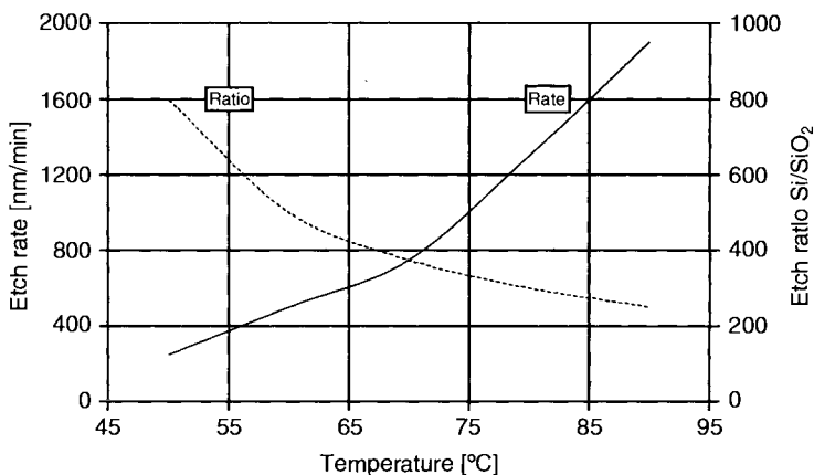
Figure 3.19. Etching rate of silicon <100> in 25 wt% KOH [43]. Used with permission of A. A. M. van de Vorst (NXP).
