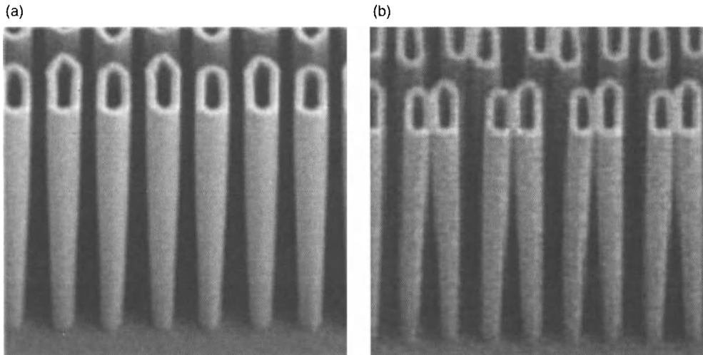
Figure 4.14. Scanning electron microscope images of a cylindrical DRAM capacitor with a) free-standing, no-stiction and b) stiction [78]. Courtesy of FSI International.
