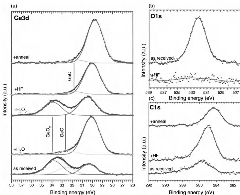
Figure 12.26. X-ray photoelectron spectroscopy data for a) Ge3d, b) O1s and c) C1s for as-received, H 2 O, H 2 O 2 , HF, and annealed surfaces. On the Ge3d core level spectra, the vertical lines indicate the center position of the GeO, GeO 2 and GeC reactive components obtained after peak decomposition [61]. Reprinted with permission from Rivillon, S., Chabal, Y. J., Amy, F., and Kahn, A., Appl. Phys. Lett. , 87(25):3101 (2005). Copyright 2005, American Institute of Physics.
