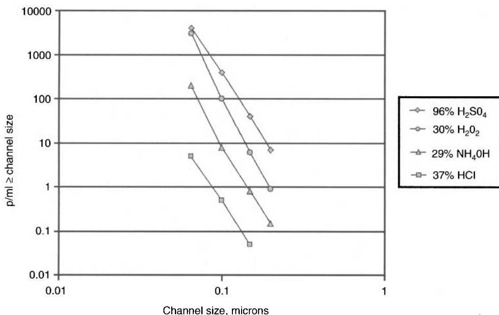
Figure 6.9. Typical production-line particle size distribution for various high purity chemicals. Used with permission from Intel Corporation.
