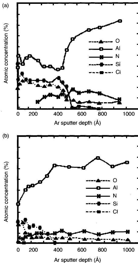
Figure 9.4. Auger electron spectroscopy spectra of aluminum sidewalls a) after aluminum line etching and with residue present and b) after sidewall residue removal with \text{BCl}_3 plasma [12]. Reproduced with permission of ECS – The Electrochemical Society from Kawamoto, H., Miyayoto, H., and Ikawa, E., Proceedings of the Tenth Symposium on Plasma Processing .
