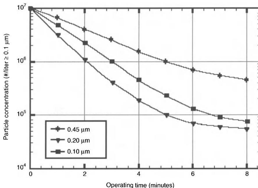
Figure 6.6. Model predictions comparing PVDF filter performance in a recirculating etch bath. Used with permission of CT Associates, Inc.
