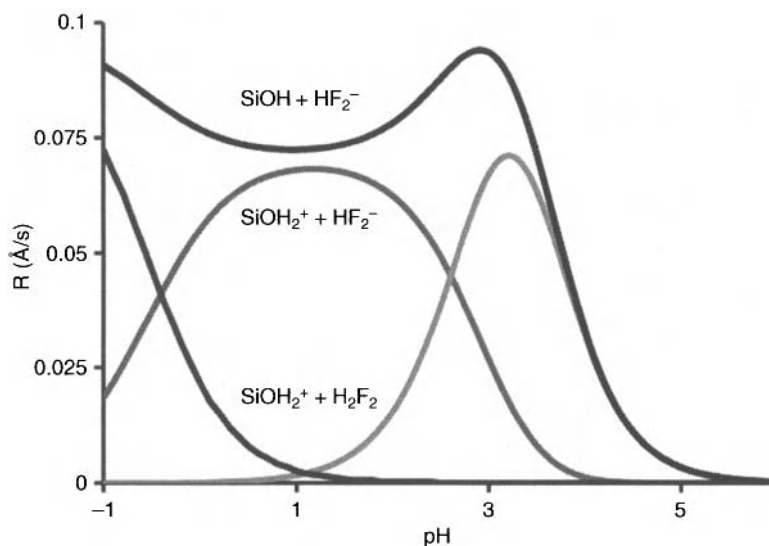
Figure 3.9. Dissolution rate of thermally grown \text{SiO}_2 in HF-based solutions with C_F = 0.1 \text{ M} ( \sim 0.2\% HF) [11]. Reprinted with permission from Knotter, D. M., J. Am. Chem. Soc. , 122(18):4345. Copyright 2000 American Chemical Society.
