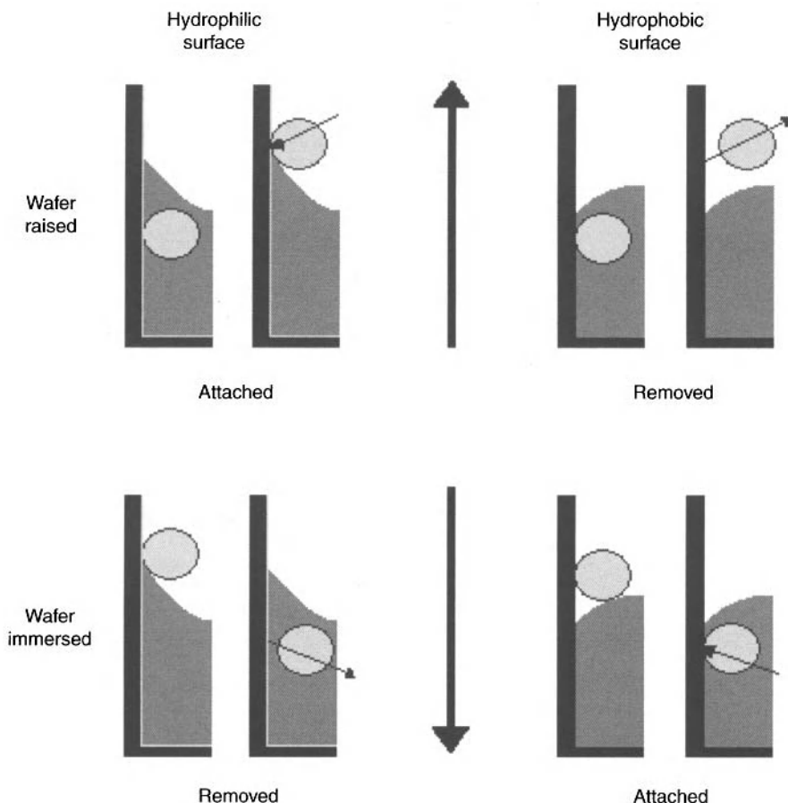
Figure 4.15. Schematic shown the effect on a particle for a hydrophilic and hydrophobic surface being immersed into or raised out of a liquid, typically in a Marangoni STG dryer \text{H}_2\text{O}/\text{IPA} . Used with permission from the author.
