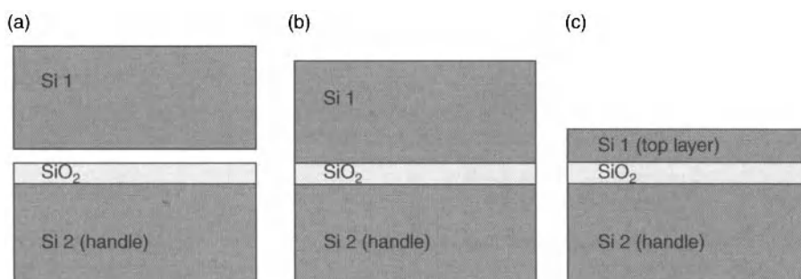
Figure 14.3. Schematic of a typical process for SOI fabrication; a) surface preparation that can include oxide formation, smoothing, and cleaning, b) direct bonding of the two Si wafers with an oxide layer between them, and c) thinning down of one wafer to obtain a top silicon layer. Reproduced with permission of CEA-LETI.
