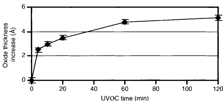
Figure 14.22. Oxide growth by \text{UV}/\text{O}_3 (UVOC) treatment of RCA-cleaned native \text{SiO}_2 surfaces vs. time. Reproduced with permission of CEA-LETI.
