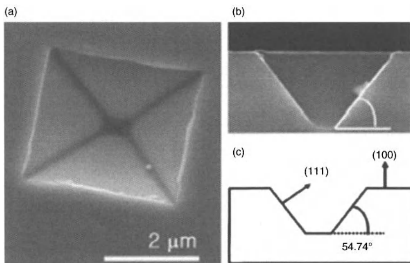
Figure 12.21. Field effect scanning electron microscopy (FE-SEM) images of a) a typical etch pit of V-groove shape formed on a Ge(100) surface exposed to \text{H}_2(\text{g}) of \sim 1 \times 10^6 \text{ L} at T = 400 \text{ K} , b) the cross sectional view of a) and c) a schematic diagram of b) showing that the etch pits are bounded by a set of four (111) planes [93]. Reprinted with permission from Lee, J. Y., Jung, S. J., Maeng, J. Y., Cho, Y. E., Kim, S., Jo, S. K., Appl. Phys. Lett. , 84(24):5028 (2004). Copyright 2004, American Institute of Physics.
