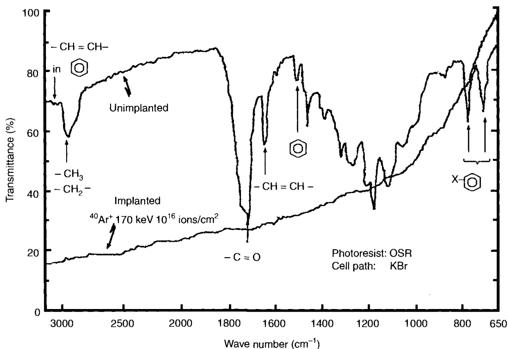
Figure 8.4. Infrared transmittance spectrum of photoresist before and after implantation. The base polymer of photoresist, OSR, is manufactured by Tokyo Oka Kogyo, is poly(-vinylxyethylcinnamate), a negative tone resist [5]. Reproduced with permission of ECS – The Electrochemical Society from Okuyama, Y., Hashimoto, T., and Koguchi, T., Journal of the Electrochemical Society .
