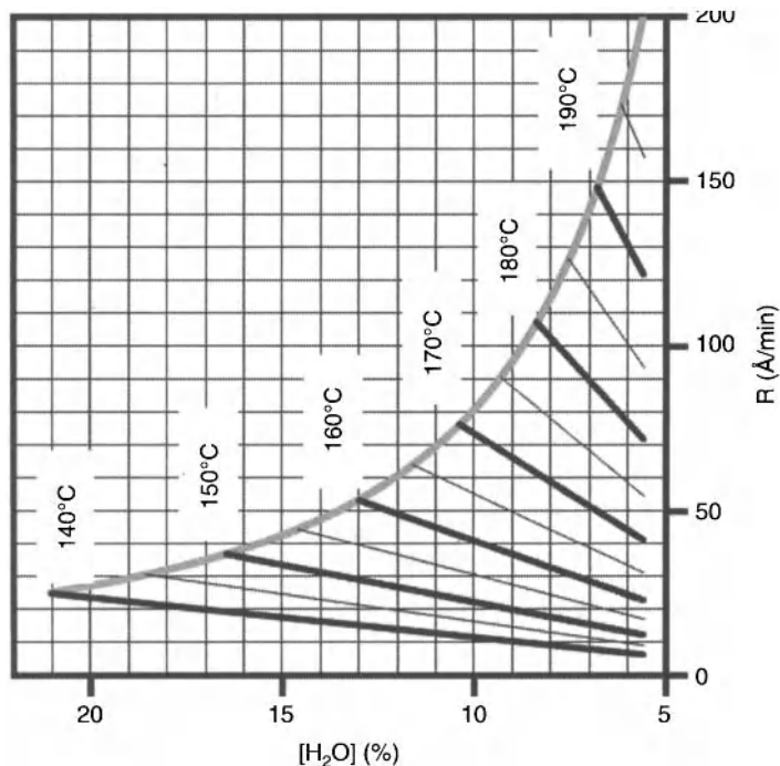
Figure 3.33. Etching rates of LPCVD \text{Si}_3\text{N}_4 (deposition temperature of 880°C) in \text{H}_3\text{PO}_4 as function of water content. Black solid lines with temperature labels are isotherms. The grey curve is \text{H}_3\text{PO}_4 at boiling temperature at 1 atmosphere pressure [49]. Reprinted from MICRO Magazine , Copyright 2005, Tom Cheney, Los Angeles, CA. Used with permission.
