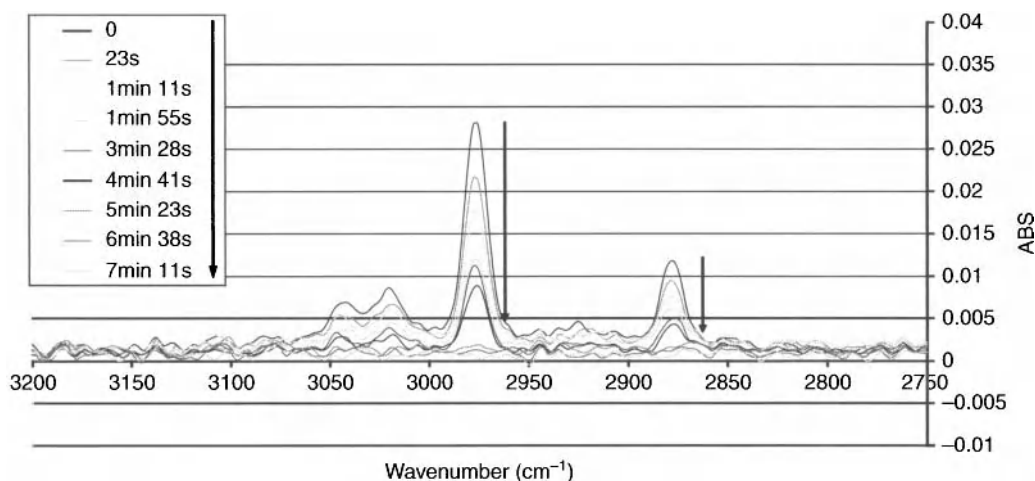
Figure 14.12. Fourier transform infrared-multiple internal reflection characterization after a low gamma solvent dry, the solvent is used in its liquid phase. The \text{CH}_x chemical signature decreases gradually in air and disappears at \sim 5 min [81]. Reproduced with permission of ECS – The Electrochemical Society from Le Tiec, Y., Fournel, F., Rochat, N., Barnes, J.-P., Veillerot, M., Morales, C., Moriceau, H., Clavelier, L., Rieutord, F., Morote, C., Vandenbossche, M., Butterbaugh, J., and Radu, I., The Electrochemical Society Transactions .
