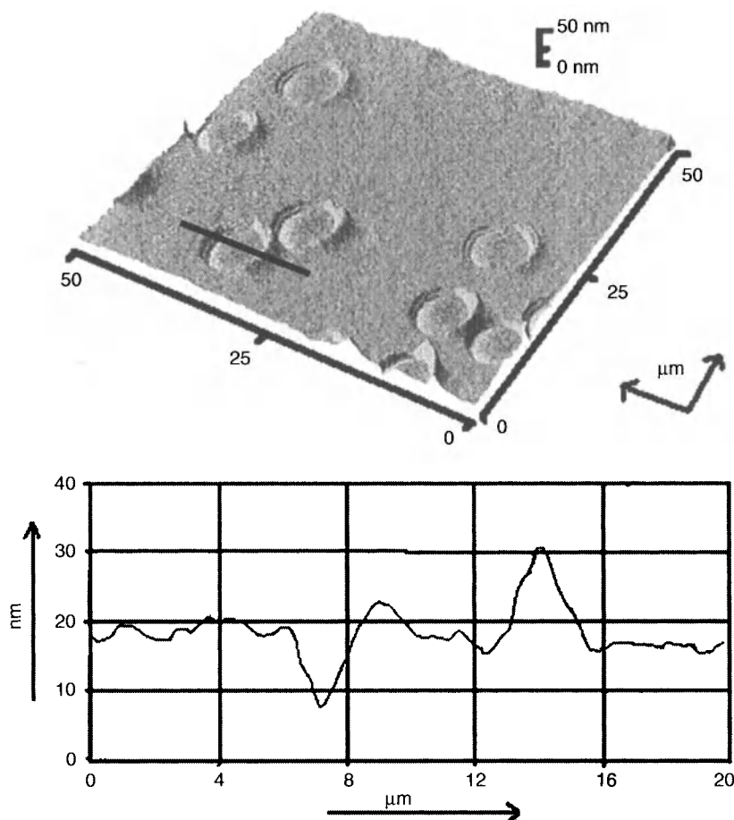
Figure 2.16. Atomic force microscopy picture of defects formed in Fe-contaminated APM [34]. Reproduced with permission of ECS – The Electrochemical Society from Knotter, D. M., Gendt, S., Mertens, P. W., and Heyns, M. M., Journal of the Electrochemical Society .
