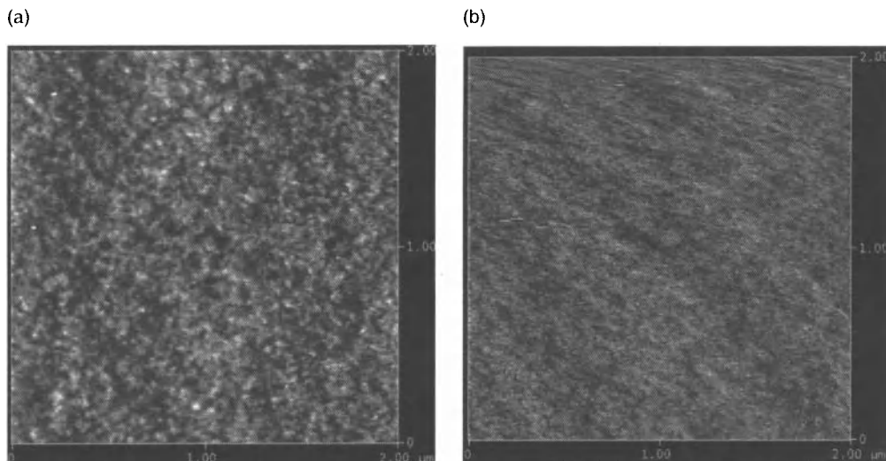
Figure 14.7. Atomic force microscopy scans of (2 \times 2) \mu\text{m}^2 samples a) before and b) after 4 nm touch-CMP removal of CVD oxide films. The roughness significantly decreases after touch-CMP. Reproduced with permission of SOITEC.
