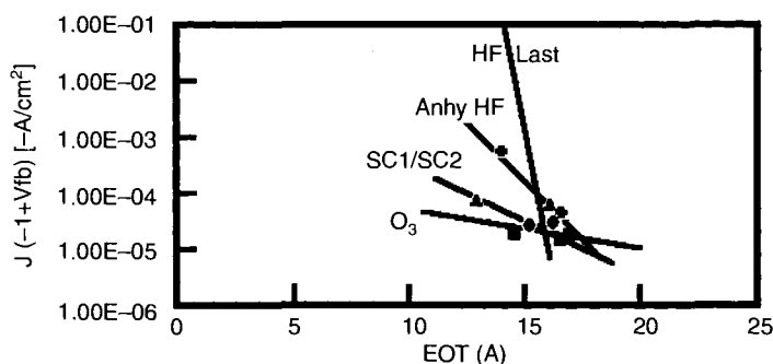
Figure 7.7. Leakage current densities of a high- \kappa stack as a function of EOT with respect to various chemical surface treatments [72]. Used with permission from SEMATECH.
