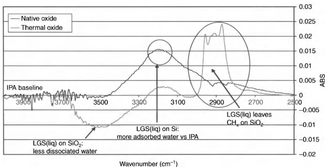
Figure 14.11. Fourier transform infrared-multiple internal reflection characterization after low gamma solvent exposure of native oxide and thermal oxide surfaces, as compared to IPA [81]. Reproduced with permission of ECS – The Electrochemical Society from Le Tiec, Y., Fournel, F., Rochat, N., Barnes, J.-P., Veillerot, M., Morales, C., Moriceau, H., Clavelier, L., Rieutord, F., Morote, C., Vandenbossche, M., Butterbaugh, J., and Radu, I., The Electrochemical Society Transactions .
