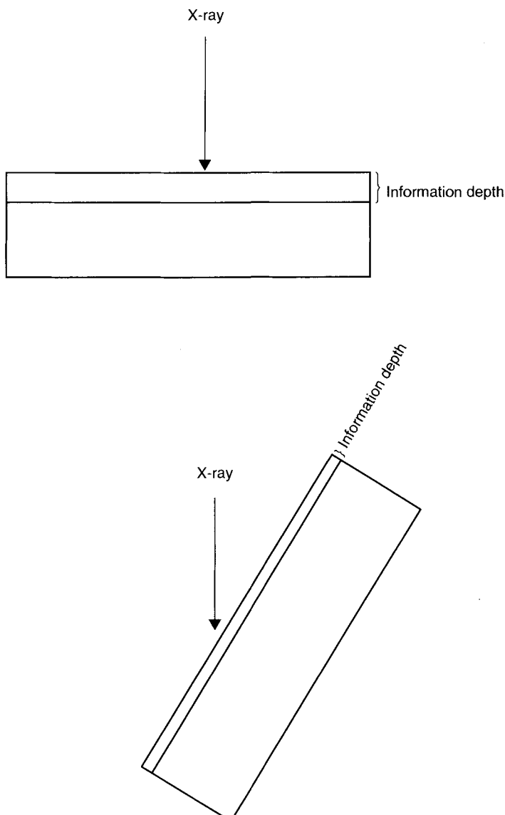
Figure 15.14. Schematic diagram of angle resolved-XPS where varying the X-ray's angle of incidence affects the information depth of the signal. Courtesy of Chris Sparks.
