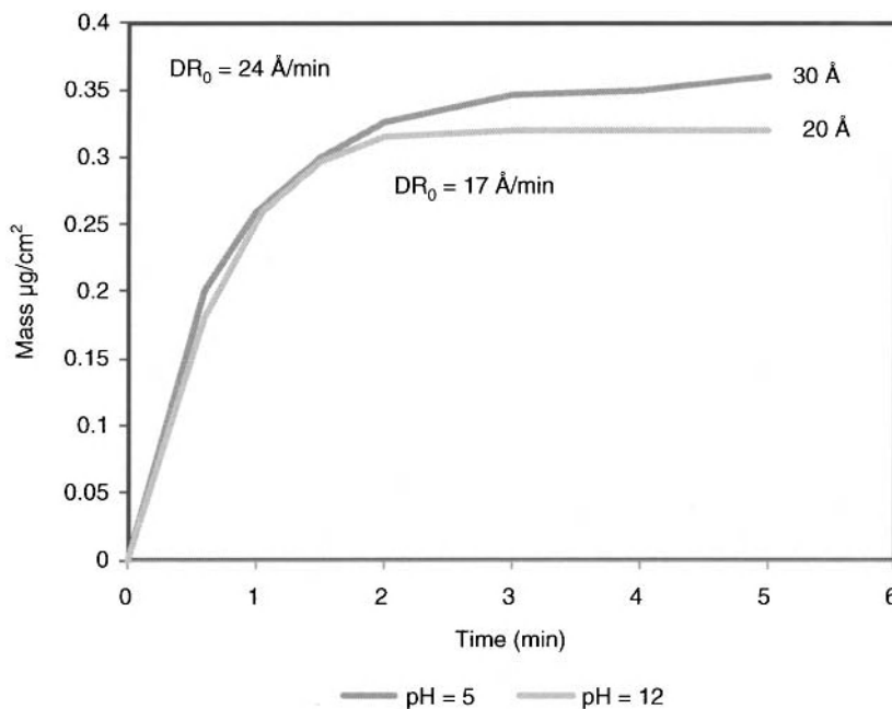
Figure 11.8. 1,2,4-triazole film deposition kinetics on Cu pH = 5 and 12 determined using a QMB in an electrochemical cell. The solution consisted of 700 ppm of TAZ in water. The film is notably thinner than that for typical BTA films (40–70 Å). The graph is based on data from [46]. Used with permission from the author.
