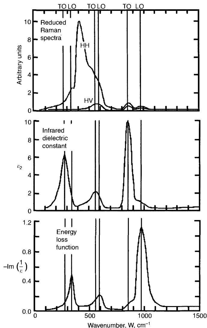
Figure 12.8. Comparison of reduced Raman spectra of bulk v\text{-GeO}_2 with the experimentally determined transverse energy loss function, \epsilon_2 , and the longitudinal energy loss function \text{Im}(-1/\epsilon) [57]. Reprinted figure with permission from Galeener, F.L. and Lucovsky, G., Phys. Rev. Lett. , 37(22):1474 (1976). Copyright 1976, American Physical Society.
