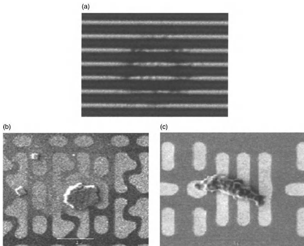
Figure 11.13. Examples of organic residue on post-copper CMP surface, all show the EDX signature of BTA. (a) Used with permission from the author. (b) and (c) [46]. Reproduced with permission of ECS – The Electrochemical Society from Peters, D., Bartosh, K., Tran, C., and Watts. C., Electrochemical Society Transactions .
