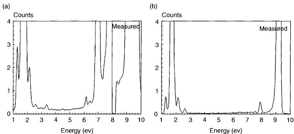
Figure 15.1. Total reflection X-ray fluorescence spectra of a 2-nm HfSiO film measured with (a) a W anode and (b) an Ir anode, showing that the Ir anode spectrum has less background noise. Used with permission from the authors.
