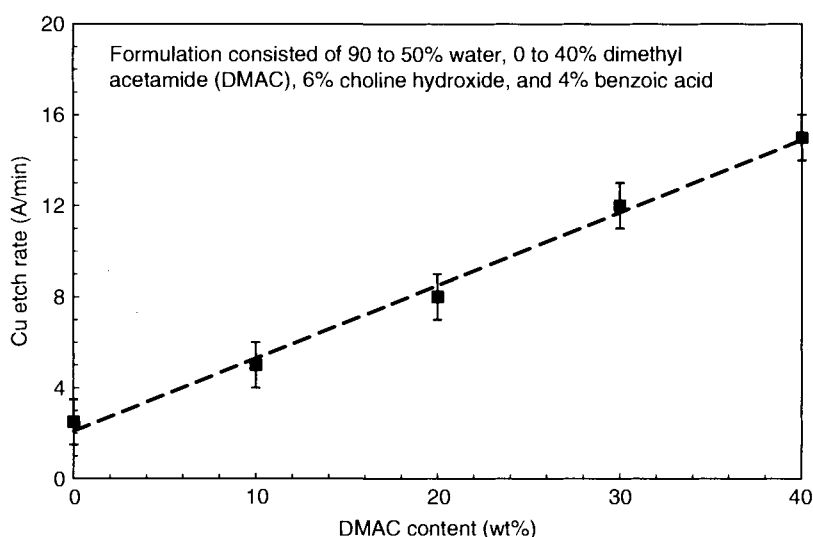
Figure 11.16. Variation in Cu etch rates with DMAC content. The complex formed with the benzoic acid anion and \text{Cu}^{+2} is soluble in DMAC but less soluble in water. Used with permission of the author.
