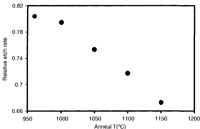
Figure 3.37. Etching rate of annealed compared to as-deposited LPCVD \text{Si}_3\text{N}_4 (relative etch rate = 1) in fresh \text{H}_3\text{PO}_4 at 160^\circ\text{C} [66]. Used with permission of A. A. M. van de Vorst (NXP).
