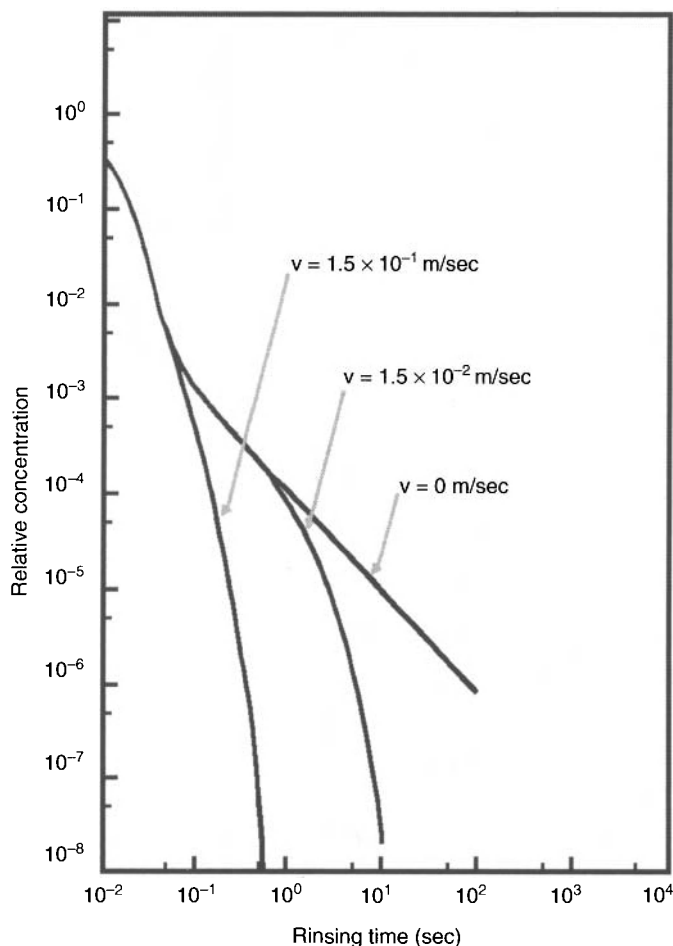
Figure 4.7. Concentrations vs. the rinsing time for a chemical solution at the bottom of a trench for various flow velocities [24]. The diffusion coefficient is 1.0 \times 10^{-9} \text{ m}^2/\text{sec} . Used with permission Reproduced with permission of ECS – The Electrochemical Society from Nakao, I., Umimoto, H., Odanaka, S., Ohzone, T., and Esaki, H., The Journal of the Electrochemical Society .
