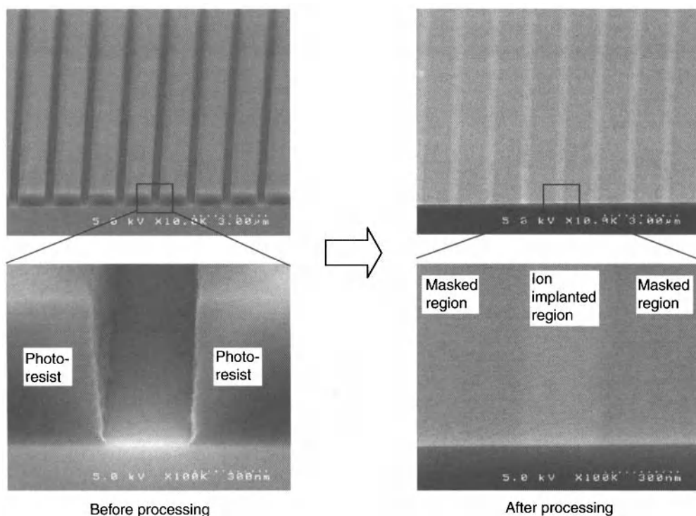
Figure 8.24. Scanning electron micrograph images of the ion-implanted surface before/after processing in a co-solvent/a chelator in SCCO 2 at 70°C, 27.6 MPa for 6 min [96]. Reproduced with permission of ECS – The Electrochemical Society from Saga, K., Kuniyasu, H., Hattori, T., Korzenski, M. B., Visintin, P. M., and Baum, T. H., ECS Transactions .
