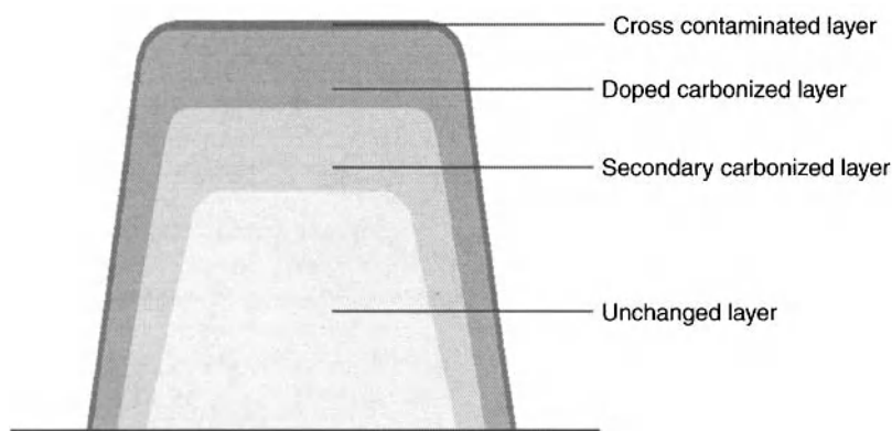
Figure 8.7. Gradient of the photoresist, adapted from [10]. Used with permission of the authors.
