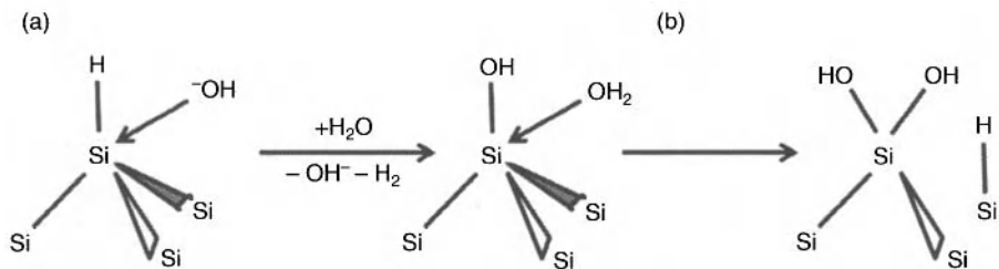
Figure 3.15. Two step reaction mechanism of the etching of silicon in KOH: A is the surface activation step where SiH is oxidized to SiOH and B is the first of three nucleophilic substitution reactions where one of three Si-Si bonds are broken. Used with permission of the author.
