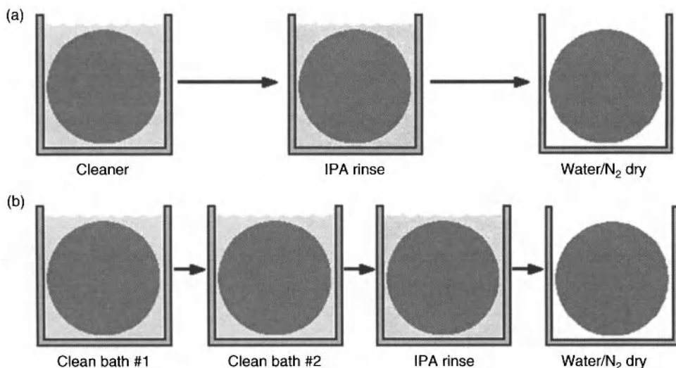
Figure 5.5. Increase in bath life by using additional chemical baths; a) standard process flow with one cleaning bath and b) process flow with two cleaning baths, the first which is more contaminated than the second, allowing the wafers to experience a clean solution before rinsing. Used with permission from the author.
