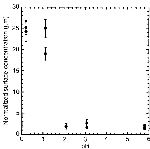
Figure 12.5. Normalized surface concentration of silica particles on the Ge surface as a function of \text{pH} [47]. The immersion time is 120 seconds. Used with permission of IMEC.
