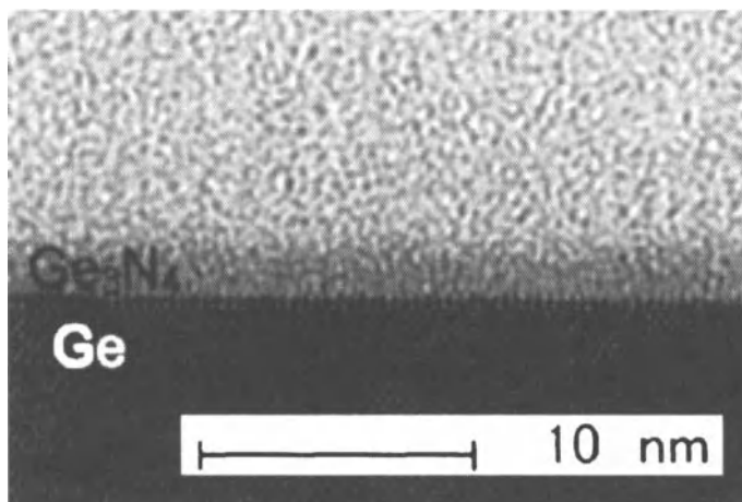
Figure 12.15. A cross sectional HR-TEM image of \text{Ge}_3\text{N}_4/\text{Ge} substrate [72]. Reprinted with permission from Maeda, T., Yasuda, T., Nishizawa, M., Miyata, N., Morita, Y., Takagi, S., Appl. Phys. Lett. , 85(15):3181 (2004). Copyright 2004, American Institute of Physics.
