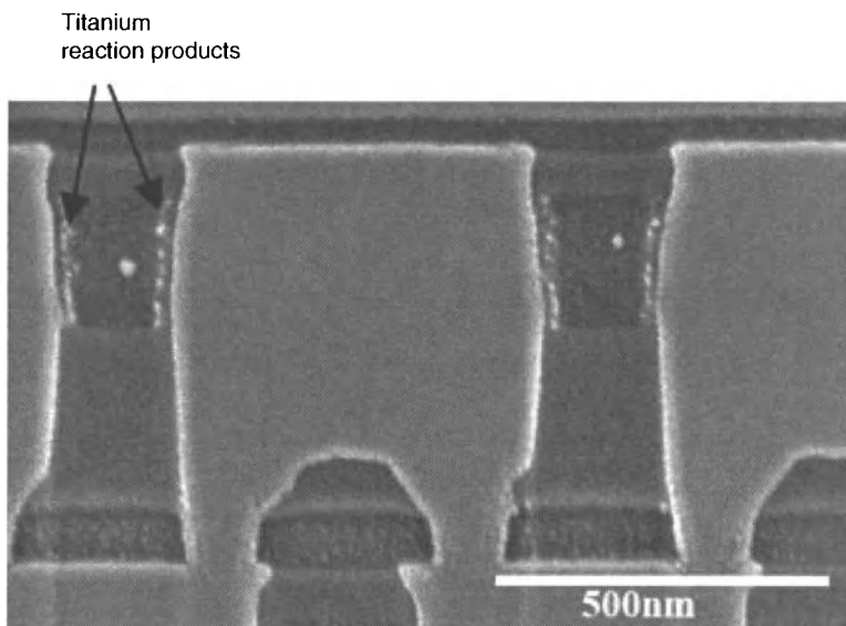
Figure 10.12. Titanium penetration into porous MSQ after reaction with TDMAT [76]. Used with the permission of the author.
