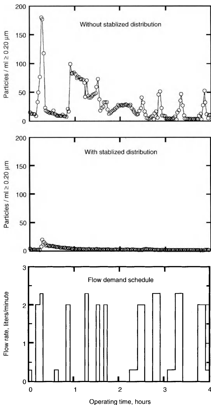
Figure 6.3. Graphs show the results of bulk chemical delivery system particle performance over time without and with recirculation [2]. Reproduced with permission of ECS – The Electrochemical Society from Deal, D. B. and Grant, D. C., Contamination Control and Defect Reduction in Semiconductor Manufacturing III .
