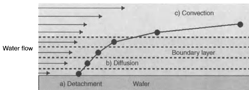
Figure 4.1. Schematic of the three steps in efficiently rinsing a planar wafer surface: a) detachment, b) diffusion, and c) convection. Courtesy of FSI International.
