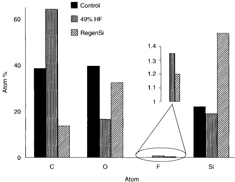
Figure 13.11. X-ray photoelectron spectroscopy analysis of \kappa = 2.2 CDO film processed using HF and RegenSi® which is a HF-based solution with surfactant as an additive, compared to unprocessed film [30]. Used with permission of the authors.
