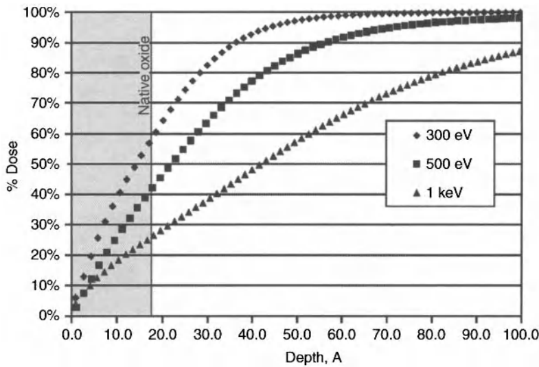
Figure 8.3. Cumulative dose vs. depth of \text{B}^+ implant at 1 \times 10^{15} \text{ atoms/cm}^2 [3]. Used with permission from Axcelis Technologies.
