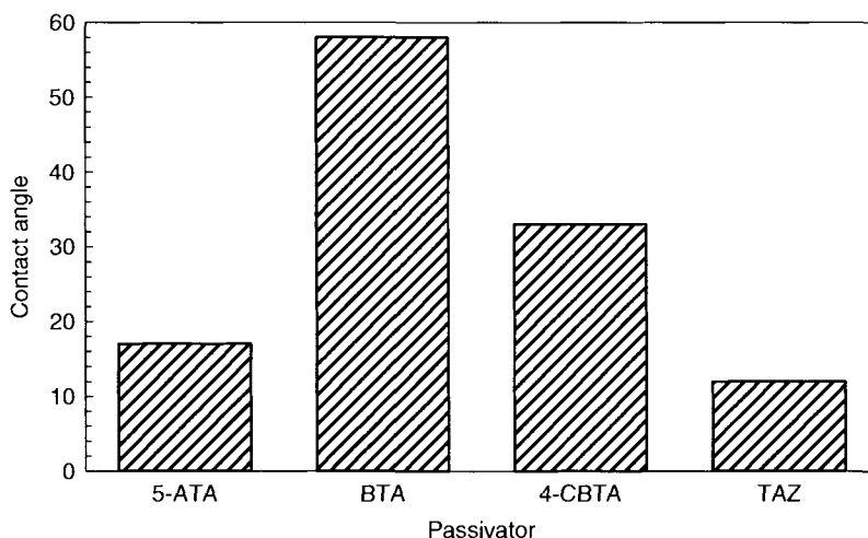
Figure 11.14. Variation in DIW water contact angle on Cu after treatment with different Cu corrosion inhibitors for the formulations shown in Figure 11.12. Used with the permission of the author.
