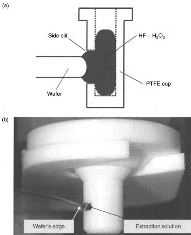
Figure 15.11. (a) Schematic of wafer horizontally supported and rotated through extraction solution and (b) image of sample collection in progress [48]. Reprinted with permission from the Proceedings of the 65th Autumn Meeting of the Japanese Society Applied Physics , Sakurai, Y., Mori, Y., and Uemura, K., Page 3p-B-17 (2004).
