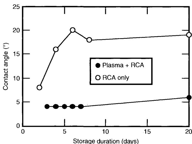
Figure 14.17. Contact angle of a water drop on silicon surface processed with either RCA cleaning or oxygen plasma followed by RCA cleaning as a function of storage duration in air [88]. From: Kissinger, G. and Kissinger, W., "Hydrophilicity of Silicon Wafers for Direct Bonding," Physica Status Solidi , 1991, A123(1):185–192. Copyright Wiley-VCH Verlag GmbH & Co. KGaA. Reproduced with permission.
