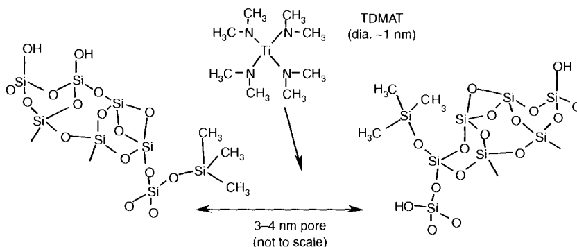
Figure 10.11. A depiction of how the addition of trimethylsilyls prevents the intrusion of TDMAT into a low- \kappa . Used by permission of the author.
