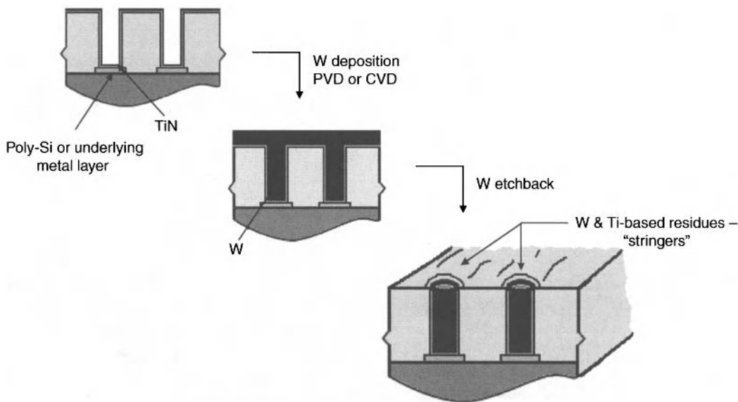
Figure 9.1. Schematic of the W etch-back process. Used with permission from author.
