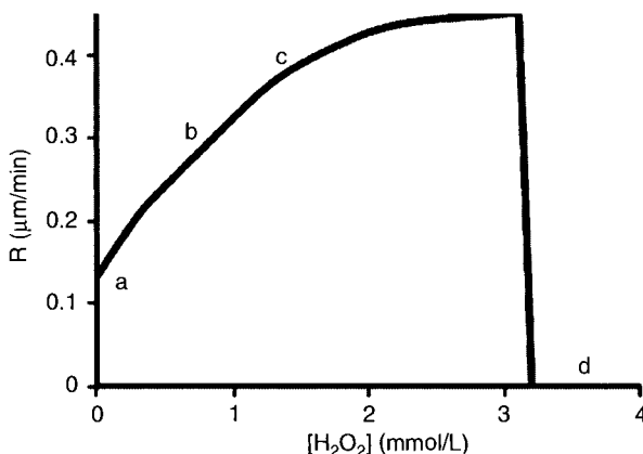
Figure 2.4. Etching rate ( R ) of Si in 1.9 M \text{NH}_3 (70°C) as a function of \text{H}_2\text{O}_2 concentration. Below 3 mM \text{H}_2\text{O}_2 dissolution of Si occurs and above 3 mM \text{H}_2\text{O}_2 dissolution of \text{SiO}_2 occurs, which is a slower process step. Letter marks indicate points from the I-E curve in Figure 2.3. Figure is adapted from [13]. Reproduced with permission of ECS – The Electrochemical Society from Meerakker, J. v. d. and Straaten, M. H. M. v. d., Journal of the Electrochemical Society.
