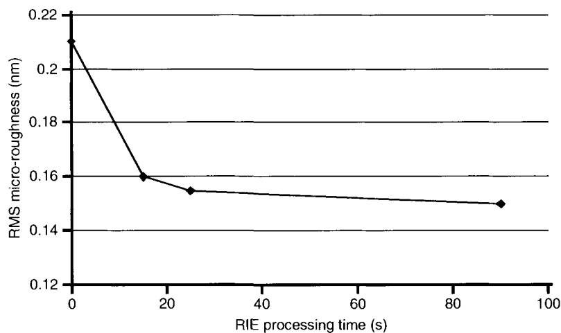
Figure 14.18. Smoothing effect of SiO 2 surface by oxygen plasma treatment versus exposure time [111]. Reproduced with permission of ECS – The Electrochemical Society from Moriceau, H., Rieutord, F., Morales, C., Sartori, S., and Charvet, A. M., and Radu, I., Semiconductor Wafer Bonding VIII: Science, Technology and Applications .
