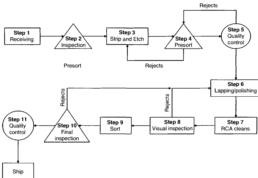
Figure 13.6. Schematic of the wafer process flow for wafer reclaim suppliers. Used with permission of the authors.
