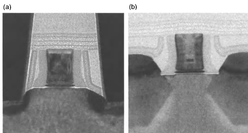
Figure 7.5. Cross section TEM image of a 45-nm HKMG using the gate-first integration a) NMOS and b) PMOS [50]. Used with permission of Auth, C., Cappellani, A., Chun, J.-S., Dalis, A., Davis, A., Ghani, T., Glass, G., Glassman, T., Harper, M., Hattendorf, M., Hentges, P., Jaloviar, S., Joshi, S., Klaus, J., Kuhn, K., Lavric, D., Lu, M., Mariappan, H., Mistry, K., Norris, B., Rahhal-orabi, N., Ranade, P., Sandford, J., Shifren, L., Souw, V., Tone, K., Tambwe, F., Thompson, A., Towner, D., Troeger, T., Vandervoorn, P., Wallace, C., Wiedemer, J., and Wiegand C., VLSI Symposium on Technology . © 2008 IEEE.
