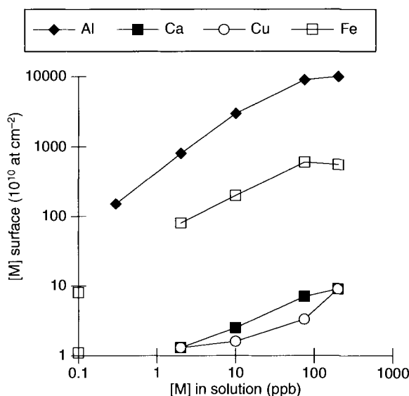
Figure 2.19. The amount of metal on a Si wafer after immersion in various concentrations of contaminated APM solution [44 Mouche]. Used with permission L. Mouche.
