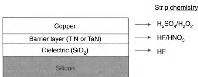
Figure 13.12. Typical stack of films to be removed from silicon wafer surface. Used with permission of the authors.
