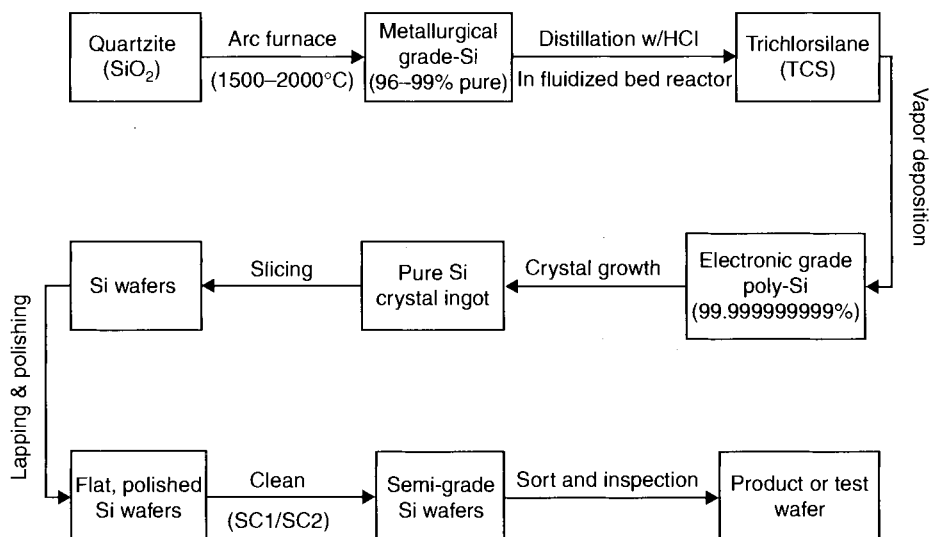
Figure 13.1. The process flow for silicon wafer manufacturing for semiconductor applications. Used with permission of the authors.
