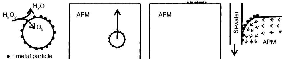
Figure 2.17. Schematic of the mechanism of cluster-LPD formation in Fe-contaminated APM. From left to right. Metal-oxide particles catalyze the decomposition of \text{H}_2\text{O}_2 thereby forming gas-bubbles. These bubbles grow and transfer metal oxide aggregates on the gas-liquid interface to the liquid surface (middle two pictures). When wafers are immersed, these aggregates are smeared over the surface as a cluster [34]. Reproduced with permission of ECS – The Electrochemical Society from Knotter, D. M., Gendt, S., Mertens, P. W., and Heyns, M. M., Journal of the Electrochemical Society .
