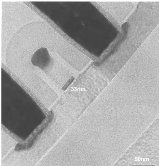
Figure 7.3. Cross section TEM image of a 32-nm HKMG using the gate-first integration scheme showing minimal loss of the substrate [49]. Used with permission of Chudzik, M., Doris, B., Mo, R., Sleight, J., Cartier, E., Dewan, C., Park, D., Bu, H., Natzle, W., Yan, W., Ouyang, C., Henson, K., Boyd, D., Callegari, S., Carter, R., Casarotto, D., Gribelyuk, M., Hargrove, M., He, W., Kim, Y., Linder, B., Moumen, N., Paruchuri, V. K., Stathis, J., Steen, M., Vayshenker, A., Wang, X., Zafar, S., Ando, T., Iijima, R., Takayanagi, M., Narayanan, V., Wise, R., Zhang, Y., Divakaruni, R., Khare, M., and Chen, T. C., VLSI Symposium Technical Digest . © 2007 IEEE.
