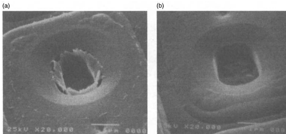
Figure 9.11. Scanning electron microscope images of a via over metal a) showing residue remaining after oxygen stripping and b) after processing with a hydroxylamine-based cleaning formulation [75]. Reproduced with permission of ECS – The Electrochemical Society from Lee, W.M., Proceedings of the Symposia on Interconnects, Contact Metalization, and Multilevel Metallization .
