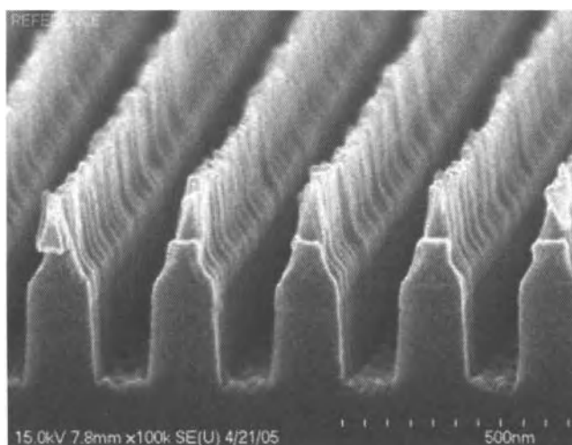
Figure 10.4. Cross section of a scanning electron microscope (SEM) image of post-etch residue on the top, sidewall, and bottom of a dual damascene via structure with \kappa \approx 2.2 . Used with permission of the author.
