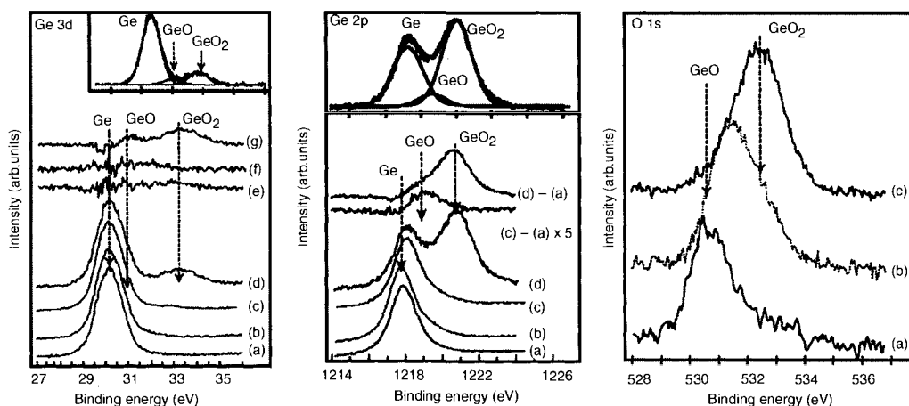
Figure 12.9. X-ray photoelectron spectroscopy of Ge3d (left panel), and Ge2p (middle panel) core level spectra of a) clean Ge(111), b) clean Ge(111) exposed to 100\text{L O}_2 at 250^\circ\text{C} , c) ex situ oxide prepared by dipping the wafer in a mixture of \text{H}_2\text{O}_2 and \text{H}_2\text{O} at room temperature, and d) clean Ge(111) exposed to clean room air for 6 hr. The difference spectra e) = (b–a), f) = (c–a), and g) = (d–a) are plotted for the Ge3d core level (left panel), and the fittings used for curves d) are shown as inset at the top of the left and middle panels. Data for O1s core level spectra (right panel) are for (a) clean Ge(111) exposed to 100\text{L O}_2 at 250^\circ\text{C} , b) Ge(111) dipped in a mixture of \text{H}_2\text{O}_2 and \text{H}_2\text{O} at room temperature, and c) Ge(111) exposed to clean air for 6h [10]. Reprinted from Surface Science Letters , Vol. 316(1), Prabhakaran, K., Ogino, T., Hull, R., Bean, J. C., and Peticolas, L. J., “An efficient method for cleaning Ge(100) surface”, page L1031. Copyright (1994) with permission from Elsevier.
