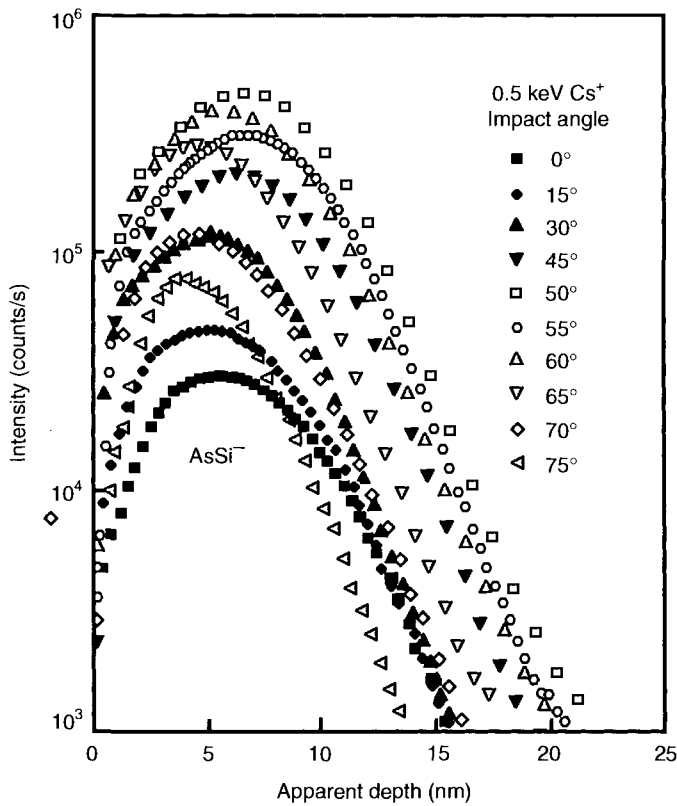
Figure 8.2. Arsenic depth profiles obtained by SIMS for 1 \times 10^{15} \text{ atoms/cm}^2 implanted at 5 keV [2]. Used with permission of Fujitsu, from Kataoka, Y., Shigeno, M., Tada, Y., Yamazaki, K., and Kase, M., Fujitsu Sci. Tech. J. , 38(1):69 (2002).
