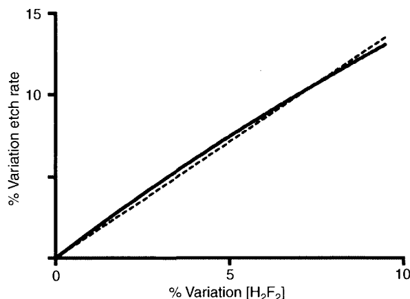
Figure 2.31. Model calculation: comparison of the etching rate variation of \text{SiO}_2 with the variation in concentration of \text{H}_2\text{F}_2 . The thin line is variations caused by concentration changes of pure 2 wt% HF, and the bold line is due to dissolving 1 g \text{SiO}_2 per liter. Used with permission of the author.
