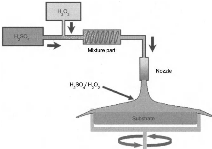
Figure 8.21. Example of a single wafer spin processor for high dose implant stripping showing point-of-use mixing of chemicals [74]. Used with permission of DNS.
