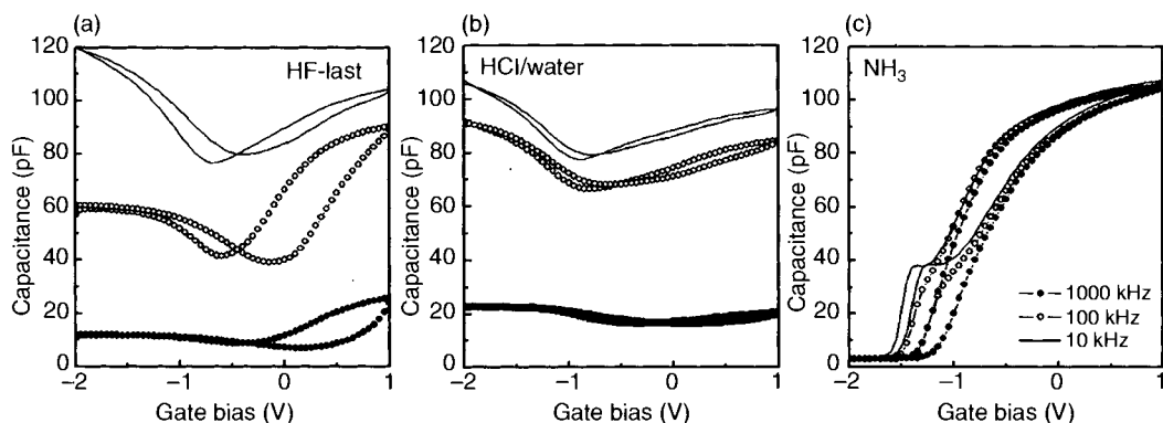
Figure 12.18. Dual-sweep high-frequency CV characteristics of Al/50-Å ALD \text{HfO}_2 /n-Ge(100) MOS capacitors involving surface preparation by a) an HF-last process, b) a dilute aqueous HCl rinse sequence, and c) a dilute aqueous HCl rinse sequence, followed by a 60 sec anneal in \text{NH}_3 at 650^\circ\text{C} . Capacitor area is 6.9 \times 10^{-5} \text{ cm}^2 [83]. Reprinted with permission from Frank, M. M., Shang, H., Rivillon, S., Amy, F., Hsueh, C.-L., Paruchuri, V. K., Mo, R. T., Copel, M., Gusev, E. P., Gribelyuk, M. A., and Chabal, Y. J., Solid State Phenomena , 103–104:3 (2005).
