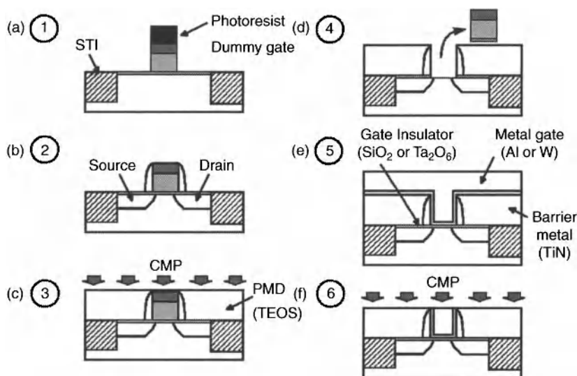
Figure 7.4. Schematic of the dual gate-last process flow with CMP step for defining the gate structures [42]. PMD is pre-metal dielectric. Used with permission of Yagishita, A., Saito, T., Nakajima, K., Inumiya, S., Akasaka, Y., Ozawa, Y., Hieda, K., Tsunashima, Y., Suguro, K., Arikado, T., and Okumura, K., Transactions of Electron Devices . © 2000 IEEE.
