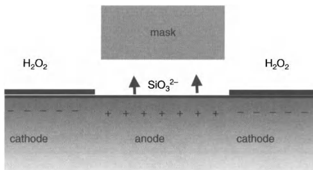
Figure 2.13. Crevice corrosion in APM – \text{H}_2\text{O}_2 becomes depleted under the mask and silicon dissolves anodically. The mask can be a particle, bubble, or photoresist residue. Used with permission of the author.
