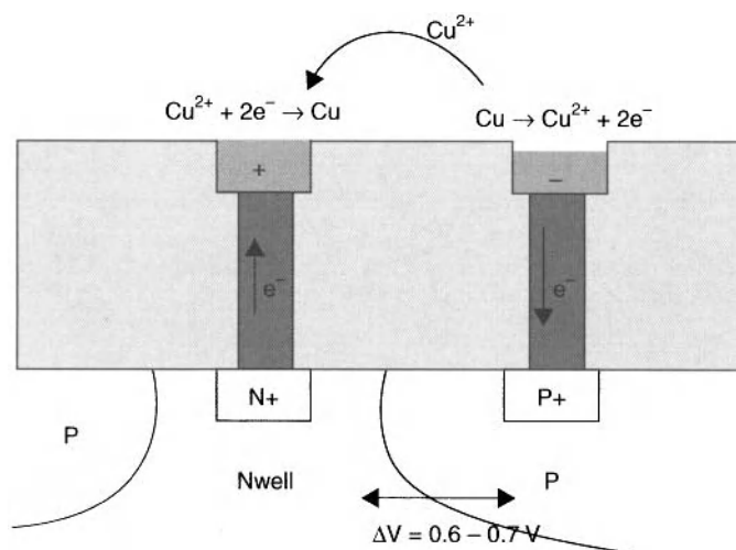
Figure 11.3. Copper ion migration from different implanted area, showing pathway for electrogalvanic corrosion [16]. Reproduced with permission of ECS – The Electrochemical Society from Gabrielli, C., Ostermann, E., Perrot, H., and Mége, S., Proceedings of Cleaning Technology in Semiconductor Manufacturing VIII .
