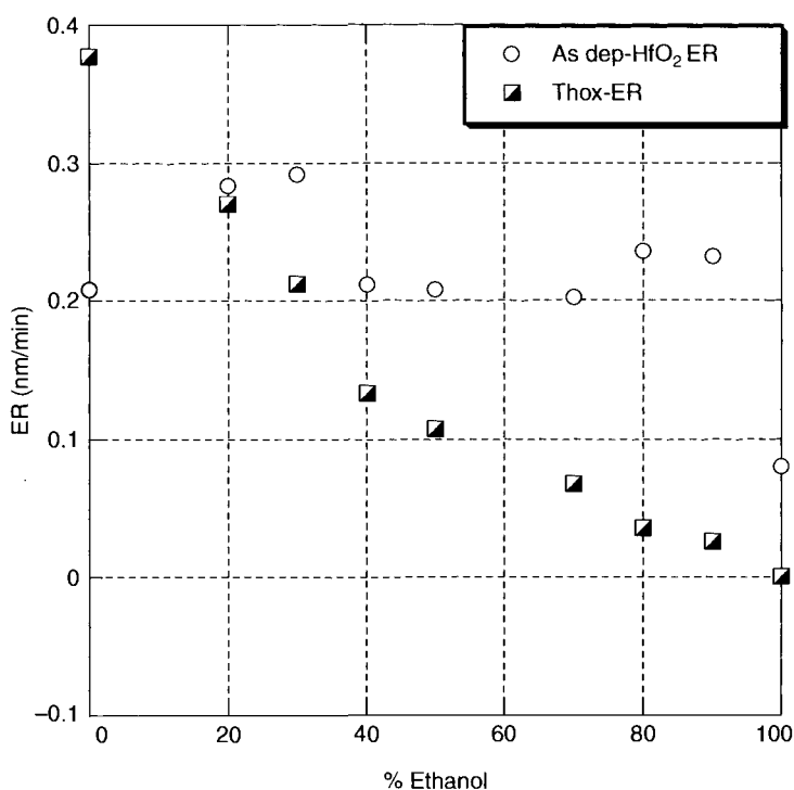
Figure 7.15. As deposited- \text{HfO}_2 and thermally grown \text{SiO}_2 etching rates as a function of the percentage of ethanol in the \text{HF}/\text{H}_2\text{O} /ethanol mixture ( [\text{HF}] = 0.05 mole/L; T = 25^\circ\text{C} ). Used with permission from Vasile Paraschiv.
