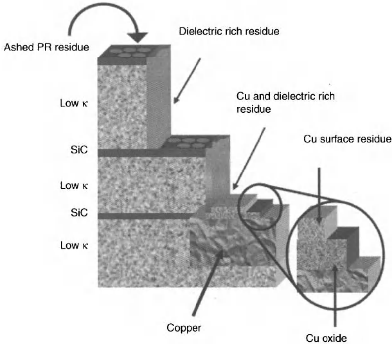
Figure 10.5. Schematic of the wafer surface after post-etch and strip cleaning showing issues related to cleaning [21]. Courtesy of DuPont/EKC Technology (2010).
