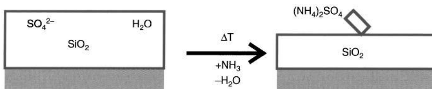
Figure 2.24. Formation of aged-LPD that are crystals of ammonia sulfates. Used with permission of the author.
