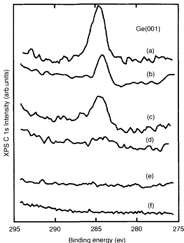
Figure 12.10. C1s core level XPS spectra from Ge(100) wafers after undergoing a) a degreasing step involving successive rinses of trichloroethylene, acetone, and methanol (process 1), b) process 1 followed by a thermal anneal to 620K, c) process 1 followed by an ultrasound rinse in DIW for 15 min (process 2), d) process 2 followed by a thermal anneal to 620K, e) process 2 followed by a 30 min UV/O 3 exposure (process 3) and f) process 3 followed by a thermal anneal to 620K [13]. Reprinted with permission from Zhang, X.-J., Xue, G., Agarwal, A., Tsu, R., Hasan, M.-A., Greene, J. E., and Rockett, A., J. Vac. Sci. Technol. , A11(5):2553 (1993). Copyright 1993, American Institute of Physics.
