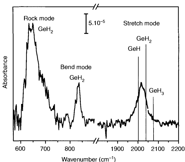
Figure 12.25. Transmission absorption IR spectrum of H/Ge (100) after HF wet chemical treatment for 10 min using the ultra-thin native epi-ready Ge wafer as reference [61]. The positions for mono-, di- and tri-hydride stretch modes are indicated with vertical lines. Reprinted with permission from Rivillon, S., Chabal, Y. J., Amy, F., and Kahn, A., Appl. Phys. Lett. , 87(25):3101 (2005). Copyright 2005, American Institute of Physics.
