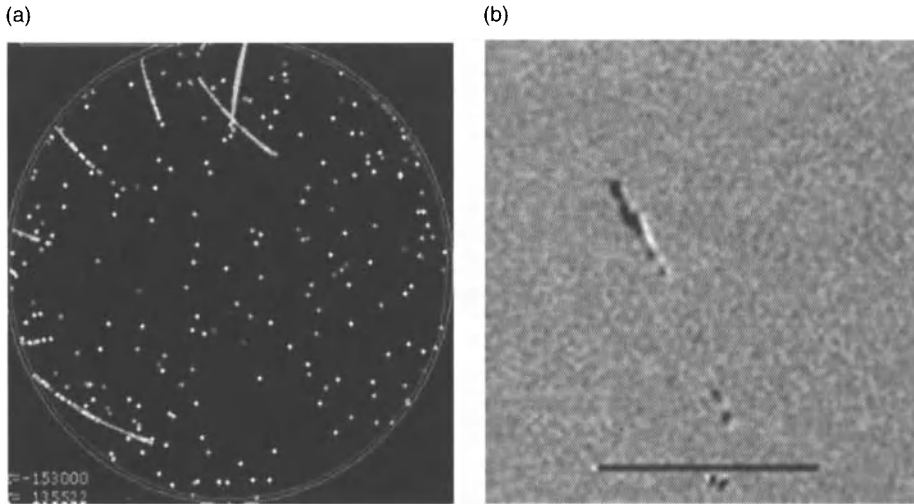
Figure 14.8. a) KLA Tencor SP2 map of light point defects (LPD) and scratches characterized on a polySi surface. b) SEM image of a scratch. Reproduced with permission of SOITEC.
