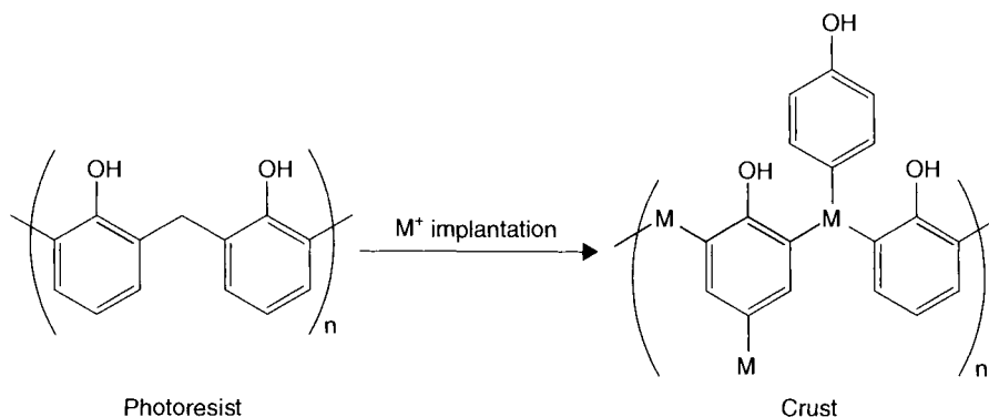
Figure 8.8. Proposed chemical reaction between the high-dose ion-implant ( M = \text{B}, \text{P}, \text{or As} ) and photoresist [10], as interpreted by [12]. This reaction results in the hard to remove crust (highly cross linked polymer). Reproduced with permission of ECS – The Electrochemical Society from Visintin, P. M., Korzenski, M. B., and Baum, T. H., Journal of the Electrochemical Society .
