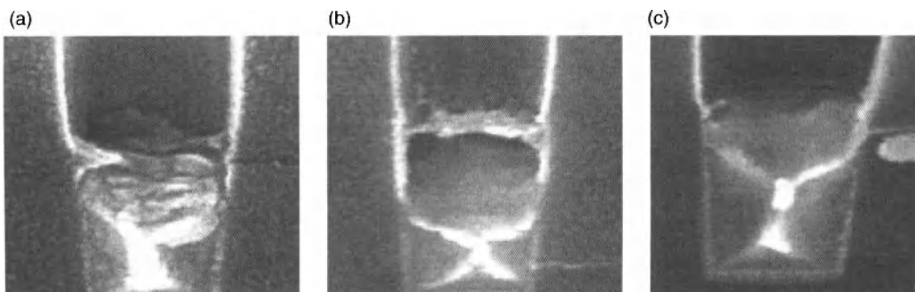
Figure 10.9. Cross-section SEM images of the bottom of a copper/low- \kappa via a) after etch and before stripping and cleaning showing post-etch polymer at the bottom and on the sidewalls of the via, b) after cleaning showing copper corrosion and article removal of the etch residue, and c) after cleaning with no copper corrosion and complete residue removal [21]. Courtesy of DuPont/EKC Technology (2010).
