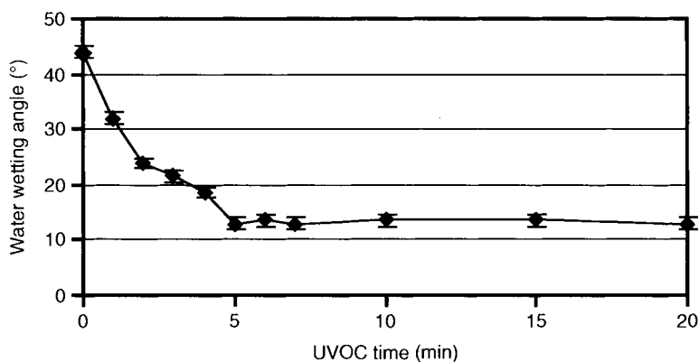
Figure 14.23. Thin thermally grown oxide surfaces after 24 hr contamination followed by UV/O 3 (UVOC) cleaned vs. times. The decrease in contact angle indicates removal of hydrocarbon contamination. Reproduced with permission of CEA-LETI.
