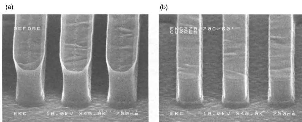
Figure 9.3. Scanning electron microscope images of Al metal lines a) after etching and stripping with residue present and b) after cleaning showing residue removal. Courtesy of DuPont/EKC Technology (2010).
