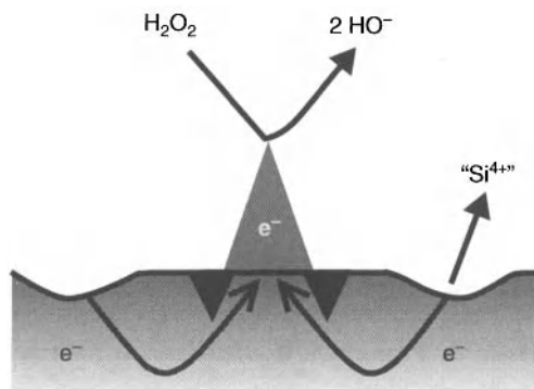
Figure 2.12. A local corrosion cell formed by the galvanic coupling of a metal (or also n-doped silicon) to a silicon surface [34]. Reproduced with permission of ECS – The Electrochemical Society from Knotter, D. M., Gendt, S., Mertens, P. W., and Heyns, M. M., Journal of the Electrochemical Society .
