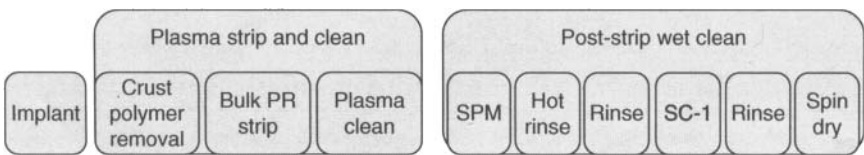
Figure 8.14. Outline of a high dose implant strip process showing the plasma and wet stripping cleaning flow. Used with permission of the authors.
