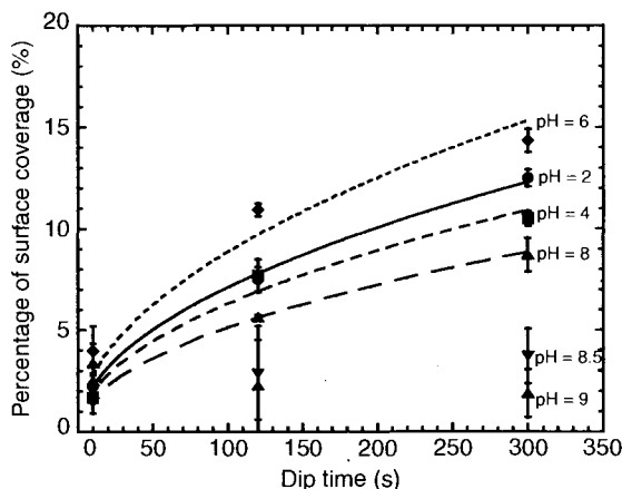
Figure 12.6. Relative surface coverage as a function of immersion time at different pH values of alumina particles [47]. Straight and dotted lines represent fittings based on diffusion limited deposition. Used with permission of IMEC.
