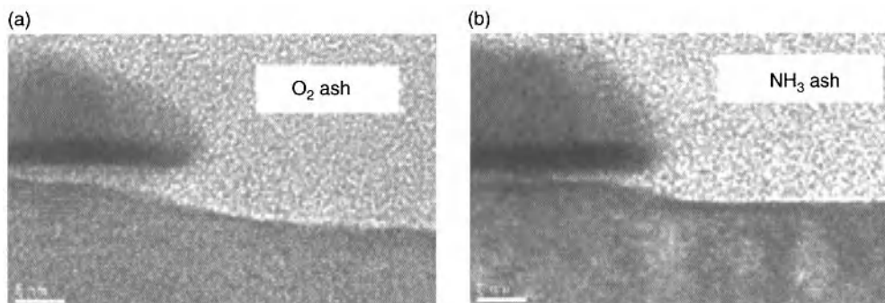
Figure 7.18. Comparison of the resulting HfO 2 high- \kappa /metal gate profiles from a) an O 2 stripped and b) a NH 3 stripped process. The sample processed with NH 3 shows no indication of bottom oxide encroachment into the gate stack edge [161]. Reproduced with permission of ECS – The Electrochemical Society from Song, S. C., Zhang, Z., Huffman, C., Bae, S. H, Sim, J. H., and Lee, B. H., Electrochemical and Solid State Letters .
