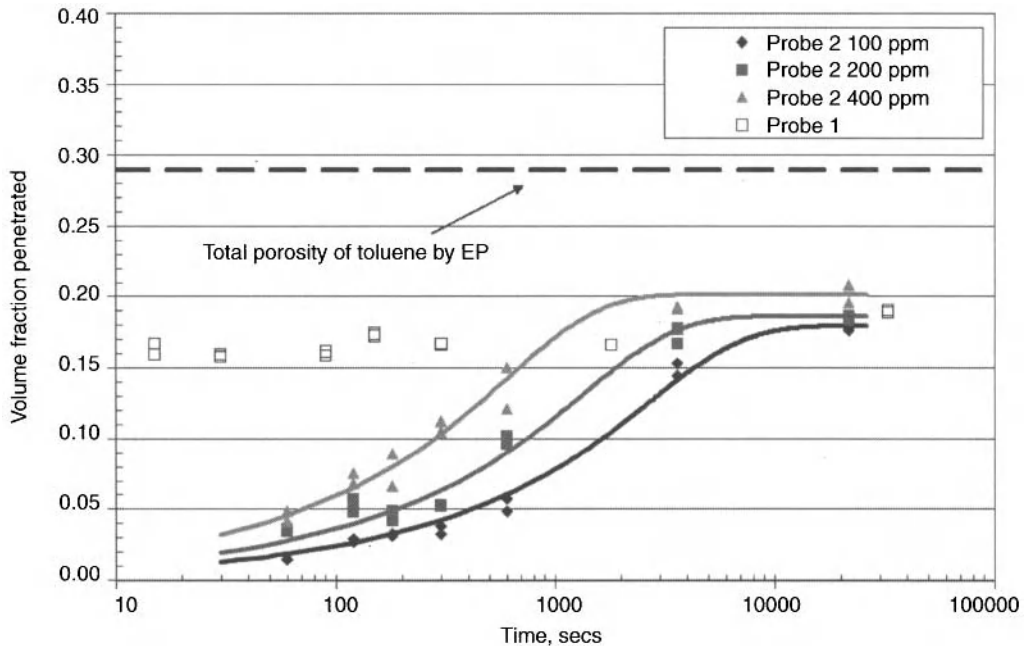
Figure 16.2. Results of ellipsometric porosimetry to show the penetration rates of a molecular probe that measures their diffusion into porous low- \kappa dielectrics [21]. Used with permission of Air Products and Chemicals.
