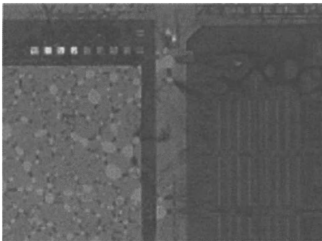
Figure 8.15. Micrograph of the high dose implanted photoresist showing popping. This occurs when the bulk photoresist is heated during the plasma strip step without first removing the crust layer [41]. Used with permission from Axcelis Technologies.
