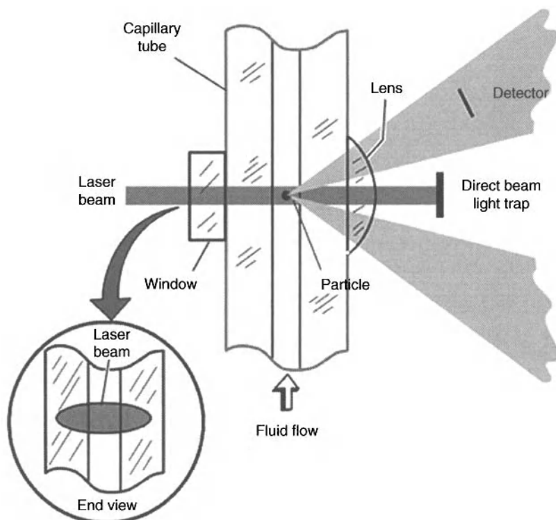
Figure 6.8. Graphical illustration of how an optical particle counter functions. Used with permission from Particle Measuring Systems.
