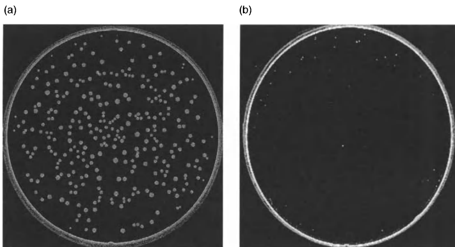
Figure 14.24. Comparison between 200-mm wafers in which both Si surfaces are treated a) without and b) with a UV/O 3 cleaning treatment prior to direct bonding. Analysis was performed by SAM after a 200°C post-bonding anneal. Reproduced with permission of CEA-LETI.
