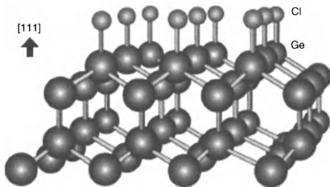
Figure 12.28. Schematic view of an ideally chlorine-terminated germanium (111) surface [108]. Reprinted with permission from Lu, Z. H., Appl. Phys. Lett. , 68(4):520 (1996). Copyright 1996, American Institute of Physics.
