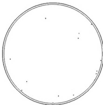
Figure 14.29. Particle size characterization with a threshold of 90 nm on Si(001) surface after a aqueous HF treatment, rinsed with progressively adding DIW to the HF bath, and then dried. No particle larger than 0.3 \mu\text{m} is detected. Reproduced with permission of CEA-LETI.
