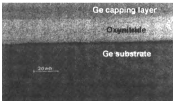
Figure 12.16. High resolution TEM image of an oxynitride film grown on a \text{Ge}(100) wafer obtained after a two stage-oxidation/nitridation process. The oxynitride layer is capped with amorphous Ge [76]. Reprinted with permission from Paine, D. C., Rosenberg, J. J., Martin, S.C., Luo, D., and Kawasaki, M., Appl. Phys. Lett. , 57(14):1443 (1990). Copyright 1990, American Institute of Physics.
