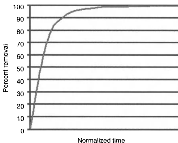
Figure 6.19. Particle removal in recirculation tank versus time of recirculation. Used with permission from Pall Corporation.
