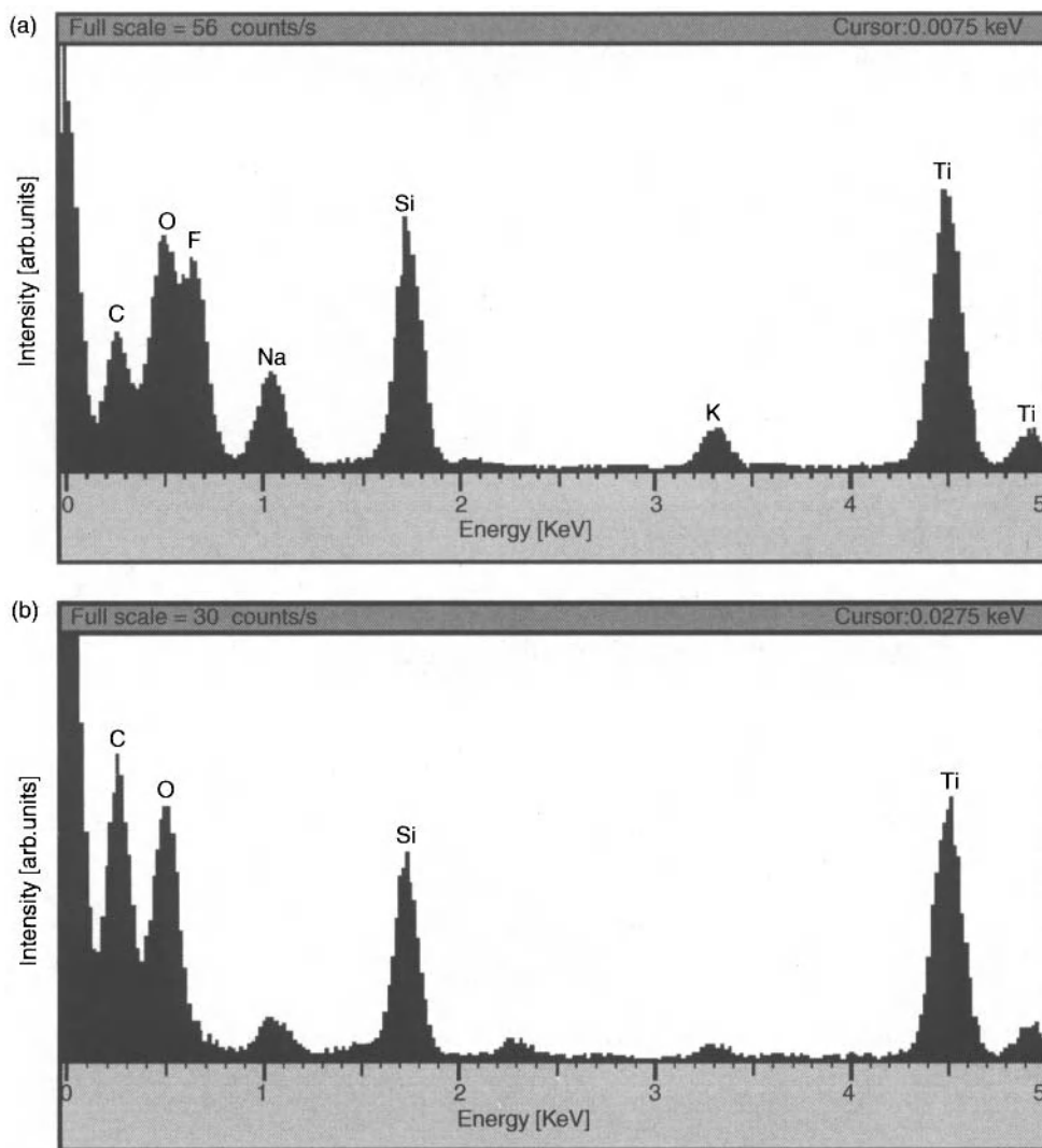
Figure 9.8. Example EDS spectra of sidewall via residue a) before and b) after O_2 plasma stripping [13]. The Na and K signals probably are due to the sample preparation. Reproduced with permission of ECS – The Electrochemical Society from Song, J., Kim, J., Seo, H., Kim, Y., and Jeon, H., Journal of the Electrochemical Society .
