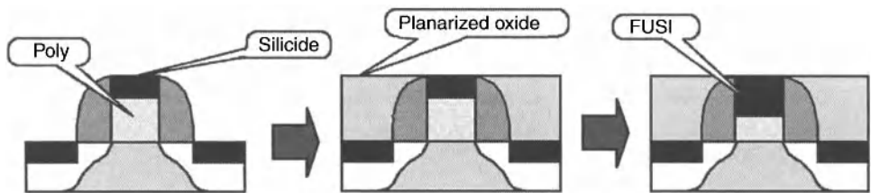
Figure 7.6. Schematic of the fully silicided gate process flow with CMP step prior to full silicidation [60]. Reproduced with permission of ECS – The Electrochemical Society from Maszara, W. P., Journal of the Electrochemical Society .
