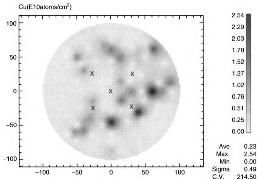
Figure 15.4. Two dimensional map of copper contamination, the X's represent coordinates for a standard 5-point map where no copper was measured [11]. Used with permission from the author.
