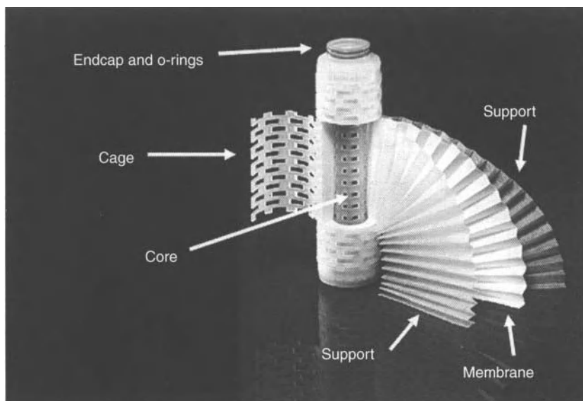
Figure 6.17. Key components for a pleated filter, the most commonly used configuration for wet cleans. Used with permission from Pall Corporation.
