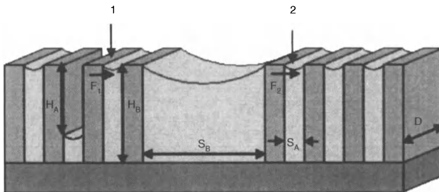
Figure 16.6. Physics of photoresist collapse, force model [39]. Reprinted with permission from J. Vac. Sci. Technol. , B18(6):3303. Copyright 2000, American Vacuum Society
