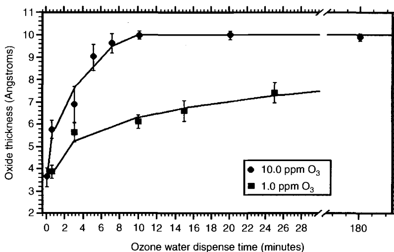
Figure 7.8. Chemical oxide thickness vs. time for two different concentrations of ozone at 22°C [75]. Courtesy of FSI International.
