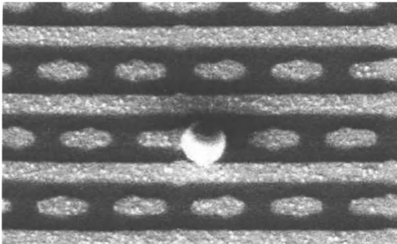
Figure 6.11. Scanning electron micrograph photo shows a wafer surface with particulate contamination that may adversely affect the electrical conductivity. Used with permission from Intel Corporation.
