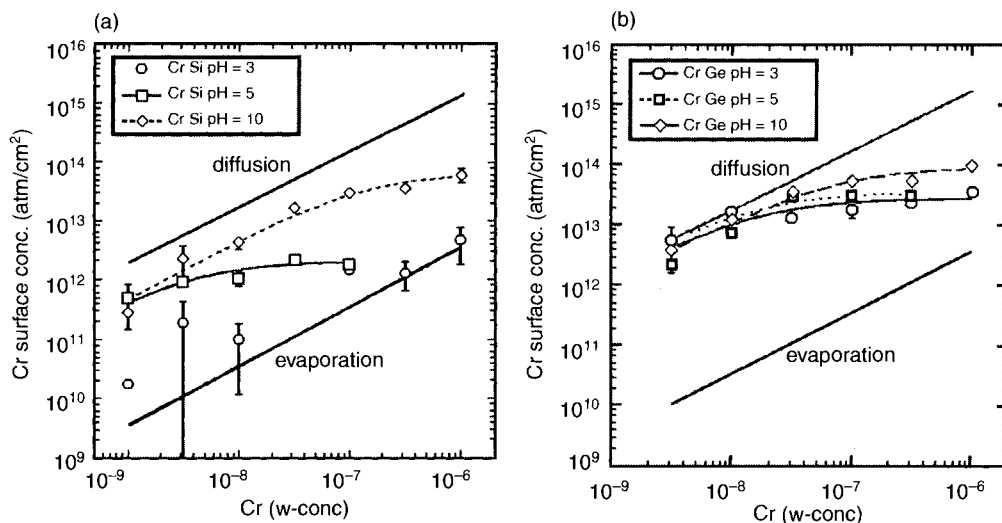
Figure 12.2. Metal deposition behavior on a) Si and b) Ge for Cr atoms from baths at different pH values. The straight lines depict the diffusion and evaporation limits which describe the maximum and minimum levels that can be achieved starting from a bath with a certain ion concentration [45]. Reproduced with permission of ECS – The Electrochemical Society from Sioncke, S., Onsia, B., Struys, K., Rip, J., Vos, R., Meuris, M., Mertens, P., and Theuwis, A., Electrochemical Society Transactions .
