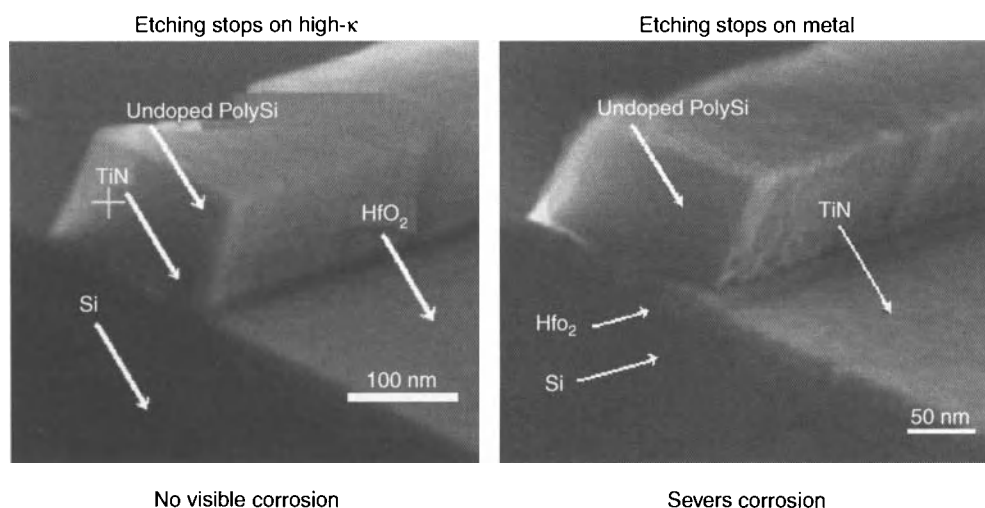
Figure 7.19. Scanning electron microscope images of undoped polySi/TiN metal gate stack after etching a) stopping on the HfO_2 dielectric layer and b) after stopping on the TiN conductor layer [166]. The corrosion is apparent on the TiN layer. Used with permission from Future Fab International .
