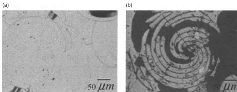
Figure 16.1. Selective attack of 20 wt% nitric acid at the thermal boundaries of a crystalline GST film; a) 10 sec and b) 50 sec [17]. Used with permission of Cheng, H.-Y., Jong, C.-A., Lee, C.-M., and Chin, T.-S. IEEE Transactions on Magnetics . © 2005 IEEE.
