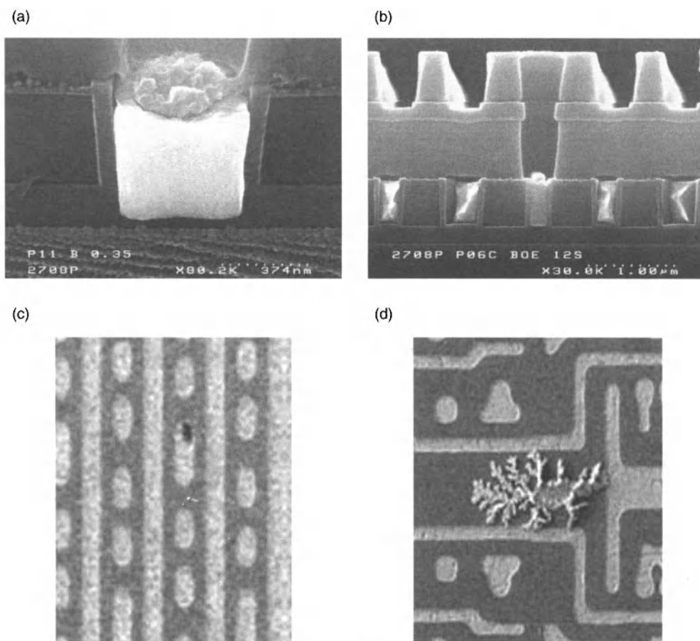
Figure 11.4. Examples of copper corrosion (a) and (b) dual Damascene post-via etch [25], (c) post-copper CMP void [24], and (d) post-copper CMP dendrite [24]. (c) and (d) Reproduced with permission of ECS – The Electrochemical Society from Petitdidier, S. Mellier, M., Guiheux, D., and Juhel, M, ECS Transactions .
