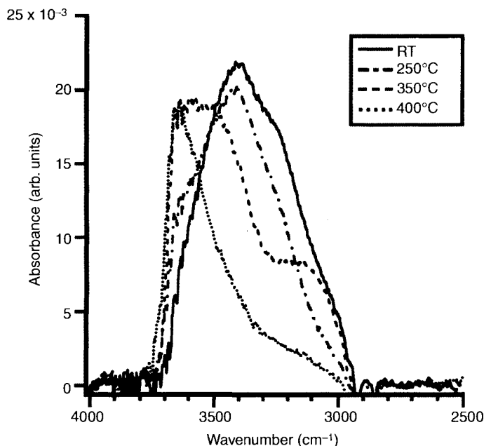
Figure 14.28. Formation of the O-H absorption band measured by FTIR-MIR at the bonding interface of \text{SiO}_2 - \text{SiO}_2 after post-bonding anneal at different temperatures [132]. Reproduced with permission of ECS – The Electrochemical Society from Ventosa, C., Morales, C., Libralesso, L., Fournel, F., Papon, A. M., Lafond, D., Moriceau, H., Penot, J.D., and Rieutord, F., Electrochemical Solid State Letters .
