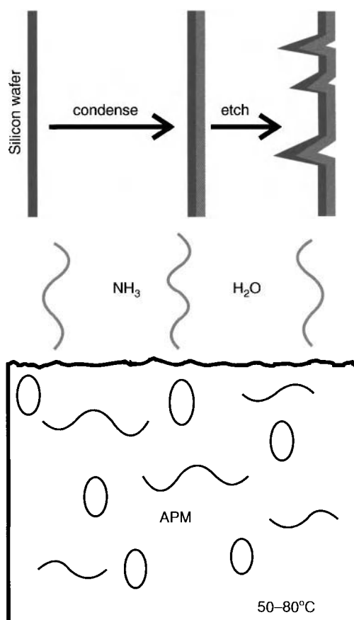
Figure 2.10. Surface roughening mechanism caused by condensation of ammonia. Used with permission of the author.
