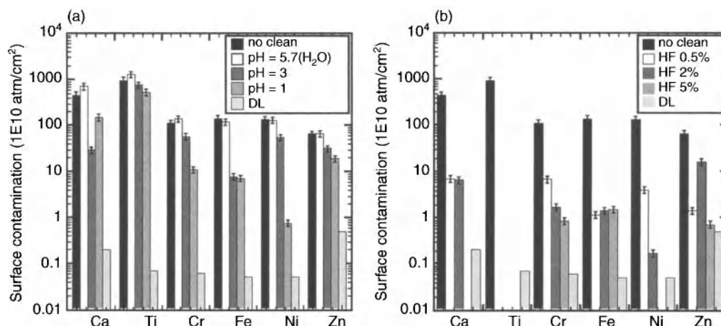
Figure 12.4. Metal contamination after dipping Ge wafers in a) acidified solutions and b) HF-containing solutions. The pH was varied by adding HCl to the bath. Hydrofluoric acid concentrations were varied between 0.5 and 5 wt%. The dip time was 5 minutes [45]. Reproduced with permission of ECS – The Electrochemical Society from Sioncke, S., Onsia, B., Struys, K., Rip, J., Vos, R., Meuris, M., Mertens, P., and Theuwis, A., Electrochemical Society Transactions .
