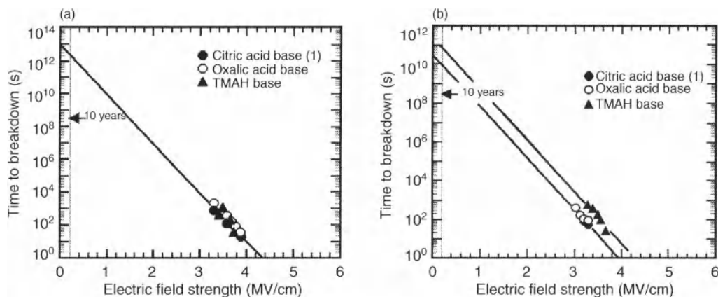
Figure 10.20. Post-CMP cleaning effect on TDDB with a) a BTA CMP passivating step and b) a BTA-free CMP process [93]. Reproduced with permission of ECS – The Electrochemical Society from Yamada, Y., Konishi, N., Noguchi, J., and Jimbo, T., Journal of the Electrochemical Society .
