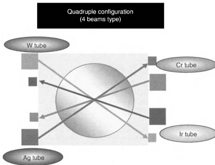
Figure 15.2. Example of a 4 beam TXRF system available from Technos International [17]. Used with permission from Technos International.
