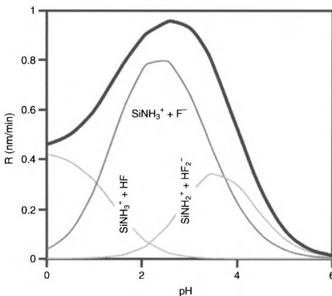
Figure 3.25. Etching of \text{Si}_3\text{N}_4 (in 1 M HF; 25^\circ\text{C} ) consists of three reaction components. The contribution of each component depends on pH [47]. Reproduced with permission of ECS – The Electrochemical Society from Knotter, D. M. and Denteneer, T. J. J., Journal of the Electrochemical Society .
