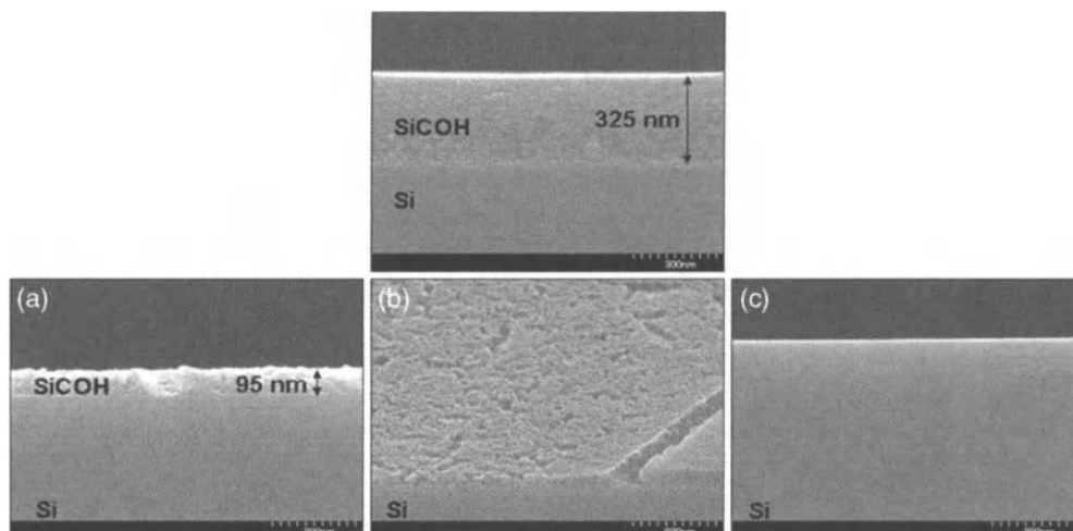
Figure 13.9. Cross section (90°) scanning electron micrograph image of CDO film \kappa = 2.2 (top view); (a) 90° view of film processed in HF, (b) 60° view of same film processed in HF, (c) 90° view of wafer processed using a dry and wet reclaim process [30]. Used with permission of the authors.
