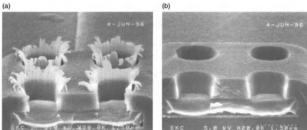
Figure 9.7. Scanning electron microscope image of via field a) showing residue remaining after etching and stripping and b) showing residue removal after cleaning. Courtesy of DuPont/EKC Technology (2010).
