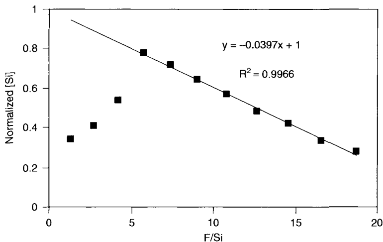
Figure 3.36. Titration of a Si-saturated \text{H}_3\text{PO}_4 bath ( 160^\circ\text{C} ) with \text{NH}_4\text{F} [62]. On the y-axis, the relative concentration of dissolved silica normalized to t = 0 . The x-axis is the added amount of fluoride as a molecular ratio of dissolved silica. Note that the initial deviation from the linear relation is caused by sample preparation. The Si-analysis is performed using inductively coupled plasma/optical emission spectroscopy (ICP/OES) of pre-diluted \text{H}_3\text{PO}_4 solutions that only measures dissolved Si. As the pre-dilution was done with water, a part of the silicates in the saturated \text{H}_3\text{PO}_4 solutions precipitated and, consequently, were not analyzed. Used with permission of the J. Kersten and the author.
