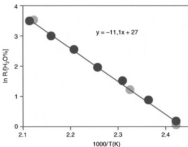
Figure 3.32. Etching rates for (Å/min) LPCVD \text{Si}_3\text{N}_4 (880°C) at various \text{H}_3\text{PO}_4 temperatures determined published by van Gelder and Hauser [55] and recalculated in reference [49]. Reprinted from MICRO Magazine , Copyright 2005, Tom Cheney, Los Angeles, CA.
