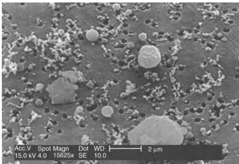
Figure 6.10. Scanning electron micrograph photo of disk filter surface showing collected particles [14]. Hugo M. Ortner, Journal of Environmental Monitoring , 1999, (4), 273–283 – Reproduced by permission of The Royal Society of Chemistry (RSC).
