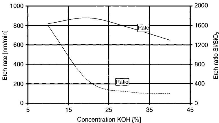
Figure 3.18. Etching rate of silicon <100> in KOH at 70°C [43]. Used with permission of A. A. M. van de Vorst (NXP).
