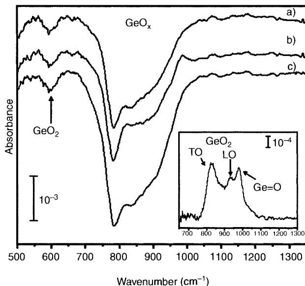
Figure 12.12. Transmission absorption IR spectra of Ge(100) after treatment in: a) DIW, b) DIW followed by 10 sec in H 2 O 2 . All the spectra are referenced to an as-received Ge(100) wafer. The insert shows the oxide region after H 2 O 2 oxidation, using the H 2 O-treated Ge(100) surface [61]. Reprinted with permission from Rivillon, S., Chabal, Y. J., Amy, F., and Kahn, A., Appl. Phys. Lett. , 87(25):3101 (2005). Copyright 2005, American Institute of Physics.
