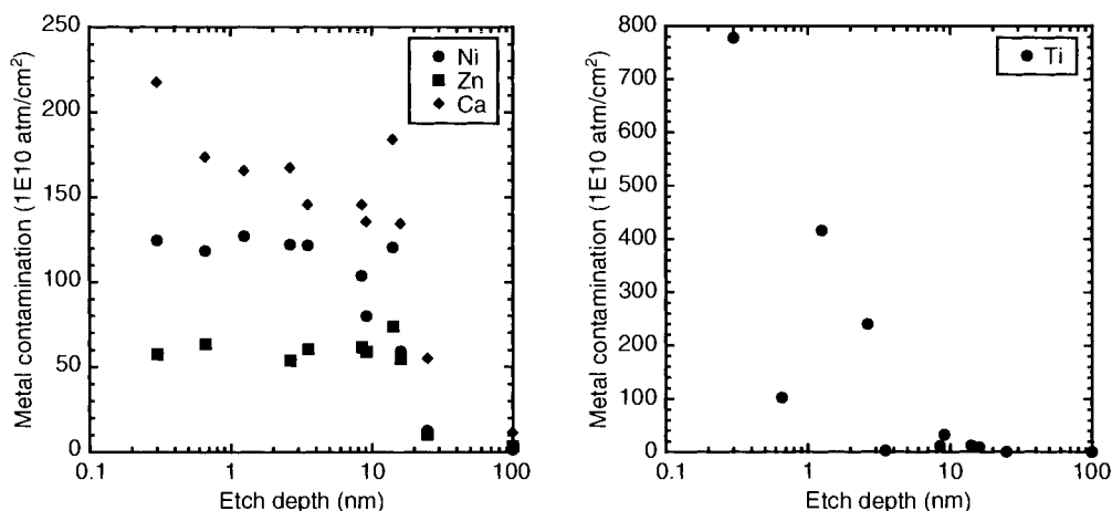
Figure 12.3. Metal contamination after using SC-1 cleaning mixtures as a function of etch depth; a) metal contamination level of Ni, Zn and Ca on the Ge wafer and b) metal contamination level of Ti on the Ge wafer [45]. Reproduced with permission of ECS – The Electrochemical Society from Sioncke, S., Onsia, B., Struys, K., Rip, J., Vos, R., Meuris, M., Mertens, P., and Theuwis, A., Electrochemical Society Transactions .
