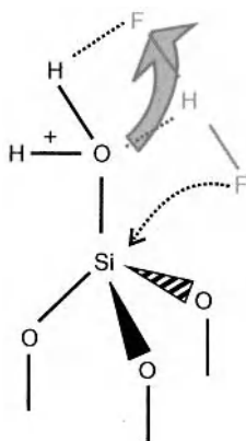
Figure 3.6. Difluoride ( \text{H}_2\text{F}_2 ) reaction with Si showing the substitution mechanism [11]. Reprinted with permission from Knotter, D. M., J. Am. Chem. Soc. , 122(18):4345. Copyright 2000 American Chemical Society.
