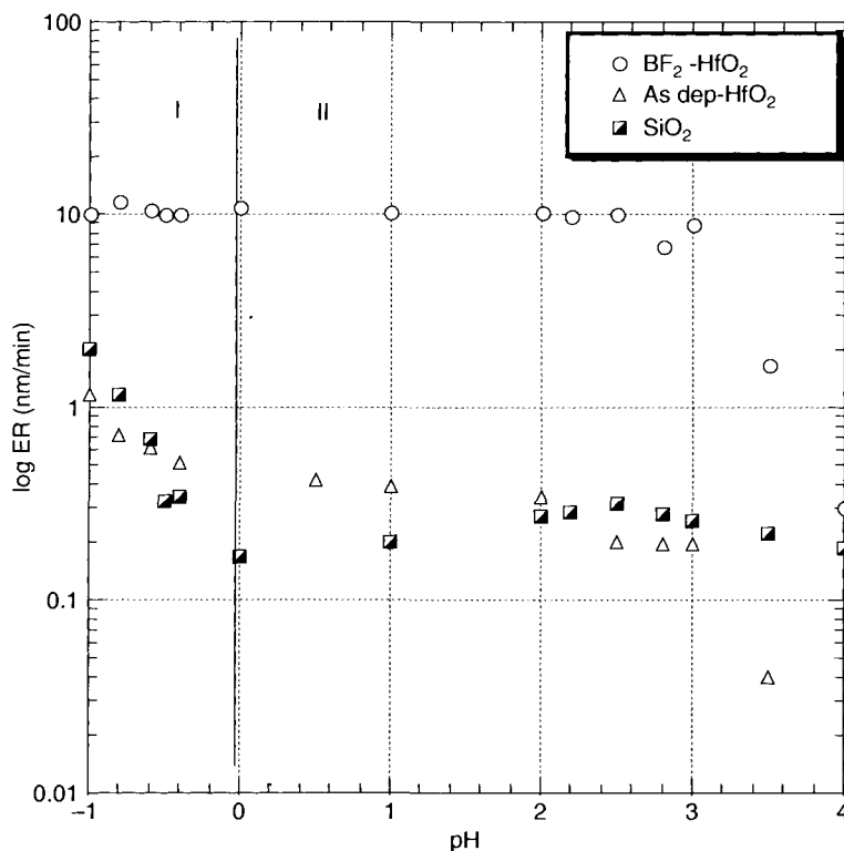
Figure 7.13. Comparison of experimental etching rates (ER), measured as a function of pH; for thermally grown \text{SiO}_2 , as-deposited- \text{HfO}_2 , and \text{BF}_2 -implanted \text{HfO}_2 at 25^\circ\text{C} ; the total fluoride concentration was fixed at 0.05 mole/L; and ER are plotted in a log scale. Used with permission from Vasile Paraschiv.
