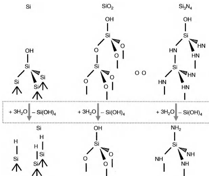
Figure 3.2. Etching of Si-OH in its matrix for Si, \text{SiO}_2 , and \text{Si}_3\text{N}_4 . Prior to the etching process, Si-H has to be oxidized to Si-OH, and the \text{NH}_2 group has to be substituted by OH. Used with permission of the author.
