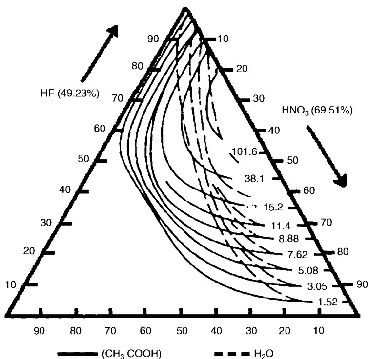
Figure 3.14. Isoetch rate curves ( \mu\text{m}/\text{min} ) of a three-component diagram \text{HNO}_3 (right), HF (left) and acetic acid or water (bottom) [31]. Reproduced with permission of ECS – The Electrochemical Society from Schwartz, B. and Robbins, H., Journal of the Electrochemical Society .
