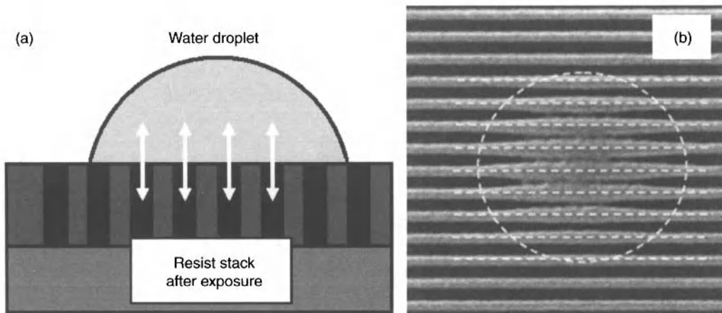
Figure 4.13. Schematic and SEM of a watermark after immersion lithography exposure; a) water droplet remaining on the resist surface after immersion exposure and b) the watermark after develop causing bridging of the 220-nm lines [71]. Reproduced with permission from Wei, Y., "Non-lensing defects and defect reduction for 193i", SPIE Newsroom, 5037:917 (February 10, 2008).
