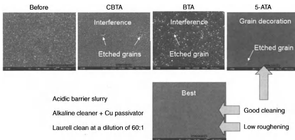
Figure 11.12. Scanning electron micrograph images showing post-CMP cleaning and the impact of the Cu inhibitor used in the cleaner which consisted of water, 2-aminoethanol, TMAH, and ascorbic acid. Some inhibitors did not protect all Cu crystallographic orientations. Compiled and based on data in [46]. Used with permission from the author.
