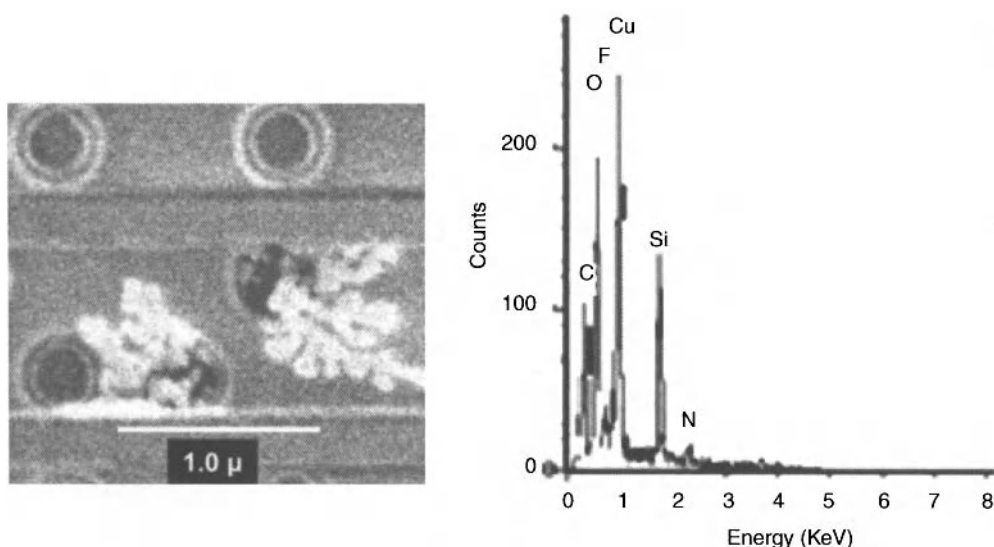
Figure 10.8. Cross-section SEM images of contamination on a low- \kappa via surface and the associated EDS image showing a high concentration of copper on the surface in addition to the carbon and fluorine from the post-etch polymeric residue [53]. Reproduced with permission of ECS – The Electrochemical Society from Mistkawi, N. G., Hussein, M. A., Ziomek-Moroz, M., and Rananavare, S. B., Journal of the Electrochemical Society .
