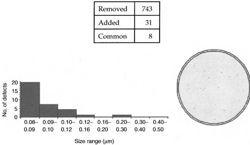
Figure 8.22. Schematic showing defectivity density and size distribution after a full sequence with ESA stripping and SC-1 cleaning [77]. Used with permission of Enrico Bellandi (Numonyx) and Lam Research AG.
