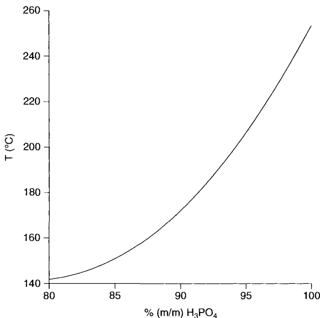
Figure 3.29. Boiling point of water as a function of H_3PO_4 concentration [56]. Reprinted with permission from Brown, E. H. and Whitt, C. D., Industrial and Engineering Chemistry , 44(3):615. Copyright 1952 American Chemical Society.
