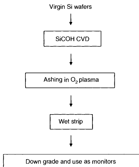
Figure 13.7. Example reclaim process flow for carbon-doped chemical vapor deposited (CVD) low- \kappa films [30]. Used with permission of the authors.
