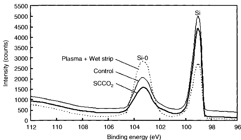
Figure 8.26. The XPS Si 2p spectra for the Si surfaces processed in \text{SCCO}_2 formulation or stripped in \text{O}_2 plasma and SPM [96]. Reproduced with permission of ECS – The Electrochemical Society from Saga, K., Kuniyasu, H., Hattori, T., Korzenski, M. B., Visintin, P. M., and Baum, T. H., ECS Transactions .
