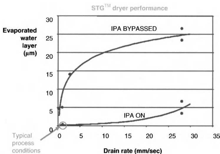
Figure 1.20. Effect of liquid drain rates along with IPA vapor on thickness of water layer. Courtesy of FSI International, Inc.
