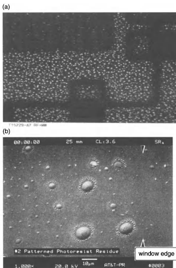
Figure 8.10. Examples of implant residues after stripping and cleaning. (a) Micrograph of post- O_2 plasma resist strip implant residue. Used with permission of Novellus Systems. (b) SEM of post-plasma resist strip and SPM clean arsenic implant residue [18]. Used with permission from Material Research Society, reprinted from Draper, C. W., Pearce, C. W., Glick, J. T., Gordon, M., Olness, G. E., Bernasek, S. L., Journal of Material Research , Vol. 12, Pittsburg, PA, (1997) page 2799.
