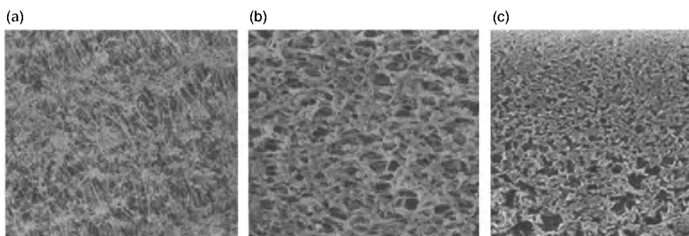
Figure 6.13. Membrane materials: (a) polytetrafluoroethylene, (b) polyvinylidene difluoride, and (c) asymmetric nylon 6,6. Used with permission from Pall Corporation.
